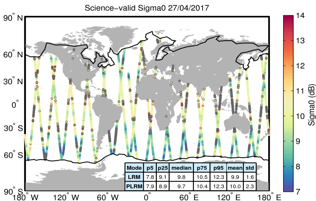
Figure 27. Geographical distribution of science-valid sigma0 data over oceans and lakes for 27/04/2017. The statistical values shown in the table refer to the sigma0 in dB and are calculated separately for LRM and PLRM regions. The black lines mark the outer limit of the Arctic and Antarctic polar polygons. Gray circles denote records that have been rejected based on the editing criteria described in Table 4.
