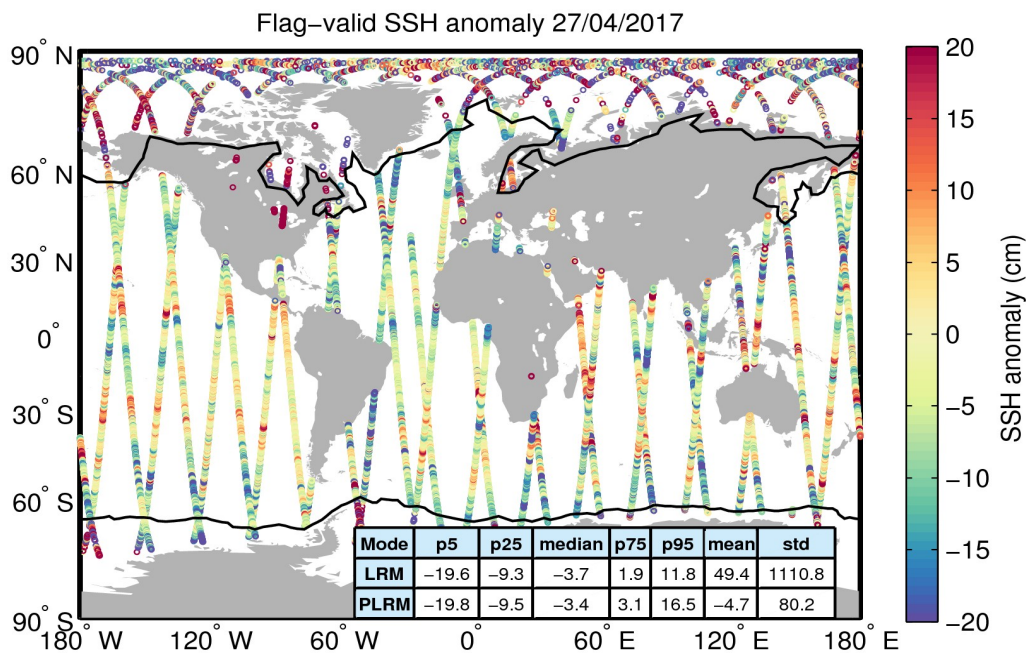
Figure 5. Geographical distribution of flag-valid 1-Hz SSH anomaly data over oceans and lakes for 27/04/2017. The statistical values shown in the table refer to the SSH anomaly in cm and are calculated separately for LRM and PLRM regions. Measurements taken over polar polygons have been excluded from the computation of the statistical values. The black lines mark the outer limit of the Arctic and Antarctic polar polygons.
