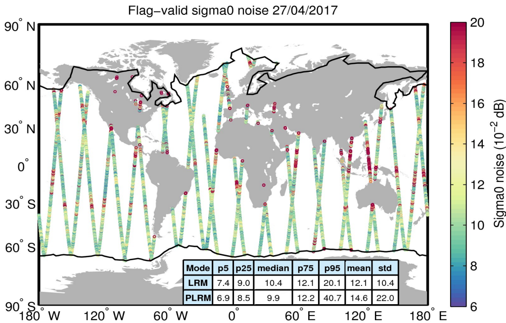
Figure 26. Geographical distribution of flag-valid 20-Hz sigma0 measurement noise over oceans and lakes for 27/04/2017. The statistical values shown in the table refer to the sigma0 noise and are calculated separately for LRM and PLRM regions. Measurements taken over polar polygons have been excluded from the computation of the statistical values. The black lines mark the outer limit of the Arctic and Antarctic polar polygons.
