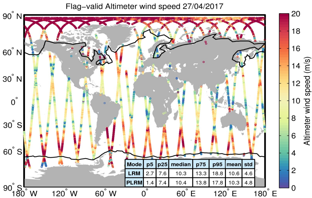
Figure 31. Geographical distribution of flag-valid wind data over oceans and lakes for 27/04/2017. The statistical values shown in the table refer to the wind in m/s and are calculated separately for LRM and PLRM regions. Measurements taken over polar polygons have been excluded from the computation of the statistical values. The black lines mark the outer limit of the Arctic and Antarctic polar polygons.
