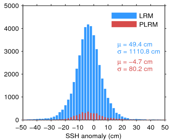
Figure 7. Histogram of flag-valid SSH anomaly over oceans and lakes for LRM (blue) and PLRM (red) for 27/04/2017. The mean ( \mu ) and standard deviation ( \sigma ) are also shown. Note that values outside [-50 50] cm are excluded from the histogram for the sake of readability but not from the computation of \mu and \sigma .
