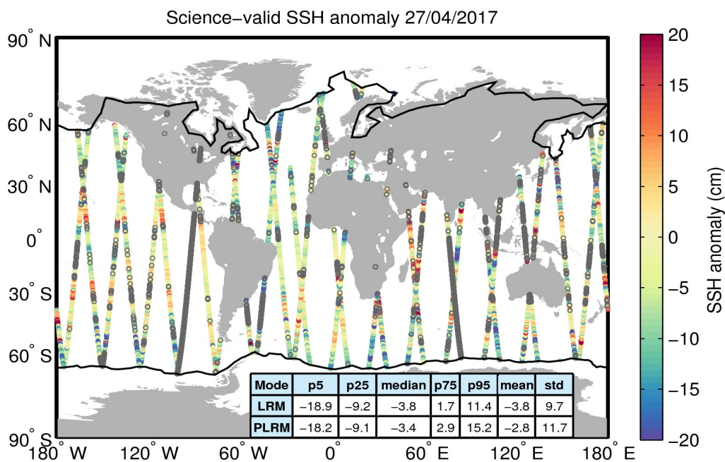
Figure 10. Geographical distribution of science-valid SSH anomaly data over oceans and lakes for 27/04/2017. The statistical values shown in the table refer to the SSH anomaly in cm and are calculated separately for LRM and PLRM regions. The black lines mark the outer limit of the Arctic and Antarctic polar polygons. Gray circles denote records that have been rejected based on the editing criteria described in Table 2.
