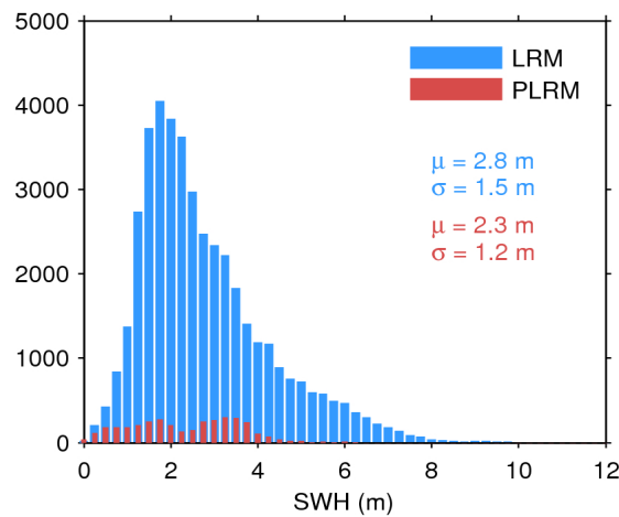
Figure 20. Histogram of science-valid SWH over oceans and lakes for LRM (blue) and PLRM (red) for 27/04/2017. The mean ( \mu ) and standard deviation ( \sigma ) are also shown. Note that values larger than 12 m are excluded from the histogram for the sake of readability but not from the computation of \mu and \sigma .
