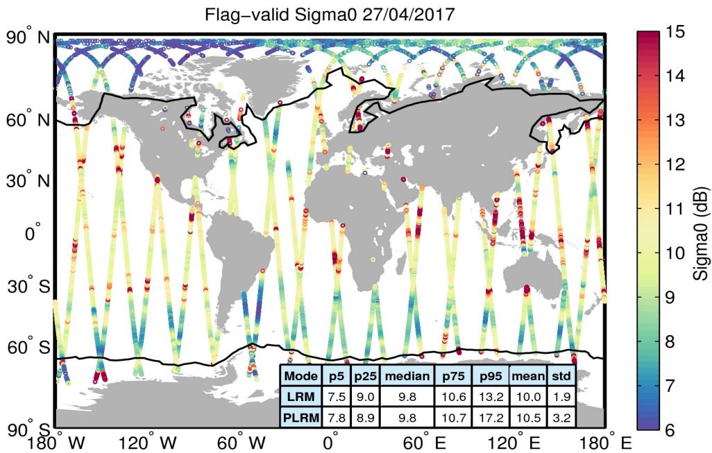
Figure 23. Geographical distribution of flag-valid sigma0 data over oceans and lakes for 27/04/2017. The statistical values shown in the table refer to the sigma0 in dB and are calculated separately for LRM and PLRM regions. Measurements taken over polar polygons have been excluded from the computation of the statistical values. The black lines mark the outer limit of the Arctic and Antarctic polar polygons.
