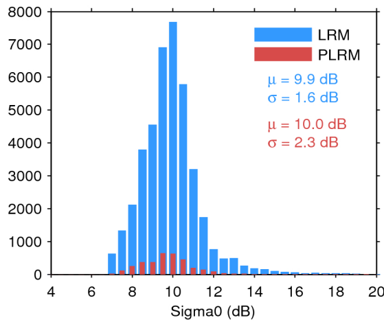
Figure 28. Histogram of science-valid sigma0 over oceans and lakes for LRM (blue) and PLRM (red) for 27/04/2017. The mean ( \mu ) and standard deviation ( \sigma ) are also shown. Note that values outside [4 20] dB are excluded from the histogram for the sake of readability but not from the computation of \mu and \sigma .
