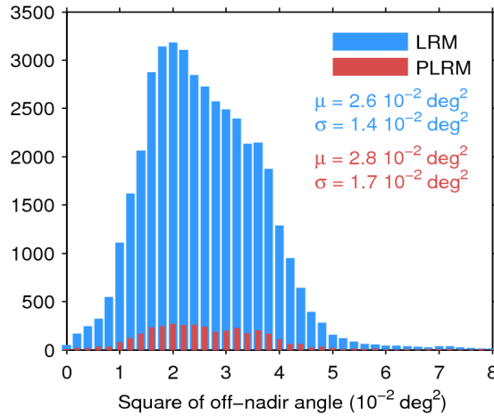
Figure 39. Histogram of flag-valid mispointing over oceans and lakes for LRM (blue) and PLRM (red) for 27/04/2017. Only positive values have been considered. The mean ( \mu ) and standard deviation ( \sigma ) are also shown. Note that values larger than 8 \cdot 10^{-2} \text{ deg}^2 are excluded from the histogram for the sake of readability but not from the computation of \mu and \sigma .
