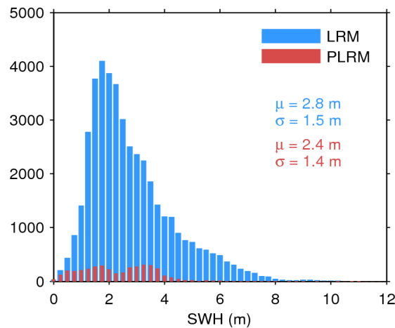
Figure 17. Histogram of flag-valid SWH over oceans and lakes for LRM (blue) and PLRM (red) for 27/04/2017. The mean ( \mu ) and standard deviation ( \sigma ) are also shown. Note that values larger than 12 m are excluded from the histogram for the sake of readability but not from the computation of \mu and \sigma .
