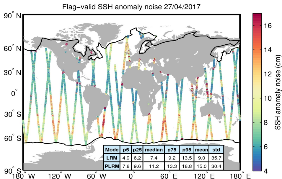
Figure 8. Geographical distribution of flag-valid 20-Hz SSH anomaly measurement noise over oceans and lakes for 27/04/2017. The statistical values shown in the table refer to the SSH anomaly noise and are calculated separately for LRM and PLRM regions. Measurements taken over polar polygons have been excluded from the computation of the statistical values. The black lines mark the outer limit of the Arctic and Antarctic polar polygons.
