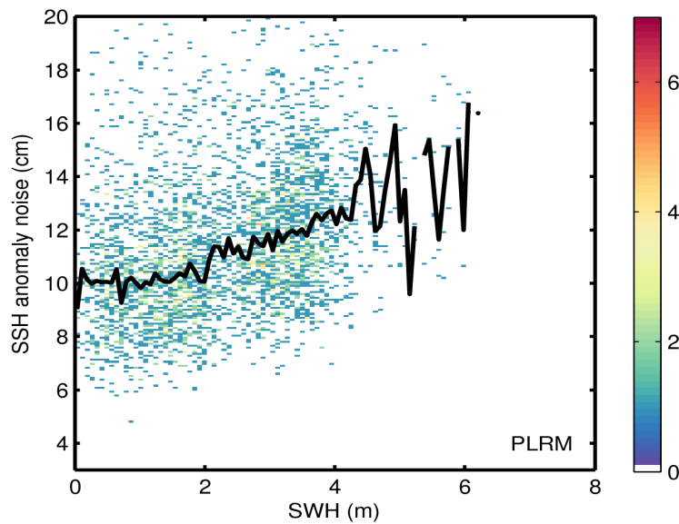
Figure 9. 2D histogram showing flag-valid SSH anomaly noise as a function of SWH for LRM (top) and PLRM (bottom) for 27/04/2017. The black line denotes the median SSH anomaly noise as a function of SWH.
