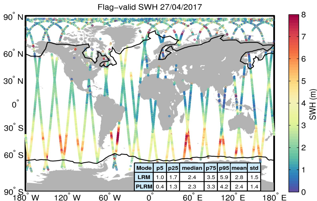
Figure 15. Geographical distribution of flag-valid SWH data over oceans and lakes for 27/04/2017. The statistical values shown in the table refer to the SWH in m and are calculated separately for LRM and PLRM regions. Measurements taken over polar polygons have been excluded from the computation of the statistical values. The black lines mark the outer limit of the Arctic and Antarctic polar polygons.
