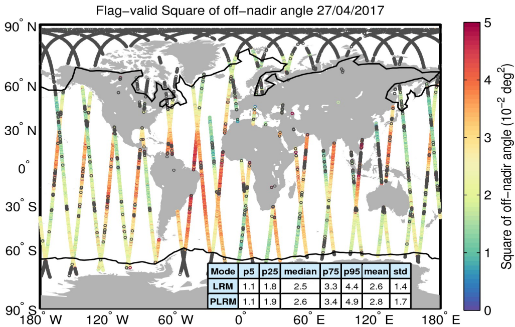
Figure 37. Geographical distribution of flag-valid mispointing data over oceans and lakes for 27/04/2017. The statistical values shown in the table refer to the mispointing in 10^{-2} deg 2 and are calculated separately for LRM and PLRM regions. Measurements taken over polar polygons have been excluded from the computation of the statistical values. The black lines mark the outer limit of the Arctic and Antarctic polar polygons. Gray circles denote negative values.
