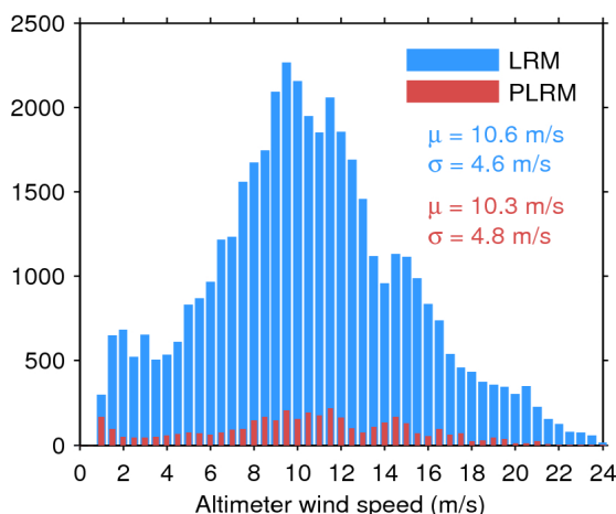
Figure 33. Histogram of flag-valid wind over oceans and lakes for LRM (blue) and PLRM (red) for 27/04/2017. The mean ( \mu ) and standard deviation ( \sigma ) are also shown. Note that values larger than 24 m/s are excluded from the histogram for the sake of readability but not from the computation of \mu and \sigma .
