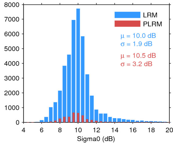
Figure 25. Histogram of flag-valid sigma0 over oceans and lakes for LRM (blue) and PLRM (red) for 27/04/2017. The mean ( \mu ) and standard deviation ( \sigma ) are also shown. Note that values outside [4 20] dB are excluded from the histogram for the sake of readability but not from the computation of \mu and \sigma .
