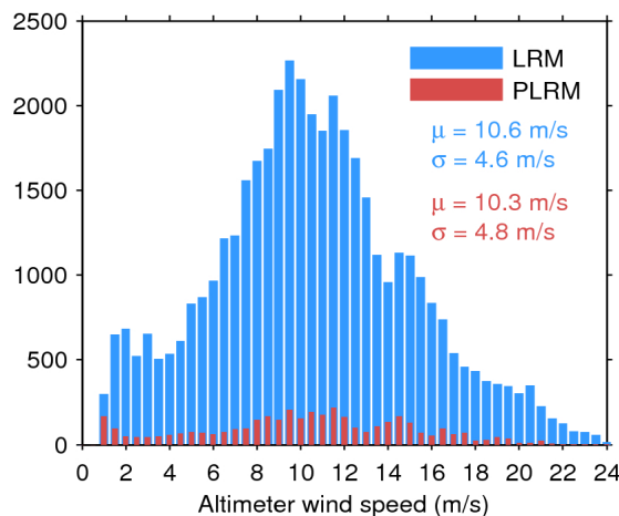
Figure 35. Histogram of science-valid wind over oceans and lakes for LRM (blue) and PLRM (red) for 27/04/2017. The mean ( \mu ) and standard deviation ( \sigma ) are also shown. Note that values larger than 24 m/s are excluded from the histogram for the sake of readability but not from the computation of \mu and \sigma .
