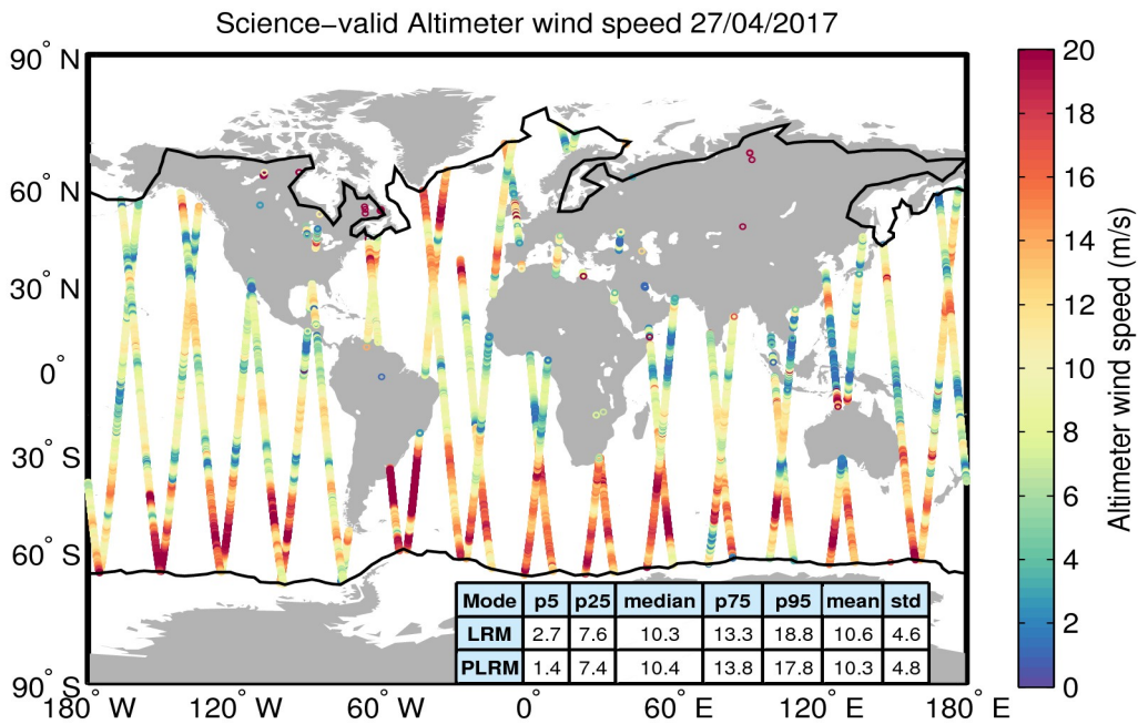
Figure 34. Geographical distribution of science-valid wind data over oceans and lakes for 27/04/2017. The statistical values shown in the table refer to the wind in m/s and are calculated separately for LRM and PLRM regions. The black lines mark the outer limit of the Arctic and Antarctic polar polygons. Gray circles denote records that have been rejected based on the editing criteria described in Table 5.
