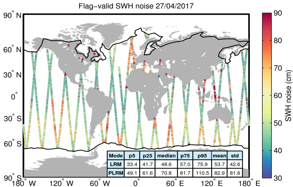
Figure 18. Geographical distribution of flag-valid 20-Hz SWH measurement noise over oceans and lakes for 27/04/2017. The statistical values shown in the table refer to the SWH noise and are calculated separately for LRM and PLRM regions. Measurements taken over polar polygons have been excluded from the computation of the statistical values. The black lines mark the outer limit of the Arctic and Antarctic polar polygons.
