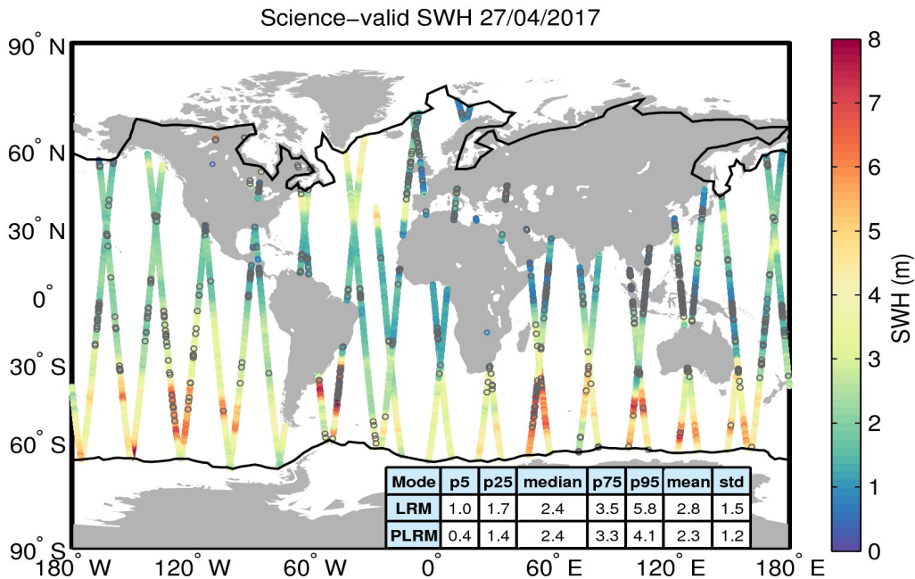
Figure 19. Geographical distribution of science-valid SWH data over oceans and lakes for 27/04/2017. The statistical values shown in the table refer to the SWH in m and are calculated separately for LRM and PLRM regions. The black lines mark the outer limit of the Arctic and Antarctic polar polygons. Gray circles denote records that have been rejected based on the editing criteria described in Table 3.
