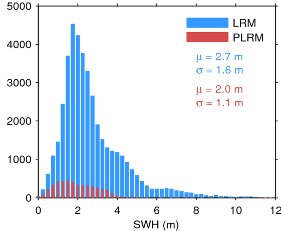
Figure 17. Histogram of flag-valid SWH over oceans and lakes for LRM (blue) and PLRM (red) for 26/04/2017. The mean ( \mu ) and standard deviation ( \sigma ) are also shown. Note that values larger than 12 m are excluded from the histogram for the sake of readability but not from the computation of \mu and \sigma .
