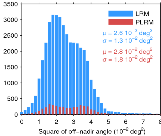
Figure 39. Histogram of flag-valid mispointing over oceans and lakes for LRM (blue) and PLRM (red) for 26/04/2017. Only positive values have been considered. The mean ( \mu ) and standard deviation ( \sigma ) are also shown. Note that values larger than 8 \cdot 10^{-2} \text{ deg}^2 are excluded from the histogram for the sake of readability but not from the computation of \mu and \sigma .
