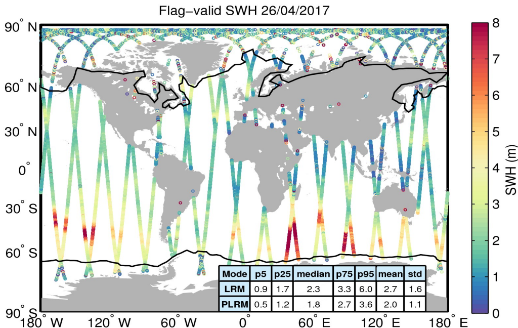
Figure 15. Geographical distribution of flag-valid SWH data over oceans and lakes for 26/04/2017. The statistical values shown in the table refer to the SWH in m and are calculated separately for LRM and PLRM regions. Measurements taken over polar polygons have been excluded from the computation of the statistical values. The black lines mark the outer limit of the Arctic and Antarctic polar polygons.
