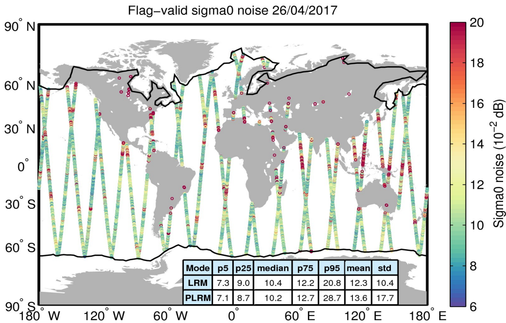
Figure 26. Geographical distribution of flag-valid 20-Hz sigma0 measurement noise over oceans and lakes for 26/04/2017. The statistical values shown in the table refer to the sigma0 noise and are calculated separately for LRM and PLRM regions. Measurements taken over polar polygons have been excluded from the computation of the statistical values. The black lines mark the outer limit of the Arctic and Antarctic polar polygons.
