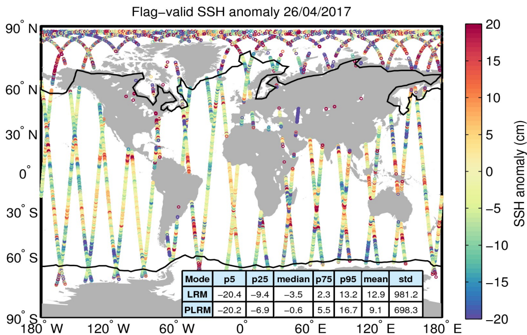
Figure 5. Geographical distribution of flag-valid 1-Hz SSH anomaly data over oceans and lakes for 26/04/2017. The statistical values shown in the table refer to the SSH anomaly in cm and are calculated separately for LRM and PLRM regions. Measurements taken over polar polygons have been excluded from the computation of the statistical values. The black lines mark the outer limit of the Arctic and Antarctic polar polygons.
