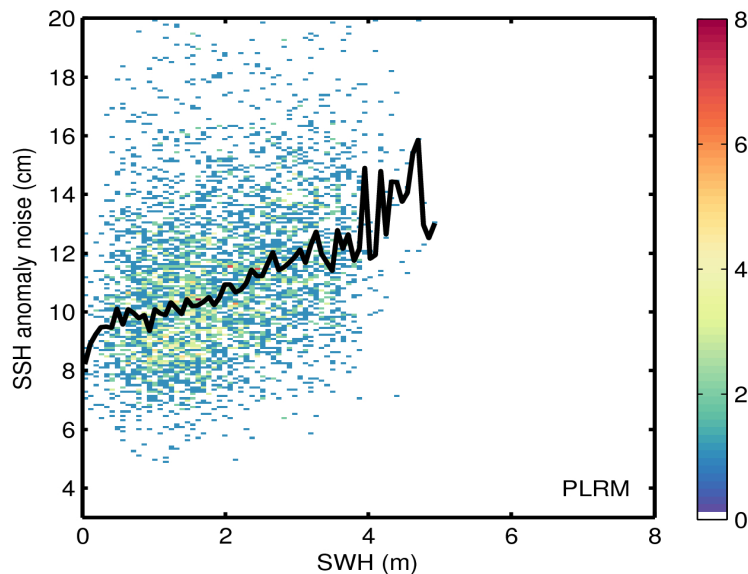
Figure 9. 2D histogram showing flag-valid SSH anomaly noise as a function of SWH for LRM (top) and PLRM (bottom) for 26/04/2017. The black line denotes the median SSH anomaly noise as a function of SWH.
