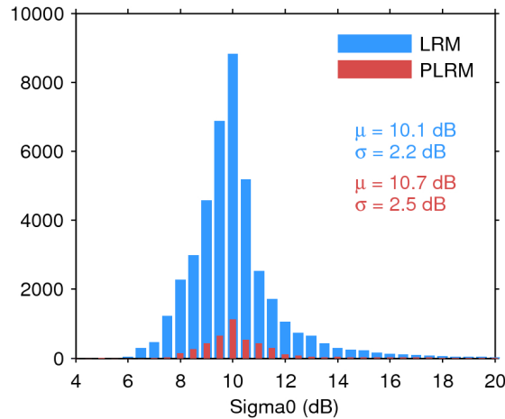
Figure 25. Histogram of flag-valid sigma0 over oceans and lakes for LRM (blue) and PLRM (red) for 26/04/2017. The mean ( \mu ) and standard deviation ( \sigma ) are also shown. Note that values outside [4 20] dB are excluded from the histogram for the sake of readability but not from the computation of \mu and \sigma .
