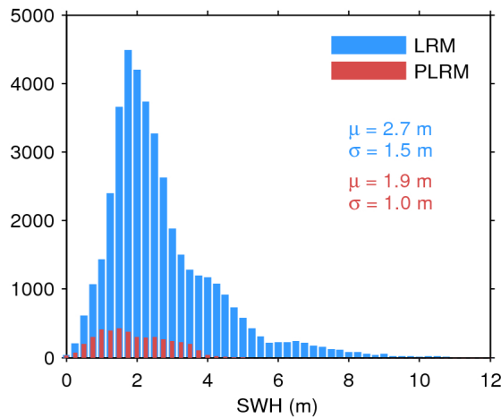
Figure 20. Histogram of science-valid SWH over oceans and lakes for LRM (blue) and PLRM (red) for 26/04/2017. The mean ( \mu ) and standard deviation ( \sigma ) are also shown. Note that values larger than 12 m are excluded from the histogram for the sake of readability but not from the computation of \mu and \sigma .
