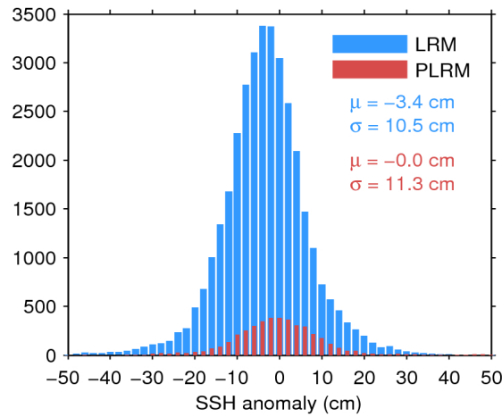
Figure 11. Histogram of science-valid SSH anomaly over oceans and lakes for LRM (blue) and PLRM (red) for 26/04/2017. The mean ( \mu ) and standard deviation ( \sigma ) are also shown. Note that values outside [-50 50] cm are excluded from the histogram for the sake of readability but not from the computation of \mu and \sigma .
