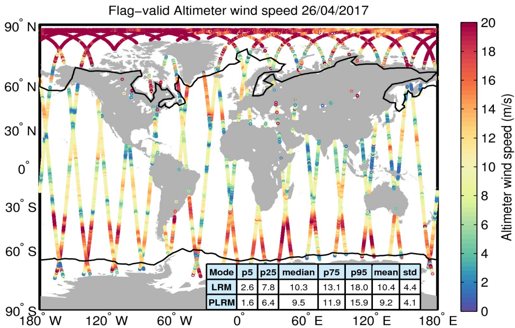
Figure 31. Geographical distribution of flag-valid wind data over oceans and lakes for 26/04/2017. The statistical values shown in the table refer to the wind in m/s and are calculated separately for LRM and PLRM regions. Measurements taken over polar polygons have been excluded from the computation of the statistical values. The black lines mark the outer limit of the Arctic and Antarctic polar polygons.
