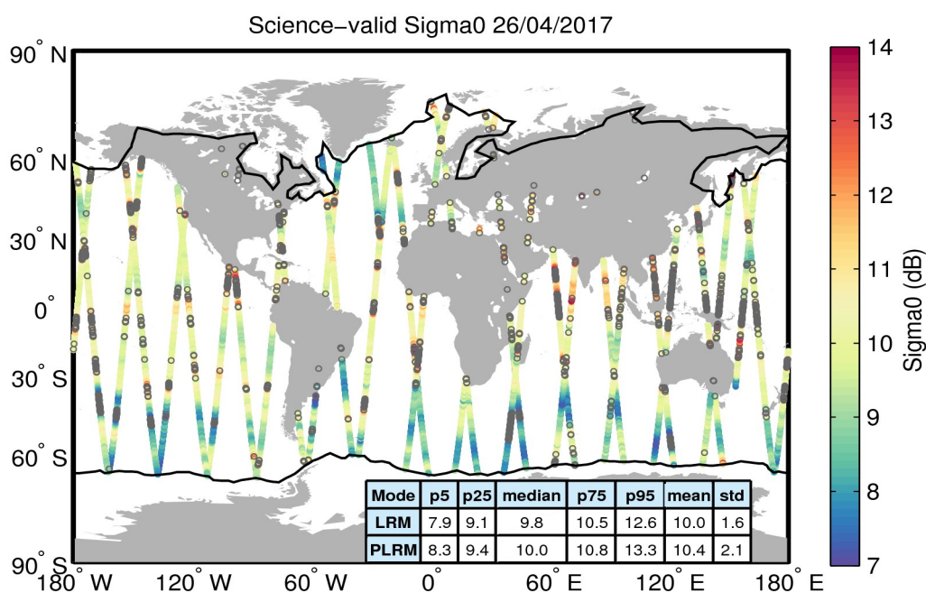
Figure 27. Geographical distribution of science-valid sigma0 data over oceans and lakes for 26/04/2017. The statistical values shown in the table refer to the sigma0 in dB and are calculated separately for LRM and PLRM regions. The black lines mark the outer limit of the Arctic and Antarctic polar polygons. Gray circles denote records that have been rejected based on the editing criteria described in Table 4.
