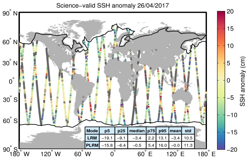
Figure 10. Geographical distribution of science-valid SSH anomaly data over oceans and lakes for 26/04/2017. The statistical values shown in the table refer to the SSH anomaly in cm and are calculated separately for LRM and PLRM regions. The black lines mark the outer limit of the Arctic and Antarctic polar polygons. Gray circles denote records that have been rejected based on the editing criteria described in Table 2.
