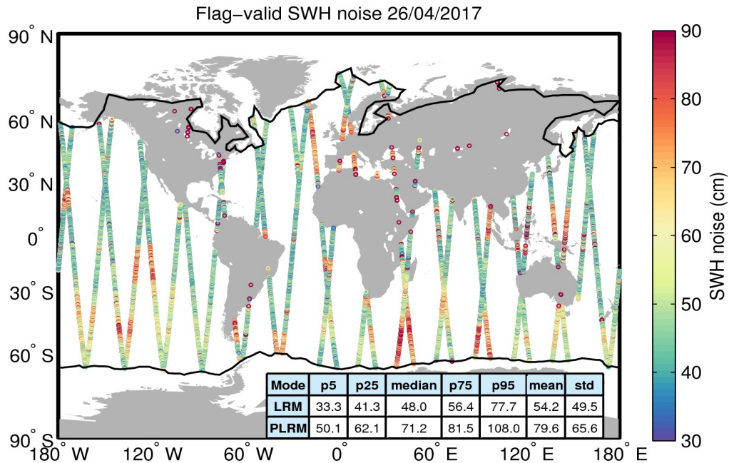
Figure 18. Geographical distribution of flag-valid 20-Hz SWH measurement noise over oceans and lakes for 26/04/2017. The statistical values shown in the table refer to the SWH noise and are calculated separately for LRM and PLRM regions. Measurements taken over polar polygons have been excluded from the computation of the statistical values. The black lines mark the outer limit of the Arctic and Antarctic polar polygons.
