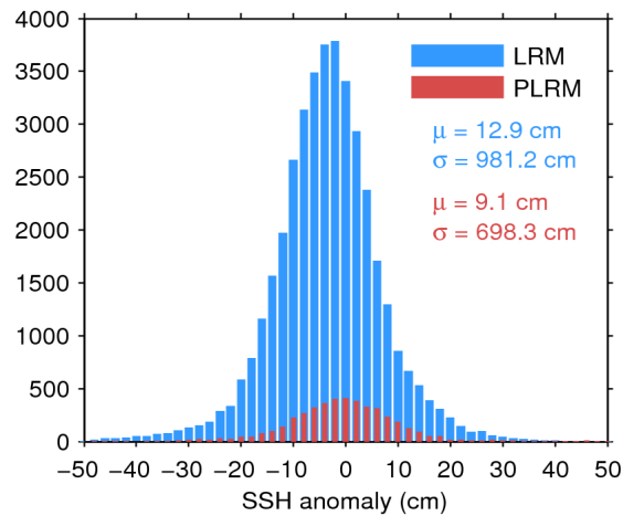
Figure 7. Histogram of flag-valid SSH anomaly over oceans and lakes for LRM (blue) and PLRM (red) for 26/04/2017. The mean ( \mu ) and standard deviation ( \sigma ) are also shown. Note that values outside [-50 50] cm are excluded from the histogram for the sake of readability but not from the computation of \mu and \sigma .
