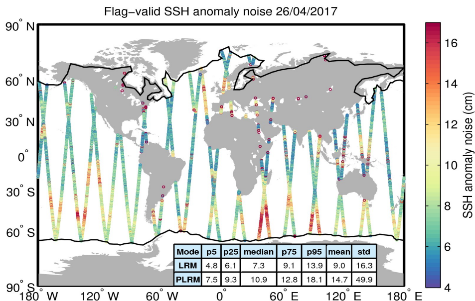
Figure 8. Geographical distribution of flag-valid 20-Hz SSH anomaly measurement noise over oceans and lakes for 26/04/2017. The statistical values shown in the table refer to the SSH anomaly noise and are calculated separately for LRM and PLRM regions. Measurements taken over polar polygons have been excluded from the computation of the statistical values. The black lines mark the outer limit of the Arctic and Antarctic polar polygons.
