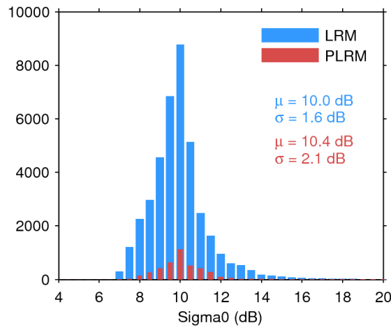
Figure 28. Histogram of science-valid sigma0 over oceans and lakes for LRM (blue) and PLRM (red) for 26/04/2017. The mean ( \mu ) and standard deviation ( \sigma ) are also shown. Note that values outside [4 20] dB are excluded from the histogram for the sake of readability but not from the computation of \mu and \sigma .
