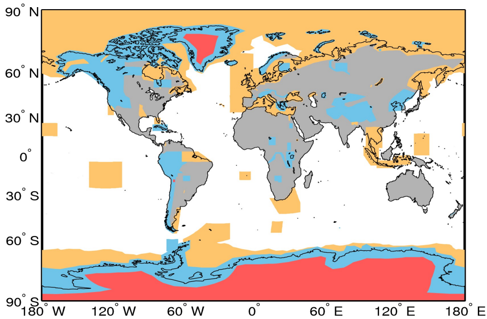
Figure A1. Extent of the regions defining the geographical mode mask for 26/04/2017. The regions where SAR, and SARIn are operated are denoted by the orange and blue polygons, respectively. LRM is operated over areas of the continental ice sheets (red polygons) and over oceans and land not covered by other modes.
