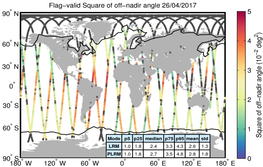
Figure 37. Geographical distribution of flag-valid mispointing data over oceans and lakes for 26/04/2017. The statistical values shown in the table refer to the mispointing in 10^{-2} deg 2 and are calculated separately for LRM and PLRM regions. Measurements taken over polar polygons have been excluded from the computation of the statistical values. The black lines mark the outer limit of the Arctic and Antarctic polar polygons. Gray circles denote negative values.
