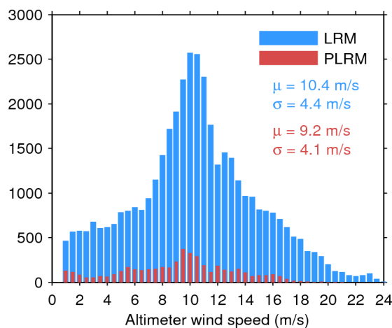
Figure 33. Histogram of flag-valid wind over oceans and lakes for LRM (blue) and PLRM (red) for 26/04/2017. The mean ( \mu ) and standard deviation ( \sigma ) are also shown. Note that values larger than 24 m/s are excluded from the histogram for the sake of readability but not from the computation of \mu and \sigma .
