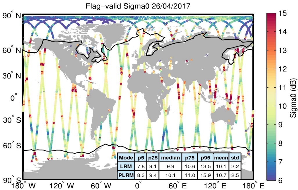
Figure 23. Geographical distribution of flag-valid sigma0 data over oceans and lakes for 26/04/2017. The statistical values shown in the table refer to the sigma0 in dB and are calculated separately for LRM and PLRM regions. Measurements taken over polar polygons have been excluded from the computation of the statistical values. The black lines mark the outer limit of the Arctic and Antarctic polar polygons.
