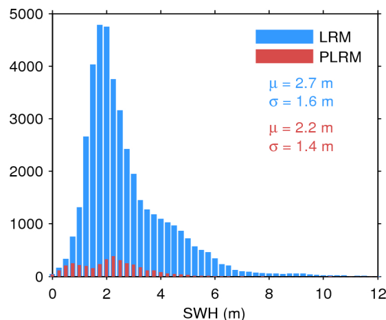
Figure 17. Histogram of flag-valid SWH over oceans and lakes for LRM (blue) and PLRM (red) for 25/04/2017. The mean ( \mu ) and standard deviation ( \sigma ) are also shown. Note that values larger than 12 m are excluded from the histogram for the sake of readability but not from the computation of \mu and \sigma .
