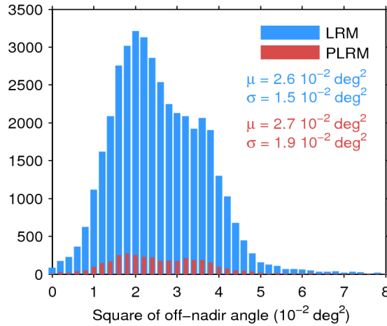
Figure 39. Histogram of flag-valid mispointing over oceans and lakes for LRM (blue) and PLRM (red) for 25/04/2017. Only positive values have been considered. The mean ( \mu ) and standard deviation ( \sigma ) are also shown. Note that values larger than 8 \cdot 10^{-2} \text{ deg}^2 are excluded from the histogram for the sake of readability but not from the computation of \mu and \sigma .
