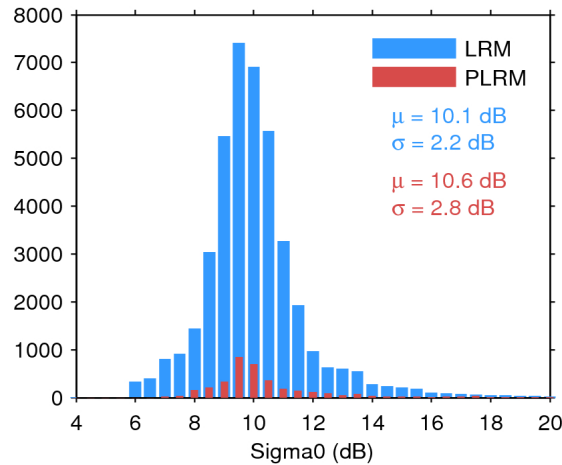
Figure 25. Histogram of flag-valid sigma0 over oceans and lakes for LRM (blue) and PLRM (red) for 25/04/2017. The mean ( \mu ) and standard deviation ( \sigma ) are also shown. Note that values outside [4 20] dB are excluded from the histogram for the sake of readability but not from the computation of \mu and \sigma .
