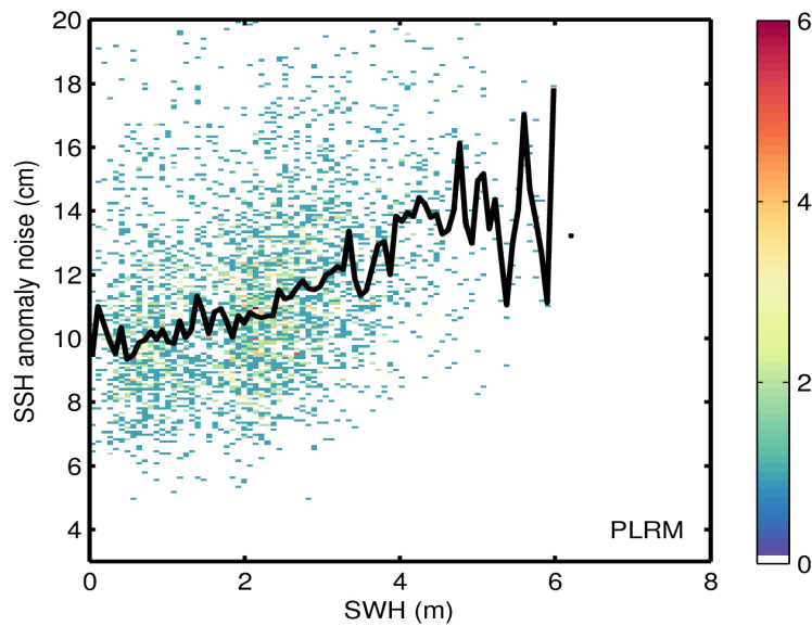
Figure 9. 2D histogram showing flag-valid SSH anomaly noise as a function of SWH for LRM (top) and PLRM (bottom) for 25/04/2017. The black line denotes the median SSH anomaly noise as a function of SWH.
