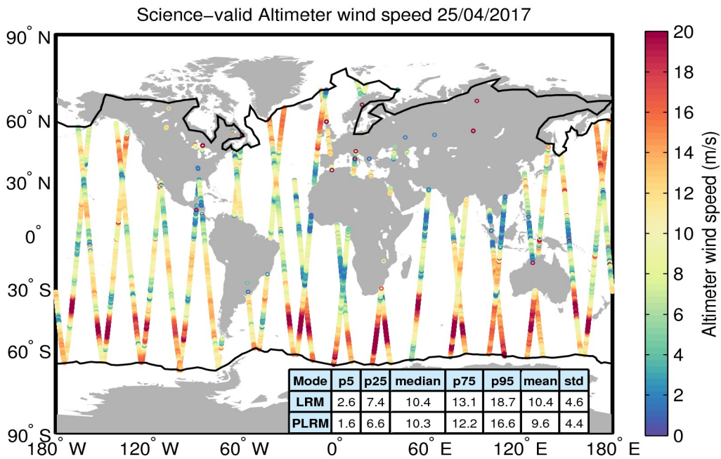
Figure 34. Geographical distribution of science-valid wind data over oceans and lakes for 25/04/2017. The statistical values shown in the table refer to the wind in m/s and are calculated separately for LRM and PLRM regions. The black lines mark the outer limit of the Arctic and Antarctic polar polygons. Gray circles denote records that have been rejected based on the editing criteria described in Table 5.
