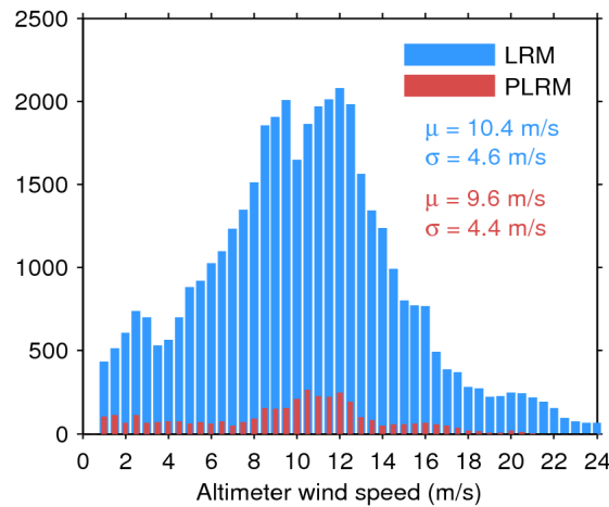
Figure 33. Histogram of flag-valid wind over oceans and lakes for LRM (blue) and PLRM (red) for 25/04/2017. The mean ( \mu ) and standard deviation ( \sigma ) are also shown. Note that values larger than 24 m/s are excluded from the histogram for the sake of readability but not from the computation of \mu and \sigma .
