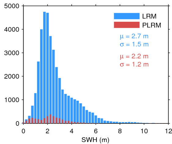
Figure 20. Histogram of science-valid SWH over oceans and lakes for LRM (blue) and PLRM (red) for 25/04/2017. The mean ( \mu ) and standard deviation ( \sigma ) are also shown. Note that values larger than 12 m are excluded from the histogram for the sake of readability but not from the computation of \mu and \sigma .
