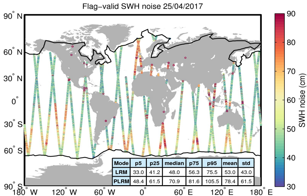
Figure 18. Geographical distribution of flag-valid 20-Hz SWH measurement noise over oceans and lakes for 25/04/2017. The statistical values shown in the table refer to the SWH noise and are calculated separately for LRM and PLRM regions. Measurements taken over polar polygons have been excluded from the computation of the statistical values. The black lines mark the outer limit of the Arctic and Antarctic polar polygons.
