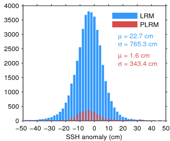
Figure 7. Histogram of flag-valid SSH anomaly over oceans and lakes for LRM (blue) and PLRM (red) for 25/04/2017. The mean ( \mu ) and standard deviation ( \sigma ) are also shown. Note that values outside [-50 50] cm are excluded from the histogram for the sake of readability but not from the computation of \mu and \sigma .
