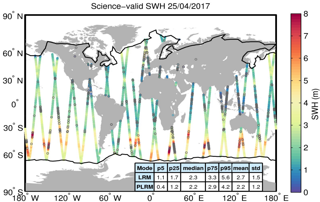
Figure 19. Geographical distribution of science-valid SWH data over oceans and lakes for 25/04/2017. The statistical values shown in the table refer to the SWH in m and are calculated separately for LRM and PLRM regions. The black lines mark the outer limit of the Arctic and Antarctic polar polygons. Gray circles denote records that have been rejected based on the editing criteria described in Table 3.
