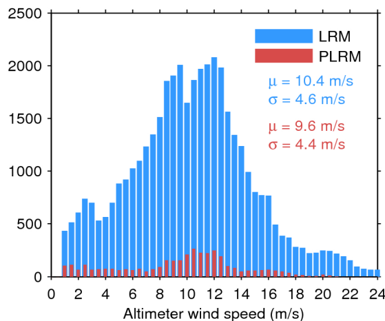
Figure 35. Histogram of science-valid wind over oceans and lakes for LRM (blue) and PLRM (red) for 25/04/2017. The mean ( \mu ) and standard deviation ( \sigma ) are also shown. Note that values larger than 24 m/s are excluded from the histogram for the sake of readability but not from the computation of \mu and \sigma .
