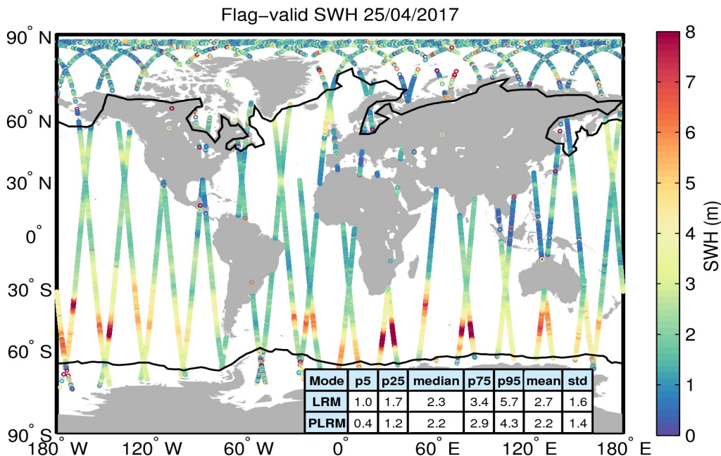
Figure 15. Geographical distribution of flag-valid SWH data over oceans and lakes for 25/04/2017. The statistical values shown in the table refer to the SWH in m and are calculated separately for LRM and PLRM regions. Measurements taken over polar polygons have been excluded from the computation of the statistical values. The black lines mark the outer limit of the Arctic and Antarctic polar polygons.
