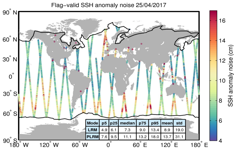
Figure 8. Geographical distribution of flag-valid 20-Hz SSH anomaly measurement noise over oceans and lakes for 25/04/2017. The statistical values shown in the table refer to the SSH anomaly noise and are calculated separately for LRM and PLRM regions. Measurements taken over polar polygons have been excluded from the computation of the statistical values. The black lines mark the outer limit of the Arctic and Antarctic polar polygons.
