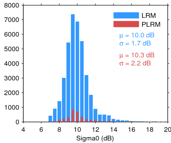
Figure 28. Histogram of science-valid sigma0 over oceans and lakes for LRM (blue) and PLRM (red) for 25/04/2017. The mean ( \mu ) and standard deviation ( \sigma ) are also shown. Note that values outside [4 20] dB are excluded from the histogram for the sake of readability but not from the computation of \mu and \sigma .
