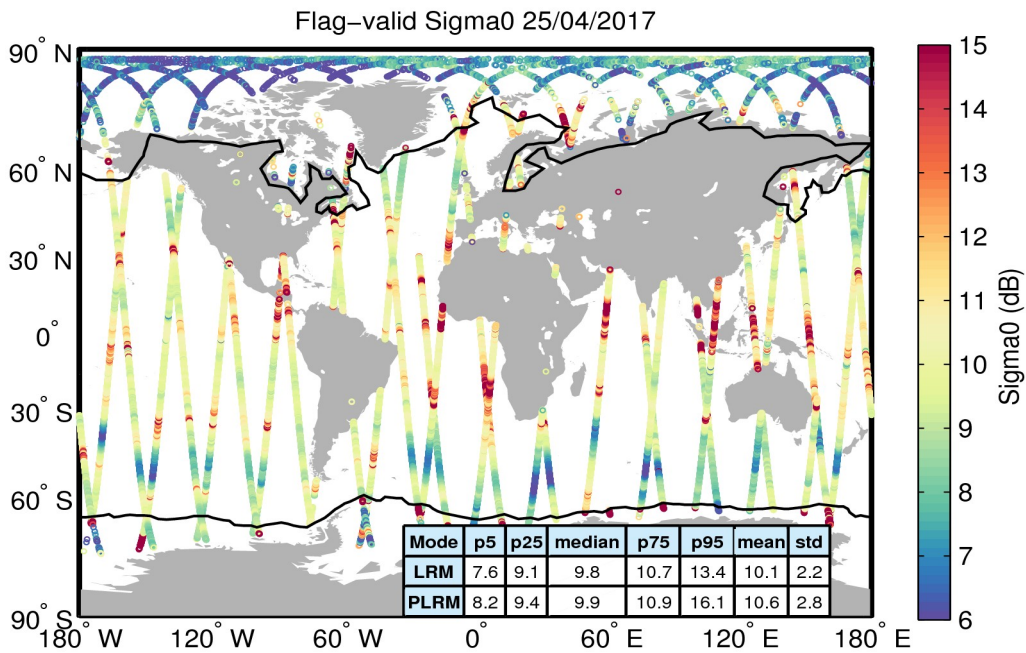
Figure 23. Geographical distribution of flag-valid sigma0 data over oceans and lakes for 25/04/2017. The statistical values shown in the table refer to the sigma0 in dB and are calculated separately for LRM and PLRM regions. Measurements taken over polar polygons have been excluded from the computation of the statistical values. The black lines mark the outer limit of the Arctic and Antarctic polar polygons.
