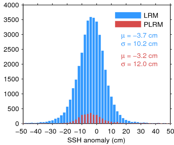
Figure 11. Histogram of science-valid SSH anomaly over oceans and lakes for LRM (blue) and PLRM (red) for 25/04/2017. The mean ( \mu ) and standard deviation ( \sigma ) are also shown. Note that values outside [-50 50] cm are excluded from the histogram for the sake of readability but not from the computation of \mu and \sigma .
