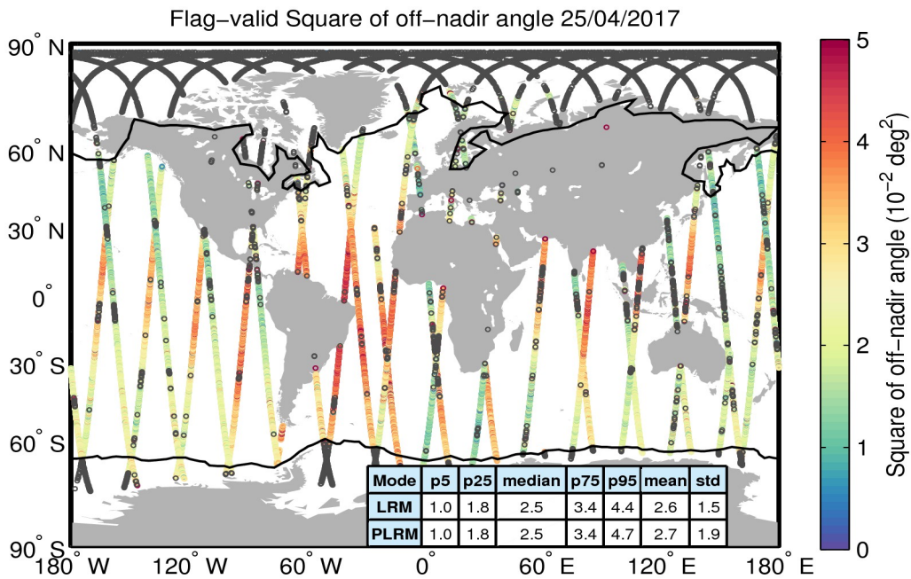
Figure 37. Geographical distribution of flag-valid mispointing data over oceans and lakes for 25/04/2017. The statistical values shown in the table refer to the mispointing in 10^{-2} deg 2 and are calculated separately for LRM and PLRM regions. Measurements taken over polar polygons have been excluded from the computation of the statistical values. The black lines mark the outer limit of the Arctic and Antarctic polar polygons. Gray circles denote negative values.
