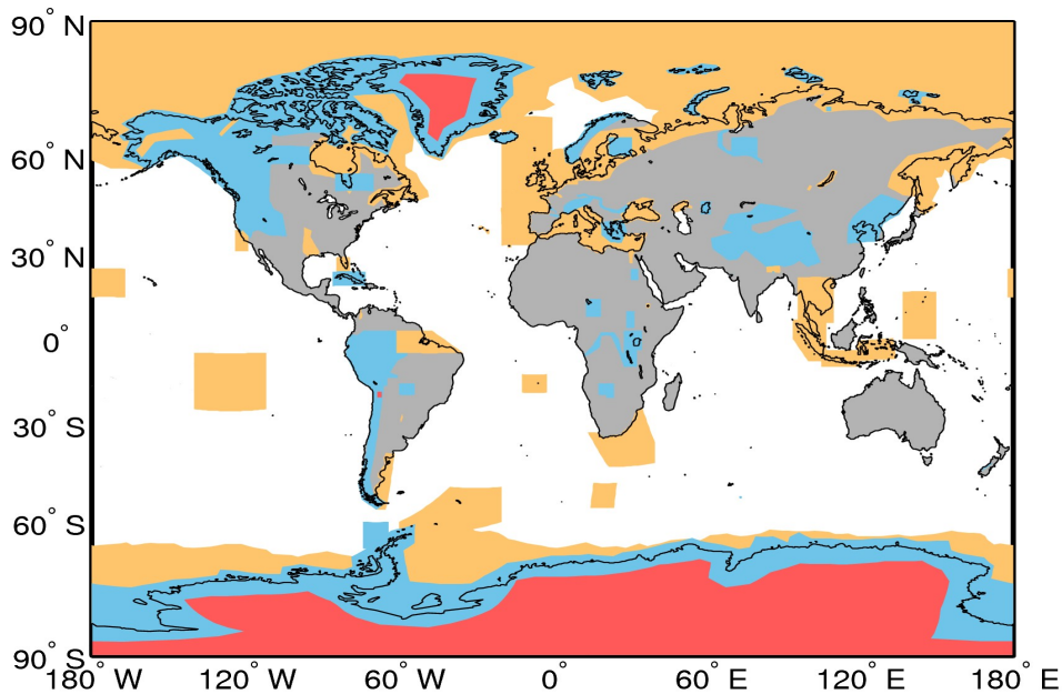
Figure A1. Extent of the regions defining the geographical mode mask for 25/04/2017. The regions where SAR, and SARIn are operated are denoted by the orange and blue polygons, respectively. LRM is operated over areas of the continental ice sheets (red polygons) and over oceans and land not covered by other modes.
