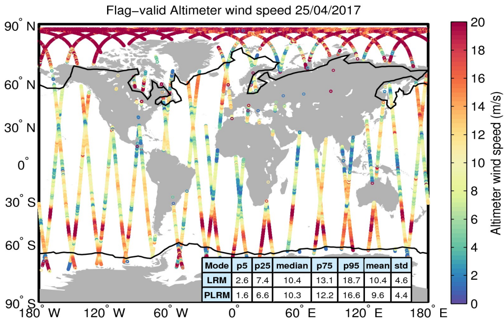
Figure 31. Geographical distribution of flag-valid wind data over oceans and lakes for 25/04/2017. The statistical values shown in the table refer to the wind in m/s and are calculated separately for LRM and PLRM regions. Measurements taken over polar polygons have been excluded from the computation of the statistical values. The black lines mark the outer limit of the Arctic and Antarctic polar polygons.
