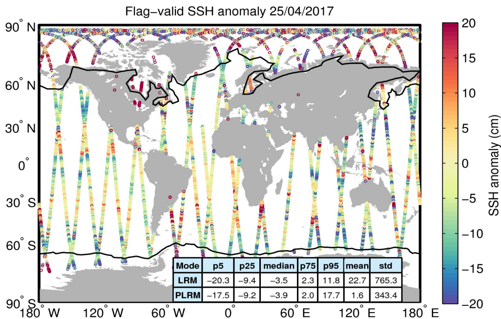
Figure 5. Geographical distribution of flag-valid 1-Hz SSH anomaly data over oceans and lakes for 25/04/2017. The statistical values shown in the table refer to the SSH anomaly in cm and are calculated separately for LRM and PLRM regions. Measurements taken over polar polygons have been excluded from the computation of the statistical values. The black lines mark the outer limit of the Arctic and Antarctic polar polygons.
