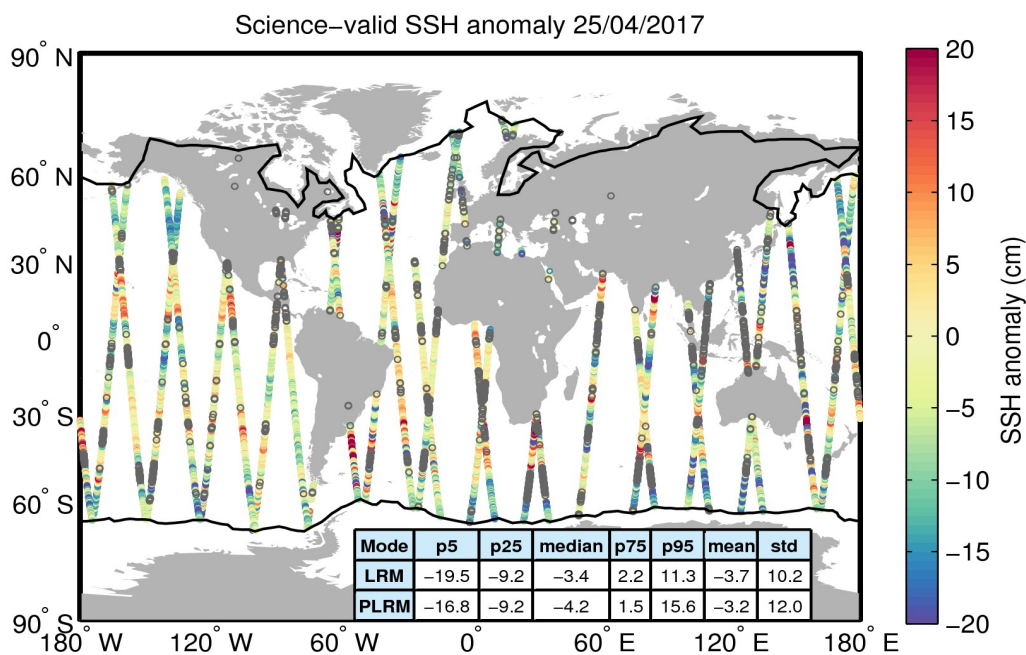
Figure 10. Geographical distribution of science-valid SSH anomaly data over oceans and lakes for 25/04/2017. The statistical values shown in the table refer to the SSH anomaly in cm and are calculated separately for LRM and PLRM regions. The black lines mark the outer limit of the Arctic and Antarctic polar polygons. Gray circles denote records that have been rejected based on the editing criteria described in Table 2.
