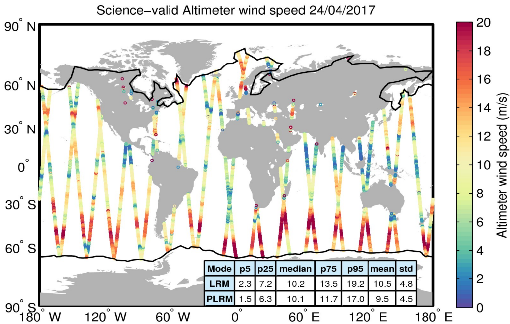
Figure 34. Geographical distribution of science-valid wind data over oceans and lakes for 24/04/2017. The statistical values shown in the table refer to the wind in m/s and are calculated separately for LRM and PLRM regions. The black lines mark the outer limit of the Arctic and Antarctic polar polygons. Gray circles denote records that have been rejected based on the editing criteria described in Table 5.
