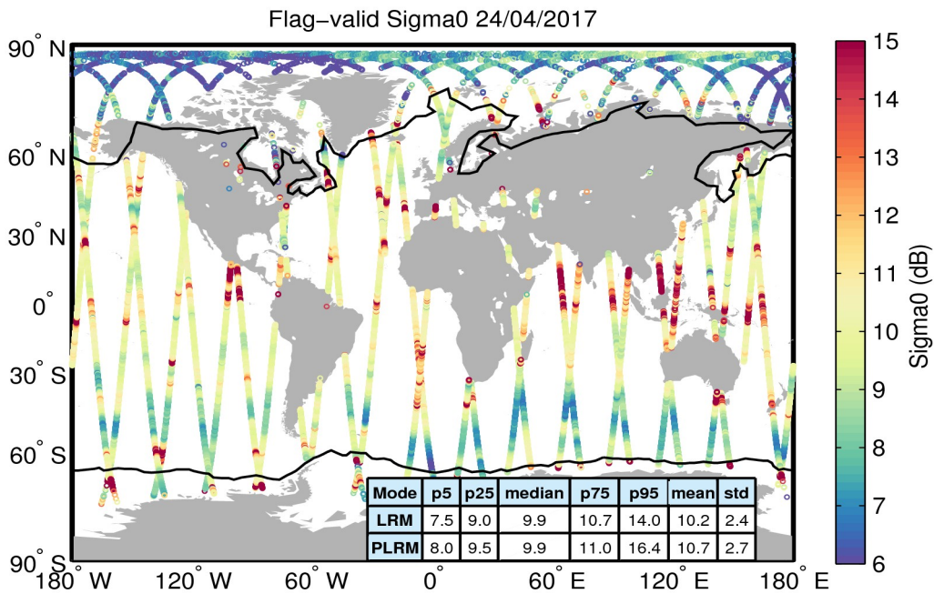
Figure 23. Geographical distribution of flag-valid sigma0 data over oceans and lakes for 24/04/2017. The statistical values shown in the table refer to the sigma0 in dB and are calculated separately for LRM and PLRM regions. Measurements taken over polar polygons have been excluded from the computation of the statistical values. The black lines mark the outer limit of the Arctic and Antarctic polar polygons.
