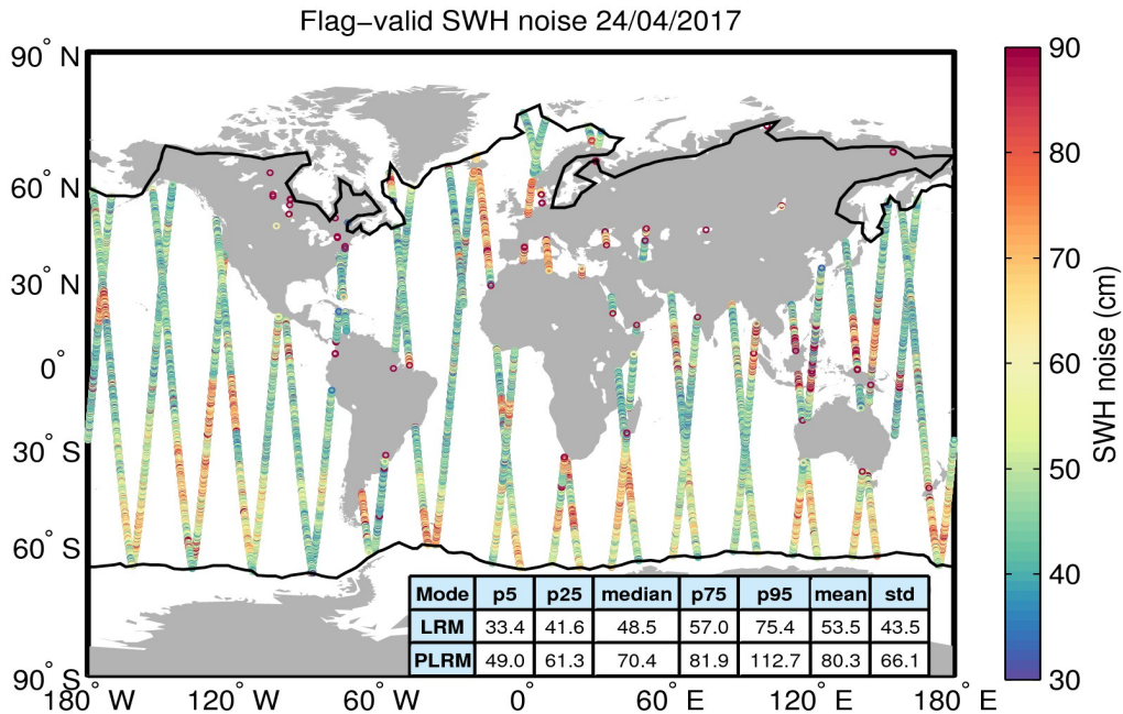
Figure 18. Geographical distribution of flag-valid 20-Hz SWH measurement noise over oceans and lakes for 24/04/2017. The statistical values shown in the table refer to the SWH noise and are calculated separately for LRM and PLRM regions. Measurements taken over polar polygons have been excluded from the computation of the statistical values. The black lines mark the outer limit of the Arctic and Antarctic polar polygons.
