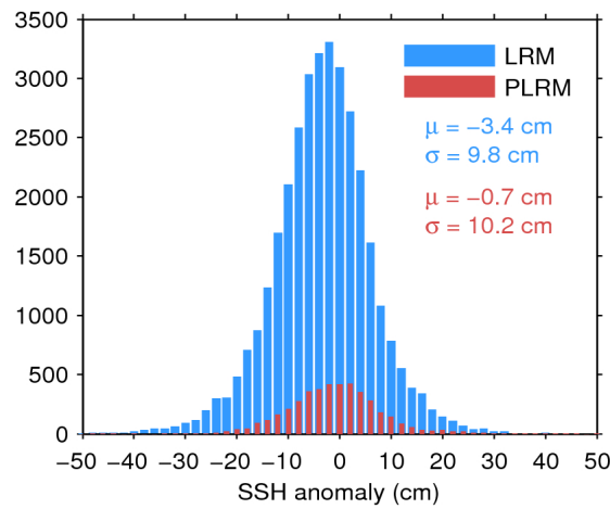
Figure 11. Histogram of science-valid SSH anomaly over oceans and lakes for LRM (blue) and PLRM (red) for 24/04/2017. The mean ( \mu ) and standard deviation ( \sigma ) are also shown. Note that values outside [-50 50] cm are excluded from the histogram for the sake of readability but not from the computation of \mu and \sigma .
