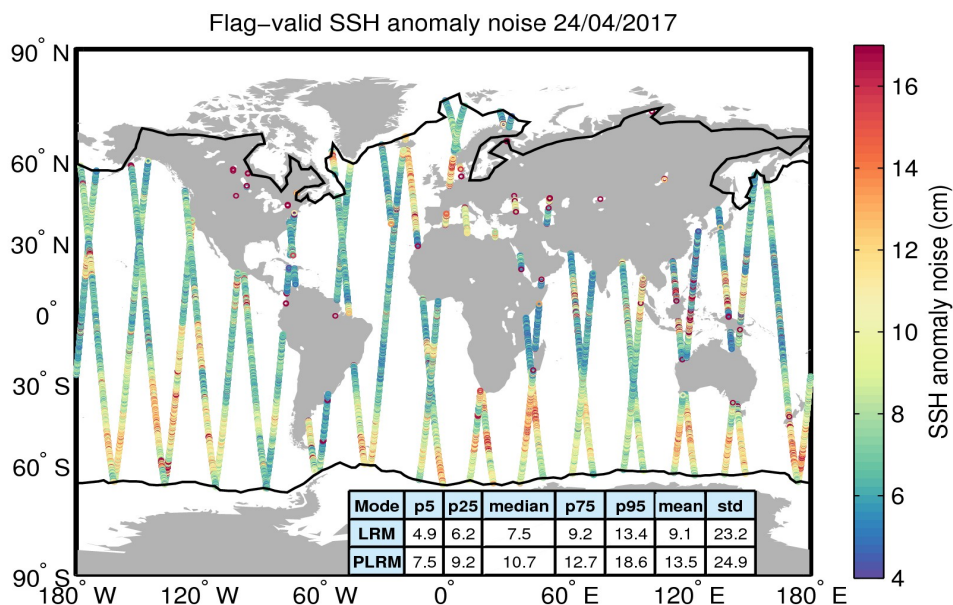
Figure 8. Geographical distribution of flag-valid 20-Hz SSH anomaly measurement noise over oceans and lakes for 24/04/2017. The statistical values shown in the table refer to the SSH anomaly noise and are calculated separately for LRM and PLRM regions. Measurements taken over polar polygons have been excluded from the computation of the statistical values. The black lines mark the outer limit of the Arctic and Antarctic polar polygons.
