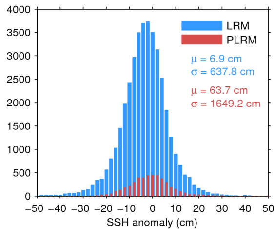
Figure 7. Histogram of flag-valid SSH anomaly over oceans and lakes for LRM (blue) and PLRM (red) for 24/04/2017. The mean ( \mu ) and standard deviation ( \sigma ) are also shown. Note that values outside [-50 \ 50] cm are excluded from the histogram for the sake of readability but not from the computation of \mu and \sigma .
