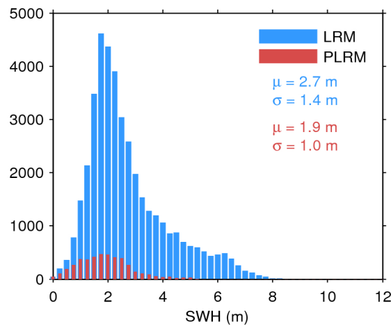
Figure 20. Histogram of science-valid SWH over oceans and lakes for LRM (blue) and PLRM (red) for 24/04/2017. The mean ( \mu ) and standard deviation ( \sigma ) are also shown. Note that values larger than 12 m are excluded from the histogram for the sake of readability but not from the computation of \mu and \sigma .
