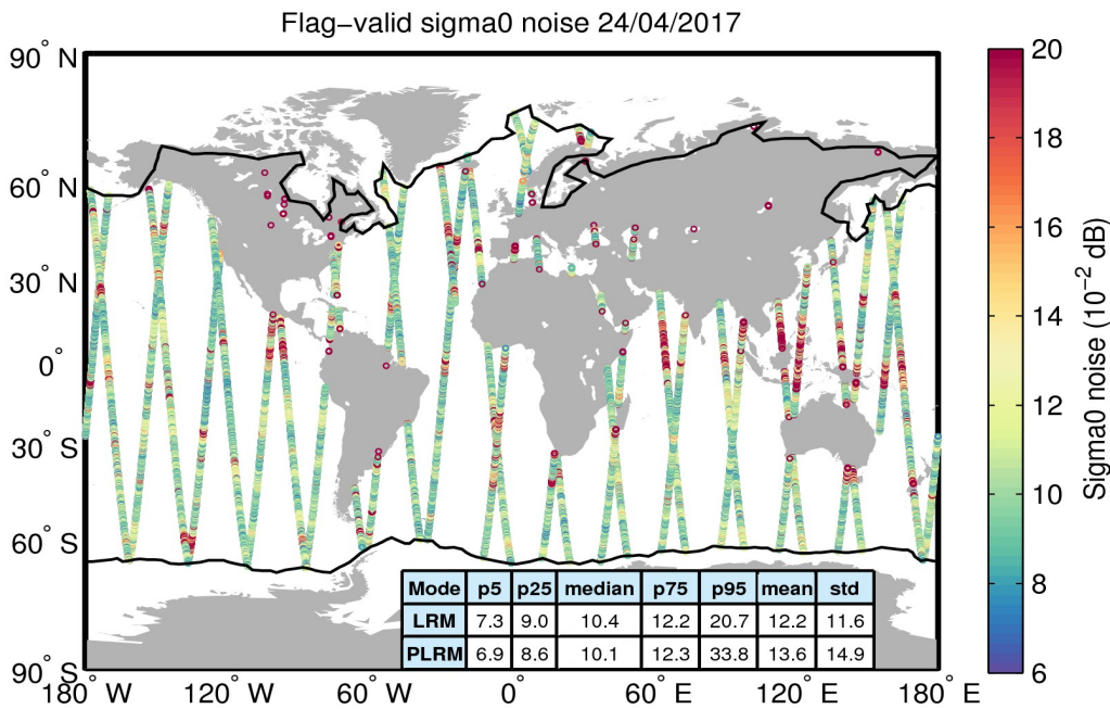
Figure 26. Geographical distribution of flag-valid 20-Hz sigma0 measurement noise over oceans and lakes for 24/04/2017. The statistical values shown in the table refer to the sigma0 noise and are calculated separately for LRM and PLRM regions. Measurements taken over polar polygons have been excluded from the computation of the statistical values. The black lines mark the outer limit of the Arctic and Antarctic polar polygons.
