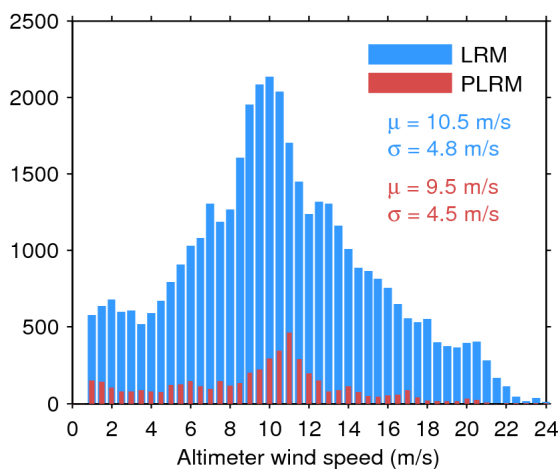
Figure 33. Histogram of flag-valid wind over oceans and lakes for LRM (blue) and PLRM (red) for 24/04/2017. The mean ( \mu ) and standard deviation ( \sigma ) are also shown. Note that values larger than 24 m/s are excluded from the histogram for the sake of readability but not from the computation of \mu and \sigma .
