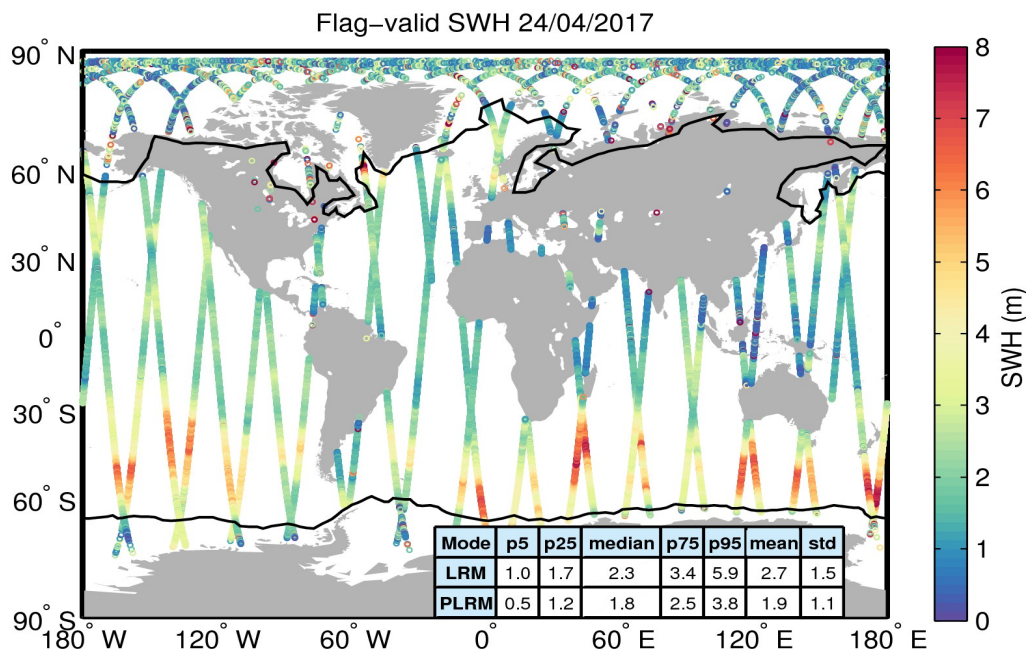
Figure 15. Geographical distribution of flag-valid SWH data over oceans and lakes for 24/04/2017. The statistical values shown in the table refer to the SWH in m and are calculated separately for LRM and PLRM regions. Measurements taken over polar polygons have been excluded from the computation of the statistical values. The black lines mark the outer limit of the Arctic and Antarctic polar polygons.
