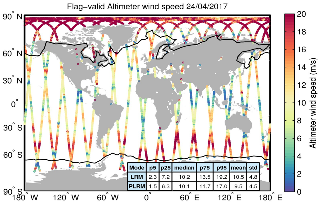
Figure 31. Geographical distribution of flag-valid wind data over oceans and lakes for 24/04/2017. The statistical values shown in the table refer to the wind in m/s and are calculated separately for LRM and PLRM regions. Measurements taken over polar polygons have been excluded from the computation of the statistical values. The black lines mark the outer limit of the Arctic and Antarctic polar polygons.
