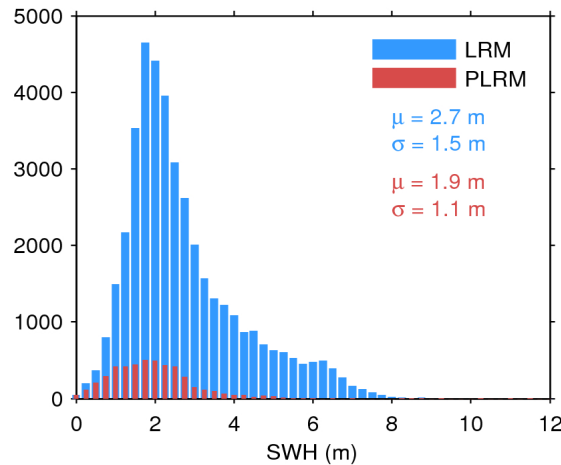
Figure 17. Histogram of flag-valid SWH over oceans and lakes for LRM (blue) and PLRM (red) for 24/04/2017. The mean ( \mu ) and standard deviation ( \sigma ) are also shown. Note that values larger than 12 m are excluded from the histogram for the sake of readability but not from the computation of \mu and \sigma .
