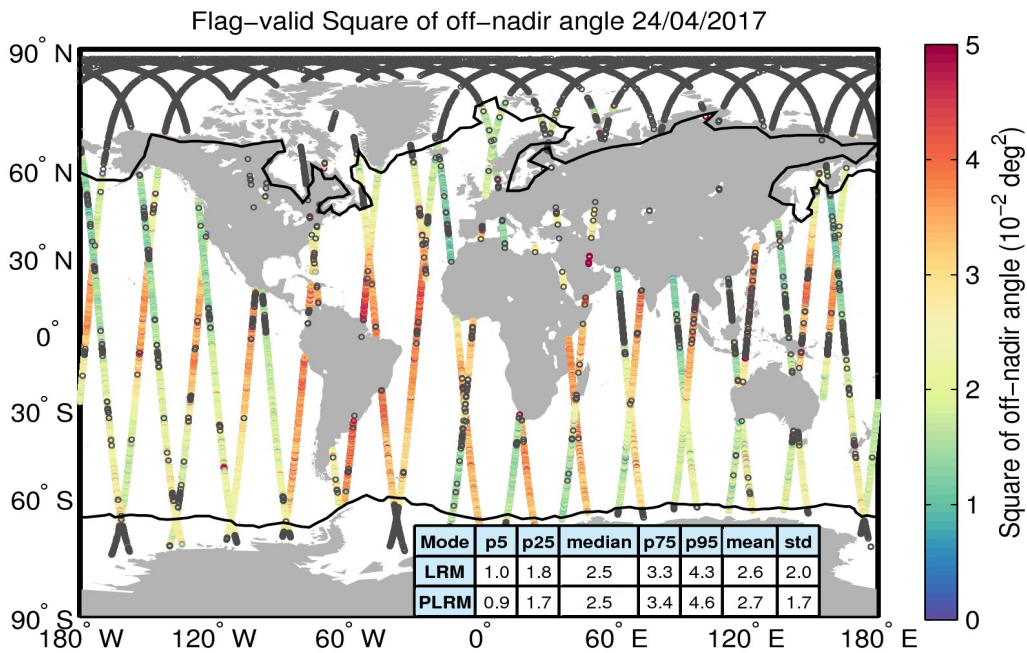
Figure 37. Geographical distribution of flag-valid mispointing data over oceans and lakes for 24/04/2017. The statistical values shown in the table refer to the mispointing in 10^{-2} deg 2 and are calculated separately for LRM and PLRM regions. Measurements taken over polar polygons have been excluded from the computation of the statistical values. The black lines mark the outer limit of the Arctic and Antarctic polar polygons. Gray circles denote negative values.
