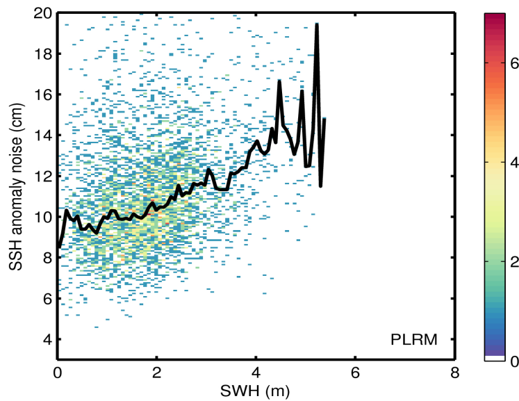
Figure 9. 2D histogram showing flag-valid SSH anomaly noise as a function of SWH for LRM (top) and PLRM (bottom) for 24/04/2017. The black line denotes the median SSH anomaly noise as a function of SWH.
