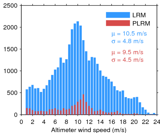
Figure 35. Histogram of science-valid wind over oceans and lakes for LRM (blue) and PLRM (red) for 24/04/2017. The mean ( \mu ) and standard deviation ( \sigma ) are also shown. Note that values larger than 24 m/s are excluded from the histogram for the sake of readability but not from the computation of \mu and \sigma .
