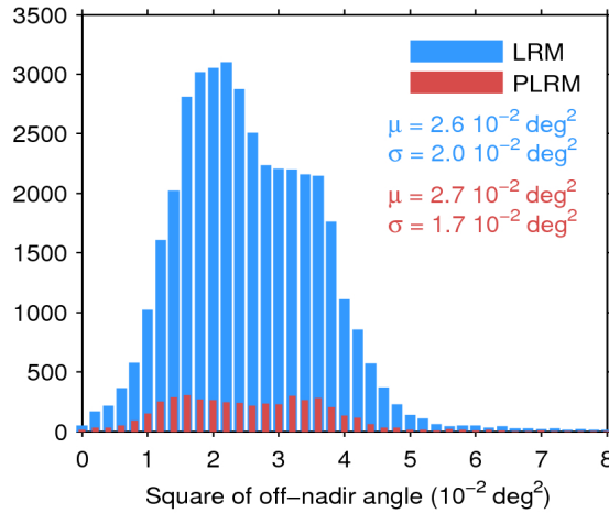
Figure 39. Histogram of flag-valid mispointing over oceans and lakes for LRM (blue) and PLRM (red) for 24/04/2017. Only positive values have been considered. The mean ( \mu ) and standard deviation ( \sigma ) are also shown. Note that values larger than 8 \cdot 10^{-2} \text{ deg}^2 are excluded from the histogram for the sake of readability but not from the computation of \mu and \sigma .
