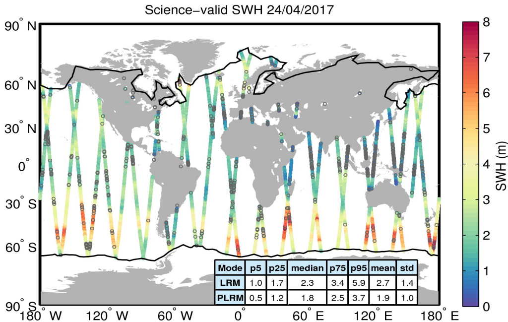
Figure 19. Geographical distribution of science-valid SWH data over oceans and lakes for 24/04/2017. The statistical values shown in the table refer to the SWH in m and are calculated separately for LRM and PLRM regions. The black lines mark the outer limit of the Arctic and Antarctic polar polygons. Gray circles denote records that have been rejected based on the editing criteria described in Table 3.
