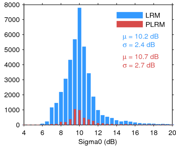
Figure 25. Histogram of flag-valid sigma0 over oceans and lakes for LRM (blue) and PLRM (red) for 24/04/2017. The mean ( \mu ) and standard deviation ( \sigma ) are also shown. Note that values outside [4 20] dB are excluded from the histogram for the sake of readability but not from the computation of \mu and \sigma .
