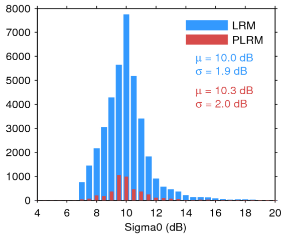
Figure 28. Histogram of science-valid sigma0 over oceans and lakes for LRM (blue) and PLRM (red) for 24/04/2017. The mean ( \mu ) and standard deviation ( \sigma ) are also shown. Note that values outside [4 20] dB are excluded from the histogram for the sake of readability but not from the computation of \mu and \sigma .
