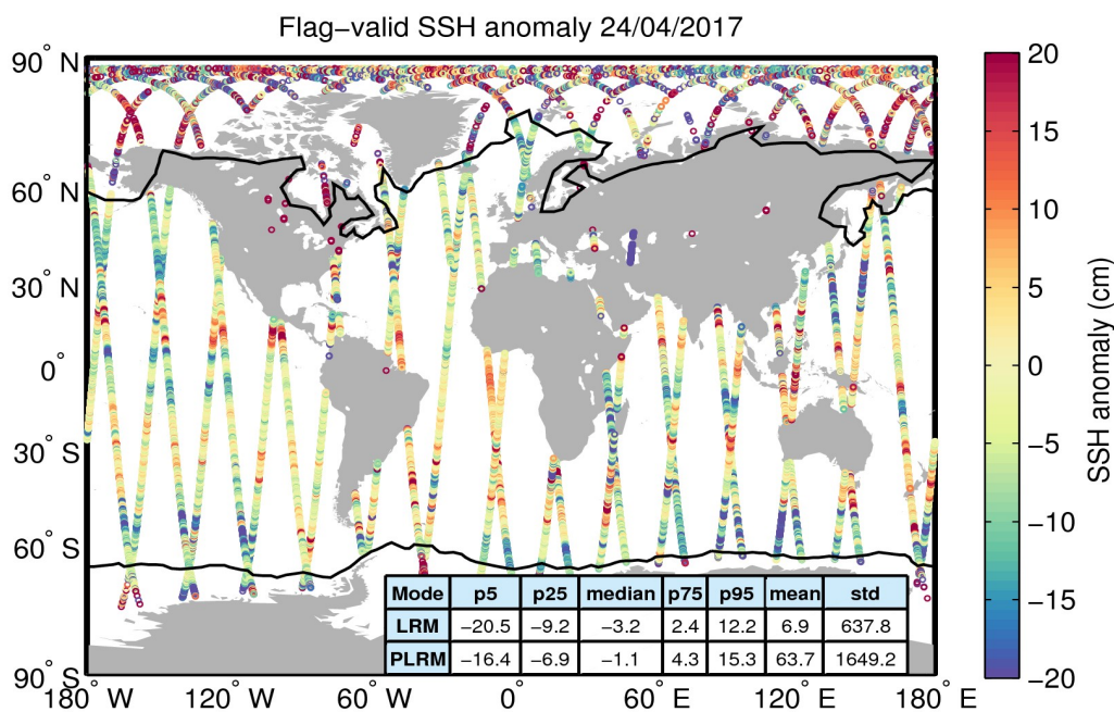
Figure 5. Geographical distribution of flag-valid 1-Hz SSH anomaly data over oceans and lakes for 24/04/2017. The statistical values shown in the table refer to the SSH anomaly in cm and are calculated separately for LRM and PLRM regions. Measurements taken over polar polygons have been excluded from the computation of the statistical values. The black lines mark the outer limit of the Arctic and Antarctic polar polygons.
