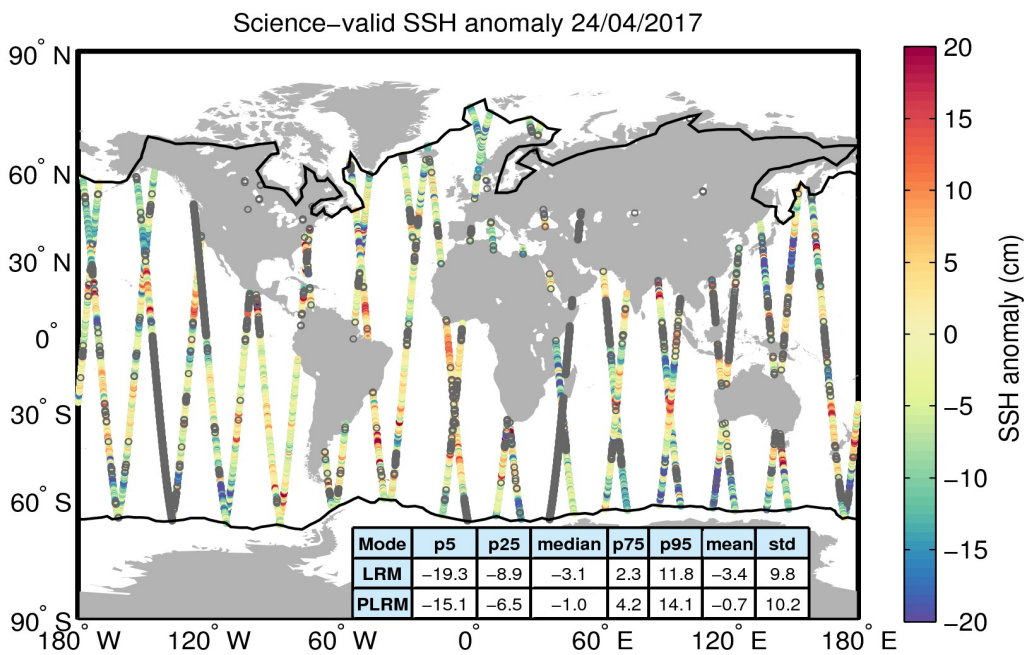
Figure 10. Geographical distribution of science-valid SSH anomaly data over oceans and lakes for 24/04/2017. The statistical values shown in the table refer to the SSH anomaly in cm and are calculated separately for LRM and PLRM regions. The black lines mark the outer limit of the Arctic and Antarctic polar polygons. Gray circles denote records that have been rejected based on the editing criteria described in Table 2.
