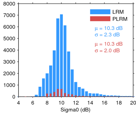
Figure 25. Histogram of flag-valid sigma0 over oceans and lakes for LRM (blue) and PLRM (red) for 23/04/2017. The mean ( \mu ) and standard deviation ( \sigma ) are also shown. Note that values outside [4 20] dB are excluded from the histogram for the sake of readability but not from the computation of \mu and \sigma .
