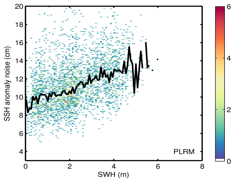
Figure 9. 2D histogram showing flag-valid SSH anomaly noise as a function of SWH for LRM (top) and PLRM (bottom) for 23/04/2017. The black line denotes the median SSH anomaly noise as a function of SWH.
