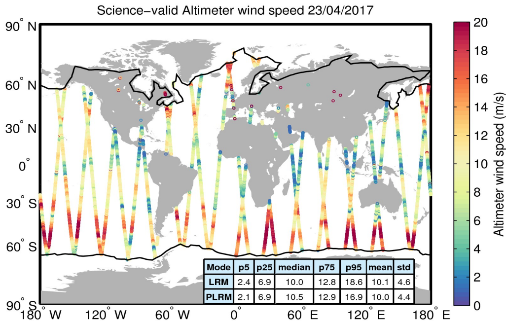
Figure 34. Geographical distribution of science-valid wind data over oceans and lakes for 23/04/2017. The statistical values shown in the table refer to the wind in m/s and are calculated separately for LRM and PLRM regions. The black lines mark the outer limit of the Arctic and Antarctic polar polygons. Gray circles denote records that have been rejected based on the editing criteria described in Table 5.
