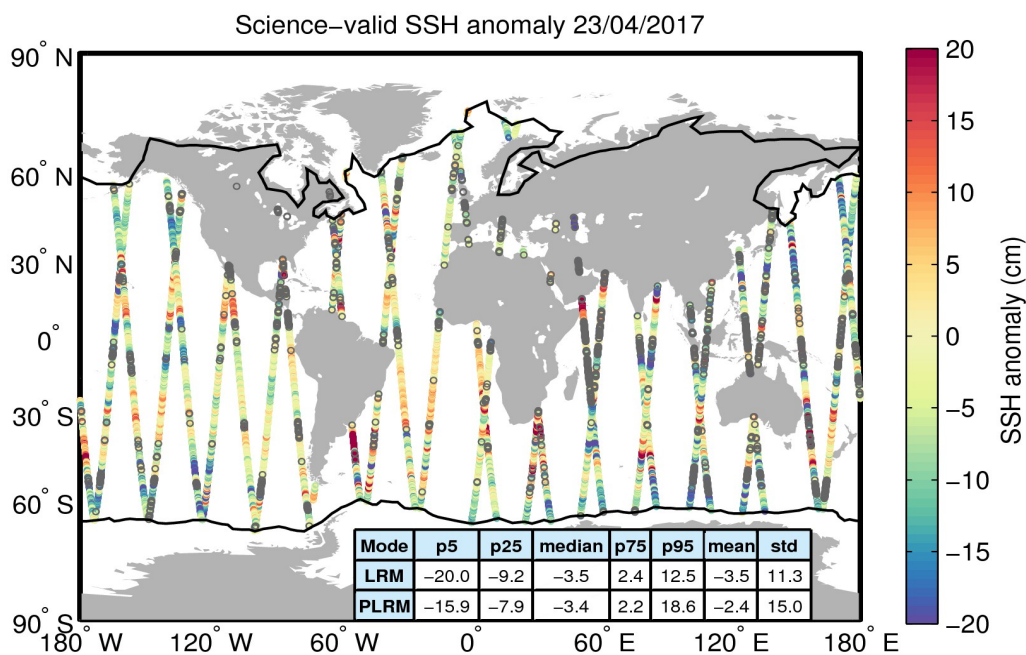
Figure 10. Geographical distribution of science-valid SSH anomaly data over oceans and lakes for 23/04/2017. The statistical values shown in the table refer to the SSH anomaly in cm and are calculated separately for LRM and PLRM regions. The black lines mark the outer limit of the Arctic and Antarctic polar polygons. Gray circles denote records that have been rejected based on the editing criteria described in Table 2.
