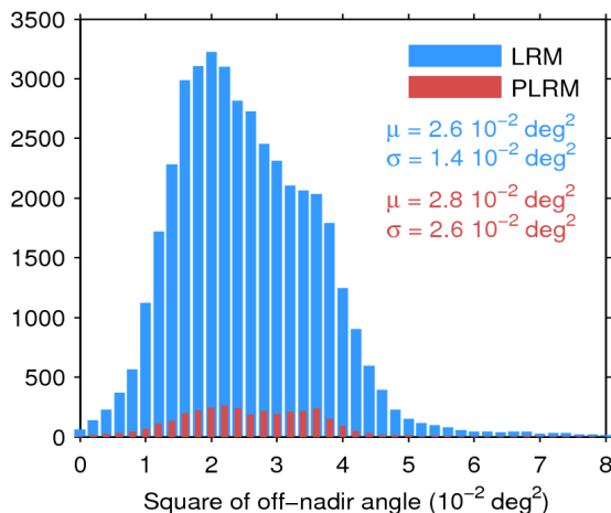
Figure 39. Histogram of flag-valid mispointing over oceans and lakes for LRM (blue) and PLRM (red) for 23/04/2017. Only positive values have been considered. The mean ( \mu ) and standard deviation ( \sigma ) are also shown. Note that values larger than 8 \cdot 10^{-2} \text{ deg}^2 are excluded from the histogram for the sake of readability but not from the computation of \mu and \sigma .
