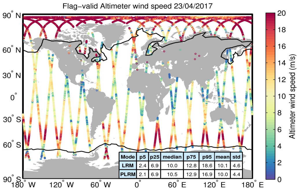
Figure 31. Geographical distribution of flag-valid wind data over oceans and lakes for 23/04/2017. The statistical values shown in the table refer to the wind in m/s and are calculated separately for LRM and PLRM regions. Measurements taken over polar polygons have been excluded from the computation of the statistical values. The black lines mark the outer limit of the Arctic and Antarctic polar polygons.
