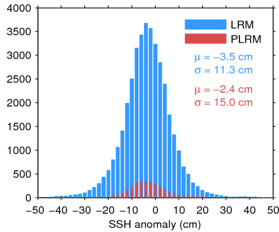
Figure 11. Histogram of science-valid SSH anomaly over oceans and lakes for LRM (blue) and PLRM (red) for 23/04/2017. The mean ( \mu ) and standard deviation ( \sigma ) are also shown. Note that values outside [-50 50] cm are excluded from the histogram for the sake of readability but not from the computation of \mu and \sigma .
