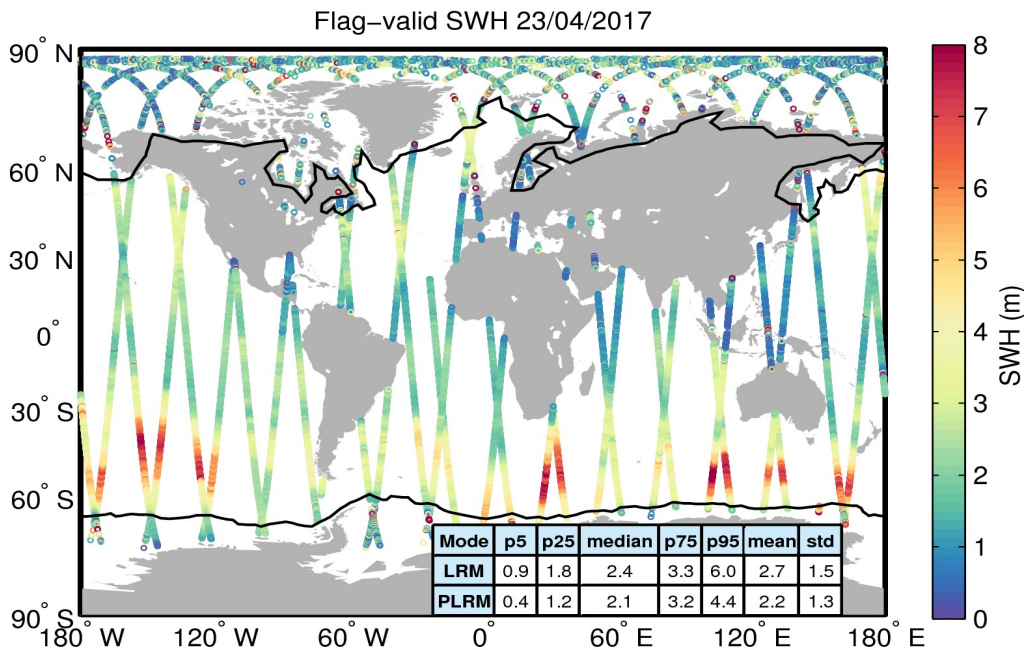
Figure 15. Geographical distribution of flag-valid SWH data over oceans and lakes for 23/04/2017. The statistical values shown in the table refer to the SWH in m and are calculated separately for LRM and PLRM regions. Measurements taken over polar polygons have been excluded from the computation of the statistical values. The black lines mark the outer limit of the Arctic and Antarctic polar polygons.
