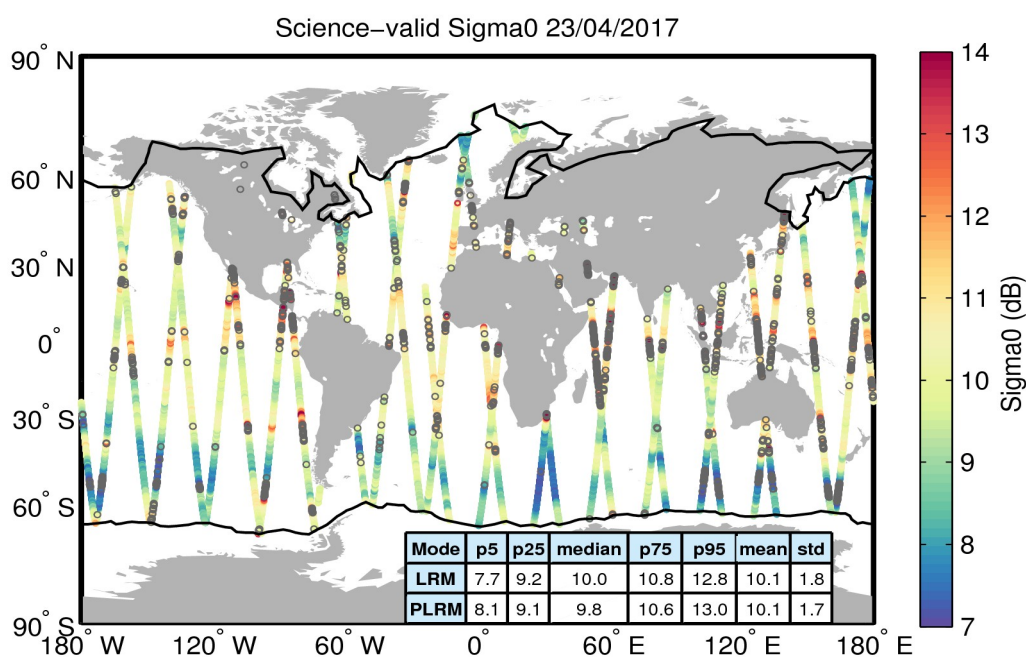
Figure 27. Geographical distribution of science-valid sigma0 data over oceans and lakes for 23/04/2017. The statistical values shown in the table refer to the sigma0 in dB and are calculated separately for LRM and PLRM regions. The black lines mark the outer limit of the Arctic and Antarctic polar polygons. Gray circles denote records that have been rejected based on the editing criteria described in Table 4.
