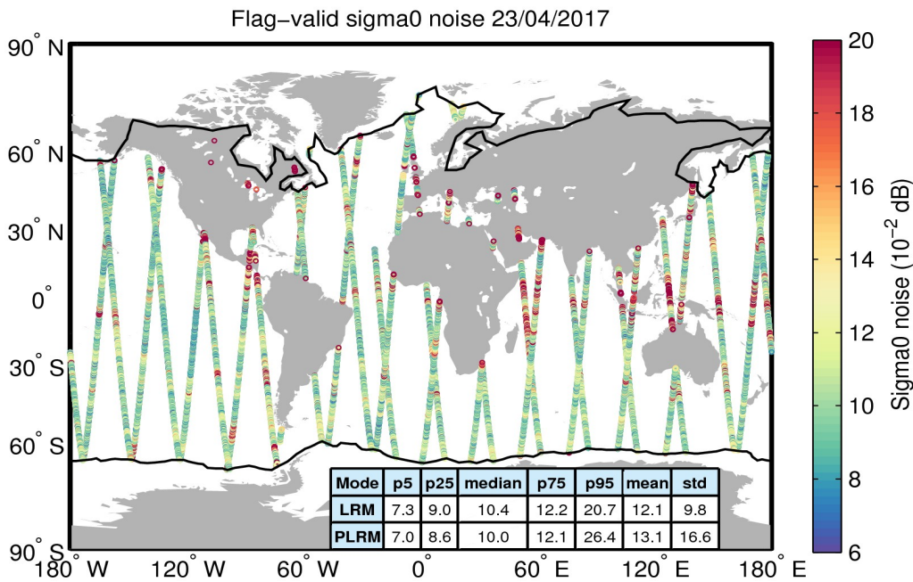
Figure 26. Geographical distribution of flag-valid 20-Hz sigma0 measurement noise over oceans and lakes for 23/04/2017. The statistical values shown in the table refer to the sigma0 noise and are calculated separately for LRM and PLRM regions. Measurements taken over polar polygons have been excluded from the computation of the statistical values. The black lines mark the outer limit of the Arctic and Antarctic polar polygons.
