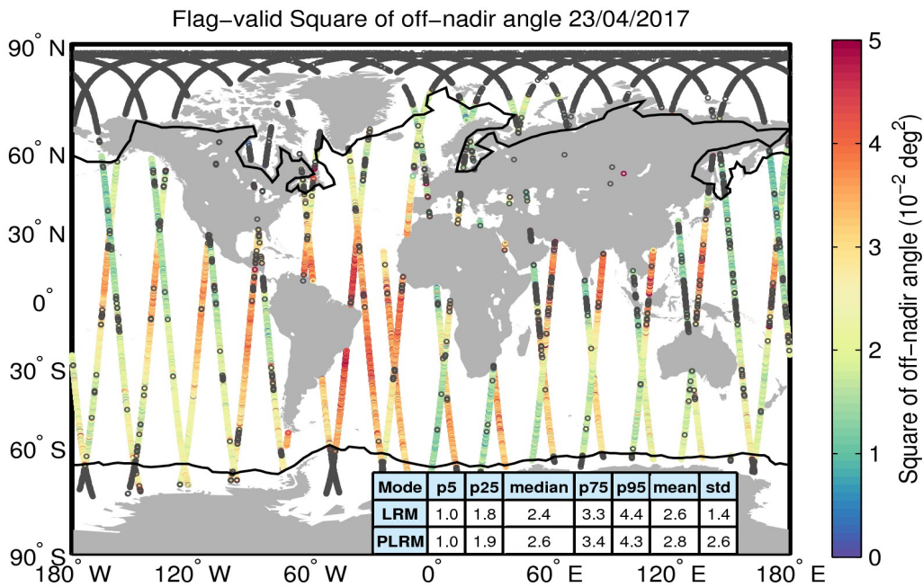
Figure 37. Geographical distribution of flag-valid mispointing data over oceans and lakes for 23/04/2017. The statistical values shown in the table refer to the mispointing in 10^{-2} deg 2 and are calculated separately for LRM and PLRM regions. Measurements taken over polar polygons have been excluded from the computation of the statistical values. The black lines mark the outer limit of the Arctic and Antarctic polar polygons. Gray circles denote negative values.
