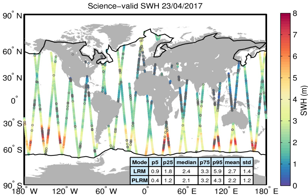
Figure 19. Geographical distribution of science-valid SWH data over oceans and lakes for 23/04/2017. The statistical values shown in the table refer to the SWH in m and are calculated separately for LRM and PLRM regions. The black lines mark the outer limit of the Arctic and Antarctic polar polygons. Gray circles denote records that have been rejected based on the editing criteria described in Table 3.
