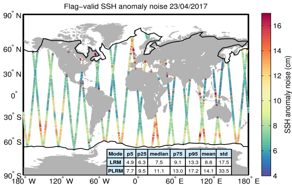
Figure 8. Geographical distribution of flag-valid 20-Hz SSH anomaly measurement noise over oceans and lakes for 23/04/2017. The statistical values shown in the table refer to the SSH anomaly noise and are calculated separately for LRM and PLRM regions. Measurements taken over polar polygons have been excluded from the computation of the statistical values. The black lines mark the outer limit of the Arctic and Antarctic polar polygons.
