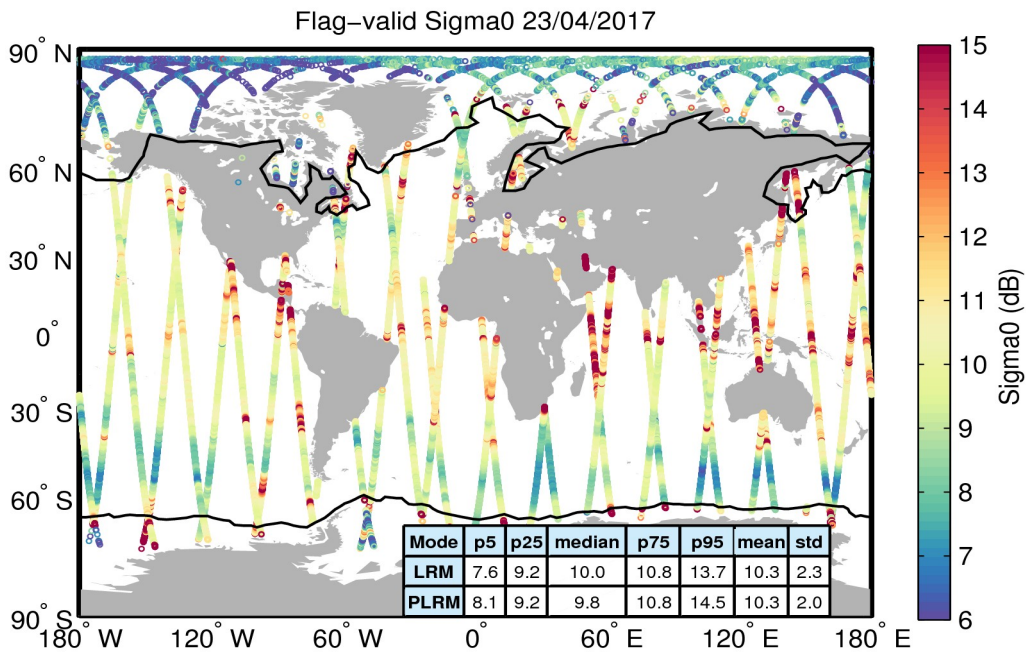
Figure 23. Geographical distribution of flag-valid sigma0 data over oceans and lakes for 23/04/2017. The statistical values shown in the table refer to the sigma0 in dB and are calculated separately for LRM and PLRM regions. Measurements taken over polar polygons have been excluded from the computation of the statistical values. The black lines mark the outer limit of the Arctic and Antarctic polar polygons.
