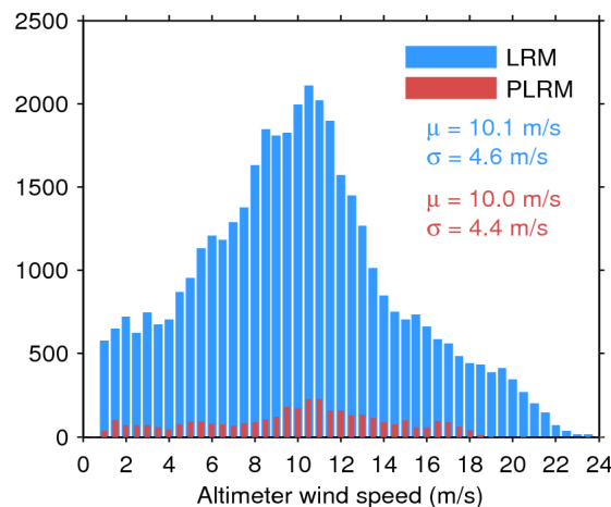
Figure 35. Histogram of science-valid wind over oceans and lakes for LRM (blue) and PLRM (red) for 23/04/2017. The mean ( \mu ) and standard deviation ( \sigma ) are also shown. Note that values larger than 24 m/s are excluded from the histogram for the sake of readability but not from the computation of \mu and \sigma .
