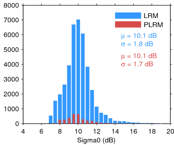
Figure 28. Histogram of science-valid sigma0 over oceans and lakes for LRM (blue) and PLRM (red) for 23/04/2017. The mean ( \mu ) and standard deviation ( \sigma ) are also shown. Note that values outside [4 20] dB are excluded from the histogram for the sake of readability but not from the computation of \mu and \sigma .
