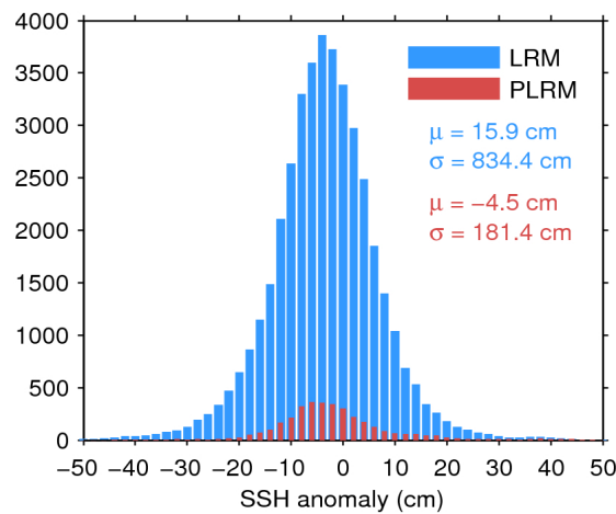
Figure 7. Histogram of flag-valid SSH anomaly over oceans and lakes for LRM (blue) and PLRM (red) for 23/04/2017. The mean ( \mu ) and standard deviation ( \sigma ) are also shown. Note that values outside [-50 50] cm are excluded from the histogram for the sake of readability but not from the computation of \mu and \sigma .
