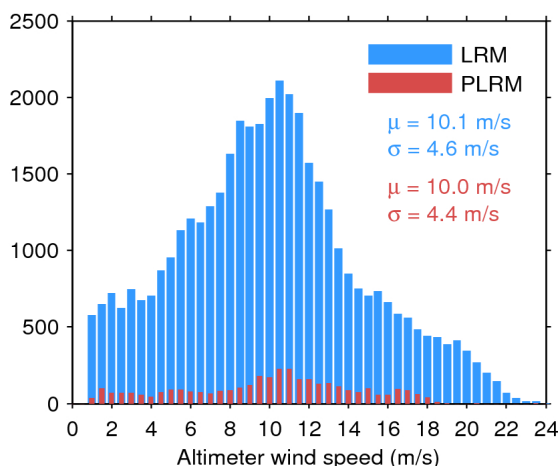
Figure 33. Histogram of flag-valid wind over oceans and lakes for LRM (blue) and PLRM (red) for 23/04/2017. The mean ( \mu ) and standard deviation ( \sigma ) are also shown. Note that values larger than 24 m/s are excluded from the histogram for the sake of readability but not from the computation of \mu and \sigma .
