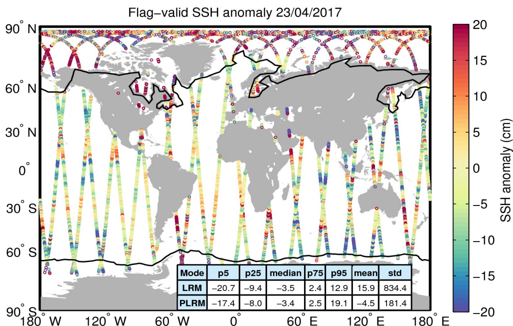
Figure 5. Geographical distribution of flag-valid 1-Hz SSH anomaly data over oceans and lakes for 23/04/2017. The statistical values shown in the table refer to the SSH anomaly in cm and are calculated separately for LRM and PLRM regions. Measurements taken over polar polygons have been excluded from the computation of the statistical values. The black lines mark the outer limit of the Arctic and Antarctic polar polygons.
