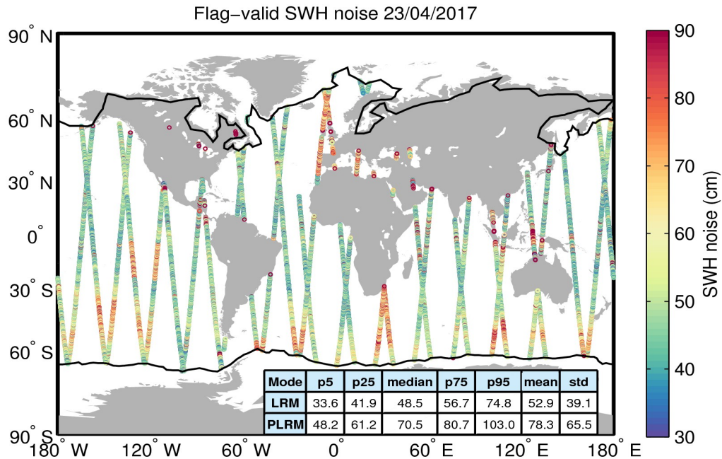
Figure 18. Geographical distribution of flag-valid 20-Hz SWH measurement noise over oceans and lakes for 23/04/2017. The statistical values shown in the table refer to the SWH noise and are calculated separately for LRM and PLRM regions. Measurements taken over polar polygons have been excluded from the computation of the statistical values. The black lines mark the outer limit of the Arctic and Antarctic polar polygons.
