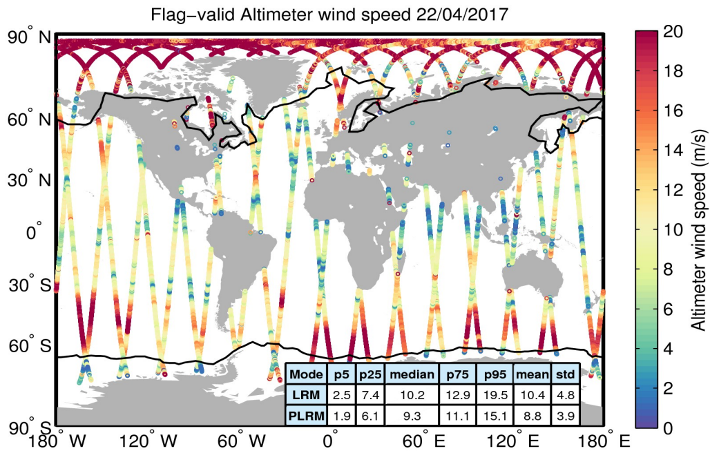
Figure 31. Geographical distribution of flag-valid wind data over oceans and lakes for 22/04/2017. The statistical values shown in the table refer to the wind in m/s and are calculated separately for LRM and PLRM regions. Measurements taken over polar polygons have been excluded from the computation of the statistical values. The black lines mark the outer limit of the Arctic and Antarctic polar polygons.
