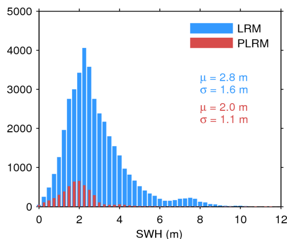
Figure 17. Histogram of flag-valid SWH over oceans and lakes for LRM (blue) and PLRM (red) for 22/04/2017. The mean ( \mu ) and standard deviation ( \sigma ) are also shown. Note that values larger than 12 m are excluded from the histogram for the sake of readability but not from the computation of \mu and \sigma .
