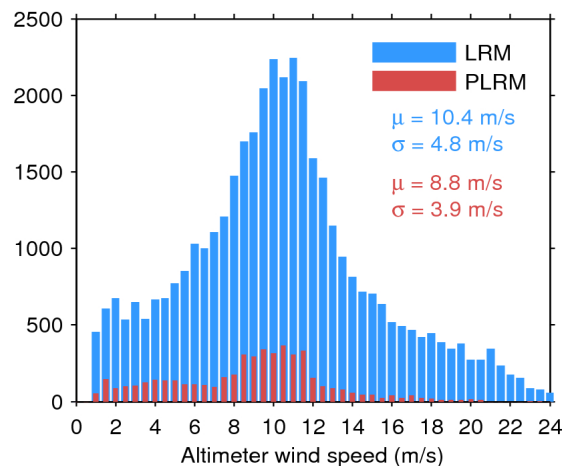
Figure 35. Histogram of science-valid wind over oceans and lakes for LRM (blue) and PLRM (red) for 22/04/2017. The mean ( \mu ) and standard deviation ( \sigma ) are also shown. Note that values larger than 24 m/s are excluded from the histogram for the sake of readability but not from the computation of \mu and \sigma .
