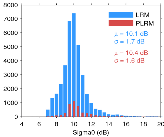
Figure 28. Histogram of science-valid sigma0 over oceans and lakes for LRM (blue) and PLRM (red) for 22/04/2017. The mean ( \mu ) and standard deviation ( \sigma ) are also shown. Note that values outside [4 20] dB are excluded from the histogram for the sake of readability but not from the computation of \mu and \sigma .
