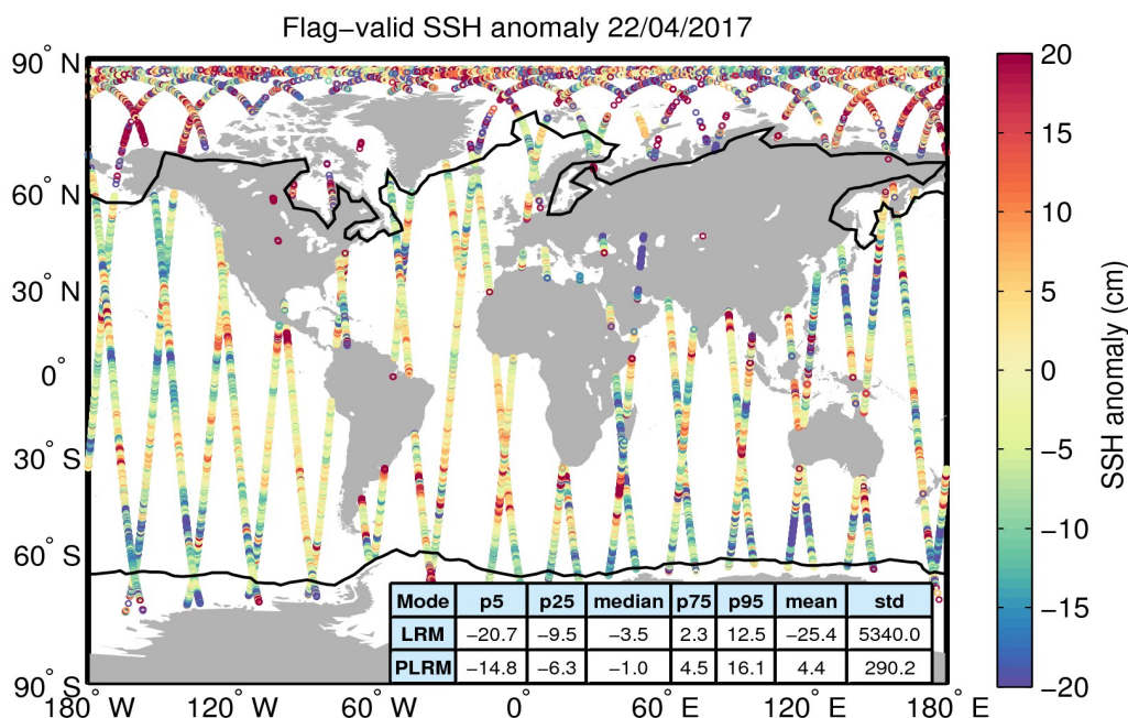
Figure 5. Geographical distribution of flag-valid 1-Hz SSH anomaly data over oceans and lakes for 22/04/2017. The statistical values shown in the table refer to the SSH anomaly in cm and are calculated separately for LRM and PLRM regions. Measurements taken over polar polygons have been excluded from the computation of the statistical values. The black lines mark the outer limit of the Arctic and Antarctic polar polygons.
