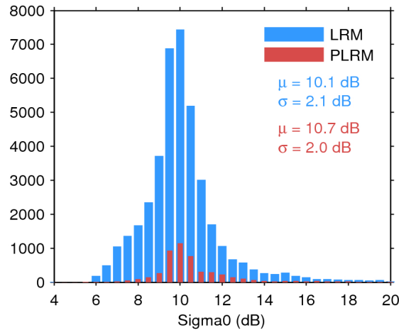
Figure 25. Histogram of flag-valid sigma0 over oceans and lakes for LRM (blue) and PLRM (red) for 22/04/2017. The mean ( \mu ) and standard deviation ( \sigma ) are also shown. Note that values outside [4 20] dB are excluded from the histogram for the sake of readability but not from the computation of \mu and \sigma .
