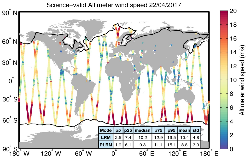
Figure 34. Geographical distribution of science-valid wind data over oceans and lakes for 22/04/2017. The statistical values shown in the table refer to the wind in m/s and are calculated separately for LRM and PLRM regions. The black lines mark the outer limit of the Arctic and Antarctic polar polygons. Gray circles denote records that have been rejected based on the editing criteria described in Table 5.
