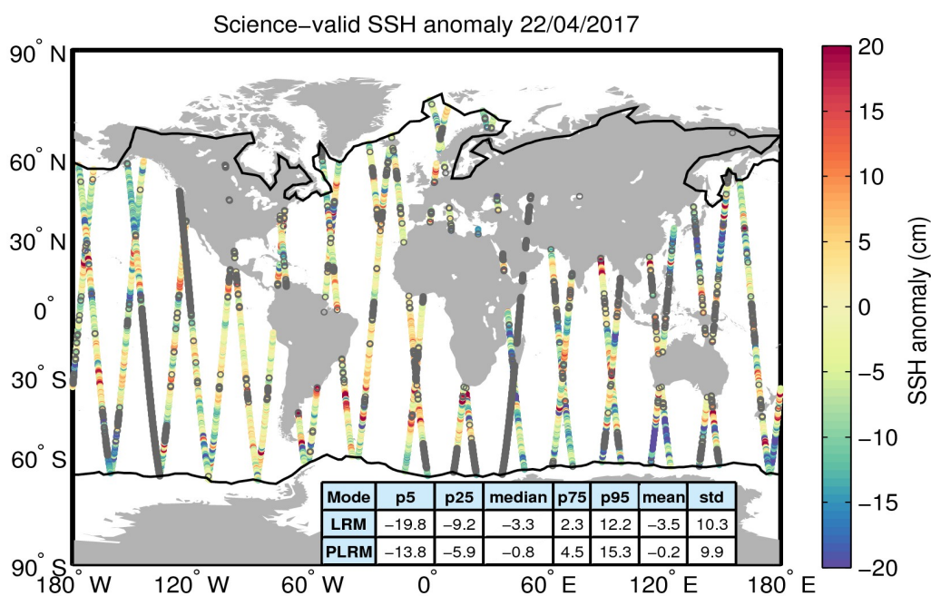
Figure 10. Geographical distribution of science-valid SSH anomaly data over oceans and lakes for 22/04/2017. The statistical values shown in the table refer to the SSH anomaly in cm and are calculated separately for LRM and PLRM regions. The black lines mark the outer limit of the Arctic and Antarctic polar polygons. Gray circles denote records that have been rejected based on the editing criteria described in Table 2.
