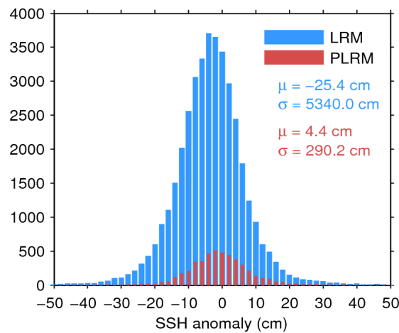
Figure 7. Histogram of flag-valid SSH anomaly over oceans and lakes for LRM (blue) and PLRM (red) for 22/04/2017. The mean ( \mu ) and standard deviation ( \sigma ) are also shown. Note that values outside [-50 50] cm are excluded from the histogram for the sake of readability but not from the computation of \mu and \sigma .
