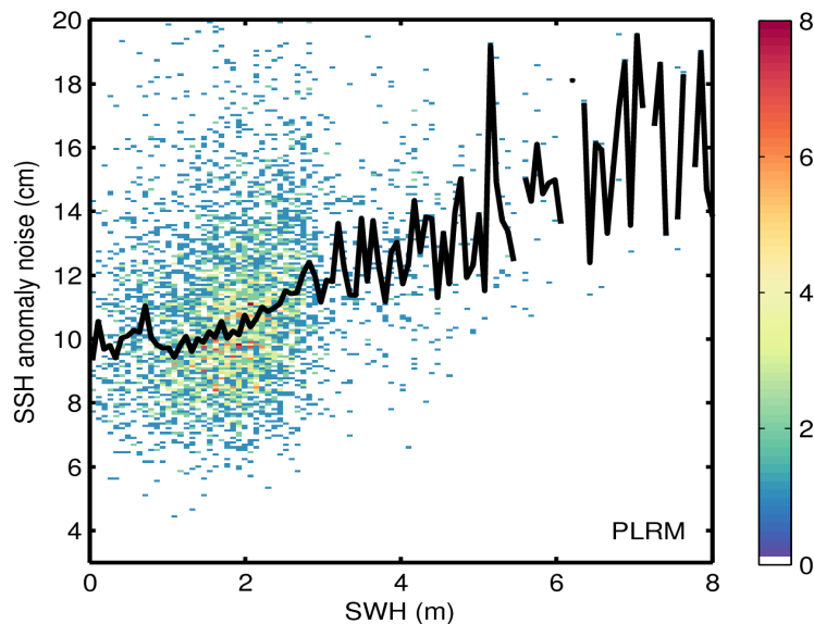
Figure 9. 2D histogram showing flag-valid SSH anomaly noise as a function of SWH for LRM (top) and PLRM (bottom) for 22/04/2017. The black line denotes the median SSH anomaly noise as a function of SWH.
