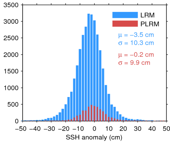
Figure 11. Histogram of science-valid SSH anomaly over oceans and lakes for LRM (blue) and PLRM (red) for 22/04/2017. The mean ( \mu ) and standard deviation ( \sigma ) are also shown. Note that values outside [-50 50] cm are excluded from the histogram for the sake of readability but not from the computation of \mu and \sigma .
