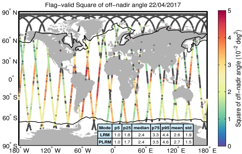
Figure 37. Geographical distribution of flag-valid mispointing data over oceans and lakes for 22/04/2017. The statistical values shown in the table refer to the mispointing in 10^{-2} deg 2 and are calculated separately for LRM and PLRM regions. Measurements taken over polar polygons have been excluded from the computation of the statistical values. The black lines mark the outer limit of the Arctic and Antarctic polar polygons. Gray circles denote negative values.
