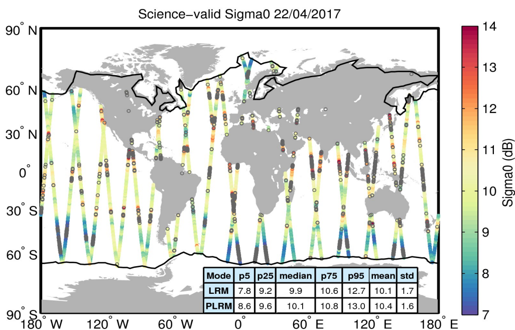
Figure 27. Geographical distribution of science-valid sigma0 data over oceans and lakes for 22/04/2017. The statistical values shown in the table refer to the sigma0 in dB and are calculated separately for LRM and PLRM regions. The black lines mark the outer limit of the Arctic and Antarctic polar polygons. Gray circles denote records that have been rejected based on the editing criteria described in Table 4.
