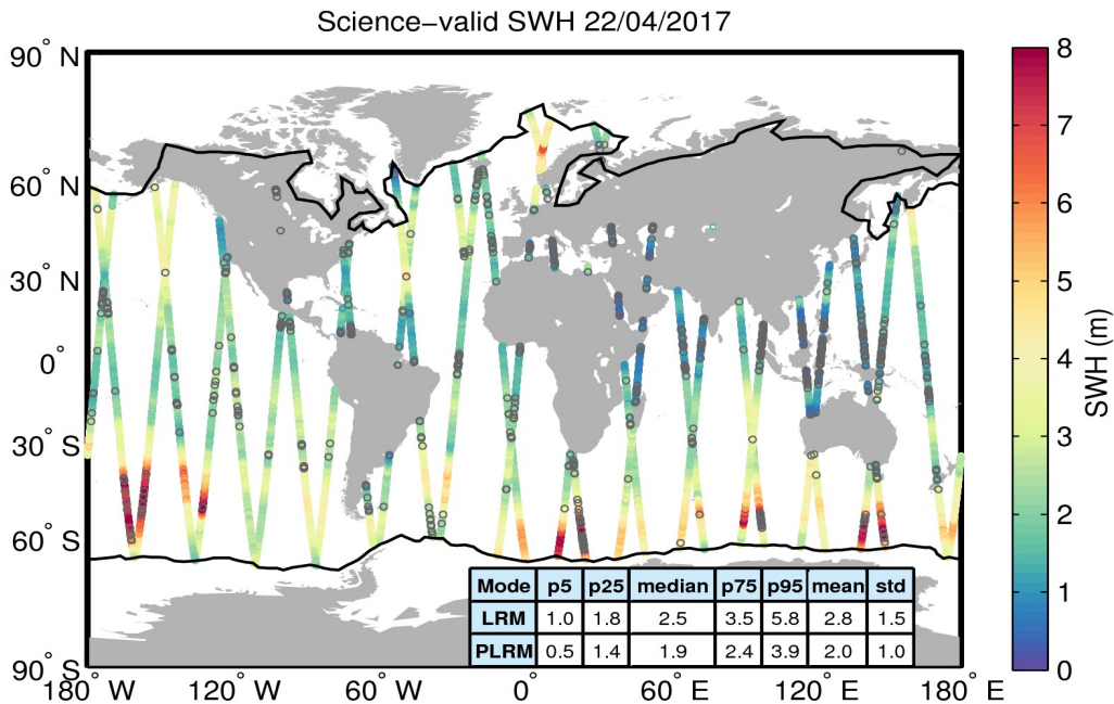
Figure 19. Geographical distribution of science-valid SWH data over oceans and lakes for 22/04/2017. The statistical values shown in the table refer to the SWH in m and are calculated separately for LRM and PLRM regions. The black lines mark the outer limit of the Arctic and Antarctic polar polygons. Gray circles denote records that have been rejected based on the editing criteria described in Table 3.
