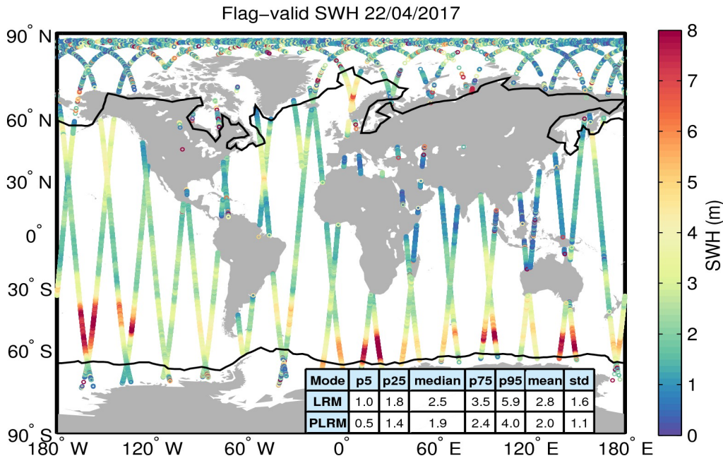
Figure 15. Geographical distribution of flag-valid SWH data over oceans and lakes for 22/04/2017. The statistical values shown in the table refer to the SWH in m and are calculated separately for LRM and PLRM regions. Measurements taken over polar polygons have been excluded from the computation of the statistical values. The black lines mark the outer limit of the Arctic and Antarctic polar polygons.
