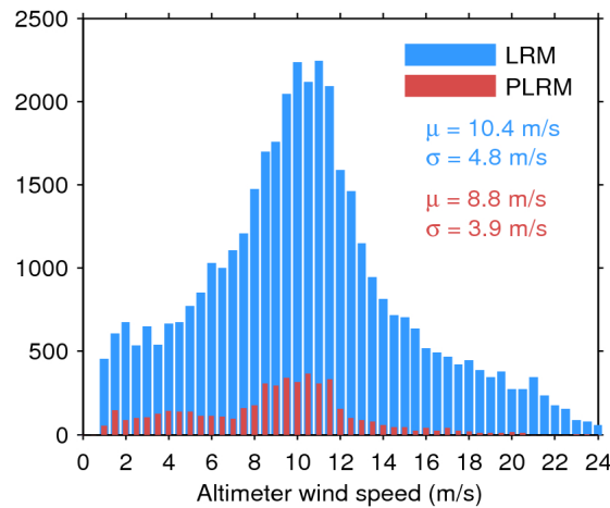
Figure 33. Histogram of flag-valid wind over oceans and lakes for LRM (blue) and PLRM (red) for 22/04/2017. The mean ( \mu ) and standard deviation ( \sigma ) are also shown. Note that values larger than 24 m/s are excluded from the histogram for the sake of readability but not from the computation of \mu and \sigma .
