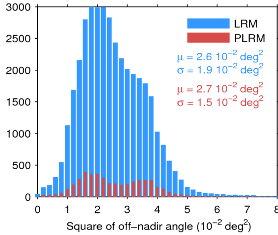
Figure 39. Histogram of flag-valid mispointing over oceans and lakes for LRM (blue) and PLRM (red) for 22/04/2017. Only positive values have been considered. The mean ( \mu ) and standard deviation ( \sigma ) are also shown. Note that values larger than 8 \cdot 10^{-2} \text{ deg}^2 are excluded from the histogram for the sake of readability but not from the computation of \mu and \sigma .
