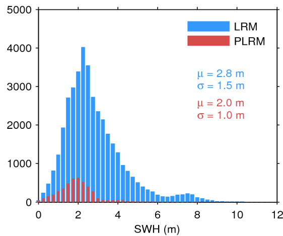
Figure 20. Histogram of science-valid SWH over oceans and lakes for LRM (blue) and PLRM (red) for 22/04/2017. The mean ( \mu ) and standard deviation ( \sigma ) are also shown. Note that values larger than 12 m are excluded from the histogram for the sake of readability but not from the computation of \mu and \sigma .
