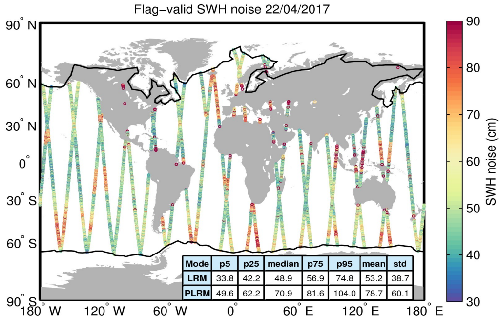
Figure 18. Geographical distribution of flag-valid 20-Hz SWH measurement noise over oceans and lakes for 22/04/2017. The statistical values shown in the table refer to the SWH noise and are calculated separately for LRM and PLRM regions. Measurements taken over polar polygons have been excluded from the computation of the statistical values. The black lines mark the outer limit of the Arctic and Antarctic polar polygons.
