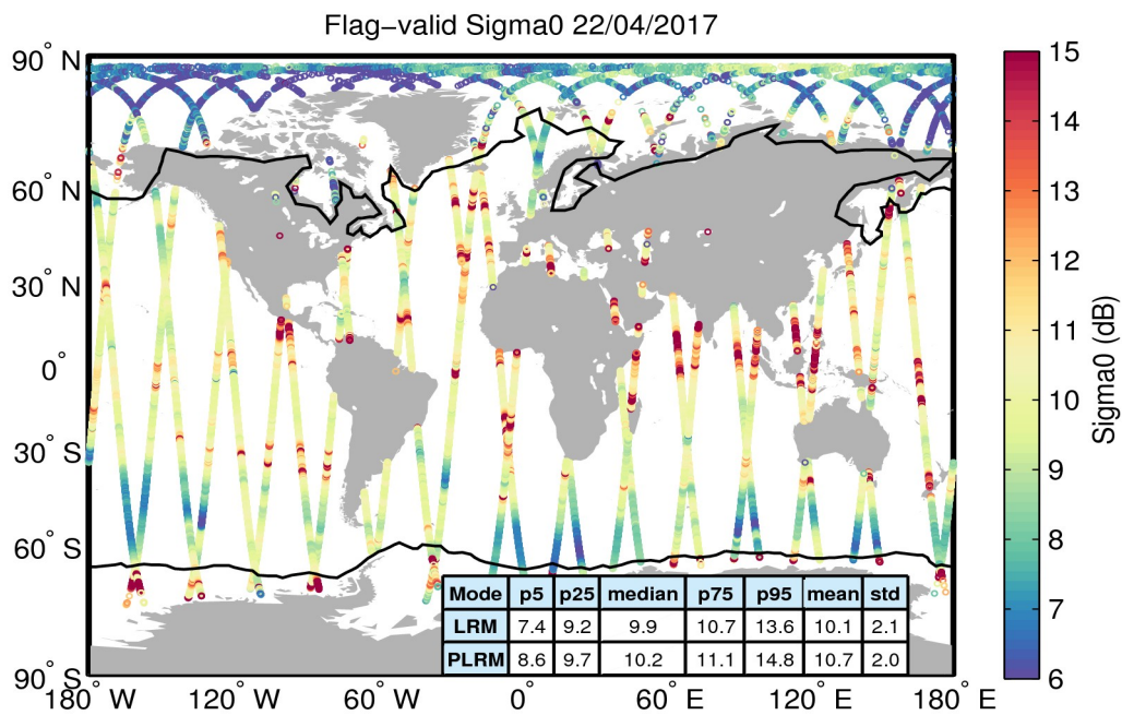
Figure 23. Geographical distribution of flag-valid sigma0 data over oceans and lakes for 22/04/2017. The statistical values shown in the table refer to the sigma0 in dB and are calculated separately for LRM and PLRM regions. Measurements taken over polar polygons have been excluded from the computation of the statistical values. The black lines mark the outer limit of the Arctic and Antarctic polar polygons.
