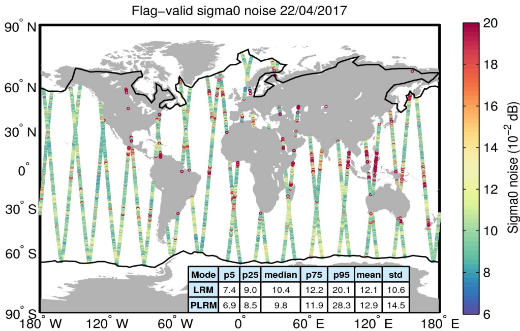
Figure 26. Geographical distribution of flag-valid 20-Hz sigma0 measurement noise over oceans and lakes for 22/04/2017. The statistical values shown in the table refer to the sigma0 noise and are calculated separately for LRM and PLRM regions. Measurements taken over polar polygons have been excluded from the computation of the statistical values. The black lines mark the outer limit of the Arctic and Antarctic polar polygons.
