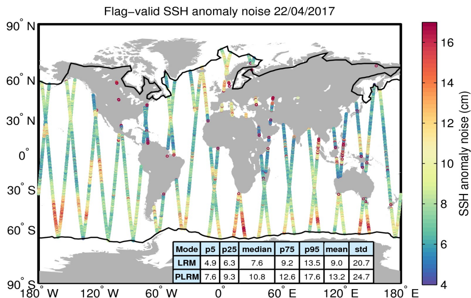
Figure 8. Geographical distribution of flag-valid 20-Hz SSH anomaly measurement noise over oceans and lakes for 22/04/2017. The statistical values shown in the table refer to the SSH anomaly noise and are calculated separately for LRM and PLRM regions. Measurements taken over polar polygons have been excluded from the computation of the statistical values. The black lines mark the outer limit of the Arctic and Antarctic polar polygons.
