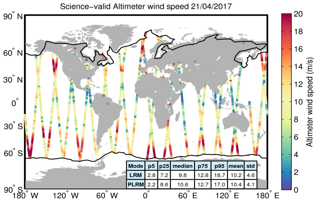
Figure 34. Geographical distribution of science-valid wind data over oceans and lakes for 21/04/2017. The statistical values shown in the table refer to the wind in m/s and are calculated separately for LRM and PLRM regions. The black lines mark the outer limit of the Arctic and Antarctic polar polygons. Gray circles denote records that have been rejected based on the editing criteria described in Table 5.
