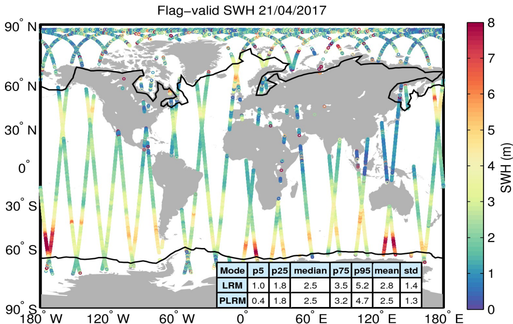
Figure 15. Geographical distribution of flag-valid SWH data over oceans and lakes for 21/04/2017. The statistical values shown in the table refer to the SWH in m and are calculated separately for LRM and PLRM regions. Measurements taken over polar polygons have been excluded from the computation of the statistical values. The black lines mark the outer limit of the Arctic and Antarctic polar polygons.
