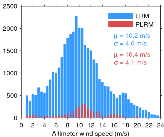
Figure 33. Histogram of flag-valid wind over oceans and lakes for LRM (blue) and PLRM (red) for 21/04/2017. The mean ( \mu ) and standard deviation ( \sigma ) are also shown. Note that values larger than 24 m/s are excluded from the histogram for the sake of readability but not from the computation of \mu and \sigma .
