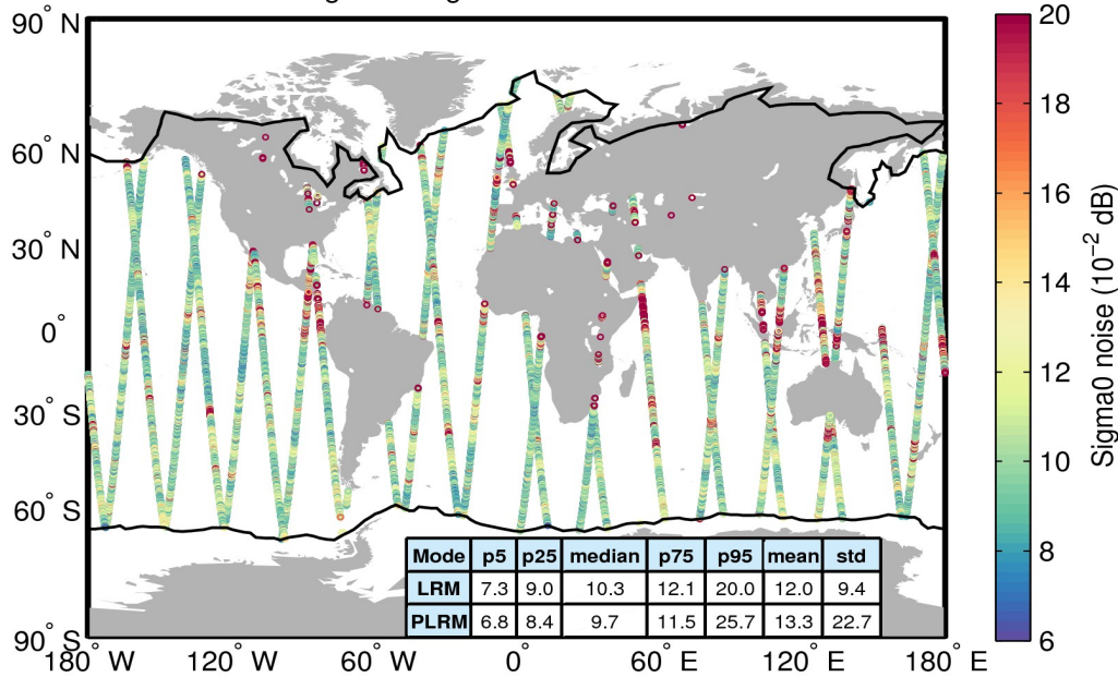
Flag-valid sigma0 noise 21/04/2017
