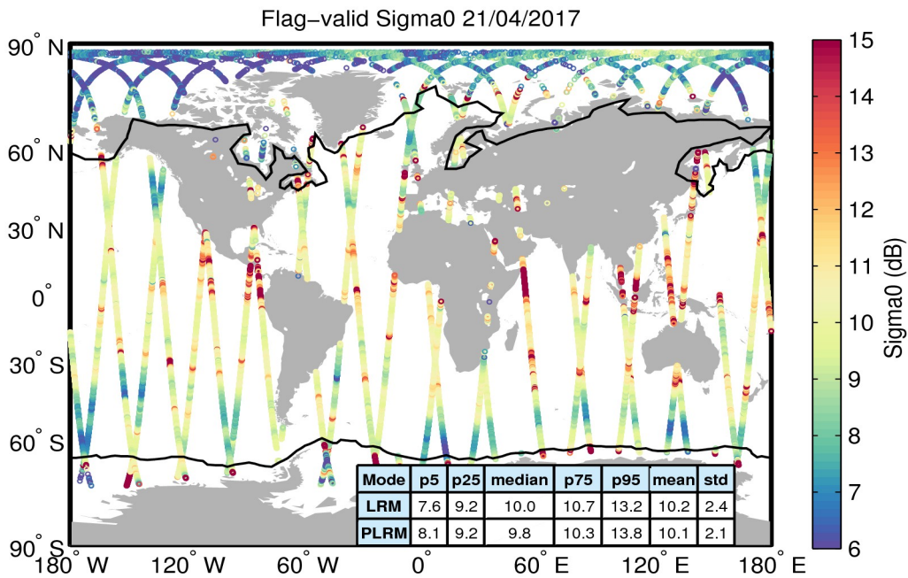
Figure 23. Geographical distribution of flag-valid sigma0 data over oceans and lakes for 21/04/2017. The statistical values shown in the table refer to the sigma0 in dB and are calculated separately for LRM and PLRM regions. Measurements taken over polar polygons have been excluded from the computation of the statistical values. The black lines mark the outer limit of the Arctic and Antarctic polar polygons.
