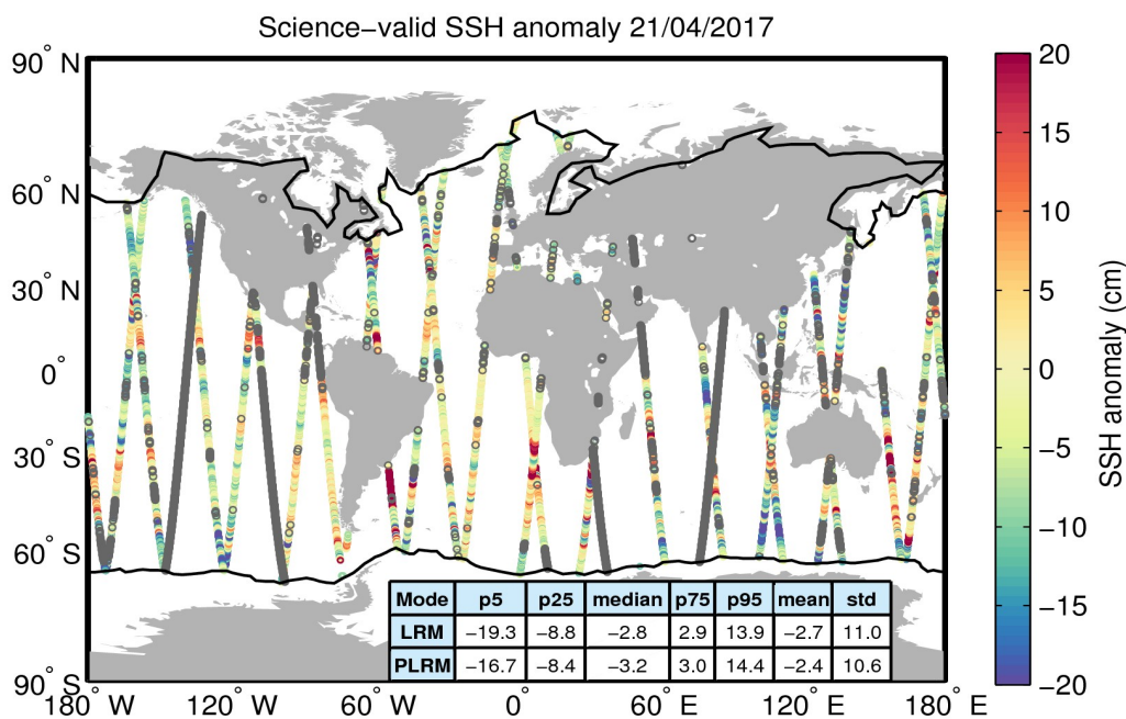
Figure 10. Geographical distribution of science-valid SSH anomaly data over oceans and lakes for 21/04/2017. The statistical values shown in the table refer to the SSH anomaly in cm and are calculated separately for LRM and PLRM regions. The black lines mark the outer limit of the Arctic and Antarctic polar polygons. Gray circles denote records that have been rejected based on the editing criteria described in Table 2.
