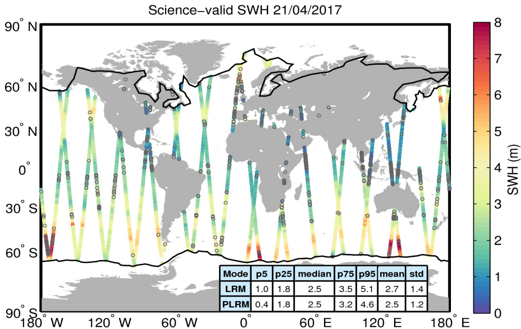
Figure 19. Geographical distribution of science-valid SWH data over oceans and lakes for 21/04/2017. The statistical values shown in the table refer to the SWH in m and are calculated separately for LRM and PLRM regions. The black lines mark the outer limit of the Arctic and Antarctic polar polygons. Gray circles denote records that have been rejected based on the editing criteria described in Table 3.
