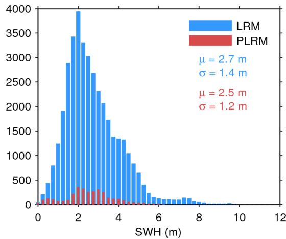
Figure 20. Histogram of science-valid SWH over oceans and lakes for LRM (blue) and PLRM (red) for 21/04/2017. The mean ( \mu ) and standard deviation ( \sigma ) are also shown. Note that values larger than 12 m are excluded from the histogram for the sake of readability but not from the computation of \mu and \sigma .
