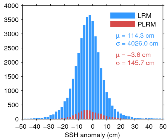
Figure 7. Histogram of flag-valid SSH anomaly over oceans and lakes for LRM (blue) and PLRM (red) for 21/04/2017. The mean ( \mu ) and standard deviation ( \sigma ) are also shown. Note that values outside [-50 50] cm are excluded from the histogram for the sake of readability but not from the computation of \mu and \sigma .
