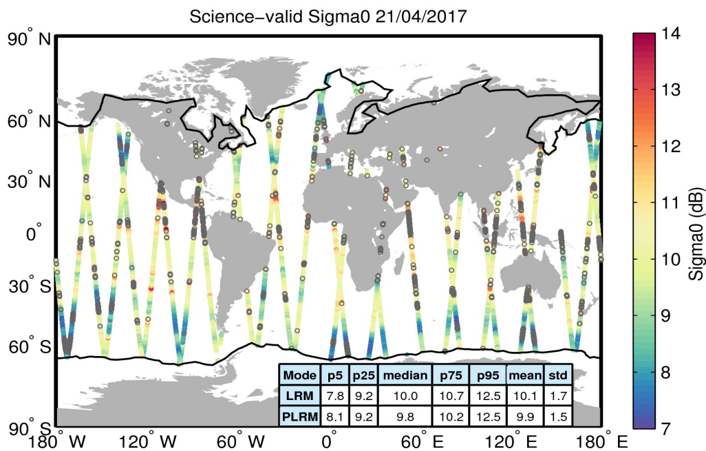
Figure 27. Geographical distribution of science-valid sigma0 data over oceans and lakes for 21/04/2017. The statistical values shown in the table refer to the sigma0 in dB and are calculated separately for LRM and PLRM regions. The black lines mark the outer limit of the Arctic and Antarctic polar polygons. Gray circles denote records that have been rejected based on the editing criteria described in Table 4.
