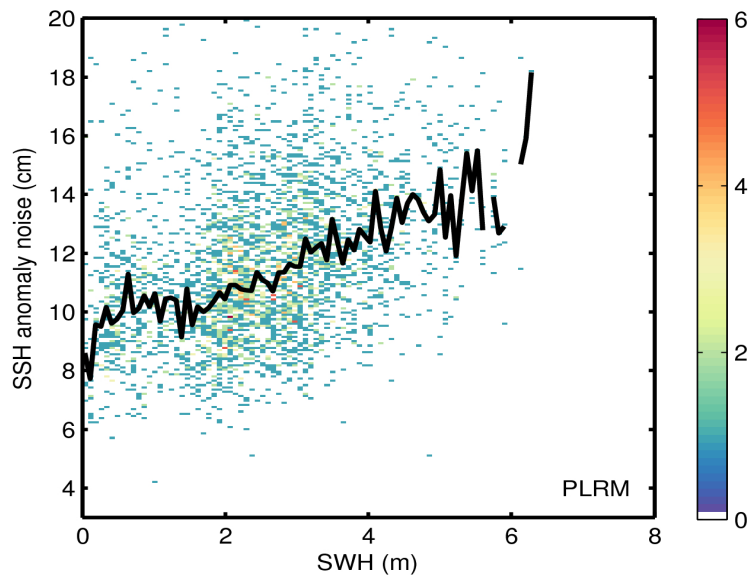
Figure 9. 2D histogram showing flag-valid SSH anomaly noise as a function of SWH for LRM (top) and PLRM (bottom) for 21/04/2017. The black line denotes the median SSH anomaly noise as a function of SWH.
