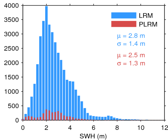
Figure 17. Histogram of flag-valid SWH over oceans and lakes for LRM (blue) and PLRM (red) for 21/04/2017. The mean ( \mu ) and standard deviation ( \sigma ) are also shown. Note that values larger than 12 m are excluded from the histogram for the sake of readability but not from the computation of \mu and \sigma .
