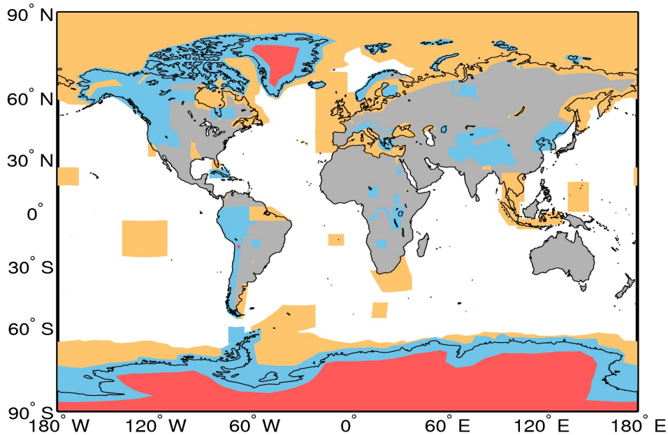
Figure A1. Extent of the regions defining the geographical mode mask for 21/04/2017. The regions where SAR, and SARIn are operated are denoted by the orange and blue polygons, respectively. LRM is operated over areas of the continental ice sheets (red polygons) and over oceans and land not covered by other modes.
