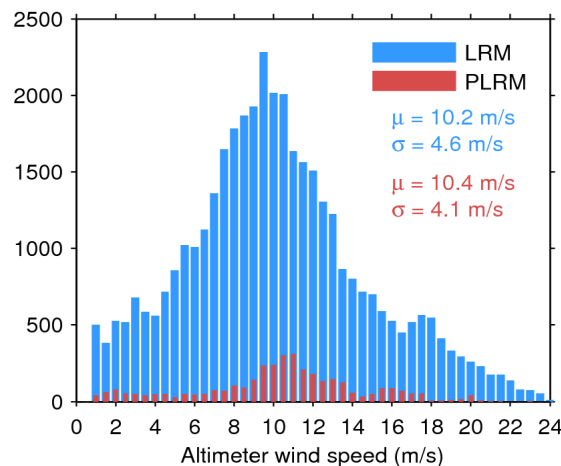
Figure 35. Histogram of science-valid wind over oceans and lakes for LRM (blue) and PLRM (red) for 21/04/2017. The mean ( \mu ) and standard deviation ( \sigma ) are also shown. Note that values larger than 24 m/s are excluded from the histogram for the sake of readability but not from the computation of \mu and \sigma .
