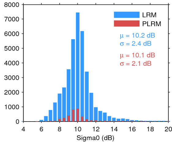
Figure 25. Histogram of flag-valid sigma0 over oceans and lakes for LRM (blue) and PLRM (red) for 21/04/2017. The mean ( \mu ) and standard deviation ( \sigma ) are also shown. Note that values outside [4 20] dB are excluded from the histogram for the sake of readability but not from the computation of \mu and \sigma .
