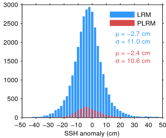
Figure 11. Histogram of science-valid SSH anomaly over oceans and lakes for LRM (blue) and PLRM (red) for 21/04/2017. The mean ( \mu ) and standard deviation ( \sigma ) are also shown. Note that values outside [-50 50] cm are excluded from the histogram for the sake of readability but not from the computation of \mu and \sigma .
