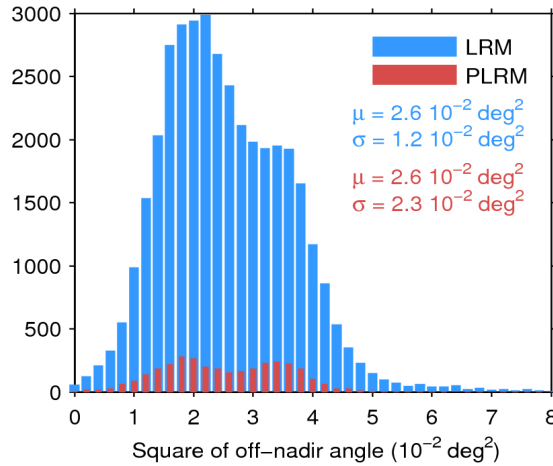
Figure 39. Histogram of flag-valid mispointing over oceans and lakes for LRM (blue) and PLRM (red) for 21/04/2017. Only positive values have been considered. The mean ( \mu ) and standard deviation ( \sigma ) are also shown. Note that values larger than 8 \times 10^{-2} \text{ deg}^2 are excluded from the histogram for the sake of readability but not from the computation of \mu and \sigma .
