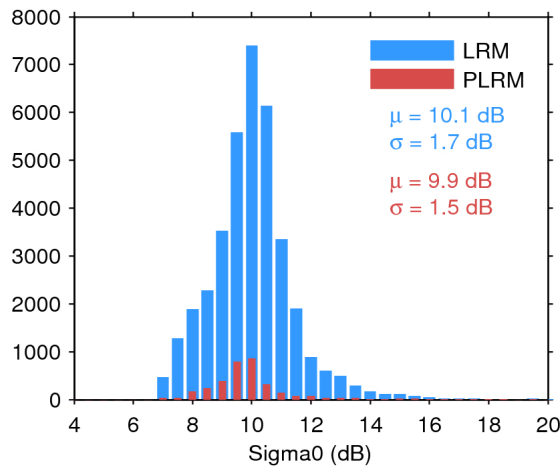
Figure 28. Histogram of science-valid sigma0 over oceans and lakes for LRM (blue) and PLRM (red) for 21/04/2017. The mean ( \mu ) and standard deviation ( \sigma ) are also shown. Note that values outside [4 20] dB are excluded from the histogram for the sake of readability but not from the computation of \mu and \sigma .
