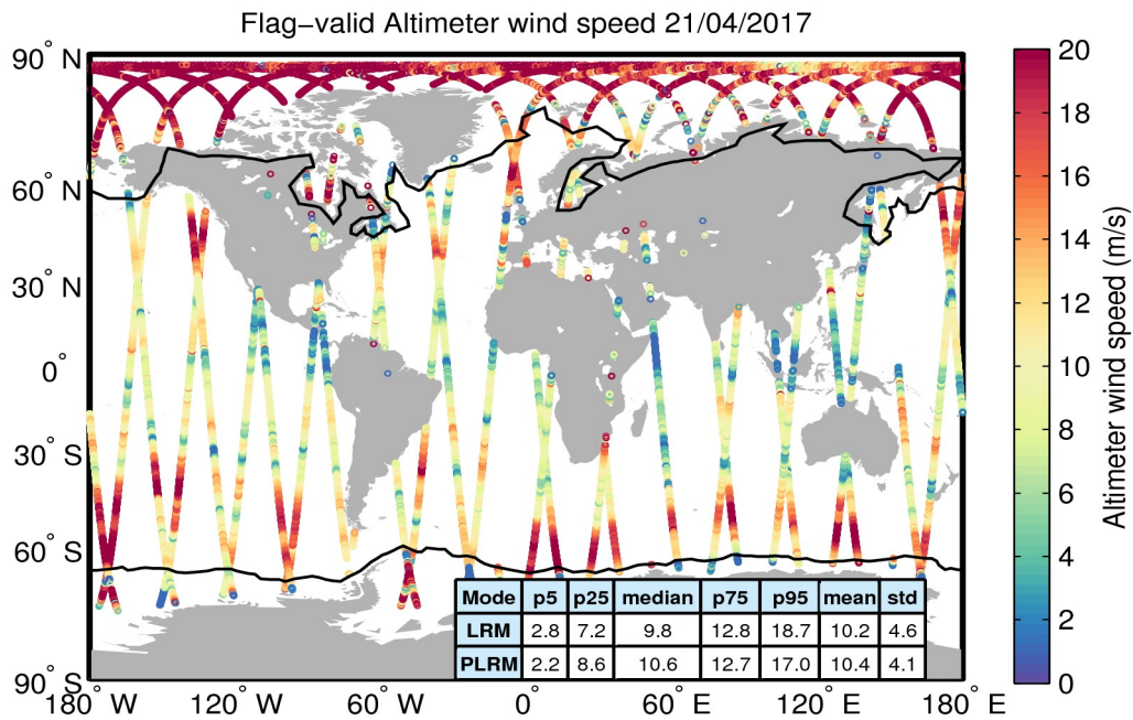
Figure 31. Geographical distribution of flag-valid wind data over oceans and lakes for 21/04/2017. The statistical values shown in the table refer to the wind in m/s and are calculated separately for LRM and PLRM regions. Measurements taken over polar polygons have been excluded from the computation of the statistical values. The black lines mark the outer limit of the Arctic and Antarctic polar polygons.
