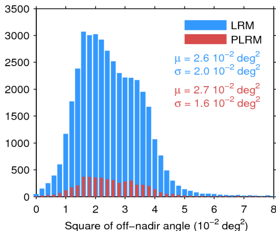
Figure 39. Histogram of flag-valid mispointing over oceans and lakes for LRM (blue) and PLRM (red) for 18/04/2017. Only positive values have been considered. The mean ( \mu ) and standard deviation ( \sigma ) are also shown. Note that values larger than 8 \cdot 10^{-2} \text{ deg}^2 are excluded from the histogram for the sake of readability but not from the computation of \mu and \sigma .
