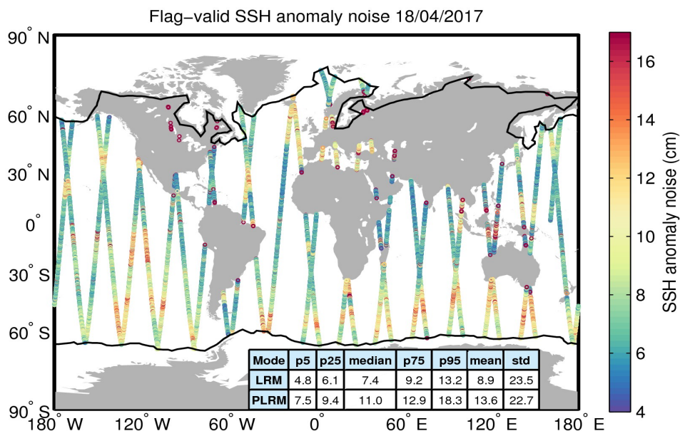
Figure 8. Geographical distribution of flag-valid 20-Hz SSH anomaly measurement noise over oceans and lakes for 18/04/2017. The statistical values shown in the table refer to the SSH anomaly noise and are calculated separately for LRM and PLRM regions. Measurements taken over polar polygons have been excluded from the computation of the statistical values. The black lines mark the outer limit of the Arctic and Antarctic polar polygons.
