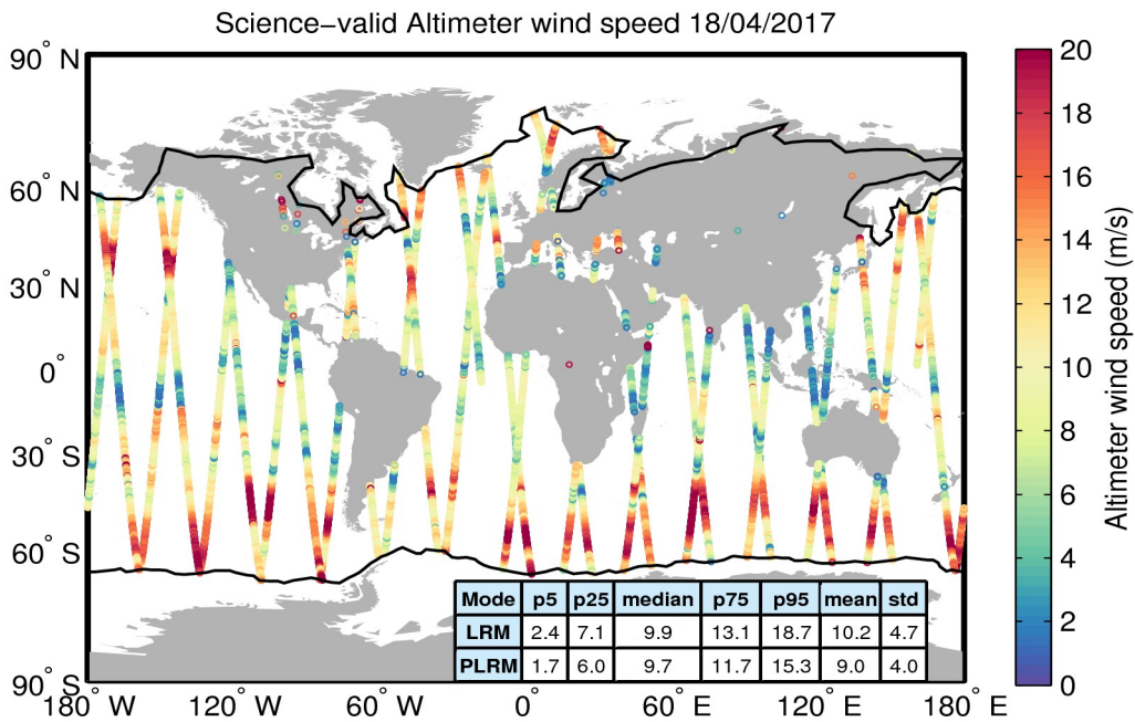
Figure 34. Geographical distribution of science-valid wind data over oceans and lakes for 18/04/2017. The statistical values shown in the table refer to the wind in m/s and are calculated separately for LRM and PLRM regions. The black lines mark the outer limit of the Arctic and Antarctic polar polygons. Gray circles denote records that have been rejected based on the editing criteria described in Table 5.
