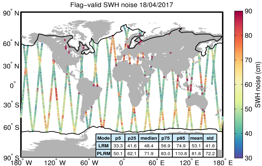
Figure 18. Geographical distribution of flag-valid 20-Hz SWH measurement noise over oceans and lakes for 18/04/2017. The statistical values shown in the table refer to the SWH noise and are calculated separately for LRM and PLRM regions. Measurements taken over polar polygons have been excluded from the computation of the statistical values. The black lines mark the outer limit of the Arctic and Antarctic polar polygons.
