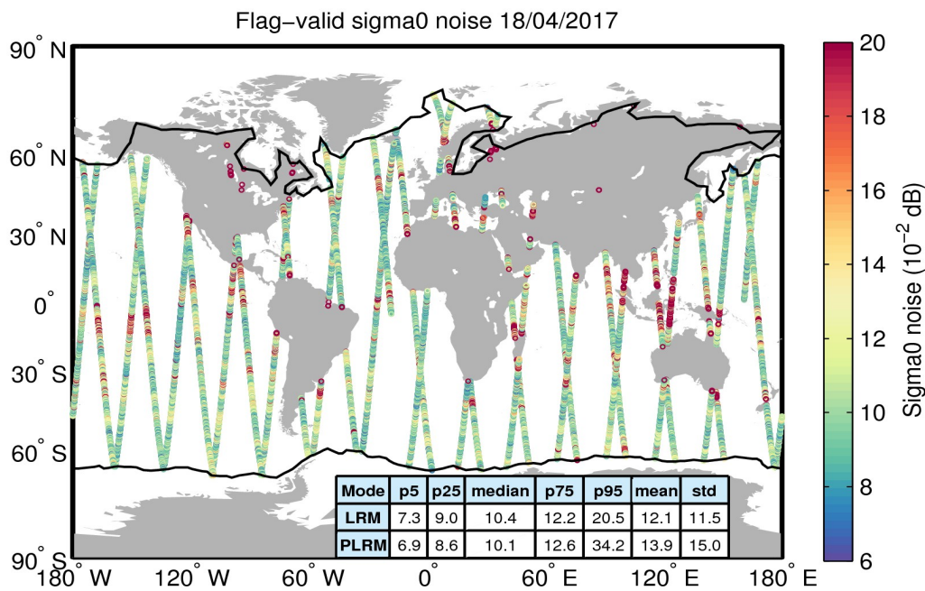
Figure 26. Geographical distribution of flag-valid 20-Hz sigma0 measurement noise over oceans and lakes for 18/04/2017. The statistical values shown in the table refer to the sigma0 noise and are calculated separately for LRM and PLRM regions. Measurements taken over polar polygons have been excluded from the computation of the statistical values. The black lines mark the outer limit of the Arctic and Antarctic polar polygons.
