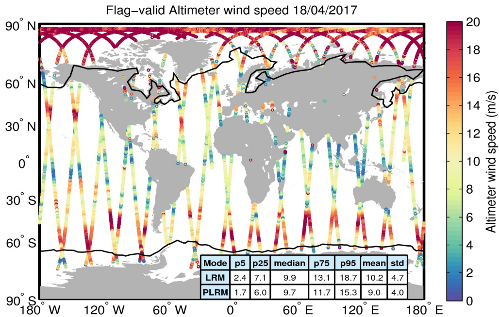
Figure 31. Geographical distribution of flag-valid wind data over oceans and lakes for 18/04/2017. The statistical values shown in the table refer to the wind in m/s and are calculated separately for LRM and PLRM regions. Measurements taken over polar polygons have been excluded from the computation of the statistical values. The black lines mark the outer limit of the Arctic and Antarctic polar polygons.
