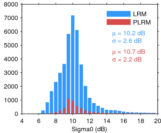
Figure 25. Histogram of flag-valid sigma0 over oceans and lakes for LRM (blue) and PLRM (red) for 18/04/2017. The mean ( \mu ) and standard deviation ( \sigma ) are also shown. Note that values outside [4 20] dB are excluded from the histogram for the sake of readability but not from the computation of \mu and \sigma .
