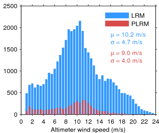
Figure 33. Histogram of flag-valid wind over oceans and lakes for LRM (blue) and PLRM (red) for 18/04/2017. The mean ( \mu ) and standard deviation ( \sigma ) are also shown. Note that values larger than 24 m/s are excluded from the histogram for the sake of readability but not from the computation of \mu and \sigma .
