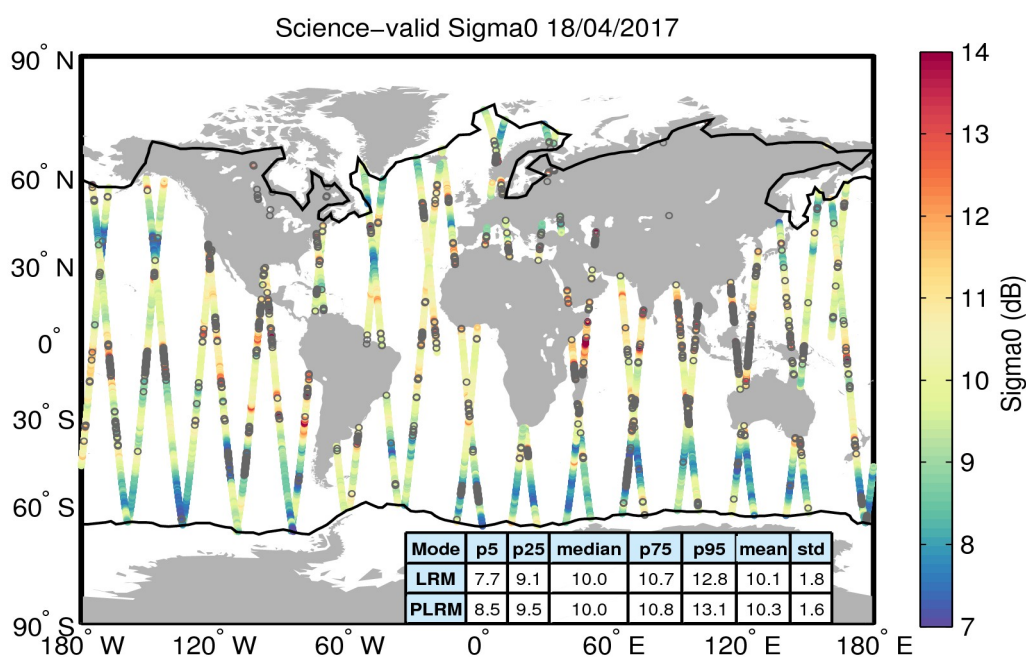
Figure 27. Geographical distribution of science-valid sigma0 data over oceans and lakes for 18/04/2017. The statistical values shown in the table refer to the sigma0 in dB and are calculated separately for LRM and PLRM regions. The black lines mark the outer limit of the Arctic and Antarctic polar polygons. Gray circles denote records that have been rejected based on the editing criteria described in Table 4.
