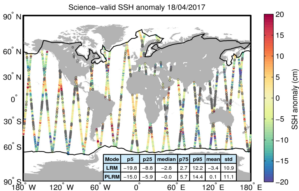
Figure 10. Geographical distribution of science-valid SSH anomaly data over oceans and lakes for 18/04/2017. The statistical values shown in the table refer to the SSH anomaly in cm and are calculated separately for LRM and PLRM regions. The black lines mark the outer limit of the Arctic and Antarctic polar polygons. Gray circles denote records that have been rejected based on the editing criteria described in Table 2.
