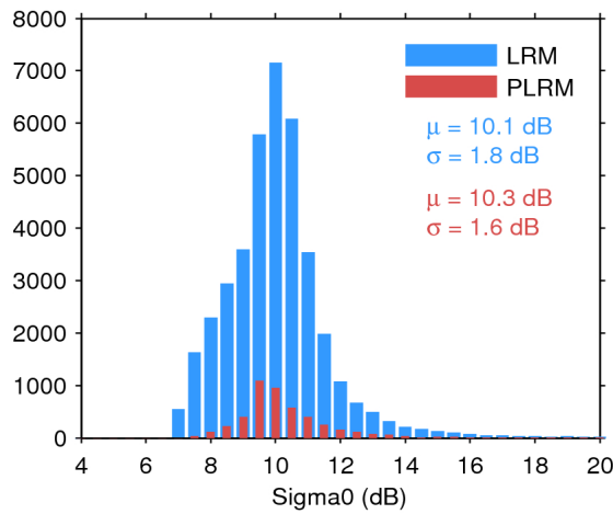
Figure 28. Histogram of science-valid sigma0 over oceans and lakes for LRM (blue) and PLRM (red) for 18/04/2017. The mean ( \mu ) and standard deviation ( \sigma ) are also shown. Note that values outside [4 20] dB are excluded from the histogram for the sake of readability but not from the computation of \mu and \sigma .
