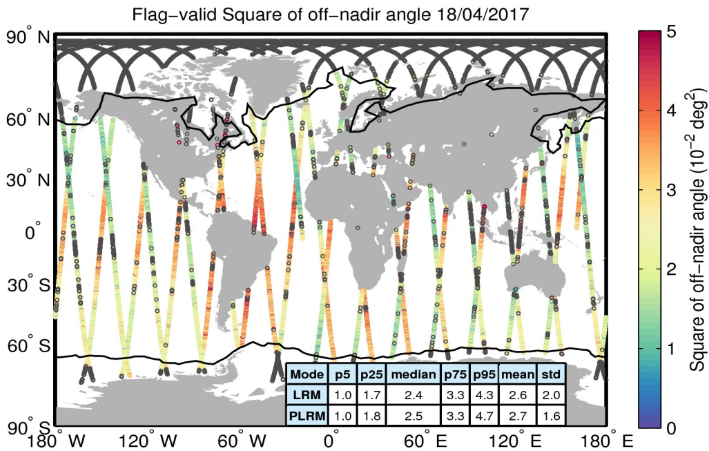
Figure 37. Geographical distribution of flag-valid mispointing data over oceans and lakes for 18/04/2017. The statistical values shown in the table refer to the mispointing in 10^{-2} deg 2 and are calculated separately for LRM and PLRM regions. Measurements taken over polar polygons have been excluded from the computation of the statistical values. The black lines mark the outer limit of the Arctic and Antarctic polar polygons. Gray circles denote negative values.
