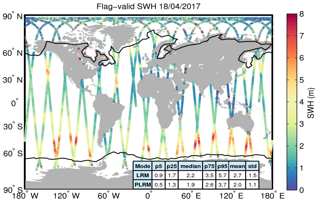
Figure 15. Geographical distribution of flag-valid SWH data over oceans and lakes for 18/04/2017. The statistical values shown in the table refer to the SWH in m and are calculated separately for LRM and PLRM regions. Measurements taken over polar polygons have been excluded from the computation of the statistical values. The black lines mark the outer limit of the Arctic and Antarctic polar polygons.
