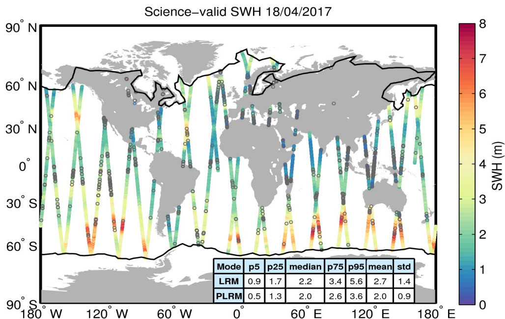
Figure 19. Geographical distribution of science-valid SWH data over oceans and lakes for 18/04/2017. The statistical values shown in the table refer to the SWH in m and are calculated separately for LRM and PLRM regions. The black lines mark the outer limit of the Arctic and Antarctic polar polygons. Gray circles denote records that have been rejected based on the editing criteria described in Table 3.
