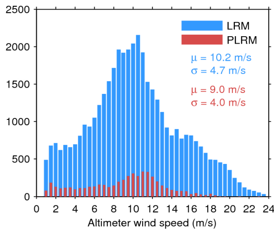
Figure 35. Histogram of science-valid wind over oceans and lakes for LRM (blue) and PLRM (red) for 18/04/2017. The mean ( \mu ) and standard deviation ( \sigma ) are also shown. Note that values larger than 24 m/s are excluded from the histogram for the sake of readability but not from the computation of \mu and \sigma .
