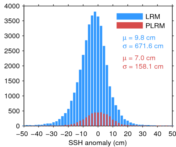
Figure 7. Histogram of flag-valid SSH anomaly over oceans and lakes for LRM (blue) and PLRM (red) for 18/04/2017. The mean ( \mu ) and standard deviation ( \sigma ) are also shown. Note that values outside [-50\ 50] cm are excluded from the histogram for the sake of readability but not from the computation of \mu and \sigma .
