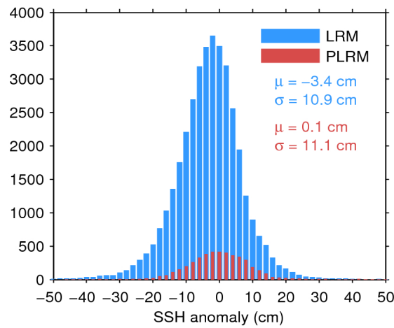
Figure 11. Histogram of science-valid SSH anomaly over oceans and lakes for LRM (blue) and PLRM (red) for 18/04/2017. The mean ( \mu ) and standard deviation ( \sigma ) are also shown. Note that values outside [-50\ 50] cm are excluded from the histogram for the sake of readability but not from the computation of \mu and \sigma .
