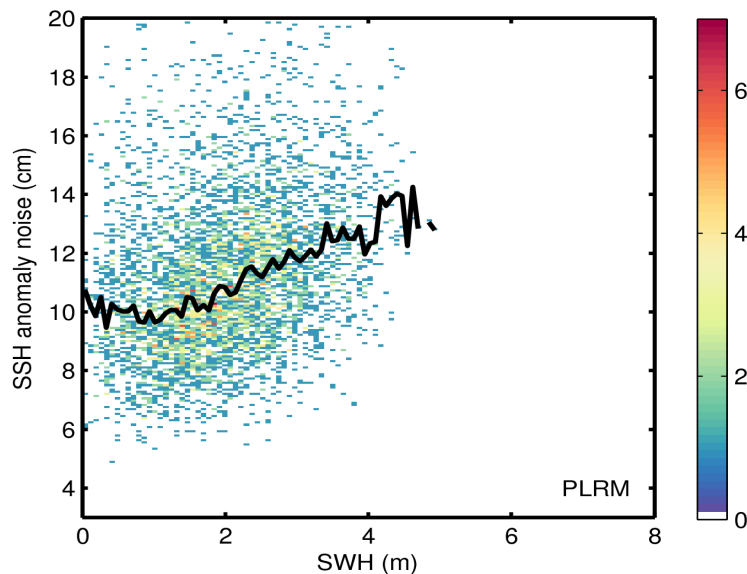
Figure 9. 2D histogram showing flag-valid SSH anomaly noise as a function of SWH for LRM (top) and PLRM (bottom) for 18/04/2017. The black line denotes the median SSH anomaly noise as a function of SWH.
