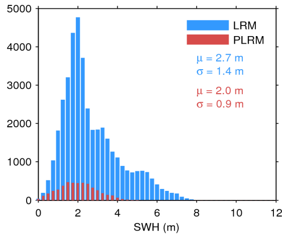
Figure 20. Histogram of science-valid SWH over oceans and lakes for LRM (blue) and PLRM (red) for 18/04/2017. The mean ( \mu ) and standard deviation ( \sigma ) are also shown. Note that values larger than 12 m are excluded from the histogram for the sake of readability but not from the computation of \mu and \sigma .
