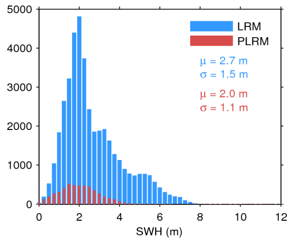
Figure 17. Histogram of flag-valid SWH over oceans and lakes for LRM (blue) and PLRM (red) for 18/04/2017. The mean ( \mu ) and standard deviation ( \sigma ) are also shown. Note that values larger than 12 m are excluded from the histogram for the sake of readability but not from the computation of \mu and \sigma .
