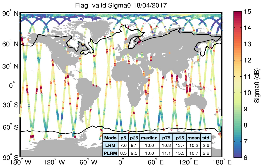
Figure 23. Geographical distribution of flag-valid sigma0 data over oceans and lakes for 18/04/2017. The statistical values shown in the table refer to the sigma0 in dB and are calculated separately for LRM and PLRM regions. Measurements taken over polar polygons have been excluded from the computation of the statistical values. The black lines mark the outer limit of the Arctic and Antarctic polar polygons.
