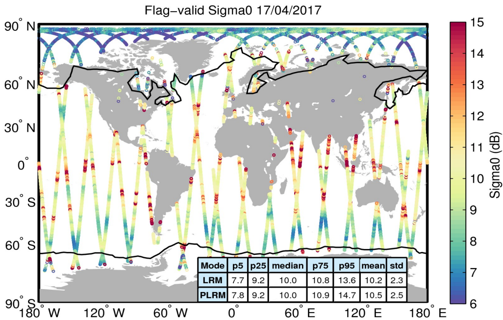
Figure 23. Geographical distribution of flag-valid sigma0 data over oceans and lakes for 17/04/2017. The statistical values shown in the table refer to the sigma0 in dB and are calculated separately for LRM and PLRM regions. Measurements taken over polar polygons have been excluded from the computation of the statistical values. The black lines mark the outer limit of the Arctic and Antarctic polar polygons.
