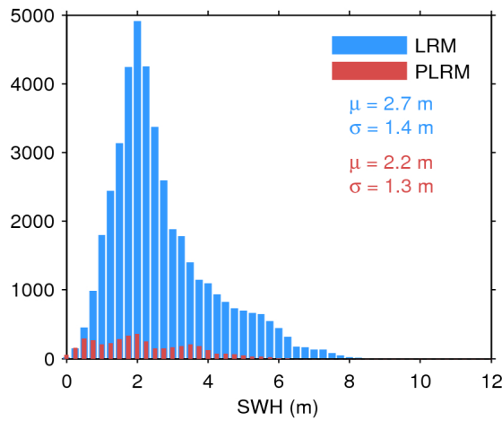
Figure 20. Histogram of science-valid SWH over oceans and lakes for LRM (blue) and PLRM (red) for 17/04/2017. The mean ( \mu ) and standard deviation ( \sigma ) are also shown. Note that values larger than 12 m are excluded from the histogram for the sake of readability but not from the computation of \mu and \sigma .
