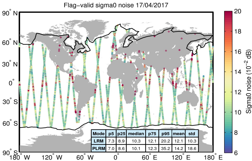
Figure 26. Geographical distribution of flag-valid 20-Hz sigma0 measurement noise over oceans and lakes for 17/04/2017. The statistical values shown in the table refer to the sigma0 noise and are calculated separately for LRM and PLRM regions. Measurements taken over polar polygons have been excluded from the computation of the statistical values. The black lines mark the outer limit of the Arctic and Antarctic polar polygons.
