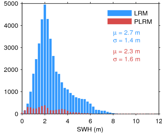
Figure 17. Histogram of flag-valid SWH over oceans and lakes for LRM (blue) and PLRM (red) for 17/04/2017. The mean ( \mu ) and standard deviation ( \sigma ) are also shown. Note that values larger than 12 m are excluded from the histogram for the sake of readability but not from the computation of \mu and \sigma .
