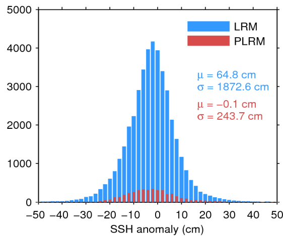
Figure 7. Histogram of flag-valid SSH anomaly over oceans and lakes for LRM (blue) and PLRM (red) for 17/04/2017. The mean ( \mu ) and standard deviation ( \sigma ) are also shown. Note that values outside [-50\ 50] cm are excluded from the histogram for the sake of readability but not from the computation of \mu and \sigma .
