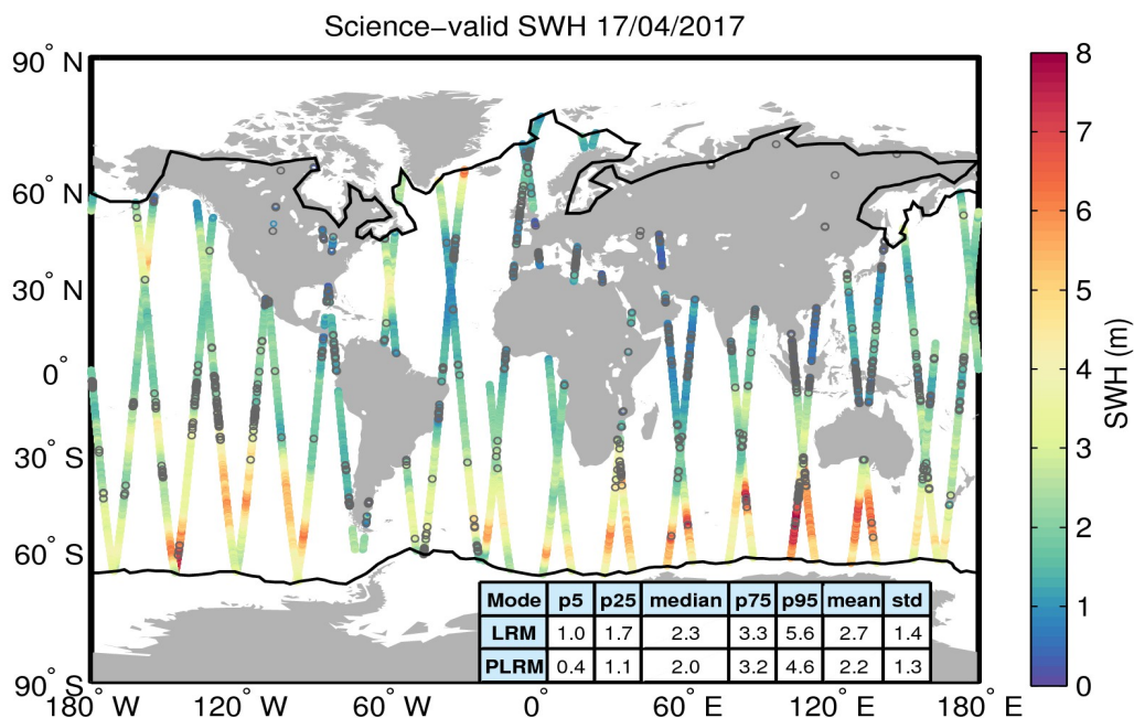
Figure 19. Geographical distribution of science-valid SWH data over oceans and lakes for 17/04/2017. The statistical values shown in the table refer to the SWH in m and are calculated separately for LRM and PLRM regions. The black lines mark the outer limit of the Arctic and Antarctic polar polygons. Gray circles denote records that have been rejected based on the editing criteria described in Table 3.
