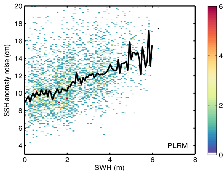
Figure 9. 2D histogram showing flag-valid SSH anomaly noise as a function of SWH for LRM (top) and PLRM (bottom) for 17/04/2017. The black line denotes the median SSH anomaly noise as a function of SWH.
