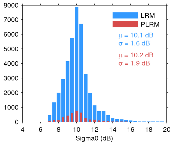
Figure 28. Histogram of science-valid sigma0 over oceans and lakes for LRM (blue) and PLRM (red) for 17/04/2017. The mean ( \mu ) and standard deviation ( \sigma ) are also shown. Note that values outside [4 20] dB are excluded from the histogram for the sake of readability but not from the computation of \mu and \sigma .
