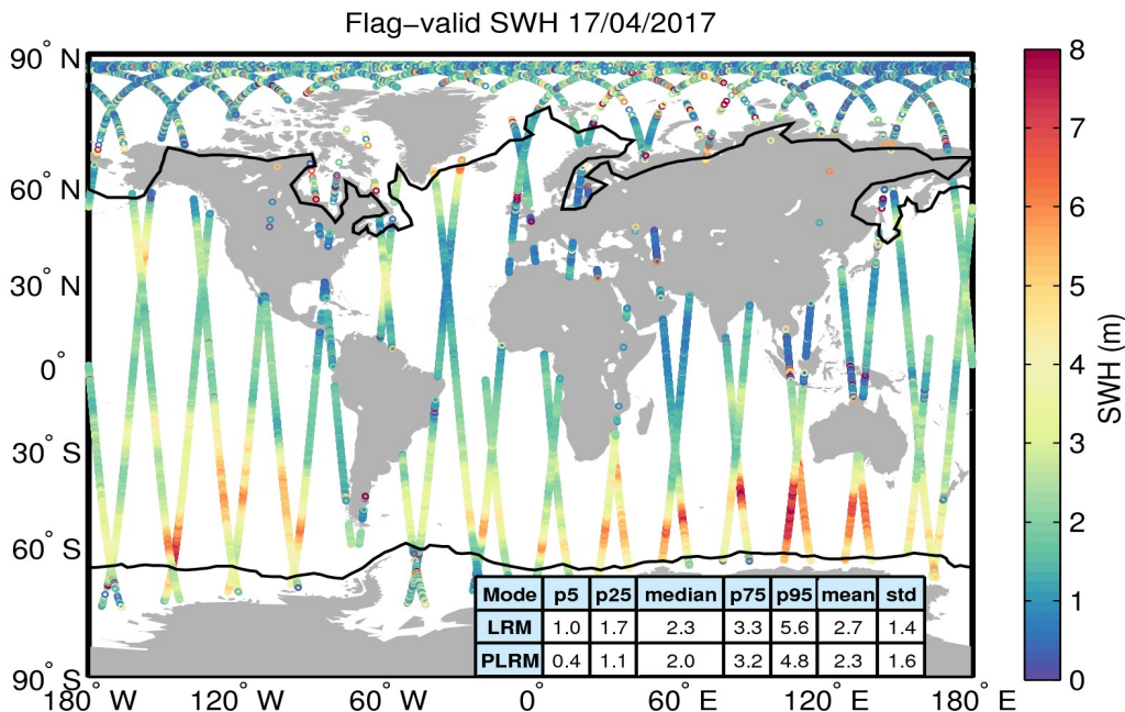
Figure 15. Geographical distribution of flag-valid SWH data over oceans and lakes for 17/04/2017. The statistical values shown in the table refer to the SWH in m and are calculated separately for LRM and PLRM regions. Measurements taken over polar polygons have been excluded from the computation of the statistical values. The black lines mark the outer limit of the Arctic and Antarctic polar polygons.
