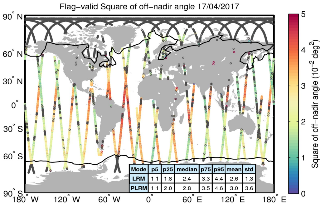
Figure 37. Geographical distribution of flag-valid mispointing data over oceans and lakes for 17/04/2017. The statistical values shown in the table refer to the mispointing in 10^{-2} deg 2 and are calculated separately for LRM and PLRM regions. Measurements taken over polar polygons have been excluded from the computation of the statistical values. The black lines mark the outer limit of the Arctic and Antarctic polar polygons. Gray circles denote negative values.
