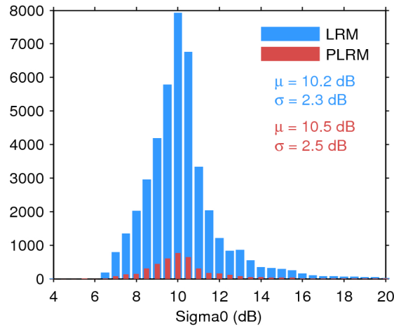
Figure 25. Histogram of flag-valid sigma0 over oceans and lakes for LRM (blue) and PLRM (red) for 17/04/2017. The mean ( \mu ) and standard deviation ( \sigma ) are also shown. Note that values outside [4 20] dB are excluded from the histogram for the sake of readability but not from the computation of \mu and \sigma .
