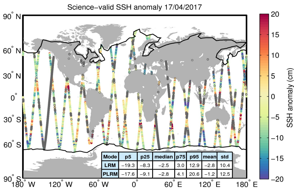
Figure 10. Geographical distribution of science-valid SSH anomaly data over oceans and lakes for 17/04/2017. The statistical values shown in the table refer to the SSH anomaly in cm and are calculated separately for LRM and PLRM regions. The black lines mark the outer limit of the Arctic and Antarctic polar polygons. Gray circles denote records that have been rejected based on the editing criteria described in Table 2.
