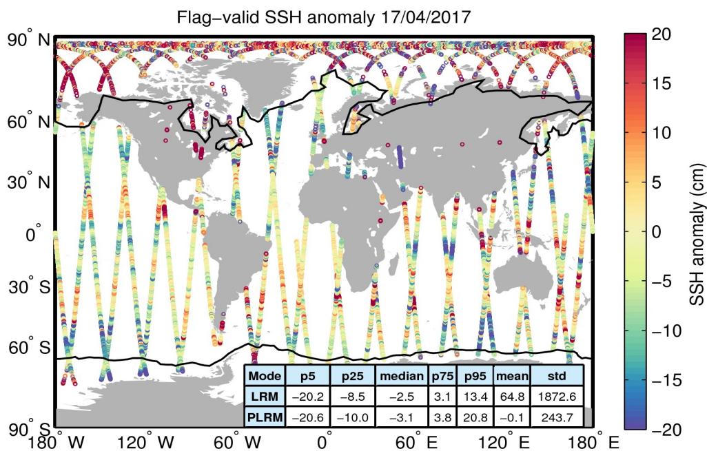
Figure 5. Geographical distribution of flag-valid 1-Hz SSH anomaly data over oceans and lakes for 17/04/2017. The statistical values shown in the table refer to the SSH anomaly in cm and are calculated separately for LRM and PLRM regions. Measurements taken over polar polygons have been excluded from the computation of the statistical values. The black lines mark the outer limit of the Arctic and Antarctic polar polygons.
