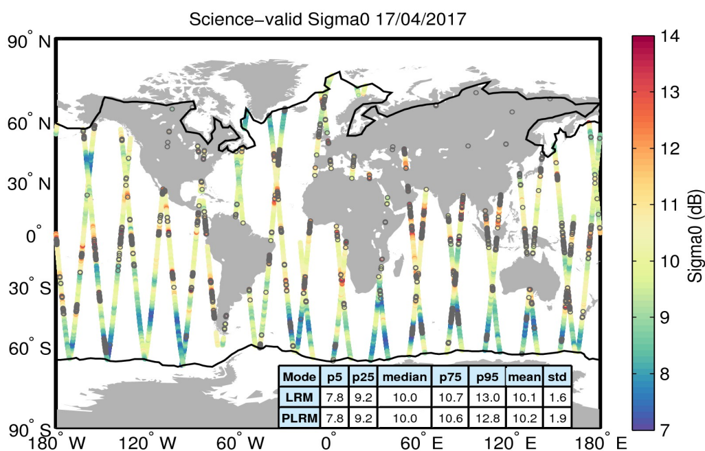
Figure 27. Geographical distribution of science-valid sigma0 data over oceans and lakes for 17/04/2017. The statistical values shown in the table refer to the sigma0 in dB and are calculated separately for LRM and PLRM regions. The black lines mark the outer limit of the Arctic and Antarctic polar polygons. Gray circles denote records that have been rejected based on the editing criteria described in Table 4.
