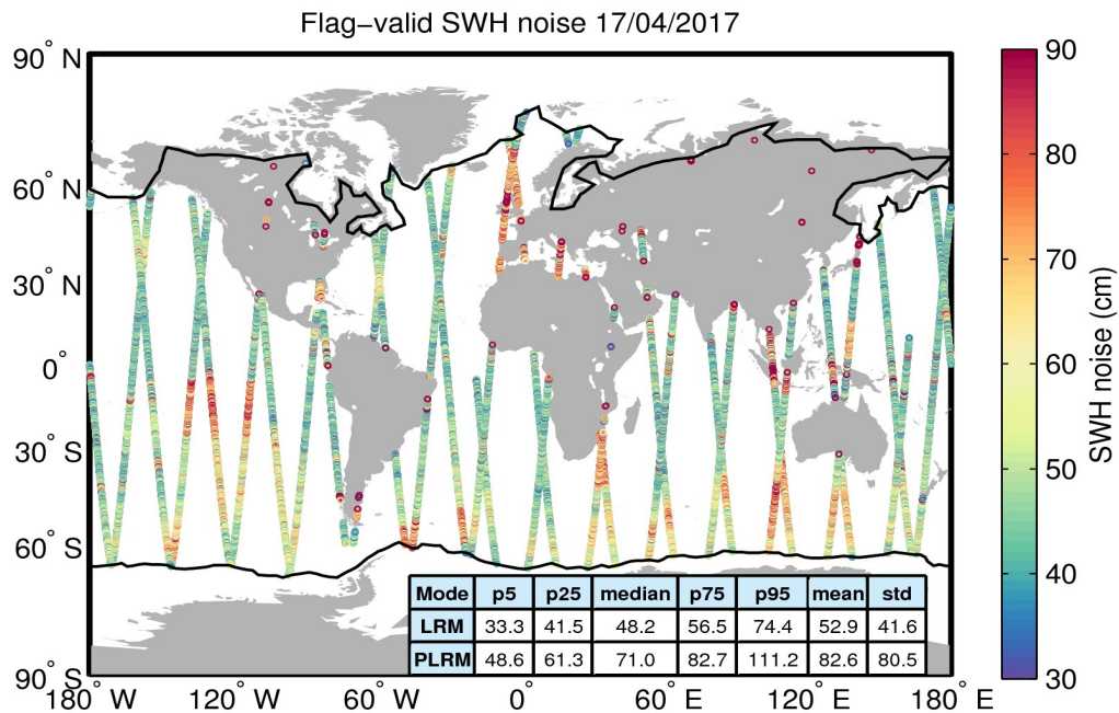
Figure 18. Geographical distribution of flag-valid 20-Hz SWH measurement noise over oceans and lakes for 17/04/2017. The statistical values shown in the table refer to the SWH noise and are calculated separately for LRM and PLRM regions. Measurements taken over polar polygons have been excluded from the computation of the statistical values. The black lines mark the outer limit of the Arctic and Antarctic polar polygons.
