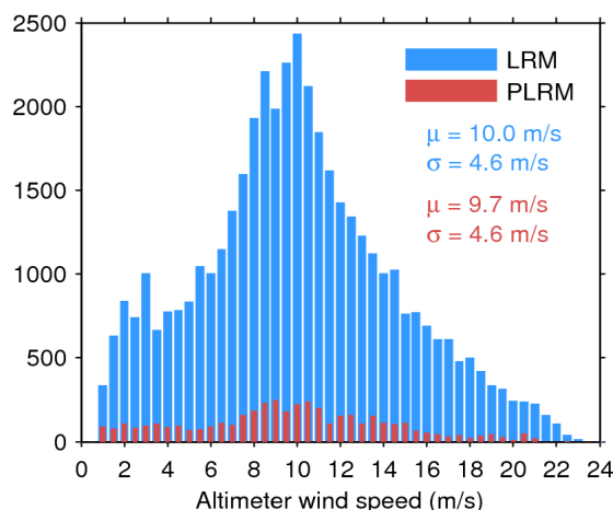
Figure 33. Histogram of flag-valid wind over oceans and lakes for LRM (blue) and PLRM (red) for 17/04/2017. The mean ( \mu ) and standard deviation ( \sigma ) are also shown. Note that values larger than 24 m/s are excluded from the histogram for the sake of readability but not from the computation of \mu and \sigma .
