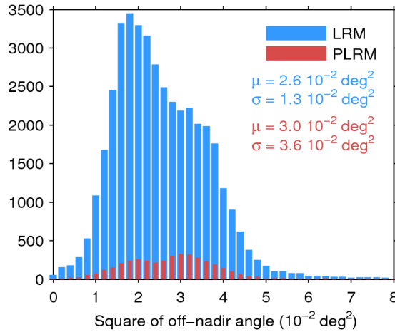
Figure 39. Histogram of flag-valid mispointing over oceans and lakes for LRM (blue) and PLRM (red) for 17/04/2017. Only positive values have been considered. The mean ( \mu ) and standard deviation ( \sigma ) are also shown. Note that values larger than 8 \cdot 10^{-2} \text{ deg}^2 are excluded from the histogram for the sake of readability but not from the computation of \mu and \sigma .
