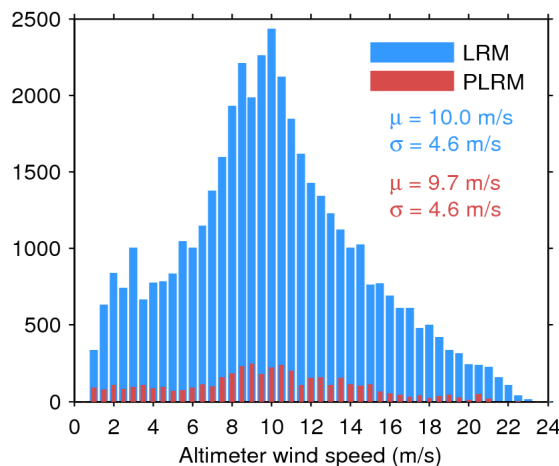
Figure 35. Histogram of science-valid wind over oceans and lakes for LRM (blue) and PLRM (red) for 17/04/2017. The mean ( \mu ) and standard deviation ( \sigma ) are also shown. Note that values larger than 24 m/s are excluded from the histogram for the sake of readability but not from the computation of \mu and \sigma .
