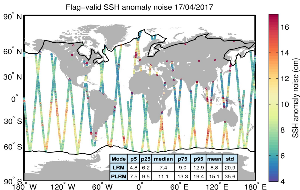
Figure 8. Geographical distribution of flag-valid 20-Hz SSH anomaly measurement noise over oceans and lakes for 17/04/2017. The statistical values shown in the table refer to the SSH anomaly noise and are calculated separately for LRM and PLRM regions. Measurements taken over polar polygons have been excluded from the computation of the statistical values. The black lines mark the outer limit of the Arctic and Antarctic polar polygons.
