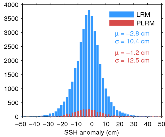
Figure 11. Histogram of science-valid SSH anomaly over oceans and lakes for LRM (blue) and PLRM (red) for 17/04/2017. The mean ( \mu ) and standard deviation ( \sigma ) are also shown. Note that values outside [-50 50] cm are excluded from the histogram for the sake of readability but not from the computation of \mu and \sigma .
