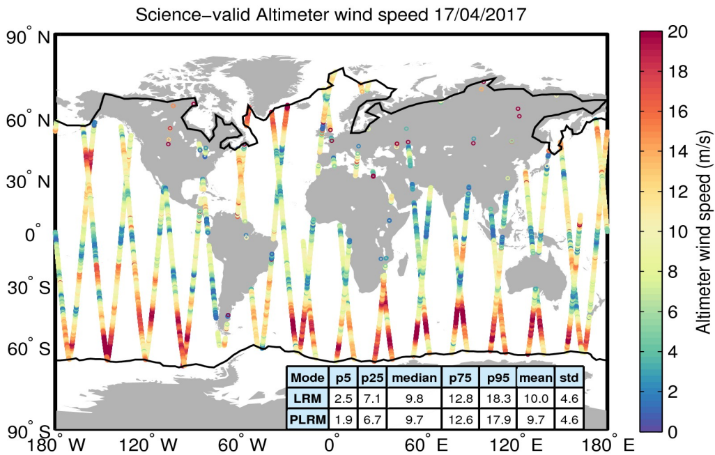
Figure 34. Geographical distribution of science-valid wind data over oceans and lakes for 17/04/2017. The statistical values shown in the table refer to the wind in m/s and are calculated separately for LRM and PLRM regions. The black lines mark the outer limit of the Arctic and Antarctic polar polygons. Gray circles denote records that have been rejected based on the editing criteria described in Table 5.
