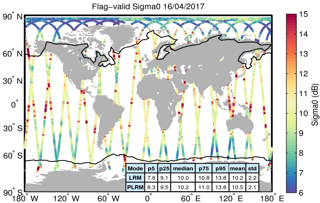
Figure 23. Geographical distribution of flag-valid sigma0 data over oceans and lakes for 16/04/2017. The statistical values shown in the table refer to the sigma0 in dB and are calculated separately for LRM and PLRM regions. Measurements taken over polar polygons have been excluded from the computation of the statistical values. The black lines mark the outer limit of the Arctic and Antarctic polar polygons.
