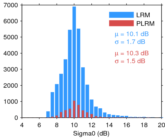
Figure 28. Histogram of science-valid sigma0 over oceans and lakes for LRM (blue) and PLRM (red) for 16/04/2017. The mean ( \mu ) and standard deviation ( \sigma ) are also shown. Note that values outside [4 20] dB are excluded from the histogram for the sake of readability but not from the computation of \mu and \sigma .
