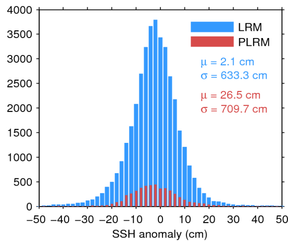
Figure 7. Histogram of flag-valid SSH anomaly over oceans and lakes for LRM (blue) and PLRM (red) for 16/04/2017. The mean ( \mu ) and standard deviation ( \sigma ) are also shown. Note that values outside [-50 \ 50] cm are excluded from the histogram for the sake of readability but not from the computation of \mu and \sigma .
