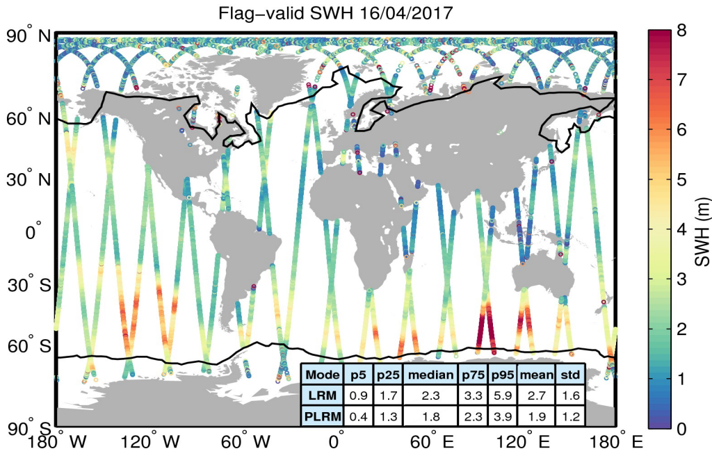
Figure 15. Geographical distribution of flag-valid SWH data over oceans and lakes for 16/04/2017. The statistical values shown in the table refer to the SWH in m and are calculated separately for LRM and PLRM regions. Measurements taken over polar polygons have been excluded from the computation of the statistical values. The black lines mark the outer limit of the Arctic and Antarctic polar polygons.
