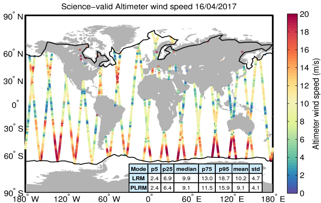
Figure 34. Geographical distribution of science-valid wind data over oceans and lakes for 16/04/2017. The statistical values shown in the table refer to the wind in m/s and are calculated separately for LRM and PLRM regions. The black lines mark the outer limit of the Arctic and Antarctic polar polygons. Gray circles denote records that have been rejected based on the editing criteria described in Table 5.
