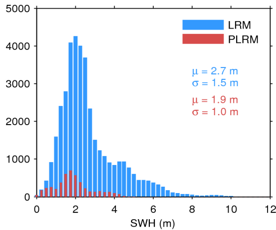
Figure 20. Histogram of science-valid SWH over oceans and lakes for LRM (blue) and PLRM (red) for 16/04/2017. The mean ( \mu ) and standard deviation ( \sigma ) are also shown. Note that values larger than 12 m are excluded from the histogram for the sake of readability but not from the computation of \mu and \sigma .
