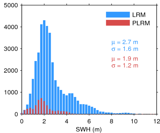
Figure 17. Histogram of flag-valid SWH over oceans and lakes for LRM (blue) and PLRM (red) for 16/04/2017. The mean ( \mu ) and standard deviation ( \sigma ) are also shown. Note that values larger than 12 m are excluded from the histogram for the sake of readability but not from the computation of \mu and \sigma .
