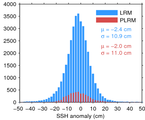
Figure 11. Histogram of science-valid SSH anomaly over oceans and lakes for LRM (blue) and PLRM (red) for 16/04/2017. The mean ( \mu ) and standard deviation ( \sigma ) are also shown. Note that values outside [-50 50] cm are excluded from the histogram for the sake of readability but not from the computation of \mu and \sigma .
