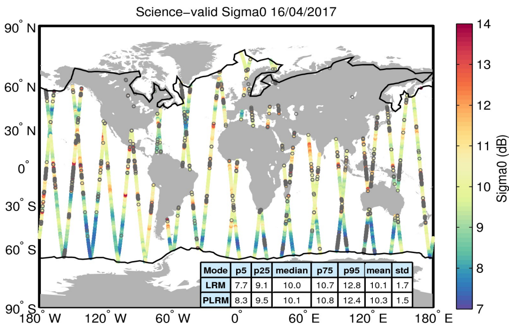
Figure 27. Geographical distribution of science-valid sigma0 data over oceans and lakes for 16/04/2017. The statistical values shown in the table refer to the sigma0 in dB and are calculated separately for LRM and PLRM regions. The black lines mark the outer limit of the Arctic and Antarctic polar polygons. Gray circles denote records that have been rejected based on the editing criteria described in Table 4.
