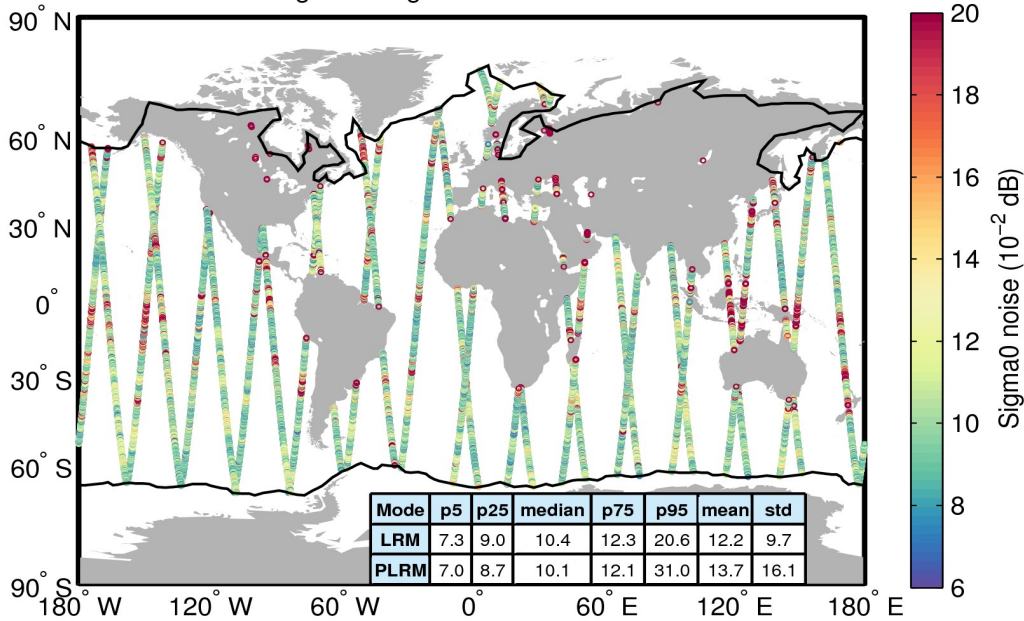
Flag-valid sigma0 noise 16/04/2017
