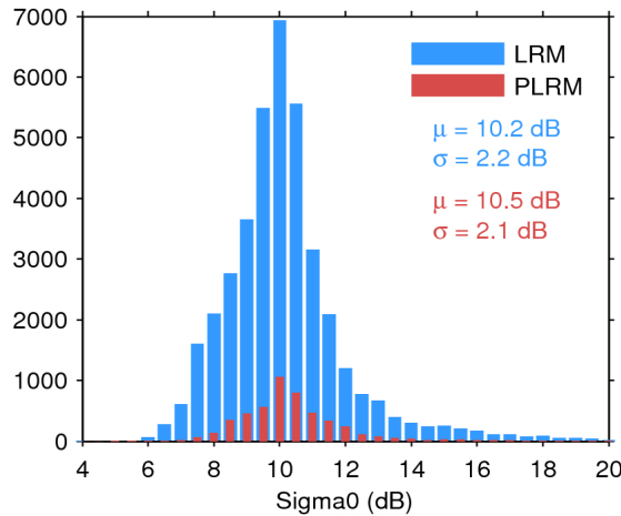
Figure 25. Histogram of flag-valid sigma0 over oceans and lakes for LRM (blue) and PLRM (red) for 16/04/2017. The mean ( \mu ) and standard deviation ( \sigma ) are also shown. Note that values outside [4 20] dB are excluded from the histogram for the sake of readability but not from the computation of \mu and \sigma .
