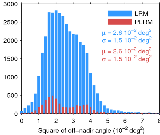
Figure 39. Histogram of flag-valid mispointing over oceans and lakes for LRM (blue) and PLRM (red) for 16/04/2017. Only positive values have been considered. The mean ( \mu ) and standard deviation ( \sigma ) are also shown. Note that values larger than 8 \cdot 10^{-2} \text{ deg}^2 are excluded from the histogram for the sake of readability but not from the computation of \mu and \sigma .
