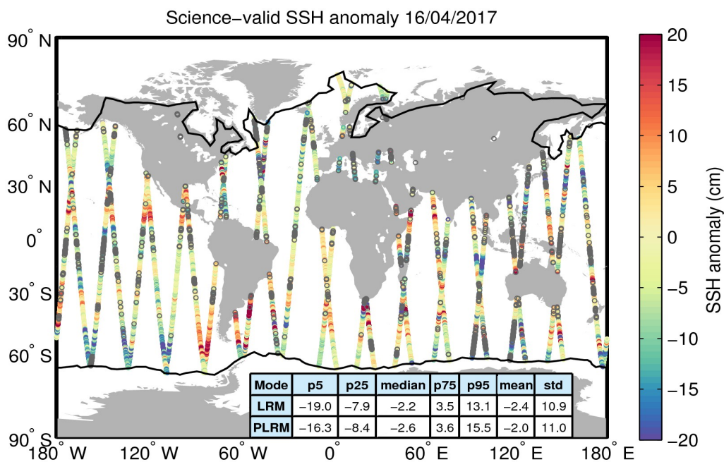
Figure 10. Geographical distribution of science-valid SSH anomaly data over oceans and lakes for 16/04/2017. The statistical values shown in the table refer to the SSH anomaly in cm and are calculated separately for LRM and PLRM regions. The black lines mark the outer limit of the Arctic and Antarctic polar polygons. Gray circles denote records that have been rejected based on the editing criteria described in Table 2.
