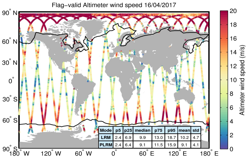
Figure 31. Geographical distribution of flag-valid wind data over oceans and lakes for 16/04/2017. The statistical values shown in the table refer to the wind in m/s and are calculated separately for LRM and PLRM regions. Measurements taken over polar polygons have been excluded from the computation of the statistical values. The black lines mark the outer limit of the Arctic and Antarctic polar polygons.
