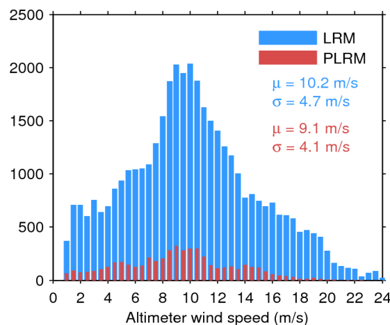
Figure 35. Histogram of science-valid wind over oceans and lakes for LRM (blue) and PLRM (red) for 16/04/2017. The mean ( \mu ) and standard deviation ( \sigma ) are also shown. Note that values larger than 24 m/s are excluded from the histogram for the sake of readability but not from the computation of \mu and \sigma .
