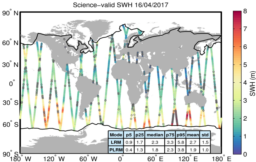
Figure 19. Geographical distribution of science-valid SWH data over oceans and lakes for 16/04/2017. The statistical values shown in the table refer to the SWH in m and are calculated separately for LRM and PLRM regions. The black lines mark the outer limit of the Arctic and Antarctic polar polygons. Gray circles denote records that have been rejected based on the editing criteria described in Table 3.
