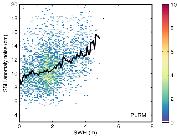
Figure 9. 2D histogram showing flag-valid SSH anomaly noise as a function of SWH for LRM (top) and PLRM (bottom) for 16/04/2017. The black line denotes the median SSH anomaly noise as a function of SWH.
