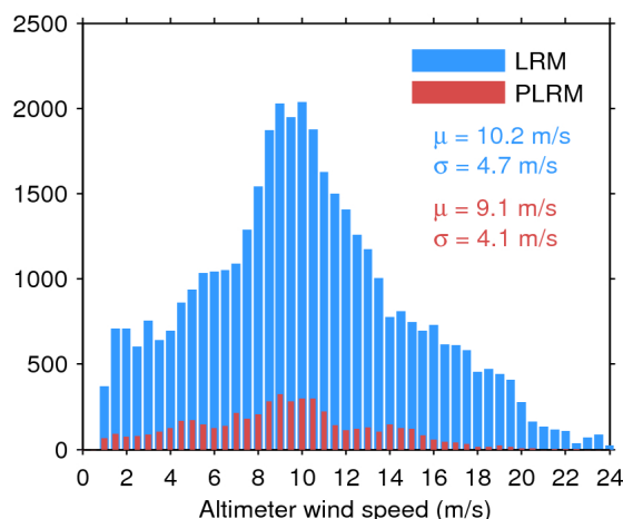
Figure 33. Histogram of flag-valid wind over oceans and lakes for LRM (blue) and PLRM (red) for 16/04/2017. The mean ( \mu ) and standard deviation ( \sigma ) are also shown. Note that values larger than 24 m/s are excluded from the histogram for the sake of readability but not from the computation of \mu and \sigma .
