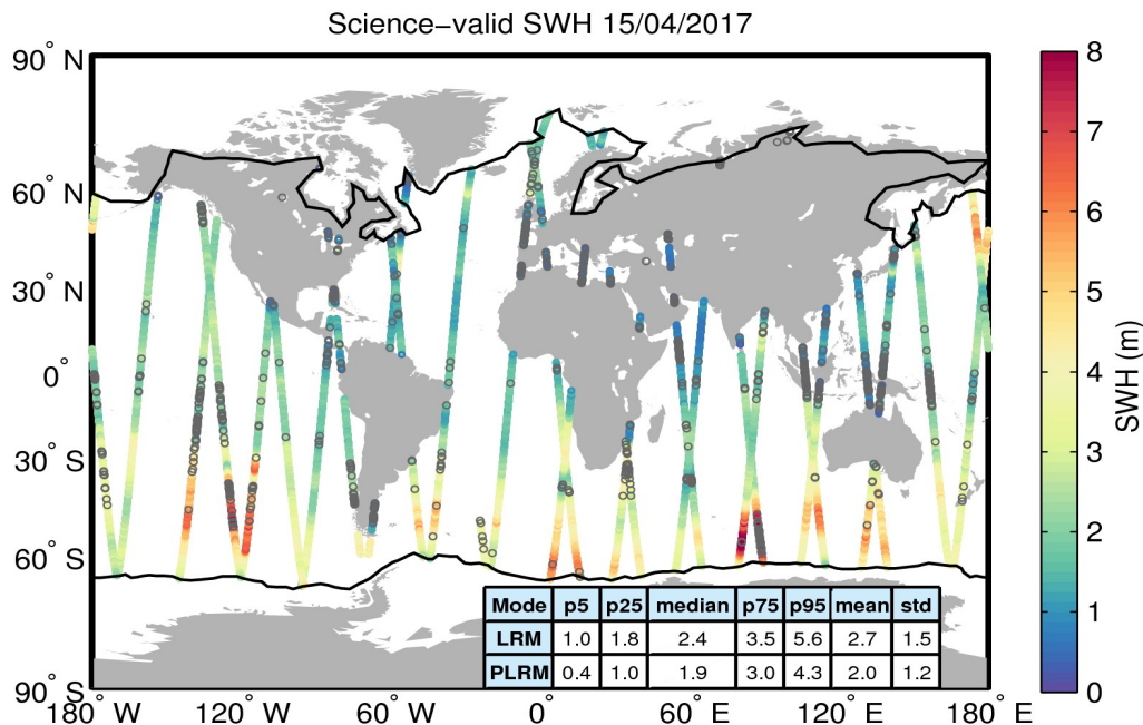
Figure 19. Geographical distribution of science-valid SWH data over oceans and lakes for 15/04/2017. The statistical values shown in the table refer to the SWH in m and are calculated separately for LRM and PLRM regions. The black lines mark the outer limit of the Arctic and Antarctic polar polygons. Gray circles denote records that have been rejected based on the editing criteria described in Table 3.
