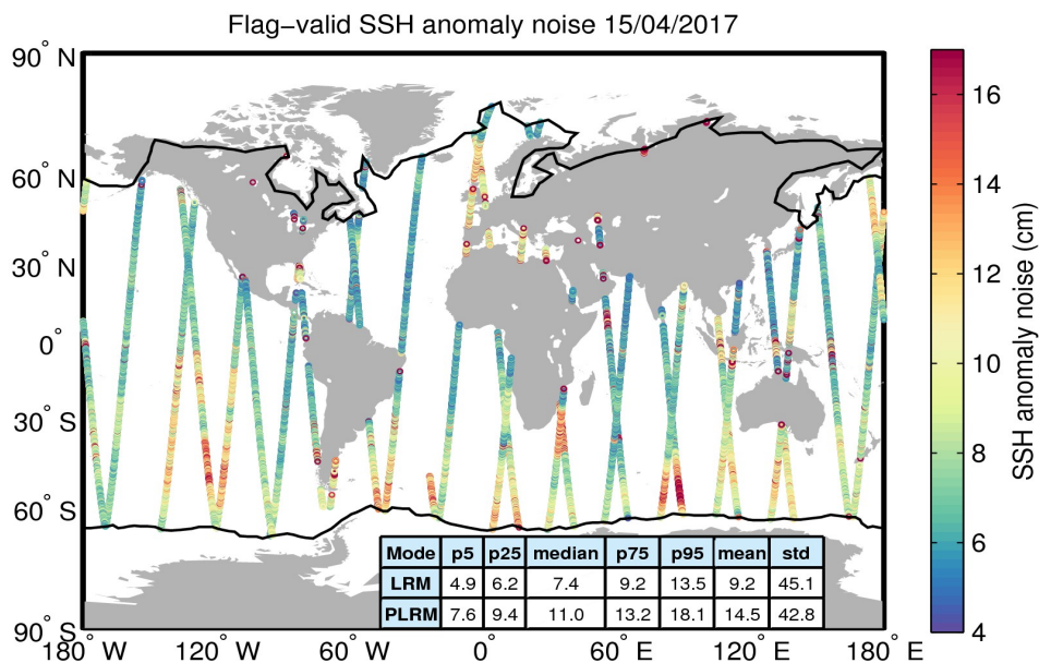
Figure 8. Geographical distribution of flag-valid 20-Hz SSH anomaly measurement noise over oceans and lakes for 15/04/2017. The statistical values shown in the table refer to the SSH anomaly noise and are calculated separately for LRM and PLRM regions. Measurements taken over polar polygons have been excluded from the computation of the statistical values. The black lines mark the outer limit of the Arctic and Antarctic polar polygons.
