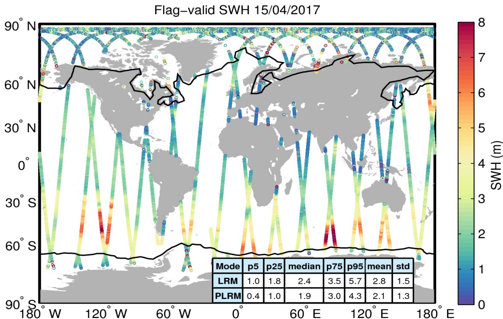
Figure 15. Geographical distribution of flag-valid SWH data over oceans and lakes for 15/04/2017. The statistical values shown in the table refer to the SWH in m and are calculated separately for LRM and PLRM regions. Measurements taken over polar polygons have been excluded from the computation of the statistical values. The black lines mark the outer limit of the Arctic and Antarctic polar polygons.
