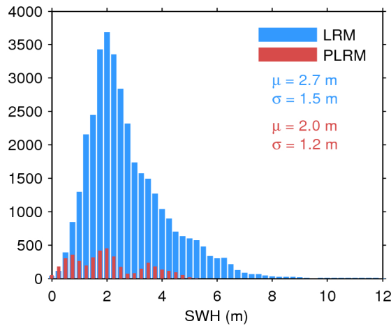
Figure 20. Histogram of science-valid SWH over oceans and lakes for LRM (blue) and PLRM (red) for 15/04/2017. The mean ( \mu ) and standard deviation ( \sigma ) are also shown. Note that values larger than 12 m are excluded from the histogram for the sake of readability but not from the computation of \mu and \sigma .
