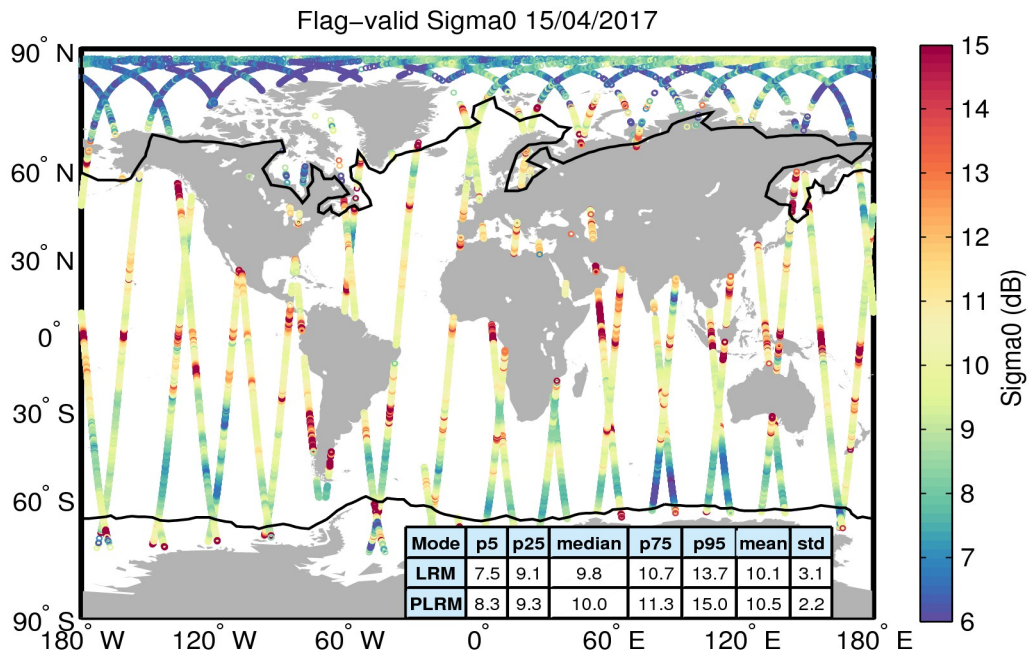
Figure 23. Geographical distribution of flag-valid sigma0 data over oceans and lakes for 15/04/2017. The statistical values shown in the table refer to the sigma0 in dB and are calculated separately for LRM and PLRM regions. Measurements taken over polar polygons have been excluded from the computation of the statistical values. The black lines mark the outer limit of the Arctic and Antarctic polar polygons.
