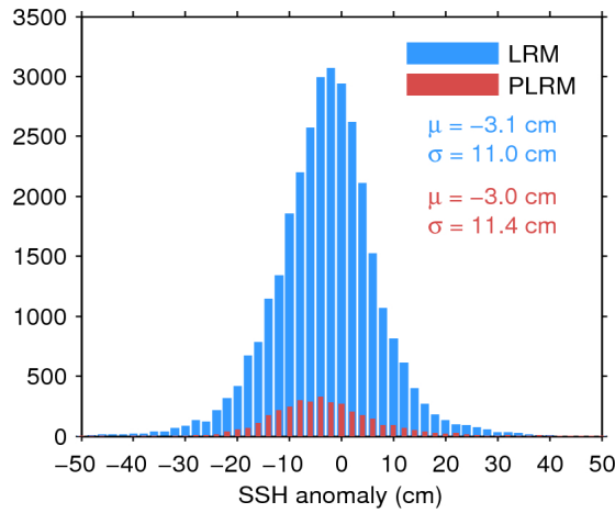
Figure 11. Histogram of science-valid SSH anomaly over oceans and lakes for LRM (blue) and PLRM (red) for 15/04/2017. The mean ( \mu ) and standard deviation ( \sigma ) are also shown. Note that values outside [-50\ 50] cm are excluded from the histogram for the sake of readability but not from the computation of \mu and \sigma .
