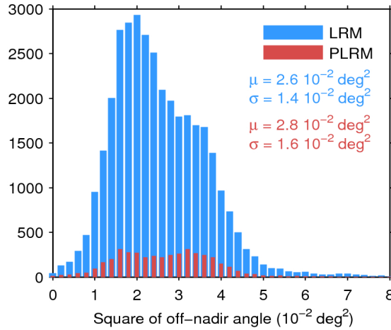
Figure 39. Histogram of flag-valid mispointing over oceans and lakes for LRM (blue) and PLRM (red) for 15/04/2017. Only positive values have been considered. The mean ( \mu ) and standard deviation ( \sigma ) are also shown. Note that values larger than 8 \cdot 10^{-2} \text{ deg}^2 are excluded from the histogram for the sake of readability but not from the computation of \mu and \sigma .
