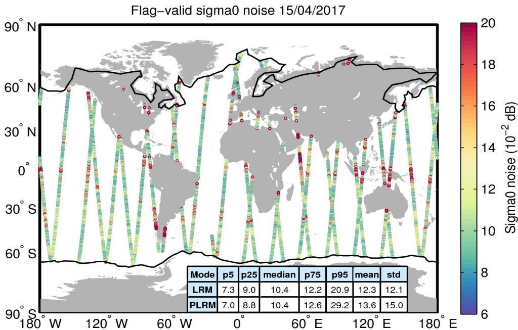
Figure 26. Geographical distribution of flag-valid 20-Hz sigma0 measurement noise over oceans and lakes for 15/04/2017. The statistical values shown in the table refer to the sigma0 noise and are calculated separately for LRM and PLRM regions. Measurements taken over polar polygons have been excluded from the computation of the statistical values. The black lines mark the outer limit of the Arctic and Antarctic polar polygons.
