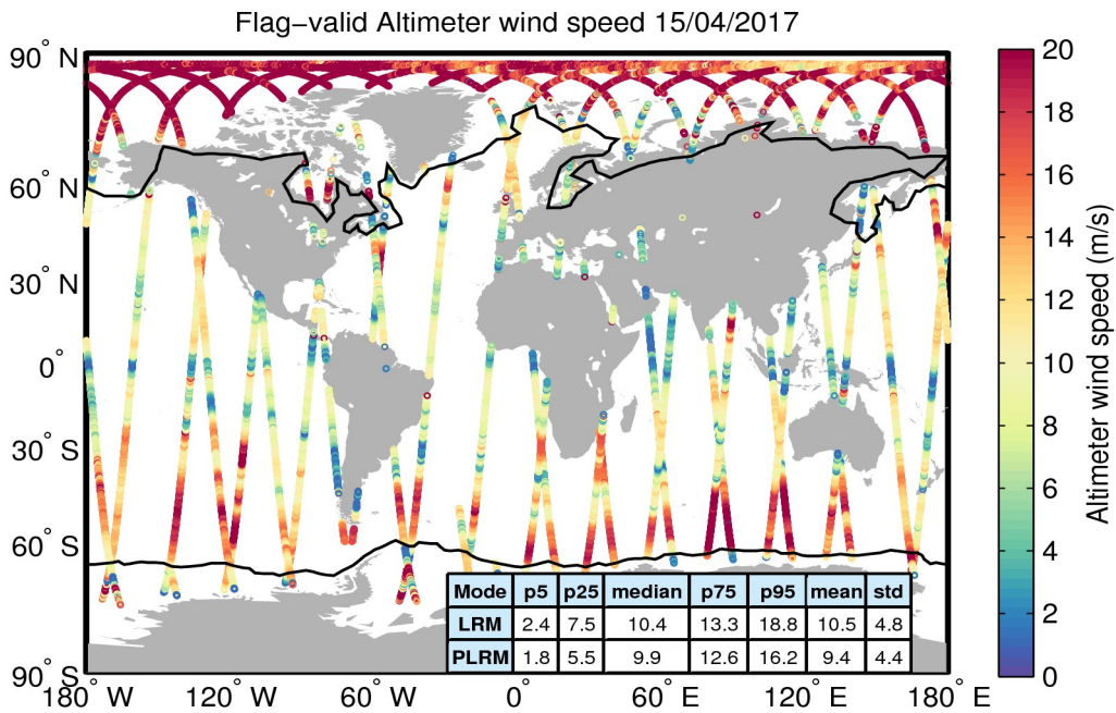
Figure 31. Geographical distribution of flag-valid wind data over oceans and lakes for 15/04/2017. The statistical values shown in the table refer to the wind in m/s and are calculated separately for LRM and PLRM regions. Measurements taken over polar polygons have been excluded from the computation of the statistical values. The black lines mark the outer limit of the Arctic and Antarctic polar polygons.
