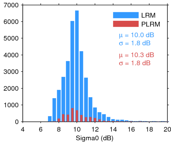
Figure 28. Histogram of science-valid sigma0 over oceans and lakes for LRM (blue) and PLRM (red) for 15/04/2017. The mean ( \mu ) and standard deviation ( \sigma ) are also shown. Note that values outside [4 20] dB are excluded from the histogram for the sake of readability but not from the computation of \mu and \sigma .
