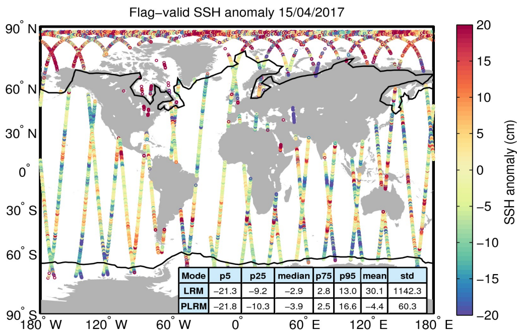
Figure 5. Geographical distribution of flag-valid 1-Hz SSH anomaly data over oceans and lakes for 15/04/2017. The statistical values shown in the table refer to the SSH anomaly in cm and are calculated separately for LRM and PLRM regions. Measurements taken over polar polygons have been excluded from the computation of the statistical values. The black lines mark the outer limit of the Arctic and Antarctic polar polygons.
