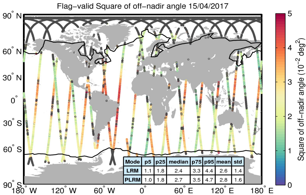
Figure 37. Geographical distribution of flag-valid mispointing data over oceans and lakes for 15/04/2017. The statistical values shown in the table refer to the mispointing in 10^{-2} deg 2 and are calculated separately for LRM and PLRM regions. Measurements taken over polar polygons have been excluded from the computation of the statistical values. The black lines mark the outer limit of the Arctic and Antarctic polar polygons. Gray circles denote negative values.
