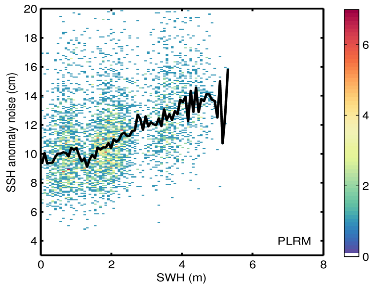
Figure 9. 2D histogram showing flag-valid SSH anomaly noise as a function of SWH for LRM (top) and PLRM (bottom) for 15/04/2017. The black line denotes the median SSH anomaly noise as a function of SWH.
