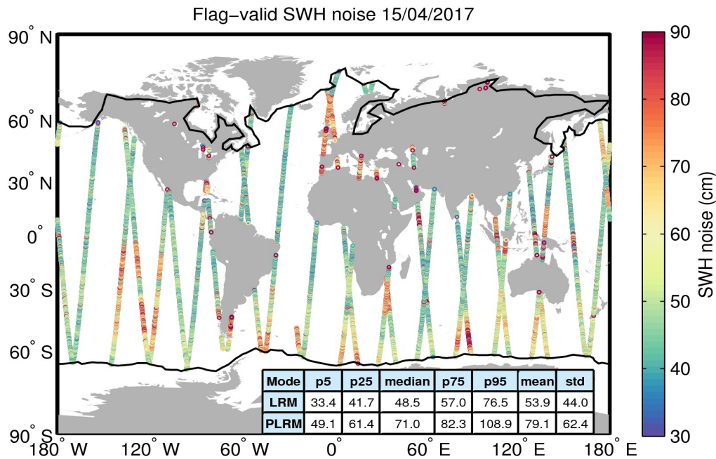
Figure 18. Geographical distribution of flag-valid 20-Hz SWH measurement noise over oceans and lakes for 15/04/2017. The statistical values shown in the table refer to the SWH noise and are calculated separately for LRM and PLRM regions. Measurements taken over polar polygons have been excluded from the computation of the statistical values. The black lines mark the outer limit of the Arctic and Antarctic polar polygons.
