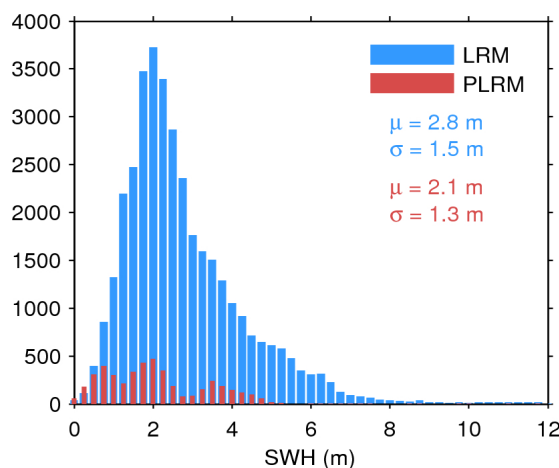
Figure 17. Histogram of flag-valid SWH over oceans and lakes for LRM (blue) and PLRM (red) for 15/04/2017. The mean ( \mu ) and standard deviation ( \sigma ) are also shown. Note that values larger than 12 m are excluded from the histogram for the sake of readability but not from the computation of \mu and \sigma .
