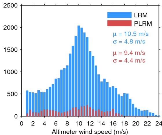
Figure 35. Histogram of science-valid wind over oceans and lakes for LRM (blue) and PLRM (red) for 15/04/2017. The mean ( \mu ) and standard deviation ( \sigma ) are also shown. Note that values larger than 24 m/s are excluded from the histogram for the sake of readability but not from the computation of \mu and \sigma .
