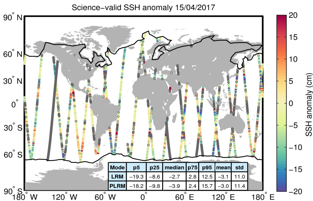
Figure 10. Geographical distribution of science-valid SSH anomaly data over oceans and lakes for 15/04/2017. The statistical values shown in the table refer to the SSH anomaly in cm and are calculated separately for LRM and PLRM regions. The black lines mark the outer limit of the Arctic and Antarctic polar polygons. Gray circles denote records that have been rejected based on the editing criteria described in Table 2.
