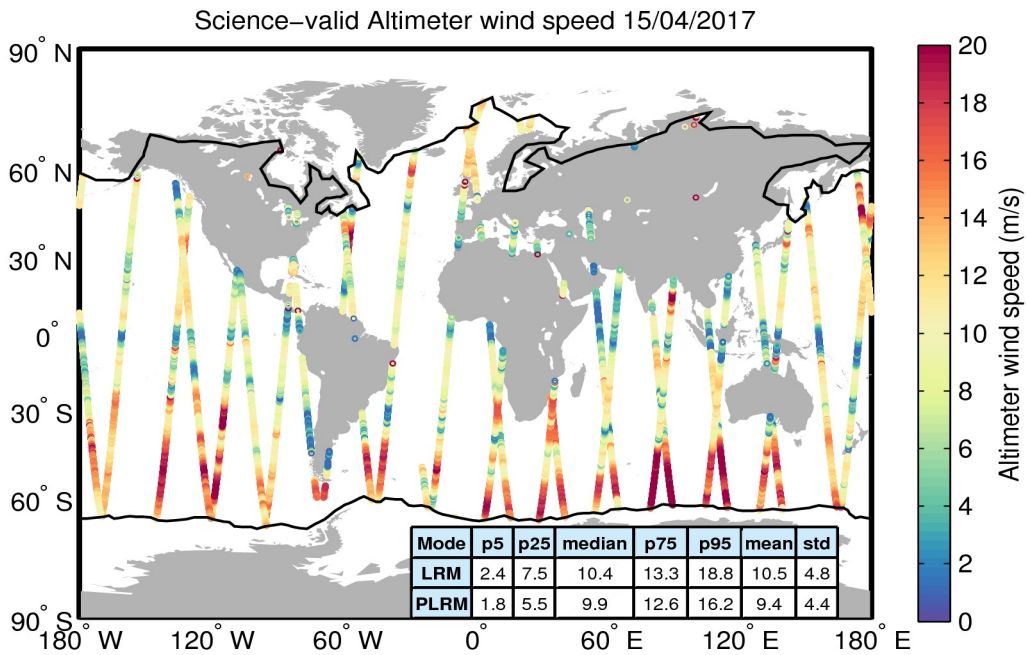
Figure 34. Geographical distribution of science-valid wind data over oceans and lakes for 15/04/2017. The statistical values shown in the table refer to the wind in m/s and are calculated separately for LRM and PLRM regions. The black lines mark the outer limit of the Arctic and Antarctic polar polygons. Gray circles denote records that have been rejected based on the editing criteria described in Table 5.
