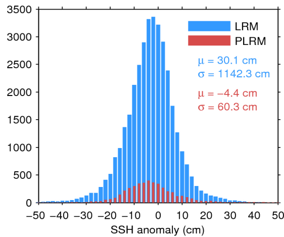
Figure 7. Histogram of flag-valid SSH anomaly over oceans and lakes for LRM (blue) and PLRM (red) for 15/04/2017. The mean ( \mu ) and standard deviation ( \sigma ) are also shown. Note that values outside [-50\ 50] cm are excluded from the histogram for the sake of readability but not from the computation of \mu and \sigma .
