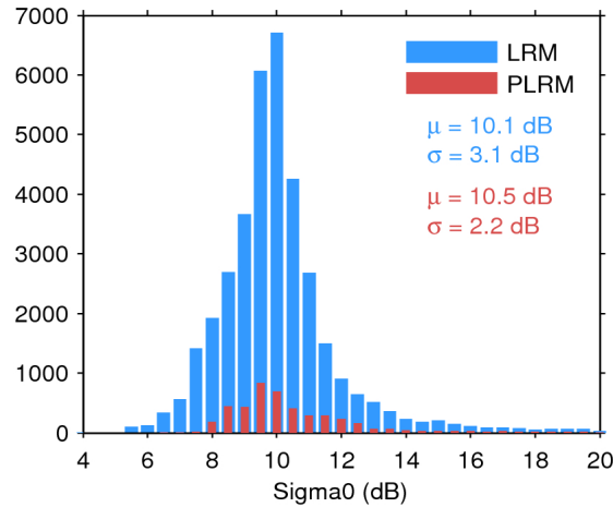
Figure 25. Histogram of flag-valid sigma0 over oceans and lakes for LRM (blue) and PLRM (red) for 15/04/2017. The mean ( \mu ) and standard deviation ( \sigma ) are also shown. Note that values outside [4 20] dB are excluded from the histogram for the sake of readability but not from the computation of \mu and \sigma .
