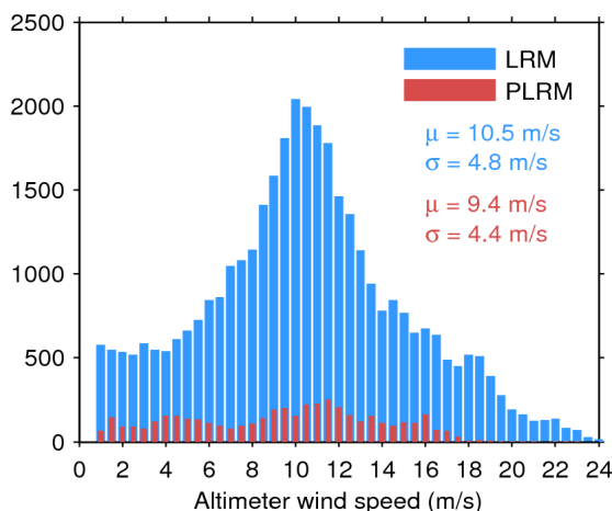
Figure 33. Histogram of flag-valid wind over oceans and lakes for LRM (blue) and PLRM (red) for 15/04/2017. The mean ( \mu ) and standard deviation ( \sigma ) are also shown. Note that values larger than 24 m/s are excluded from the histogram for the sake of readability but not from the computation of \mu and \sigma .
