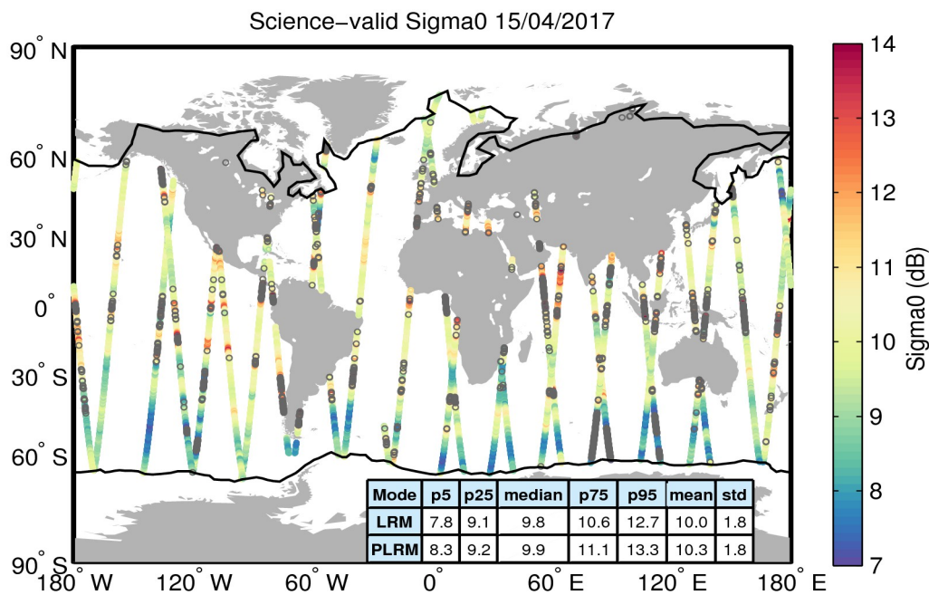
Figure 27. Geographical distribution of science-valid sigma0 data over oceans and lakes for 15/04/2017. The statistical values shown in the table refer to the sigma0 in dB and are calculated separately for LRM and PLRM regions. The black lines mark the outer limit of the Arctic and Antarctic polar polygons. Gray circles denote records that have been rejected based on the editing criteria described in Table 4.
