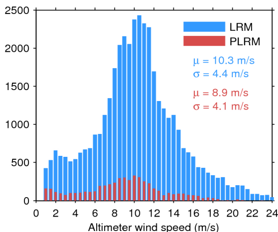
Figure 33. Histogram of flag-valid wind over oceans and lakes for LRM (blue) and PLRM (red) for 14/04/2017. The mean ( \mu ) and standard deviation ( \sigma ) are also shown. Note that values larger than 24 m/s are excluded from the histogram for the sake of readability but not from the computation of \mu and \sigma .
