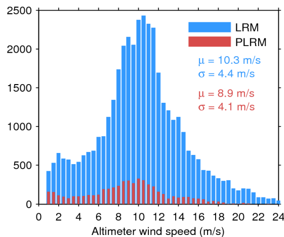
Figure 35. Histogram of science-valid wind over oceans and lakes for LRM (blue) and PLRM (red) for 14/04/2017. The mean ( \mu ) and standard deviation ( \sigma ) are also shown. Note that values larger than 24 m/s are excluded from the histogram for the sake of readability but not from the computation of \mu and \sigma .
