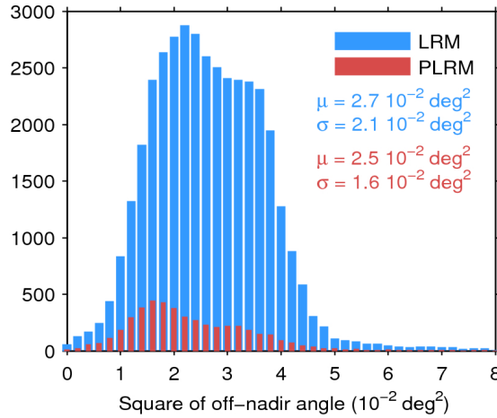
Figure 39. Histogram of flag-valid mispointing over oceans and lakes for LRM (blue) and PLRM (red) for 14/04/2017. Only positive values have been considered. The mean ( \mu ) and standard deviation ( \sigma ) are also shown. Note that values larger than 8 \cdot 10^{-2} \text{ deg}^2 are excluded from the histogram for the sake of readability but not from the computation of \mu and \sigma .
