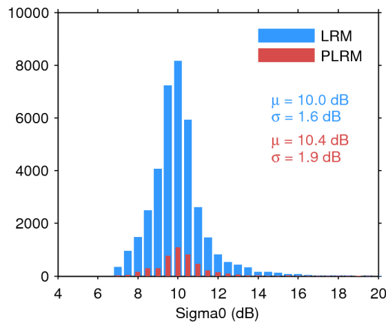
Figure 28. Histogram of science-valid sigma0 over oceans and lakes for LRM (blue) and PLRM (red) for 14/04/2017. The mean ( \mu ) and standard deviation ( \sigma ) are also shown. Note that values outside [4 20] dB are excluded from the histogram for the sake of readability but not from the computation of \mu and \sigma .
