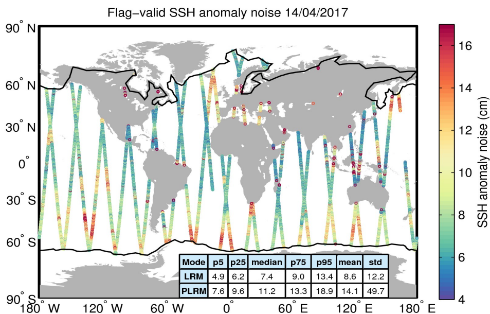
Figure 8. Geographical distribution of flag-valid 20-Hz SSH anomaly measurement noise over oceans and lakes for 14/04/2017. The statistical values shown in the table refer to the SSH anomaly noise and are calculated separately for LRM and PLRM regions. Measurements taken over polar polygons have been excluded from the computation of the statistical values. The black lines mark the outer limit of the Arctic and Antarctic polar polygons.
