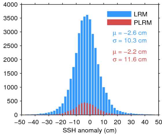
Figure 11. Histogram of science-valid SSH anomaly over oceans and lakes for LRM (blue) and PLRM (red) for 14/04/2017. The mean ( \mu ) and standard deviation ( \sigma ) are also shown. Note that values outside [-50 50] cm are excluded from the histogram for the sake of readability but not from the computation of \mu and \sigma .
