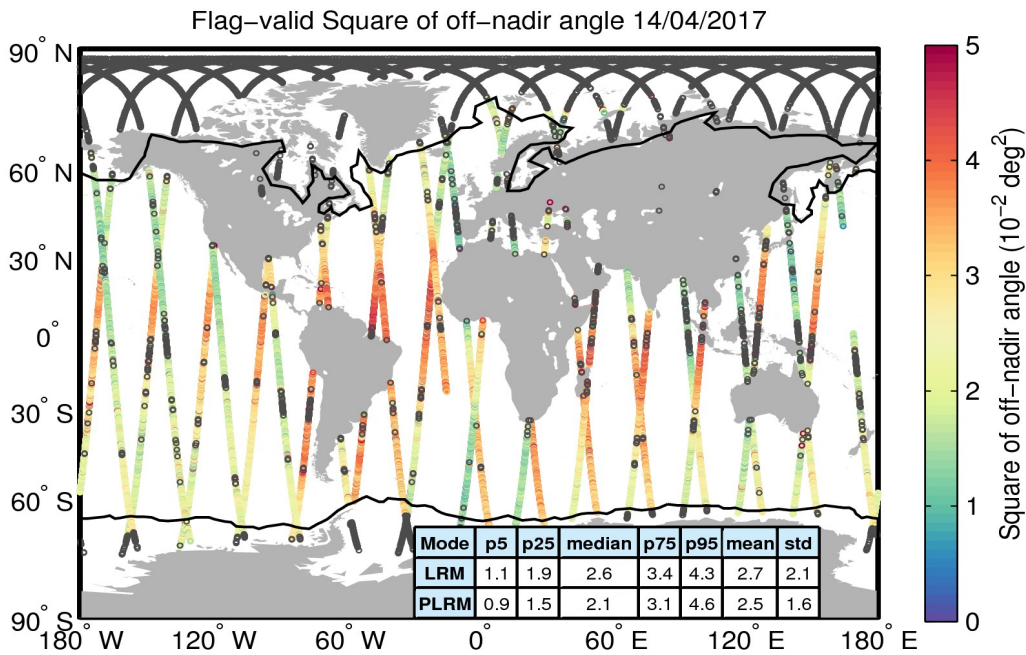
Figure 37. Geographical distribution of flag-valid mispointing data over oceans and lakes for 14/04/2017. The statistical values shown in the table refer to the mispointing in 10^{-2} deg 2 and are calculated separately for LRM and PLRM regions. Measurements taken over polar polygons have been excluded from the computation of the statistical values. The black lines mark the outer limit of the Arctic and Antarctic polar polygons. Gray circles denote negative values.
