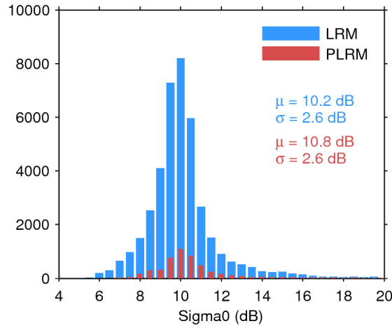
Figure 25. Histogram of flag-valid sigma0 over oceans and lakes for LRM (blue) and PLRM (red) for 14/04/2017. The mean ( \mu ) and standard deviation ( \sigma ) are also shown. Note that values outside [4 20] dB are excluded from the histogram for the sake of readability but not from the computation of \mu and \sigma .
