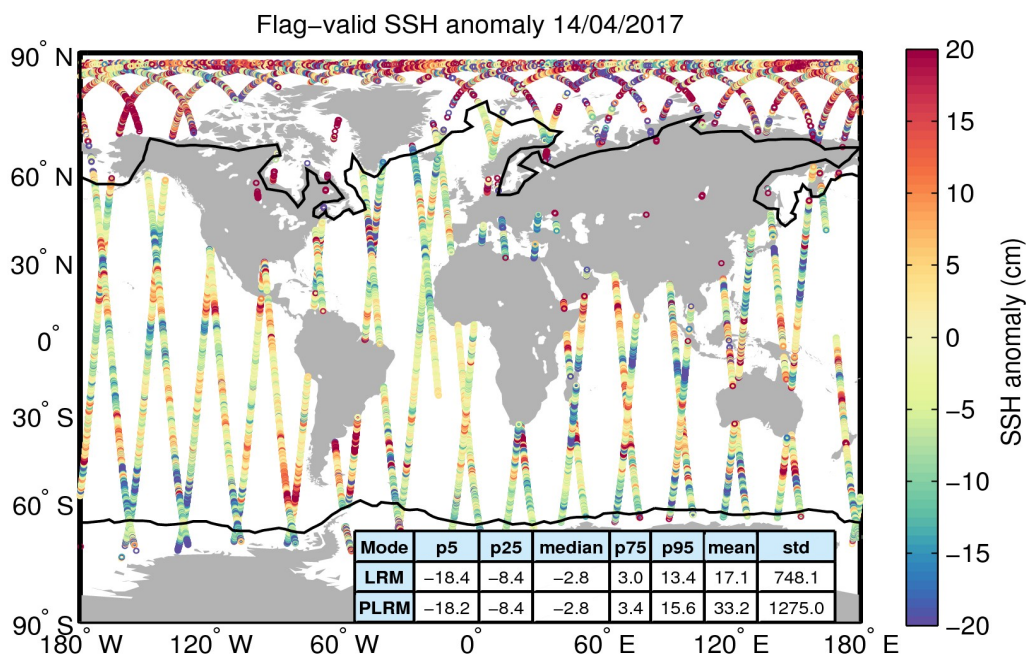
Figure 5. Geographical distribution of flag-valid 1-Hz SSH anomaly data over oceans and lakes for 14/04/2017. The statistical values shown in the table refer to the SSH anomaly in cm and are calculated separately for LRM and PLRM regions. Measurements taken over polar polygons have been excluded from the computation of the statistical values. The black lines mark the outer limit of the Arctic and Antarctic polar polygons.
