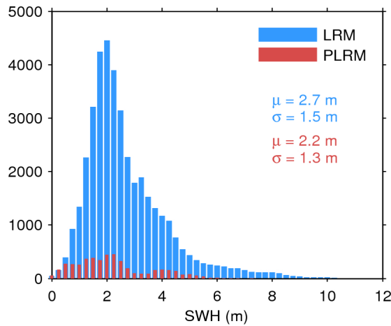
Figure 20. Histogram of science-valid SWH over oceans and lakes for LRM (blue) and PLRM (red) for 14/04/2017. The mean ( \mu ) and standard deviation ( \sigma ) are also shown. Note that values larger than 12 m are excluded from the histogram for the sake of readability but not from the computation of \mu and \sigma .
