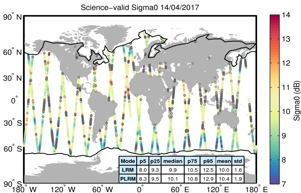
Figure 27. Geographical distribution of science-valid sigma0 data over oceans and lakes for 14/04/2017. The statistical values shown in the table refer to the sigma0 in dB and are calculated separately for LRM and PLRM regions. The black lines mark the outer limit of the Arctic and Antarctic polar polygons. Gray circles denote records that have been rejected based on the editing criteria described in Table 4.
