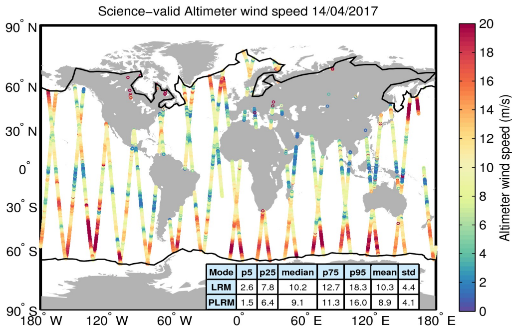
Figure 34. Geographical distribution of science-valid wind data over oceans and lakes for 14/04/2017. The statistical values shown in the table refer to the wind in m/s and are calculated separately for LRM and PLRM regions. The black lines mark the outer limit of the Arctic and Antarctic polar polygons. Gray circles denote records that have been rejected based on the editing criteria described in Table 5.
