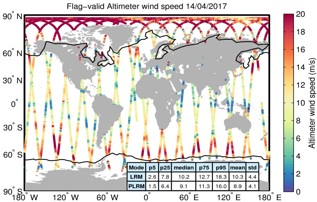
Figure 31. Geographical distribution of flag-valid wind data over oceans and lakes for 14/04/2017. The statistical values shown in the table refer to the wind in m/s and are calculated separately for LRM and PLRM regions. Measurements taken over polar polygons have been excluded from the computation of the statistical values. The black lines mark the outer limit of the Arctic and Antarctic polar polygons.
