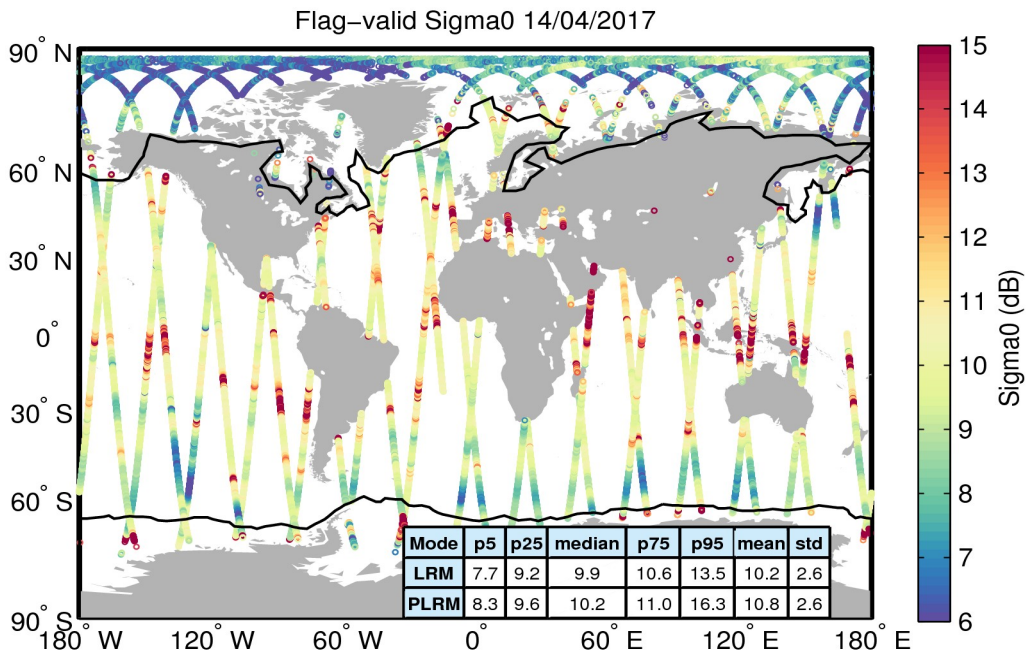
Figure 23. Geographical distribution of flag-valid sigma0 data over oceans and lakes for 14/04/2017. The statistical values shown in the table refer to the sigma0 in dB and are calculated separately for LRM and PLRM regions. Measurements taken over polar polygons have been excluded from the computation of the statistical values. The black lines mark the outer limit of the Arctic and Antarctic polar polygons.
