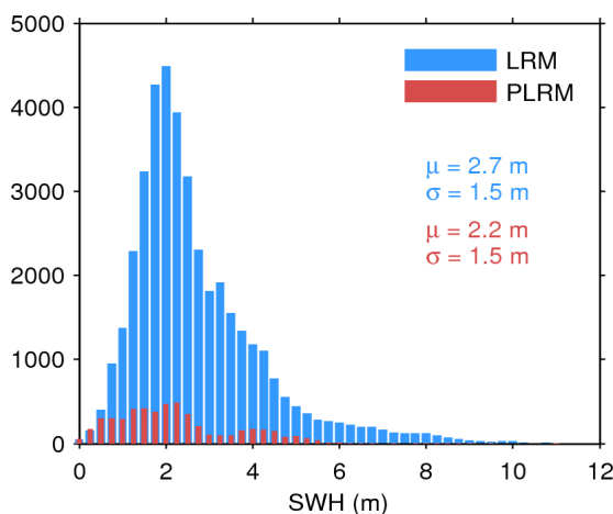
Figure 17. Histogram of flag-valid SWH over oceans and lakes for LRM (blue) and PLRM (red) for 14/04/2017. The mean ( \mu ) and standard deviation ( \sigma ) are also shown. Note that values larger than 12 m are excluded from the histogram for the sake of readability but not from the computation of \mu and \sigma .
