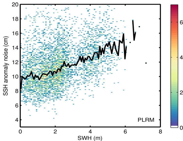
Figure 9. 2D histogram showing flag-valid SSH anomaly noise as a function of SWH for LRM (top) and PLRM (bottom) for 14/04/2017. The black line denotes the median SSH anomaly noise as a function of SWH.
