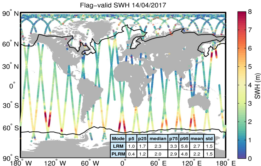
Figure 15. Geographical distribution of flag-valid SWH data over oceans and lakes for 14/04/2017. The statistical values shown in the table refer to the SWH in m and are calculated separately for LRM and PLRM regions. Measurements taken over polar polygons have been excluded from the computation of the statistical values. The black lines mark the outer limit of the Arctic and Antarctic polar polygons.
