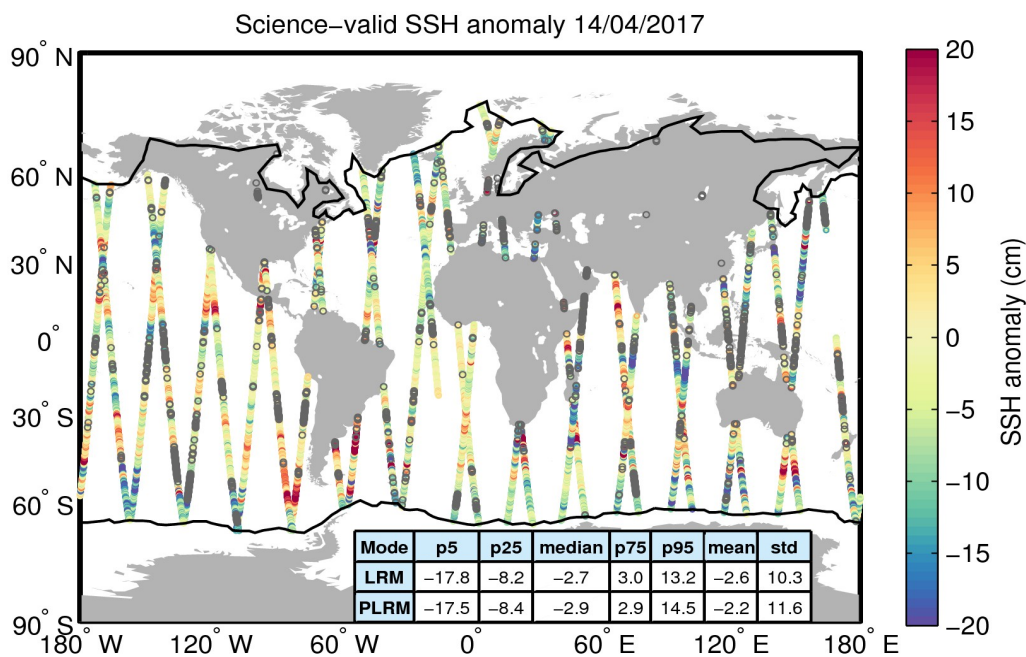
Figure 10. Geographical distribution of science-valid SSH anomaly data over oceans and lakes for 14/04/2017. The statistical values shown in the table refer to the SSH anomaly in cm and are calculated separately for LRM and PLRM regions. The black lines mark the outer limit of the Arctic and Antarctic polar polygons. Gray circles denote records that have been rejected based on the editing criteria described in Table 2.
