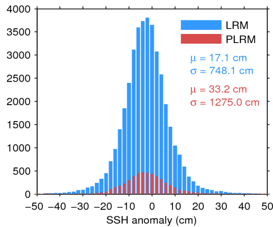
Figure 7. Histogram of flag-valid SSH anomaly over oceans and lakes for LRM (blue) and PLRM (red) for 14/04/2017. The mean ( \mu ) and standard deviation ( \sigma ) are also shown. Note that values outside [-50\ 50] cm are excluded from the histogram for the sake of readability but not from the computation of \mu and \sigma .
