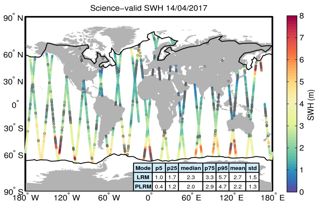
Figure 19. Geographical distribution of science-valid SWH data over oceans and lakes for 14/04/2017. The statistical values shown in the table refer to the SWH in m and are calculated separately for LRM and PLRM regions. The black lines mark the outer limit of the Arctic and Antarctic polar polygons. Gray circles denote records that have been rejected based on the editing criteria described in Table 3.
