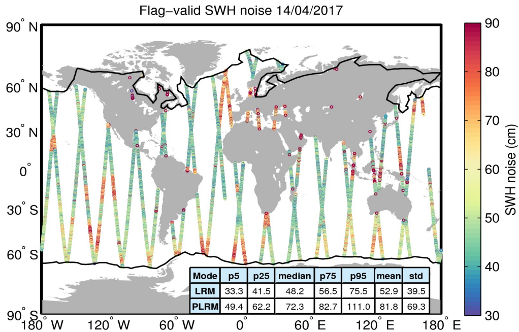
Figure 18. Geographical distribution of flag-valid 20-Hz SWH measurement noise over oceans and lakes for 14/04/2017. The statistical values shown in the table refer to the SWH noise and are calculated separately for LRM and PLRM regions. Measurements taken over polar polygons have been excluded from the computation of the statistical values. The black lines mark the outer limit of the Arctic and Antarctic polar polygons.
