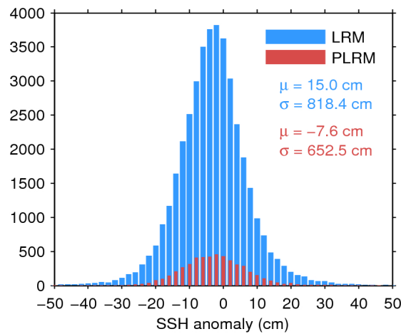
Figure 7. Histogram of flag-valid SSH anomaly over oceans and lakes for LRM (blue) and PLRM (red) for 12/04/2017. The mean ( \mu ) and standard deviation ( \sigma ) are also shown. Note that values outside [-50 50] cm are excluded from the histogram for the sake of readability but not from the computation of \mu and \sigma .
