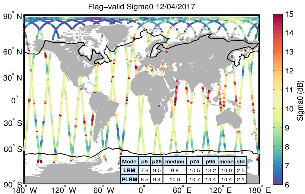
Figure 23. Geographical distribution of flag-valid sigma0 data over oceans and lakes for 12/04/2017. The statistical values shown in the table refer to the sigma0 in dB and are calculated separately for LRM and PLRM regions. Measurements taken over polar polygons have been excluded from the computation of the statistical values. The black lines mark the outer limit of the Arctic and Antarctic polar polygons.
