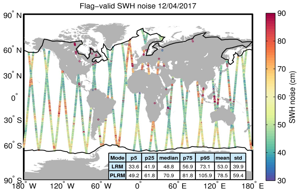
Figure 18. Geographical distribution of flag-valid 20-Hz SWH measurement noise over oceans and lakes for 12/04/2017. The statistical values shown in the table refer to the SWH noise and are calculated separately for LRM and PLRM regions. Measurements taken over polar polygons have been excluded from the computation of the statistical values. The black lines mark the outer limit of the Arctic and Antarctic polar polygons.
