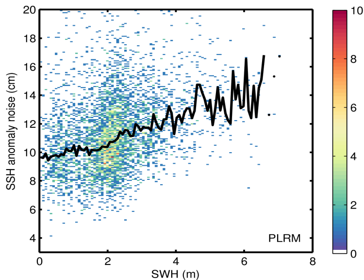
Figure 9. 2D histogram showing flag-valid SSH anomaly noise as a function of SWH for LRM (top) and PLRM (bottom) for 12/04/2017. The black line denotes the median SSH anomaly noise as a function of SWH.
