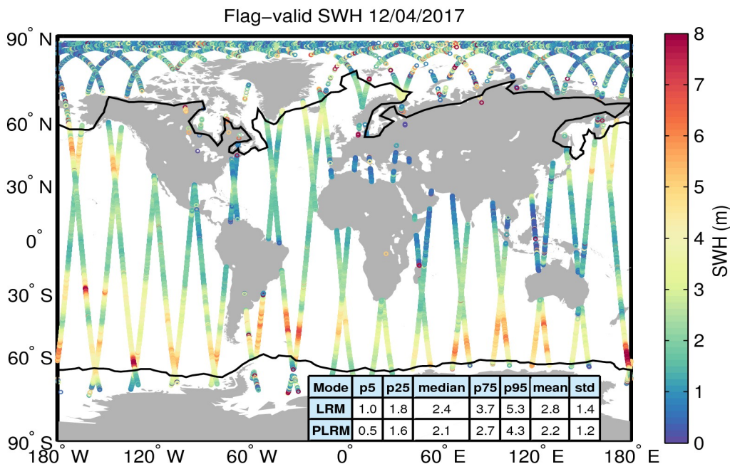
Figure 15. Geographical distribution of flag-valid SWH data over oceans and lakes for 12/04/2017. The statistical values shown in the table refer to the SWH in m and are calculated separately for LRM and PLRM regions. Measurements taken over polar polygons have been excluded from the computation of the statistical values. The black lines mark the outer limit of the Arctic and Antarctic polar polygons.
