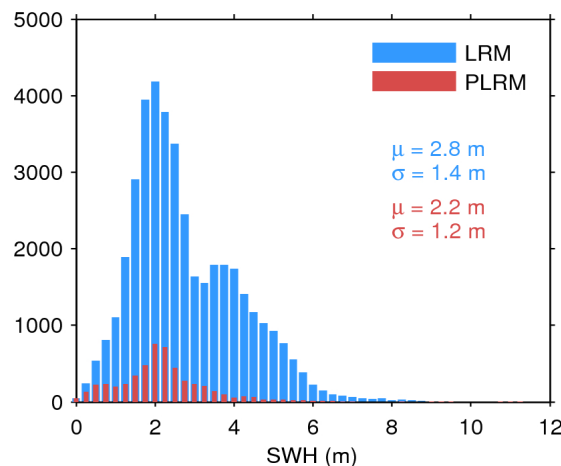
Figure 17. Histogram of flag-valid SWH over oceans and lakes for LRM (blue) and PLRM (red) for 12/04/2017. The mean ( \mu ) and standard deviation ( \sigma ) are also shown. Note that values larger than 12 m are excluded from the histogram for the sake of readability but not from the computation of \mu and \sigma .
