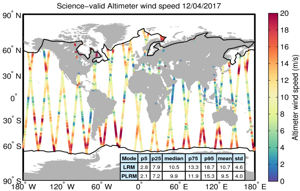
Figure 34. Geographical distribution of science-valid wind data over oceans and lakes for 12/04/2017. The statistical values shown in the table refer to the wind in m/s and are calculated separately for LRM and PLRM regions. The black lines mark the outer limit of the Arctic and Antarctic polar polygons. Gray circles denote records that have been rejected based on the editing criteria described in Table 5.
