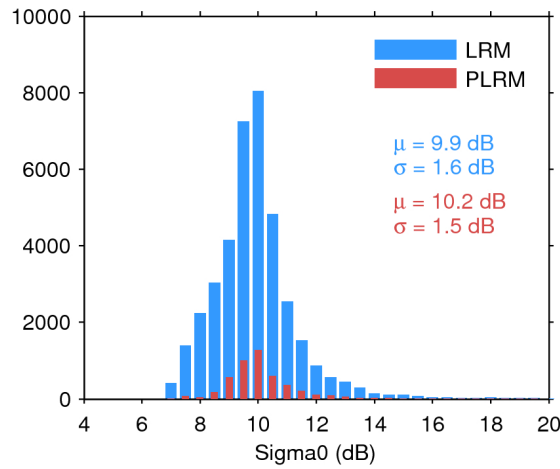
Figure 28. Histogram of science-valid sigma0 over oceans and lakes for LRM (blue) and PLRM (red) for 12/04/2017. The mean ( \mu ) and standard deviation ( \sigma ) are also shown. Note that values outside [4 20] dB are excluded from the histogram for the sake of readability but not from the computation of \mu and \sigma .
