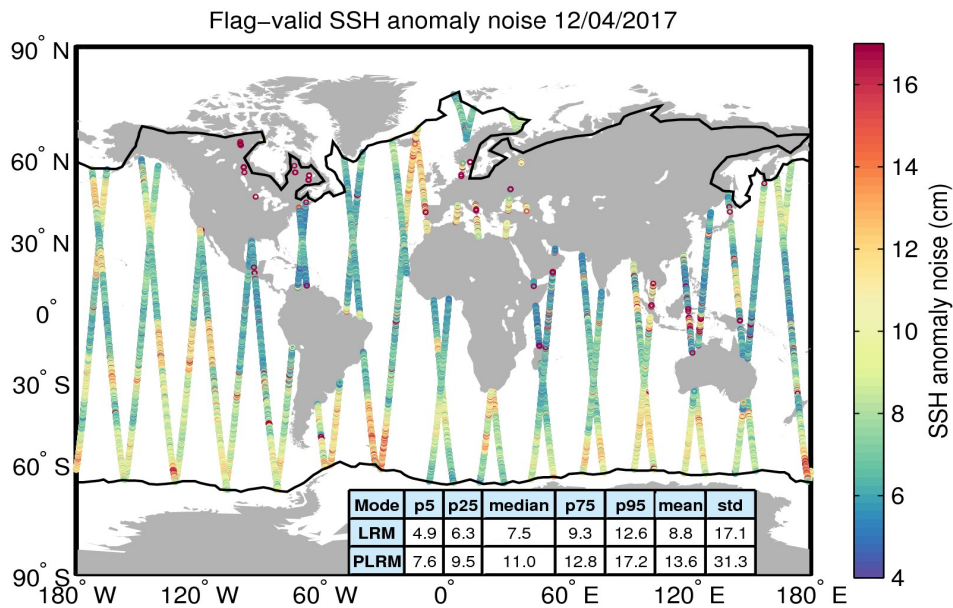
Figure 8. Geographical distribution of flag-valid 20-Hz SSH anomaly measurement noise over oceans and lakes for 12/04/2017. The statistical values shown in the table refer to the SSH anomaly noise and are calculated separately for LRM and PLRM regions. Measurements taken over polar polygons have been excluded from the computation of the statistical values. The black lines mark the outer limit of the Arctic and Antarctic polar polygons.
