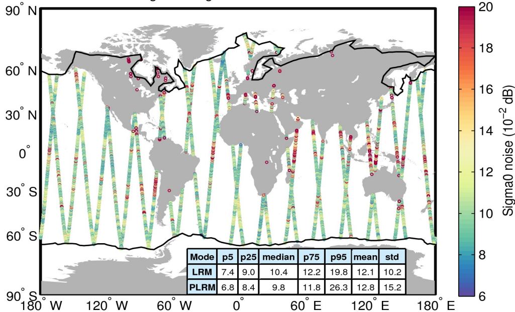
Flag-valid sigma0 noise 12/04/2017
