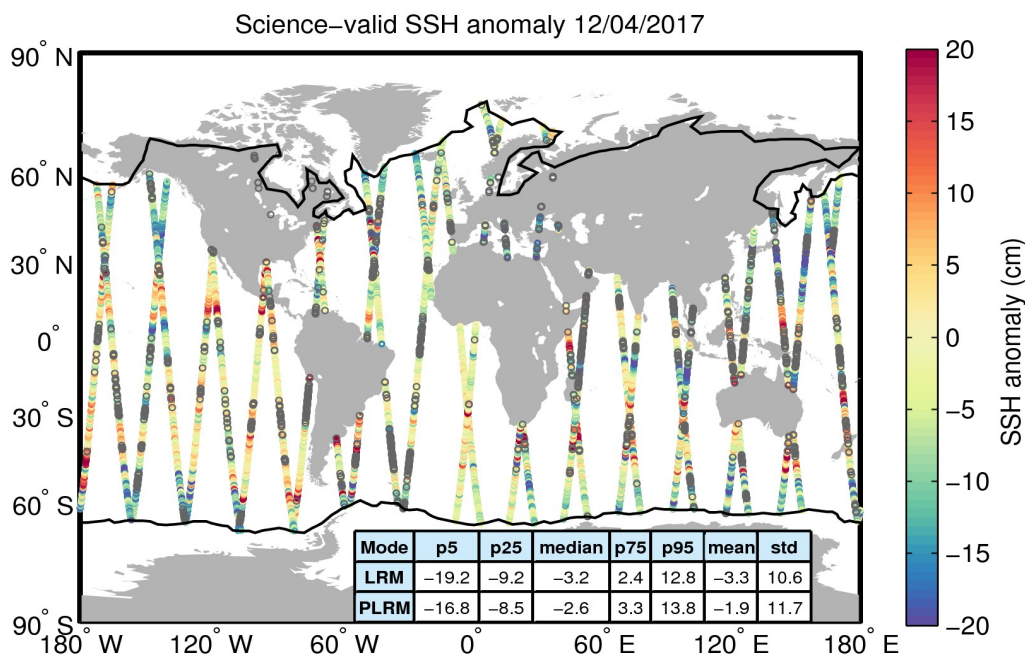
Figure 10. Geographical distribution of science-valid SSH anomaly data over oceans and lakes for 12/04/2017. The statistical values shown in the table refer to the SSH anomaly in cm and are calculated separately for LRM and PLRM regions. The black lines mark the outer limit of the Arctic and Antarctic polar polygons. Gray circles denote records that have been rejected based on the editing criteria described in Table 2.
