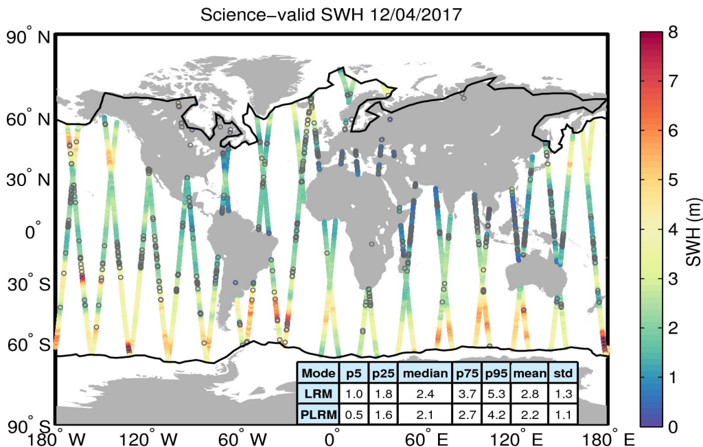
Figure 19. Geographical distribution of science-valid SWH data over oceans and lakes for 12/04/2017. The statistical values shown in the table refer to the SWH in m and are calculated separately for LRM and PLRM regions. The black lines mark the outer limit of the Arctic and Antarctic polar polygons. Gray circles denote records that have been rejected based on the editing criteria described in Table 3.
