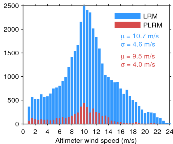
Figure 35. Histogram of science-valid wind over oceans and lakes for LRM (blue) and PLRM (red) for 12/04/2017. The mean ( \mu ) and standard deviation ( \sigma ) are also shown. Note that values larger than 24 m/s are excluded from the histogram for the sake of readability but not from the computation of \mu and \sigma .
