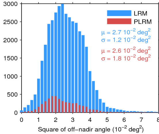
Figure 39. Histogram of flag-valid mispointing over oceans and lakes for LRM (blue) and PLRM (red) for 12/04/2017. Only positive values have been considered. The mean ( \mu ) and standard deviation ( \sigma ) are also shown. Note that values larger than 8 \cdot 10^{-2} \text{ deg}^2 are excluded from the histogram for the sake of readability but not from the computation of \mu and \sigma .
