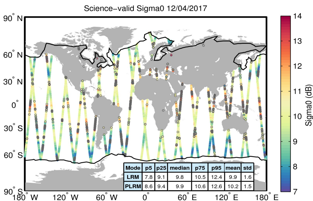
Figure 27. Geographical distribution of science-valid sigma0 data over oceans and lakes for 12/04/2017. The statistical values shown in the table refer to the sigma0 in dB and are calculated separately for LRM and PLRM regions. The black lines mark the outer limit of the Arctic and Antarctic polar polygons. Gray circles denote records that have been rejected based on the editing criteria described in Table 4.
