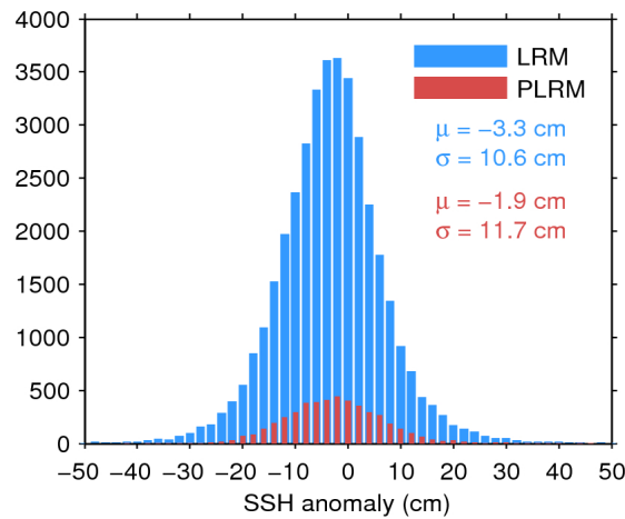
Figure 11. Histogram of science-valid SSH anomaly over oceans and lakes for LRM (blue) and PLRM (red) for 12/04/2017. The mean ( \mu ) and standard deviation ( \sigma ) are also shown. Note that values outside [-50 50] cm are excluded from the histogram for the sake of readability but not from the computation of \mu and \sigma .
