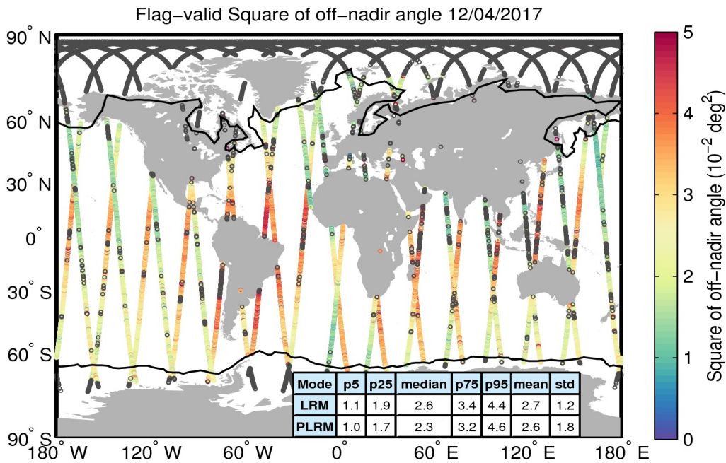
Figure 37. Geographical distribution of flag-valid mispointing data over oceans and lakes for 12/04/2017. The statistical values shown in the table refer to the mispointing in 10^{-2} deg 2 and are calculated separately for LRM and PLRM regions. Measurements taken over polar polygons have been excluded from the computation of the statistical values. The black lines mark the outer limit of the Arctic and Antarctic polar polygons. Gray circles denote negative values.
