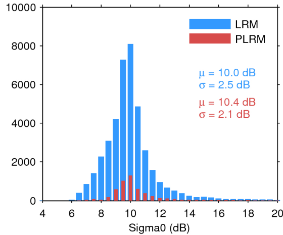
Figure 25. Histogram of flag-valid sigma0 over oceans and lakes for LRM (blue) and PLRM (red) for 12/04/2017. The mean ( \mu ) and standard deviation ( \sigma ) are also shown. Note that values outside [4 20] dB are excluded from the histogram for the sake of readability but not from the computation of \mu and \sigma .
