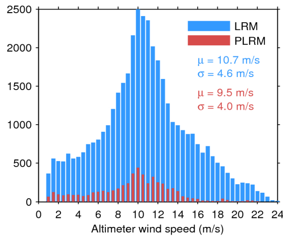
Figure 33. Histogram of flag-valid wind over oceans and lakes for LRM (blue) and PLRM (red) for 12/04/2017. The mean ( \mu ) and standard deviation ( \sigma ) are also shown. Note that values larger than 24 m/s are excluded from the histogram for the sake of readability but not from the computation of \mu and \sigma .
