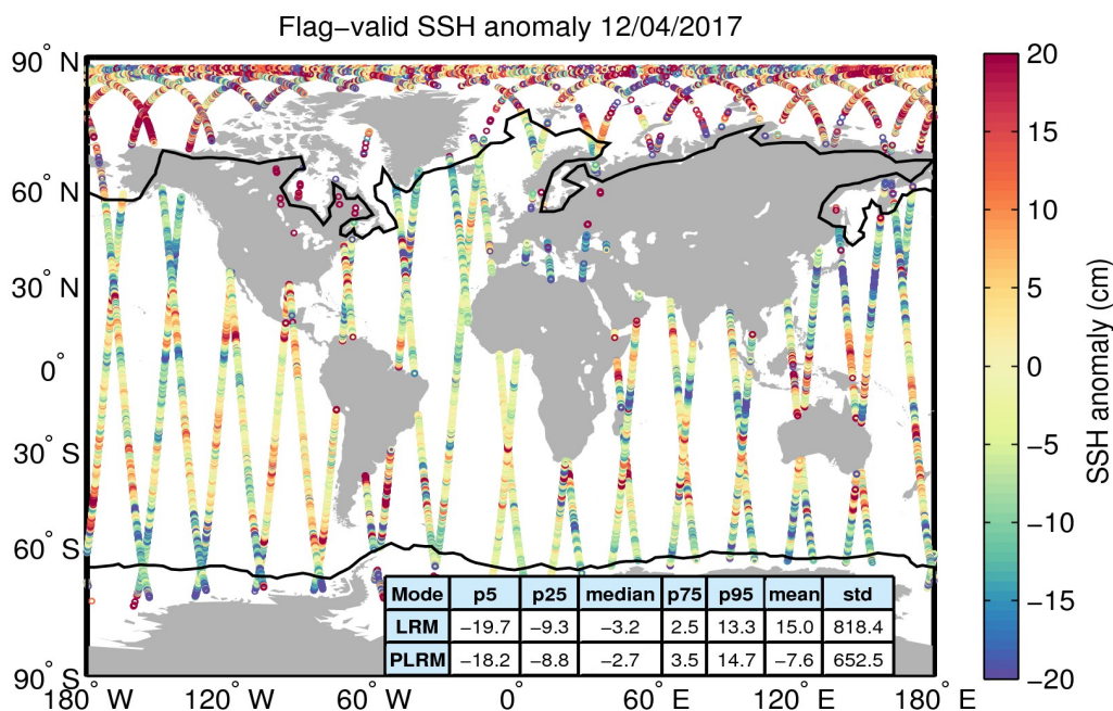
Figure 5. Geographical distribution of flag-valid 1-Hz SSH anomaly data over oceans and lakes for 12/04/2017. The statistical values shown in the table refer to the SSH anomaly in cm and are calculated separately for LRM and PLRM regions. Measurements taken over polar polygons have been excluded from the computation of the statistical values. The black lines mark the outer limit of the Arctic and Antarctic polar polygons.
