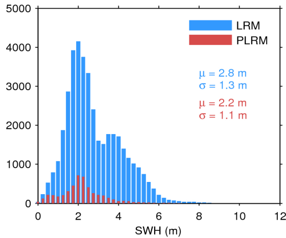
Figure 20. Histogram of science-valid SWH over oceans and lakes for LRM (blue) and PLRM (red) for 12/04/2017. The mean ( \mu ) and standard deviation ( \sigma ) are also shown. Note that values larger than 12 m are excluded from the histogram for the sake of readability but not from the computation of \mu and \sigma .
