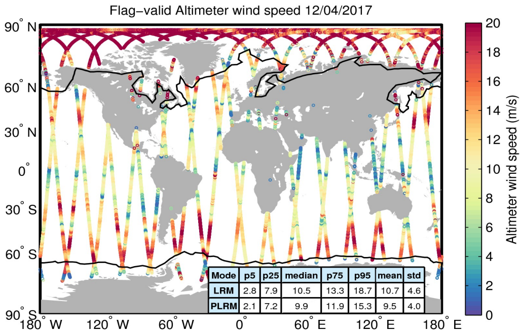
Figure 31. Geographical distribution of flag-valid wind data over oceans and lakes for 12/04/2017. The statistical values shown in the table refer to the wind in m/s and are calculated separately for LRM and PLRM regions. Measurements taken over polar polygons have been excluded from the computation of the statistical values. The black lines mark the outer limit of the Arctic and Antarctic polar polygons.
