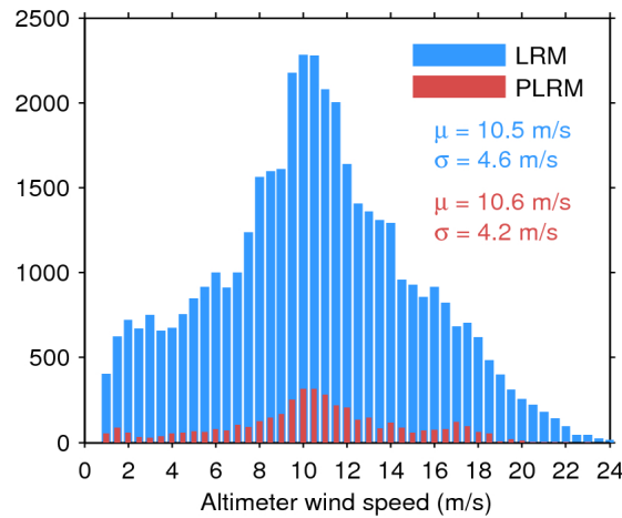
Figure 33. Histogram of flag-valid wind over oceans and lakes for LRM (blue) and PLRM (red) for 11/04/2017. The mean ( \mu ) and standard deviation ( \sigma ) are also shown. Note that values larger than 24 m/s are excluded from the histogram for the sake of readability but not from the computation of \mu and \sigma .
