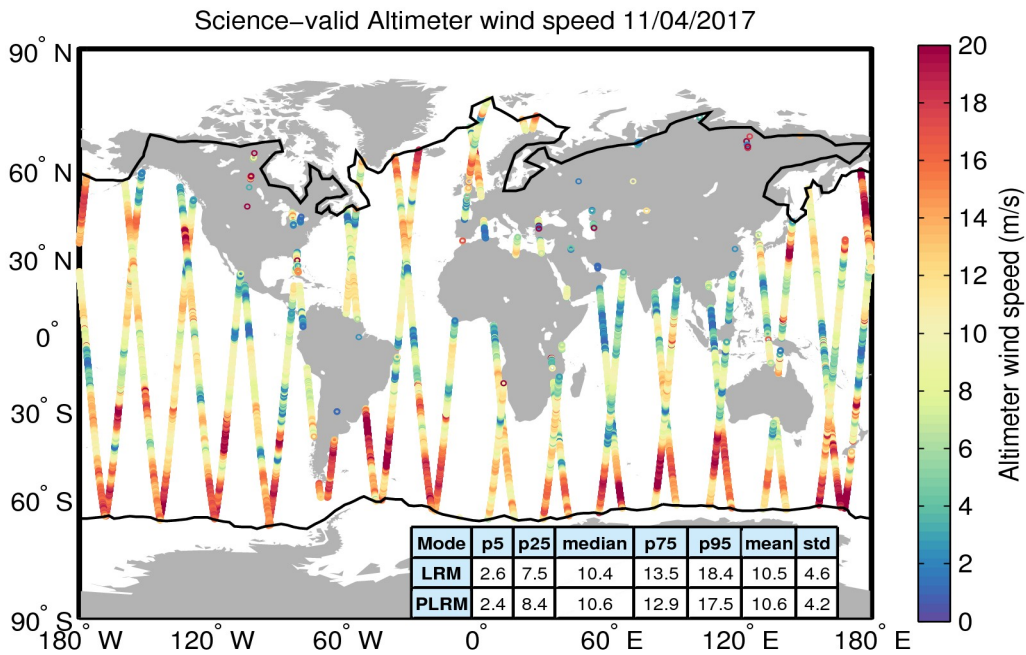
Figure 34. Geographical distribution of science-valid wind data over oceans and lakes for 11/04/2017. The statistical values shown in the table refer to the wind in m/s and are calculated separately for LRM and PLRM regions. The black lines mark the outer limit of the Arctic and Antarctic polar polygons. Gray circles denote records that have been rejected based on the editing criteria described in Table 5.
