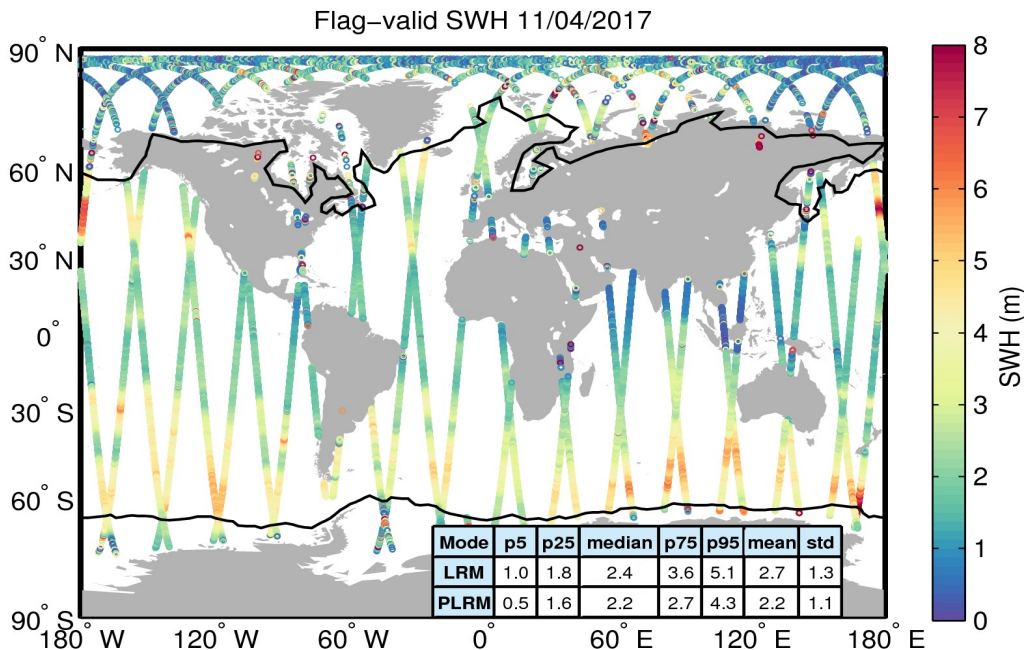
Figure 15. Geographical distribution of flag-valid SWH data over oceans and lakes for 11/04/2017. The statistical values shown in the table refer to the SWH in m and are calculated separately for LRM and PLRM regions. Measurements taken over polar polygons have been excluded from the computation of the statistical values. The black lines mark the outer limit of the Arctic and Antarctic polar polygons.
