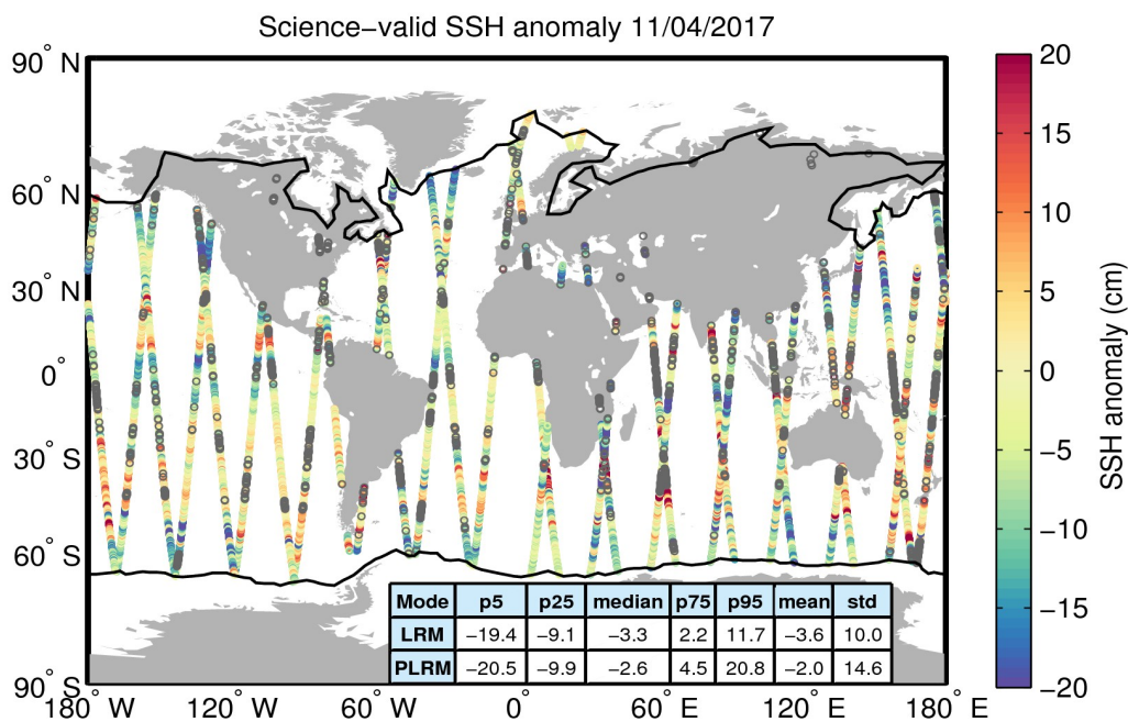
Figure 10. Geographical distribution of science-valid SSH anomaly data over oceans and lakes for 11/04/2017. The statistical values shown in the table refer to the SSH anomaly in cm and are calculated separately for LRM and PLRM regions. The black lines mark the outer limit of the Arctic and Antarctic polar polygons. Gray circles denote records that have been rejected based on the editing criteria described in Table 2.
