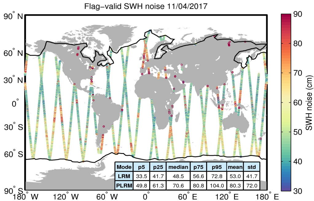
Figure 18. Geographical distribution of flag-valid 20-Hz SWH measurement noise over oceans and lakes for 11/04/2017. The statistical values shown in the table refer to the SWH noise and are calculated separately for LRM and PLRM regions. Measurements taken over polar polygons have been excluded from the computation of the statistical values. The black lines mark the outer limit of the Arctic and Antarctic polar polygons.
