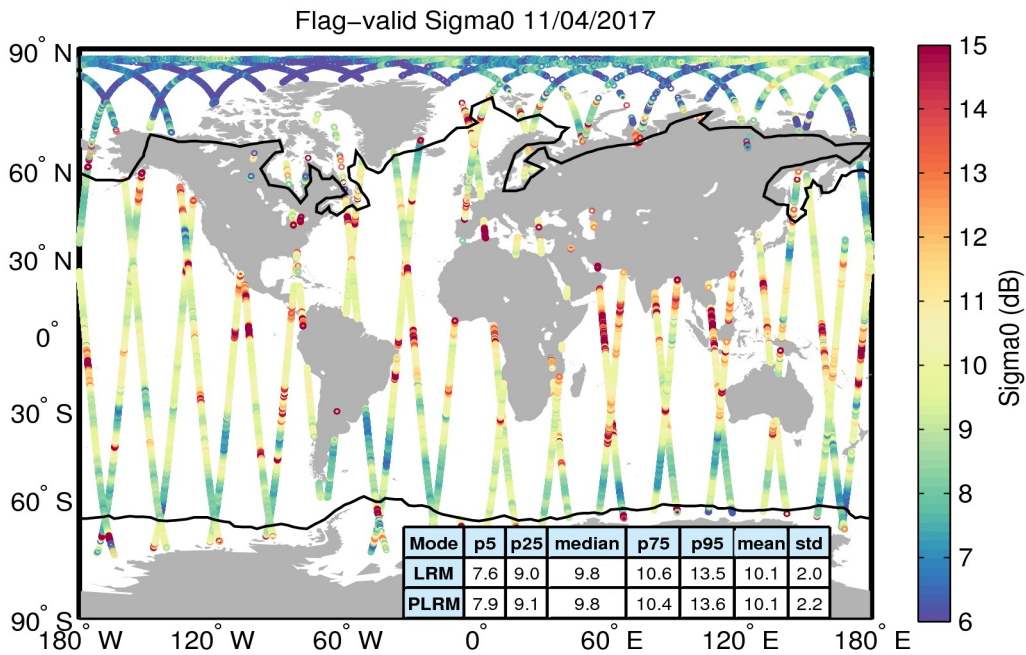
Figure 23. Geographical distribution of flag-valid sigma0 data over oceans and lakes for 11/04/2017. The statistical values shown in the table refer to the sigma0 in dB and are calculated separately for LRM and PLRM regions. Measurements taken over polar polygons have been excluded from the computation of the statistical values. The black lines mark the outer limit of the Arctic and Antarctic polar polygons.
