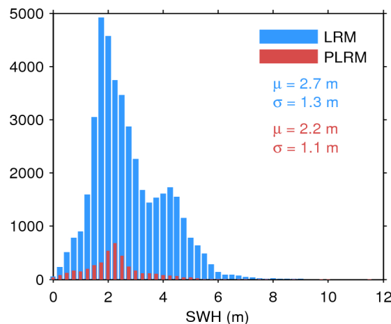
Figure 17. Histogram of flag-valid SWH over oceans and lakes for LRM (blue) and PLRM (red) for 11/04/2017. The mean ( \mu ) and standard deviation ( \sigma ) are also shown. Note that values larger than 12 m are excluded from the histogram for the sake of readability but not from the computation of \mu and \sigma .
