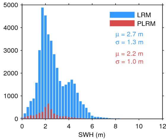
Figure 20. Histogram of science-valid SWH over oceans and lakes for LRM (blue) and PLRM (red) for 11/04/2017. The mean ( \mu ) and standard deviation ( \sigma ) are also shown. Note that values larger than 12 m are excluded from the histogram for the sake of readability but not from the computation of \mu and \sigma .
