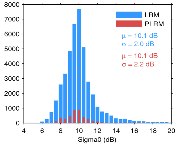
Figure 25. Histogram of flag-valid sigma0 over oceans and lakes for LRM (blue) and PLRM (red) for 11/04/2017. The mean ( \mu ) and standard deviation ( \sigma ) are also shown. Note that values outside [4 20] dB are excluded from the histogram for the sake of readability but not from the computation of \mu and \sigma .
