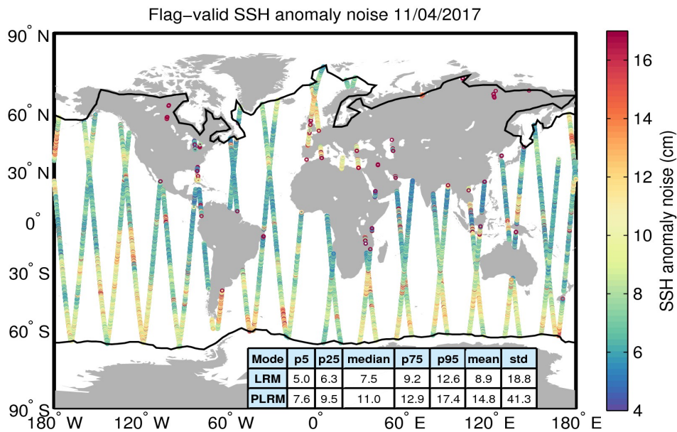
Figure 8. Geographical distribution of flag-valid 20-Hz SSH anomaly measurement noise over oceans and lakes for 11/04/2017. The statistical values shown in the table refer to the SSH anomaly noise and are calculated separately for LRM and PLRM regions. Measurements taken over polar polygons have been excluded from the computation of the statistical values. The black lines mark the outer limit of the Arctic and Antarctic polar polygons.
