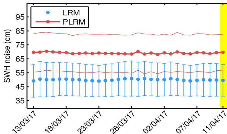
Figure 22. Average science-valid SWH noise for LRM (blue dot) and PLRM (red dot). The corresponding standard deviation (blue error bar and thin red lines, respectively) for each day in last 30-day window is also shown. The yellow shading highlights the day analyzed in this report.
