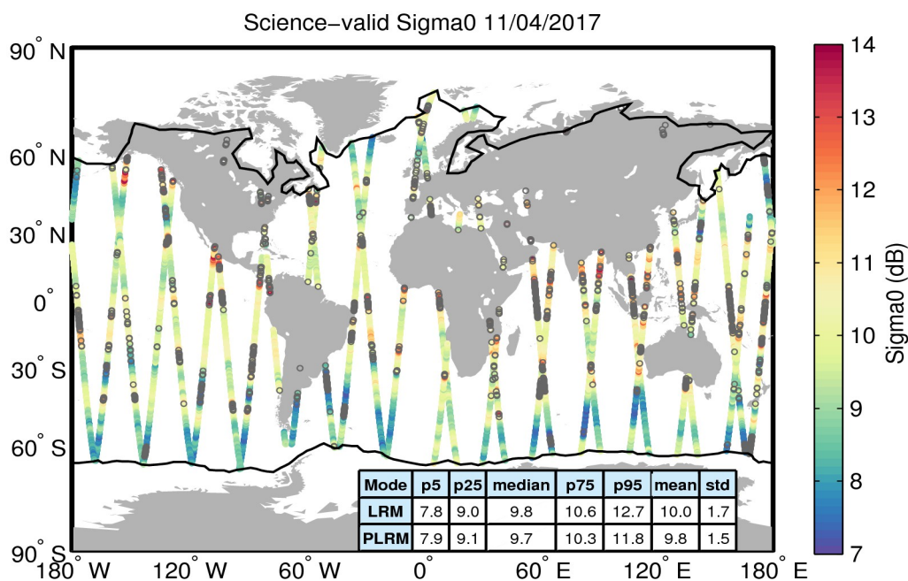
Figure 27. Geographical distribution of science-valid sigma0 data over oceans and lakes for 11/04/2017. The statistical values shown in the table refer to the sigma0 in dB and are calculated separately for LRM and PLRM regions. The black lines mark the outer limit of the Arctic and Antarctic polar polygons. Gray circles denote records that have been rejected based on the editing criteria described in Table 4.
