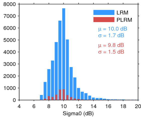
Figure 28. Histogram of science-valid sigma0 over oceans and lakes for LRM (blue) and PLRM (red) for 11/04/2017. The mean ( \mu ) and standard deviation ( \sigma ) are also shown. Note that values outside [4 20] dB are excluded from the histogram for the sake of readability but not from the computation of \mu and \sigma .
