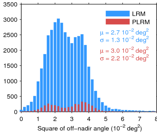
Figure 39. Histogram of flag-valid mispointing over oceans and lakes for LRM (blue) and PLRM (red) for 11/04/2017. Only positive values have been considered. The mean ( \mu ) and standard deviation ( \sigma ) are also shown. Note that values larger than 8 \cdot 10^{-2} \text{ deg}^2 are excluded from the histogram for the sake of readability but not from the computation of \mu and \sigma .
