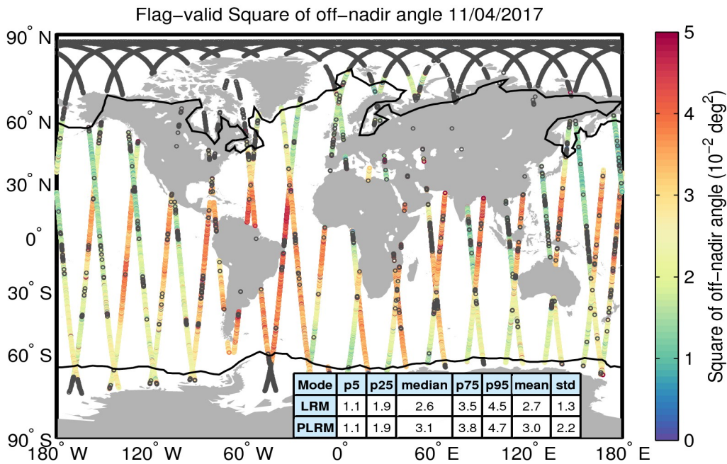
Figure 37. Geographical distribution of flag-valid mispointing data over oceans and lakes for 11/04/2017. The statistical values shown in the table refer to the mispointing in 10^{-2} deg 2 and are calculated separately for LRM and PLRM regions. Measurements taken over polar polygons have been excluded from the computation of the statistical values. The black lines mark the outer limit of the Arctic and Antarctic polar polygons. Gray circles denote negative values.
