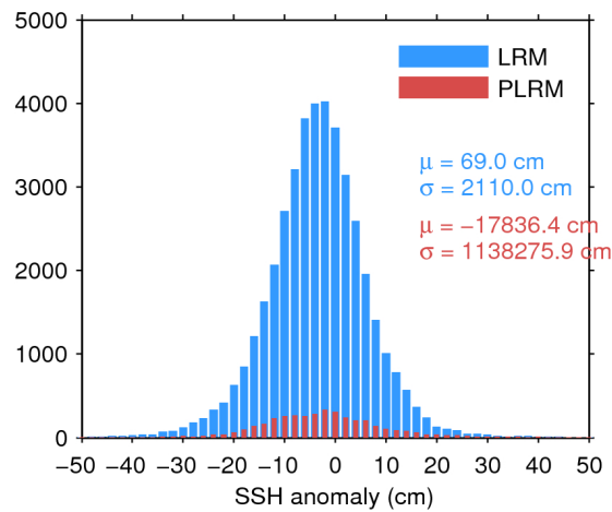
Figure 7. Histogram of flag-valid SSH anomaly over oceans and lakes for LRM (blue) and PLRM (red) for 11/04/2017. The mean ( \mu ) and standard deviation ( \sigma ) are also shown. Note that values outside [-50 50] cm are excluded from the histogram for the sake of readability but not from the computation of \mu and \sigma .
