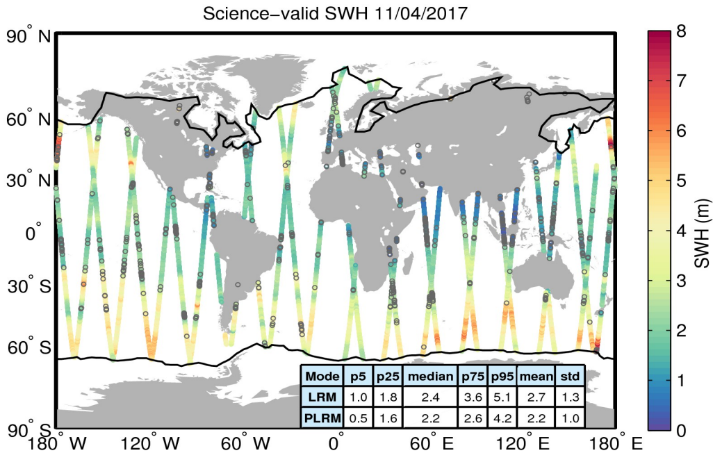
Figure 19. Geographical distribution of science-valid SWH data over oceans and lakes for 11/04/2017. The statistical values shown in the table refer to the SWH in m and are calculated separately for LRM and PLRM regions. The black lines mark the outer limit of the Arctic and Antarctic polar polygons. Gray circles denote records that have been rejected based on the editing criteria described in Table 3.
