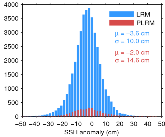
Figure 11. Histogram of science-valid SSH anomaly over oceans and lakes for LRM (blue) and PLRM (red) for 11/04/2017. The mean ( \mu ) and standard deviation ( \sigma ) are also shown. Note that values outside [-50 50] cm are excluded from the histogram for the sake of readability but not from the computation of \mu and \sigma .
