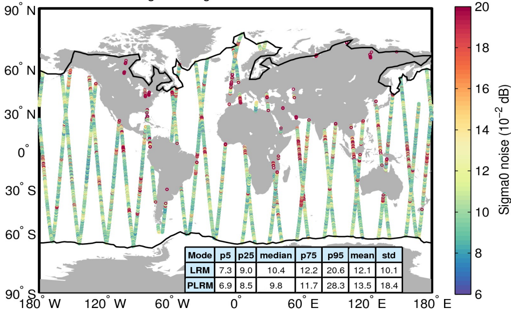
Flag-valid sigma0 noise 11/04/2017
