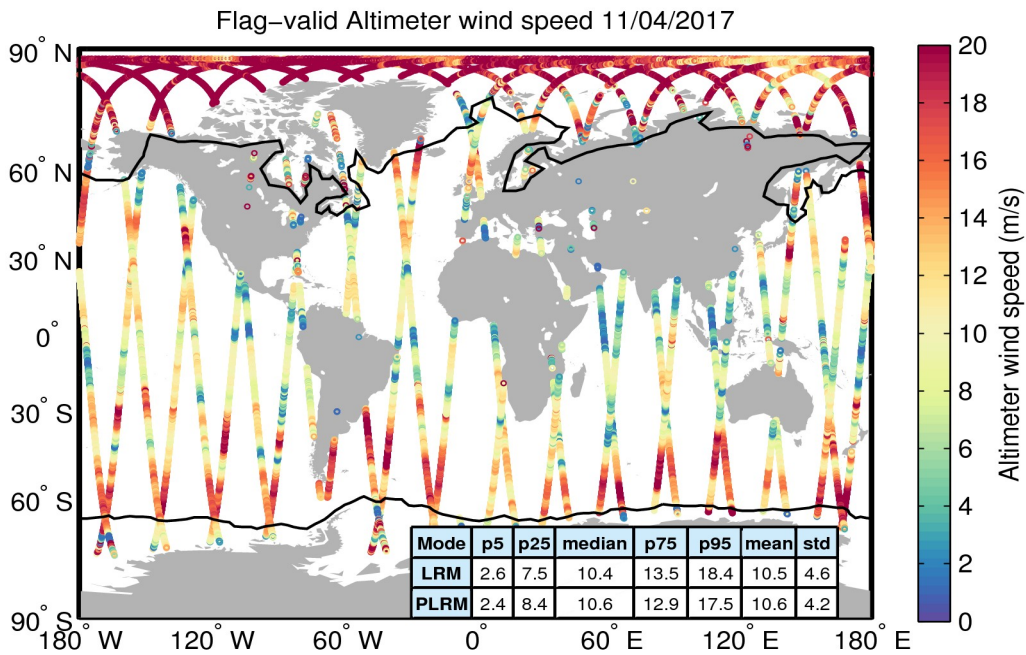
Figure 31. Geographical distribution of flag-valid wind data over oceans and lakes for 11/04/2017. The statistical values shown in the table refer to the wind in m/s and are calculated separately for LRM and PLRM regions. Measurements taken over polar polygons have been excluded from the computation of the statistical values. The black lines mark the outer limit of the Arctic and Antarctic polar polygons.
