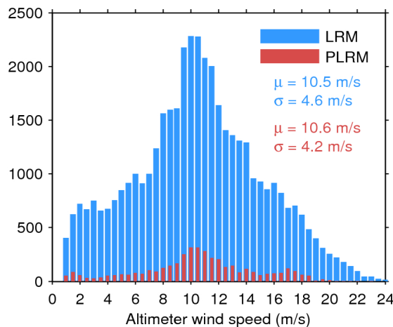
Figure 35. Histogram of science-valid wind over oceans and lakes for LRM (blue) and PLRM (red) for 11/04/2017. The mean ( \mu ) and standard deviation ( \sigma ) are also shown. Note that values larger than 24 m/s are excluded from the histogram for the sake of readability but not from the computation of \mu and \sigma .
