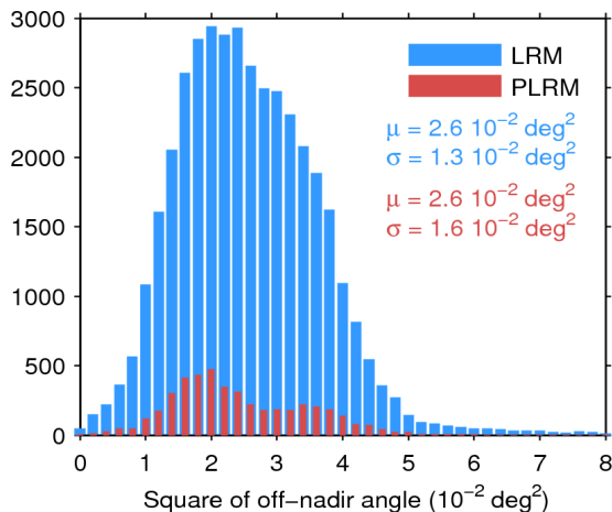
Figure 39. Histogram of flag-valid mispointing over oceans and lakes for LRM (blue) and PLRM (red) for 10/04/2017. Only positive values have been considered. The mean ( \mu ) and standard deviation ( \sigma ) are also shown. Note that values larger than 8 \times 10^{-2} \text{ deg}^2 are excluded from the histogram for the sake of readability but not from the computation of \mu and \sigma .
