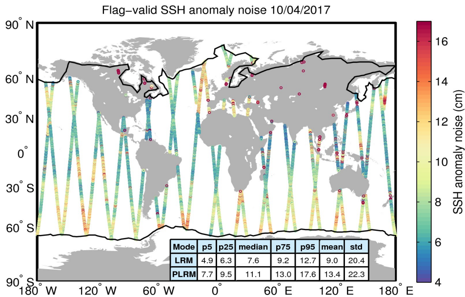
Figure 8. Geographical distribution of flag-valid 20-Hz SSH anomaly measurement noise over oceans and lakes for 10/04/2017. The statistical values shown in the table refer to the SSH anomaly noise and are calculated separately for LRM and PLRM regions. Measurements taken over polar polygons have been excluded from the computation of the statistical values. The black lines mark the outer limit of the Arctic and Antarctic polar polygons.
