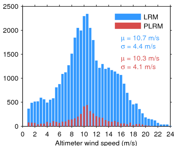
Figure 33. Histogram of flag-valid wind over oceans and lakes for LRM (blue) and PLRM (red) for 10/04/2017. The mean ( \mu ) and standard deviation ( \sigma ) are also shown. Note that values larger than 24 m/s are excluded from the histogram for the sake of readability but not from the computation of \mu and \sigma .
