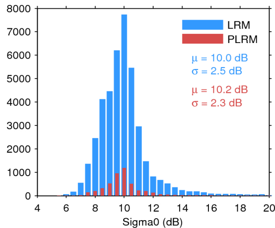
Figure 25. Histogram of flag-valid sigma0 over oceans and lakes for LRM (blue) and PLRM (red) for 10/04/2017. The mean ( \mu ) and standard deviation ( \sigma ) are also shown. Note that values outside [4 20] dB are excluded from the histogram for the sake of readability but not from the computation of \mu and \sigma .
