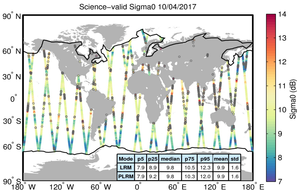
Figure 27. Geographical distribution of science-valid sigma0 data over oceans and lakes for 10/04/2017. The statistical values shown in the table refer to the sigma0 in dB and are calculated separately for LRM and PLRM regions. The black lines mark the outer limit of the Arctic and Antarctic polar polygons. Gray circles denote records that have been rejected based on the editing criteria described in Table 4.
