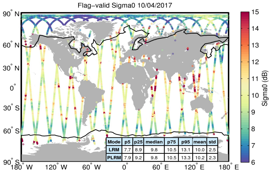
Figure 23. Geographical distribution of flag-valid sigma0 data over oceans and lakes for 10/04/2017. The statistical values shown in the table refer to the sigma0 in dB and are calculated separately for LRM and PLRM regions. Measurements taken over polar polygons have been excluded from the computation of the statistical values. The black lines mark the outer limit of the Arctic and Antarctic polar polygons.
