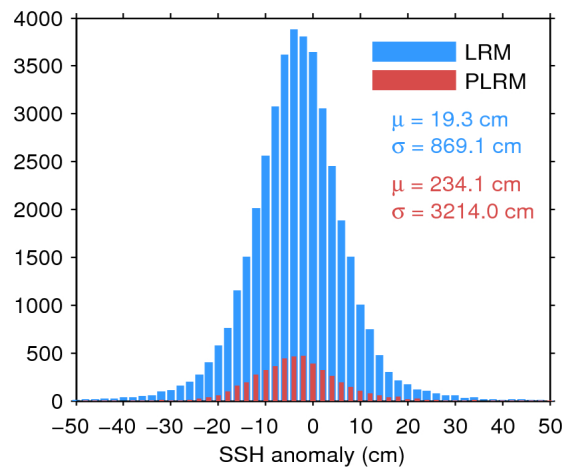
Figure 7. Histogram of flag-valid SSH anomaly over oceans and lakes for LRM (blue) and PLRM (red) for 10/04/2017. The mean ( \mu ) and standard deviation ( \sigma ) are also shown. Note that values outside [-50 50] cm are excluded from the histogram for the sake of readability but not from the computation of \mu and \sigma .
