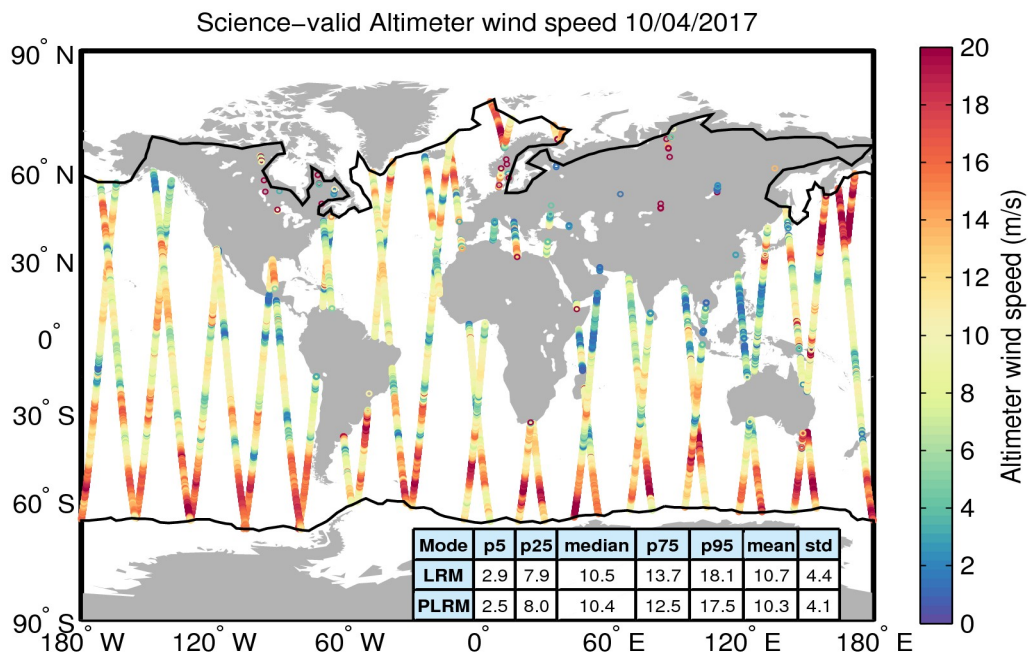
Figure 34. Geographical distribution of science-valid wind data over oceans and lakes for 10/04/2017. The statistical values shown in the table refer to the wind in m/s and are calculated separately for LRM and PLRM regions. The black lines mark the outer limit of the Arctic and Antarctic polar polygons. Gray circles denote records that have been rejected based on the editing criteria described in Table 5.
