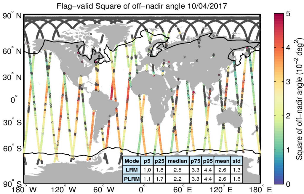
Figure 37. Geographical distribution of flag-valid mispointing data over oceans and lakes for 10/04/2017. The statistical values shown in the table refer to the mispointing in 10^{-2} deg 2 and are calculated separately for LRM and PLRM regions. Measurements taken over polar polygons have been excluded from the computation of the statistical values. The black lines mark the outer limit of the Arctic and Antarctic polar polygons. Gray circles denote negative values.
