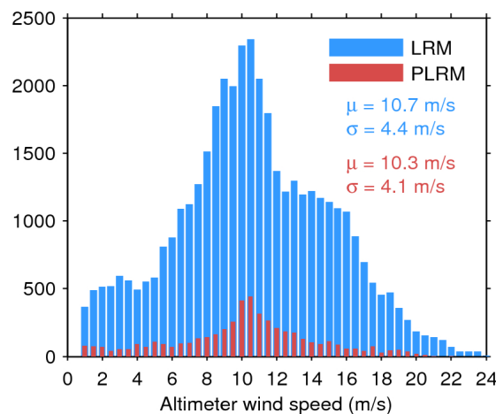
Figure 35. Histogram of science-valid wind over oceans and lakes for LRM (blue) and PLRM (red) for 10/04/2017. The mean ( \mu ) and standard deviation ( \sigma ) are also shown. Note that values larger than 24 m/s are excluded from the histogram for the sake of readability but not from the computation of \mu and \sigma .
