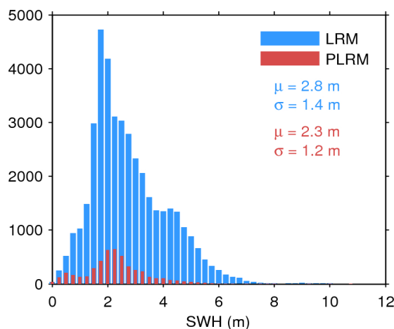
Figure 17. Histogram of flag-valid SWH over oceans and lakes for LRM (blue) and PLRM (red) for 10/04/2017. The mean ( \mu ) and standard deviation ( \sigma ) are also shown. Note that values larger than 12 m are excluded from the histogram for the sake of readability but not from the computation of \mu and \sigma .
