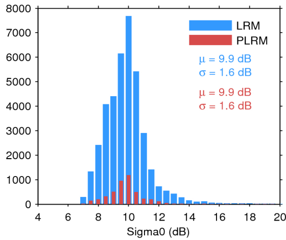
Figure 28. Histogram of science-valid sigma0 over oceans and lakes for LRM (blue) and PLRM (red) for 10/04/2017. The mean ( \mu ) and standard deviation ( \sigma ) are also shown. Note that values outside [4 20] dB are excluded from the histogram for the sake of readability but not from the computation of \mu and \sigma .
