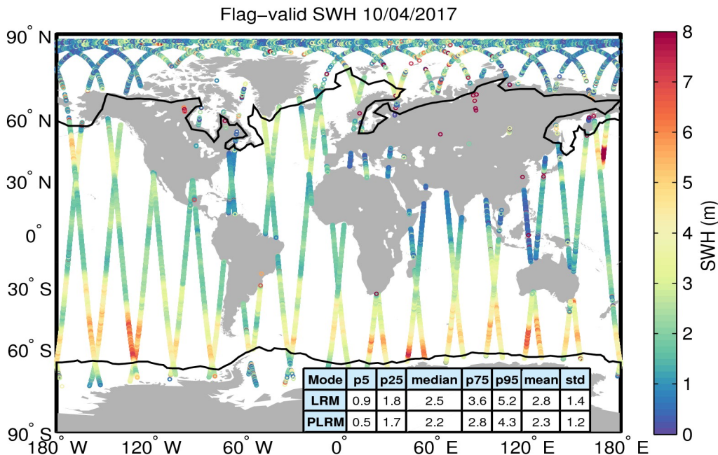
Figure 15. Geographical distribution of flag-valid SWH data over oceans and lakes for 10/04/2017. The statistical values shown in the table refer to the SWH in m and are calculated separately for LRM and PLRM regions. Measurements taken over polar polygons have been excluded from the computation of the statistical values. The black lines mark the outer limit of the Arctic and Antarctic polar polygons.
