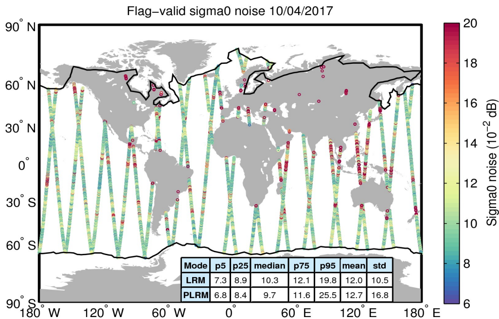
Figure 26. Geographical distribution of flag-valid 20-Hz sigma0 measurement noise over oceans and lakes for 10/04/2017. The statistical values shown in the table refer to the sigma0 noise and are calculated separately for LRM and PLRM regions. Measurements taken over polar polygons have been excluded from the computation of the statistical values. The black lines mark the outer limit of the Arctic and Antarctic polar polygons.
