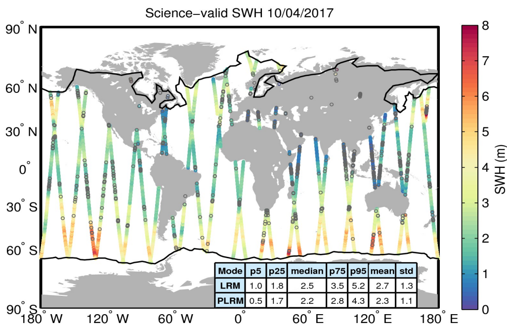
Figure 19. Geographical distribution of science-valid SWH data over oceans and lakes for 10/04/2017. The statistical values shown in the table refer to the SWH in m and are calculated separately for LRM and PLRM regions. The black lines mark the outer limit of the Arctic and Antarctic polar polygons. Gray circles denote records that have been rejected based on the editing criteria described in Table 3.
