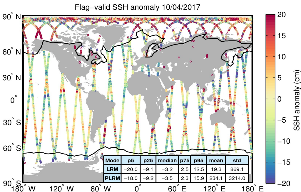
Figure 5. Geographical distribution of flag-valid 1-Hz SSH anomaly data over oceans and lakes for 10/04/2017. The statistical values shown in the table refer to the SSH anomaly in cm and are calculated separately for LRM and PLRM regions. Measurements taken over polar polygons have been excluded from the computation of the statistical values. The black lines mark the outer limit of the Arctic and Antarctic polar polygons.
