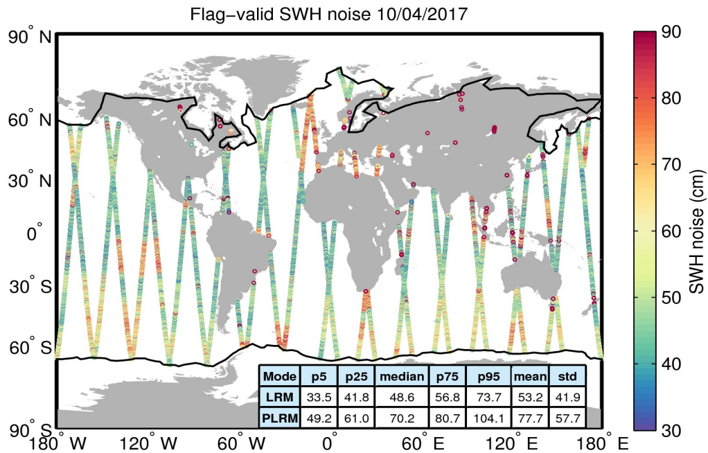
Figure 18. Geographical distribution of flag-valid 20-Hz SWH measurement noise over oceans and lakes for 10/04/2017. The statistical values shown in the table refer to the SWH noise and are calculated separately for LRM and PLRM regions. Measurements taken over polar polygons have been excluded from the computation of the statistical values. The black lines mark the outer limit of the Arctic and Antarctic polar polygons.
