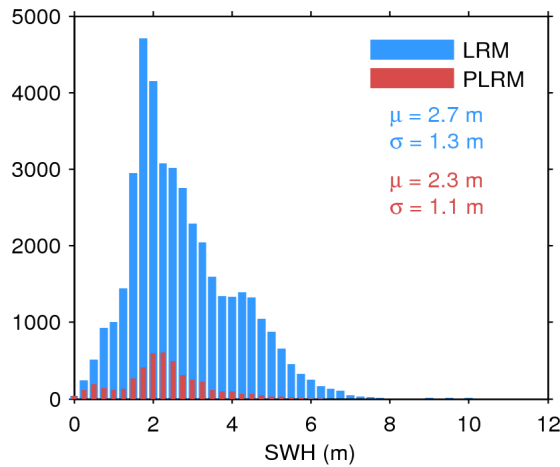
Figure 20. Histogram of science-valid SWH over oceans and lakes for LRM (blue) and PLRM (red) for 10/04/2017. The mean ( \mu ) and standard deviation ( \sigma ) are also shown. Note that values larger than 12 m are excluded from the histogram for the sake of readability but not from the computation of \mu and \sigma .
