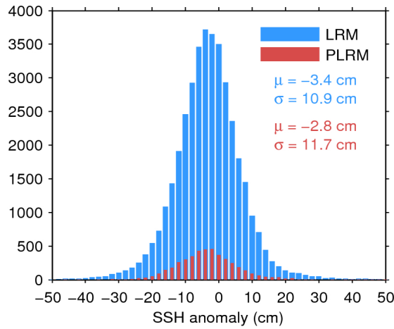
Figure 11. Histogram of science-valid SSH anomaly over oceans and lakes for LRM (blue) and PLRM (red) for 10/04/2017. The mean ( \mu ) and standard deviation ( \sigma ) are also shown. Note that values outside [-50\ 50] cm are excluded from the histogram for the sake of readability but not from the computation of \mu and \sigma .
