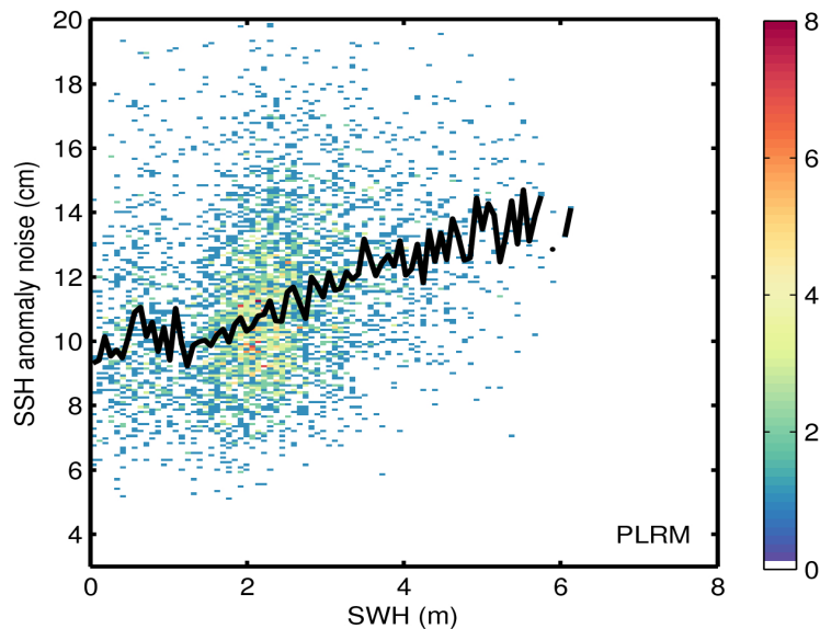
Figure 9. 2D histogram showing flag-valid SSH anomaly noise as a function of SWH for LRM (top) and PLRM (bottom) for 10/04/2017. The black line denotes the median SSH anomaly noise as a function of SWH.
