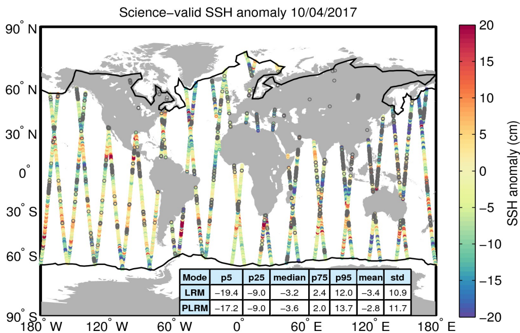
Figure 10. Geographical distribution of science-valid SSH anomaly data over oceans and lakes for 10/04/2017. The statistical values shown in the table refer to the SSH anomaly in cm and are calculated separately for LRM and PLRM regions. The black lines mark the outer limit of the Arctic and Antarctic polar polygons. Gray circles denote records that have been rejected based on the editing criteria described in Table 2.
