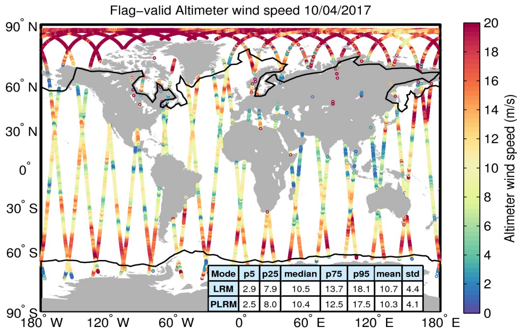
Figure 31. Geographical distribution of flag-valid wind data over oceans and lakes for 10/04/2017. The statistical values shown in the table refer to the wind in m/s and are calculated separately for LRM and PLRM regions. Measurements taken over polar polygons have been excluded from the computation of the statistical values. The black lines mark the outer limit of the Arctic and Antarctic polar polygons.
