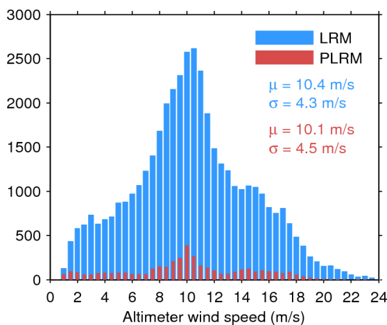
Figure 33. Histogram of flag-valid wind over oceans and lakes for LRM (blue) and PLRM (red) for 09/04/2017. The mean ( \mu ) and standard deviation ( \sigma ) are also shown. Note that values larger than 24 m/s are excluded from the histogram for the sake of readability but not from the computation of \mu and \sigma .
