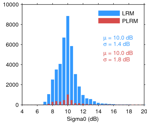
Figure 28. Histogram of science-valid sigma0 over oceans and lakes for LRM (blue) and PLRM (red) for 09/04/2017. The mean ( \mu ) and standard deviation ( \sigma ) are also shown. Note that values outside [4 20] dB are excluded from the histogram for the sake of readability but not from the computation of \mu and \sigma .
