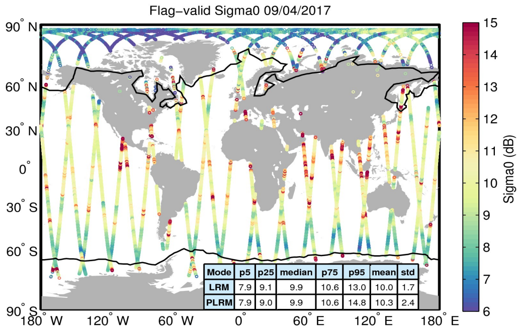
Figure 23. Geographical distribution of flag-valid sigma0 data over oceans and lakes for 09/04/2017. The statistical values shown in the table refer to the sigma0 in dB and are calculated separately for LRM and PLRM regions. Measurements taken over polar polygons have been excluded from the computation of the statistical values. The black lines mark the outer limit of the Arctic and Antarctic polar polygons.
