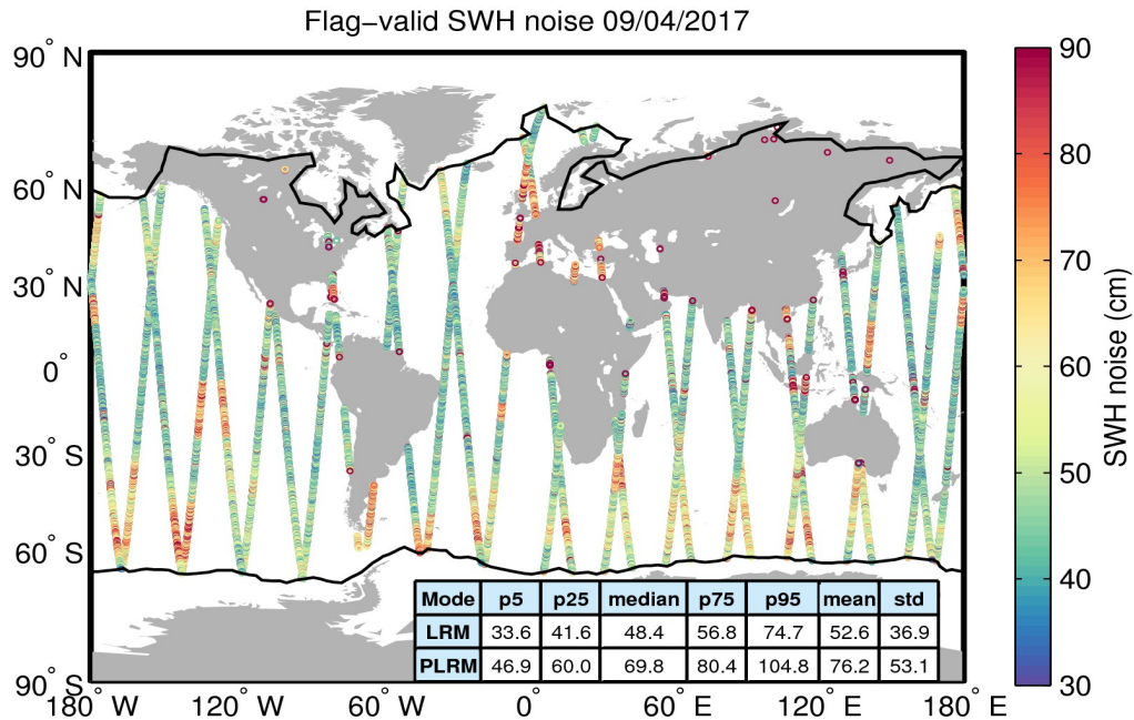
Figure 18. Geographical distribution of flag-valid 20-Hz SWH measurement noise over oceans and lakes for 09/04/2017. The statistical values shown in the table refer to the SWH noise and are calculated separately for LRM and PLRM regions. Measurements taken over polar polygons have been excluded from the computation of the statistical values. The black lines mark the outer limit of the Arctic and Antarctic polar polygons.
