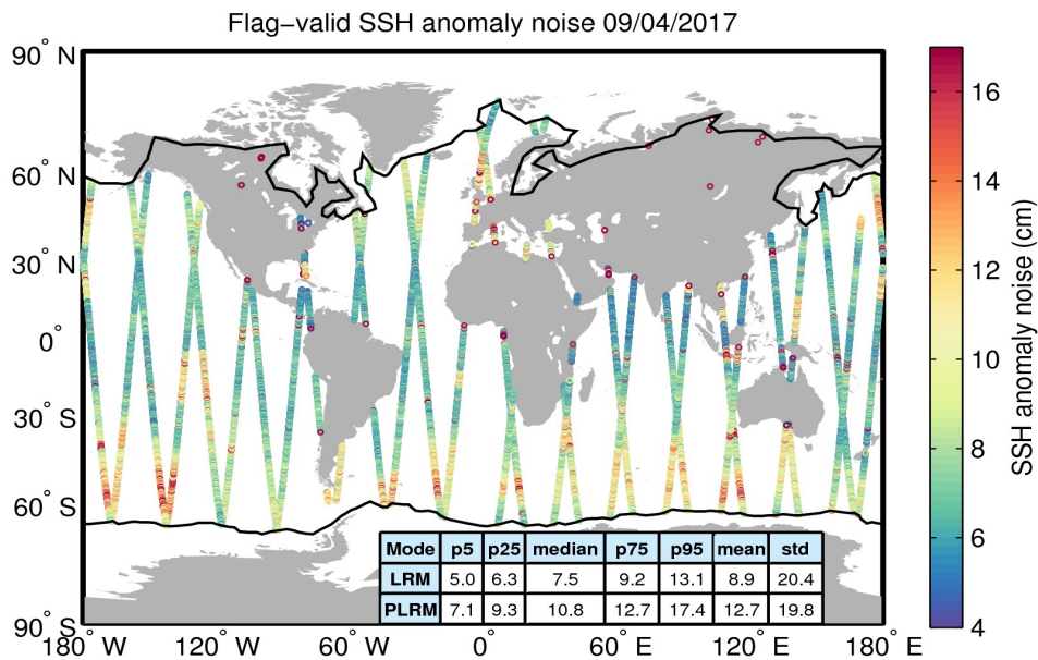
Figure 8. Geographical distribution of flag-valid 20-Hz SSH anomaly measurement noise over oceans and lakes for 09/04/2017. The statistical values shown in the table refer to the SSH anomaly noise and are calculated separately for LRM and PLRM regions. Measurements taken over polar polygons have been excluded from the computation of the statistical values. The black lines mark the outer limit of the Arctic and Antarctic polar polygons.
