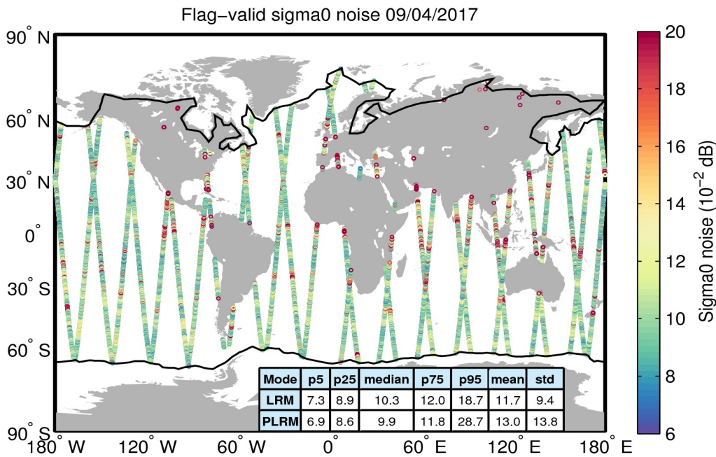
Figure 26. Geographical distribution of flag-valid 20-Hz sigma0 measurement noise over oceans and lakes for 09/04/2017. The statistical values shown in the table refer to the sigma0 noise and are calculated separately for LRM and PLRM regions. Measurements taken over polar polygons have been excluded from the computation of the statistical values. The black lines mark the outer limit of the Arctic and Antarctic polar polygons.
