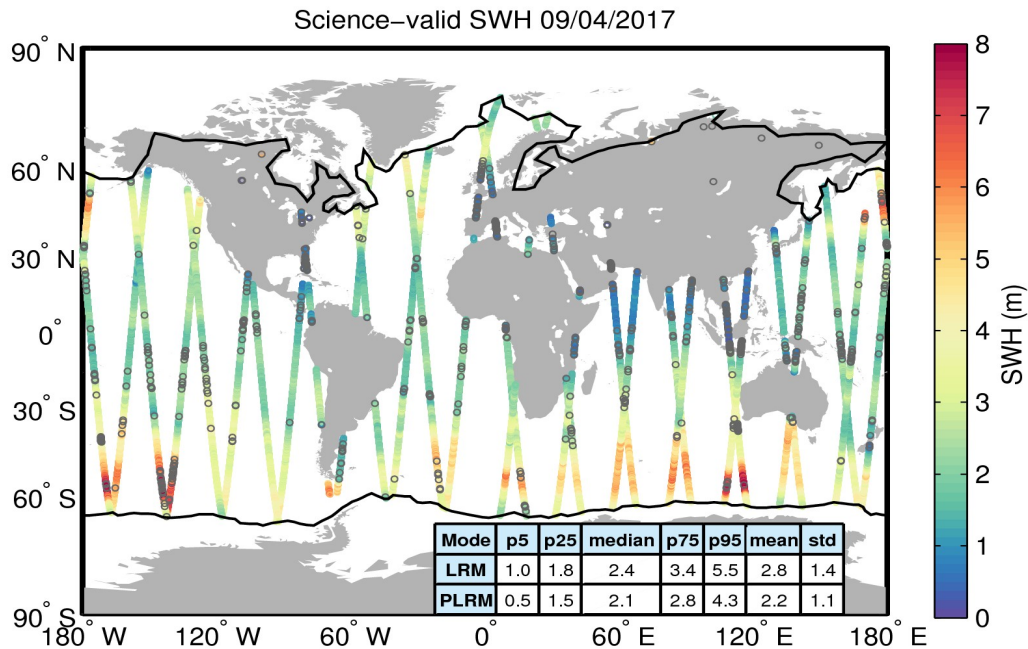
Figure 19. Geographical distribution of science-valid SWH data over oceans and lakes for 09/04/2017. The statistical values shown in the table refer to the SWH in m and are calculated separately for LRM and PLRM regions. The black lines mark the outer limit of the Arctic and Antarctic polar polygons. Gray circles denote records that have been rejected based on the editing criteria described in Table 3.
