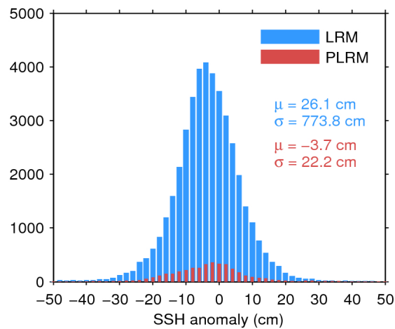
Figure 7. Histogram of flag-valid SSH anomaly over oceans and lakes for LRM (blue) and PLRM (red) for 09/04/2017. The mean ( \mu ) and standard deviation ( \sigma ) are also shown. Note that values outside [-50 50] cm are excluded from the histogram for the sake of readability but not from the computation of \mu and \sigma .
