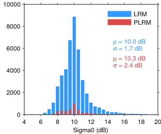
Figure 25. Histogram of flag-valid sigma0 over oceans and lakes for LRM (blue) and PLRM (red) for 09/04/2017. The mean ( \mu ) and standard deviation ( \sigma ) are also shown. Note that values outside [4 20] dB are excluded from the histogram for the sake of readability but not from the computation of \mu and \sigma .
