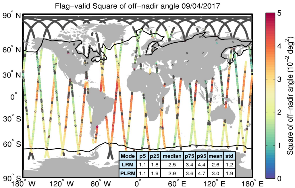
Figure 37. Geographical distribution of flag-valid mispointing data over oceans and lakes for 09/04/2017. The statistical values shown in the table refer to the mispointing in 10^{-2} deg 2 and are calculated separately for LRM and PLRM regions. Measurements taken over polar polygons have been excluded from the computation of the statistical values. The black lines mark the outer limit of the Arctic and Antarctic polar polygons. Gray circles denote negative values.
