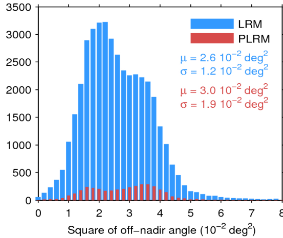
Figure 39. Histogram of flag-valid mispointing over oceans and lakes for LRM (blue) and PLRM (red) for 09/04/2017. Only positive values have been considered. The mean ( \mu ) and standard deviation ( \sigma ) are also shown. Note that values larger than 8 \cdot 10^{-2} \text{ deg}^2 are excluded from the histogram for the sake of readability but not from the computation of \mu and \sigma .
