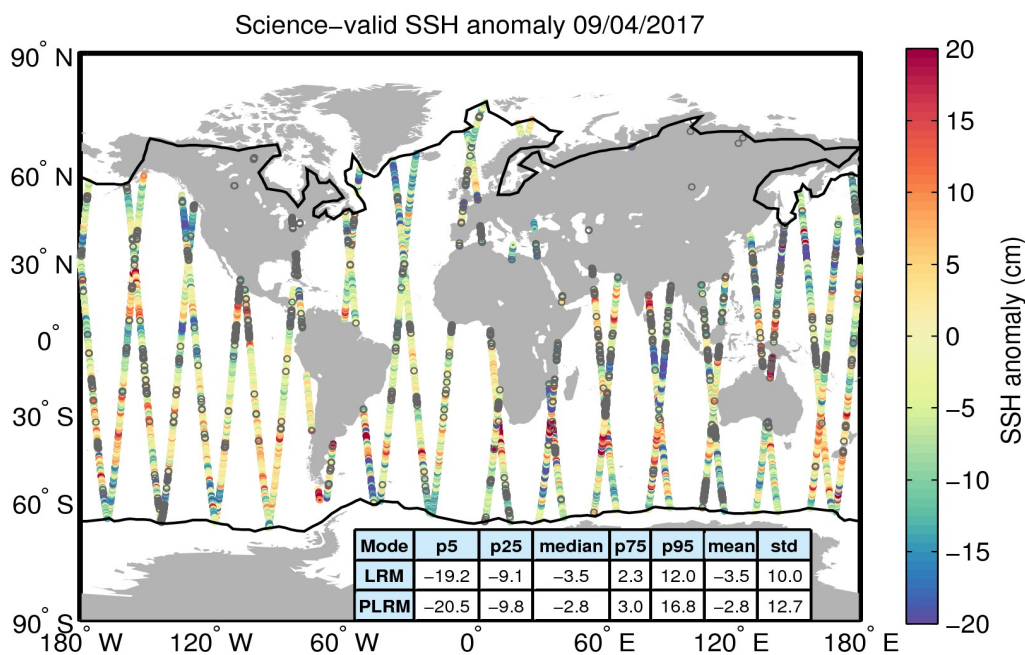
Figure 10. Geographical distribution of science-valid SSH anomaly data over oceans and lakes for 09/04/2017. The statistical values shown in the table refer to the SSH anomaly in cm and are calculated separately for LRM and PLRM regions. The black lines mark the outer limit of the Arctic and Antarctic polar polygons. Gray circles denote records that have been rejected based on the editing criteria described in Table 2.
