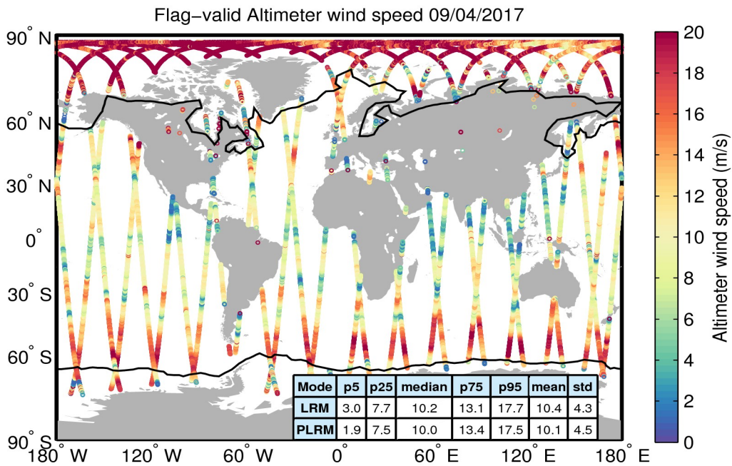
Figure 31. Geographical distribution of flag-valid wind data over oceans and lakes for 09/04/2017. The statistical values shown in the table refer to the wind in m/s and are calculated separately for LRM and PLRM regions. Measurements taken over polar polygons have been excluded from the computation of the statistical values. The black lines mark the outer limit of the Arctic and Antarctic polar polygons.
