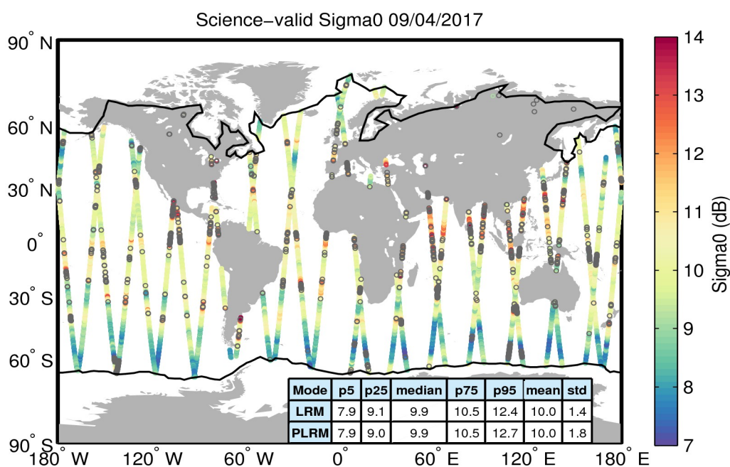
Figure 27. Geographical distribution of science-valid sigma0 data over oceans and lakes for 09/04/2017. The statistical values shown in the table refer to the sigma0 in dB and are calculated separately for LRM and PLRM regions. The black lines mark the outer limit of the Arctic and Antarctic polar polygons. Gray circles denote records that have been rejected based on the editing criteria described in Table 4.
