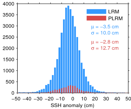
Figure 11. Histogram of science-valid SSH anomaly over oceans and lakes for LRM (blue) and PLRM (red) for 09/04/2017. The mean ( \mu ) and standard deviation ( \sigma ) are also shown. Note that values outside [-50\ 50] cm are excluded from the histogram for the sake of readability but not from the computation of \mu and \sigma .
