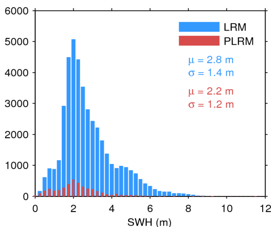
Figure 17. Histogram of flag-valid SWH over oceans and lakes for LRM (blue) and PLRM (red) for 09/04/2017. The mean ( \mu ) and standard deviation ( \sigma ) are also shown. Note that values larger than 12 m are excluded from the histogram for the sake of readability but not from the computation of \mu and \sigma .
