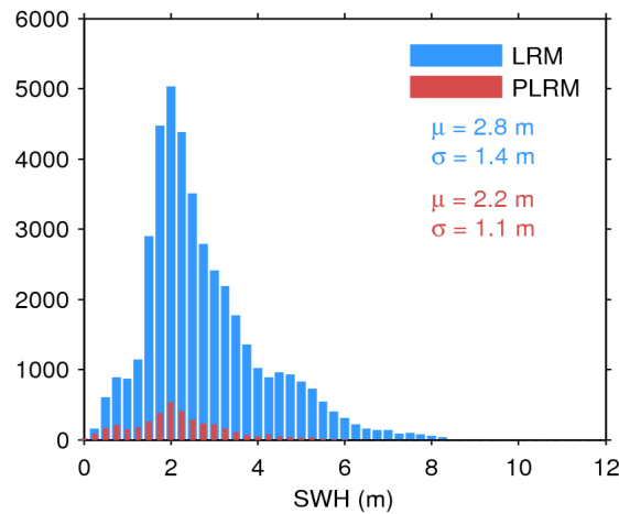
Figure 20. Histogram of science-valid SWH over oceans and lakes for LRM (blue) and PLRM (red) for 09/04/2017. The mean ( \mu ) and standard deviation ( \sigma ) are also shown. Note that values larger than 12 m are excluded from the histogram for the sake of readability but not from the computation of \mu and \sigma .
