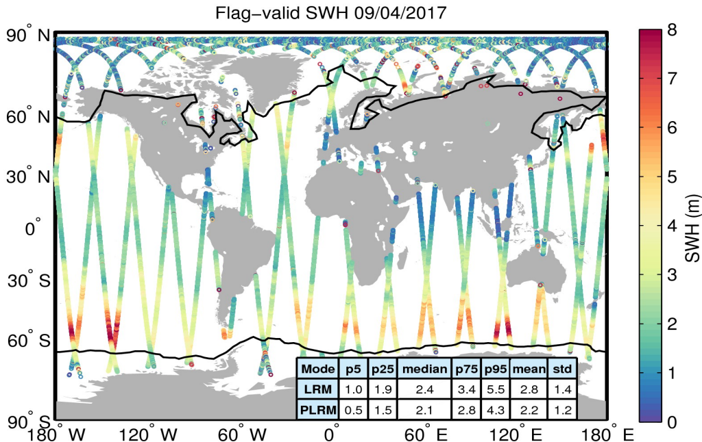
Figure 15. Geographical distribution of flag-valid SWH data over oceans and lakes for 09/04/2017. The statistical values shown in the table refer to the SWH in m and are calculated separately for LRM and PLRM regions. Measurements taken over polar polygons have been excluded from the computation of the statistical values. The black lines mark the outer limit of the Arctic and Antarctic polar polygons.
