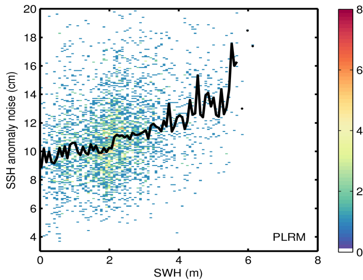
Figure 9. 2D histogram showing flag-valid SSH anomaly noise as a function of SWH for LRM (top) and PLRM (bottom) for 09/04/2017. The black line denotes the median SSH anomaly noise as a function of SWH.
