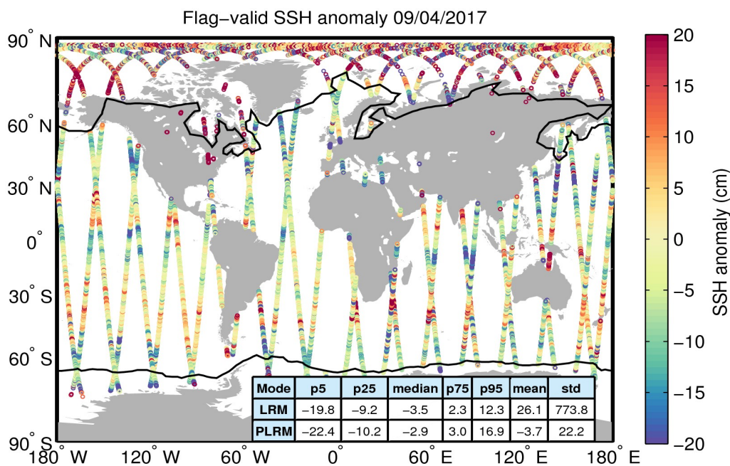
Figure 5. Geographical distribution of flag-valid 1-Hz SSH anomaly data over oceans and lakes for 09/04/2017. The statistical values shown in the table refer to the SSH anomaly in cm and are calculated separately for LRM and PLRM regions. Measurements taken over polar polygons have been excluded from the computation of the statistical values. The black lines mark the outer limit of the Arctic and Antarctic polar polygons.
