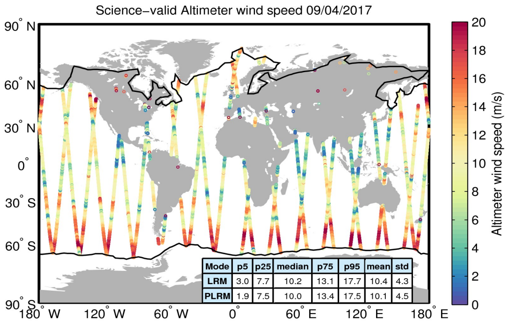
Figure 34. Geographical distribution of science-valid wind data over oceans and lakes for 09/04/2017. The statistical values shown in the table refer to the wind in m/s and are calculated separately for LRM and PLRM regions. The black lines mark the outer limit of the Arctic and Antarctic polar polygons. Gray circles denote records that have been rejected based on the editing criteria described in Table 5.
