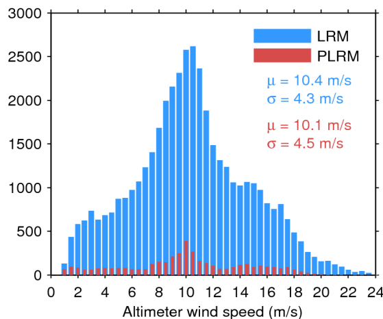
Figure 35. Histogram of science-valid wind over oceans and lakes for LRM (blue) and PLRM (red) for 09/04/2017. The mean ( \mu ) and standard deviation ( \sigma ) are also shown. Note that values larger than 24 m/s are excluded from the histogram for the sake of readability but not from the computation of \mu and \sigma .
