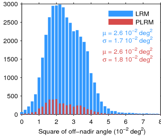
Figure 39. Histogram of flag-valid mispointing over oceans and lakes for LRM (blue) and PLRM (red) for 08/04/2017. Only positive values have been considered. The mean ( \mu ) and standard deviation ( \sigma ) are also shown. Note that values larger than 8 \cdot 10^{-2} \text{ deg}^2 are excluded from the histogram for the sake of readability but not from the computation of \mu and \sigma .
