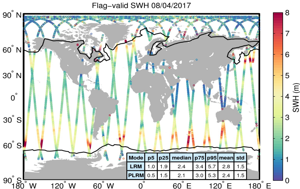
Figure 15. Geographical distribution of flag-valid SWH data over oceans and lakes for 08/04/2017. The statistical values shown in the table refer to the SWH in m and are calculated separately for LRM and PLRM regions. Measurements taken over polar polygons have been excluded from the computation of the statistical values. The black lines mark the outer limit of the Arctic and Antarctic polar polygons.
