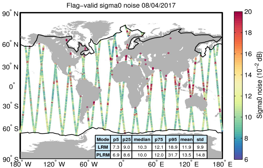
Figure 26. Geographical distribution of flag-valid 20-Hz sigma0 measurement noise over oceans and lakes for 08/04/2017. The statistical values shown in the table refer to the sigma0 noise and are calculated separately for LRM and PLRM regions. Measurements taken over polar polygons have been excluded from the computation of the statistical values. The black lines mark the outer limit of the Arctic and Antarctic polar polygons.
