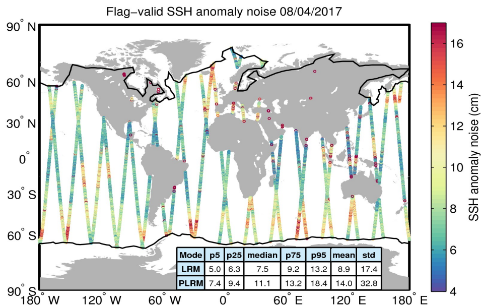
Figure 8. Geographical distribution of flag-valid 20-Hz SSH anomaly measurement noise over oceans and lakes for 08/04/2017. The statistical values shown in the table refer to the SSH anomaly noise and are calculated separately for LRM and PLRM regions. Measurements taken over polar polygons have been excluded from the computation of the statistical values. The black lines mark the outer limit of the Arctic and Antarctic polar polygons.
