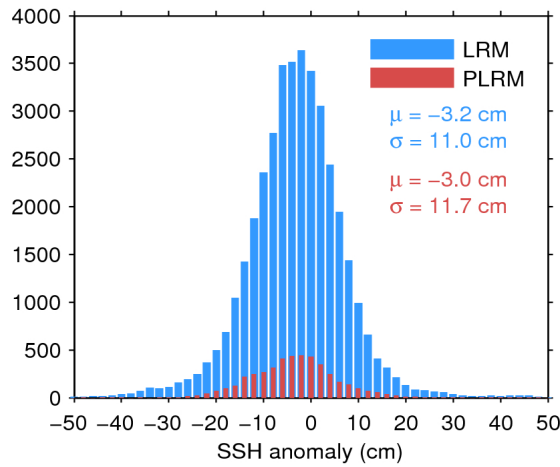
Figure 11. Histogram of science-valid SSH anomaly over oceans and lakes for LRM (blue) and PLRM (red) for 08/04/2017. The mean ( \mu ) and standard deviation ( \sigma ) are also shown. Note that values outside [-50 50] cm are excluded from the histogram for the sake of readability but not from the computation of \mu and \sigma .
