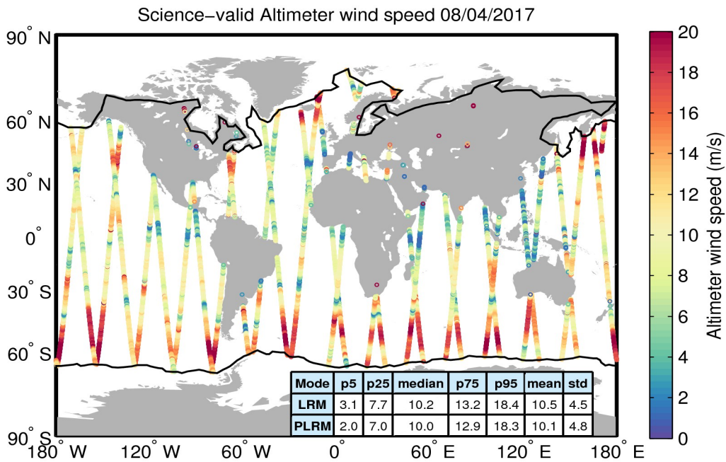
Figure 34. Geographical distribution of science-valid wind data over oceans and lakes for 08/04/2017. The statistical values shown in the table refer to the wind in m/s and are calculated separately for LRM and PLRM regions. The black lines mark the outer limit of the Arctic and Antarctic polar polygons. Gray circles denote records that have been rejected based on the editing criteria described in Table 5.
