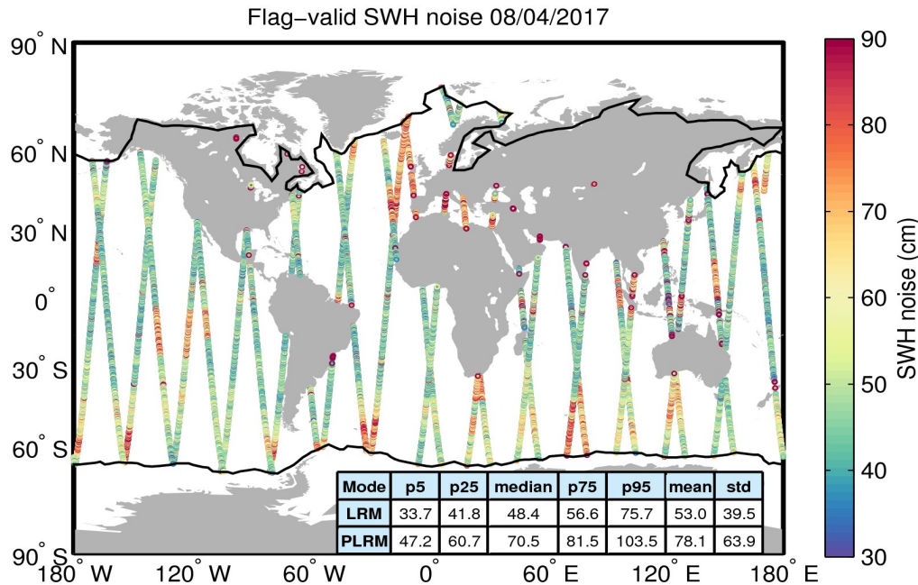
Figure 18. Geographical distribution of flag-valid 20-Hz SWH measurement noise over oceans and lakes for 08/04/2017. The statistical values shown in the table refer to the SWH noise and are calculated separately for LRM and PLRM regions. Measurements taken over polar polygons have been excluded from the computation of the statistical values. The black lines mark the outer limit of the Arctic and Antarctic polar polygons.
