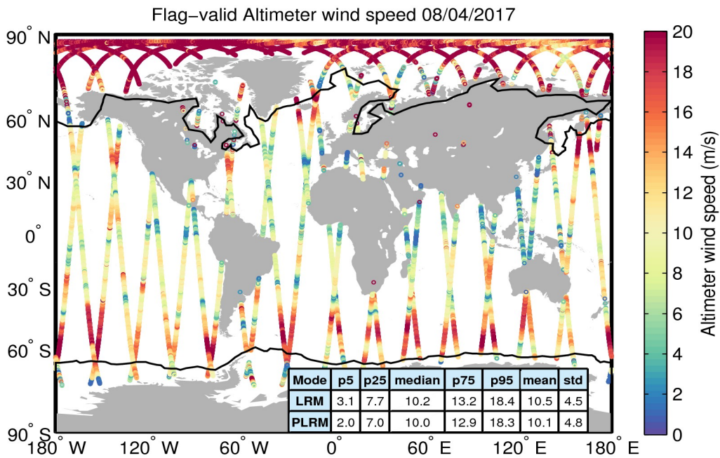
Figure 31. Geographical distribution of flag-valid wind data over oceans and lakes for 08/04/2017. The statistical values shown in the table refer to the wind in m/s and are calculated separately for LRM and PLRM regions. Measurements taken over polar polygons have been excluded from the computation of the statistical values. The black lines mark the outer limit of the Arctic and Antarctic polar polygons.
