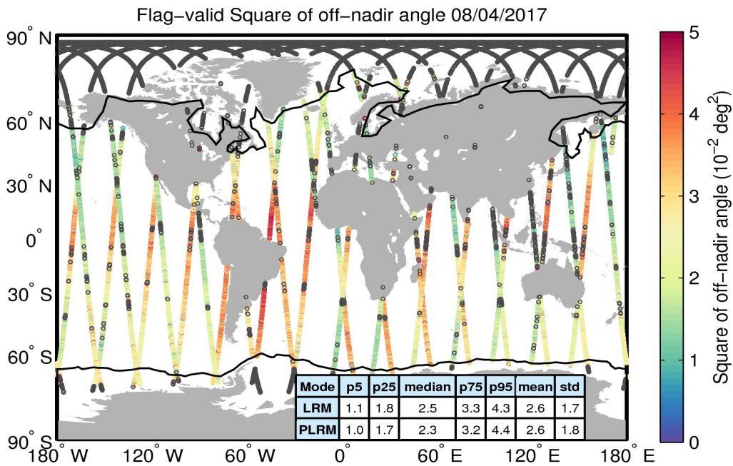
Figure 37. Geographical distribution of flag-valid mispointing data over oceans and lakes for 08/04/2017. The statistical values shown in the table refer to the mispointing in 10^{-2} deg 2 and are calculated separately for LRM and PLRM regions. Measurements taken over polar polygons have been excluded from the computation of the statistical values. The black lines mark the outer limit of the Arctic and Antarctic polar polygons. Gray circles denote negative values.
