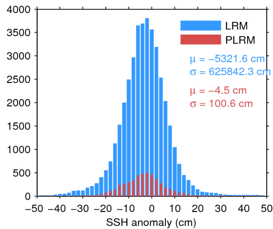
Figure 7. Histogram of flag-valid SSH anomaly over oceans and lakes for LRM (blue) and PLRM (red) for 08/04/2017. The mean ( \mu ) and standard deviation ( \sigma ) are also shown. Note that values outside [-50 \ 50] cm are excluded from the histogram for the sake of readability but not from the computation of \mu and \sigma .
