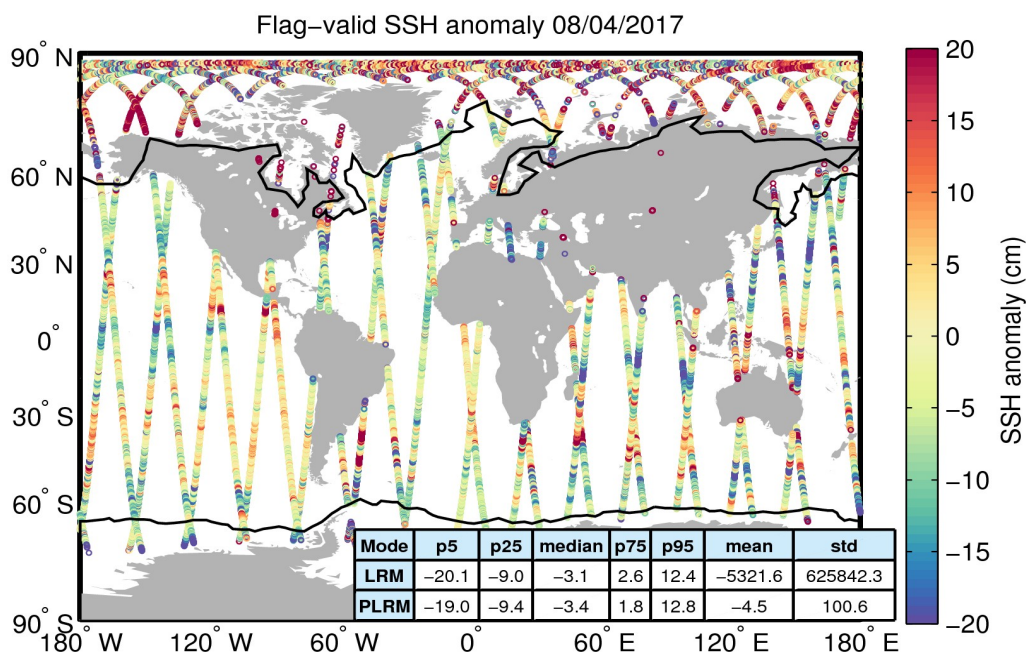
Figure 5. Geographical distribution of flag-valid 1-Hz SSH anomaly data over oceans and lakes for 08/04/2017. The statistical values shown in the table refer to the SSH anomaly in cm and are calculated separately for LRM and PLRM regions. Measurements taken over polar polygons have been excluded from the computation of the statistical values. The black lines mark the outer limit of the Arctic and Antarctic polar polygons.
