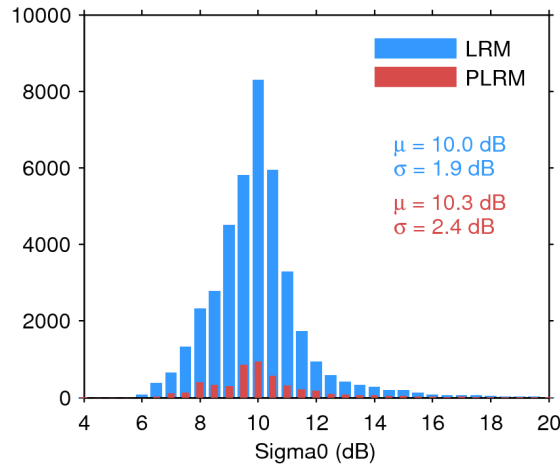
Figure 25. Histogram of flag-valid sigma0 over oceans and lakes for LRM (blue) and PLRM (red) for 08/04/2017. The mean ( \mu ) and standard deviation ( \sigma ) are also shown. Note that values outside [4 20] dB are excluded from the histogram for the sake of readability but not from the computation of \mu and \sigma .
