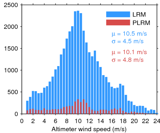
Figure 33. Histogram of flag-valid wind over oceans and lakes for LRM (blue) and PLRM (red) for 08/04/2017. The mean ( \mu ) and standard deviation ( \sigma ) are also shown. Note that values larger than 24 m/s are excluded from the histogram for the sake of readability but not from the computation of \mu and \sigma .
