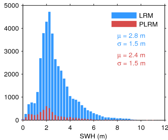
Figure 17. Histogram of flag-valid SWH over oceans and lakes for LRM (blue) and PLRM (red) for 08/04/2017. The mean ( \mu ) and standard deviation ( \sigma ) are also shown. Note that values larger than 12 m are excluded from the histogram for the sake of readability but not from the computation of \mu and \sigma .
