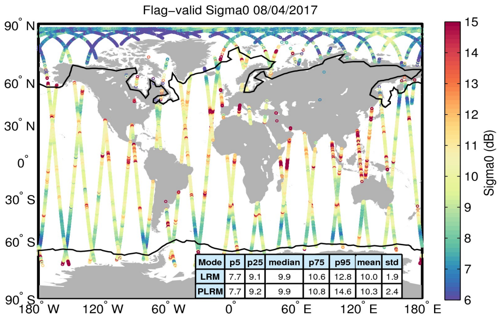
Figure 23. Geographical distribution of flag-valid sigma0 data over oceans and lakes for 08/04/2017. The statistical values shown in the table refer to the sigma0 in dB and are calculated separately for LRM and PLRM regions. Measurements taken over polar polygons have been excluded from the computation of the statistical values. The black lines mark the outer limit of the Arctic and Antarctic polar polygons.
