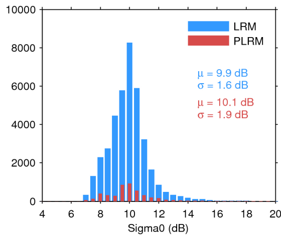
Figure 28. Histogram of science-valid sigma0 over oceans and lakes for LRM (blue) and PLRM (red) for 08/04/2017. The mean ( \mu ) and standard deviation ( \sigma ) are also shown. Note that values outside [4 20] dB are excluded from the histogram for the sake of readability but not from the computation of \mu and \sigma .
