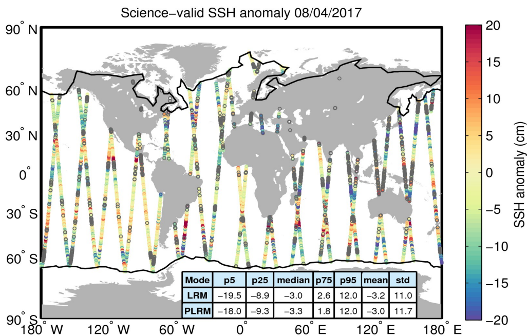
Figure 10. Geographical distribution of science-valid SSH anomaly data over oceans and lakes for 08/04/2017. The statistical values shown in the table refer to the SSH anomaly in cm and are calculated separately for LRM and PLRM regions. The black lines mark the outer limit of the Arctic and Antarctic polar polygons. Gray circles denote records that have been rejected based on the editing criteria described in Table 2.
