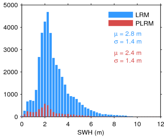
Figure 20. Histogram of science-valid SWH over oceans and lakes for LRM (blue) and PLRM (red) for 08/04/2017. The mean ( \mu ) and standard deviation ( \sigma ) are also shown. Note that values larger than 12 m are excluded from the histogram for the sake of readability but not from the computation of \mu and \sigma .
