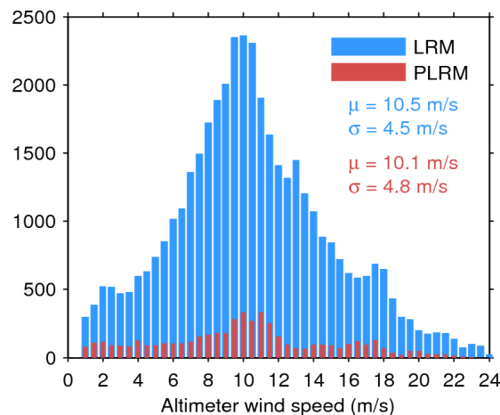
Figure 35. Histogram of science-valid wind over oceans and lakes for LRM (blue) and PLRM (red) for 08/04/2017. The mean ( \mu ) and standard deviation ( \sigma ) are also shown. Note that values larger than 24 m/s are excluded from the histogram for the sake of readability but not from the computation of \mu and \sigma .
