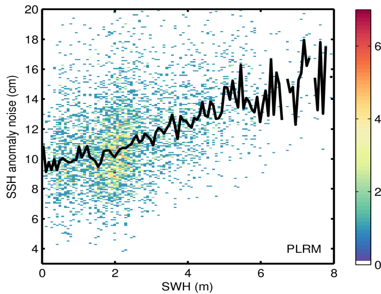
Figure 9. 2D histogram showing flag-valid SSH anomaly noise as a function of SWH for LRM (top) and PLRM (bottom) for 08/04/2017. The black line denotes the median SSH anomaly noise as a function of SWH.
