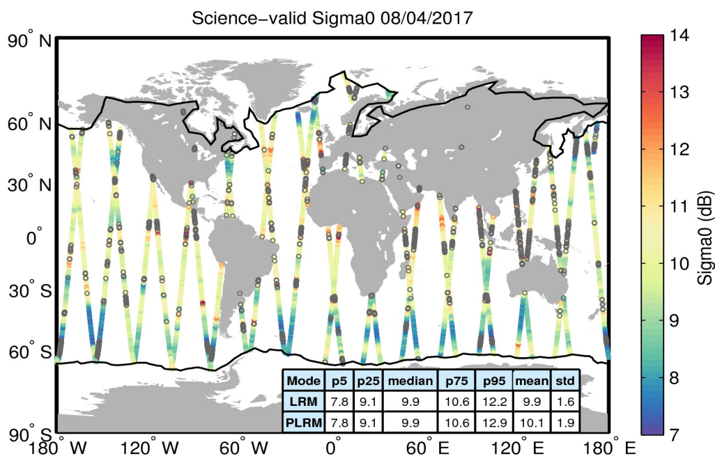
Figure 27. Geographical distribution of science-valid sigma0 data over oceans and lakes for 08/04/2017. The statistical values shown in the table refer to the sigma0 in dB and are calculated separately for LRM and PLRM regions. The black lines mark the outer limit of the Arctic and Antarctic polar polygons. Gray circles denote records that have been rejected based on the editing criteria described in Table 4.
