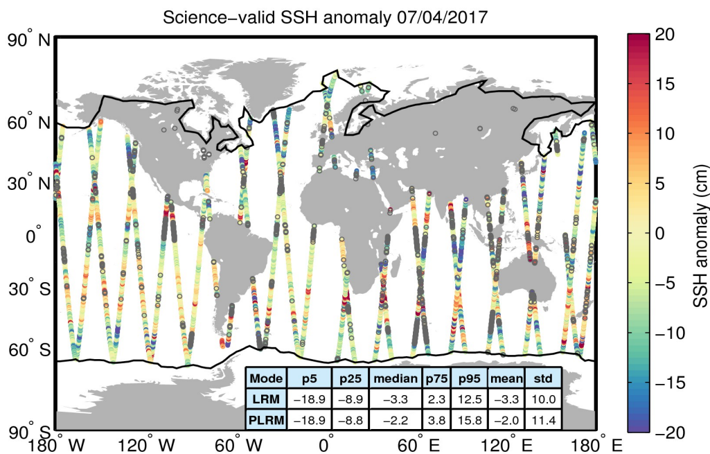
Figure 10. Geographical distribution of science-valid SSH anomaly data over oceans and lakes for 07/04/2017. The statistical values shown in the table refer to the SSH anomaly in cm and are calculated separately for LRM and PLRM regions. The black lines mark the outer limit of the Arctic and Antarctic polar polygons. Gray circles denote records that have been rejected based on the editing criteria described in Table 2.
