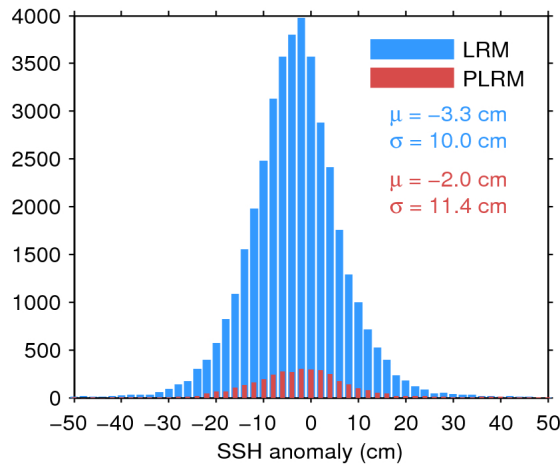
Figure 11. Histogram of science-valid SSH anomaly over oceans and lakes for LRM (blue) and PLRM (red) for 07/04/2017. The mean ( \mu ) and standard deviation ( \sigma ) are also shown. Note that values outside [-50 50] cm are excluded from the histogram for the sake of readability but not from the computation of \mu and \sigma .
