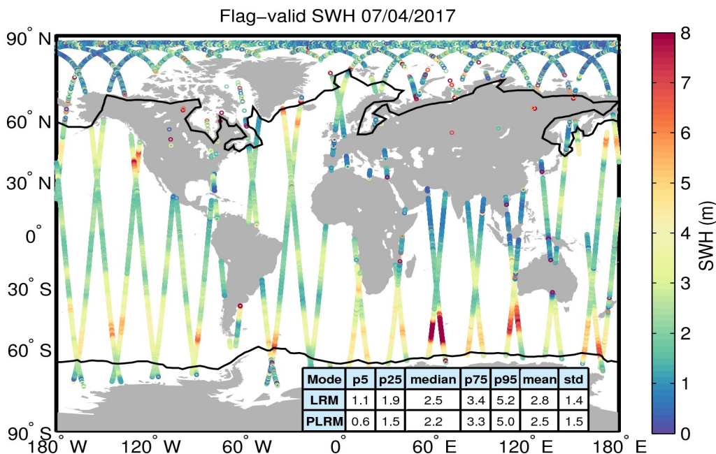
Figure 15. Geographical distribution of flag-valid SWH data over oceans and lakes for 07/04/2017. The statistical values shown in the table refer to the SWH in m and are calculated separately for LRM and PLRM regions. Measurements taken over polar polygons have been excluded from the computation of the statistical values. The black lines mark the outer limit of the Arctic and Antarctic polar polygons.
