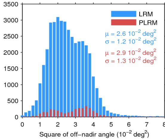
Figure 39. Histogram of flag-valid mispointing over oceans and lakes for LRM (blue) and PLRM (red) for 07/04/2017. Only positive values have been considered. The mean ( \mu ) and standard deviation ( \sigma ) are also shown. Note that values larger than 8 \cdot 10^{-2} \text{ deg}^2 are excluded from the histogram for the sake of readability but not from the computation of \mu and \sigma .
