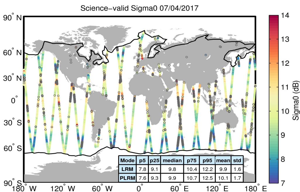
Figure 27. Geographical distribution of science-valid sigma0 data over oceans and lakes for 07/04/2017. The statistical values shown in the table refer to the sigma0 in dB and are calculated separately for LRM and PLRM regions. The black lines mark the outer limit of the Arctic and Antarctic polar polygons. Gray circles denote records that have been rejected based on the editing criteria described in Table 4.
