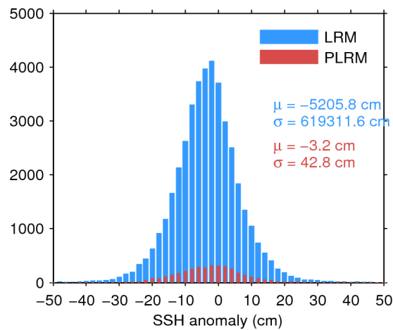
Figure 7. Histogram of flag-valid SSH anomaly over oceans and lakes for LRM (blue) and PLRM (red) for 07/04/2017. The mean ( \mu ) and standard deviation ( \sigma ) are also shown. Note that values outside [-50\ 50] cm are excluded from the histogram for the sake of readability but not from the computation of \mu and \sigma .
