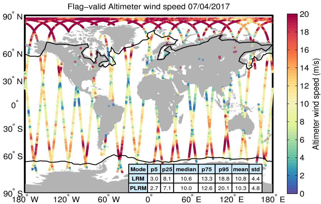
Figure 31. Geographical distribution of flag-valid wind data over oceans and lakes for 07/04/2017. The statistical values shown in the table refer to the wind in m/s and are calculated separately for LRM and PLRM regions. Measurements taken over polar polygons have been excluded from the computation of the statistical values. The black lines mark the outer limit of the Arctic and Antarctic polar polygons.
