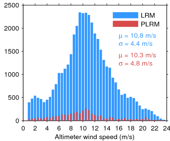
Figure 33. Histogram of flag-valid wind over oceans and lakes for LRM (blue) and PLRM (red) for 07/04/2017. The mean ( \mu ) and standard deviation ( \sigma ) are also shown. Note that values larger than 24 m/s are excluded from the histogram for the sake of readability but not from the computation of \mu and \sigma .
