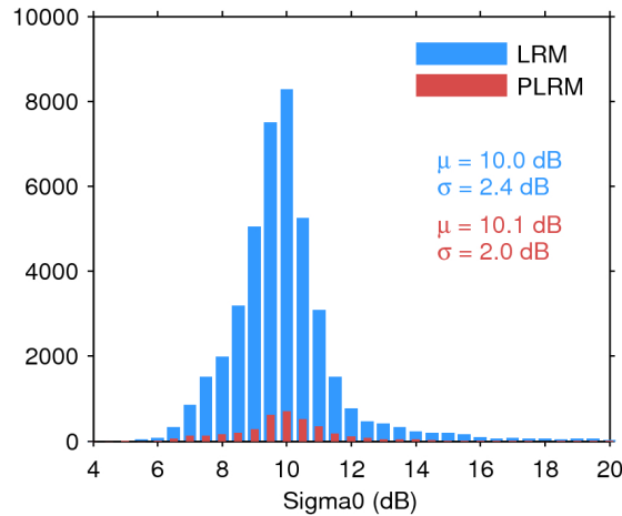
Figure 25. Histogram of flag-valid sigma0 over oceans and lakes for LRM (blue) and PLRM (red) for 07/04/2017. The mean ( \mu ) and standard deviation ( \sigma ) are also shown. Note that values outside [4 20] dB are excluded from the histogram for the sake of readability but not from the computation of \mu and \sigma .
