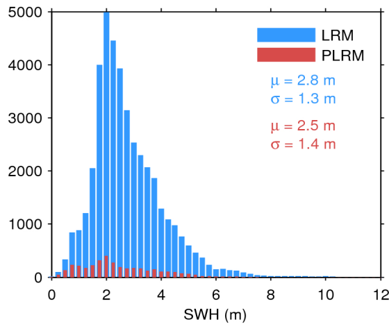
Figure 20. Histogram of science-valid SWH over oceans and lakes for LRM (blue) and PLRM (red) for 07/04/2017. The mean ( \mu ) and standard deviation ( \sigma ) are also shown. Note that values larger than 12 m are excluded from the histogram for the sake of readability but not from the computation of \mu and \sigma .
