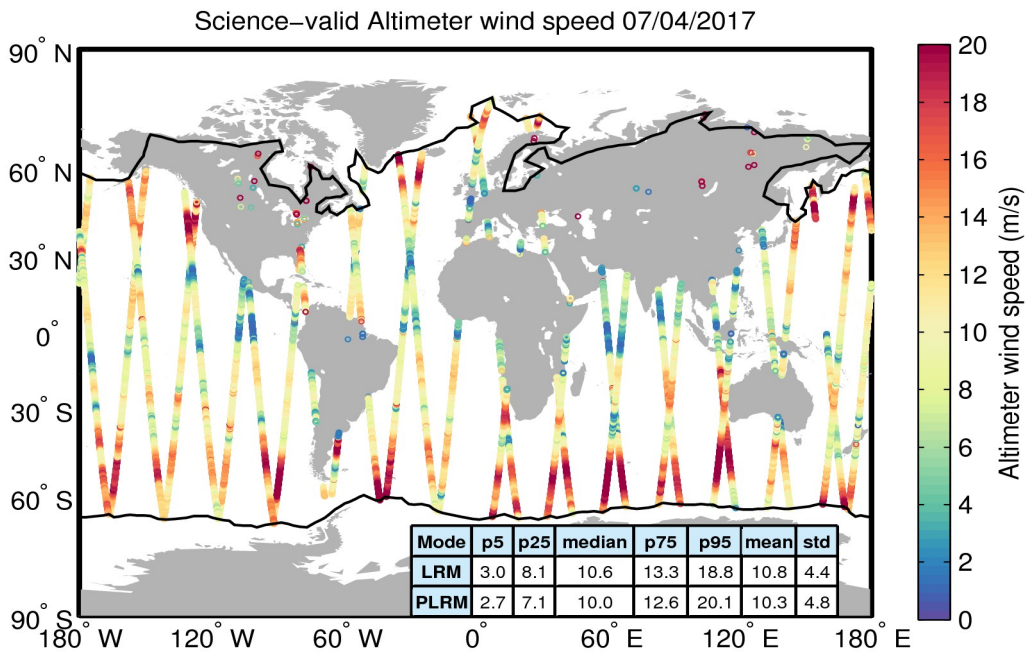
Figure 34. Geographical distribution of science-valid wind data over oceans and lakes for 07/04/2017. The statistical values shown in the table refer to the wind in m/s and are calculated separately for LRM and PLRM regions. The black lines mark the outer limit of the Arctic and Antarctic polar polygons. Gray circles denote records that have been rejected based on the editing criteria described in Table 5.
