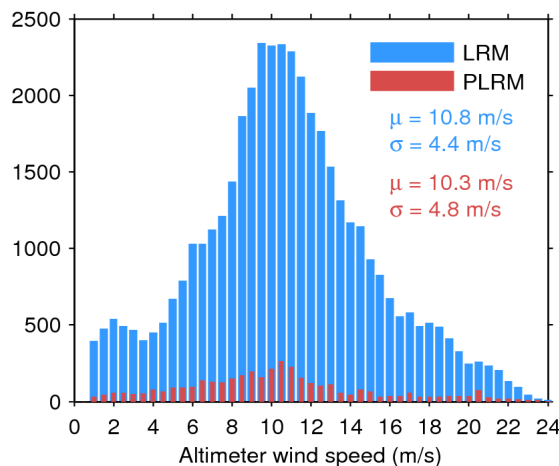
Figure 35. Histogram of science-valid wind over oceans and lakes for LRM (blue) and PLRM (red) for 07/04/2017. The mean ( \mu ) and standard deviation ( \sigma ) are also shown. Note that values larger than 24 m/s are excluded from the histogram for the sake of readability but not from the computation of \mu and \sigma .
