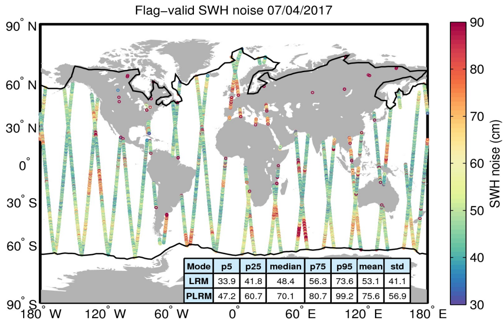
Figure 18. Geographical distribution of flag-valid 20-Hz SWH measurement noise over oceans and lakes for 07/04/2017. The statistical values shown in the table refer to the SWH noise and are calculated separately for LRM and PLRM regions. Measurements taken over polar polygons have been excluded from the computation of the statistical values. The black lines mark the outer limit of the Arctic and Antarctic polar polygons.
