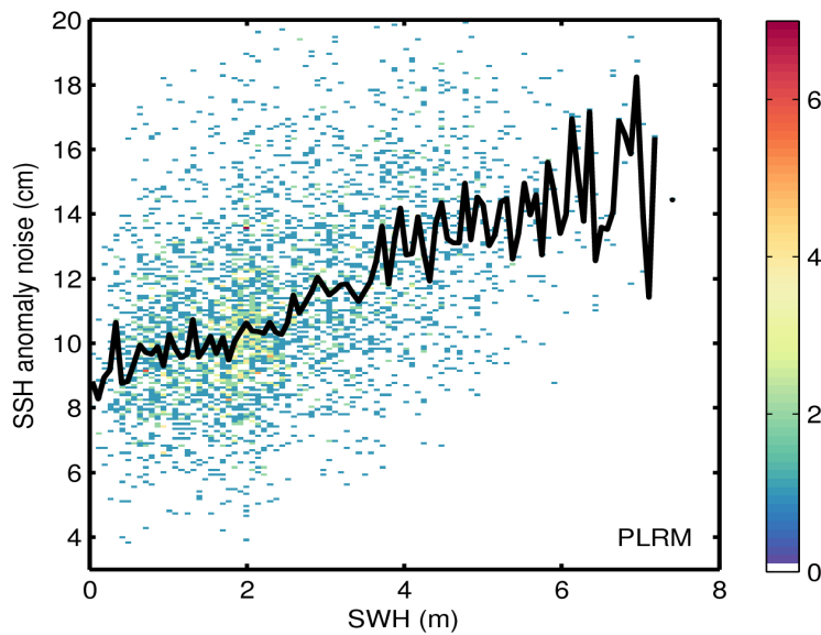
Figure 9. 2D histogram showing flag-valid SSH anomaly noise as a function of SWH for LRM (top) and PLRM (bottom) for 07/04/2017. The black line denotes the median SSH anomaly noise as a function of SWH.
