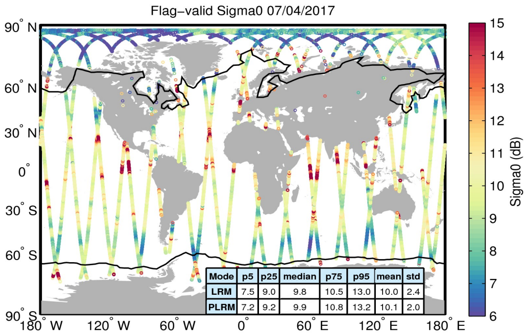
Figure 23. Geographical distribution of flag-valid sigma0 data over oceans and lakes for 07/04/2017. The statistical values shown in the table refer to the sigma0 in dB and are calculated separately for LRM and PLRM regions. Measurements taken over polar polygons have been excluded from the computation of the statistical values. The black lines mark the outer limit of the Arctic and Antarctic polar polygons.
