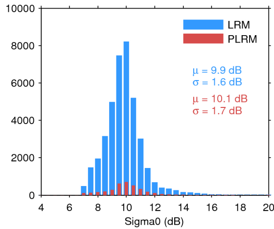
Figure 28. Histogram of science-valid sigma0 over oceans and lakes for LRM (blue) and PLRM (red) for 07/04/2017. The mean ( \mu ) and standard deviation ( \sigma ) are also shown. Note that values outside [4 20] dB are excluded from the histogram for the sake of readability but not from the computation of \mu and \sigma .
