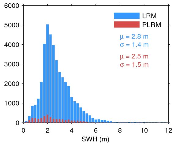
Figure 17. Histogram of flag-valid SWH over oceans and lakes for LRM (blue) and PLRM (red) for 07/04/2017. The mean ( \mu ) and standard deviation ( \sigma ) are also shown. Note that values larger than 12 m are excluded from the histogram for the sake of readability but not from the computation of \mu and \sigma .
