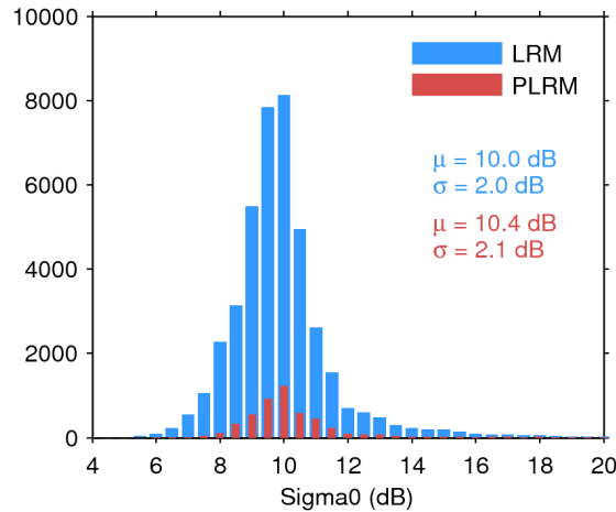
Figure 25. Histogram of flag-valid sigma0 over oceans and lakes for LRM (blue) and PLRM (red) for 06/04/2017. The mean ( \mu ) and standard deviation ( \sigma ) are also shown. Note that values outside [4 20] dB are excluded from the histogram for the sake of readability but not from the computation of \mu and \sigma .
