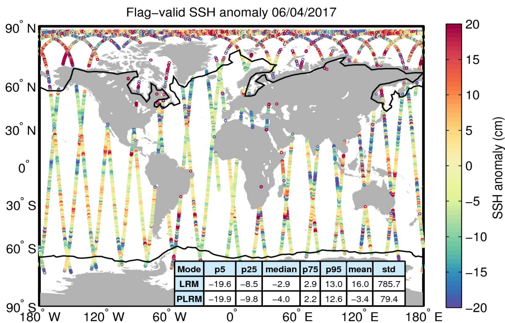
Figure 5. Geographical distribution of flag-valid 1-Hz SSH anomaly data over oceans and lakes for 06/04/2017. The statistical values shown in the table refer to the SSH anomaly in cm and are calculated separately for LRM and PLRM regions. Measurements taken over polar polygons have been excluded from the computation of the statistical values. The black lines mark the outer limit of the Arctic and Antarctic polar polygons.
