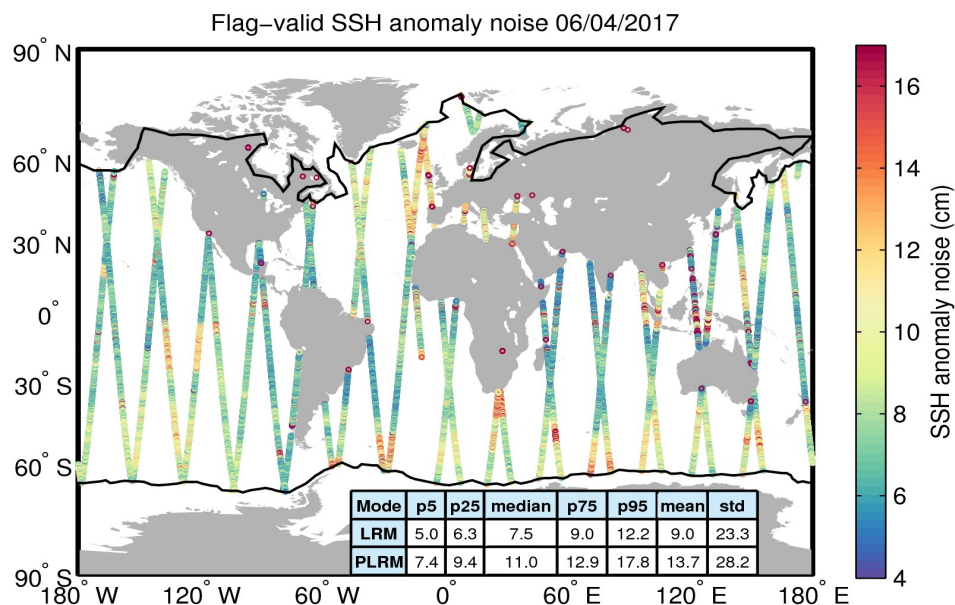
Figure 8. Geographical distribution of flag-valid 20-Hz SSH anomaly measurement noise over oceans and lakes for 06/04/2017. The statistical values shown in the table refer to the SSH anomaly noise and are calculated separately for LRM and PLRM regions. Measurements taken over polar polygons have been excluded from the computation of the statistical values. The black lines mark the outer limit of the Arctic and Antarctic polar polygons.
