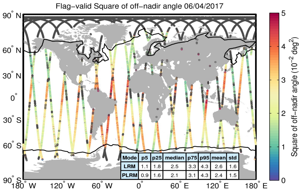
Figure 37. Geographical distribution of flag-valid mispointing data over oceans and lakes for 06/04/2017. The statistical values shown in the table refer to the mispointing in 10^{-2} deg 2 and are calculated separately for LRM and PLRM regions. Measurements taken over polar polygons have been excluded from the computation of the statistical values. The black lines mark the outer limit of the Arctic and Antarctic polar polygons. Gray circles denote negative values.
