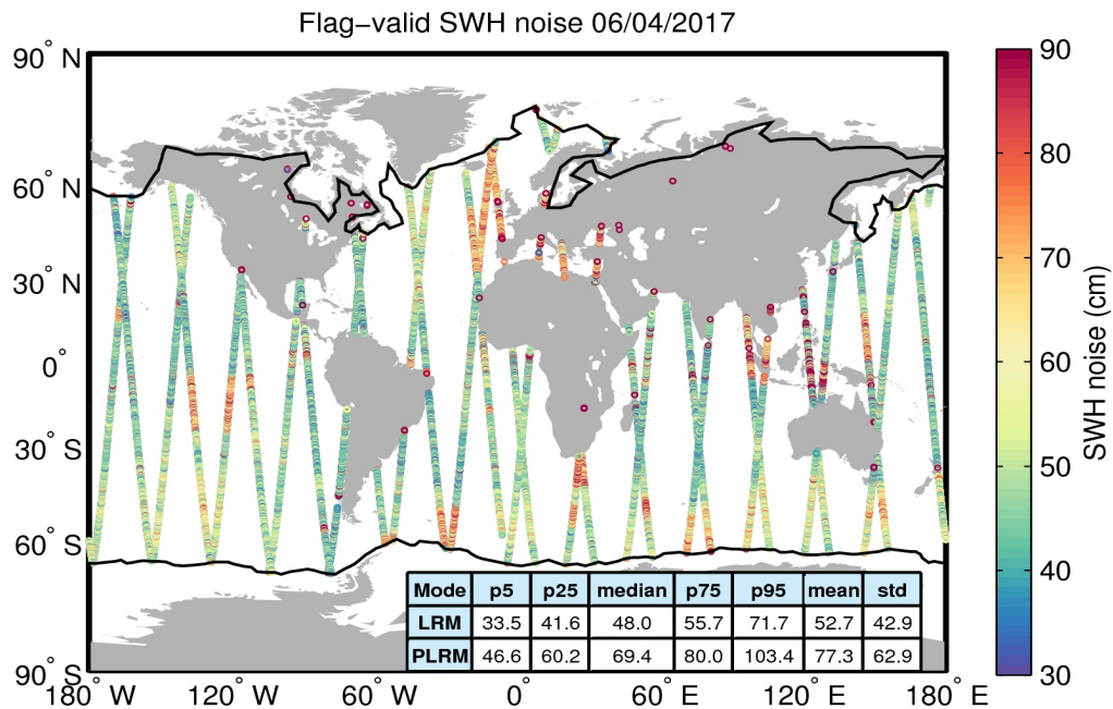
Figure 18. Geographical distribution of flag-valid 20-Hz SWH measurement noise over oceans and lakes for 06/04/2017. The statistical values shown in the table refer to the SWH noise and are calculated separately for LRM and PLRM regions. Measurements taken over polar polygons have been excluded from the computation of the statistical values. The black lines mark the outer limit of the Arctic and Antarctic polar polygons.
