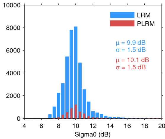
Figure 28. Histogram of science-valid sigma0 over oceans and lakes for LRM (blue) and PLRM (red) for 06/04/2017. The mean ( \mu ) and standard deviation ( \sigma ) are also shown. Note that values outside [4 20] dB are excluded from the histogram for the sake of readability but not from the computation of \mu and \sigma .
