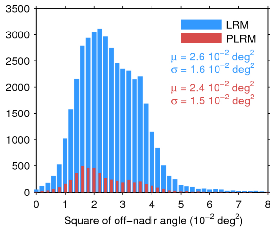
Figure 39. Histogram of flag-valid mispointing over oceans and lakes for LRM (blue) and PLRM (red) for 06/04/2017. Only positive values have been considered. The mean ( \mu ) and standard deviation ( \sigma ) are also shown. Note that values larger than 8 \cdot 10^{-2} \text{ deg}^2 are excluded from the histogram for the sake of readability but not from the computation of \mu and \sigma .
