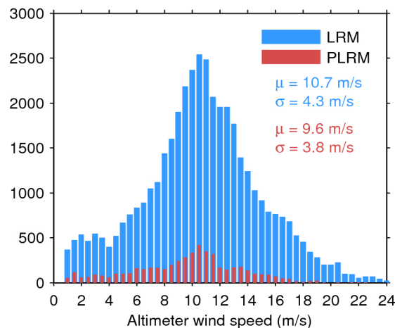
Figure 35. Histogram of science-valid wind over oceans and lakes for LRM (blue) and PLRM (red) for 06/04/2017. The mean ( \mu ) and standard deviation ( \sigma ) are also shown. Note that values larger than 24 m/s are excluded from the histogram for the sake of readability but not from the computation of \mu and \sigma .
