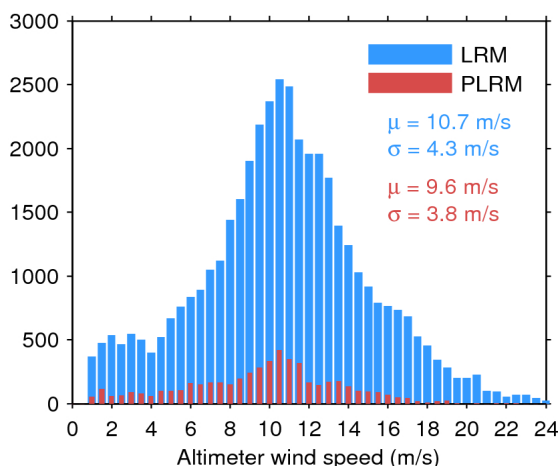
Figure 33. Histogram of flag-valid wind over oceans and lakes for LRM (blue) and PLRM (red) for 06/04/2017. The mean ( \mu ) and standard deviation ( \sigma ) are also shown. Note that values larger than 24 m/s are excluded from the histogram for the sake of readability but not from the computation of \mu and \sigma .
