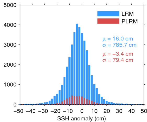
Figure 7. Histogram of flag-valid SSH anomaly over oceans and lakes for LRM (blue) and PLRM (red) for 06/04/2017. The mean ( \mu ) and standard deviation ( \sigma ) are also shown. Note that values outside [-50\ 50] cm are excluded from the histogram for the sake of readability but not from the computation of \mu and \sigma .
