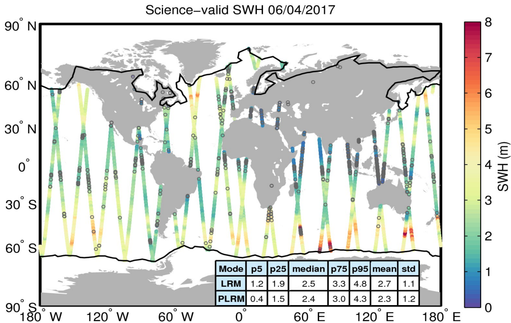
Figure 19. Geographical distribution of science-valid SWH data over oceans and lakes for 06/04/2017. The statistical values shown in the table refer to the SWH in m and are calculated separately for LRM and PLRM regions. The black lines mark the outer limit of the Arctic and Antarctic polar polygons. Gray circles denote records that have been rejected based on the editing criteria described in Table 3.
