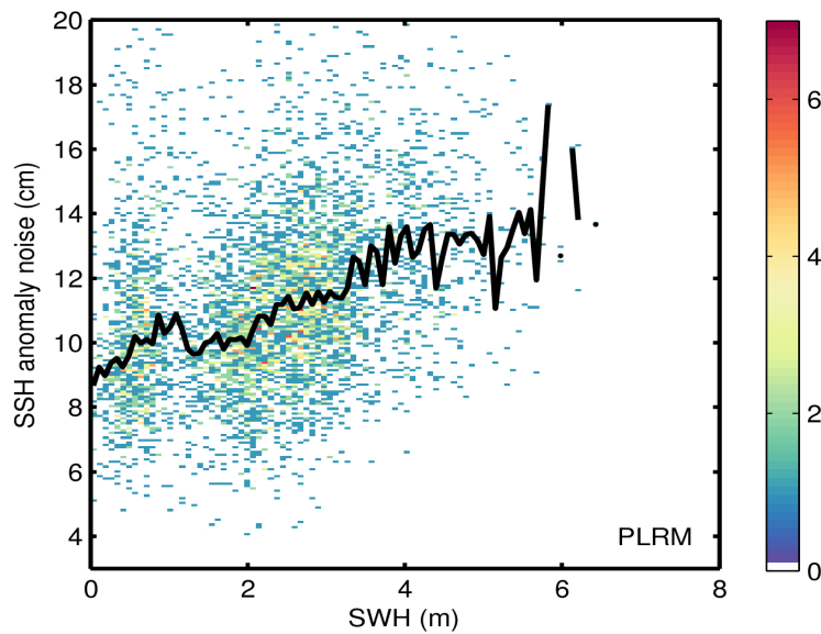
Figure 9. 2D histogram showing flag-valid SSH anomaly noise as a function of SWH for LRM (top) and PLRM (bottom) for 06/04/2017. The black line denotes the median SSH anomaly noise as a function of SWH.
