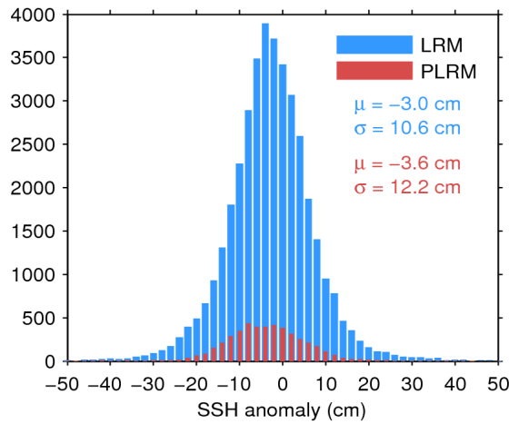
Figure 11. Histogram of science-valid SSH anomaly over oceans and lakes for LRM (blue) and PLRM (red) for 06/04/2017. The mean ( \mu ) and standard deviation ( \sigma ) are also shown. Note that values outside [-50\ 50] cm are excluded from the histogram for the sake of readability but not from the computation of \mu and \sigma .
