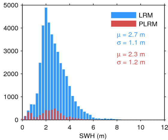
Figure 20. Histogram of science-valid SWH over oceans and lakes for LRM (blue) and PLRM (red) for 06/04/2017. The mean ( \mu ) and standard deviation ( \sigma ) are also shown. Note that values larger than 12 m are excluded from the histogram for the sake of readability but not from the computation of \mu and \sigma .
