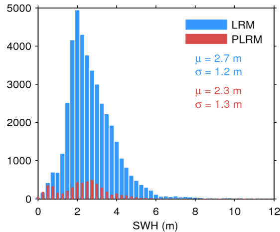
Figure 17. Histogram of flag-valid SWH over oceans and lakes for LRM (blue) and PLRM (red) for 06/04/2017. The mean ( \mu ) and standard deviation ( \sigma ) are also shown. Note that values larger than 12 m are excluded from the histogram for the sake of readability but not from the computation of \mu and \sigma .
