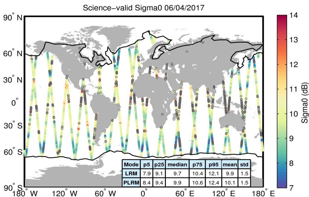
Figure 27. Geographical distribution of science-valid sigma0 data over oceans and lakes for 06/04/2017. The statistical values shown in the table refer to the sigma0 in dB and are calculated separately for LRM and PLRM regions. The black lines mark the outer limit of the Arctic and Antarctic polar polygons. Gray circles denote records that have been rejected based on the editing criteria described in Table 4.
