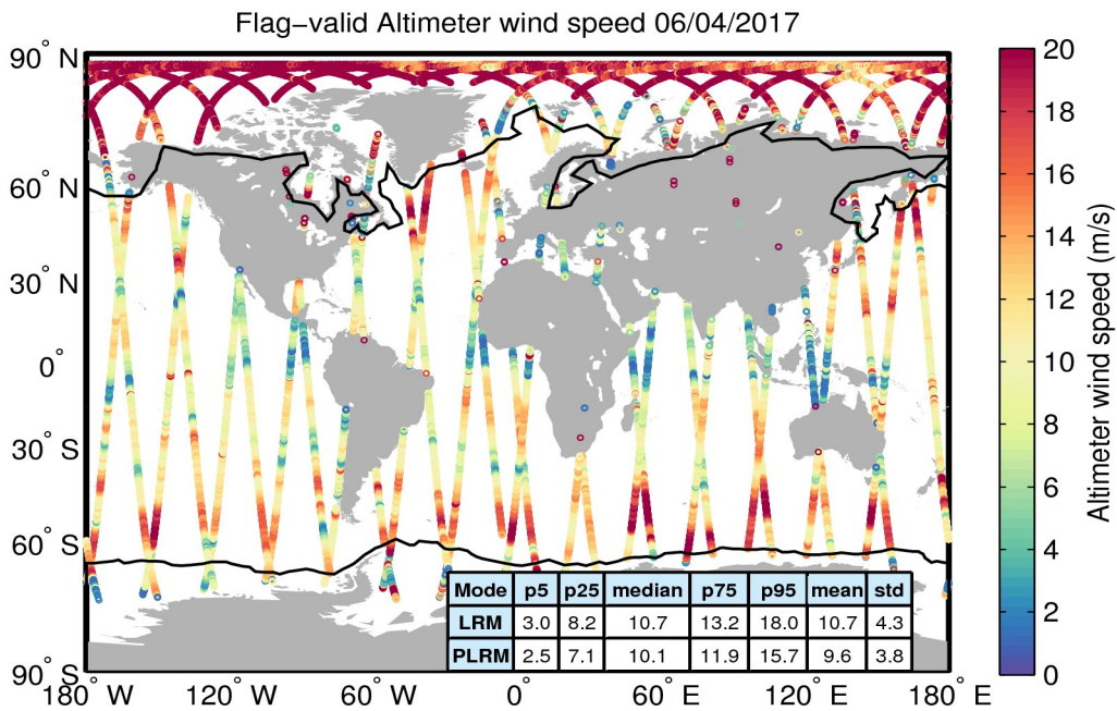
Figure 31. Geographical distribution of flag-valid wind data over oceans and lakes for 06/04/2017. The statistical values shown in the table refer to the wind in m/s and are calculated separately for LRM and PLRM regions. Measurements taken over polar polygons have been excluded from the computation of the statistical values. The black lines mark the outer limit of the Arctic and Antarctic polar polygons.
