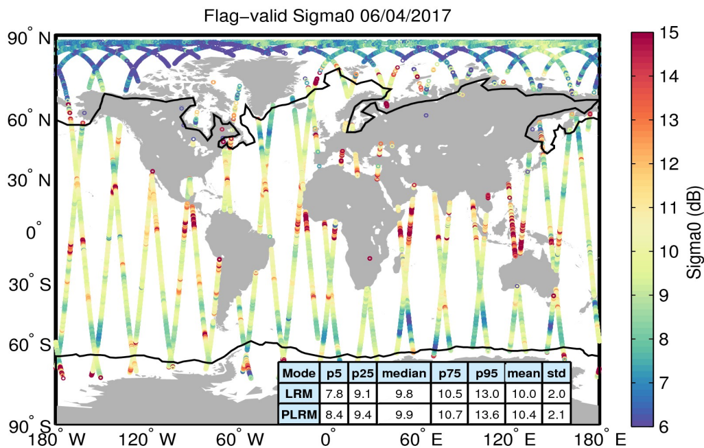
Figure 23. Geographical distribution of flag-valid sigma0 data over oceans and lakes for 06/04/2017. The statistical values shown in the table refer to the sigma0 in dB and are calculated separately for LRM and PLRM regions. Measurements taken over polar polygons have been excluded from the computation of the statistical values. The black lines mark the outer limit of the Arctic and Antarctic polar polygons.
