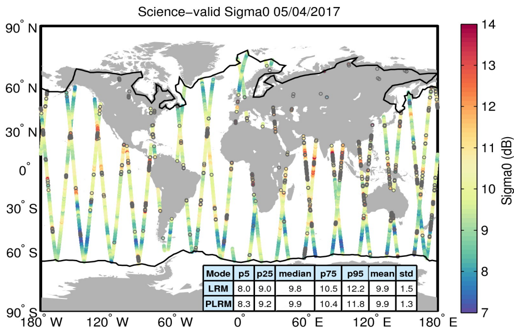
Figure 27. Geographical distribution of science-valid sigma0 data over oceans and lakes for 05/04/2017. The statistical values shown in the table refer to the sigma0 in dB and are calculated separately for LRM and PLRM regions. The black lines mark the outer limit of the Arctic and Antarctic polar polygons. Gray circles denote records that have been rejected based on the editing criteria described in Table 4.
