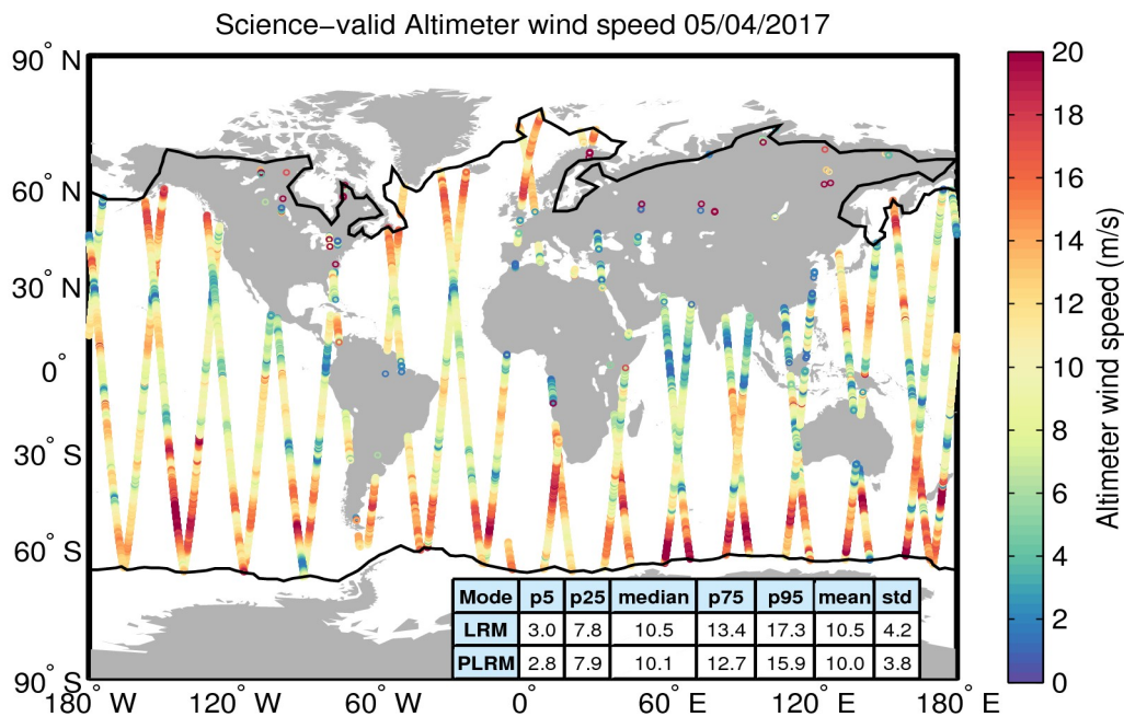
Figure 34. Geographical distribution of science-valid wind data over oceans and lakes for 05/04/2017. The statistical values shown in the table refer to the wind in m/s and are calculated separately for LRM and PLRM regions. The black lines mark the outer limit of the Arctic and Antarctic polar polygons. Gray circles denote records that have been rejected based on the editing criteria described in Table 5.
