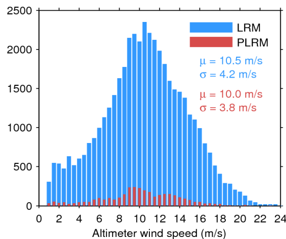
Figure 35. Histogram of science-valid wind over oceans and lakes for LRM (blue) and PLRM (red) for 05/04/2017. The mean ( \mu ) and standard deviation ( \sigma ) are also shown. Note that values larger than 24 m/s are excluded from the histogram for the sake of readability but not from the computation of \mu and \sigma .
