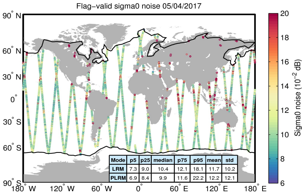
Figure 26. Geographical distribution of flag-valid 20-Hz sigma0 measurement noise over oceans and lakes for 05/04/2017. The statistical values shown in the table refer to the sigma0 noise and are calculated separately for LRM and PLRM regions. Measurements taken over polar polygons have been excluded from the computation of the statistical values. The black lines mark the outer limit of the Arctic and Antarctic polar polygons.
