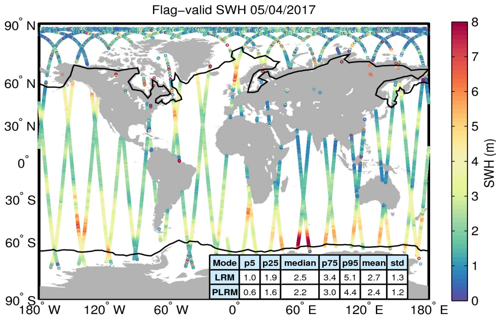
Figure 15. Geographical distribution of flag-valid SWH data over oceans and lakes for 05/04/2017. The statistical values shown in the table refer to the SWH in m and are calculated separately for LRM and PLRM regions. Measurements taken over polar polygons have been excluded from the computation of the statistical values. The black lines mark the outer limit of the Arctic and Antarctic polar polygons.
