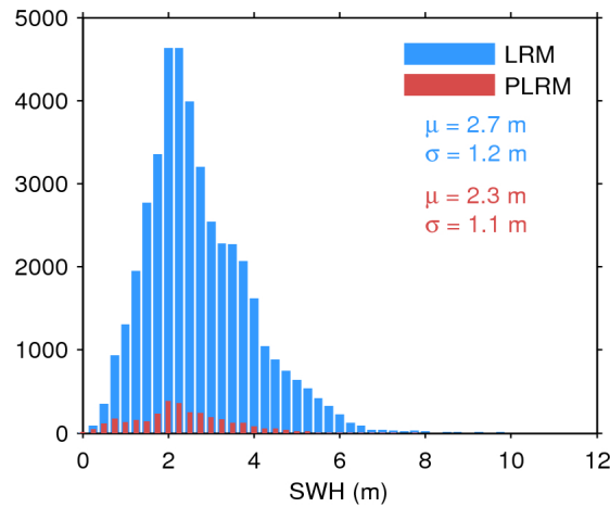
Figure 20. Histogram of science-valid SWH over oceans and lakes for LRM (blue) and PLRM (red) for 05/04/2017. The mean ( \mu ) and standard deviation ( \sigma ) are also shown. Note that values larger than 12 m are excluded from the histogram for the sake of readability but not from the computation of \mu and \sigma .
