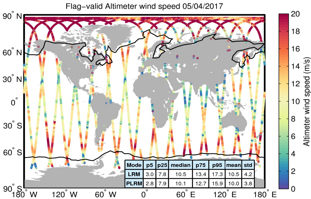
Figure 31. Geographical distribution of flag-valid wind data over oceans and lakes for 05/04/2017. The statistical values shown in the table refer to the wind in m/s and are calculated separately for LRM and PLRM regions. Measurements taken over polar polygons have been excluded from the computation of the statistical values. The black lines mark the outer limit of the Arctic and Antarctic polar polygons.
