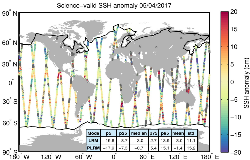
Figure 10. Geographical distribution of science-valid SSH anomaly data over oceans and lakes for 05/04/2017. The statistical values shown in the table refer to the SSH anomaly in cm and are calculated separately for LRM and PLRM regions. The black lines mark the outer limit of the Arctic and Antarctic polar polygons. Gray circles denote records that have been rejected based on the editing criteria described in Table 2.
