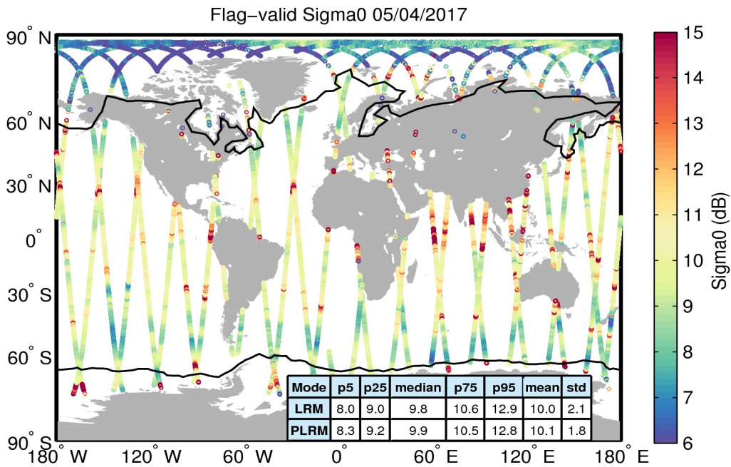
Figure 23. Geographical distribution of flag-valid sigma0 data over oceans and lakes for 05/04/2017. The statistical values shown in the table refer to the sigma0 in dB and are calculated separately for LRM and PLRM regions. Measurements taken over polar polygons have been excluded from the computation of the statistical values. The black lines mark the outer limit of the Arctic and Antarctic polar polygons.
