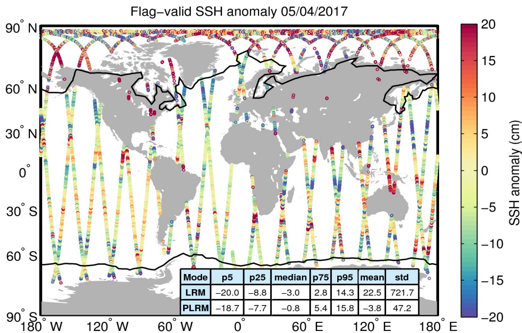
Figure 5. Geographical distribution of flag-valid 1-Hz SSH anomaly data over oceans and lakes for 05/04/2017. The statistical values shown in the table refer to the SSH anomaly in cm and are calculated separately for LRM and PLRM regions. Measurements taken over polar polygons have been excluded from the computation of the statistical values. The black lines mark the outer limit of the Arctic and Antarctic polar polygons.
