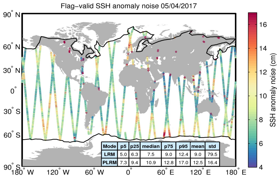
Figure 8. Geographical distribution of flag-valid 20-Hz SSH anomaly measurement noise over oceans and lakes for 05/04/2017. The statistical values shown in the table refer to the SSH anomaly noise and are calculated separately for LRM and PLRM regions. Measurements taken over polar polygons have been excluded from the computation of the statistical values. The black lines mark the outer limit of the Arctic and Antarctic polar polygons.
