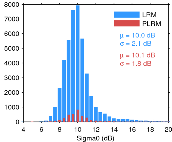
Figure 25. Histogram of flag-valid sigma0 over oceans and lakes for LRM (blue) and PLRM (red) for 05/04/2017. The mean ( \mu ) and standard deviation ( \sigma ) are also shown. Note that values outside [4 20] dB are excluded from the histogram for the sake of readability but not from the computation of \mu and \sigma .
