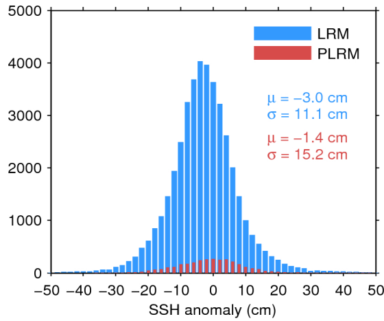
Figure 11. Histogram of science-valid SSH anomaly over oceans and lakes for LRM (blue) and PLRM (red) for 05/04/2017. The mean ( \mu ) and standard deviation ( \sigma ) are also shown. Note that values outside [-50\ 50] cm are excluded from the histogram for the sake of readability but not from the computation of \mu and \sigma .
