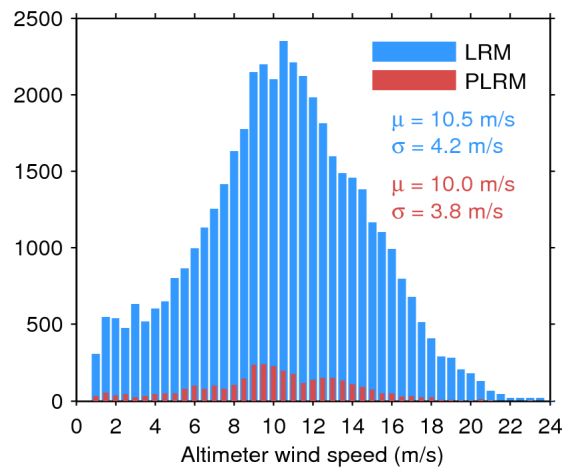
Figure 33. Histogram of flag-valid wind over oceans and lakes for LRM (blue) and PLRM (red) for 05/04/2017. The mean ( \mu ) and standard deviation ( \sigma ) are also shown. Note that values larger than 24 m/s are excluded from the histogram for the sake of readability but not from the computation of \mu and \sigma .
