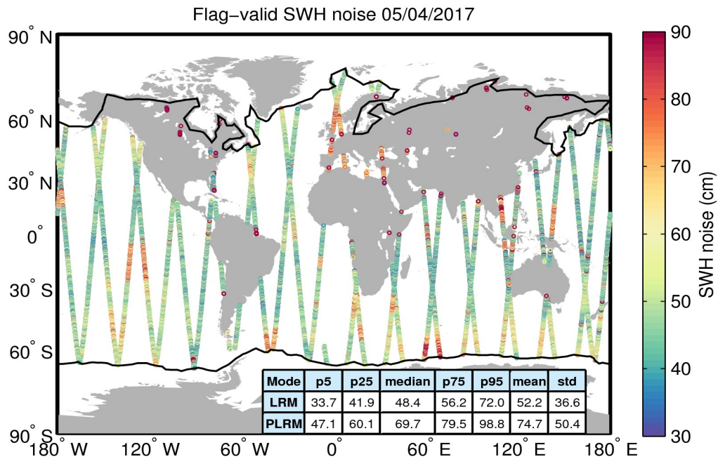
Figure 18. Geographical distribution of flag-valid 20-Hz SWH measurement noise over oceans and lakes for 05/04/2017. The statistical values shown in the table refer to the SWH noise and are calculated separately for LRM and PLRM regions. Measurements taken over polar polygons have been excluded from the computation of the statistical values. The black lines mark the outer limit of the Arctic and Antarctic polar polygons.
