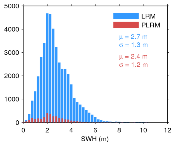
Figure 17. Histogram of flag-valid SWH over oceans and lakes for LRM (blue) and PLRM (red) for 05/04/2017. The mean ( \mu ) and standard deviation ( \sigma ) are also shown. Note that values larger than 12 m are excluded from the histogram for the sake of readability but not from the computation of \mu and \sigma .
