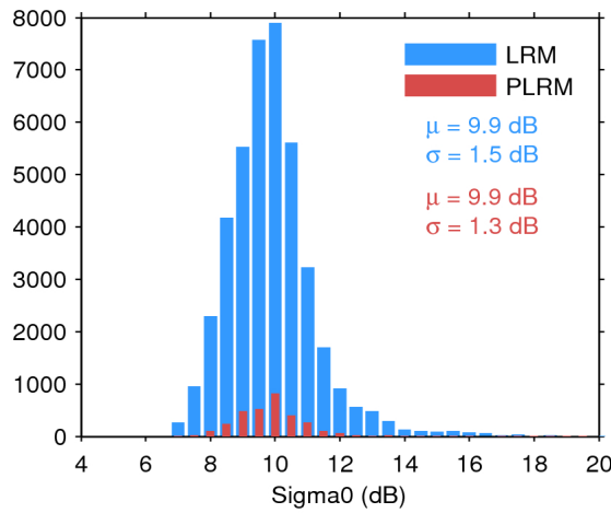
Figure 28. Histogram of science-valid sigma0 over oceans and lakes for LRM (blue) and PLRM (red) for 05/04/2017. The mean ( \mu ) and standard deviation ( \sigma ) are also shown. Note that values outside [4 20] dB are excluded from the histogram for the sake of readability but not from the computation of \mu and \sigma .
