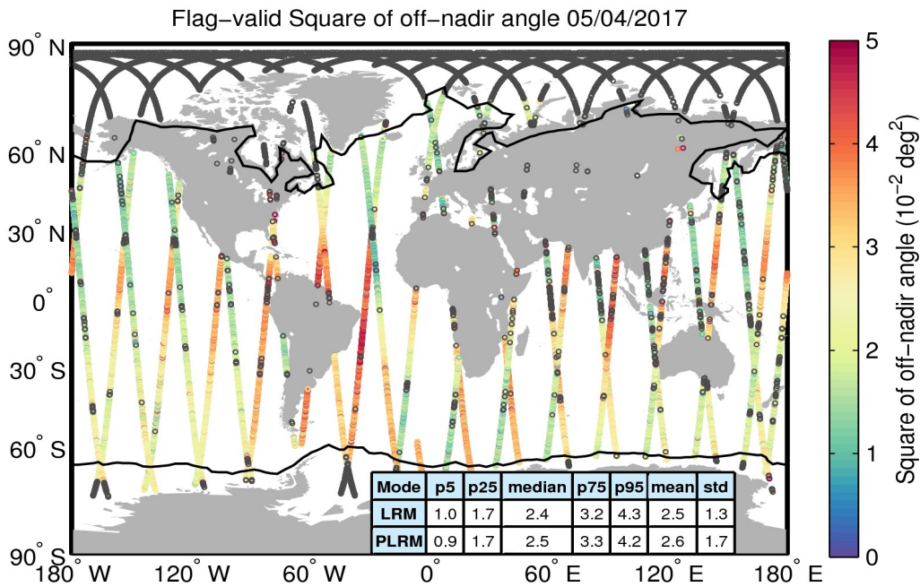
Figure 37. Geographical distribution of flag-valid mispointing data over oceans and lakes for 05/04/2017. The statistical values shown in the table refer to the mispointing in 10^{-2} deg 2 and are calculated separately for LRM and PLRM regions. Measurements taken over polar polygons have been excluded from the computation of the statistical values. The black lines mark the outer limit of the Arctic and Antarctic polar polygons. Gray circles denote negative values.
