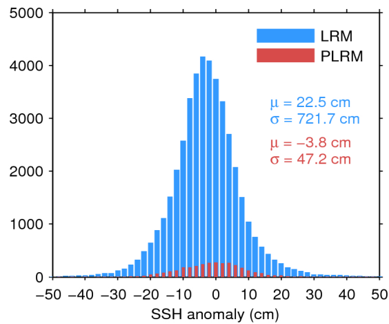
Figure 7. Histogram of flag-valid SSH anomaly over oceans and lakes for LRM (blue) and PLRM (red) for 05/04/2017. The mean ( \mu ) and standard deviation ( \sigma ) are also shown. Note that values outside [-50 50] cm are excluded from the histogram for the sake of readability but not from the computation of \mu and \sigma .
