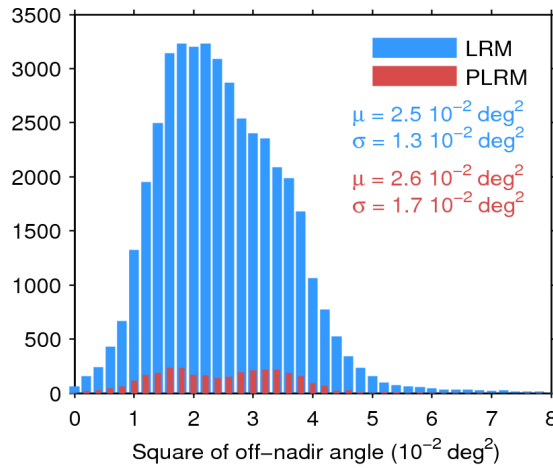
Figure 39. Histogram of flag-valid mispointing over oceans and lakes for LRM (blue) and PLRM (red) for 05/04/2017. Only positive values have been considered. The mean ( \mu ) and standard deviation ( \sigma ) are also shown. Note that values larger than 8 \cdot 10^{-2} \text{ deg}^2 are excluded from the histogram for the sake of readability but not from the computation of \mu and \sigma .
