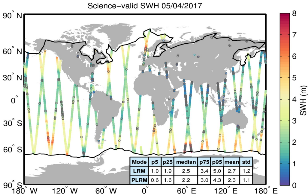
Figure 19. Geographical distribution of science-valid SWH data over oceans and lakes for 05/04/2017. The statistical values shown in the table refer to the SWH in m and are calculated separately for LRM and PLRM regions. The black lines mark the outer limit of the Arctic and Antarctic polar polygons. Gray circles denote records that have been rejected based on the editing criteria described in Table 3.
