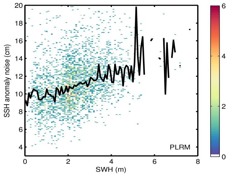
Figure 9. 2D histogram showing flag-valid SSH anomaly noise as a function of SWH for LRM (top) and PLRM (bottom) for 05/04/2017. The black line denotes the median SSH anomaly noise as a function of SWH.
