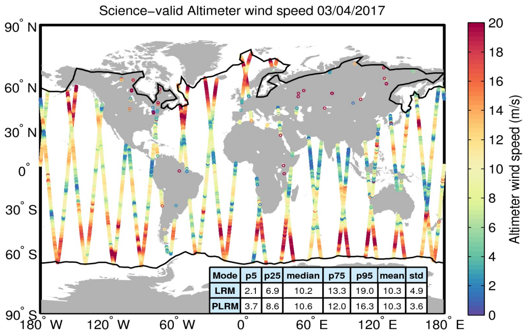
Figure 34. Geographical distribution of science-valid wind data over oceans and lakes for 03/04/2017. The statistical values shown in the table refer to the wind in m/s and are calculated separately for LRM and PLRM regions. The black lines mark the outer limit of the Arctic and Antarctic polar polygons. Gray circles denote records that have been rejected based on the editing criteria described in Table 5.
