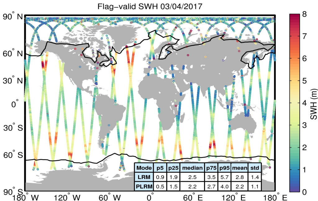
Figure 15. Geographical distribution of flag-valid SWH data over oceans and lakes for 03/04/2017. The statistical values shown in the table refer to the SWH in m and are calculated separately for LRM and PLRM regions. Measurements taken over polar polygons have been excluded from the computation of the statistical values. The black lines mark the outer limit of the Arctic and Antarctic polar polygons.
