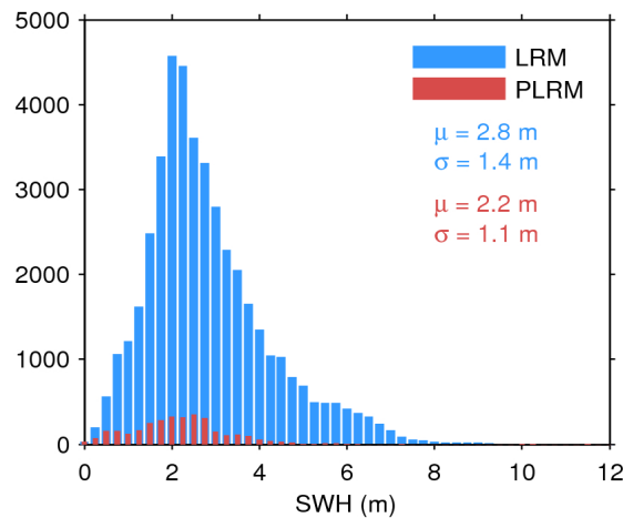
Figure 17. Histogram of flag-valid SWH over oceans and lakes for LRM (blue) and PLRM (red) for 03/04/2017. The mean ( \mu ) and standard deviation ( \sigma ) are also shown. Note that values larger than 12 m are excluded from the histogram for the sake of readability but not from the computation of \mu and \sigma .
