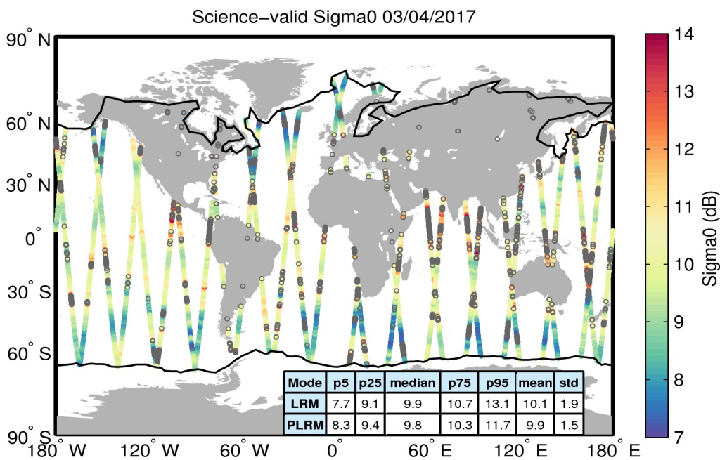
Figure 27. Geographical distribution of science-valid sigma0 data over oceans and lakes for 03/04/2017. The statistical values shown in the table refer to the sigma0 in dB and are calculated separately for LRM and PLRM regions. The black lines mark the outer limit of the Arctic and Antarctic polar polygons. Gray circles denote records that have been rejected based on the editing criteria described in Table 4.
