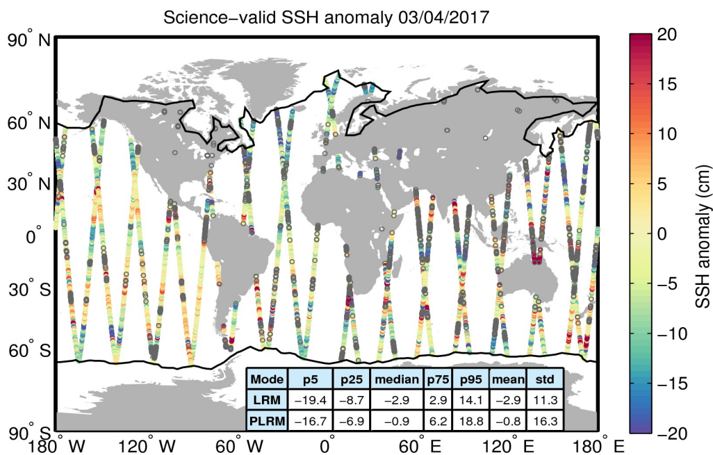
Figure 10. Geographical distribution of science-valid SSH anomaly data over oceans and lakes for 03/04/2017. The statistical values shown in the table refer to the SSH anomaly in cm and are calculated separately for LRM and PLRM regions. The black lines mark the outer limit of the Arctic and Antarctic polar polygons. Gray circles denote records that have been rejected based on the editing criteria described in Table 2.
