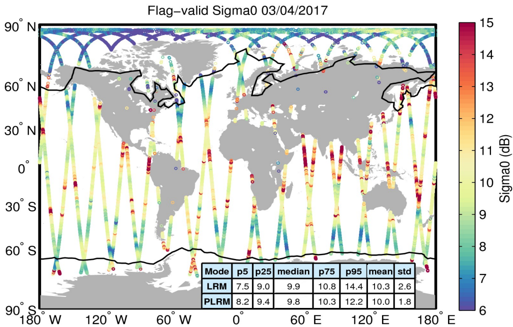
Figure 23. Geographical distribution of flag-valid sigma0 data over oceans and lakes for 03/04/2017. The statistical values shown in the table refer to the sigma0 in dB and are calculated separately for LRM and PLRM regions. Measurements taken over polar polygons have been excluded from the computation of the statistical values. The black lines mark the outer limit of the Arctic and Antarctic polar polygons.
