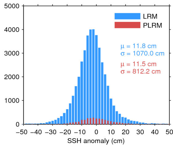
Figure 7. Histogram of flag-valid SSH anomaly over oceans and lakes for LRM (blue) and PLRM (red) for 03/04/2017. The mean ( \mu ) and standard deviation ( \sigma ) are also shown. Note that values outside [-50\ 50] cm are excluded from the histogram for the sake of readability but not from the computation of \mu and \sigma .
