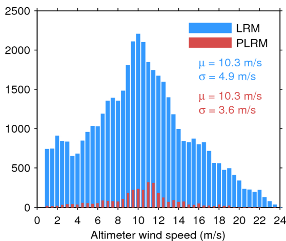
Figure 33. Histogram of flag-valid wind over oceans and lakes for LRM (blue) and PLRM (red) for 03/04/2017. The mean ( \mu ) and standard deviation ( \sigma ) are also shown. Note that values larger than 24 m/s are excluded from the histogram for the sake of readability but not from the computation of \mu and \sigma .
