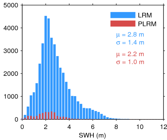
Figure 20. Histogram of science-valid SWH over oceans and lakes for LRM (blue) and PLRM (red) for 03/04/2017. The mean ( \mu ) and standard deviation ( \sigma ) are also shown. Note that values larger than 12 m are excluded from the histogram for the sake of readability but not from the computation of \mu and \sigma .
