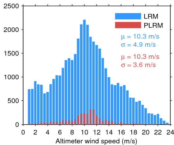
Figure 35. Histogram of science-valid wind over oceans and lakes for LRM (blue) and PLRM (red) for 03/04/2017. The mean ( \mu ) and standard deviation ( \sigma ) are also shown. Note that values larger than 24 m/s are excluded from the histogram for the sake of readability but not from the computation of \mu and \sigma .
