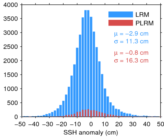
Figure 11. Histogram of science-valid SSH anomaly over oceans and lakes for LRM (blue) and PLRM (red) for 03/04/2017. The mean ( \mu ) and standard deviation ( \sigma ) are also shown. Note that values outside [-50\ 50] cm are excluded from the histogram for the sake of readability but not from the computation of \mu and \sigma .
