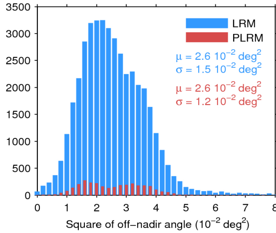
Figure 39. Histogram of flag-valid mispointing over oceans and lakes for LRM (blue) and PLRM (red) for 03/04/2017. Only positive values have been considered. The mean ( \mu ) and standard deviation ( \sigma ) are also shown. Note that values larger than 8 \cdot 10^{-2} \text{ deg}^2 are excluded from the histogram for the sake of readability but not from the computation of \mu and \sigma .
