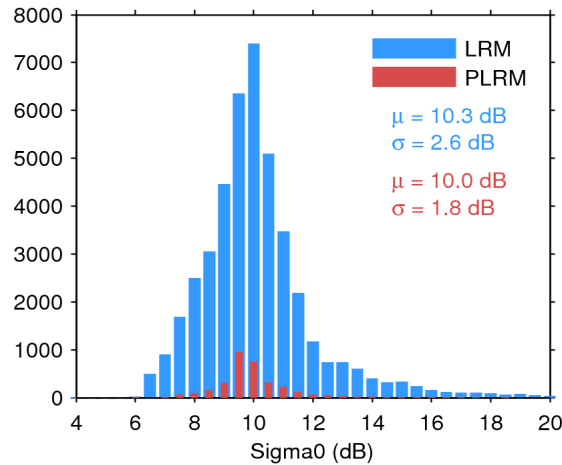
Figure 25. Histogram of flag-valid sigma0 over oceans and lakes for LRM (blue) and PLRM (red) for 03/04/2017. The mean ( \mu ) and standard deviation ( \sigma ) are also shown. Note that values outside [4 20] dB are excluded from the histogram for the sake of readability but not from the computation of \mu and \sigma .
