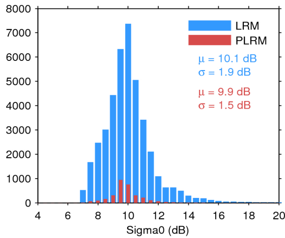
Figure 28. Histogram of science-valid sigma0 over oceans and lakes for LRM (blue) and PLRM (red) for 03/04/2017. The mean ( \mu ) and standard deviation ( \sigma ) are also shown. Note that values outside [4 20] dB are excluded from the histogram for the sake of readability but not from the computation of \mu and \sigma .
