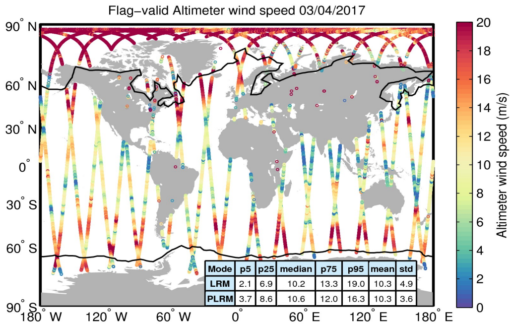
Figure 31. Geographical distribution of flag-valid wind data over oceans and lakes for 03/04/2017. The statistical values shown in the table refer to the wind in m/s and are calculated separately for LRM and PLRM regions. Measurements taken over polar polygons have been excluded from the computation of the statistical values. The black lines mark the outer limit of the Arctic and Antarctic polar polygons.
