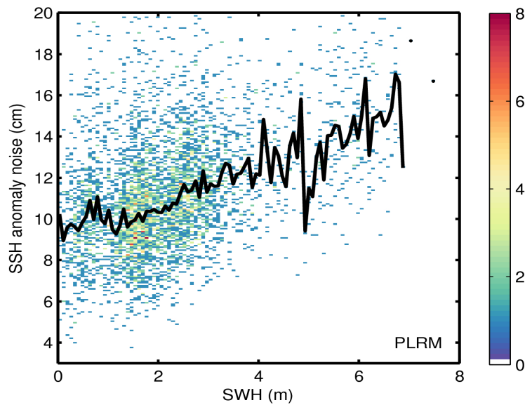
Figure 9. 2D histogram showing flag-valid SSH anomaly noise as a function of SWH for LRM (top) and PLRM (bottom) for 02/04/2017. The black line denotes the median SSH anomaly noise as a function of SWH.
