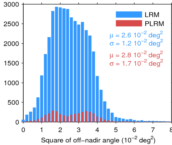
Figure 39. Histogram of flag-valid mispointing over oceans and lakes for LRM (blue) and PLRM (red) for 26/03/2017. Only positive values have been considered. The mean ( \mu ) and standard deviation ( \sigma ) are also shown. Note that values larger than 8 \cdot 10^{-2} \text{ deg}^2 are excluded from the histogram for the sake of readability but not from the computation of \mu and \sigma .
