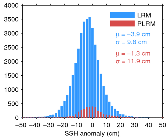
Figure 11. Histogram of science-valid SSH anomaly over oceans and lakes for LRM (blue) and PLRM (red) for 26/03/2017. The mean ( \mu ) and standard deviation ( \sigma ) are also shown. Note that values outside [-50 50] cm are excluded from the histogram for the sake of readability but not from the computation of \mu and \sigma .
