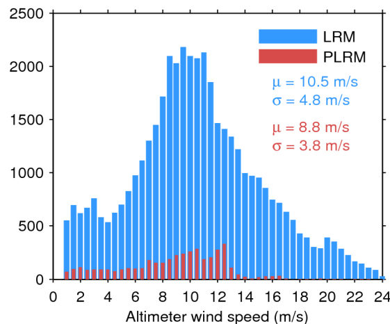
Figure 35. Histogram of science-valid wind over oceans and lakes for LRM (blue) and PLRM (red) for 26/03/2017. The mean ( \mu ) and standard deviation ( \sigma ) are also shown. Note that values larger than 24 m/s are excluded from the histogram for the sake of readability but not from the computation of \mu and \sigma .
