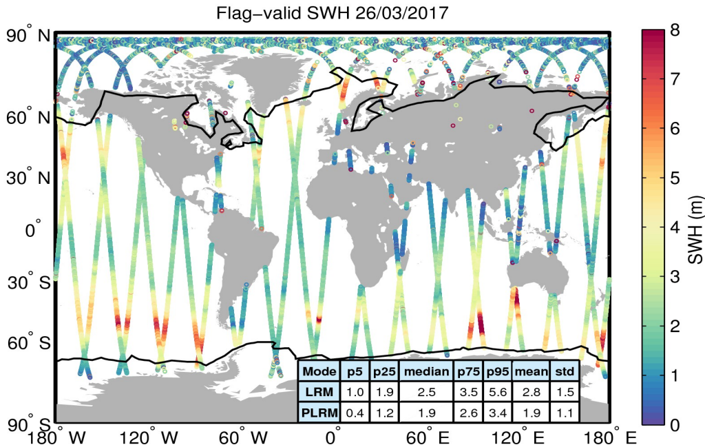
Figure 15. Geographical distribution of flag-valid SWH data over oceans and lakes for 26/03/2017. The statistical values shown in the table refer to the SWH in m and are calculated separately for LRM and PLRM regions. Measurements taken over polar polygons have been excluded from the computation of the statistical values. The black lines mark the outer limit of the Arctic and Antarctic polar polygons.
