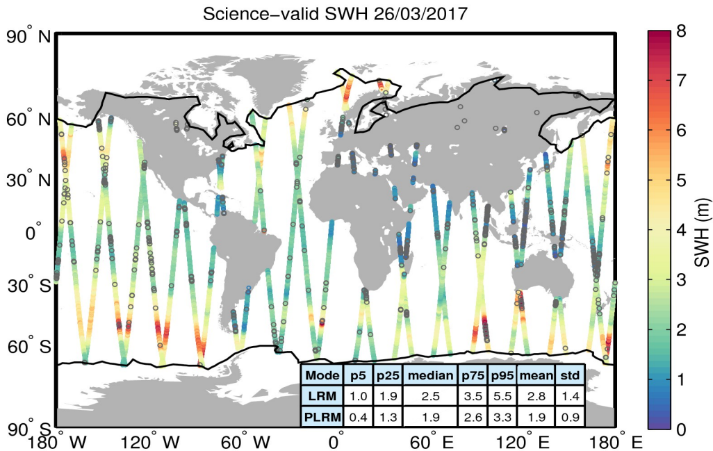
Figure 19. Geographical distribution of science-valid SWH data over oceans and lakes for 26/03/2017. The statistical values shown in the table refer to the SWH in m and are calculated separately for LRM and PLRM regions. The black lines mark the outer limit of the Arctic and Antarctic polar polygons. Gray circles denote records that have been rejected based on the editing criteria described in Table 3.
