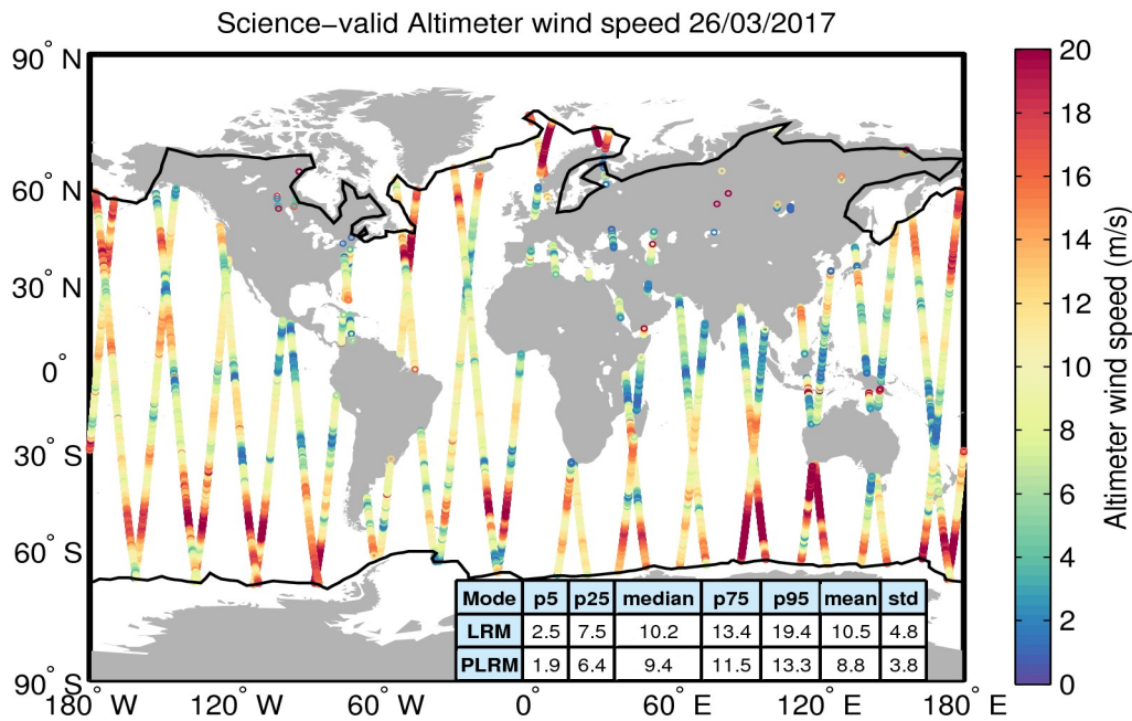
Figure 34. Geographical distribution of science-valid wind data over oceans and lakes for 26/03/2017. The statistical values shown in the table refer to the wind in m/s and are calculated separately for LRM and PLRM regions. The black lines mark the outer limit of the Arctic and Antarctic polar polygons. Gray circles denote records that have been rejected based on the editing criteria described in Table 5.
