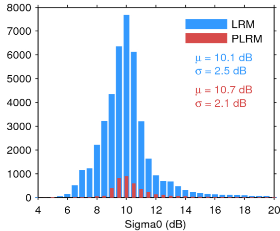
Figure 25. Histogram of flag-valid sigma0 over oceans and lakes for LRM (blue) and PLRM (red) for 26/03/2017. The mean ( \mu ) and standard deviation ( \sigma ) are also shown. Note that values outside [4 20] dB are excluded from the histogram for the sake of readability but not from the computation of \mu and \sigma .
