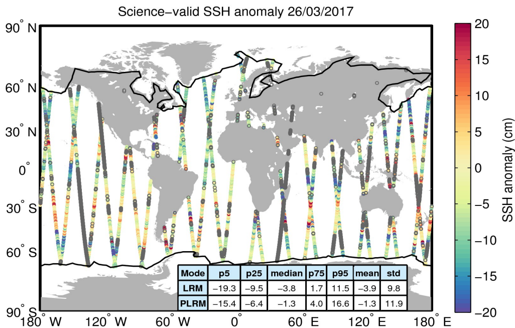
Figure 10. Geographical distribution of science-valid SSH anomaly data over oceans and lakes for 26/03/2017. The statistical values shown in the table refer to the SSH anomaly in cm and are calculated separately for LRM and PLRM regions. The black lines mark the outer limit of the Arctic and Antarctic polar polygons. Gray circles denote records that have been rejected based on the editing criteria described in Table 2.
