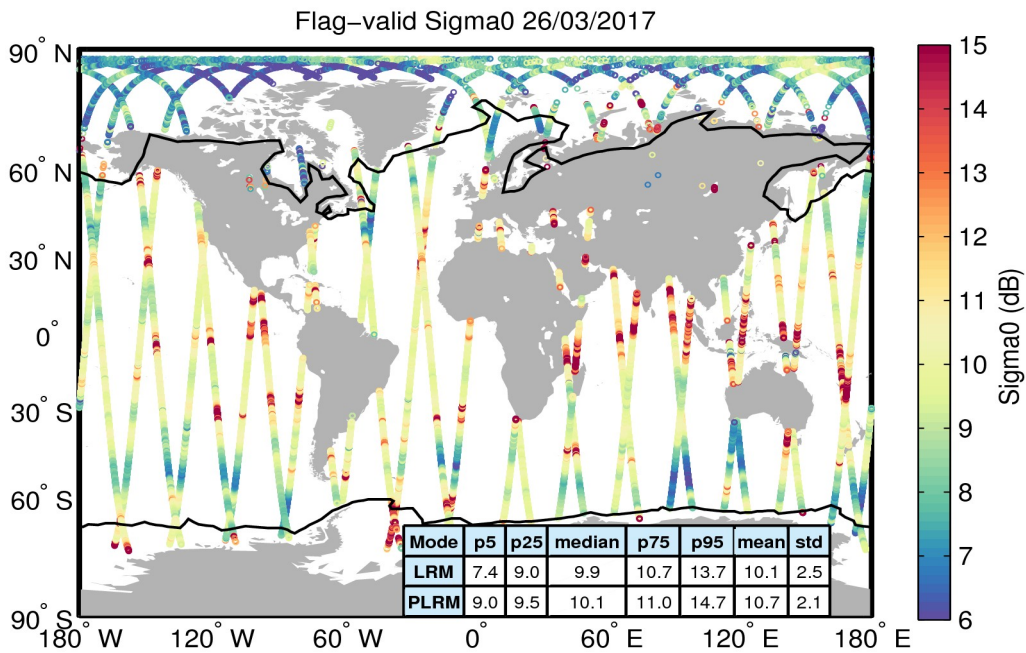
Figure 23. Geographical distribution of flag-valid sigma0 data over oceans and lakes for 26/03/2017. The statistical values shown in the table refer to the sigma0 in dB and are calculated separately for LRM and PLRM regions. Measurements taken over polar polygons have been excluded from the computation of the statistical values. The black lines mark the outer limit of the Arctic and Antarctic polar polygons.
