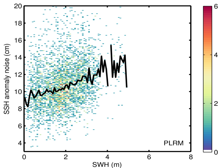
Figure 9. 2D histogram showing flag-valid SSH anomaly noise as a function of SWH for LRM (top) and PLRM (bottom) for 26/03/2017. The black line denotes the median SSH anomaly noise as a function of SWH.
