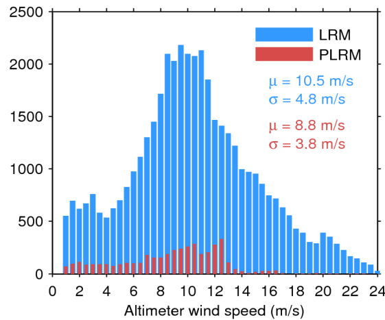
Figure 33. Histogram of flag-valid wind over oceans and lakes for LRM (blue) and PLRM (red) for 26/03/2017. The mean ( \mu ) and standard deviation ( \sigma ) are also shown. Note that values larger than 24 m/s are excluded from the histogram for the sake of readability but not from the computation of \mu and \sigma .
