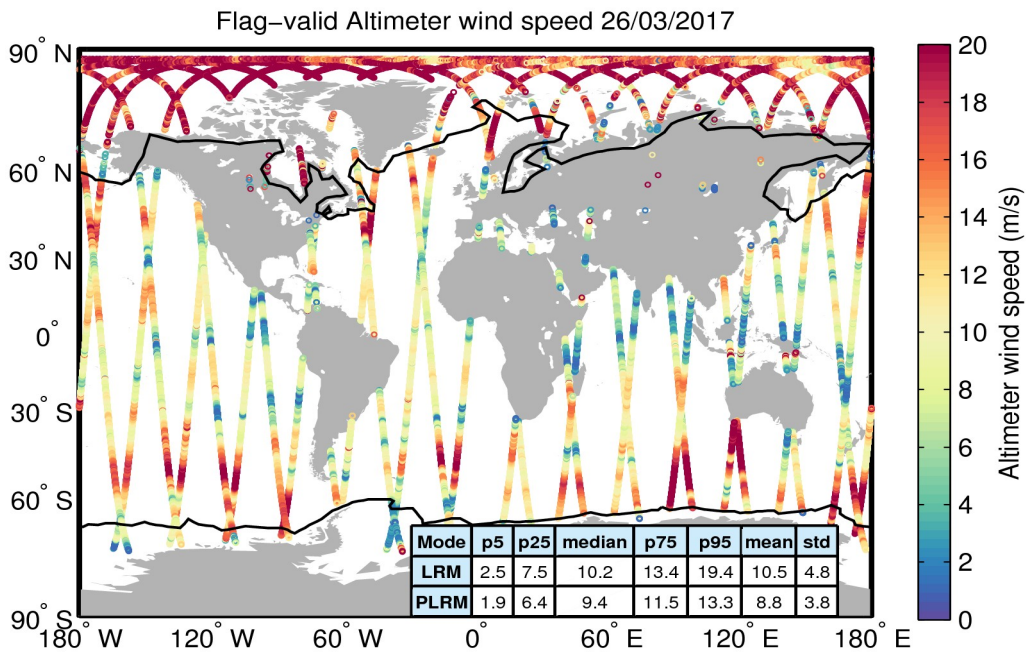
Figure 31. Geographical distribution of flag-valid wind data over oceans and lakes for 26/03/2017. The statistical values shown in the table refer to the wind in m/s and are calculated separately for LRM and PLRM regions. Measurements taken over polar polygons have been excluded from the computation of the statistical values. The black lines mark the outer limit of the Arctic and Antarctic polar polygons.
