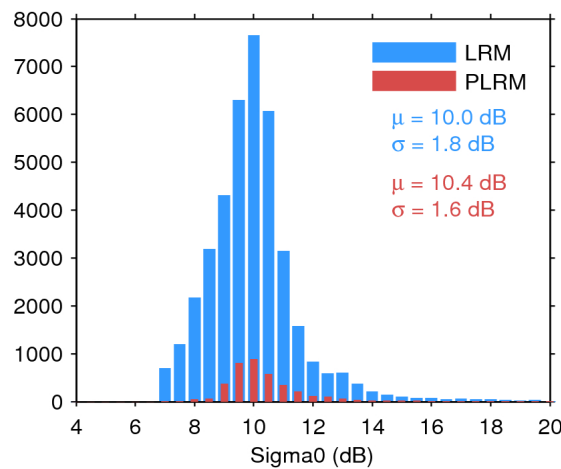
Figure 28. Histogram of science-valid sigma0 over oceans and lakes for LRM (blue) and PLRM (red) for 26/03/2017. The mean ( \mu ) and standard deviation ( \sigma ) are also shown. Note that values outside [4 20] dB are excluded from the histogram for the sake of readability but not from the computation of \mu and \sigma .
