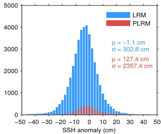
Figure 7. Histogram of flag-valid SSH anomaly over oceans and lakes for LRM (blue) and PLRM (red) for 26/03/2017. The mean ( \mu ) and standard deviation ( \sigma ) are also shown. Note that values outside [-50 50] cm are excluded from the histogram for the sake of readability but not from the computation of \mu and \sigma .
