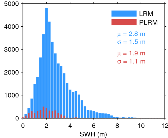
Figure 17. Histogram of flag-valid SWH over oceans and lakes for LRM (blue) and PLRM (red) for 26/03/2017. The mean ( \mu ) and standard deviation ( \sigma ) are also shown. Note that values larger than 12 m are excluded from the histogram for the sake of readability but not from the computation of \mu and \sigma .
