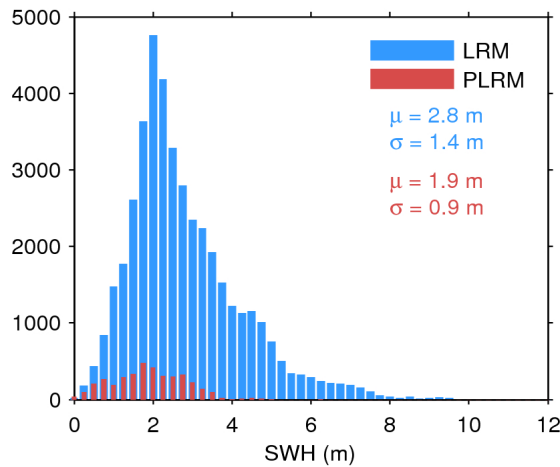
Figure 20. Histogram of science-valid SWH over oceans and lakes for LRM (blue) and PLRM (red) for 26/03/2017. The mean ( \mu ) and standard deviation ( \sigma ) are also shown. Note that values larger than 12 m are excluded from the histogram for the sake of readability but not from the computation of \mu and \sigma .
