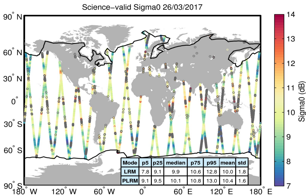
Figure 27. Geographical distribution of science-valid sigma0 data over oceans and lakes for 26/03/2017. The statistical values shown in the table refer to the sigma0 in dB and are calculated separately for LRM and PLRM regions. The black lines mark the outer limit of the Arctic and Antarctic polar polygons. Gray circles denote records that have been rejected based on the editing criteria described in Table 4.
