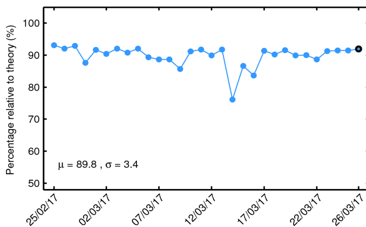
Figure 6. Percentage of flag-valid 1-Hz SSH records over ocean and lakes (including polar regions) relative to theory for each day in last 30-day window. The mean ( \mu ) and standard deviation ( \sigma ) are also shown.
