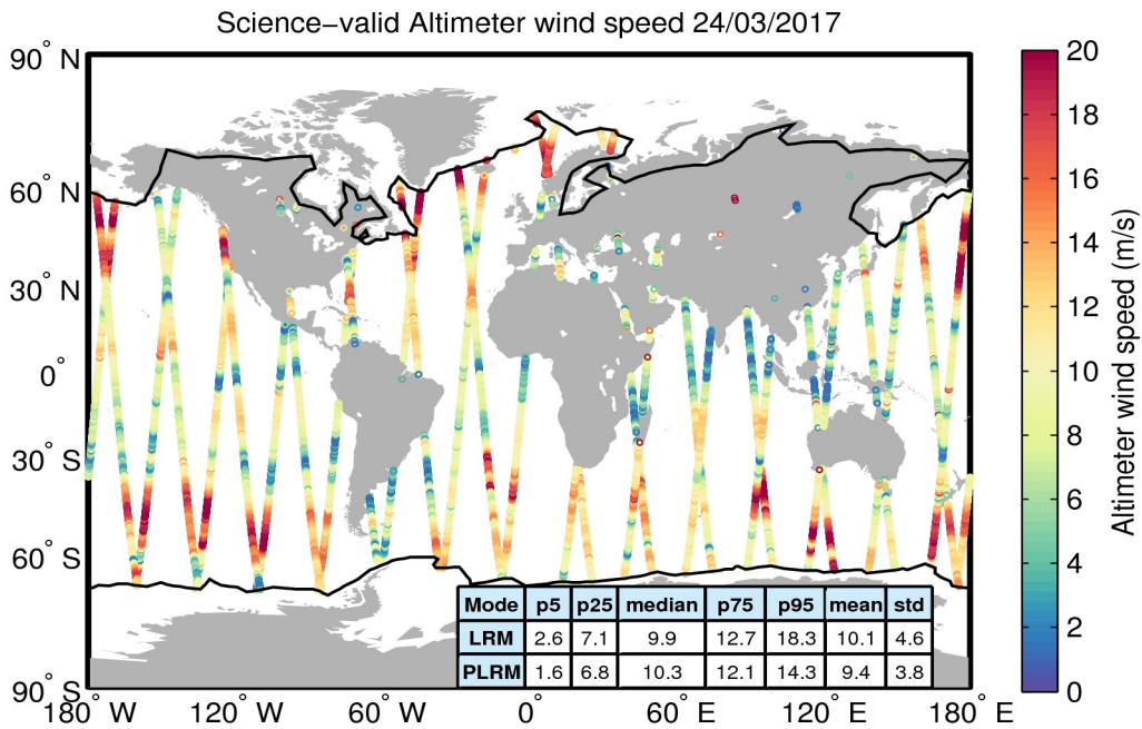
Figure 34. Geographical distribution of science-valid wind data over oceans and lakes for 24/03/2017. The statistical values shown in the table refer to the wind in m/s and are calculated separately for LRM and PLRM regions. The black lines mark the outer limit of the Arctic and Antarctic polar polygons. Gray circles denote records that have been rejected based on the editing criteria described in Table 5.
