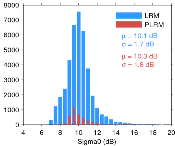
Figure 28. Histogram of science-valid sigma0 over oceans and lakes for LRM (blue) and PLRM (red) for 24/03/2017. The mean ( \mu ) and standard deviation ( \sigma ) are also shown. Note that values outside [4 20] dB are excluded from the histogram for the sake of readability but not from the computation of \mu and \sigma .
