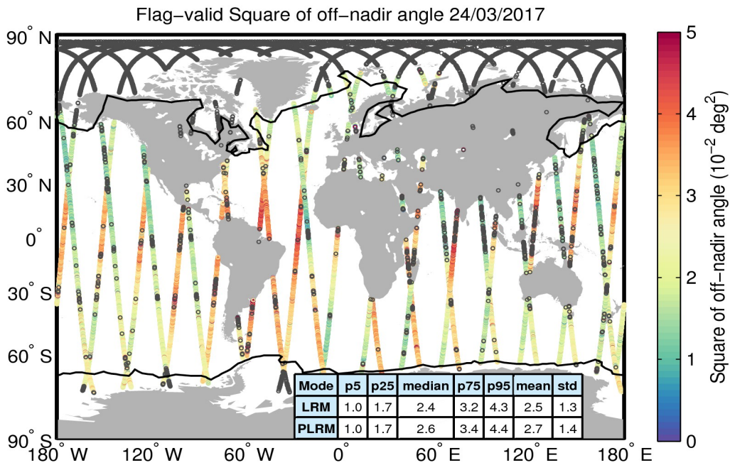
Figure 37. Geographical distribution of flag-valid mispointing data over oceans and lakes for 24/03/2017. The statistical values shown in the table refer to the mispointing in 10^{-2} deg 2 and are calculated separately for LRM and PLRM regions. Measurements taken over polar polygons have been excluded from the computation of the statistical values. The black lines mark the outer limit of the Arctic and Antarctic polar polygons. Gray circles denote negative values.
