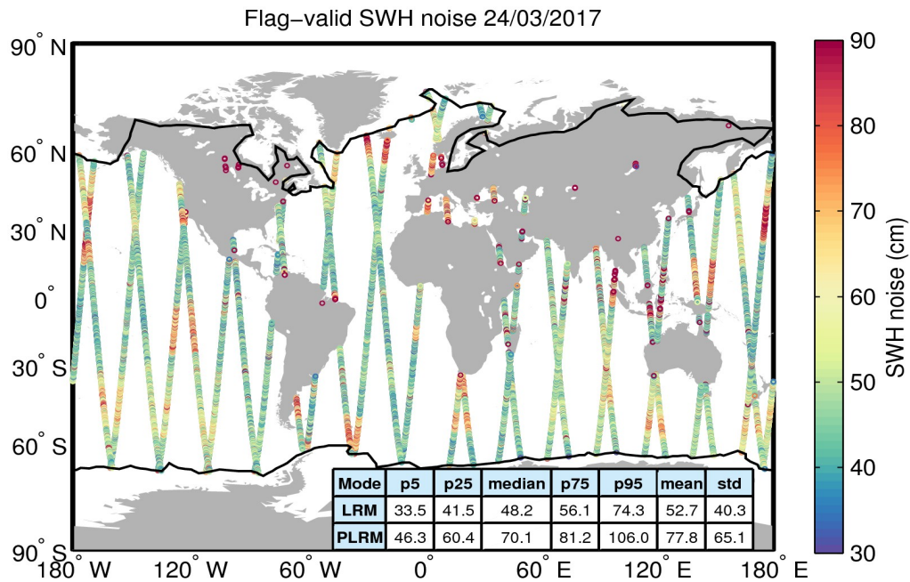
Figure 18. Geographical distribution of flag-valid 20-Hz SWH measurement noise over oceans and lakes for 24/03/2017. The statistical values shown in the table refer to the SWH noise and are calculated separately for LRM and PLRM regions. Measurements taken over polar polygons have been excluded from the computation of the statistical values. The black lines mark the outer limit of the Arctic and Antarctic polar polygons.
