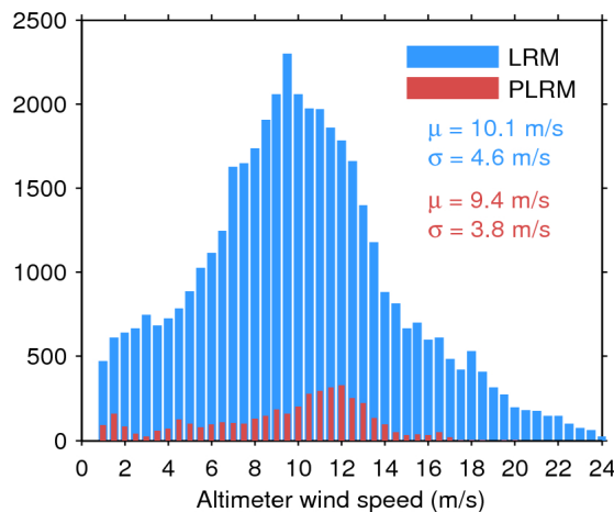
Figure 35. Histogram of science-valid wind over oceans and lakes for LRM (blue) and PLRM (red) for 24/03/2017. The mean ( \mu ) and standard deviation ( \sigma ) are also shown. Note that values larger than 24 m/s are excluded from the histogram for the sake of readability but not from the computation of \mu and \sigma .
