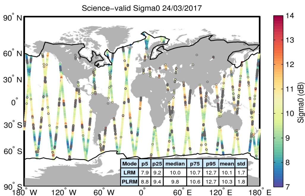
Figure 27. Geographical distribution of science-valid sigma0 data over oceans and lakes for 24/03/2017. The statistical values shown in the table refer to the sigma0 in dB and are calculated separately for LRM and PLRM regions. The black lines mark the outer limit of the Arctic and Antarctic polar polygons. Gray circles denote records that have been rejected based on the editing criteria described in Table 4.
