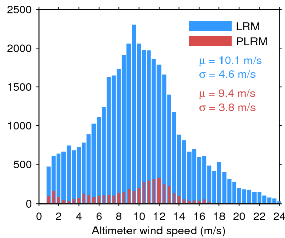
Figure 33. Histogram of flag-valid wind over oceans and lakes for LRM (blue) and PLRM (red) for 24/03/2017. The mean ( \mu ) and standard deviation ( \sigma ) are also shown. Note that values larger than 24 m/s are excluded from the histogram for the sake of readability but not from the computation of \mu and \sigma .
