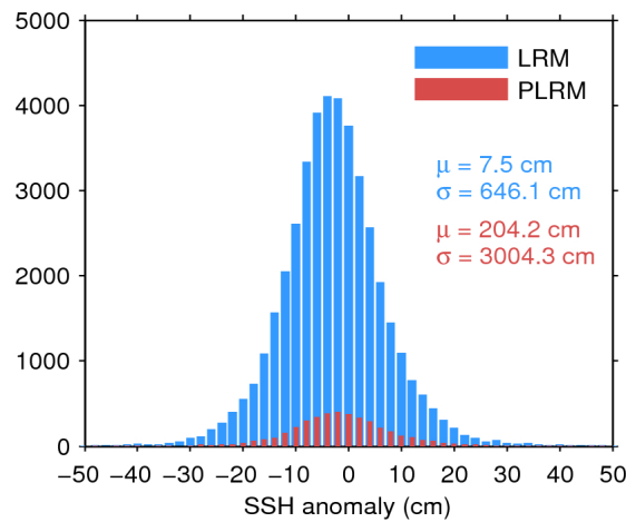
Figure 7. Histogram of flag-valid SSH anomaly over oceans and lakes for LRM (blue) and PLRM (red) for 24/03/2017. The mean ( \mu ) and standard deviation ( \sigma ) are also shown. Note that values outside [-50 50] cm are excluded from the histogram for the sake of readability but not from the computation of \mu and \sigma .
