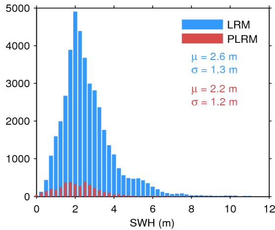
Figure 20. Histogram of science-valid SWH over oceans and lakes for LRM (blue) and PLRM (red) for 24/03/2017. The mean ( \mu ) and standard deviation ( \sigma ) are also shown. Note that values larger than 12 m are excluded from the histogram for the sake of readability but not from the computation of \mu and \sigma .
