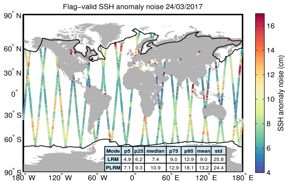
Figure 8. Geographical distribution of flag-valid 20-Hz SSH anomaly measurement noise over oceans and lakes for 24/03/2017. The statistical values shown in the table refer to the SSH anomaly noise and are calculated separately for LRM and PLRM regions. Measurements taken over polar polygons have been excluded from the computation of the statistical values. The black lines mark the outer limit of the Arctic and Antarctic polar polygons.
