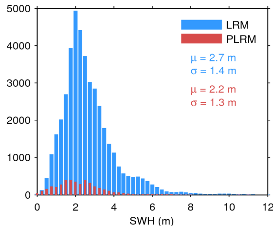
Figure 17. Histogram of flag-valid SWH over oceans and lakes for LRM (blue) and PLRM (red) for 24/03/2017. The mean ( \mu ) and standard deviation ( \sigma ) are also shown. Note that values larger than 12 m are excluded from the histogram for the sake of readability but not from the computation of \mu and \sigma .
