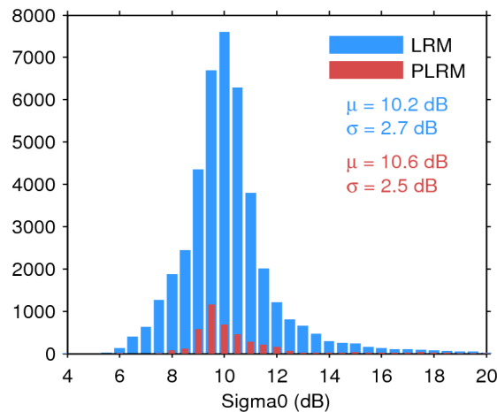
Figure 25. Histogram of flag-valid sigma0 over oceans and lakes for LRM (blue) and PLRM (red) for 24/03/2017. The mean ( \mu ) and standard deviation ( \sigma ) are also shown. Note that values outside [4 20] dB are excluded from the histogram for the sake of readability but not from the computation of \mu and \sigma .
