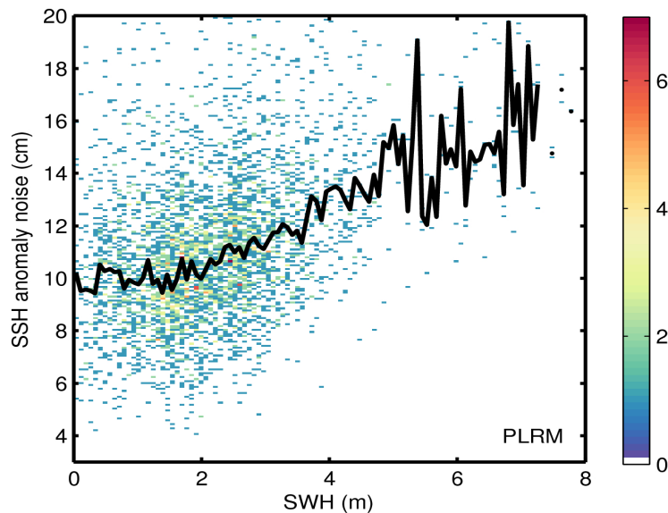
Figure 9. 2D histogram showing flag-valid SSH anomaly noise as a function of SWH for LRM (top) and PLRM (bottom) for 24/03/2017. The black line denotes the median SSH anomaly noise as a function of SWH.
