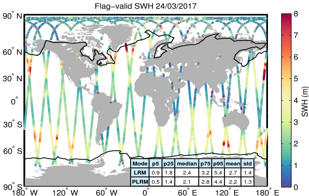
Figure 15. Geographical distribution of flag-valid SWH data over oceans and lakes for 24/03/2017. The statistical values shown in the table refer to the SWH in m and are calculated separately for LRM and PLRM regions. Measurements taken over polar polygons have been excluded from the computation of the statistical values. The black lines mark the outer limit of the Arctic and Antarctic polar polygons.
