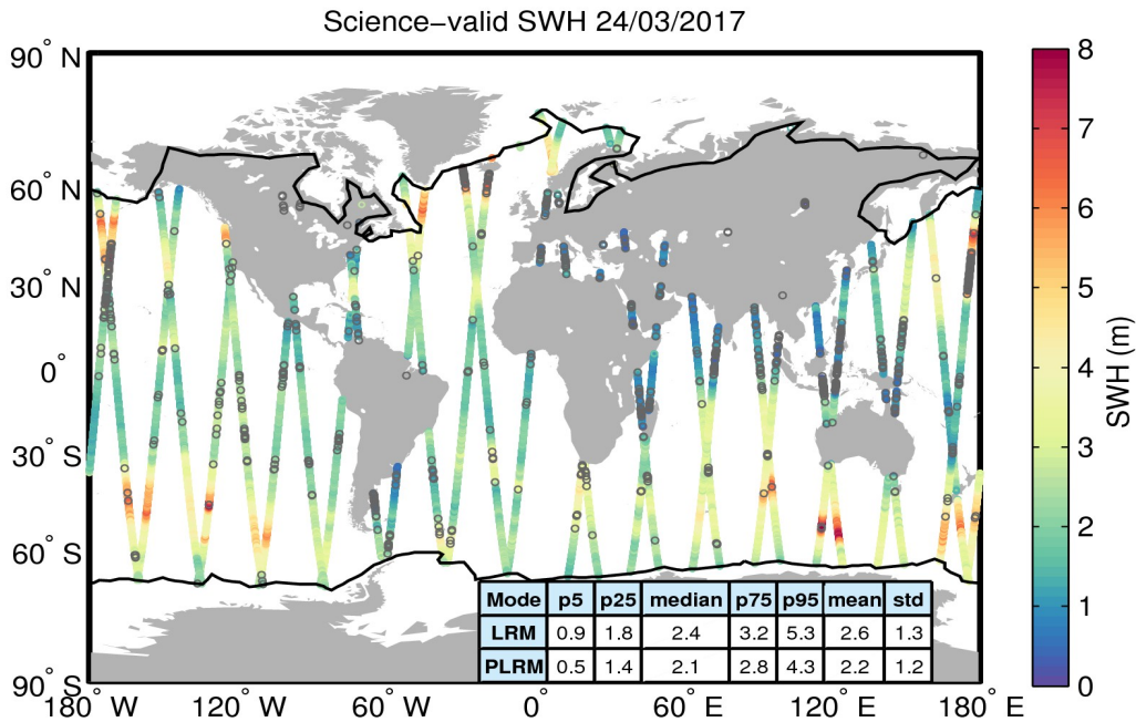
Figure 19. Geographical distribution of science-valid SWH data over oceans and lakes for 24/03/2017. The statistical values shown in the table refer to the SWH in m and are calculated separately for LRM and PLRM regions. The black lines mark the outer limit of the Arctic and Antarctic polar polygons. Gray circles denote records that have been rejected based on the editing criteria described in Table 3.
