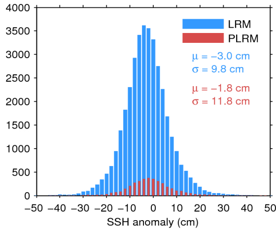
Figure 11. Histogram of science-valid SSH anomaly over oceans and lakes for LRM (blue) and PLRM (red) for 24/03/2017. The mean ( \mu ) and standard deviation ( \sigma ) are also shown. Note that values outside [-50 50] cm are excluded from the histogram for the sake of readability but not from the computation of \mu and \sigma .
