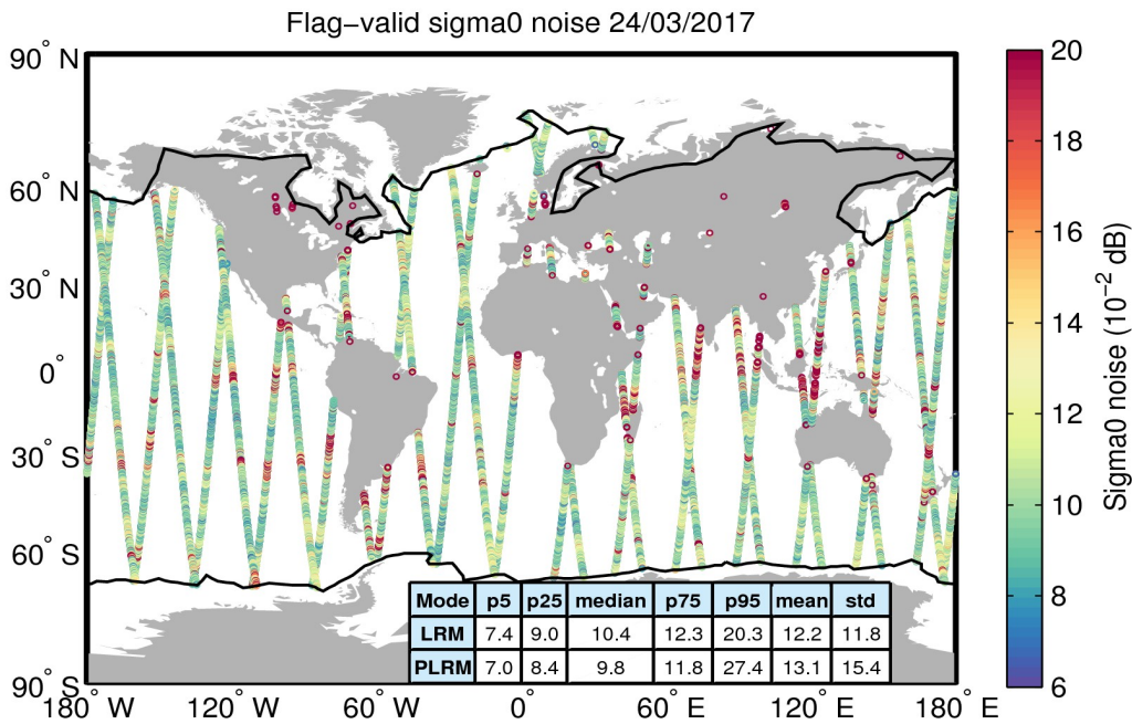
Figure 26. Geographical distribution of flag-valid 20-Hz sigma0 measurement noise over oceans and lakes for 24/03/2017. The statistical values shown in the table refer to the sigma0 noise and are calculated separately for LRM and PLRM regions. Measurements taken over polar polygons have been excluded from the computation of the statistical values. The black lines mark the outer limit of the Arctic and Antarctic polar polygons.
