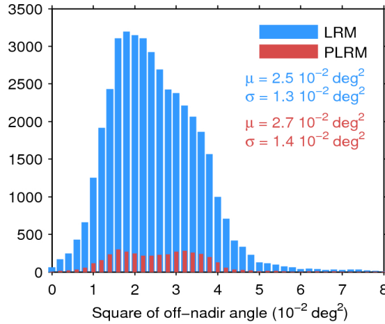
Figure 39. Histogram of flag-valid mispointing over oceans and lakes for LRM (blue) and PLRM (red) for 24/03/2017. Only positive values have been considered. The mean ( \mu ) and standard deviation ( \sigma ) are also shown. Note that values larger than 8 \cdot 10^{-2} \text{ deg}^2 are excluded from the histogram for the sake of readability but not from the computation of \mu and \sigma .
