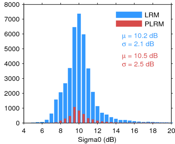
Figure 25. Histogram of flag-valid sigma0 over oceans and lakes for LRM (blue) and PLRM (red) for 22/03/2017. The mean ( \mu ) and standard deviation ( \sigma ) are also shown. Note that values outside [4 20] dB are excluded from the histogram for the sake of readability but not from the computation of \mu and \sigma .
