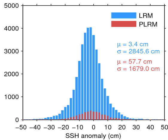
Figure 7. Histogram of flag-valid SSH anomaly over oceans and lakes for LRM (blue) and PLRM (red) for 22/03/2017. The mean ( \mu ) and standard deviation ( \sigma ) are also shown. Note that values outside [-50 50] cm are excluded from the histogram for the sake of readability but not from the computation of \mu and \sigma .
