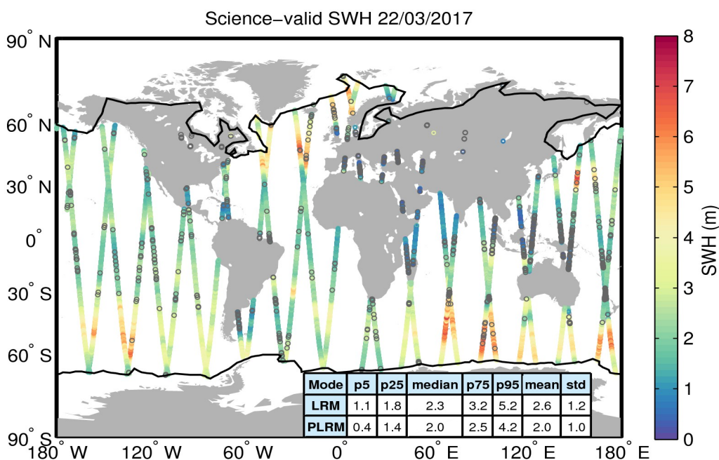
Figure 19. Geographical distribution of science-valid SWH data over oceans and lakes for 22/03/2017. The statistical values shown in the table refer to the SWH in m and are calculated separately for LRM and PLRM regions. The black lines mark the outer limit of the Arctic and Antarctic polar polygons. Gray circles denote records that have been rejected based on the editing criteria described in Table 3.
