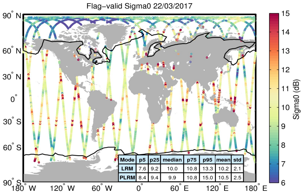
Figure 23. Geographical distribution of flag-valid sigma0 data over oceans and lakes for 22/03/2017. The statistical values shown in the table refer to the sigma0 in dB and are calculated separately for LRM and PLRM regions. Measurements taken over polar polygons have been excluded from the computation of the statistical values. The black lines mark the outer limit of the Arctic and Antarctic polar polygons.
