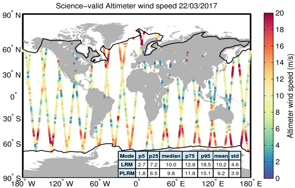
Figure 34. Geographical distribution of science-valid wind data over oceans and lakes for 22/03/2017. The statistical values shown in the table refer to the wind in m/s and are calculated separately for LRM and PLRM regions. The black lines mark the outer limit of the Arctic and Antarctic polar polygons. Gray circles denote records that have been rejected based on the editing criteria described in Table 5.
