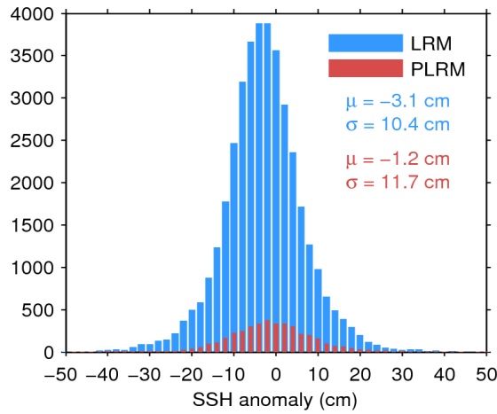
Figure 11. Histogram of science-valid SSH anomaly over oceans and lakes for LRM (blue) and PLRM (red) for 22/03/2017. The mean ( \mu ) and standard deviation ( \sigma ) are also shown. Note that values outside [-50\ 50] cm are excluded from the histogram for the sake of readability but not from the computation of \mu and \sigma .
