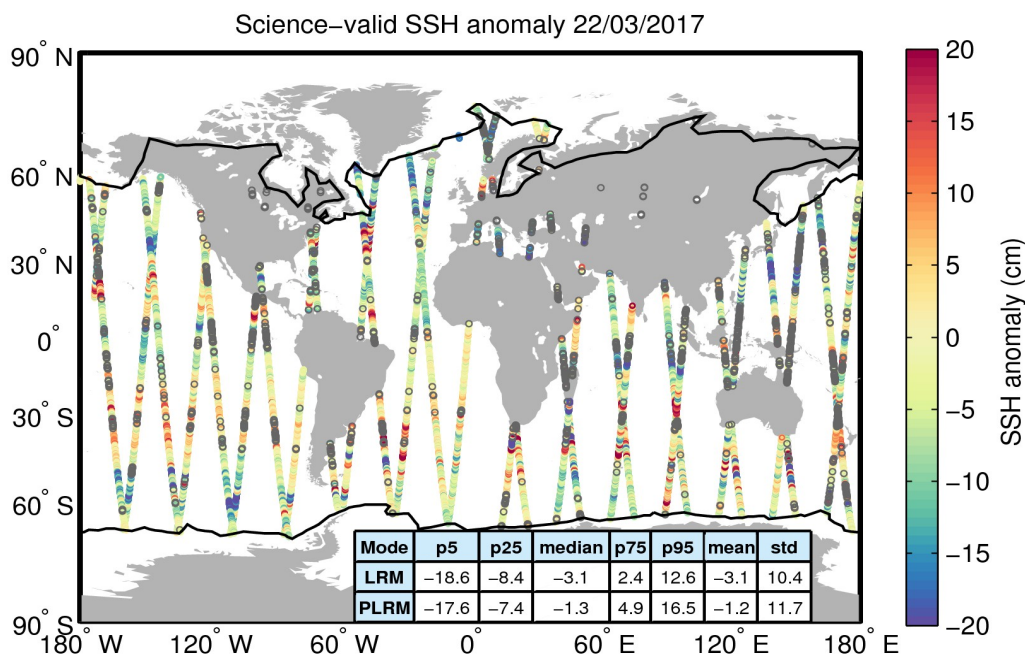
Figure 10. Geographical distribution of science-valid SSH anomaly data over oceans and lakes for 22/03/2017. The statistical values shown in the table refer to the SSH anomaly in cm and are calculated separately for LRM and PLRM regions. The black lines mark the outer limit of the Arctic and Antarctic polar polygons. Gray circles denote records that have been rejected based on the editing criteria described in Table 2.
