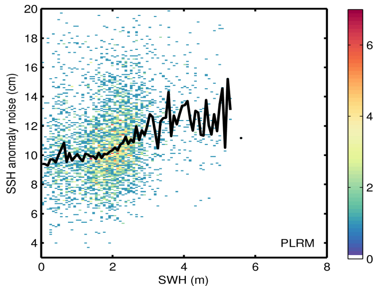
Figure 9. 2D histogram showing flag-valid SSH anomaly noise as a function of SWH for LRM (top) and PLRM (bottom) for 22/03/2017. The black line denotes the median SSH anomaly noise as a function of SWH.
