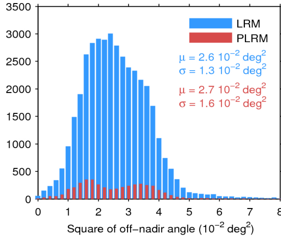
Figure 39. Histogram of flag-valid mispointing over oceans and lakes for LRM (blue) and PLRM (red) for 22/03/2017. Only positive values have been considered. The mean ( \mu ) and standard deviation ( \sigma ) are also shown. Note that values larger than 8 \cdot 10^{-2} \text{ deg}^2 are excluded from the histogram for the sake of readability but not from the computation of \mu and \sigma .
