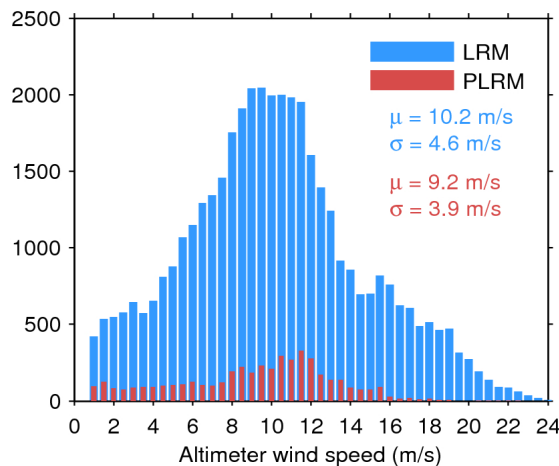
Figure 35. Histogram of science-valid wind over oceans and lakes for LRM (blue) and PLRM (red) for 22/03/2017. The mean ( \mu ) and standard deviation ( \sigma ) are also shown. Note that values larger than 24 m/s are excluded from the histogram for the sake of readability but not from the computation of \mu and \sigma .
