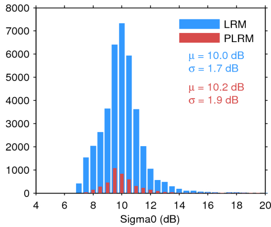
Figure 28. Histogram of science-valid sigma0 over oceans and lakes for LRM (blue) and PLRM (red) for 22/03/2017. The mean ( \mu ) and standard deviation ( \sigma ) are also shown. Note that values outside [4 20] dB are excluded from the histogram for the sake of readability but not from the computation of \mu and \sigma .
