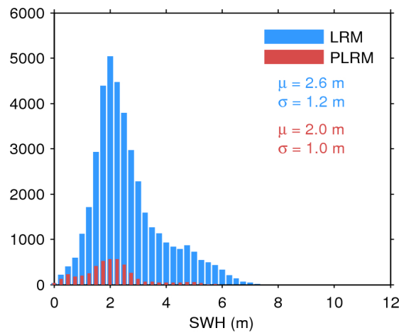
Figure 20. Histogram of science-valid SWH over oceans and lakes for LRM (blue) and PLRM (red) for 22/03/2017. The mean ( \mu ) and standard deviation ( \sigma ) are also shown. Note that values larger than 12 m are excluded from the histogram for the sake of readability but not from the computation of \mu and \sigma .
