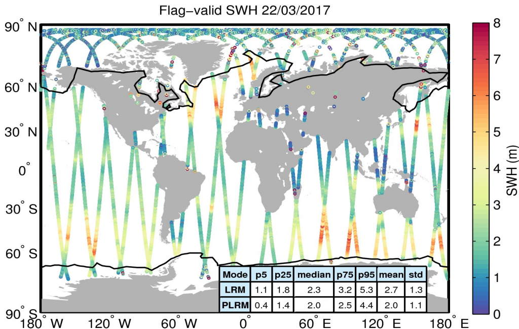
Figure 15. Geographical distribution of flag-valid SWH data over oceans and lakes for 22/03/2017. The statistical values shown in the table refer to the SWH in m and are calculated separately for LRM and PLRM regions. Measurements taken over polar polygons have been excluded from the computation of the statistical values. The black lines mark the outer limit of the Arctic and Antarctic polar polygons.
