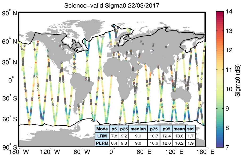
Figure 27. Geographical distribution of science-valid sigma0 data over oceans and lakes for 22/03/2017. The statistical values shown in the table refer to the sigma0 in dB and are calculated separately for LRM and PLRM regions. The black lines mark the outer limit of the Arctic and Antarctic polar polygons. Gray circles denote records that have been rejected based on the editing criteria described in Table 4.
