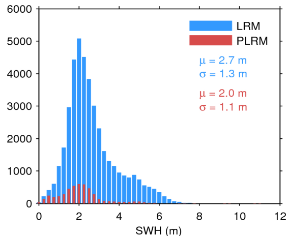
Figure 17. Histogram of flag-valid SWH over oceans and lakes for LRM (blue) and PLRM (red) for 22/03/2017. The mean ( \mu ) and standard deviation ( \sigma ) are also shown. Note that values larger than 12 m are excluded from the histogram for the sake of readability but not from the computation of \mu and \sigma .
