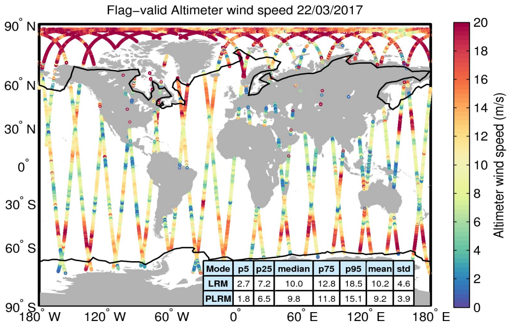
Figure 31. Geographical distribution of flag-valid wind data over oceans and lakes for 22/03/2017. The statistical values shown in the table refer to the wind in m/s and are calculated separately for LRM and PLRM regions. Measurements taken over polar polygons have been excluded from the computation of the statistical values. The black lines mark the outer limit of the Arctic and Antarctic polar polygons.
