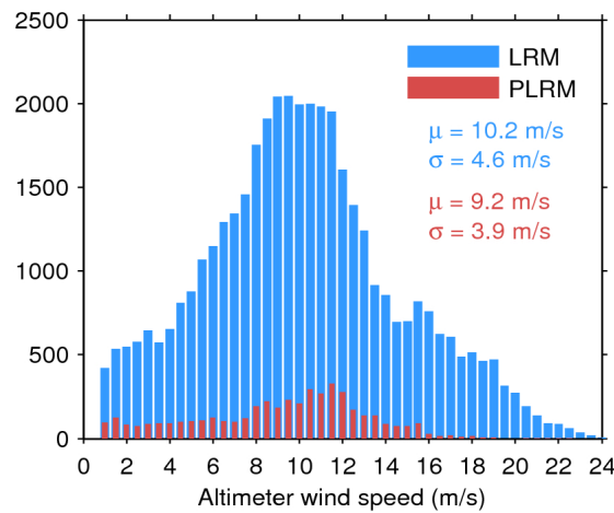
Figure 33. Histogram of flag-valid wind over oceans and lakes for LRM (blue) and PLRM (red) for 22/03/2017. The mean ( \mu ) and standard deviation ( \sigma ) are also shown. Note that values larger than 24 m/s are excluded from the histogram for the sake of readability but not from the computation of \mu and \sigma .
