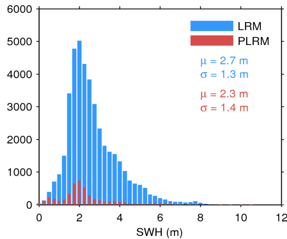
Figure 17. Histogram of flag-valid SWH over oceans and lakes for LRM (blue) and PLRM (red) for 21/03/2017. The mean ( \mu ) and standard deviation ( \sigma ) are also shown. Note that values larger than 12 m are excluded from the histogram for the sake of readability but not from the computation of \mu and \sigma .
