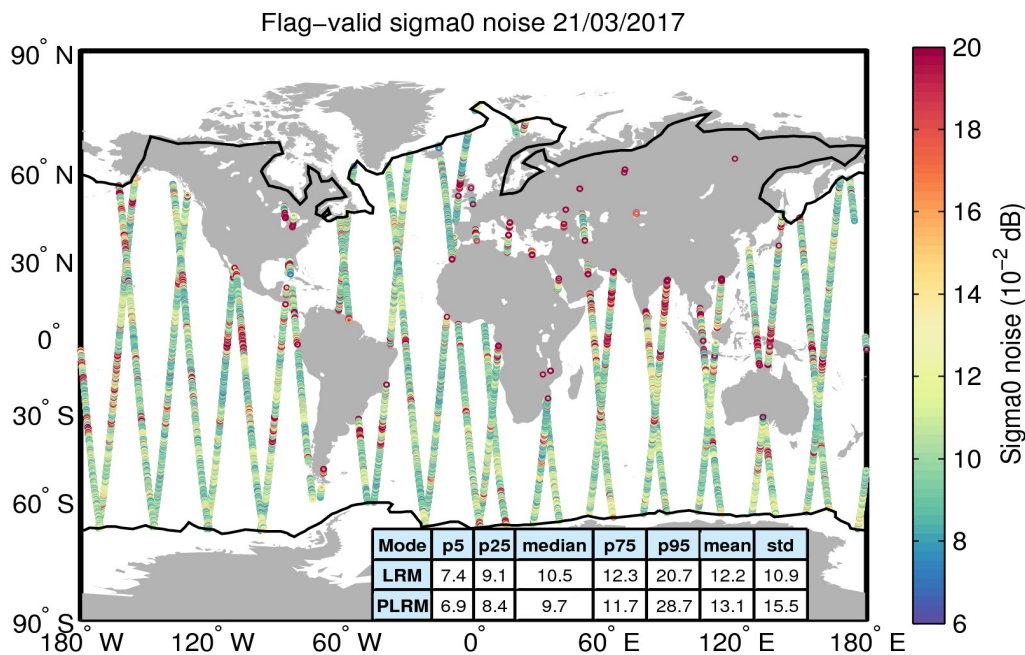
Figure 26. Geographical distribution of flag-valid 20-Hz sigma0 measurement noise over oceans and lakes for 21/03/2017. The statistical values shown in the table refer to the sigma0 noise and are calculated separately for LRM and PLRM regions. Measurements taken over polar polygons have been excluded from the computation of the statistical values. The black lines mark the outer limit of the Arctic and Antarctic polar polygons.
