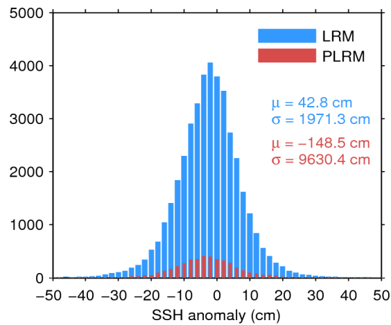
Figure 7. Histogram of flag-valid SSH anomaly over oceans and lakes for LRM (blue) and PLRM (red) for 21/03/2017. The mean ( \mu ) and standard deviation ( \sigma ) are also shown. Note that values outside [-50\ 50] cm are excluded from the histogram for the sake of readability but not from the computation of \mu and \sigma .
