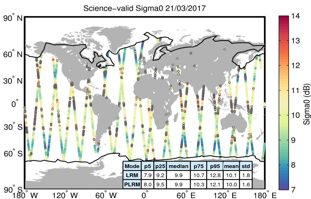
Figure 27. Geographical distribution of science-valid sigma0 data over oceans and lakes for 21/03/2017. The statistical values shown in the table refer to the sigma0 in dB and are calculated separately for LRM and PLRM regions. The black lines mark the outer limit of the Arctic and Antarctic polar polygons. Gray circles denote records that have been rejected based on the editing criteria described in Table 4.
