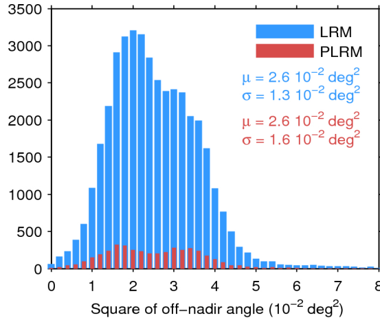
Figure 39. Histogram of flag-valid mispointing over oceans and lakes for LRM (blue) and PLRM (red) for 21/03/2017. Only positive values have been considered. The mean ( \mu ) and standard deviation ( \sigma ) are also shown. Note that values larger than 8 \cdot 10^{-2} \text{ deg}^2 are excluded from the histogram for the sake of readability but not from the computation of \mu and \sigma .
