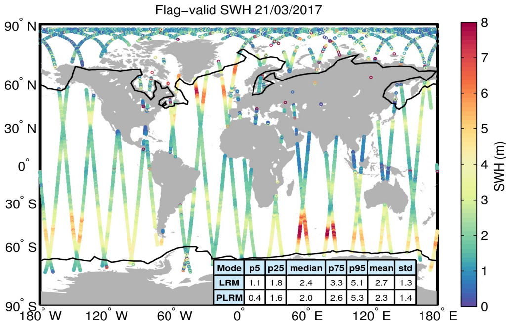
Figure 15. Geographical distribution of flag-valid SWH data over oceans and lakes for 21/03/2017. The statistical values shown in the table refer to the SWH in m and are calculated separately for LRM and PLRM regions. Measurements taken over polar polygons have been excluded from the computation of the statistical values. The black lines mark the outer limit of the Arctic and Antarctic polar polygons.
