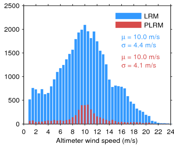
Figure 33. Histogram of flag-valid wind over oceans and lakes for LRM (blue) and PLRM (red) for 21/03/2017. The mean ( \mu ) and standard deviation ( \sigma ) are also shown. Note that values larger than 24 m/s are excluded from the histogram for the sake of readability but not from the computation of \mu and \sigma .
