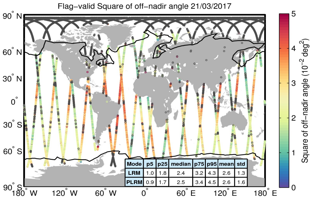
Figure 37. Geographical distribution of flag-valid mispointing data over oceans and lakes for 21/03/2017. The statistical values shown in the table refer to the mispointing in 10^{-2} deg 2 and are calculated separately for LRM and PLRM regions. Measurements taken over polar polygons have been excluded from the computation of the statistical values. The black lines mark the outer limit of the Arctic and Antarctic polar polygons. Gray circles denote negative values.
