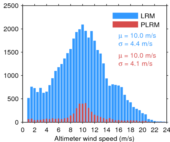
Figure 35. Histogram of science-valid wind over oceans and lakes for LRM (blue) and PLRM (red) for 21/03/2017. The mean ( \mu ) and standard deviation ( \sigma ) are also shown. Note that values larger than 24 m/s are excluded from the histogram for the sake of readability but not from the computation of \mu and \sigma .
