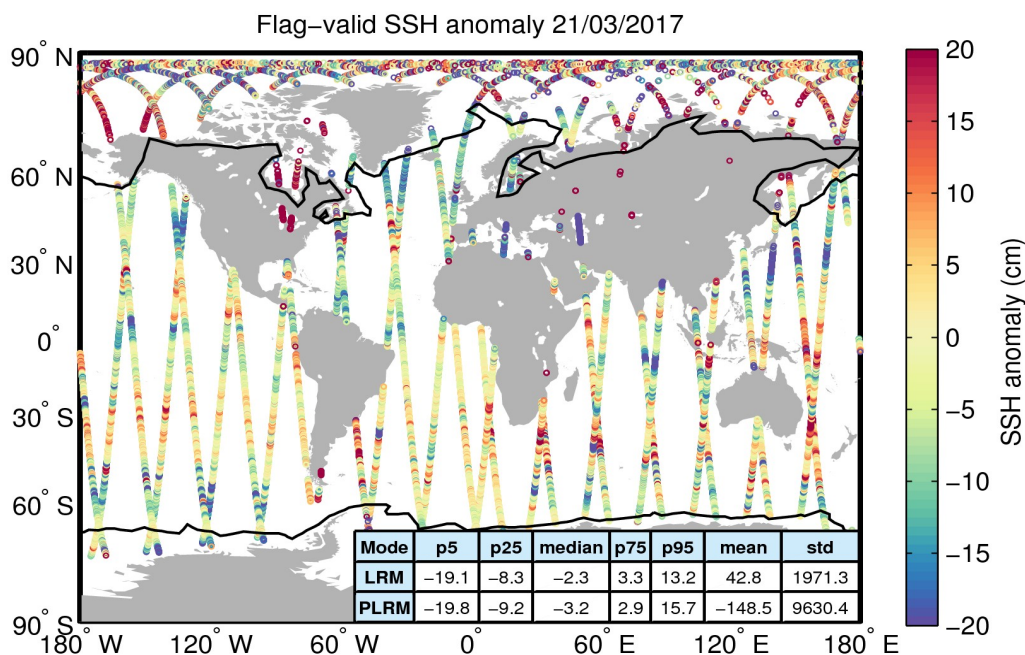
Figure 5. Geographical distribution of flag-valid 1-Hz SSH anomaly data over oceans and lakes for 21/03/2017. The statistical values shown in the table refer to the SSH anomaly in cm and are calculated separately for LRM and PLRM regions. Measurements taken over polar polygons have been excluded from the computation of the statistical values. The black lines mark the outer limit of the Arctic and Antarctic polar polygons.
