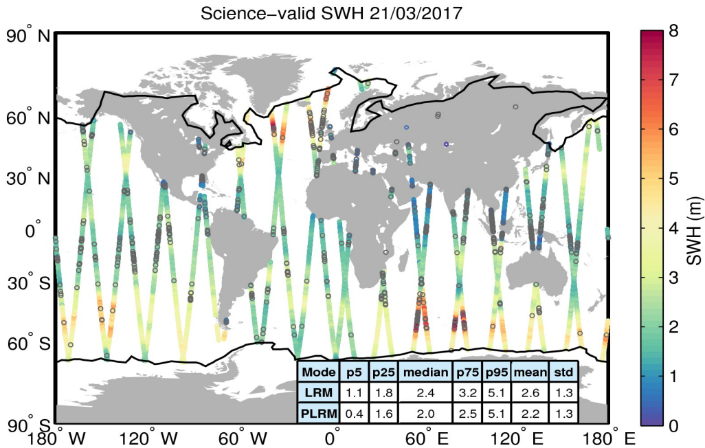
Figure 19. Geographical distribution of science-valid SWH data over oceans and lakes for 21/03/2017. The statistical values shown in the table refer to the SWH in m and are calculated separately for LRM and PLRM regions. The black lines mark the outer limit of the Arctic and Antarctic polar polygons. Gray circles denote records that have been rejected based on the editing criteria described in Table 3.
