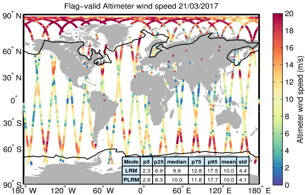
Figure 31. Geographical distribution of flag-valid wind data over oceans and lakes for 21/03/2017. The statistical values shown in the table refer to the wind in m/s and are calculated separately for LRM and PLRM regions. Measurements taken over polar polygons have been excluded from the computation of the statistical values. The black lines mark the outer limit of the Arctic and Antarctic polar polygons.
