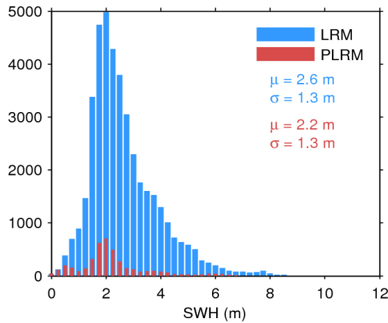
Figure 20. Histogram of science-valid SWH over oceans and lakes for LRM (blue) and PLRM (red) for 21/03/2017. The mean ( \mu ) and standard deviation ( \sigma ) are also shown. Note that values larger than 12 m are excluded from the histogram for the sake of readability but not from the computation of \mu and \sigma .
