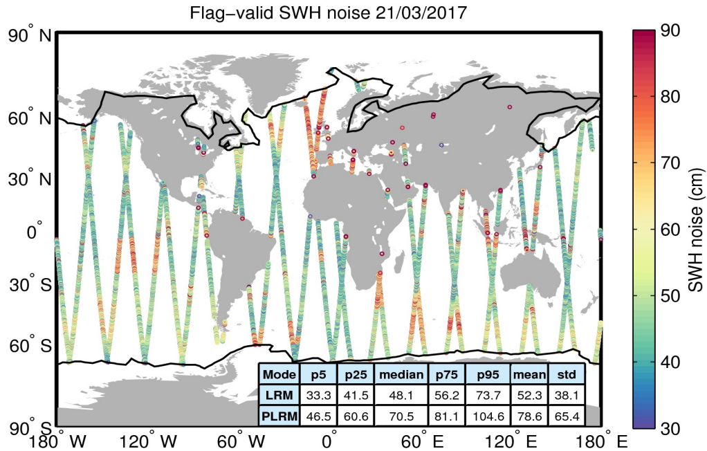
Figure 18. Geographical distribution of flag-valid 20-Hz SWH measurement noise over oceans and lakes for 21/03/2017. The statistical values shown in the table refer to the SWH noise and are calculated separately for LRM and PLRM regions. Measurements taken over polar polygons have been excluded from the computation of the statistical values. The black lines mark the outer limit of the Arctic and Antarctic polar polygons.
