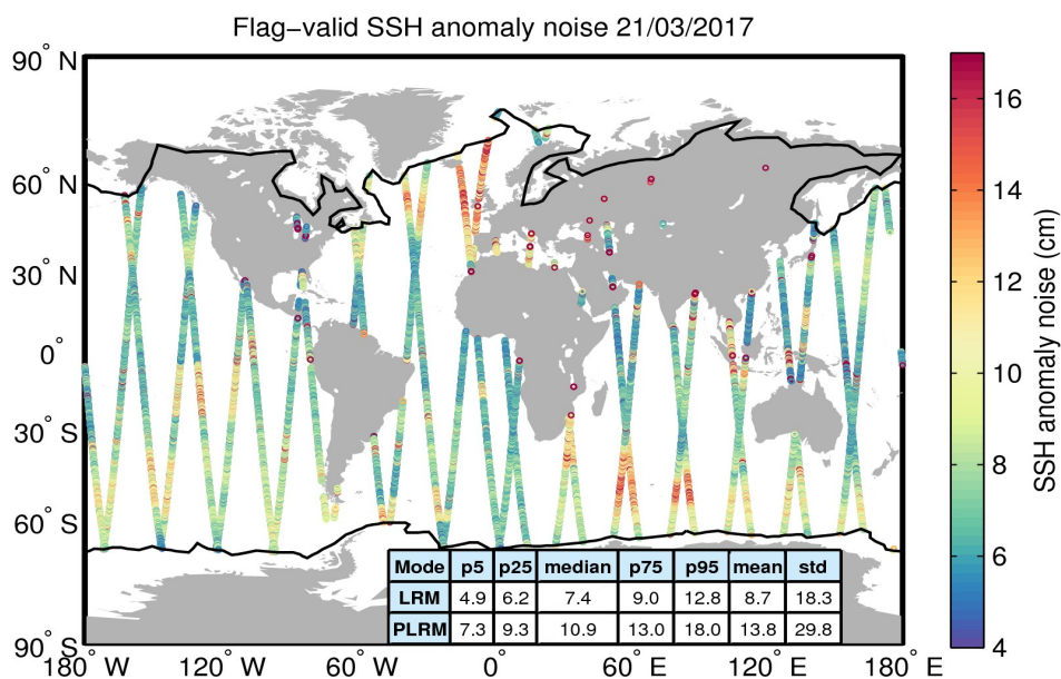
Figure 8. Geographical distribution of flag-valid 20-Hz SSH anomaly measurement noise over oceans and lakes for 21/03/2017. The statistical values shown in the table refer to the SSH anomaly noise and are calculated separately for LRM and PLRM regions. Measurements taken over polar polygons have been excluded from the computation of the statistical values. The black lines mark the outer limit of the Arctic and Antarctic polar polygons.
