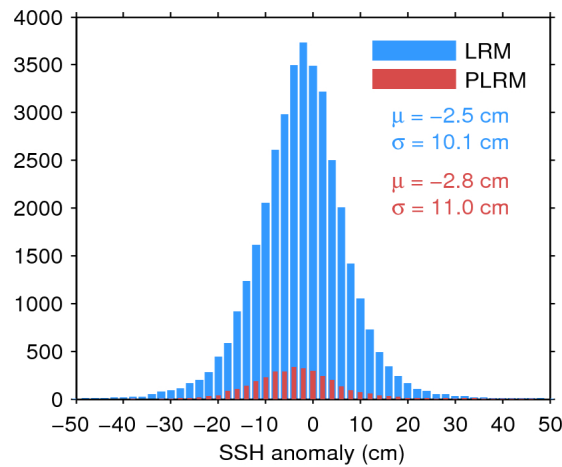
Figure 11. Histogram of science-valid SSH anomaly over oceans and lakes for LRM (blue) and PLRM (red) for 21/03/2017. The mean ( \mu ) and standard deviation ( \sigma ) are also shown. Note that values outside [-50 50] cm are excluded from the histogram for the sake of readability but not from the computation of \mu and \sigma .
