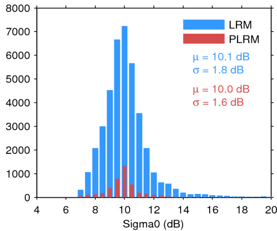
Figure 28. Histogram of science-valid sigma0 over oceans and lakes for LRM (blue) and PLRM (red) for 21/03/2017. The mean ( \mu ) and standard deviation ( \sigma ) are also shown. Note that values outside [4 20] dB are excluded from the histogram for the sake of readability but not from the computation of \mu and \sigma .
