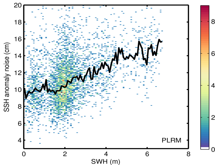
Figure 9. 2D histogram showing flag-valid SSH anomaly noise as a function of SWH for LRM (top) and PLRM (bottom) for 21/03/2017. The black line denotes the median SSH anomaly noise as a function of SWH.
