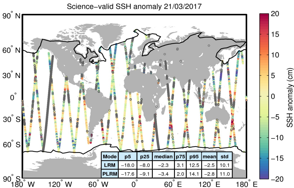
Figure 10. Geographical distribution of science-valid SSH anomaly data over oceans and lakes for 21/03/2017. The statistical values shown in the table refer to the SSH anomaly in cm and are calculated separately for LRM and PLRM regions. The black lines mark the outer limit of the Arctic and Antarctic polar polygons. Gray circles denote records that have been rejected based on the editing criteria described in Table 2.
