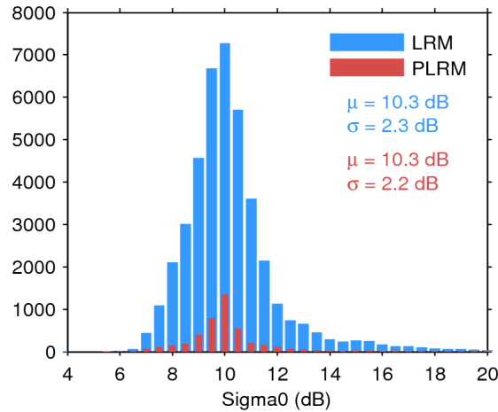
Figure 25. Histogram of flag-valid sigma0 over oceans and lakes for LRM (blue) and PLRM (red) for 21/03/2017. The mean ( \mu ) and standard deviation ( \sigma ) are also shown. Note that values outside [4 20] dB are excluded from the histogram for the sake of readability but not from the computation of \mu and \sigma .
