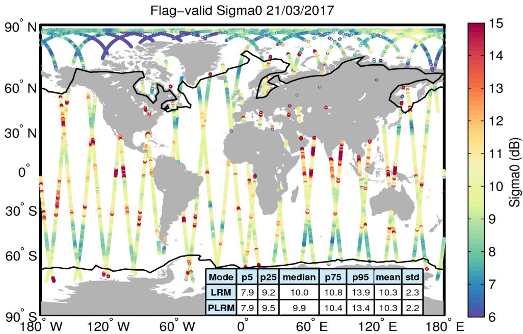
Figure 23. Geographical distribution of flag-valid sigma0 data over oceans and lakes for 21/03/2017. The statistical values shown in the table refer to the sigma0 in dB and are calculated separately for LRM and PLRM regions. Measurements taken over polar polygons have been excluded from the computation of the statistical values. The black lines mark the outer limit of the Arctic and Antarctic polar polygons.
