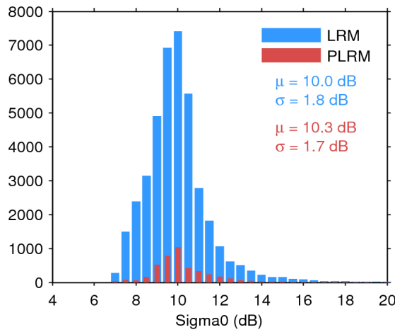
Figure 28. Histogram of science-valid sigma0 over oceans and lakes for LRM (blue) and PLRM (red) for 20/03/2017. The mean ( \mu ) and standard deviation ( \sigma ) are also shown. Note that values outside [4 20] dB are excluded from the histogram for the sake of readability but not from the computation of \mu and \sigma .
