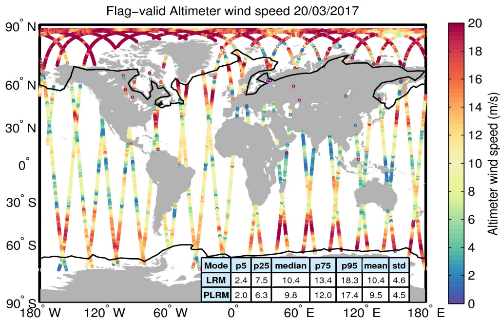
Figure 31. Geographical distribution of flag-valid wind data over oceans and lakes for 20/03/2017. The statistical values shown in the table refer to the wind in m/s and are calculated separately for LRM and PLRM regions. Measurements taken over polar polygons have been excluded from the computation of the statistical values. The black lines mark the outer limit of the Arctic and Antarctic polar polygons.
