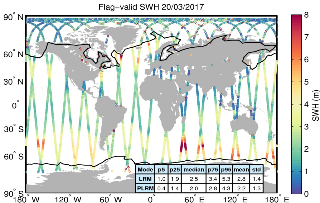
Figure 15. Geographical distribution of flag-valid SWH data over oceans and lakes for 20/03/2017. The statistical values shown in the table refer to the SWH in m and are calculated separately for LRM and PLRM regions. Measurements taken over polar polygons have been excluded from the computation of the statistical values. The black lines mark the outer limit of the Arctic and Antarctic polar polygons.
