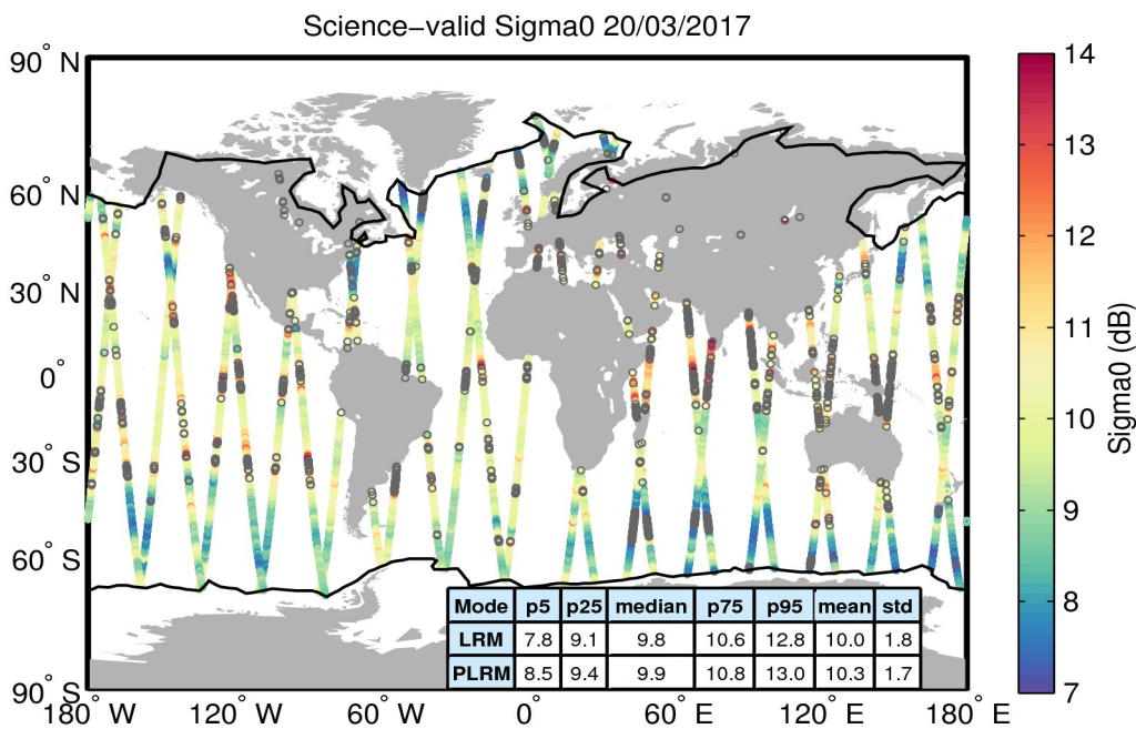
Figure 27. Geographical distribution of science-valid sigma0 data over oceans and lakes for 20/03/2017. The statistical values shown in the table refer to the sigma0 in dB and are calculated separately for LRM and PLRM regions. The black lines mark the outer limit of the Arctic and Antarctic polar polygons. Gray circles denote records that have been rejected based on the editing criteria described in Table 4.
