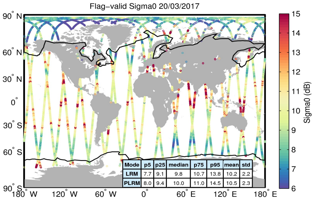
Figure 23. Geographical distribution of flag-valid sigma0 data over oceans and lakes for 20/03/2017. The statistical values shown in the table refer to the sigma0 in dB and are calculated separately for LRM and PLRM regions. Measurements taken over polar polygons have been excluded from the computation of the statistical values. The black lines mark the outer limit of the Arctic and Antarctic polar polygons.
