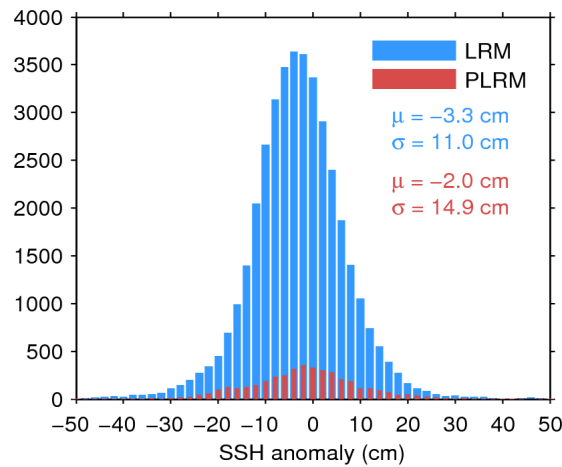
Figure 11. Histogram of science-valid SSH anomaly over oceans and lakes for LRM (blue) and PLRM (red) for 20/03/2017. The mean ( \mu ) and standard deviation ( \sigma ) are also shown. Note that values outside [-50\ 50] cm are excluded from the histogram for the sake of readability but not from the computation of \mu and \sigma .
