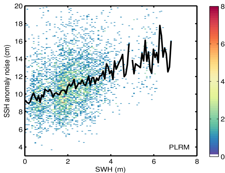
Figure 9. 2D histogram showing flag-valid SSH anomaly noise as a function of SWH for LRM (top) and PLRM (bottom) for 20/03/2017. The black line denotes the median SSH anomaly noise as a function of SWH.
