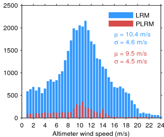
Figure 35. Histogram of science-valid wind over oceans and lakes for LRM (blue) and PLRM (red) for 20/03/2017. The mean ( \mu ) and standard deviation ( \sigma ) are also shown. Note that values larger than 24 m/s are excluded from the histogram for the sake of readability but not from the computation of \mu and \sigma .
