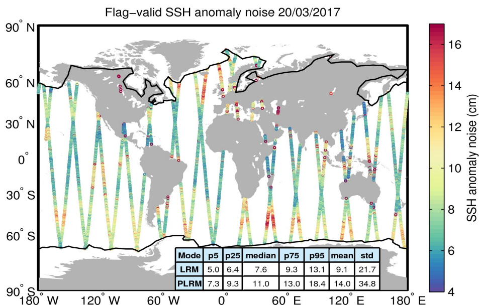
Figure 8. Geographical distribution of flag-valid 20-Hz SSH anomaly measurement noise over oceans and lakes for 20/03/2017. The statistical values shown in the table refer to the SSH anomaly noise and are calculated separately for LRM and PLRM regions. Measurements taken over polar polygons have been excluded from the computation of the statistical values. The black lines mark the outer limit of the Arctic and Antarctic polar polygons.
