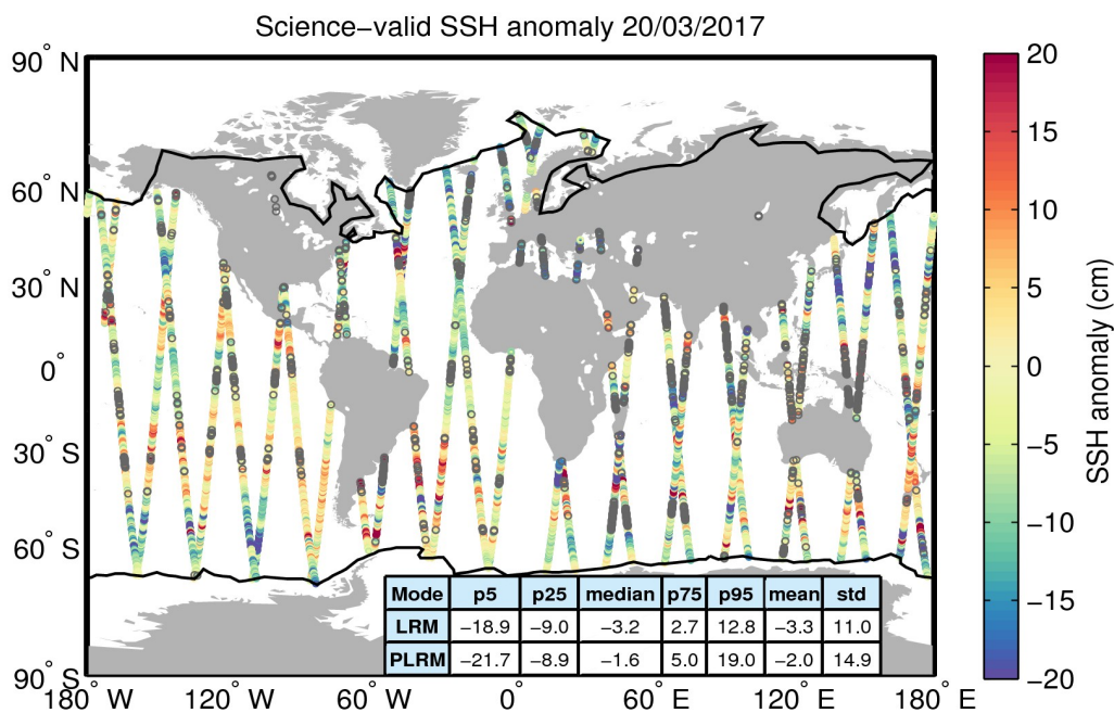
Figure 10. Geographical distribution of science-valid SSH anomaly data over oceans and lakes for 20/03/2017. The statistical values shown in the table refer to the SSH anomaly in cm and are calculated separately for LRM and PLRM regions. The black lines mark the outer limit of the Arctic and Antarctic polar polygons. Gray circles denote records that have been rejected based on the editing criteria described in Table 2.
