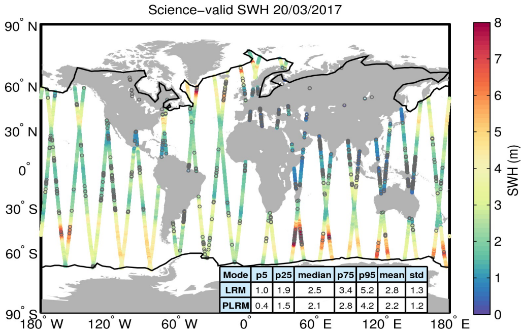
Figure 19. Geographical distribution of science-valid SWH data over oceans and lakes for 20/03/2017. The statistical values shown in the table refer to the SWH in m and are calculated separately for LRM and PLRM regions. The black lines mark the outer limit of the Arctic and Antarctic polar polygons. Gray circles denote records that have been rejected based on the editing criteria described in Table 3.
