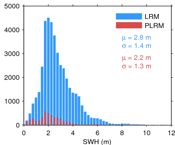
Figure 17. Histogram of flag-valid SWH over oceans and lakes for LRM (blue) and PLRM (red) for 20/03/2017. The mean ( \mu ) and standard deviation ( \sigma ) are also shown. Note that values larger than 12 m are excluded from the histogram for the sake of readability but not from the computation of \mu and \sigma .
