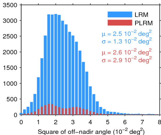
Figure 39. Histogram of flag-valid mispointing over oceans and lakes for LRM (blue) and PLRM (red) for 20/03/2017. Only positive values have been considered. The mean ( \mu ) and standard deviation ( \sigma ) are also shown. Note that values larger than 8 \cdot 10^{-2} \text{ deg}^2 are excluded from the histogram for the sake of readability but not from the computation of \mu and \sigma .
