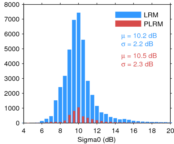
Figure 25. Histogram of flag-valid sigma0 over oceans and lakes for LRM (blue) and PLRM (red) for 20/03/2017. The mean ( \mu ) and standard deviation ( \sigma ) are also shown. Note that values outside [4 20] dB are excluded from the histogram for the sake of readability but not from the computation of \mu and \sigma .
