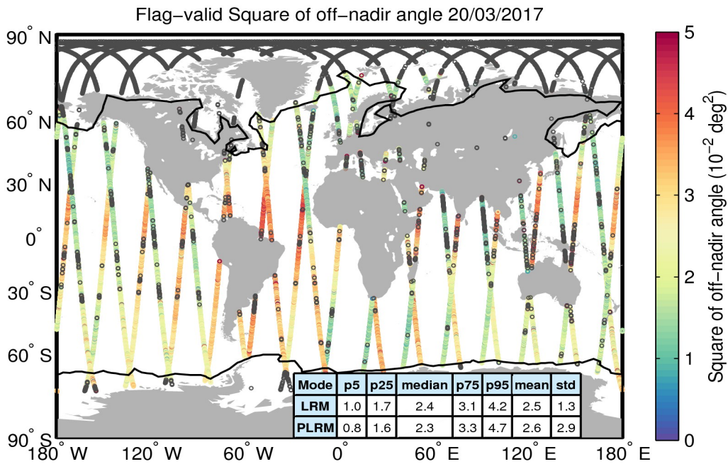
Figure 37. Geographical distribution of flag-valid mispointing data over oceans and lakes for 20/03/2017. The statistical values shown in the table refer to the mispointing in 10^{-2} deg 2 and are calculated separately for LRM and PLRM regions. Measurements taken over polar polygons have been excluded from the computation of the statistical values. The black lines mark the outer limit of the Arctic and Antarctic polar polygons. Gray circles denote negative values.
