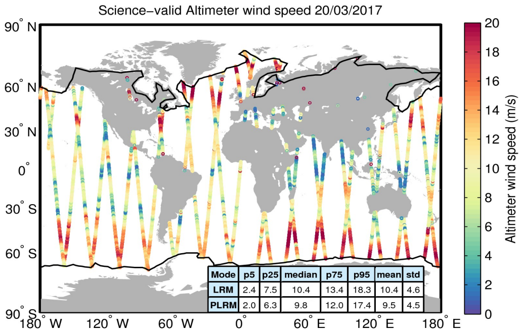
Figure 34. Geographical distribution of science-valid wind data over oceans and lakes for 20/03/2017. The statistical values shown in the table refer to the wind in m/s and are calculated separately for LRM and PLRM regions. The black lines mark the outer limit of the Arctic and Antarctic polar polygons. Gray circles denote records that have been rejected based on the editing criteria described in Table 5.
