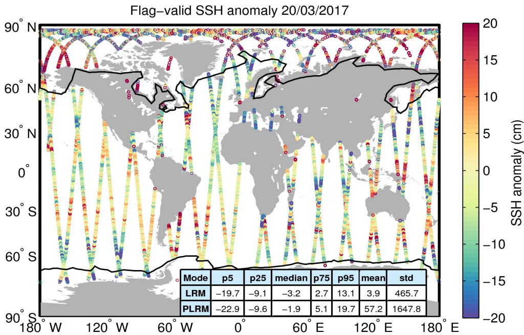
Figure 5. Geographical distribution of flag-valid 1-Hz SSH anomaly data over oceans and lakes for 20/03/2017. The statistical values shown in the table refer to the SSH anomaly in cm and are calculated separately for LRM and PLRM regions. Measurements taken over polar polygons have been excluded from the computation of the statistical values. The black lines mark the outer limit of the Arctic and Antarctic polar polygons.
