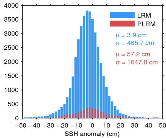
Figure 7. Histogram of flag-valid SSH anomaly over oceans and lakes for LRM (blue) and PLRM (red) for 20/03/2017. The mean ( \mu ) and standard deviation ( \sigma ) are also shown. Note that values outside [-50 50] cm are excluded from the histogram for the sake of readability but not from the computation of \mu and \sigma .
