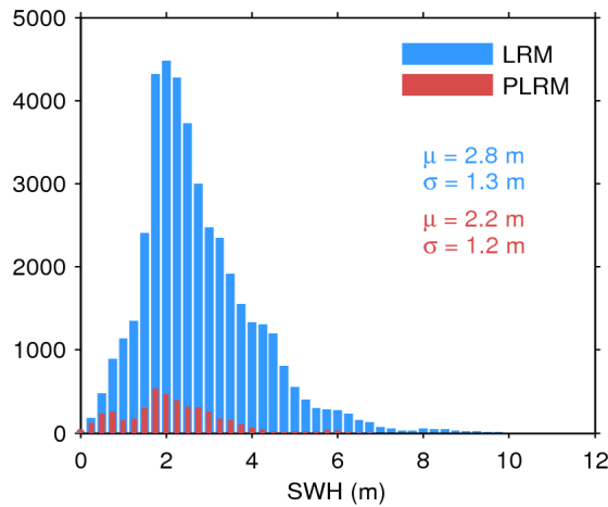
Figure 20. Histogram of science-valid SWH over oceans and lakes for LRM (blue) and PLRM (red) for 20/03/2017. The mean ( \mu ) and standard deviation ( \sigma ) are also shown. Note that values larger than 12 m are excluded from the histogram for the sake of readability but not from the computation of \mu and \sigma .
