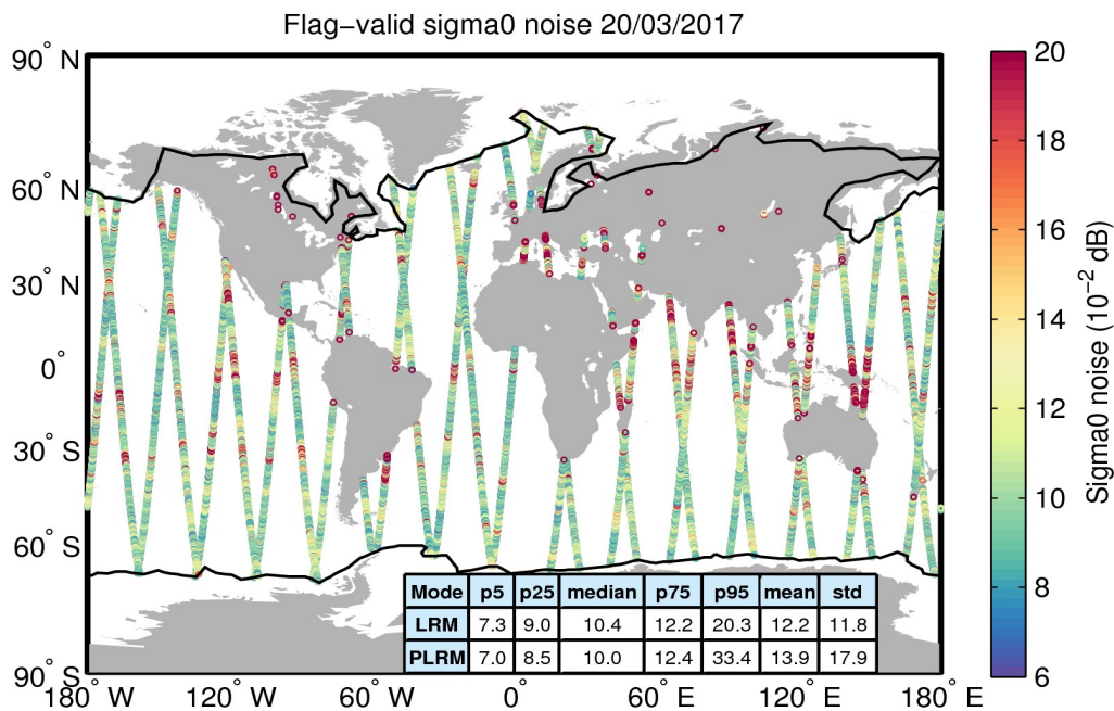
Figure 26. Geographical distribution of flag-valid 20-Hz sigma0 measurement noise over oceans and lakes for 20/03/2017. The statistical values shown in the table refer to the sigma0 noise and are calculated separately for LRM and PLRM regions. Measurements taken over polar polygons have been excluded from the computation of the statistical values. The black lines mark the outer limit of the Arctic and Antarctic polar polygons.
