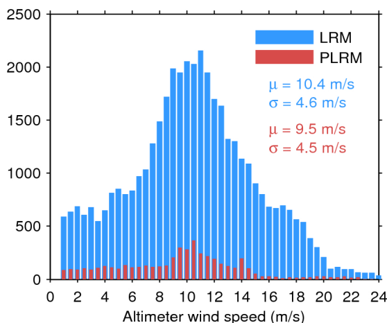
Figure 33. Histogram of flag-valid wind over oceans and lakes for LRM (blue) and PLRM (red) for 20/03/2017. The mean ( \mu ) and standard deviation ( \sigma ) are also shown. Note that values larger than 24 m/s are excluded from the histogram for the sake of readability but not from the computation of \mu and \sigma .
