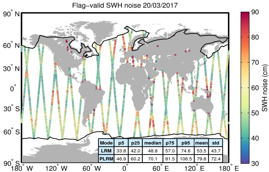
Figure 18. Geographical distribution of flag-valid 20-Hz SWH measurement noise over oceans and lakes for 20/03/2017. The statistical values shown in the table refer to the SWH noise and are calculated separately for LRM and PLRM regions. Measurements taken over polar polygons have been excluded from the computation of the statistical values. The black lines mark the outer limit of the Arctic and Antarctic polar polygons.
