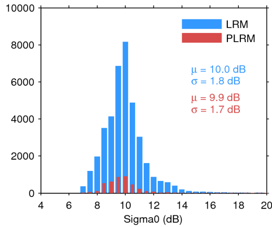
Figure 28. Histogram of science-valid sigma0 over oceans and lakes for LRM (blue) and PLRM (red) for 18/03/2017. The mean ( \mu ) and standard deviation ( \sigma ) are also shown. Note that values outside [4 20] dB are excluded from the histogram for the sake of readability but not from the computation of \mu and \sigma .
