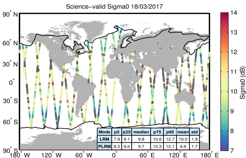
Figure 27. Geographical distribution of science-valid sigma0 data over oceans and lakes for 18/03/2017. The statistical values shown in the table refer to the sigma0 in dB and are calculated separately for LRM and PLRM regions. The black lines mark the outer limit of the Arctic and Antarctic polar polygons. Gray circles denote records that have been rejected based on the editing criteria described in Table 4.
