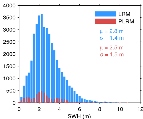
Figure 17. Histogram of flag-valid SWH over oceans and lakes for LRM (blue) and PLRM (red) for 18/03/2017. The mean ( \mu ) and standard deviation ( \sigma ) are also shown. Note that values larger than 12 m are excluded from the histogram for the sake of readability but not from the computation of \mu and \sigma .
