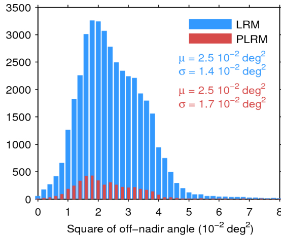
Figure 39. Histogram of flag-valid mispointing over oceans and lakes for LRM (blue) and PLRM (red) for 18/03/2017. Only positive values have been considered. The mean ( \mu ) and standard deviation ( \sigma ) are also shown. Note that values larger than 8 \cdot 10^{-2} \text{ deg}^2 are excluded from the histogram for the sake of readability but not from the computation of \mu and \sigma .
