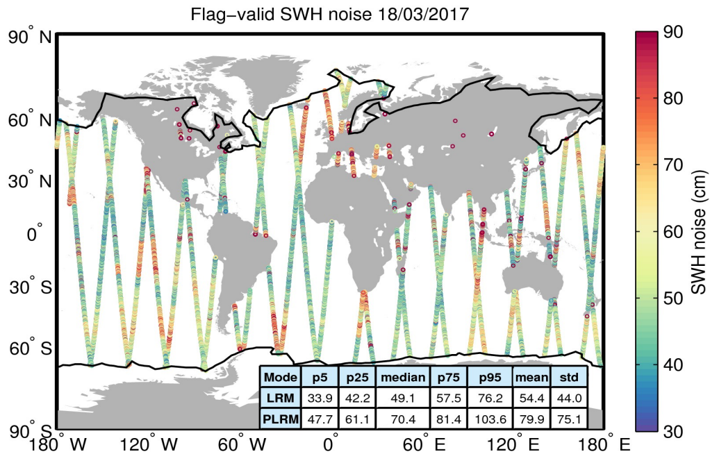
Figure 18. Geographical distribution of flag-valid 20-Hz SWH measurement noise over oceans and lakes for 18/03/2017. The statistical values shown in the table refer to the SWH noise and are calculated separately for LRM and PLRM regions. Measurements taken over polar polygons have been excluded from the computation of the statistical values. The black lines mark the outer limit of the Arctic and Antarctic polar polygons.
