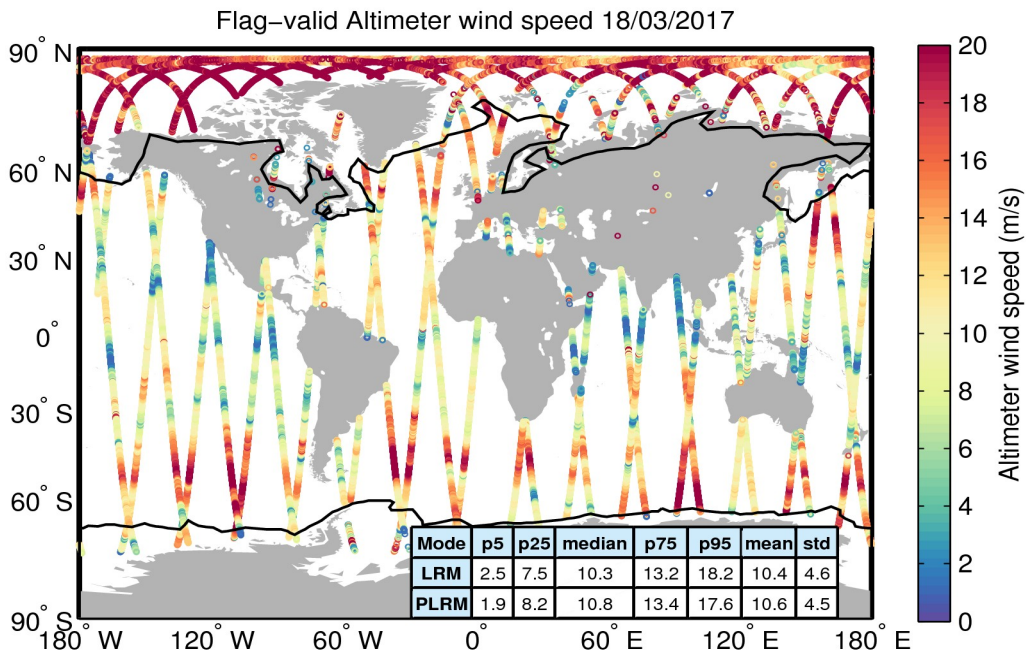
Figure 31. Geographical distribution of flag-valid wind data over oceans and lakes for 18/03/2017. The statistical values shown in the table refer to the wind in m/s and are calculated separately for LRM and PLRM regions. Measurements taken over polar polygons have been excluded from the computation of the statistical values. The black lines mark the outer limit of the Arctic and Antarctic polar polygons.
