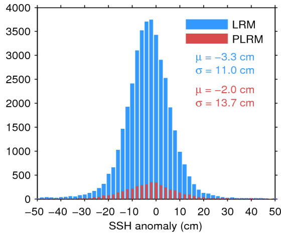
Figure 11. Histogram of science-valid SSH anomaly over oceans and lakes for LRM (blue) and PLRM (red) for 18/03/2017. The mean ( \mu ) and standard deviation ( \sigma ) are also shown. Note that values outside [-50 50] cm are excluded from the histogram for the sake of readability but not from the computation of \mu and \sigma .
