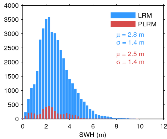
Figure 20. Histogram of science-valid SWH over oceans and lakes for LRM (blue) and PLRM (red) for 18/03/2017. The mean ( \mu ) and standard deviation ( \sigma ) are also shown. Note that values larger than 12 m are excluded from the histogram for the sake of readability but not from the computation of \mu and \sigma .
