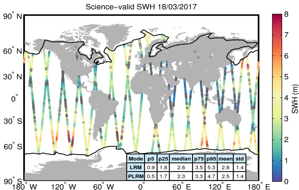
Figure 19. Geographical distribution of science-valid SWH data over oceans and lakes for 18/03/2017. The statistical values shown in the table refer to the SWH in m and are calculated separately for LRM and PLRM regions. The black lines mark the outer limit of the Arctic and Antarctic polar polygons. Gray circles denote records that have been rejected based on the editing criteria described in Table 3.
