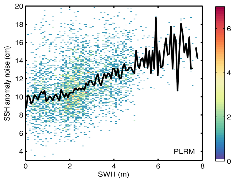
Figure 9. 2D histogram showing flag-valid SSH anomaly noise as a function of SWH for LRM (top) and PLRM (bottom) for 18/03/2017. The black line denotes the median SSH anomaly noise as a function of SWH.
