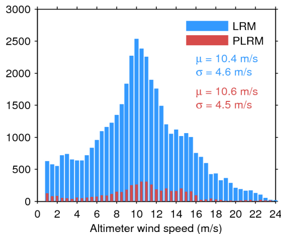
Figure 35. Histogram of science-valid wind over oceans and lakes for LRM (blue) and PLRM (red) for 18/03/2017. The mean ( \mu ) and standard deviation ( \sigma ) are also shown. Note that values larger than 24 m/s are excluded from the histogram for the sake of readability but not from the computation of \mu and \sigma .
