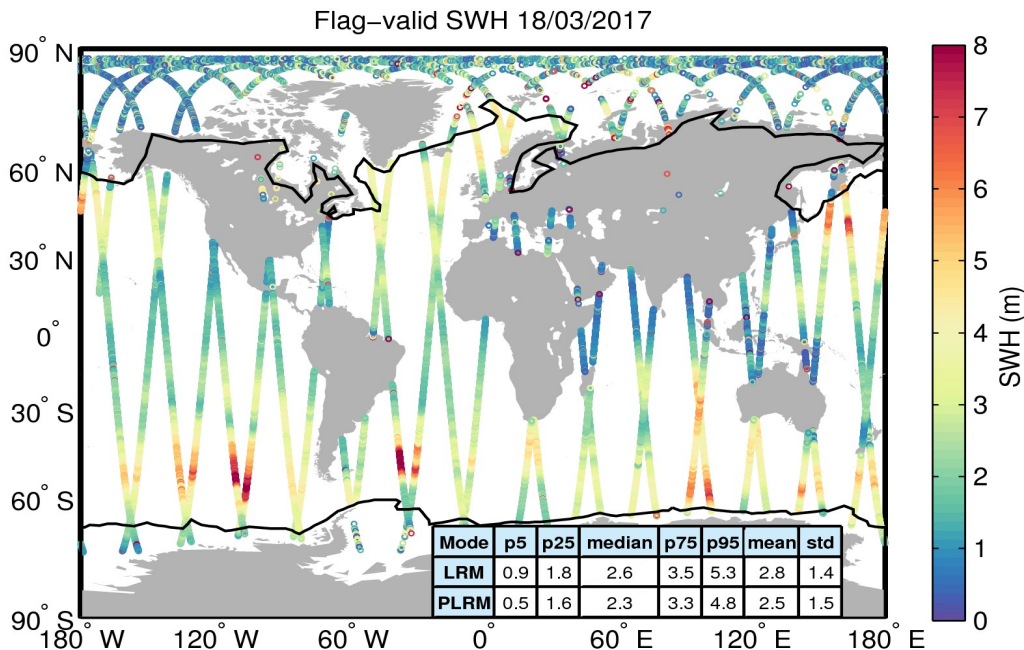
Figure 15. Geographical distribution of flag-valid SWH data over oceans and lakes for 18/03/2017. The statistical values shown in the table refer to the SWH in m and are calculated separately for LRM and PLRM regions. Measurements taken over polar polygons have been excluded from the computation of the statistical values. The black lines mark the outer limit of the Arctic and Antarctic polar polygons.
