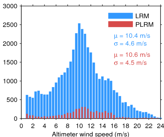
Figure 33. Histogram of flag-valid wind over oceans and lakes for LRM (blue) and PLRM (red) for 18/03/2017. The mean ( \mu ) and standard deviation ( \sigma ) are also shown. Note that values larger than 24 m/s are excluded from the histogram for the sake of readability but not from the computation of \mu and \sigma .
