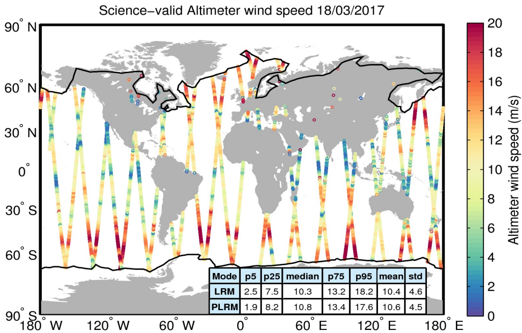
Figure 34. Geographical distribution of science-valid wind data over oceans and lakes for 18/03/2017. The statistical values shown in the table refer to the wind in m/s and are calculated separately for LRM and PLRM regions. The black lines mark the outer limit of the Arctic and Antarctic polar polygons. Gray circles denote records that have been rejected based on the editing criteria described in Table 5.
