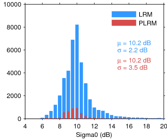
Figure 25. Histogram of flag-valid sigma0 over oceans and lakes for LRM (blue) and PLRM (red) for 18/03/2017. The mean ( \mu ) and standard deviation ( \sigma ) are also shown. Note that values outside [4 20] dB are excluded from the histogram for the sake of readability but not from the computation of \mu and \sigma .
