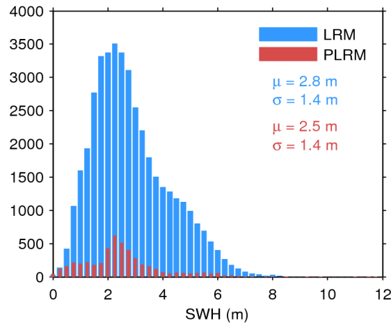
Figure 17. Histogram of flag-valid SWH over oceans and lakes for LRM (blue) and PLRM (red) for 17/03/2017. The mean ( \mu ) and standard deviation ( \sigma ) are also shown. Note that values larger than 12 m are excluded from the histogram for the sake of readability but not from the computation of \mu and \sigma .
