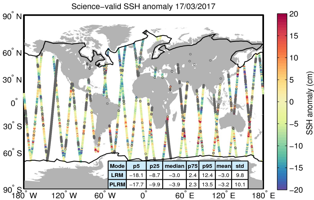
Figure 10. Geographical distribution of science-valid SSH anomaly data over oceans and lakes for 17/03/2017. The statistical values shown in the table refer to the SSH anomaly in cm and are calculated separately for LRM and PLRM regions. The black lines mark the outer limit of the Arctic and Antarctic polar polygons. Gray circles denote records that have been rejected based on the editing criteria described in Table 2.
