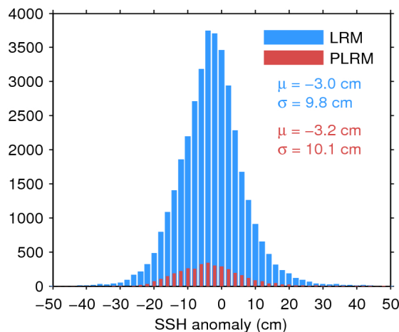
Figure 11. Histogram of science-valid SSH anomaly over oceans and lakes for LRM (blue) and PLRM (red) for 17/03/2017. The mean ( \mu ) and standard deviation ( \sigma ) are also shown. Note that values outside [-50 50] cm are excluded from the histogram for the sake of readability but not from the computation of \mu and \sigma .
