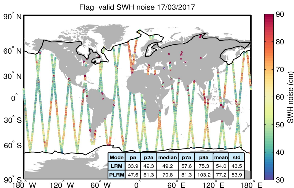
Figure 18. Geographical distribution of flag-valid 20-Hz SWH measurement noise over oceans and lakes for 17/03/2017. The statistical values shown in the table refer to the SWH noise and are calculated separately for LRM and PLRM regions. Measurements taken over polar polygons have been excluded from the computation of the statistical values. The black lines mark the outer limit of the Arctic and Antarctic polar polygons.
