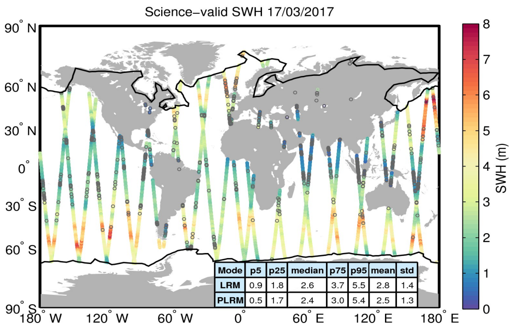
Figure 19. Geographical distribution of science-valid SWH data over oceans and lakes for 17/03/2017. The statistical values shown in the table refer to the SWH in m and are calculated separately for LRM and PLRM regions. The black lines mark the outer limit of the Arctic and Antarctic polar polygons. Gray circles denote records that have been rejected based on the editing criteria described in Table 3.
