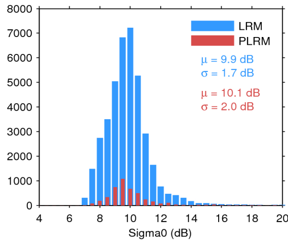
Figure 28. Histogram of science-valid sigma0 over oceans and lakes for LRM (blue) and PLRM (red) for 17/03/2017. The mean ( \mu ) and standard deviation ( \sigma ) are also shown. Note that values outside [4 20] dB are excluded from the histogram for the sake of readability but not from the computation of \mu and \sigma .
