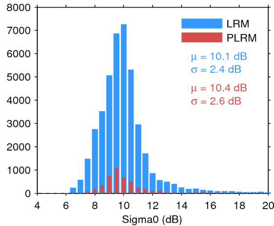
Figure 25. Histogram of flag-valid sigma0 over oceans and lakes for LRM (blue) and PLRM (red) for 17/03/2017. The mean ( \mu ) and standard deviation ( \sigma ) are also shown. Note that values outside [4 20] dB are excluded from the histogram for the sake of readability but not from the computation of \mu and \sigma .
