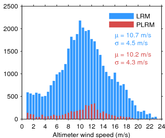
Figure 35. Histogram of science-valid wind over oceans and lakes for LRM (blue) and PLRM (red) for 17/03/2017. The mean ( \mu ) and standard deviation ( \sigma ) are also shown. Note that values larger than 24 m/s are excluded from the histogram for the sake of readability but not from the computation of \mu and \sigma .
