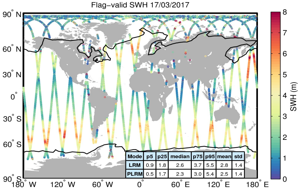
Figure 15. Geographical distribution of flag-valid SWH data over oceans and lakes for 17/03/2017. The statistical values shown in the table refer to the SWH in m and are calculated separately for LRM and PLRM regions. Measurements taken over polar polygons have been excluded from the computation of the statistical values. The black lines mark the outer limit of the Arctic and Antarctic polar polygons.
