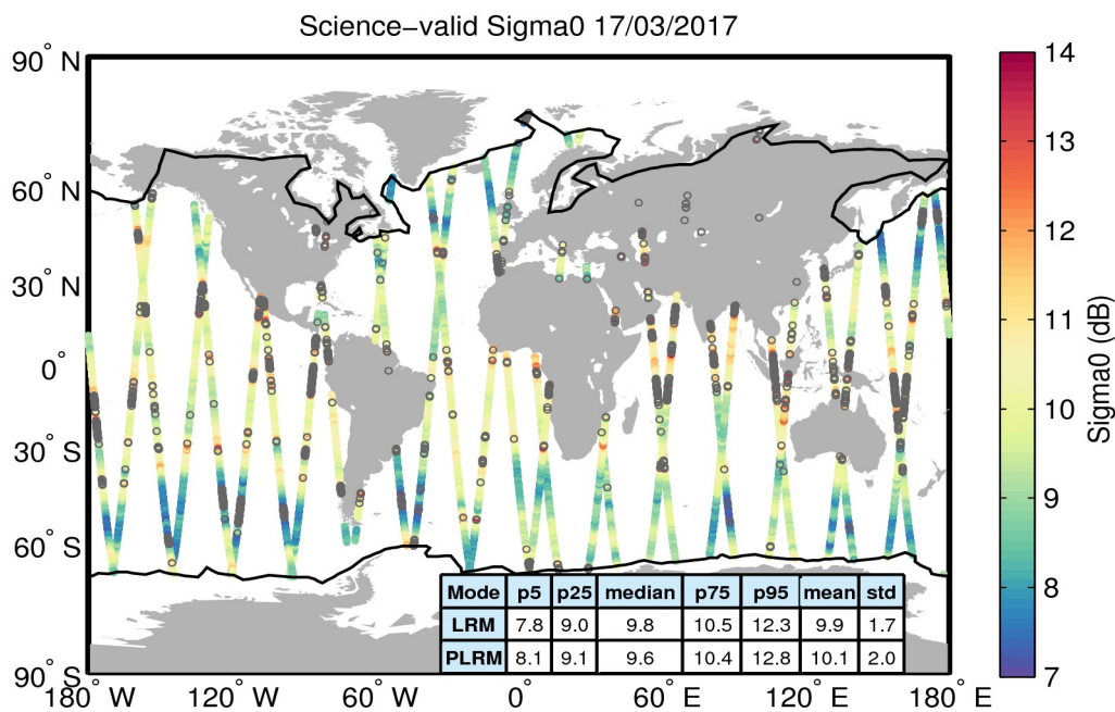
Figure 27. Geographical distribution of science-valid sigma0 data over oceans and lakes for 17/03/2017. The statistical values shown in the table refer to the sigma0 in dB and are calculated separately for LRM and PLRM regions. The black lines mark the outer limit of the Arctic and Antarctic polar polygons. Gray circles denote records that have been rejected based on the editing criteria described in Table 4.
