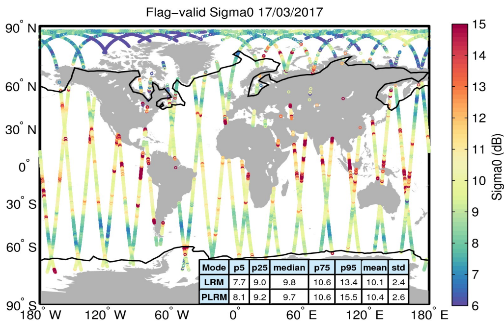
Figure 23. Geographical distribution of flag-valid sigma0 data over oceans and lakes for 17/03/2017. The statistical values shown in the table refer to the sigma0 in dB and are calculated separately for LRM and PLRM regions. Measurements taken over polar polygons have been excluded from the computation of the statistical values. The black lines mark the outer limit of the Arctic and Antarctic polar polygons.
