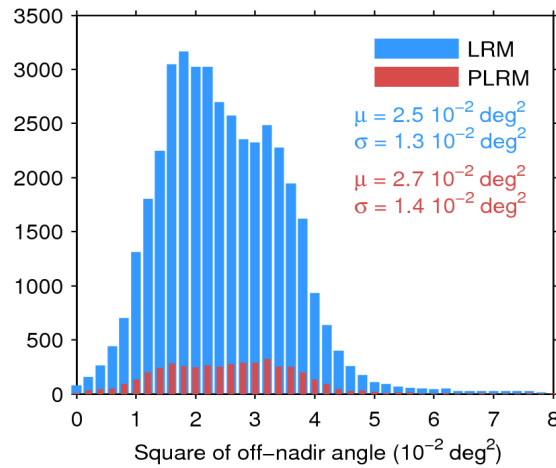
Figure 39. Histogram of flag-valid mispointing over oceans and lakes for LRM (blue) and PLRM (red) for 17/03/2017. Only positive values have been considered. The mean ( \mu ) and standard deviation ( \sigma ) are also shown. Note that values larger than 8 \cdot 10^{-2} \text{ deg}^2 are excluded from the histogram for the sake of readability but not from the computation of \mu and \sigma .
