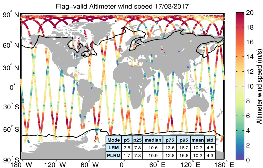
Figure 31. Geographical distribution of flag-valid wind data over oceans and lakes for 17/03/2017. The statistical values shown in the table refer to the wind in m/s and are calculated separately for LRM and PLRM regions. Measurements taken over polar polygons have been excluded from the computation of the statistical values. The black lines mark the outer limit of the Arctic and Antarctic polar polygons.
