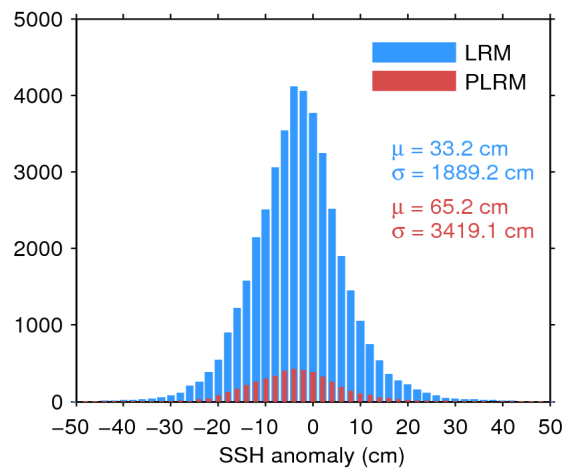
Figure 7. Histogram of flag-valid SSH anomaly over oceans and lakes for LRM (blue) and PLRM (red) for 17/03/2017. The mean ( \mu ) and standard deviation ( \sigma ) are also shown. Note that values outside [-50\ 50] cm are excluded from the histogram for the sake of readability but not from the computation of \mu and \sigma .
