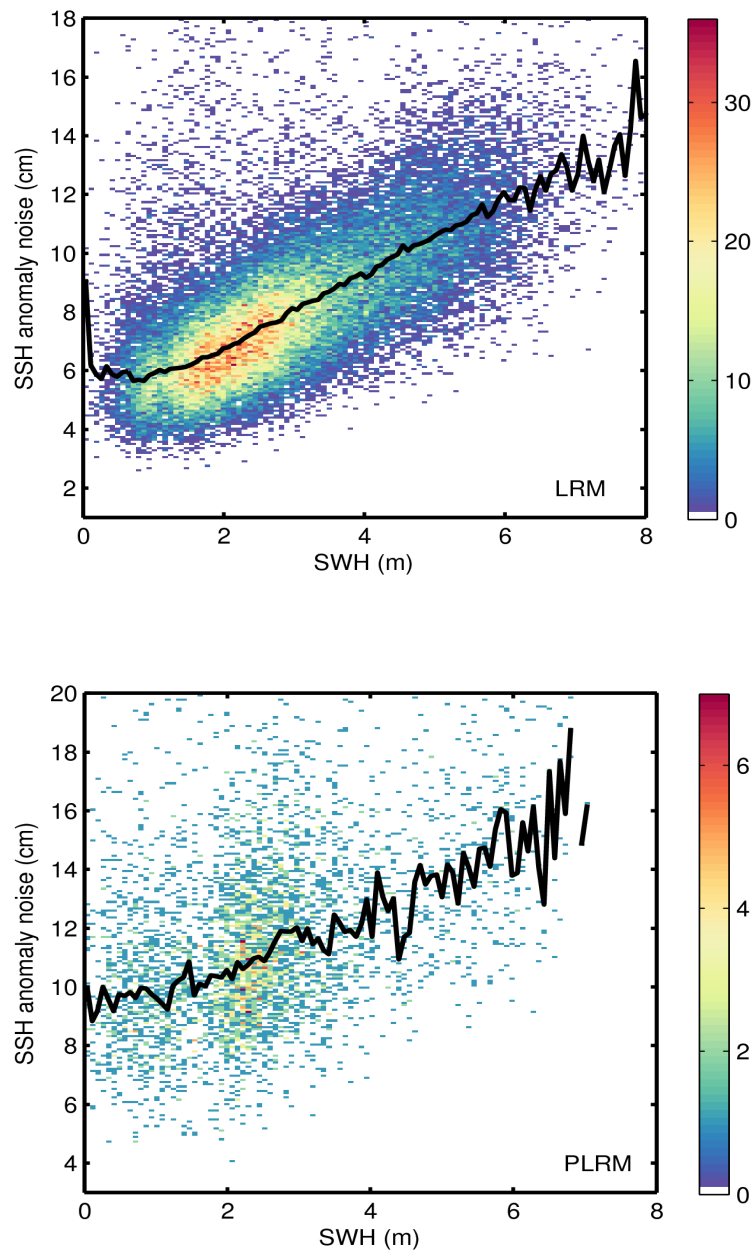
Figure 9. 2D histogram showing flag-valid SSH anomaly noise as a function of SWH for LRM (top) and PLRM (bottom) for 17/03/2017. The black line denotes the median SSH anomaly noise as a function of SWH.
