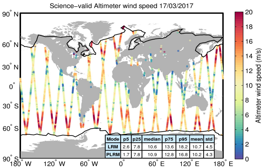
Figure 34. Geographical distribution of science-valid wind data over oceans and lakes for 17/03/2017. The statistical values shown in the table refer to the wind in m/s and are calculated separately for LRM and PLRM regions. The black lines mark the outer limit of the Arctic and Antarctic polar polygons. Gray circles denote records that have been rejected based on the editing criteria described in Table 5.
