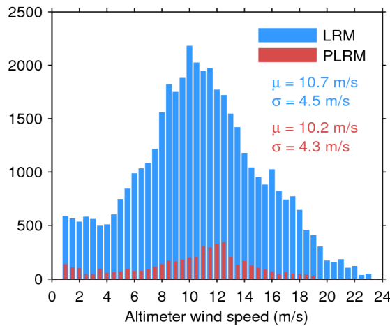
Figure 33. Histogram of flag-valid wind over oceans and lakes for LRM (blue) and PLRM (red) for 17/03/2017. The mean ( \mu ) and standard deviation ( \sigma ) are also shown. Note that values larger than 24 m/s are excluded from the histogram for the sake of readability but not from the computation of \mu and \sigma .
