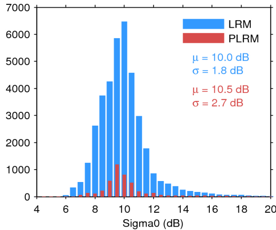
Figure 25. Histogram of flag-valid sigma0 over oceans and lakes for LRM (blue) and PLRM (red) for 16/03/2017. The mean ( \mu ) and standard deviation ( \sigma ) are also shown. Note that values outside [4 20] dB are excluded from the histogram for the sake of readability but not from the computation of \mu and \sigma .
