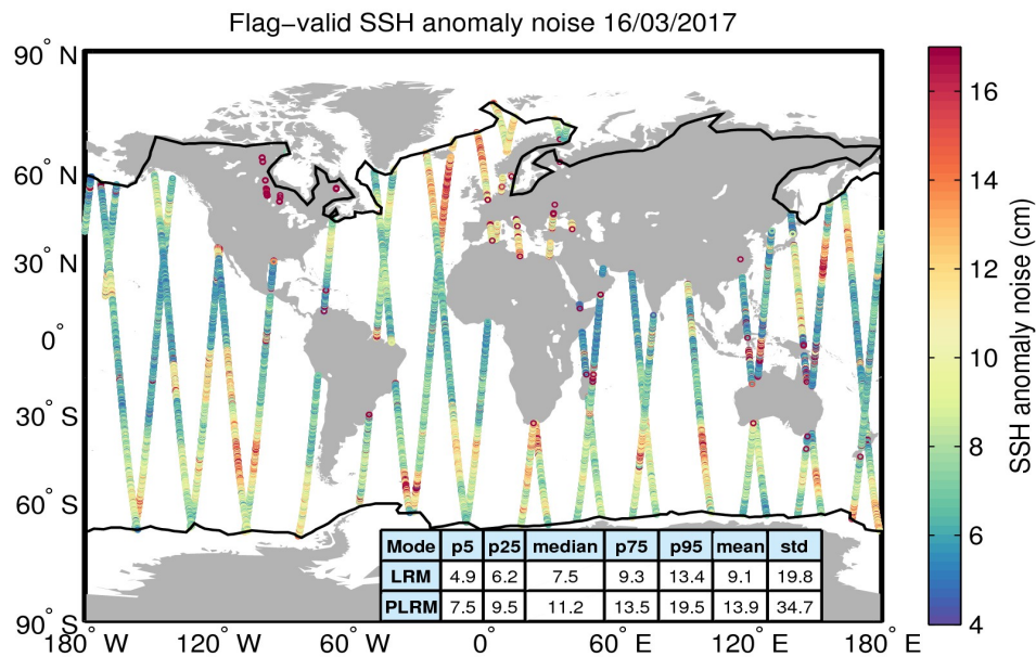
Figure 8. Geographical distribution of flag-valid 20-Hz SSH anomaly measurement noise over oceans and lakes for 16/03/2017. The statistical values shown in the table refer to the SSH anomaly noise and are calculated separately for LRM and PLRM regions. Measurements taken over polar polygons have been excluded from the computation of the statistical values. The black lines mark the outer limit of the Arctic and Antarctic polar polygons.
