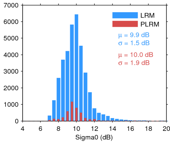
Figure 28. Histogram of science-valid sigma0 over oceans and lakes for LRM (blue) and PLRM (red) for 16/03/2017. The mean ( \mu ) and standard deviation ( \sigma ) are also shown. Note that values outside [4 20] dB are excluded from the histogram for the sake of readability but not from the computation of \mu and \sigma .
