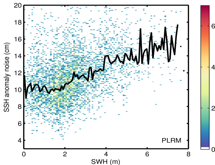
Figure 9. 2D histogram showing flag-valid SSH anomaly noise as a function of SWH for LRM (top) and PLRM (bottom) for 16/03/2017. The black line denotes the median SSH anomaly noise as a function of SWH.
