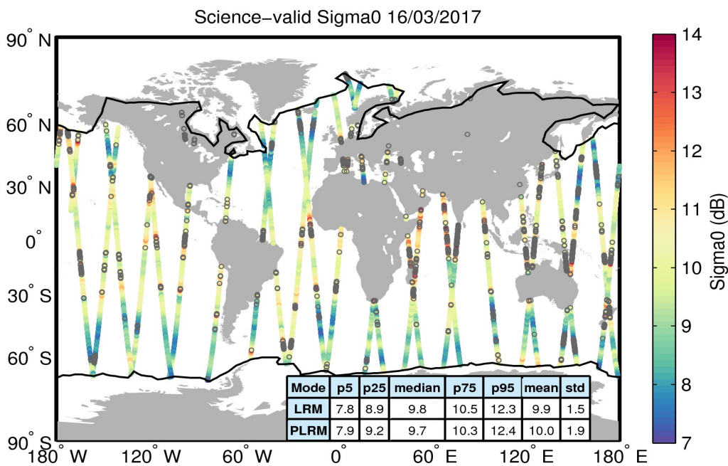
Figure 27. Geographical distribution of science-valid sigma0 data over oceans and lakes for 16/03/2017. The statistical values shown in the table refer to the sigma0 in dB and are calculated separately for LRM and PLRM regions. The black lines mark the outer limit of the Arctic and Antarctic polar polygons. Gray circles denote records that have been rejected based on the editing criteria described in Table 4.
