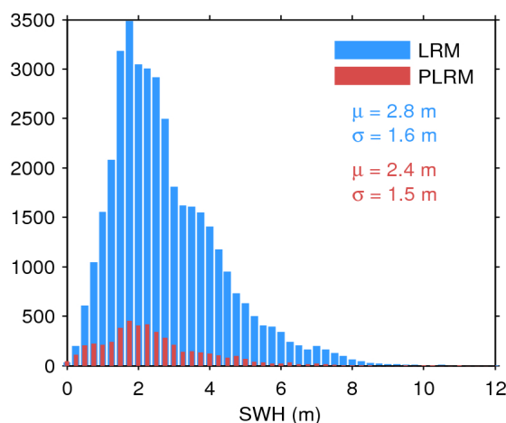
Figure 17. Histogram of flag-valid SWH over oceans and lakes for LRM (blue) and PLRM (red) for 16/03/2017. The mean ( \mu ) and standard deviation ( \sigma ) are also shown. Note that values larger than 12 m are excluded from the histogram for the sake of readability but not from the computation of \mu and \sigma .
