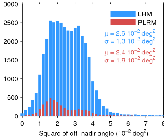
Figure 39. Histogram of flag-valid mispointing over oceans and lakes for LRM (blue) and PLRM (red) for 16/03/2017. Only positive values have been considered. The mean ( \mu ) and standard deviation ( \sigma ) are also shown. Note that values larger than 8 \cdot 10^{-2} \text{ deg}^2 are excluded from the histogram for the sake of readability but not from the computation of \mu and \sigma .
