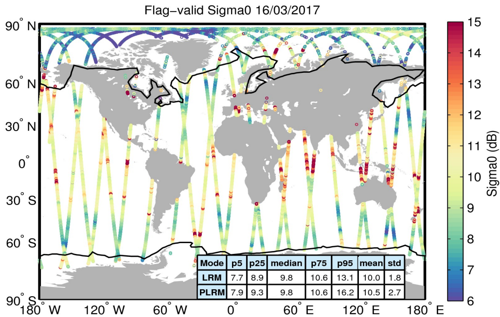
Figure 23. Geographical distribution of flag-valid sigma0 data over oceans and lakes for 16/03/2017. The statistical values shown in the table refer to the sigma0 in dB and are calculated separately for LRM and PLRM regions. Measurements taken over polar polygons have been excluded from the computation of the statistical values. The black lines mark the outer limit of the Arctic and Antarctic polar polygons.
