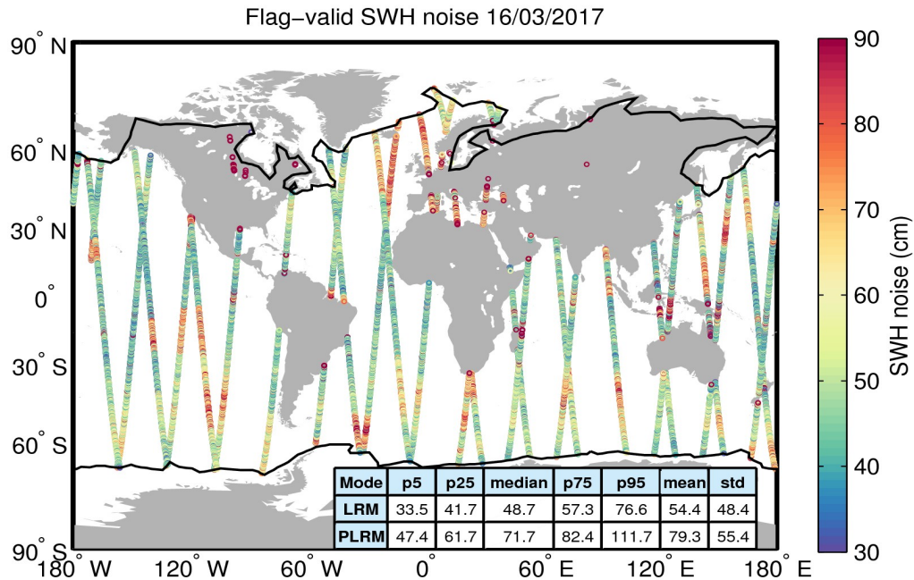
Figure 18. Geographical distribution of flag-valid 20-Hz SWH measurement noise over oceans and lakes for 16/03/2017. The statistical values shown in the table refer to the SWH noise and are calculated separately for LRM and PLRM regions. Measurements taken over polar polygons have been excluded from the computation of the statistical values. The black lines mark the outer limit of the Arctic and Antarctic polar polygons.
