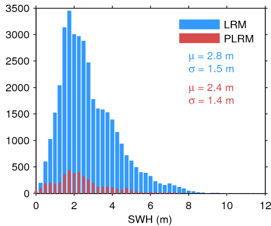
Figure 20. Histogram of science-valid SWH over oceans and lakes for LRM (blue) and PLRM (red) for 16/03/2017. The mean ( \mu ) and standard deviation ( \sigma ) are also shown. Note that values larger than 12 m are excluded from the histogram for the sake of readability but not from the computation of \mu and \sigma .
