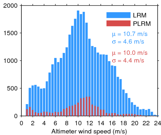
Figure 35. Histogram of science-valid wind over oceans and lakes for LRM (blue) and PLRM (red) for 16/03/2017. The mean ( \mu ) and standard deviation ( \sigma ) are also shown. Note that values larger than 24 m/s are excluded from the histogram for the sake of readability but not from the computation of \mu and \sigma .
