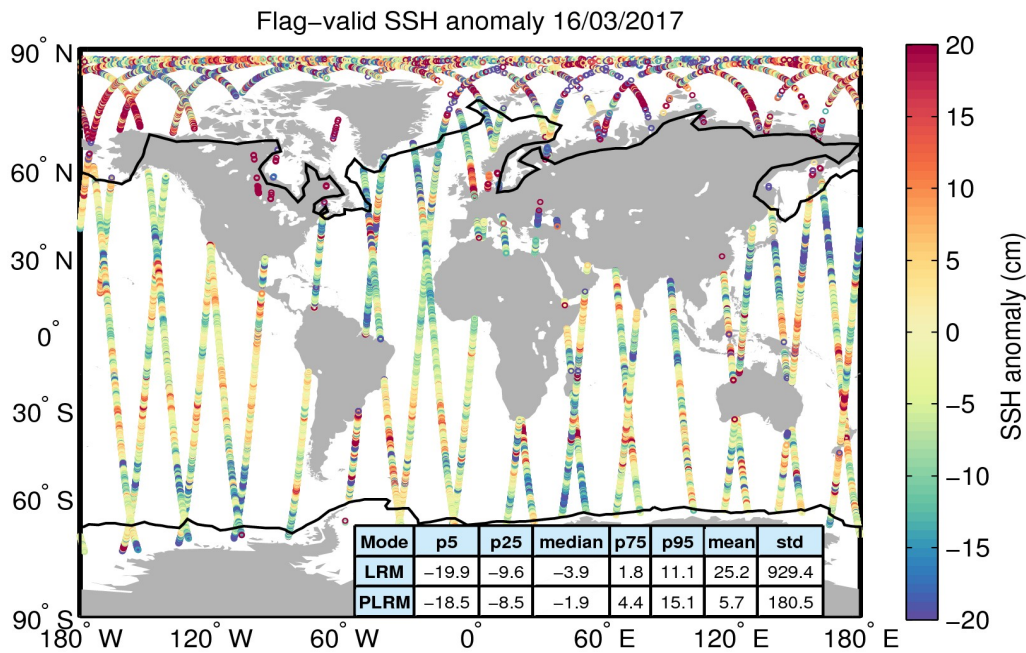
Figure 5. Geographical distribution of flag-valid 1-Hz SSH anomaly data over oceans and lakes for 16/03/2017. The statistical values shown in the table refer to the SSH anomaly in cm and are calculated separately for LRM and PLRM regions. Measurements taken over polar polygons have been excluded from the computation of the statistical values. The black lines mark the outer limit of the Arctic and Antarctic polar polygons.
