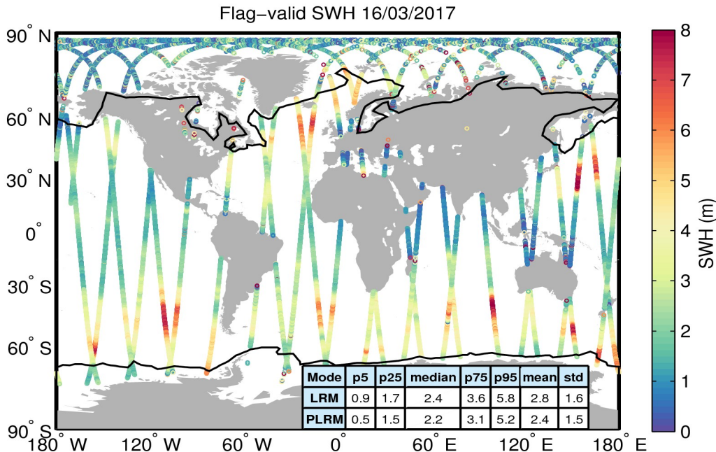
Figure 15. Geographical distribution of flag-valid SWH data over oceans and lakes for 16/03/2017. The statistical values shown in the table refer to the SWH in m and are calculated separately for LRM and PLRM regions. Measurements taken over polar polygons have been excluded from the computation of the statistical values. The black lines mark the outer limit of the Arctic and Antarctic polar polygons.
