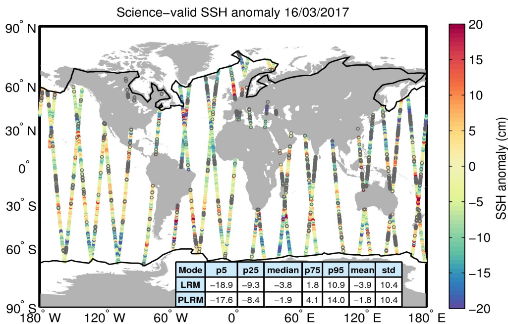
Figure 10. Geographical distribution of science-valid SSH anomaly data over oceans and lakes for 16/03/2017. The statistical values shown in the table refer to the SSH anomaly in cm and are calculated separately for LRM and PLRM regions. The black lines mark the outer limit of the Arctic and Antarctic polar polygons. Gray circles denote records that have been rejected based on the editing criteria described in Table 2.
