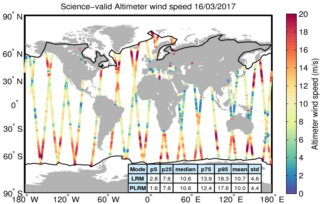
Figure 34. Geographical distribution of science-valid wind data over oceans and lakes for 16/03/2017. The statistical values shown in the table refer to the wind in m/s and are calculated separately for LRM and PLRM regions. The black lines mark the outer limit of the Arctic and Antarctic polar polygons. Gray circles denote records that have been rejected based on the editing criteria described in Table 5.
