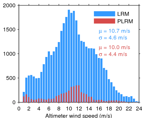
Figure 33. Histogram of flag-valid wind over oceans and lakes for LRM (blue) and PLRM (red) for 16/03/2017. The mean ( \mu ) and standard deviation ( \sigma ) are also shown. Note that values larger than 24 m/s are excluded from the histogram for the sake of readability but not from the computation of \mu and \sigma .
