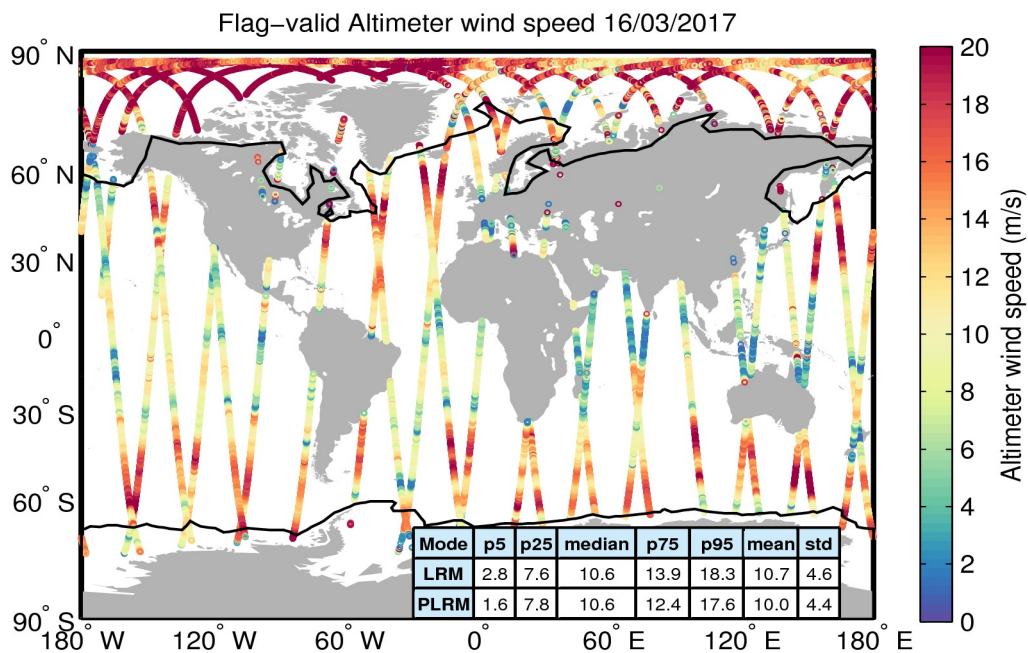
Figure 31. Geographical distribution of flag-valid wind data over oceans and lakes for 16/03/2017. The statistical values shown in the table refer to the wind in m/s and are calculated separately for LRM and PLRM regions. Measurements taken over polar polygons have been excluded from the computation of the statistical values. The black lines mark the outer limit of the Arctic and Antarctic polar polygons.
