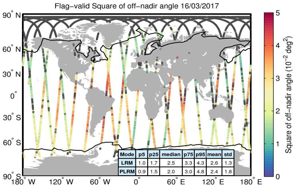
Figure 37. Geographical distribution of flag-valid mispointing data over oceans and lakes for 16/03/2017. The statistical values shown in the table refer to the mispointing in 10^{-2} deg 2 and are calculated separately for LRM and PLRM regions. Measurements taken over polar polygons have been excluded from the computation of the statistical values. The black lines mark the outer limit of the Arctic and Antarctic polar polygons. Gray circles denote negative values.
