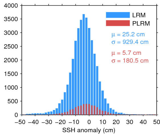
Figure 7. Histogram of flag-valid SSH anomaly over oceans and lakes for LRM (blue) and PLRM (red) for 16/03/2017. The mean ( \mu ) and standard deviation ( \sigma ) are also shown. Note that values outside [-50 50] cm are excluded from the histogram for the sake of readability but not from the computation of \mu and \sigma .
