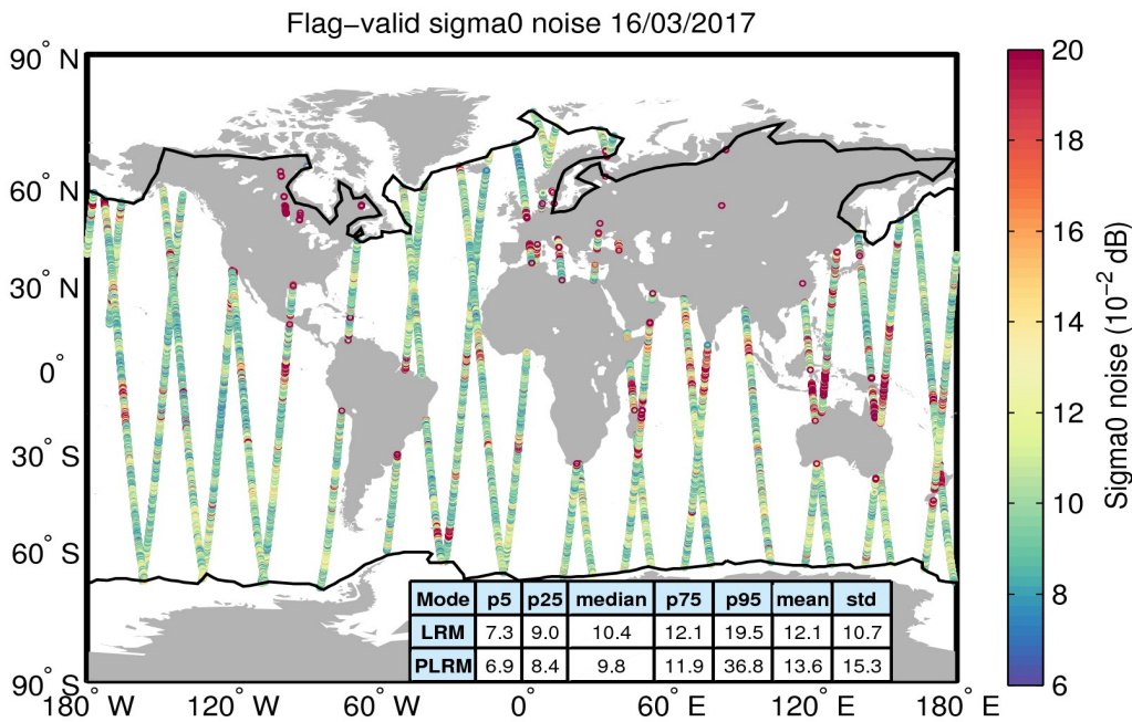
Figure 26. Geographical distribution of flag-valid 20-Hz sigma0 measurement noise over oceans and lakes for 16/03/2017. The statistical values shown in the table refer to the sigma0 noise and are calculated separately for LRM and PLRM regions. Measurements taken over polar polygons have been excluded from the computation of the statistical values. The black lines mark the outer limit of the Arctic and Antarctic polar polygons.
