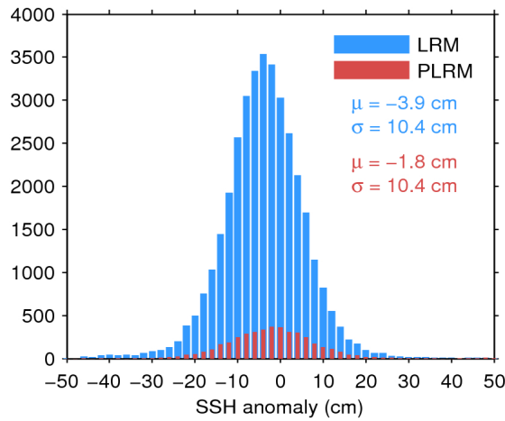
Figure 11. Histogram of science-valid SSH anomaly over oceans and lakes for LRM (blue) and PLRM (red) for 16/03/2017. The mean ( \mu ) and standard deviation ( \sigma ) are also shown. Note that values outside [-50 50] cm are excluded from the histogram for the sake of readability but not from the computation of \mu and \sigma .
