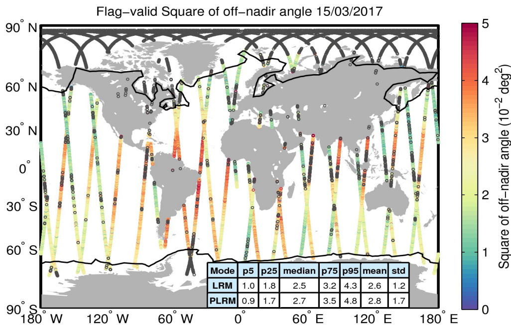
Figure 37. Geographical distribution of flag-valid mispointing data over oceans and lakes for 15/03/2017. The statistical values shown in the table refer to the mispointing in 10^{-2} deg 2 and are calculated separately for LRM and PLRM regions. Measurements taken over polar polygons have been excluded from the computation of the statistical values. The black lines mark the outer limit of the Arctic and Antarctic polar polygons. Gray circles denote negative values.
