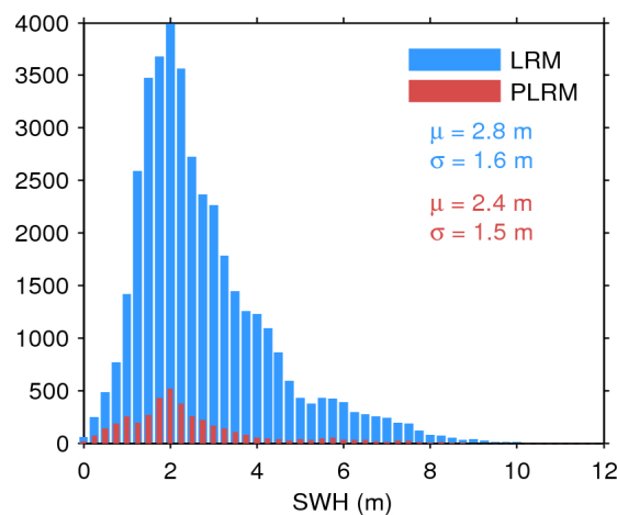
Figure 20. Histogram of science-valid SWH over oceans and lakes for LRM (blue) and PLRM (red) for 15/03/2017. The mean ( \mu ) and standard deviation ( \sigma ) are also shown. Note that values larger than 12 m are excluded from the histogram for the sake of readability but not from the computation of \mu and \sigma .
