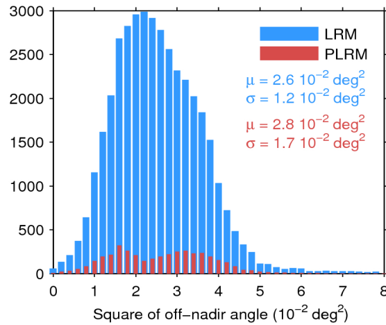
Figure 39. Histogram of flag-valid mispointing over oceans and lakes for LRM (blue) and PLRM (red) for 15/03/2017. Only positive values have been considered. The mean ( \mu ) and standard deviation ( \sigma ) are also shown. Note that values larger than 8 \cdot 10^{-2} \text{ deg}^2 are excluded from the histogram for the sake of readability but not from the computation of \mu and \sigma .
