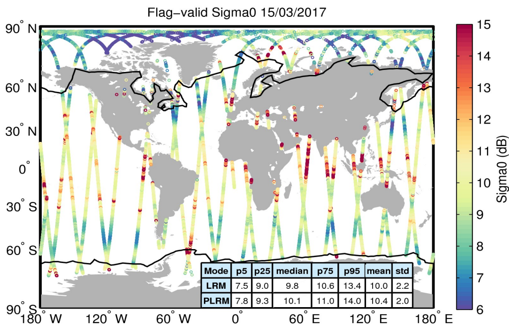
Figure 23. Geographical distribution of flag-valid sigma0 data over oceans and lakes for 15/03/2017. The statistical values shown in the table refer to the sigma0 in dB and are calculated separately for LRM and PLRM regions. Measurements taken over polar polygons have been excluded from the computation of the statistical values. The black lines mark the outer limit of the Arctic and Antarctic polar polygons.
