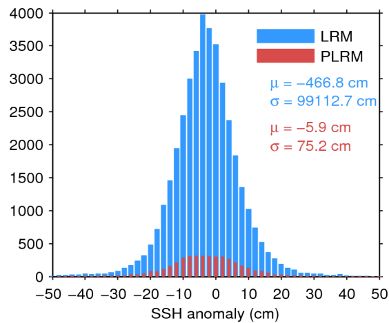
Figure 7. Histogram of flag-valid SSH anomaly over oceans and lakes for LRM (blue) and PLRM (red) for 15/03/2017. The mean ( \mu ) and standard deviation ( \sigma ) are also shown. Note that values outside [-50 \ 50] cm are excluded from the histogram for the sake of readability but not from the computation of \mu and \sigma .
