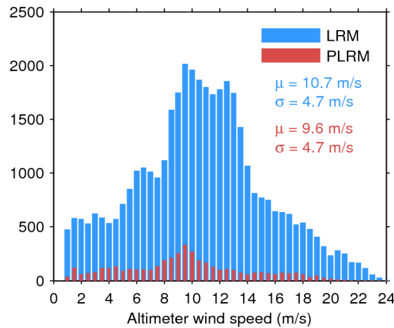
Figure 33. Histogram of flag-valid wind over oceans and lakes for LRM (blue) and PLRM (red) for 15/03/2017. The mean ( \mu ) and standard deviation ( \sigma ) are also shown. Note that values larger than 24 m/s are excluded from the histogram for the sake of readability but not from the computation of \mu and \sigma .
