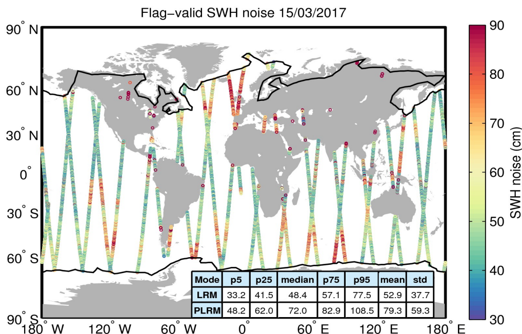
Figure 18. Geographical distribution of flag-valid 20-Hz SWH measurement noise over oceans and lakes for 15/03/2017. The statistical values shown in the table refer to the SWH noise and are calculated separately for LRM and PLRM regions. Measurements taken over polar polygons have been excluded from the computation of the statistical values. The black lines mark the outer limit of the Arctic and Antarctic polar polygons.
