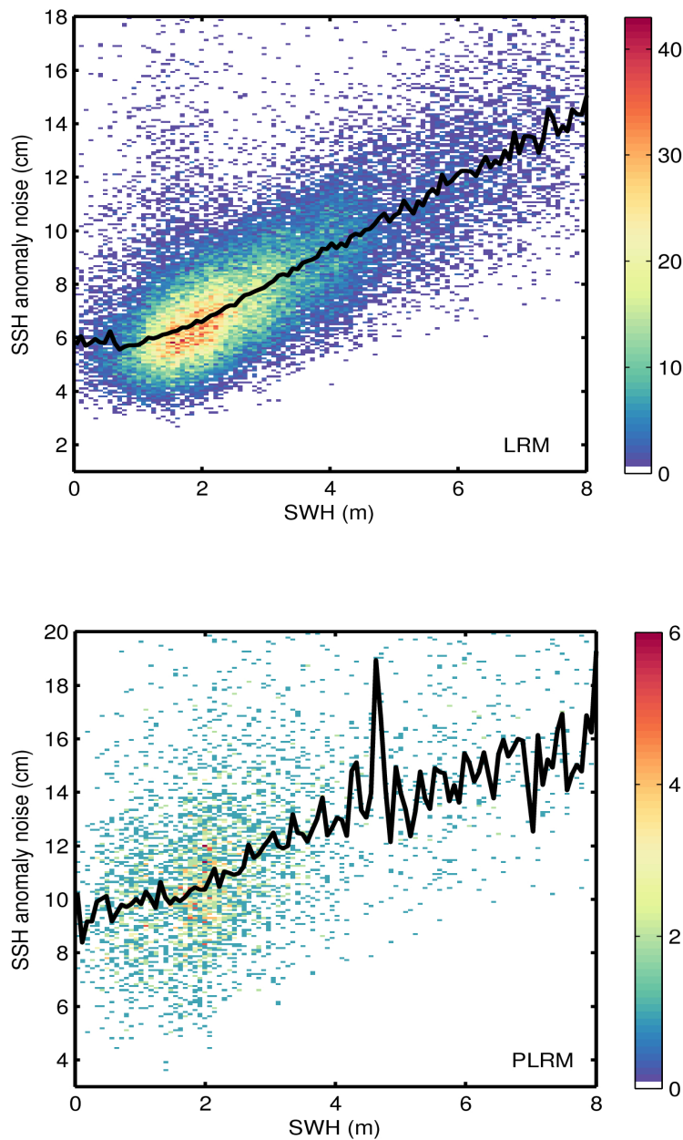
Figure 9. 2D histogram showing flag-valid SSH anomaly noise as a function of SWH for LRM (top) and PLRM (bottom) for 15/03/2017. The black line denotes the median SSH anomaly noise as a function of SWH.
