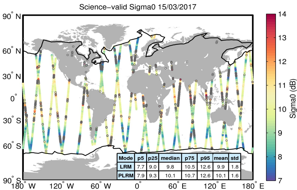
Figure 27. Geographical distribution of science-valid sigma0 data over oceans and lakes for 15/03/2017. The statistical values shown in the table refer to the sigma0 in dB and are calculated separately for LRM and PLRM regions. The black lines mark the outer limit of the Arctic and Antarctic polar polygons. Gray circles denote records that have been rejected based on the editing criteria described in Table 4.
