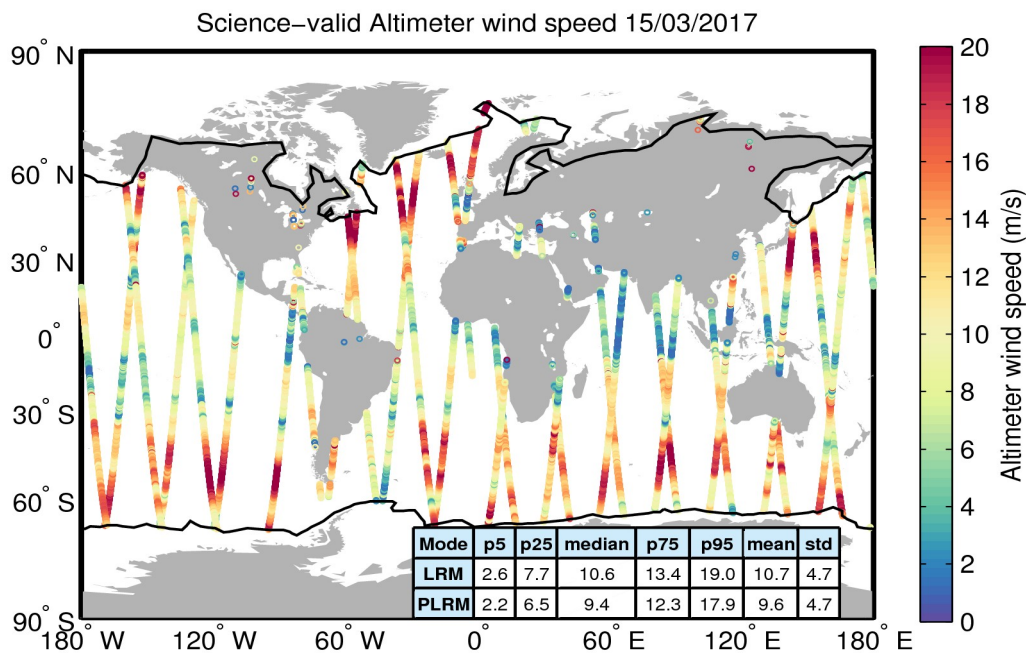
Figure 34. Geographical distribution of science-valid wind data over oceans and lakes for 15/03/2017. The statistical values shown in the table refer to the wind in m/s and are calculated separately for LRM and PLRM regions. The black lines mark the outer limit of the Arctic and Antarctic polar polygons. Gray circles denote records that have been rejected based on the editing criteria described in Table 5.
