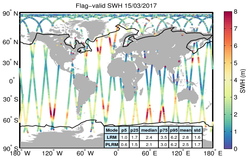
Figure 15. Geographical distribution of flag-valid SWH data over oceans and lakes for 15/03/2017. The statistical values shown in the table refer to the SWH in m and are calculated separately for LRM and PLRM regions. Measurements taken over polar polygons have been excluded from the computation of the statistical values. The black lines mark the outer limit of the Arctic and Antarctic polar polygons.
