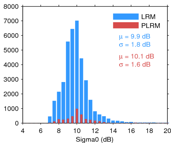
Figure 28. Histogram of science-valid sigma0 over oceans and lakes for LRM (blue) and PLRM (red) for 15/03/2017. The mean ( \mu ) and standard deviation ( \sigma ) are also shown. Note that values outside [4 20] dB are excluded from the histogram for the sake of readability but not from the computation of \mu and \sigma .
