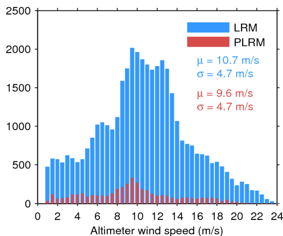
Figure 35. Histogram of science-valid wind over oceans and lakes for LRM (blue) and PLRM (red) for 15/03/2017. The mean ( \mu ) and standard deviation ( \sigma ) are also shown. Note that values larger than 24 m/s are excluded from the histogram for the sake of readability but not from the computation of \mu and \sigma .
