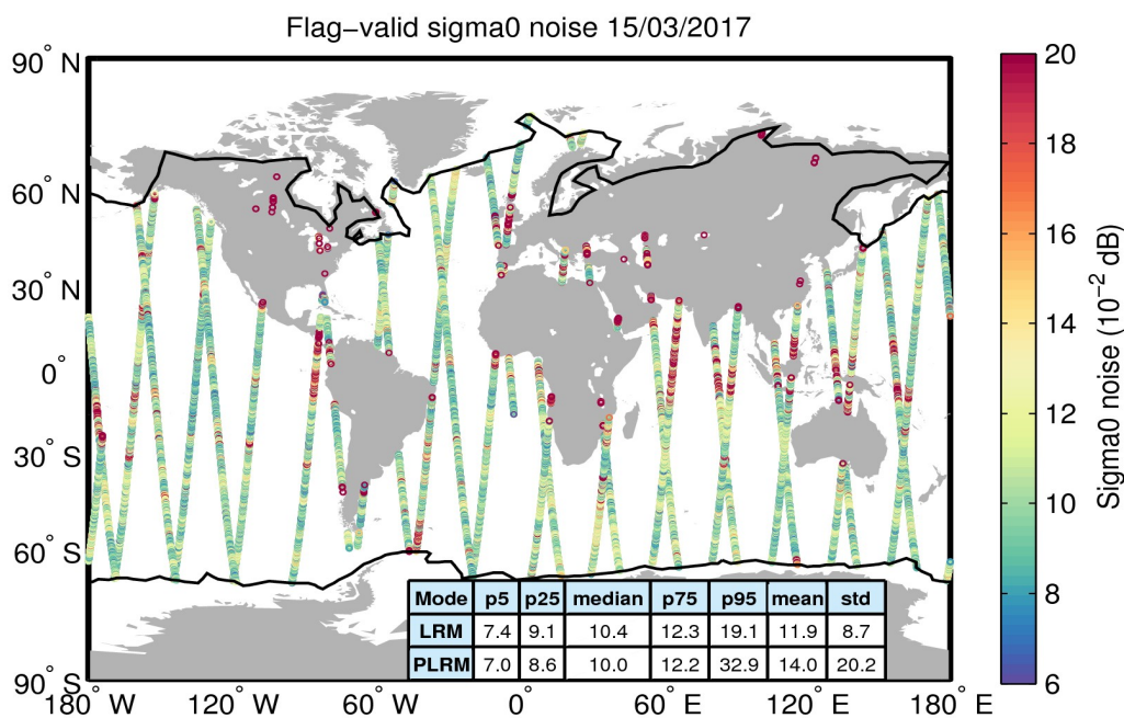
Figure 26. Geographical distribution of flag-valid 20-Hz sigma0 measurement noise over oceans and lakes for 15/03/2017. The statistical values shown in the table refer to the sigma0 noise and are calculated separately for LRM and PLRM regions. Measurements taken over polar polygons have been excluded from the computation of the statistical values. The black lines mark the outer limit of the Arctic and Antarctic polar polygons.
