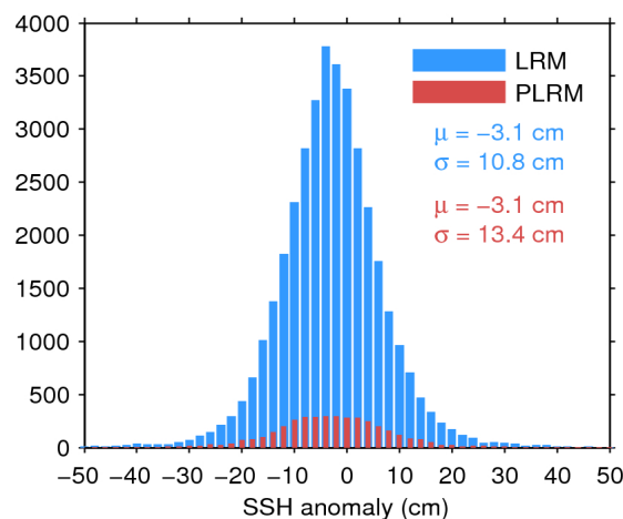
Figure 11. Histogram of science-valid SSH anomaly over oceans and lakes for LRM (blue) and PLRM (red) for 15/03/2017. The mean ( \mu ) and standard deviation ( \sigma ) are also shown. Note that values outside [-50 50] cm are excluded from the histogram for the sake of readability but not from the computation of \mu and \sigma .
