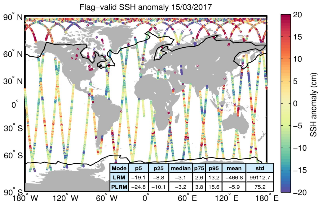
Figure 5. Geographical distribution of flag-valid 1-Hz SSH anomaly data over oceans and lakes for 15/03/2017. The statistical values shown in the table refer to the SSH anomaly in cm and are calculated separately for LRM and PLRM regions. Measurements taken over polar polygons have been excluded from the computation of the statistical values. The black lines mark the outer limit of the Arctic and Antarctic polar polygons.
