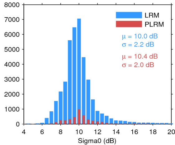
Figure 25. Histogram of flag-valid sigma0 over oceans and lakes for LRM (blue) and PLRM (red) for 15/03/2017. The mean ( \mu ) and standard deviation ( \sigma ) are also shown. Note that values outside [4 20] dB are excluded from the histogram for the sake of readability but not from the computation of \mu and \sigma .
