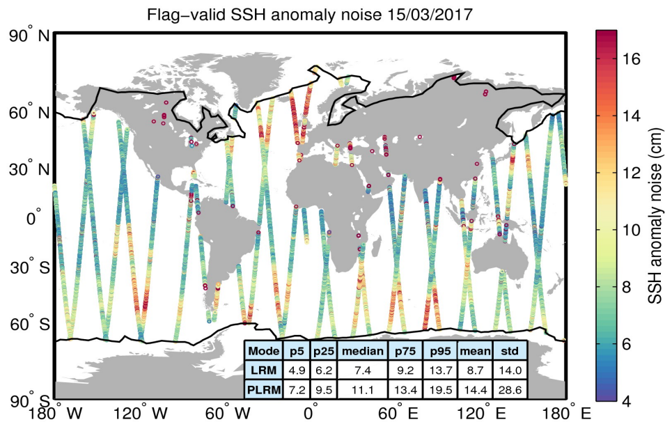
Figure 8. Geographical distribution of flag-valid 20-Hz SSH anomaly measurement noise over oceans and lakes for 15/03/2017. The statistical values shown in the table refer to the SSH anomaly noise and are calculated separately for LRM and PLRM regions. Measurements taken over polar polygons have been excluded from the computation of the statistical values. The black lines mark the outer limit of the Arctic and Antarctic polar polygons.
