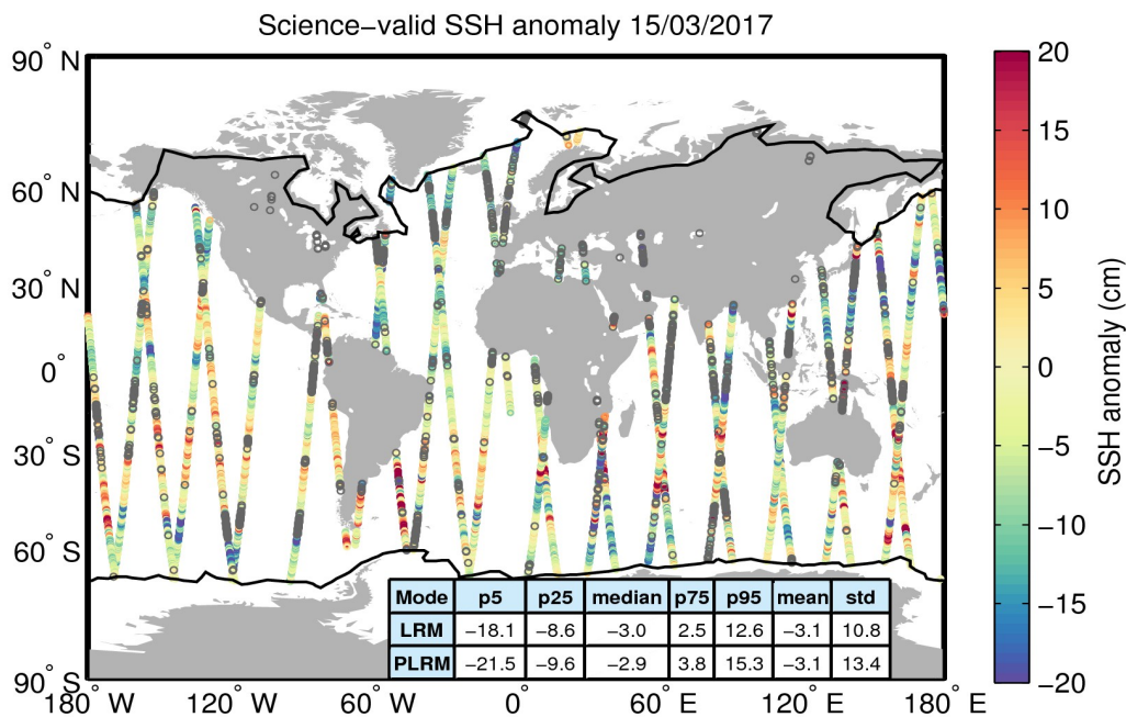
Figure 10. Geographical distribution of science-valid SSH anomaly data over oceans and lakes for 15/03/2017. The statistical values shown in the table refer to the SSH anomaly in cm and are calculated separately for LRM and PLRM regions. The black lines mark the outer limit of the Arctic and Antarctic polar polygons. Gray circles denote records that have been rejected based on the editing criteria described in Table 2.
