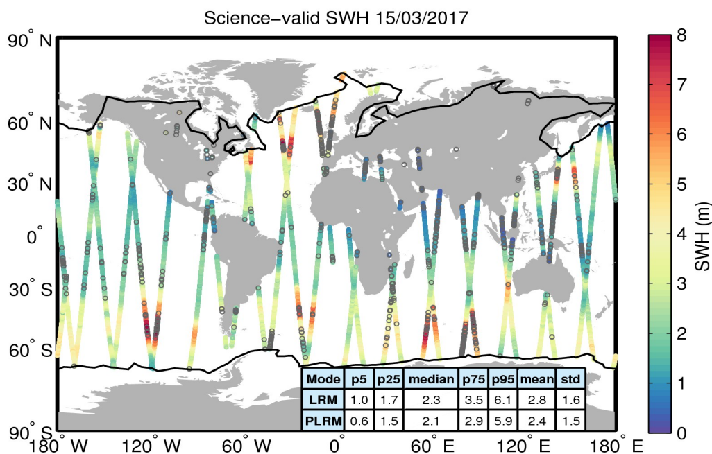
Figure 19. Geographical distribution of science-valid SWH data over oceans and lakes for 15/03/2017. The statistical values shown in the table refer to the SWH in m and are calculated separately for LRM and PLRM regions. The black lines mark the outer limit of the Arctic and Antarctic polar polygons. Gray circles denote records that have been rejected based on the editing criteria described in Table 3.
