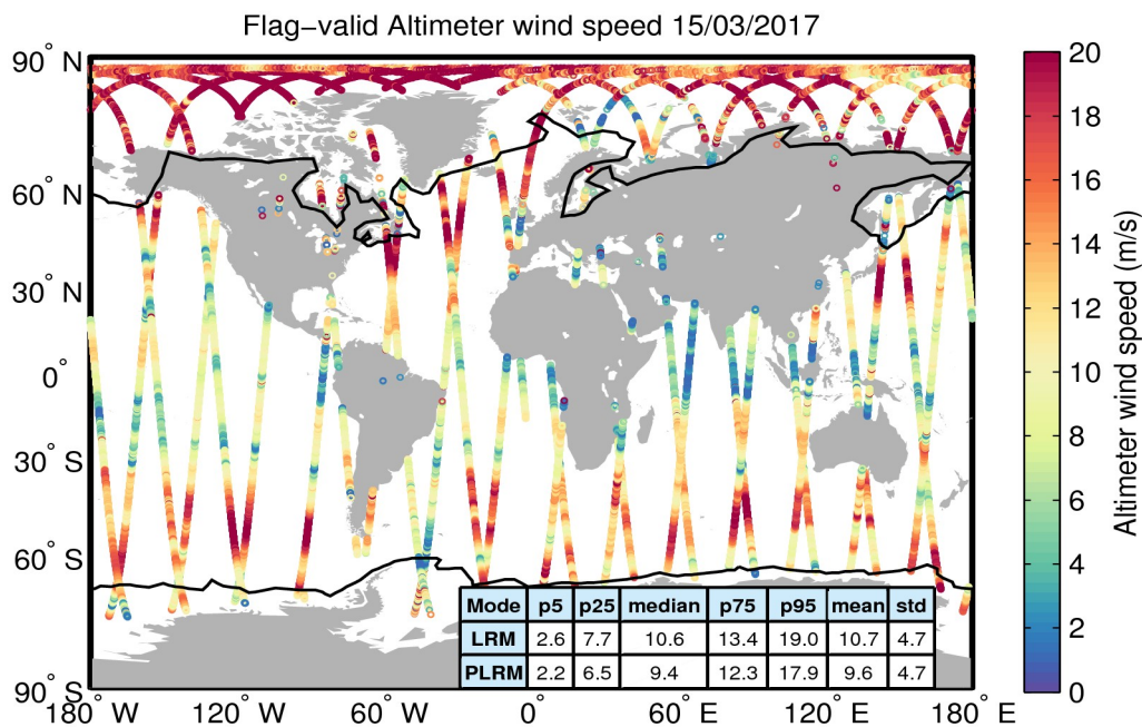
Figure 31. Geographical distribution of flag-valid wind data over oceans and lakes for 15/03/2017. The statistical values shown in the table refer to the wind in m/s and are calculated separately for LRM and PLRM regions. Measurements taken over polar polygons have been excluded from the computation of the statistical values. The black lines mark the outer limit of the Arctic and Antarctic polar polygons.
