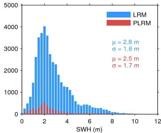
Figure 17. Histogram of flag-valid SWH over oceans and lakes for LRM (blue) and PLRM (red) for 15/03/2017. The mean ( \mu ) and standard deviation ( \sigma ) are also shown. Note that values larger than 12 m are excluded from the histogram for the sake of readability but not from the computation of \mu and \sigma .
