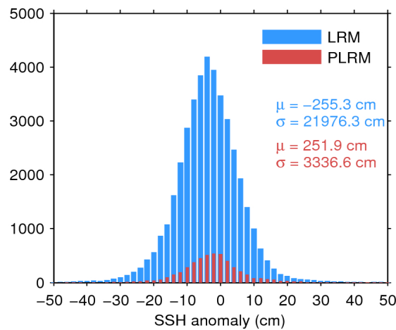
Figure 7. Histogram of flag-valid SSH anomaly over oceans and lakes for LRM (blue) and PLRM (red) for 12/03/2017. The mean ( \mu ) and standard deviation ( \sigma ) are also shown. Note that values outside [-50\ 50] cm are excluded from the histogram for the sake of readability but not from the computation of \mu and \sigma .
