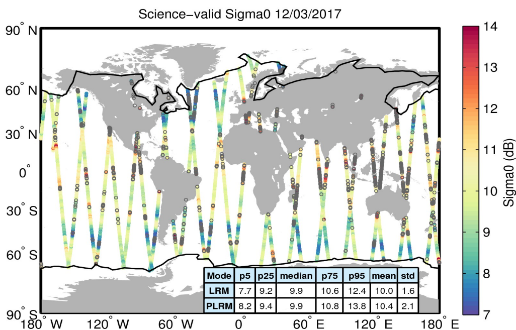
Figure 27. Geographical distribution of science-valid sigma0 data over oceans and lakes for 12/03/2017. The statistical values shown in the table refer to the sigma0 in dB and are calculated separately for LRM and PLRM regions. The black lines mark the outer limit of the Arctic and Antarctic polar polygons. Gray circles denote records that have been rejected based on the editing criteria described in Table 4.
