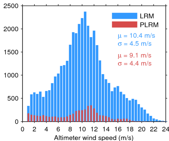
Figure 35. Histogram of science-valid wind over oceans and lakes for LRM (blue) and PLRM (red) for 12/03/2017. The mean ( \mu ) and standard deviation ( \sigma ) are also shown. Note that values larger than 24 m/s are excluded from the histogram for the sake of readability but not from the computation of \mu and \sigma .
