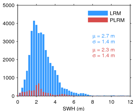
Figure 17. Histogram of flag-valid SWH over oceans and lakes for LRM (blue) and PLRM (red) for 12/03/2017. The mean ( \mu ) and standard deviation ( \sigma ) are also shown. Note that values larger than 12 m are excluded from the histogram for the sake of readability but not from the computation of \mu and \sigma .
