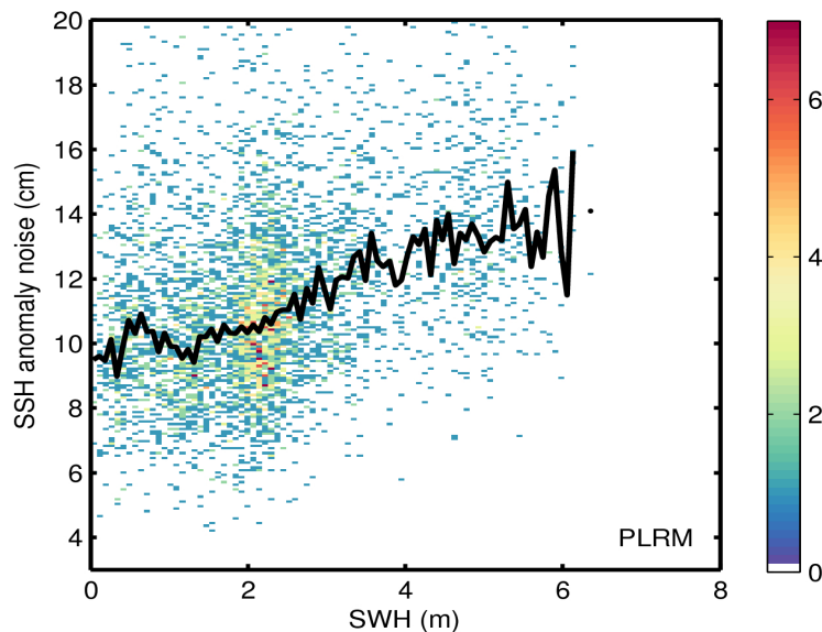
Figure 9. 2D histogram showing flag-valid SSH anomaly noise as a function of SWH for LRM (top) and PLRM (bottom) for 12/03/2017. The black line denotes the median SSH anomaly noise as a function of SWH.
