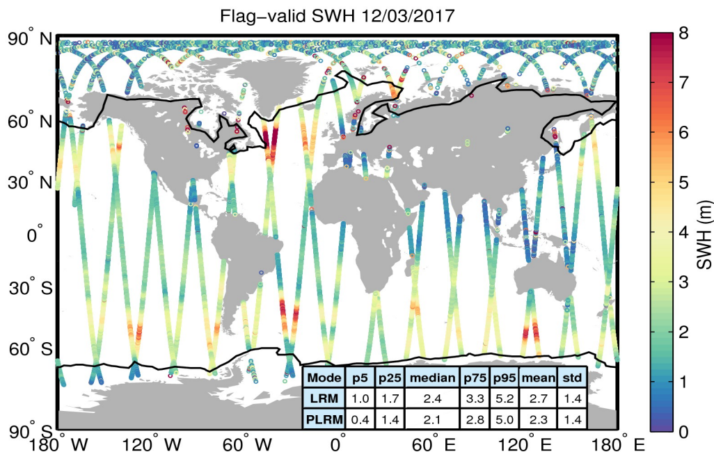
Figure 15. Geographical distribution of flag-valid SWH data over oceans and lakes for 12/03/2017. The statistical values shown in the table refer to the SWH in m and are calculated separately for LRM and PLRM regions. Measurements taken over polar polygons have been excluded from the computation of the statistical values. The black lines mark the outer limit of the Arctic and Antarctic polar polygons.
