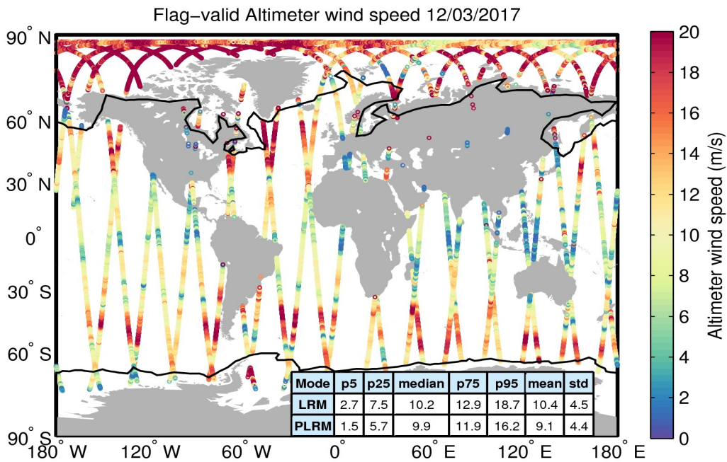
Figure 31. Geographical distribution of flag-valid wind data over oceans and lakes for 12/03/2017. The statistical values shown in the table refer to the wind in m/s and are calculated separately for LRM and PLRM regions. Measurements taken over polar polygons have been excluded from the computation of the statistical values. The black lines mark the outer limit of the Arctic and Antarctic polar polygons.
