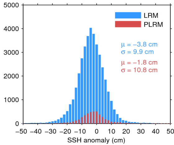
Figure 11. Histogram of science-valid SSH anomaly over oceans and lakes for LRM (blue) and PLRM (red) for 12/03/2017. The mean ( \mu ) and standard deviation ( \sigma ) are also shown. Note that values outside [-50 50] cm are excluded from the histogram for the sake of readability but not from the computation of \mu and \sigma .
