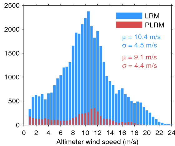
Figure 33. Histogram of flag-valid wind over oceans and lakes for LRM (blue) and PLRM (red) for 12/03/2017. The mean ( \mu ) and standard deviation ( \sigma ) are also shown. Note that values larger than 24 m/s are excluded from the histogram for the sake of readability but not from the computation of \mu and \sigma .
