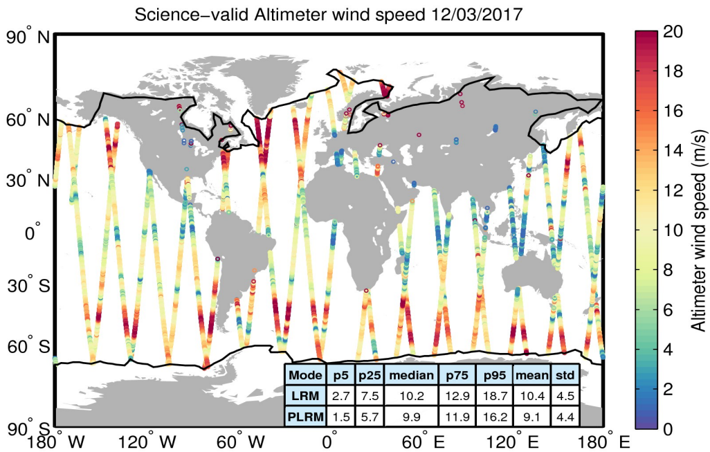
Figure 34. Geographical distribution of science-valid wind data over oceans and lakes for 12/03/2017. The statistical values shown in the table refer to the wind in m/s and are calculated separately for LRM and PLRM regions. The black lines mark the outer limit of the Arctic and Antarctic polar polygons. Gray circles denote records that have been rejected based on the editing criteria described in Table 5.
