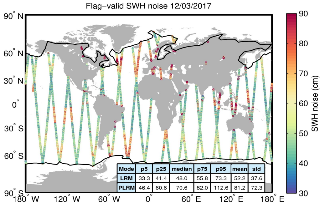
Figure 18. Geographical distribution of flag-valid 20-Hz SWH measurement noise over oceans and lakes for 12/03/2017. The statistical values shown in the table refer to the SWH noise and are calculated separately for LRM and PLRM regions. Measurements taken over polar polygons have been excluded from the computation of the statistical values. The black lines mark the outer limit of the Arctic and Antarctic polar polygons.
