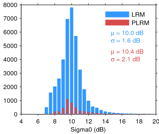
Figure 28. Histogram of science-valid sigma0 over oceans and lakes for LRM (blue) and PLRM (red) for 12/03/2017. The mean ( \mu ) and standard deviation ( \sigma ) are also shown. Note that values outside [4 20] dB are excluded from the histogram for the sake of readability but not from the computation of \mu and \sigma .
