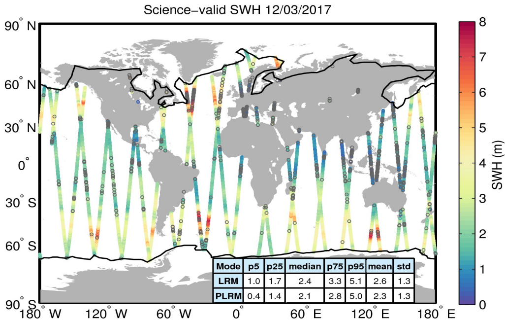
Figure 19. Geographical distribution of science-valid SWH data over oceans and lakes for 12/03/2017. The statistical values shown in the table refer to the SWH in m and are calculated separately for LRM and PLRM regions. The black lines mark the outer limit of the Arctic and Antarctic polar polygons. Gray circles denote records that have been rejected based on the editing criteria described in Table 3.
