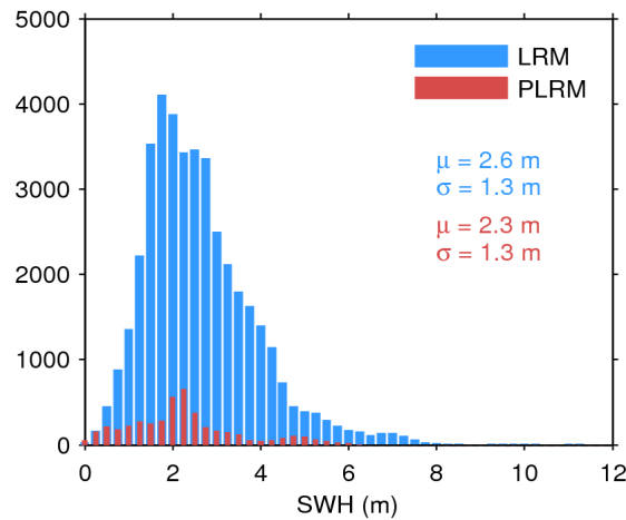
Figure 20. Histogram of science-valid SWH over oceans and lakes for LRM (blue) and PLRM (red) for 12/03/2017. The mean ( \mu ) and standard deviation ( \sigma ) are also shown. Note that values larger than 12 m are excluded from the histogram for the sake of readability but not from the computation of \mu and \sigma .
