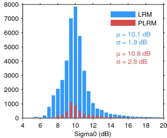
Figure 25. Histogram of flag-valid sigma0 over oceans and lakes for LRM (blue) and PLRM (red) for 12/03/2017. The mean ( \mu ) and standard deviation ( \sigma ) are also shown. Note that values outside [4 20] dB are excluded from the histogram for the sake of readability but not from the computation of \mu and \sigma .
