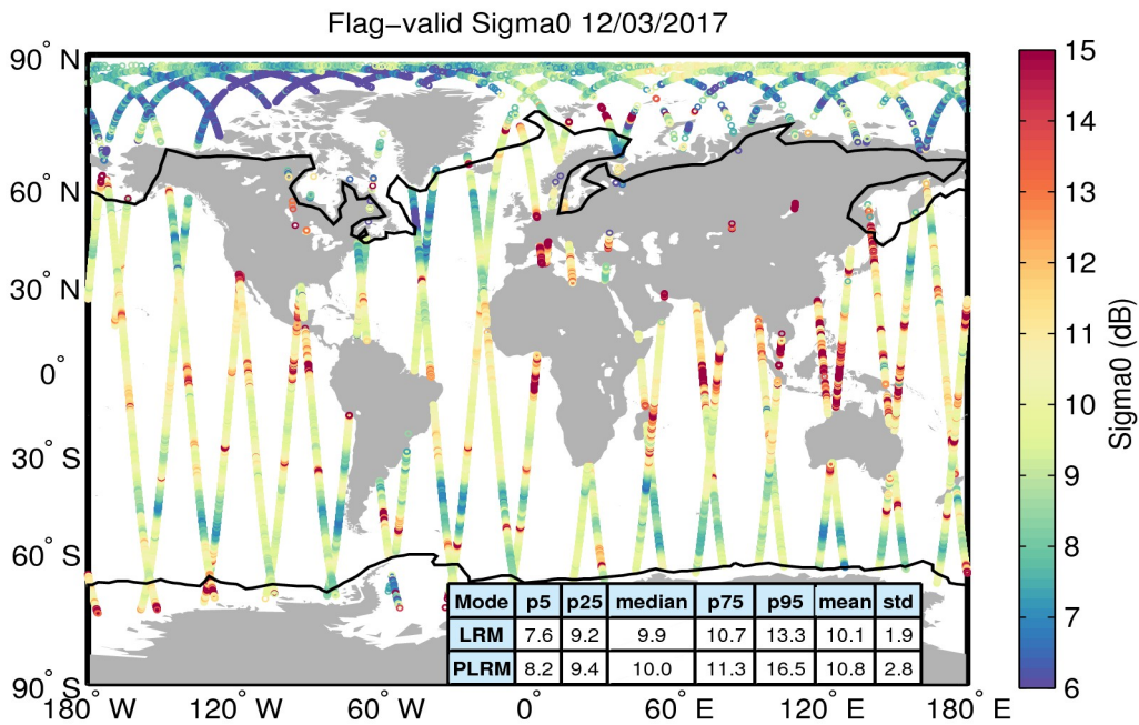
Figure 23. Geographical distribution of flag-valid sigma0 data over oceans and lakes for 12/03/2017. The statistical values shown in the table refer to the sigma0 in dB and are calculated separately for LRM and PLRM regions. Measurements taken over polar polygons have been excluded from the computation of the statistical values. The black lines mark the outer limit of the Arctic and Antarctic polar polygons.
