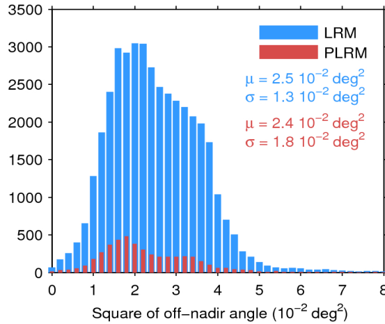
Figure 39. Histogram of flag-valid mispointing over oceans and lakes for LRM (blue) and PLRM (red) for 12/03/2017. Only positive values have been considered. The mean ( \mu ) and standard deviation ( \sigma ) are also shown. Note that values larger than 8 \cdot 10^{-2} \text{ deg}^2 are excluded from the histogram for the sake of readability but not from the computation of \mu and \sigma .
