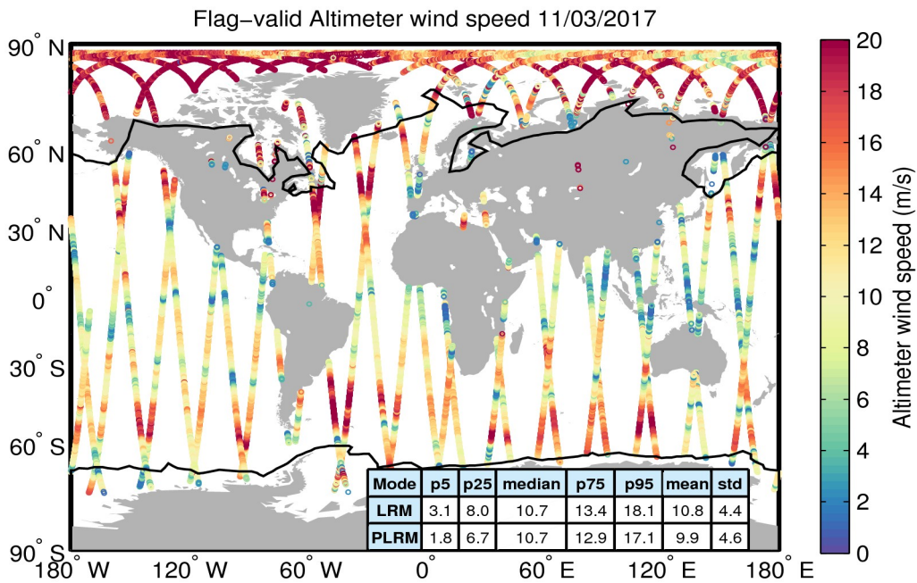
Figure 31. Geographical distribution of flag-valid wind data over oceans and lakes for 11/03/2017. The statistical values shown in the table refer to the wind in m/s and are calculated separately for LRM and PLRM regions. Measurements taken over polar polygons have been excluded from the computation of the statistical values. The black lines mark the outer limit of the Arctic and Antarctic polar polygons.
