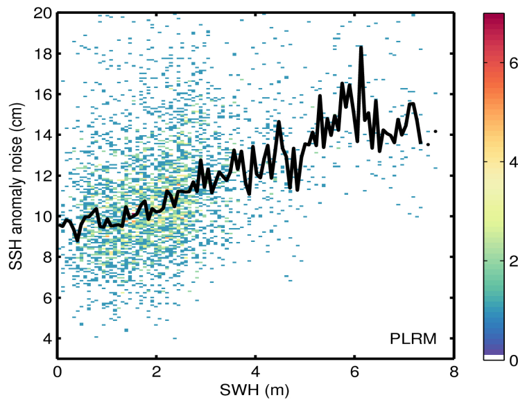
Figure 9. 2D histogram showing flag-valid SSH anomaly noise as a function of SWH for LRM (top) and PLRM (bottom) for 11/03/2017. The black line denotes the median SSH anomaly noise as a function of SWH.
