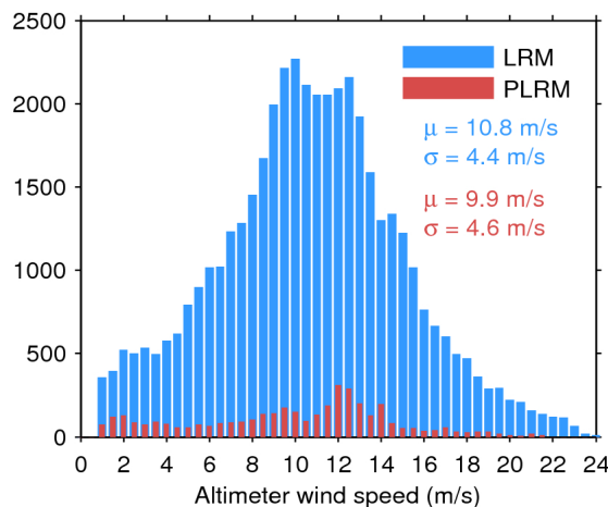
Figure 35. Histogram of science-valid wind over oceans and lakes for LRM (blue) and PLRM (red) for 11/03/2017. The mean ( \mu ) and standard deviation ( \sigma ) are also shown. Note that values larger than 24 m/s are excluded from the histogram for the sake of readability but not from the computation of \mu and \sigma .
