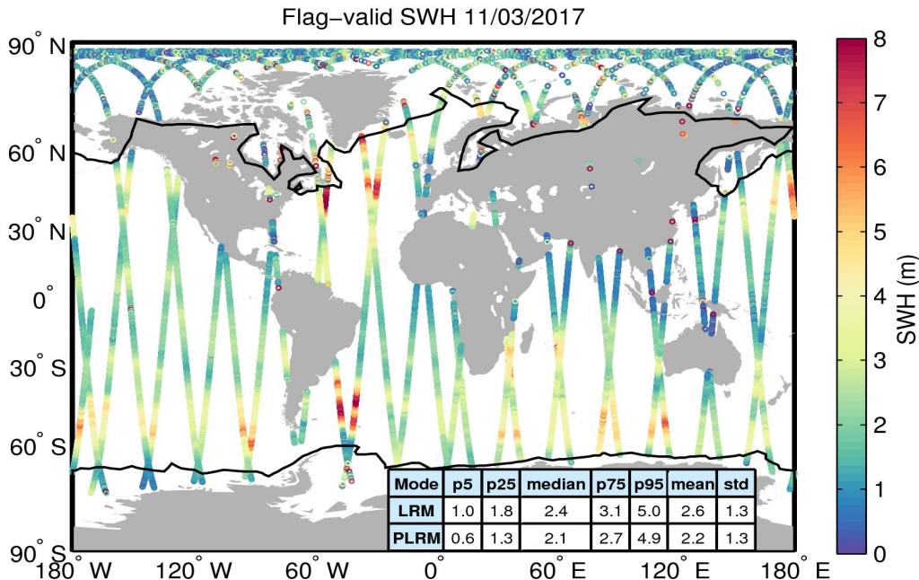
Figure 15. Geographical distribution of flag-valid SWH data over oceans and lakes for 11/03/2017. The statistical values shown in the table refer to the SWH in m and are calculated separately for LRM and PLRM regions. Measurements taken over polar polygons have been excluded from the computation of the statistical values. The black lines mark the outer limit of the Arctic and Antarctic polar polygons.
