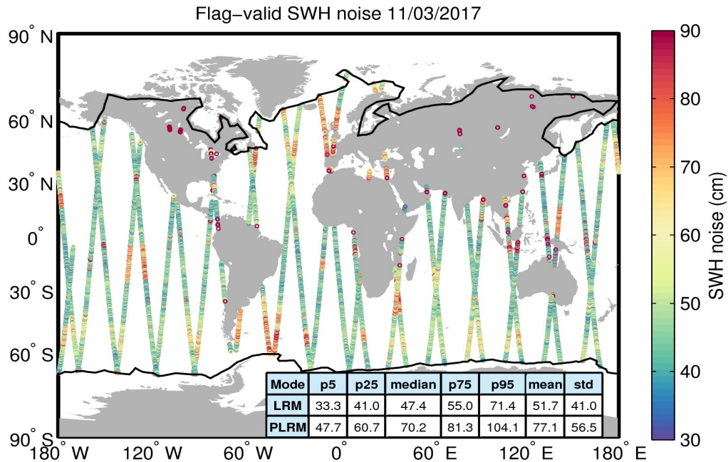
Figure 18. Geographical distribution of flag-valid 20-Hz SWH measurement noise over oceans and lakes for 11/03/2017. The statistical values shown in the table refer to the SWH noise and are calculated separately for LRM and PLRM regions. Measurements taken over polar polygons have been excluded from the computation of the statistical values. The black lines mark the outer limit of the Arctic and Antarctic polar polygons.
