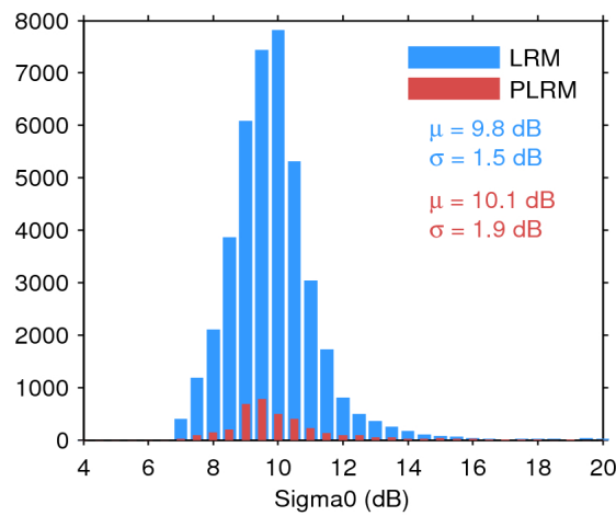
Figure 28. Histogram of science-valid sigma0 over oceans and lakes for LRM (blue) and PLRM (red) for 11/03/2017. The mean ( \mu ) and standard deviation ( \sigma ) are also shown. Note that values outside [4 20] dB are excluded from the histogram for the sake of readability but not from the computation of \mu and \sigma .
