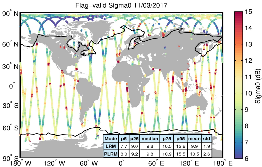
Figure 23. Geographical distribution of flag-valid sigma0 data over oceans and lakes for 11/03/2017. The statistical values shown in the table refer to the sigma0 in dB and are calculated separately for LRM and PLRM regions. Measurements taken over polar polygons have been excluded from the computation of the statistical values. The black lines mark the outer limit of the Arctic and Antarctic polar polygons.
