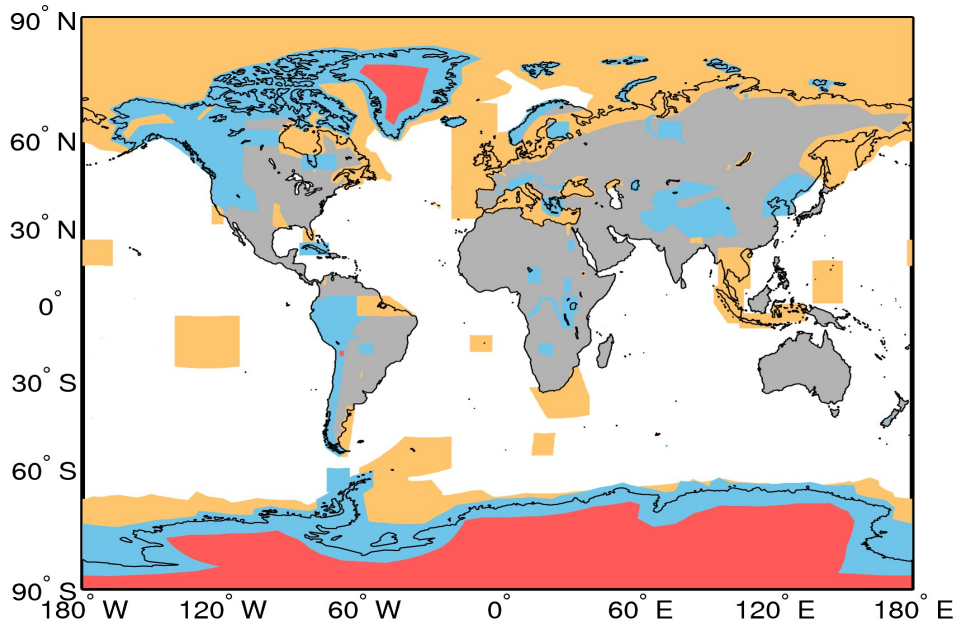
Figure A1. Extent of the regions defining the geographical mode mask for 11/03/2017. The regions where SAR, and SARIn are operated are denoted by the orange and blue polygons, respectively. LRM is operated over areas of the continental ice sheets (red polygons) and over oceans and land not covered by other modes.
