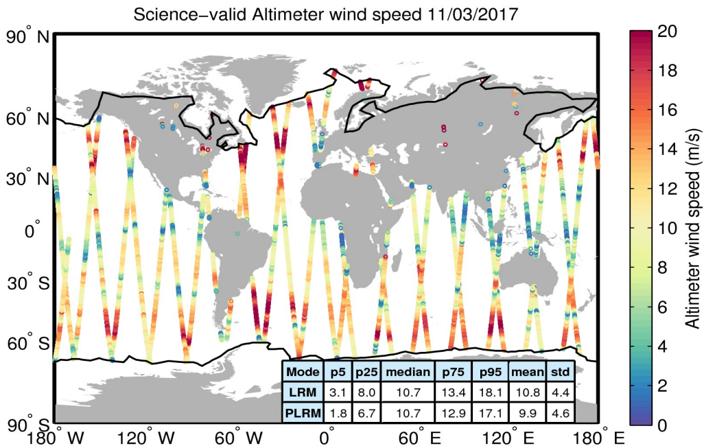
Figure 34. Geographical distribution of science-valid wind data over oceans and lakes for 11/03/2017. The statistical values shown in the table refer to the wind in m/s and are calculated separately for LRM and PLRM regions. The black lines mark the outer limit of the Arctic and Antarctic polar polygons. Gray circles denote records that have been rejected based on the editing criteria described in Table 5.
