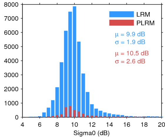
Figure 25. Histogram of flag-valid sigma0 over oceans and lakes for LRM (blue) and PLRM (red) for 11/03/2017. The mean ( \mu ) and standard deviation ( \sigma ) are also shown. Note that values outside [4 20] dB are excluded from the histogram for the sake of readability but not from the computation of \mu and \sigma .
