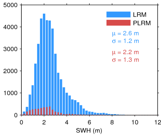
Figure 20. Histogram of science-valid SWH over oceans and lakes for LRM (blue) and PLRM (red) for 11/03/2017. The mean ( \mu ) and standard deviation ( \sigma ) are also shown. Note that values larger than 12 m are excluded from the histogram for the sake of readability but not from the computation of \mu and \sigma .
