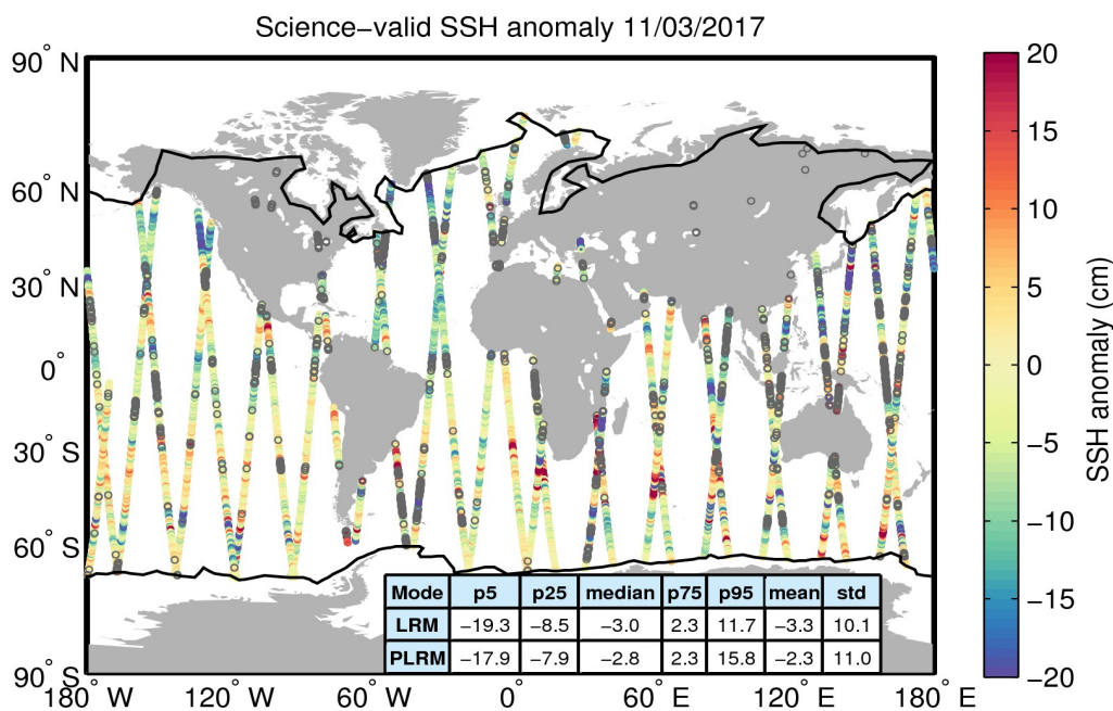
Figure 10. Geographical distribution of science-valid SSH anomaly data over oceans and lakes for 11/03/2017. The statistical values shown in the table refer to the SSH anomaly in cm and are calculated separately for LRM and PLRM regions. The black lines mark the outer limit of the Arctic and Antarctic polar polygons. Gray circles denote records that have been rejected based on the editing criteria described in Table 2.
