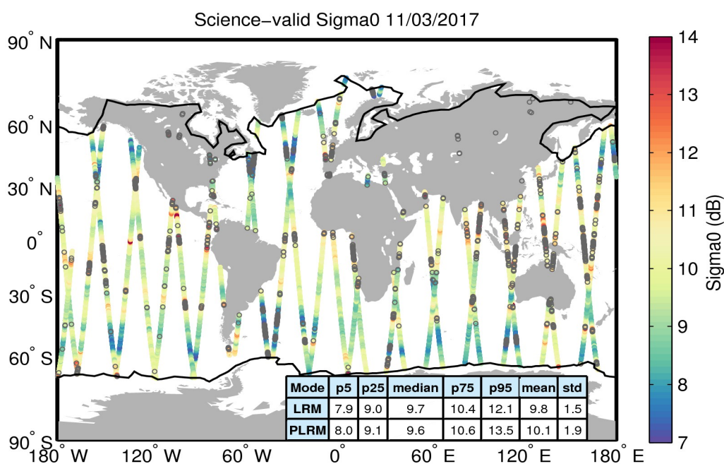
Figure 27. Geographical distribution of science-valid sigma0 data over oceans and lakes for 11/03/2017. The statistical values shown in the table refer to the sigma0 in dB and are calculated separately for LRM and PLRM regions. The black lines mark the outer limit of the Arctic and Antarctic polar polygons. Gray circles denote records that have been rejected based on the editing criteria described in Table 4.
