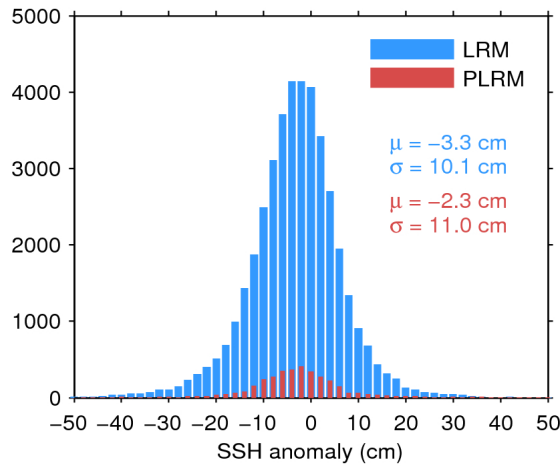
Figure 11. Histogram of science-valid SSH anomaly over oceans and lakes for LRM (blue) and PLRM (red) for 11/03/2017. The mean ( \mu ) and standard deviation ( \sigma ) are also shown. Note that values outside [-50 50] cm are excluded from the histogram for the sake of readability but not from the computation of \mu and \sigma .
