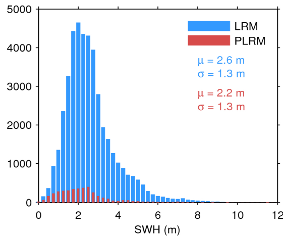
Figure 17. Histogram of flag-valid SWH over oceans and lakes for LRM (blue) and PLRM (red) for 11/03/2017. The mean ( \mu ) and standard deviation ( \sigma ) are also shown. Note that values larger than 12 m are excluded from the histogram for the sake of readability but not from the computation of \mu and \sigma .
