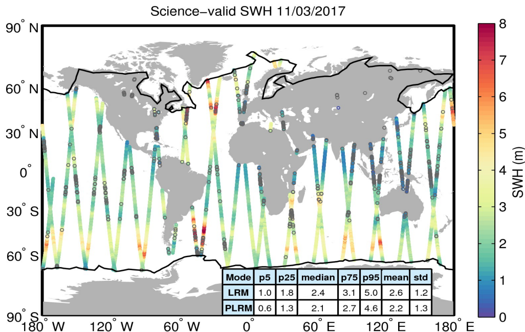
Figure 19. Geographical distribution of science-valid SWH data over oceans and lakes for 11/03/2017. The statistical values shown in the table refer to the SWH in m and are calculated separately for LRM and PLRM regions. The black lines mark the outer limit of the Arctic and Antarctic polar polygons. Gray circles denote records that have been rejected based on the editing criteria described in Table 3.
