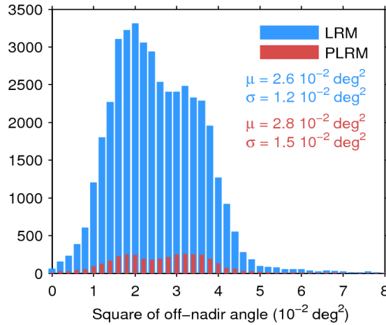
Figure 39. Histogram of flag-valid mispointing over oceans and lakes for LRM (blue) and PLRM (red) for 11/03/2017. Only positive values have been considered. The mean ( \mu ) and standard deviation ( \sigma ) are also shown. Note that values larger than 8 \cdot 10^{-2} \text{ deg}^2 are excluded from the histogram for the sake of readability but not from the computation of \mu and \sigma .
