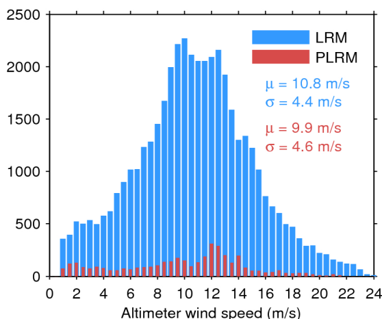
Figure 33. Histogram of flag-valid wind over oceans and lakes for LRM (blue) and PLRM (red) for 11/03/2017. The mean ( \mu ) and standard deviation ( \sigma ) are also shown. Note that values larger than 24 m/s are excluded from the histogram for the sake of readability but not from the computation of \mu and \sigma .
