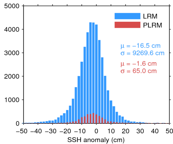
Figure 7. Histogram of flag-valid SSH anomaly over oceans and lakes for LRM (blue) and PLRM (red) for 11/03/2017. The mean ( \mu ) and standard deviation ( \sigma ) are also shown. Note that values outside [-50 50] cm are excluded from the histogram for the sake of readability but not from the computation of \mu and \sigma .
