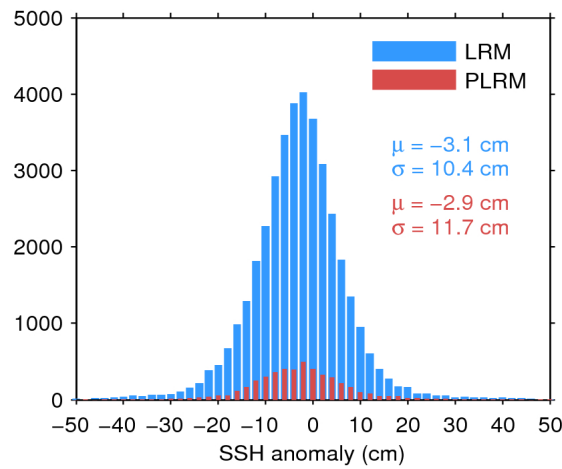
Figure 11. Histogram of science-valid SSH anomaly over oceans and lakes for LRM (blue) and PLRM (red) for 08/03/2017. The mean ( \mu ) and standard deviation ( \sigma ) are also shown. Note that values outside [-50 50] cm are excluded from the histogram for the sake of readability but not from the computation of \mu and \sigma .
