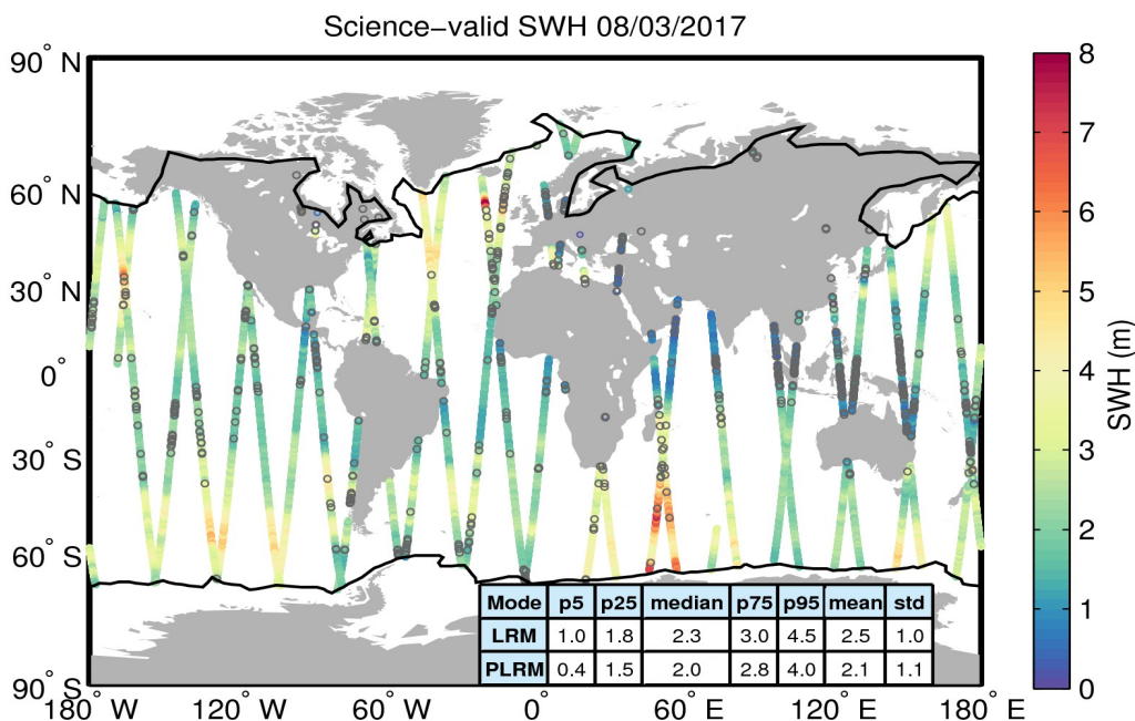
Figure 19. Geographical distribution of science-valid SWH data over oceans and lakes for 08/03/2017. The statistical values shown in the table refer to the SWH in m and are calculated separately for LRM and PLRM regions. The black lines mark the outer limit of the Arctic and Antarctic polar polygons. Gray circles denote records that have been rejected based on the editing criteria described in Table 3.
