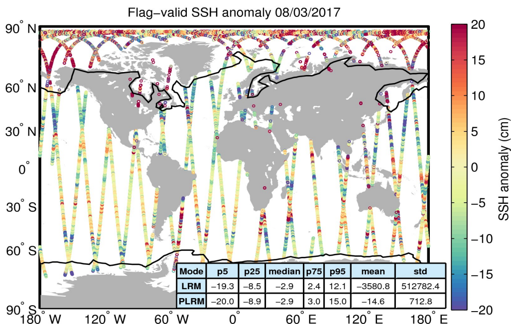
Figure 5. Geographical distribution of flag-valid 1-Hz SSH anomaly data over oceans and lakes for 08/03/2017. The statistical values shown in the table refer to the SSH anomaly in cm and are calculated separately for LRM and PLRM regions. Measurements taken over polar polygons have been excluded from the computation of the statistical values. The black lines mark the outer limit of the Arctic and Antarctic polar polygons.
