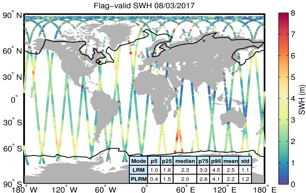
Figure 15. Geographical distribution of flag-valid SWH data over oceans and lakes for 08/03/2017. The statistical values shown in the table refer to the SWH in m and are calculated separately for LRM and PLRM regions. Measurements taken over polar polygons have been excluded from the computation of the statistical values. The black lines mark the outer limit of the Arctic and Antarctic polar polygons.
