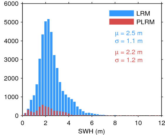
Figure 17. Histogram of flag-valid SWH over oceans and lakes for LRM (blue) and PLRM (red) for 08/03/2017. The mean ( \mu ) and standard deviation ( \sigma ) are also shown. Note that values larger than 12 m are excluded from the histogram for the sake of readability but not from the computation of \mu and \sigma .
