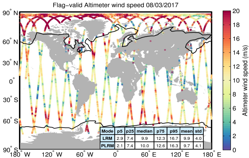
Figure 31. Geographical distribution of flag-valid wind data over oceans and lakes for 08/03/2017. The statistical values shown in the table refer to the wind in m/s and are calculated separately for LRM and PLRM regions. Measurements taken over polar polygons have been excluded from the computation of the statistical values. The black lines mark the outer limit of the Arctic and Antarctic polar polygons.
