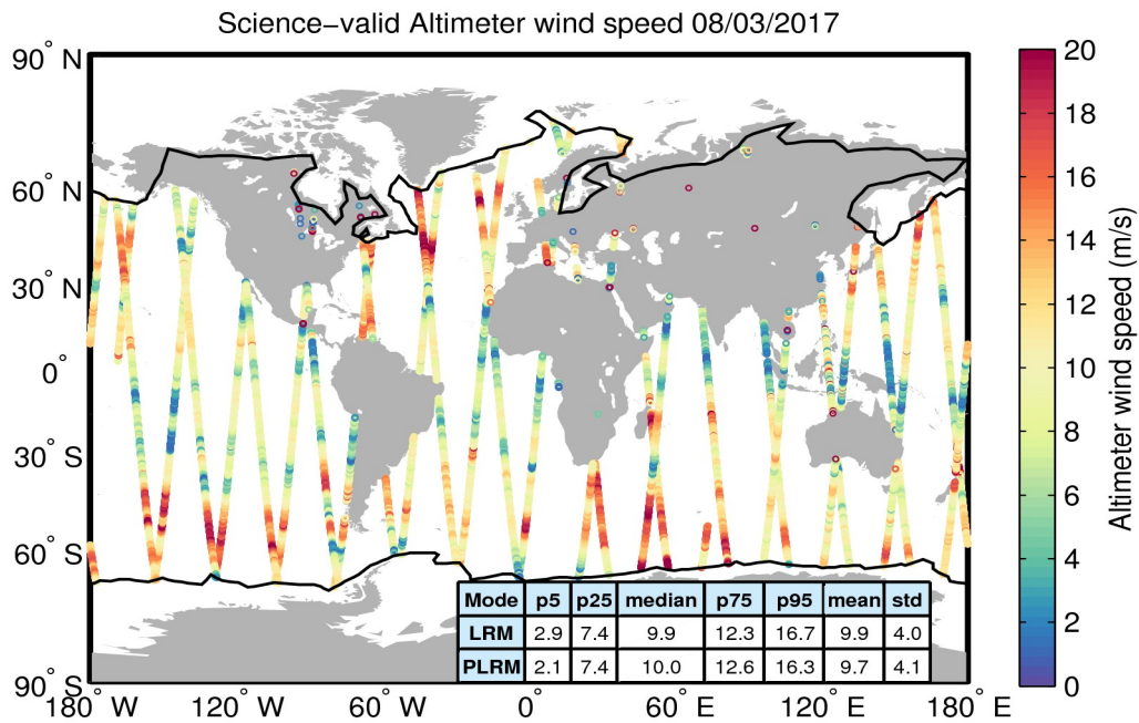
Figure 34. Geographical distribution of science-valid wind data over oceans and lakes for 08/03/2017. The statistical values shown in the table refer to the wind in m/s and are calculated separately for LRM and PLRM regions. The black lines mark the outer limit of the Arctic and Antarctic polar polygons. Gray circles denote records that have been rejected based on the editing criteria described in Table 5.
