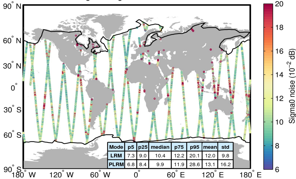
Flag-valid sigma0 noise 08/03/2017
