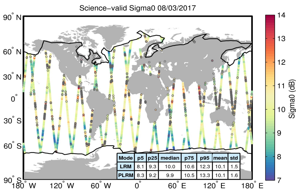
Figure 27. Geographical distribution of science-valid sigma0 data over oceans and lakes for 08/03/2017. The statistical values shown in the table refer to the sigma0 in dB and are calculated separately for LRM and PLRM regions. The black lines mark the outer limit of the Arctic and Antarctic polar polygons. Gray circles denote records that have been rejected based on the editing criteria described in Table 4.
