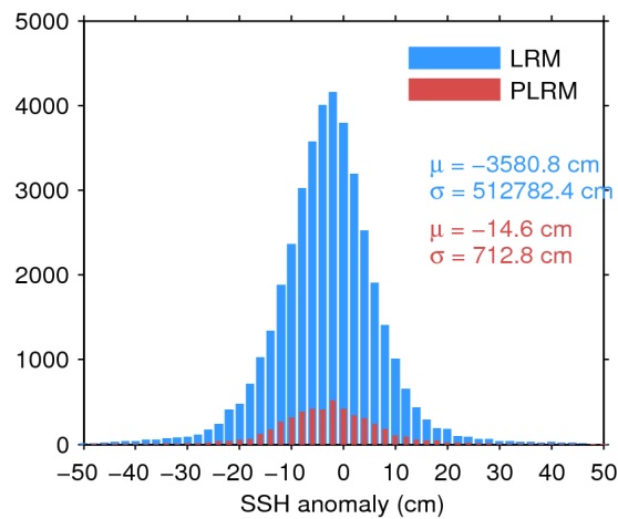
Figure 7. Histogram of flag-valid SSH anomaly over oceans and lakes for LRM (blue) and PLRM (red) for 08/03/2017. The mean ( \mu ) and standard deviation ( \sigma ) are also shown. Note that values outside [-50 50] cm are excluded from the histogram for the sake of readability but not from the computation of \mu and \sigma .
