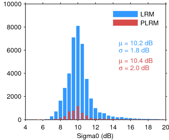
Figure 25. Histogram of flag-valid sigma0 over oceans and lakes for LRM (blue) and PLRM (red) for 08/03/2017. The mean ( \mu ) and standard deviation ( \sigma ) are also shown. Note that values outside [4 20] dB are excluded from the histogram for the sake of readability but not from the computation of \mu and \sigma .
