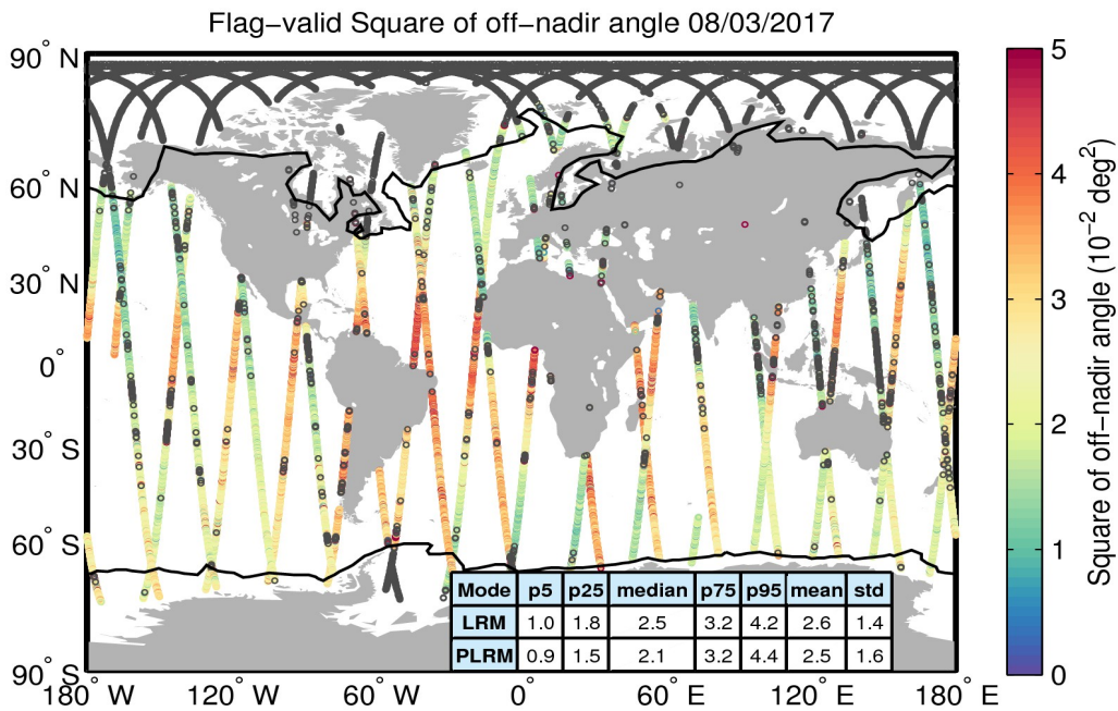
Figure 37. Geographical distribution of flag-valid mispointing data over oceans and lakes for 08/03/2017. The statistical values shown in the table refer to the mispointing in 10^{-2} deg 2 and are calculated separately for LRM and PLRM regions. Measurements taken over polar polygons have been excluded from the computation of the statistical values. The black lines mark the outer limit of the Arctic and Antarctic polar polygons. Gray circles denote negative values.
