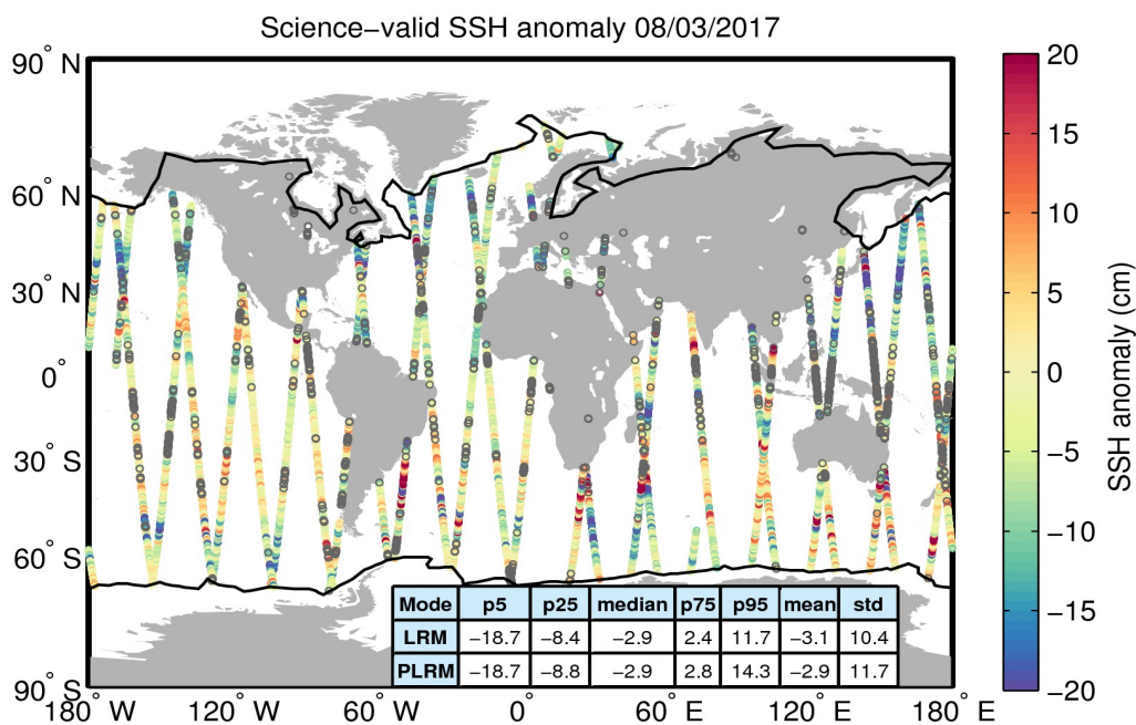
Figure 10. Geographical distribution of science-valid SSH anomaly data over oceans and lakes for 08/03/2017. The statistical values shown in the table refer to the SSH anomaly in cm and are calculated separately for LRM and PLRM regions. The black lines mark the outer limit of the Arctic and Antarctic polar polygons. Gray circles denote records that have been rejected based on the editing criteria described in Table 2.
