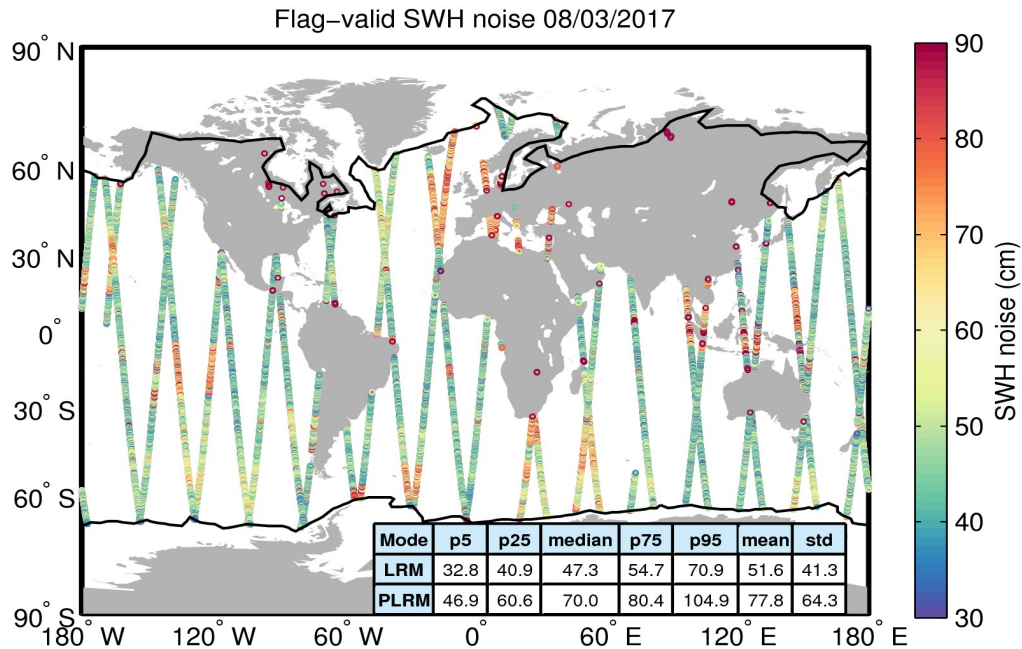
Figure 18. Geographical distribution of flag-valid 20-Hz SWH measurement noise over oceans and lakes for 08/03/2017. The statistical values shown in the table refer to the SWH noise and are calculated separately for LRM and PLRM regions. Measurements taken over polar polygons have been excluded from the computation of the statistical values. The black lines mark the outer limit of the Arctic and Antarctic polar polygons.
