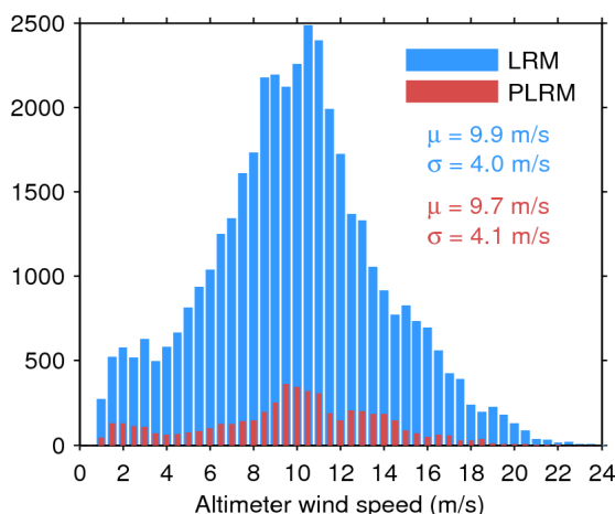
Figure 33. Histogram of flag-valid wind over oceans and lakes for LRM (blue) and PLRM (red) for 08/03/2017. The mean ( \mu ) and standard deviation ( \sigma ) are also shown. Note that values larger than 24 m/s are excluded from the histogram for the sake of readability but not from the computation of \mu and \sigma .
