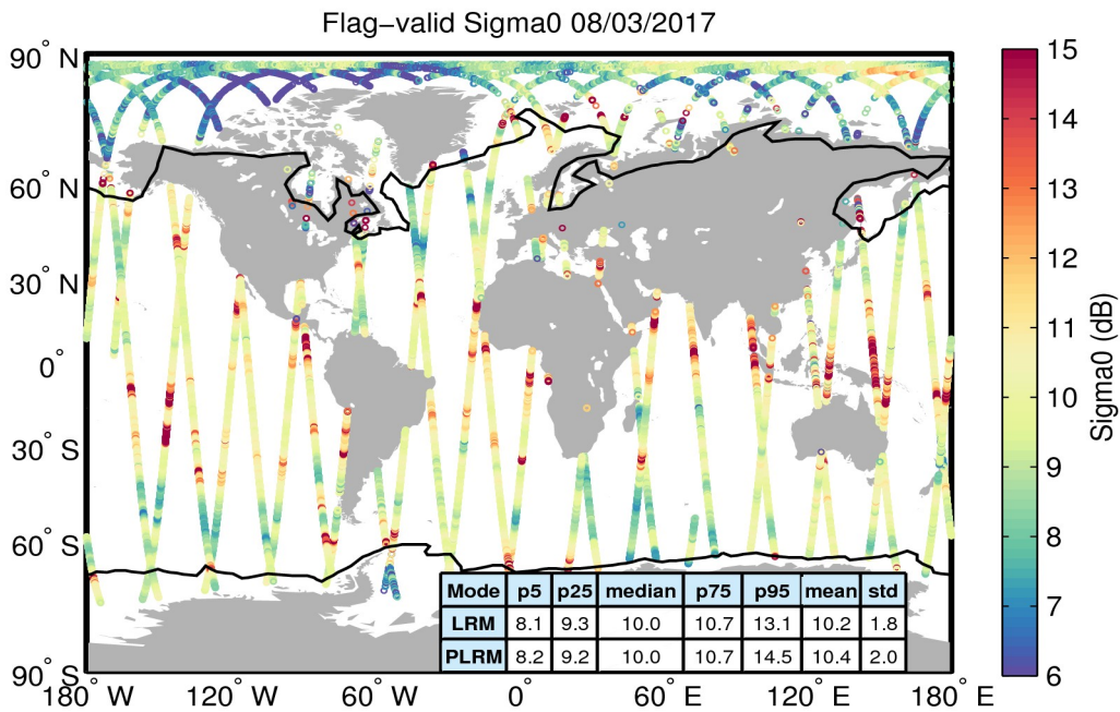
Figure 23. Geographical distribution of flag-valid sigma0 data over oceans and lakes for 08/03/2017. The statistical values shown in the table refer to the sigma0 in dB and are calculated separately for LRM and PLRM regions. Measurements taken over polar polygons have been excluded from the computation of the statistical values. The black lines mark the outer limit of the Arctic and Antarctic polar polygons.
