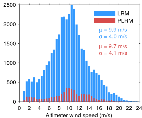
Figure 35. Histogram of science-valid wind over oceans and lakes for LRM (blue) and PLRM (red) for 08/03/2017. The mean ( \mu ) and standard deviation ( \sigma ) are also shown. Note that values larger than 24 m/s are excluded from the histogram for the sake of readability but not from the computation of \mu and \sigma .
