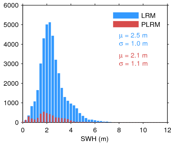
Figure 20. Histogram of science-valid SWH over oceans and lakes for LRM (blue) and PLRM (red) for 08/03/2017. The mean ( \mu ) and standard deviation ( \sigma ) are also shown. Note that values larger than 12 m are excluded from the histogram for the sake of readability but not from the computation of \mu and \sigma .
