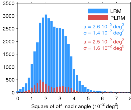
Figure 39. Histogram of flag-valid mispointing over oceans and lakes for LRM (blue) and PLRM (red) for 08/03/2017. Only positive values have been considered. The mean ( \mu ) and standard deviation ( \sigma ) are also shown. Note that values larger than 8 \cdot 10^{-2} \text{ deg}^2 are excluded from the histogram for the sake of readability but not from the computation of \mu and \sigma .
