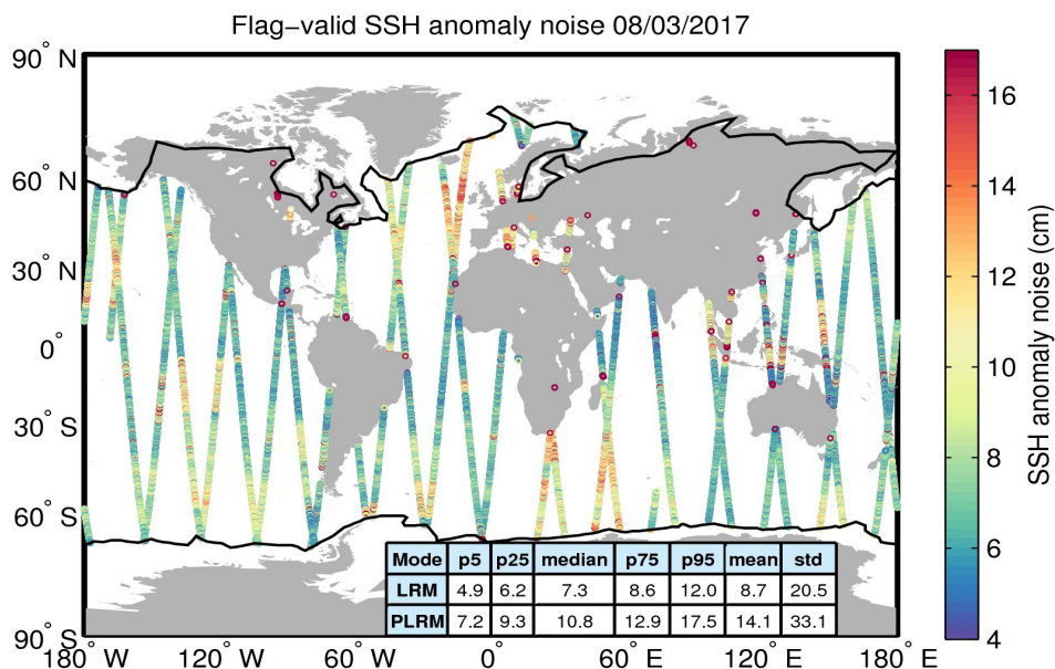
Figure 8. Geographical distribution of flag-valid 20-Hz SSH anomaly measurement noise over oceans and lakes for 08/03/2017. The statistical values shown in the table refer to the SSH anomaly noise and are calculated separately for LRM and PLRM regions. Measurements taken over polar polygons have been excluded from the computation of the statistical values. The black lines mark the outer limit of the Arctic and Antarctic polar polygons.
