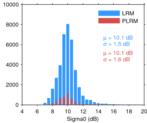
Figure 28. Histogram of science-valid sigma0 over oceans and lakes for LRM (blue) and PLRM (red) for 08/03/2017. The mean ( \mu ) and standard deviation ( \sigma ) are also shown. Note that values outside [4 20] dB are excluded from the histogram for the sake of readability but not from the computation of \mu and \sigma .
