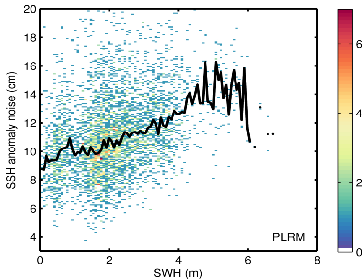
Figure 9. 2D histogram showing flag-valid SSH anomaly noise as a function of SWH for LRM (top) and PLRM (bottom) for 08/03/2017. The black line denotes the median SSH anomaly noise as a function of SWH.
