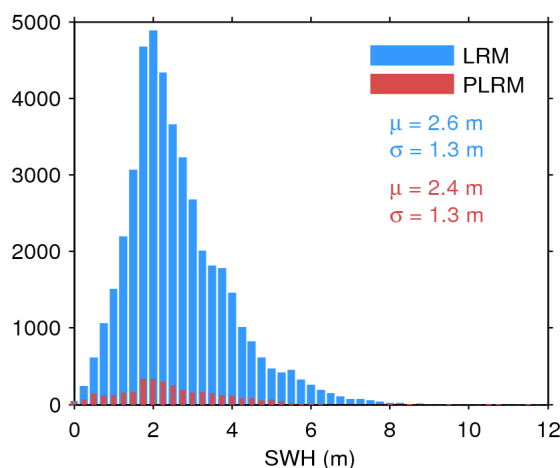
Figure 17. Histogram of flag-valid SWH over oceans and lakes for LRM (blue) and PLRM (red) for 05/03/2017. The mean ( \mu ) and standard deviation ( \sigma ) are also shown. Note that values larger than 12 m are excluded from the histogram for the sake of readability but not from the computation of \mu and \sigma .
