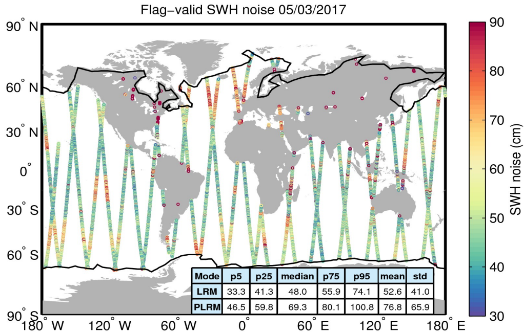
Figure 18. Geographical distribution of flag-valid 20-Hz SWH measurement noise over oceans and lakes for 05/03/2017. The statistical values shown in the table refer to the SWH noise and are calculated separately for LRM and PLRM regions. Measurements taken over polar polygons have been excluded from the computation of the statistical values. The black lines mark the outer limit of the Arctic and Antarctic polar polygons.
