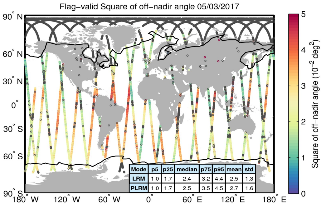
Figure 37. Geographical distribution of flag-valid mispointing data over oceans and lakes for 05/03/2017. The statistical values shown in the table refer to the mispointing in 10^{-2} deg 2 and are calculated separately for LRM and PLRM regions. Measurements taken over polar polygons have been excluded from the computation of the statistical values. The black lines mark the outer limit of the Arctic and Antarctic polar polygons. Gray circles denote negative values.
