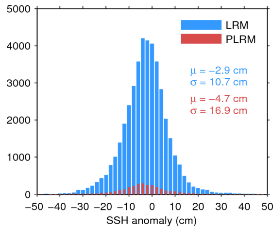
Figure 11. Histogram of science-valid SSH anomaly over oceans and lakes for LRM (blue) and PLRM (red) for 05/03/2017. The mean ( \mu ) and standard deviation ( \sigma ) are also shown. Note that values outside [-50\ 50] cm are excluded from the histogram for the sake of readability but not from the computation of \mu and \sigma .
