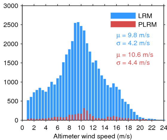
Figure 35. Histogram of science-valid wind over oceans and lakes for LRM (blue) and PLRM (red) for 05/03/2017. The mean ( \mu ) and standard deviation ( \sigma ) are also shown. Note that values larger than 24 m/s are excluded from the histogram for the sake of readability but not from the computation of \mu and \sigma .
