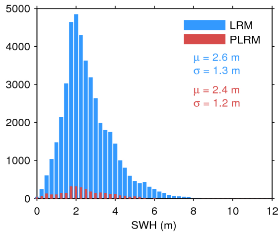
Figure 20. Histogram of science-valid SWH over oceans and lakes for LRM (blue) and PLRM (red) for 05/03/2017. The mean ( \mu ) and standard deviation ( \sigma ) are also shown. Note that values larger than 12 m are excluded from the histogram for the sake of readability but not from the computation of \mu and \sigma .
