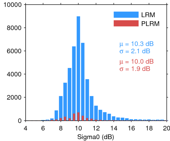
Figure 25. Histogram of flag-valid sigma0 over oceans and lakes for LRM (blue) and PLRM (red) for 05/03/2017. The mean ( \mu ) and standard deviation ( \sigma ) are also shown. Note that values outside [4 20] dB are excluded from the histogram for the sake of readability but not from the computation of \mu and \sigma .
