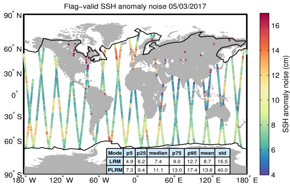
Figure 8. Geographical distribution of flag-valid 20-Hz SSH anomaly measurement noise over oceans and lakes for 05/03/2017. The statistical values shown in the table refer to the SSH anomaly noise and are calculated separately for LRM and PLRM regions. Measurements taken over polar polygons have been excluded from the computation of the statistical values. The black lines mark the outer limit of the Arctic and Antarctic polar polygons.
