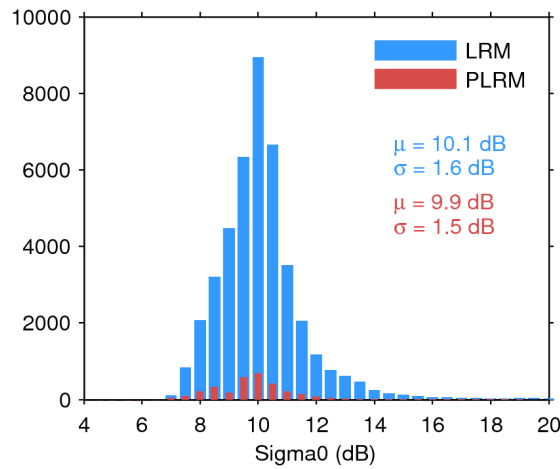
Figure 28. Histogram of science-valid sigma0 over oceans and lakes for LRM (blue) and PLRM (red) for 05/03/2017. The mean ( \mu ) and standard deviation ( \sigma ) are also shown. Note that values outside [4 20] dB are excluded from the histogram for the sake of readability but not from the computation of \mu and \sigma .
