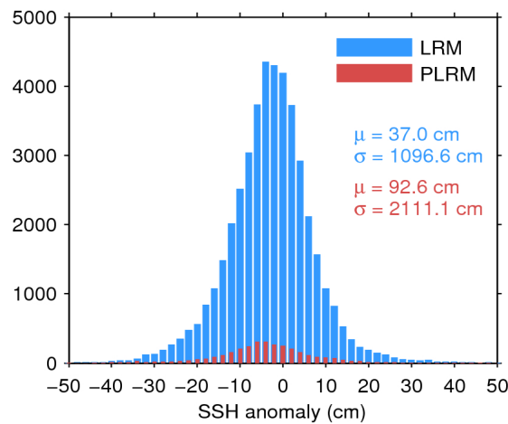
Figure 7. Histogram of flag-valid SSH anomaly over oceans and lakes for LRM (blue) and PLRM (red) for 05/03/2017. The mean ( \mu ) and standard deviation ( \sigma ) are also shown. Note that values outside [-50\ 50] cm are excluded from the histogram for the sake of readability but not from the computation of \mu and \sigma .
