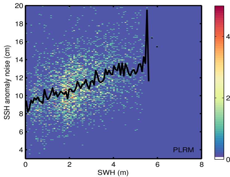
Figure 9. 2D histogram showing flag-valid SSH anomaly noise as a function of SWH for LRM (top) and PLRM (bottom) for 05/03/2017. The black line denotes the median SSH anomaly noise as a function of SWH.
