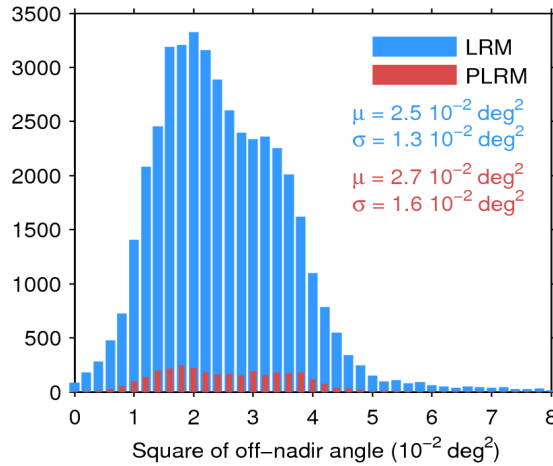
Figure 39. Histogram of flag-valid mispointing over oceans and lakes for LRM (blue) and PLRM (red) for 05/03/2017. Only positive values have been considered. The mean ( \mu ) and standard deviation ( \sigma ) are also shown. Note that values larger than 8 \cdot 10^{-2} \text{ deg}^2 are excluded from the histogram for the sake of readability but not from the computation of \mu and \sigma .
