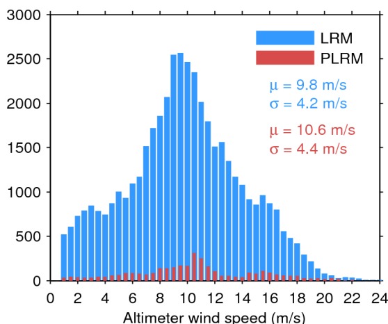
Figure 33. Histogram of flag-valid wind over oceans and lakes for LRM (blue) and PLRM (red) for 05/03/2017. The mean ( \mu ) and standard deviation ( \sigma ) are also shown. Note that values larger than 24 m/s are excluded from the histogram for the sake of readability but not from the computation of \mu and \sigma .
