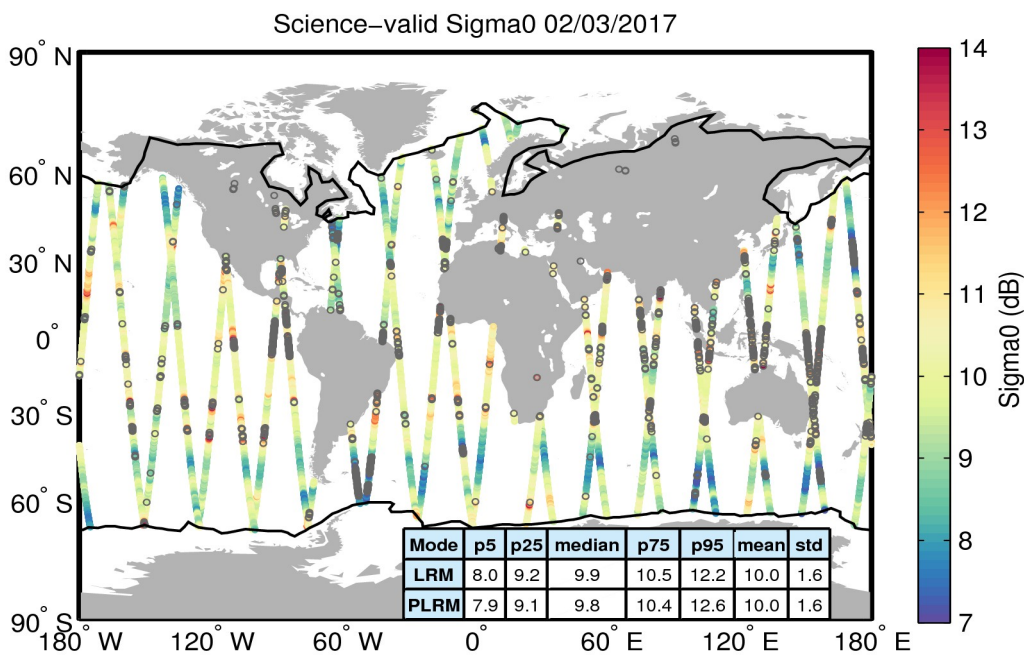
Figure 27. Geographical distribution of science-valid sigma0 data over oceans and lakes for 02/03/2017. The statistical values shown in the table refer to the sigma0 in dB and are calculated separately for LRM and PLRM regions. The black lines mark the outer limit of the Arctic and Antarctic polar polygons. Gray circles denote records that have been rejected based on the editing criteria described in Table 4.
