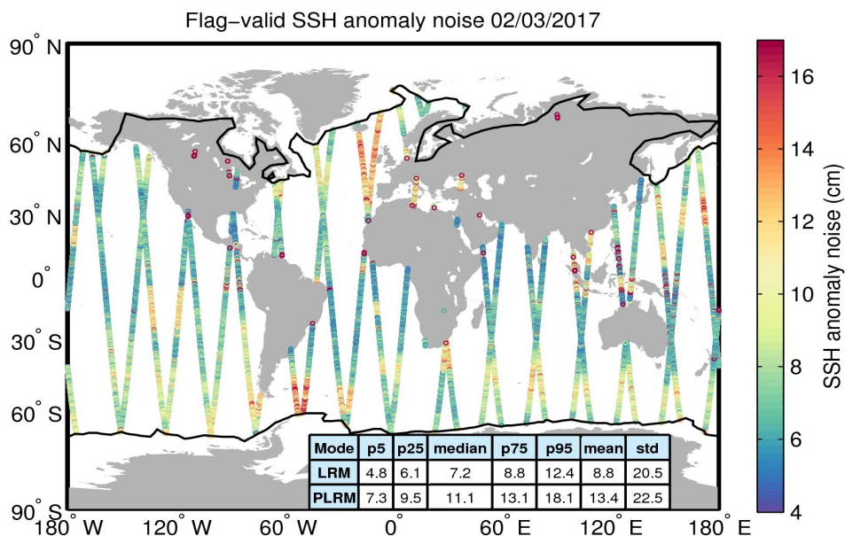
Figure 8. Geographical distribution of flag-valid 20-Hz SSH anomaly measurement noise over oceans and lakes for 02/03/2017. The statistical values shown in the table refer to the SSH anomaly noise and are calculated separately for LRM and PLRM regions. Measurements taken over polar polygons have been excluded from the computation of the statistical values. The black lines mark the outer limit of the Arctic and Antarctic polar polygons.
