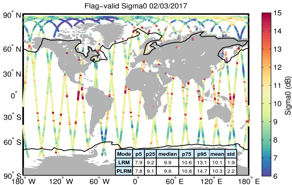
Figure 23. Geographical distribution of flag-valid sigma0 data over oceans and lakes for 02/03/2017. The statistical values shown in the table refer to the sigma0 in dB and are calculated separately for LRM and PLRM regions. Measurements taken over polar polygons have been excluded from the computation of the statistical values. The black lines mark the outer limit of the Arctic and Antarctic polar polygons.
