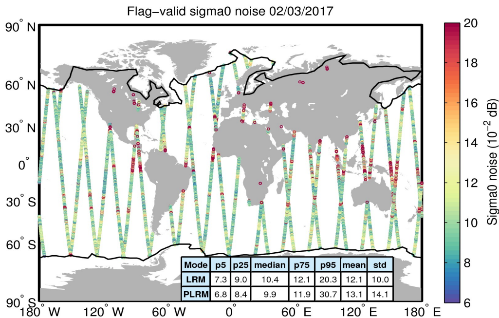
Figure 26. Geographical distribution of flag-valid 20-Hz sigma0 measurement noise over oceans and lakes for 02/03/2017. The statistical values shown in the table refer to the sigma0 noise and are calculated separately for LRM and PLRM regions. Measurements taken over polar polygons have been excluded from the computation of the statistical values. The black lines mark the outer limit of the Arctic and Antarctic polar polygons.
