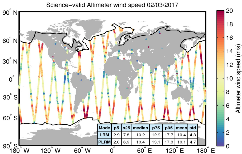
Figure 34. Geographical distribution of science-valid wind data over oceans and lakes for 02/03/2017. The statistical values shown in the table refer to the wind in m/s and are calculated separately for LRM and PLRM regions. The black lines mark the outer limit of the Arctic and Antarctic polar polygons. Gray circles denote records that have been rejected based on the editing criteria described in Table 5.
