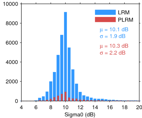
Figure 25. Histogram of flag-valid sigma0 over oceans and lakes for LRM (blue) and PLRM (red) for 02/03/2017. The mean ( \mu ) and standard deviation ( \sigma ) are also shown. Note that values outside [4 20] dB are excluded from the histogram for the sake of readability but not from the computation of \mu and \sigma .
