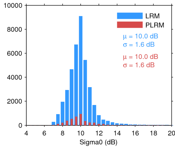
Figure 28. Histogram of science-valid sigma0 over oceans and lakes for LRM (blue) and PLRM (red) for 02/03/2017. The mean ( \mu ) and standard deviation ( \sigma ) are also shown. Note that values outside [4 20] dB are excluded from the histogram for the sake of readability but not from the computation of \mu and \sigma .
