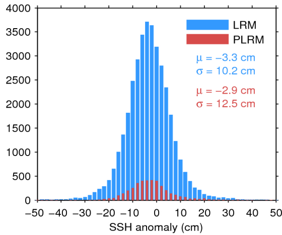
Figure 11. Histogram of science-valid SSH anomaly over oceans and lakes for LRM (blue) and PLRM (red) for 02/03/2017. The mean ( \mu ) and standard deviation ( \sigma ) are also shown. Note that values outside [-50\ 50] cm are excluded from the histogram for the sake of readability but not from the computation of \mu and \sigma .
