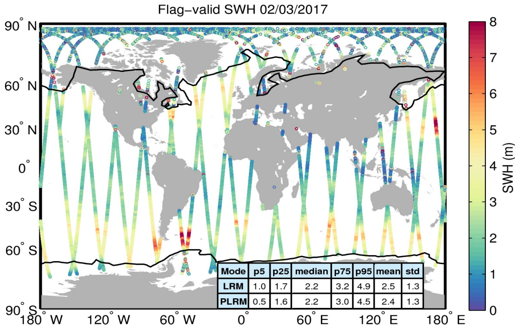
Figure 15. Geographical distribution of flag-valid SWH data over oceans and lakes for 02/03/2017. The statistical values shown in the table refer to the SWH in m and are calculated separately for LRM and PLRM regions. Measurements taken over polar polygons have been excluded from the computation of the statistical values. The black lines mark the outer limit of the Arctic and Antarctic polar polygons.
