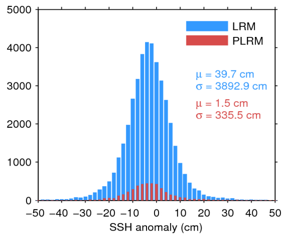
Figure 7. Histogram of flag-valid SSH anomaly over oceans and lakes for LRM (blue) and PLRM (red) for 02/03/2017. The mean ( \mu ) and standard deviation ( \sigma ) are also shown. Note that values outside [-50\ 50] cm are excluded from the histogram for the sake of readability but not from the computation of \mu and \sigma .
