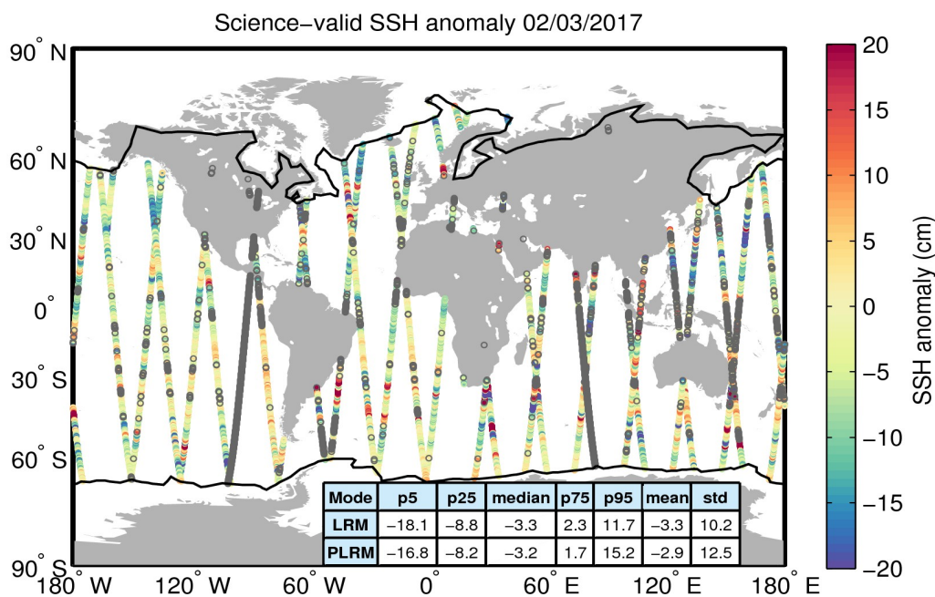
Figure 10. Geographical distribution of science-valid SSH anomaly data over oceans and lakes for 02/03/2017. The statistical values shown in the table refer to the SSH anomaly in cm and are calculated separately for LRM and PLRM regions. The black lines mark the outer limit of the Arctic and Antarctic polar polygons. Gray circles denote records that have been rejected based on the editing criteria described in Table 2.
