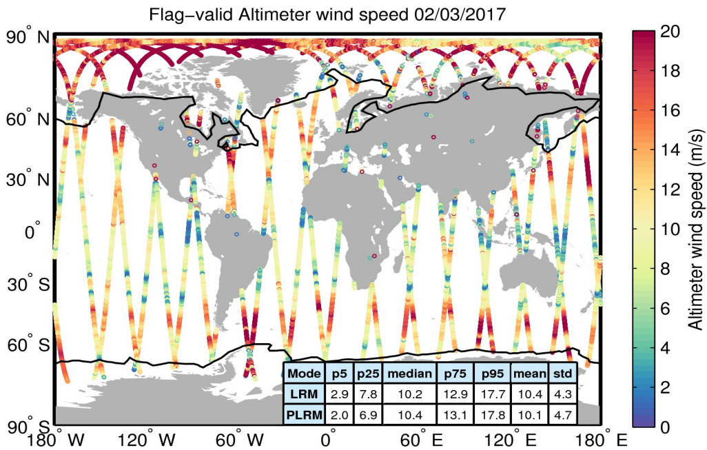
Figure 31. Geographical distribution of flag-valid wind data over oceans and lakes for 02/03/2017. The statistical values shown in the table refer to the wind in m/s and are calculated separately for LRM and PLRM regions. Measurements taken over polar polygons have been excluded from the computation of the statistical values. The black lines mark the outer limit of the Arctic and Antarctic polar polygons.
