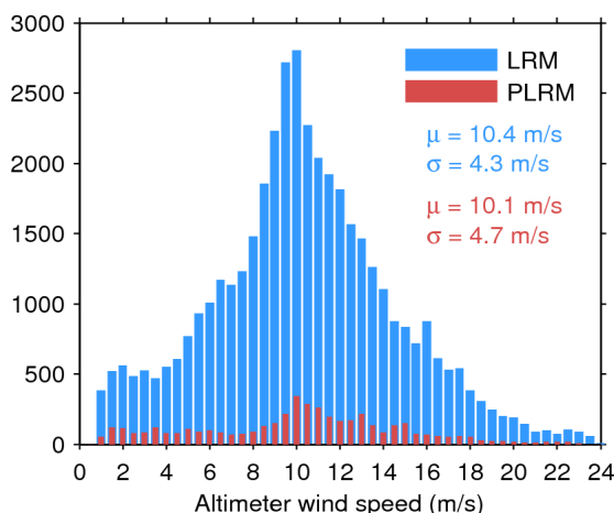
Figure 33. Histogram of flag-valid wind over oceans and lakes for LRM (blue) and PLRM (red) for 02/03/2017. The mean ( \mu ) and standard deviation ( \sigma ) are also shown. Note that values larger than 24 m/s are excluded from the histogram for the sake of readability but not from the computation of \mu and \sigma .
