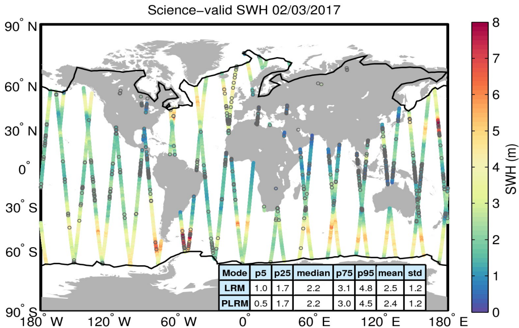
Figure 19. Geographical distribution of science-valid SWH data over oceans and lakes for 02/03/2017. The statistical values shown in the table refer to the SWH in m and are calculated separately for LRM and PLRM regions. The black lines mark the outer limit of the Arctic and Antarctic polar polygons. Gray circles denote records that have been rejected based on the editing criteria described in Table 3.
