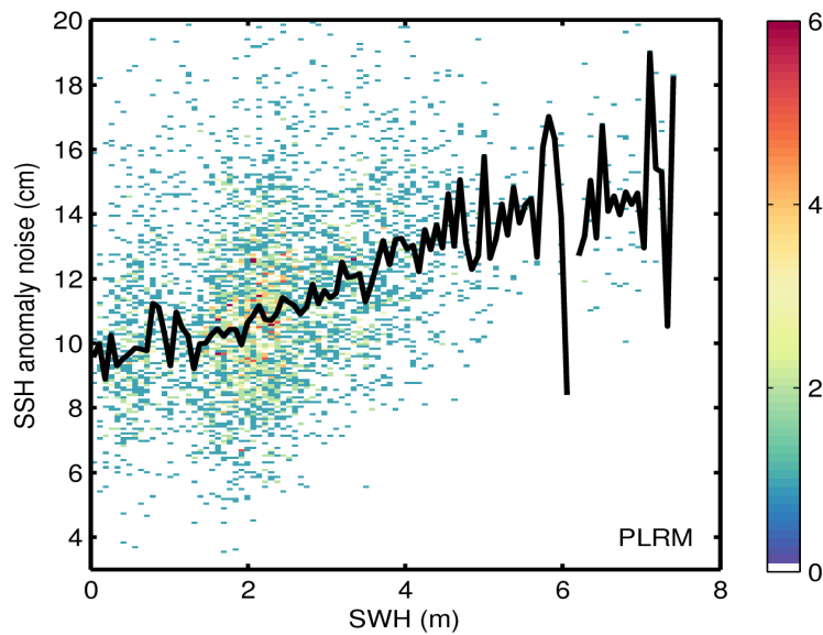
Figure 9. 2D histogram showing flag-valid SSH anomaly noise as a function of SWH for LRM (top) and PLRM (bottom) for 02/03/2017. The black line denotes the median SSH anomaly noise as a function of SWH.
