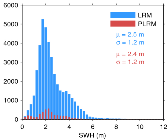
Figure 20. Histogram of science-valid SWH over oceans and lakes for LRM (blue) and PLRM (red) for 02/03/2017. The mean ( \mu ) and standard deviation ( \sigma ) are also shown. Note that values larger than 12 m are excluded from the histogram for the sake of readability but not from the computation of \mu and \sigma .
