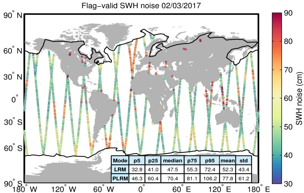
Figure 18. Geographical distribution of flag-valid 20-Hz SWH measurement noise over oceans and lakes for 02/03/2017. The statistical values shown in the table refer to the SWH noise and are calculated separately for LRM and PLRM regions. Measurements taken over polar polygons have been excluded from the computation of the statistical values. The black lines mark the outer limit of the Arctic and Antarctic polar polygons.
