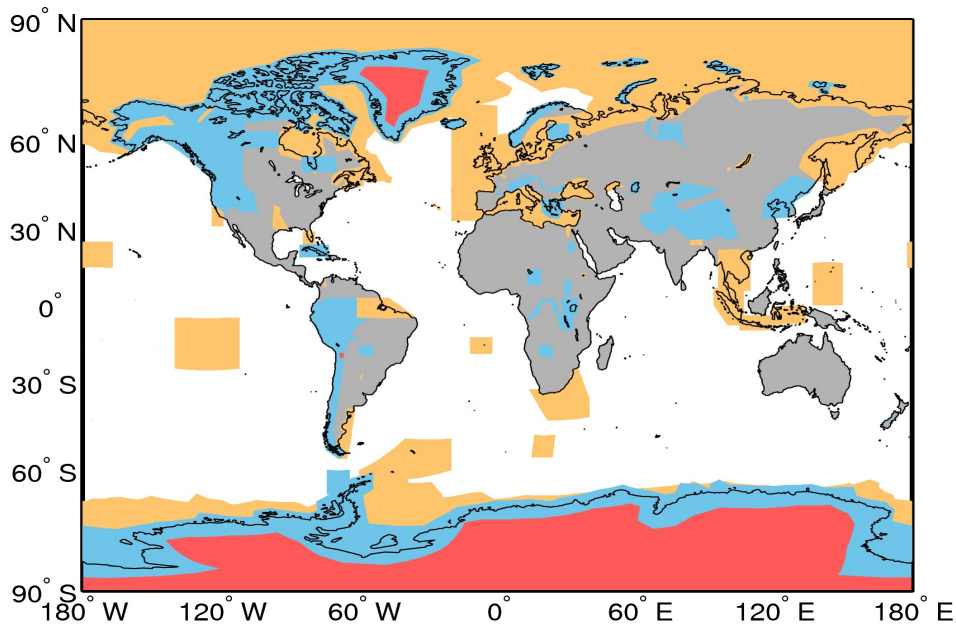
Figure A1. Extent of the regions defining the geographical mode mask for 02/03/2017. The regions where SAR, and SARIn are operated are denoted by the orange and blue polygons, respectively. LRM is operated over areas of the continental ice sheets (red polygons) and over oceans and land not covered by other modes.
