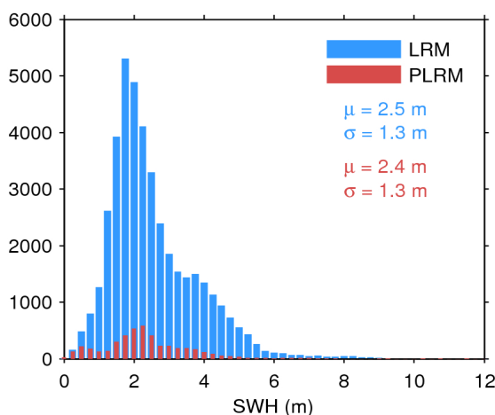
Figure 17. Histogram of flag-valid SWH over oceans and lakes for LRM (blue) and PLRM (red) for 02/03/2017. The mean ( \mu ) and standard deviation ( \sigma ) are also shown. Note that values larger than 12 m are excluded from the histogram for the sake of readability but not from the computation of \mu and \sigma .
