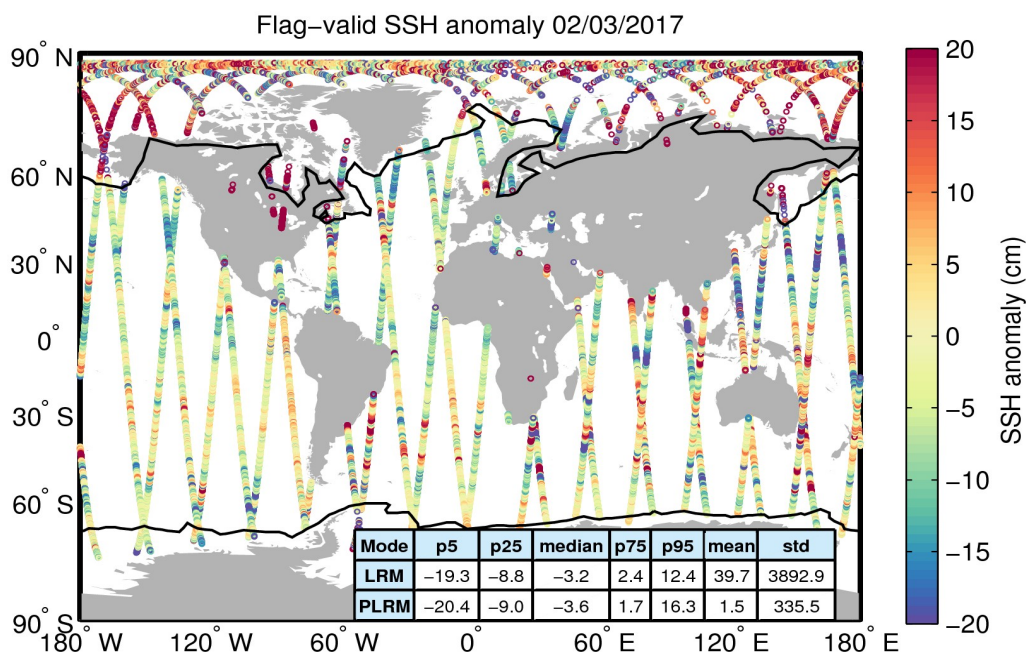
Figure 5. Geographical distribution of flag-valid 1-Hz SSH anomaly data over oceans and lakes for 02/03/2017. The statistical values shown in the table refer to the SSH anomaly in cm and are calculated separately for LRM and PLRM regions. Measurements taken over polar polygons have been excluded from the computation of the statistical values. The black lines mark the outer limit of the Arctic and Antarctic polar polygons.
