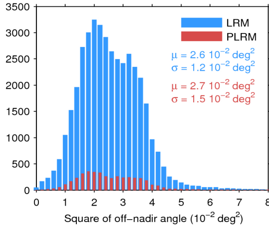
Figure 39. Histogram of flag-valid mispointing over oceans and lakes for LRM (blue) and PLRM (red) for 02/03/2017. Only positive values have been considered. The mean ( \mu ) and standard deviation ( \sigma ) are also shown. Note that values larger than 8 \cdot 10^{-2} \text{ deg}^2 are excluded from the histogram for the sake of readability but not from the computation of \mu and \sigma .
