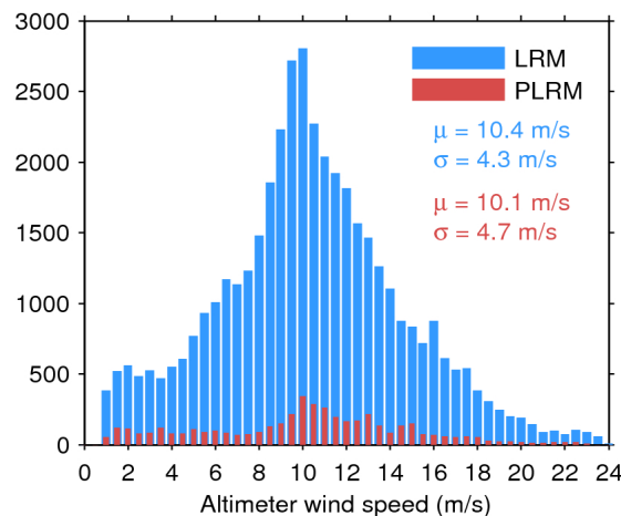
Figure 35. Histogram of science-valid wind over oceans and lakes for LRM (blue) and PLRM (red) for 02/03/2017. The mean ( \mu ) and standard deviation ( \sigma ) are also shown. Note that values larger than 24 m/s are excluded from the histogram for the sake of readability but not from the computation of \mu and \sigma .
