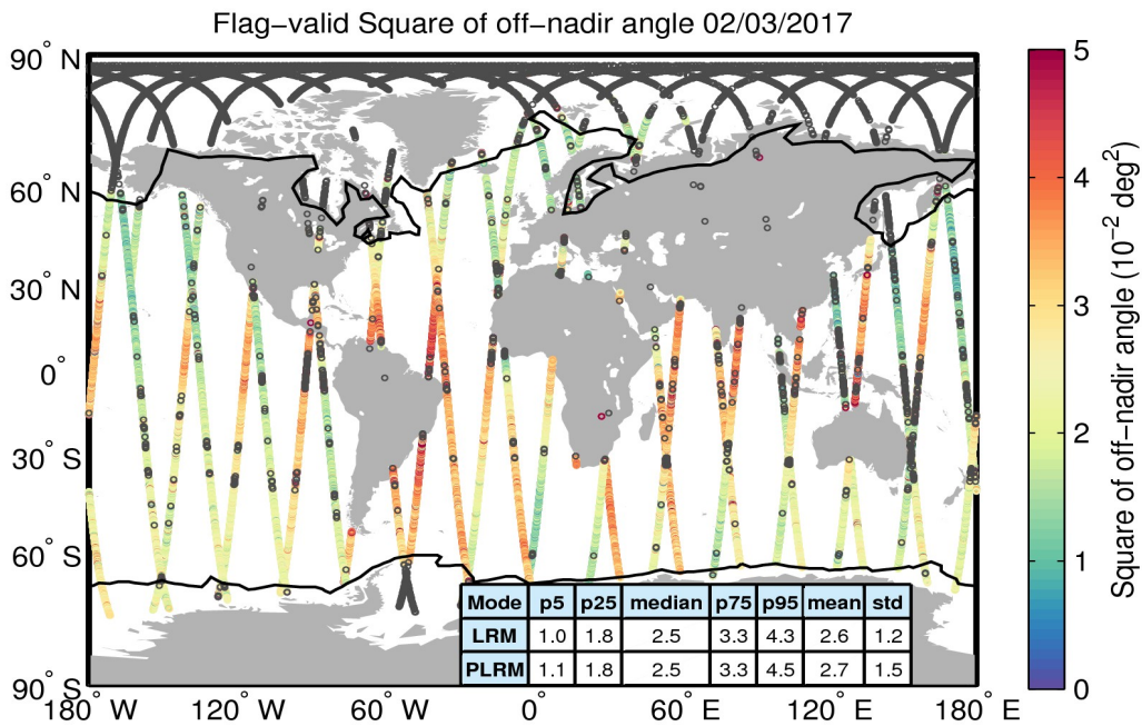
Figure 37. Geographical distribution of flag-valid mispointing data over oceans and lakes for 02/03/2017. The statistical values shown in the table refer to the mispointing in 10^{-2} deg 2 and are calculated separately for LRM and PLRM regions. Measurements taken over polar polygons have been excluded from the computation of the statistical values. The black lines mark the outer limit of the Arctic and Antarctic polar polygons. Gray circles denote negative values.
