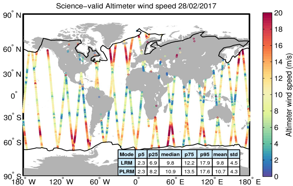
Figure 34. Geographical distribution of science-valid wind data over oceans and lakes for 28/02/2017. The statistical values shown in the table refer to the wind in m/s and are calculated separately for LRM and PLRM regions. The black lines mark the outer limit of the Arctic and Antarctic polar polygons. Gray circles denote records that have been rejected based on the editing criteria described in Table 5.
