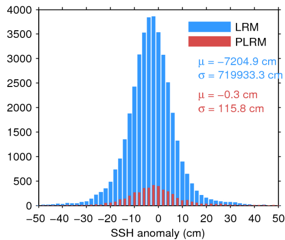
Figure 7. Histogram of flag-valid SSH anomaly over oceans and lakes for LRM (blue) and PLRM (red) for 28/02/2017. The mean ( \mu ) and standard deviation ( \sigma ) are also shown. Note that values outside [-50\ 50] cm are excluded from the histogram for the sake of readability but not from the computation of \mu and \sigma .
