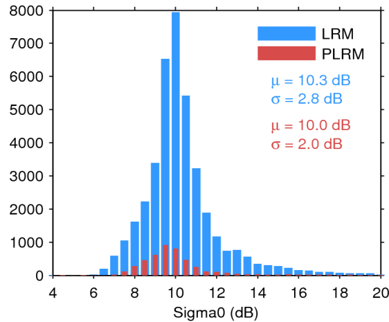
Figure 25. Histogram of flag-valid sigma0 over oceans and lakes for LRM (blue) and PLRM (red) for 28/02/2017. The mean ( \mu ) and standard deviation ( \sigma ) are also shown. Note that values outside [4 20] dB are excluded from the histogram for the sake of readability but not from the computation of \mu and \sigma .
