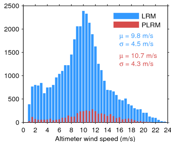
Figure 35. Histogram of science-valid wind over oceans and lakes for LRM (blue) and PLRM (red) for 28/02/2017. The mean ( \mu ) and standard deviation ( \sigma ) are also shown. Note that values larger than 24 m/s are excluded from the histogram for the sake of readability but not from the computation of \mu and \sigma .
