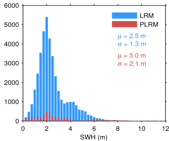
Figure 17. Histogram of flag-valid SWH over oceans and lakes for LRM (blue) and PLRM (red) for 28/02/2017. The mean ( \mu ) and standard deviation ( \sigma ) are also shown. Note that values larger than 12 m are excluded from the histogram for the sake of readability but not from the computation of \mu and \sigma .
