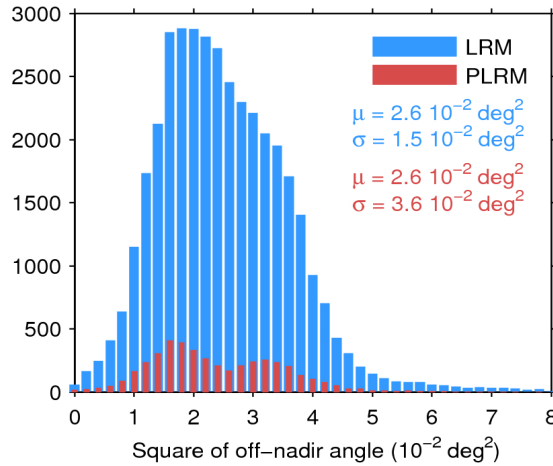
Figure 39. Histogram of flag-valid mispointing over oceans and lakes for LRM (blue) and PLRM (red) for 28/02/2017. Only positive values have been considered. The mean ( \mu ) and standard deviation ( \sigma ) are also shown. Note that values larger than 8 \cdot 10^{-2} \text{ deg}^2 are excluded from the histogram for the sake of readability but not from the computation of \mu and \sigma .
