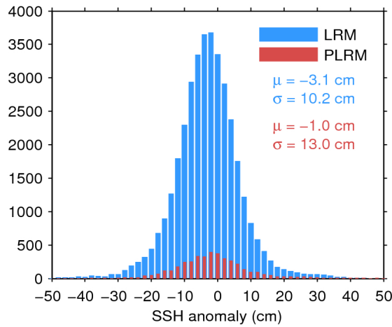
Figure 11. Histogram of science-valid SSH anomaly over oceans and lakes for LRM (blue) and PLRM (red) for 28/02/2017. The mean ( \mu ) and standard deviation ( \sigma ) are also shown. Note that values outside [-50 50] cm are excluded from the histogram for the sake of readability but not from the computation of \mu and \sigma .
