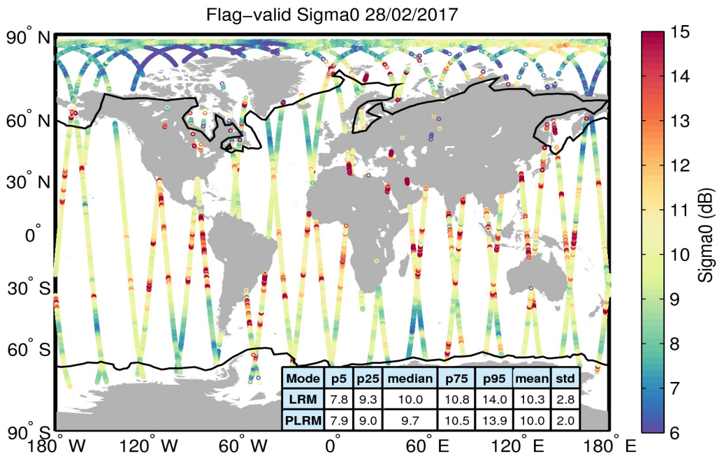
Figure 23. Geographical distribution of flag-valid sigma0 data over oceans and lakes for 28/02/2017. The statistical values shown in the table refer to the sigma0 in dB and are calculated separately for LRM and PLRM regions. Measurements taken over polar polygons have been excluded from the computation of the statistical values. The black lines mark the outer limit of the Arctic and Antarctic polar polygons.
