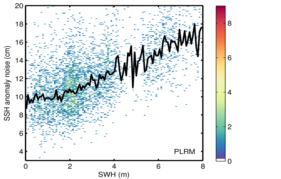
Figure 9. 2D histogram showing flag-valid SSH anomaly noise as a function of SWH for LRM (top) and PLRM (bottom) for 28/02/2017. The black line denotes the median SSH anomaly noise as a function of SWH.
