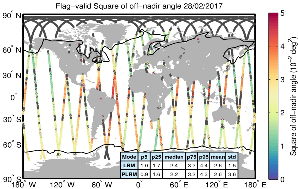
Figure 37. Geographical distribution of flag-valid mispointing data over oceans and lakes for 28/02/2017. The statistical values shown in the table refer to the mispointing in 10^{-2} deg 2 and are calculated separately for LRM and PLRM regions. Measurements taken over polar polygons have been excluded from the computation of the statistical values. The black lines mark the outer limit of the Arctic and Antarctic polar polygons. Gray circles denote negative values.
