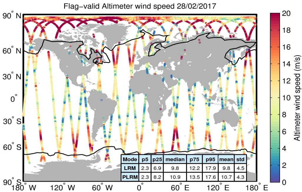
Figure 31. Geographical distribution of flag-valid wind data over oceans and lakes for 28/02/2017. The statistical values shown in the table refer to the wind in m/s and are calculated separately for LRM and PLRM regions. Measurements taken over polar polygons have been excluded from the computation of the statistical values. The black lines mark the outer limit of the Arctic and Antarctic polar polygons.
