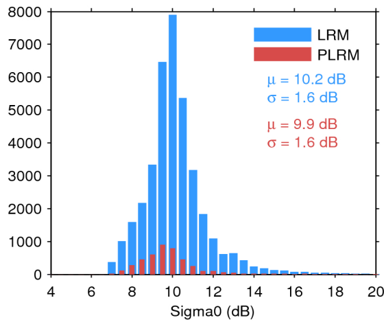
Figure 28. Histogram of science-valid sigma0 over oceans and lakes for LRM (blue) and PLRM (red) for 28/02/2017. The mean ( \mu ) and standard deviation ( \sigma ) are also shown. Note that values outside [4 20] dB are excluded from the histogram for the sake of readability but not from the computation of \mu and \sigma .
