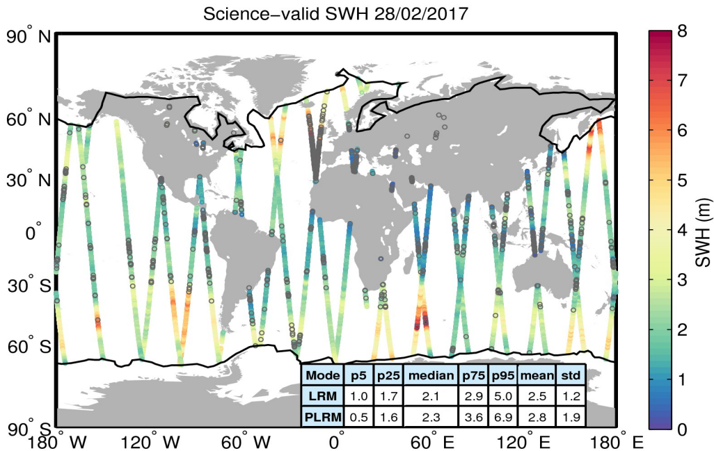
Figure 19. Geographical distribution of science-valid SWH data over oceans and lakes for 28/02/2017. The statistical values shown in the table refer to the SWH in m and are calculated separately for LRM and PLRM regions. The black lines mark the outer limit of the Arctic and Antarctic polar polygons. Gray circles denote records that have been rejected based on the editing criteria described in Table 3.
