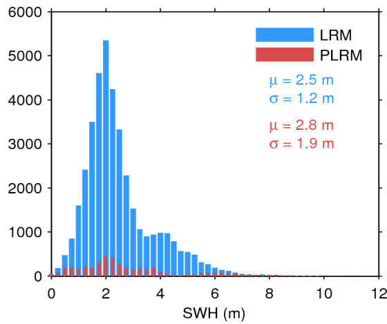
Figure 20. Histogram of science-valid SWH over oceans and lakes for LRM (blue) and PLRM (red) for 28/02/2017. The mean ( \mu ) and standard deviation ( \sigma ) are also shown. Note that values larger than 12 m are excluded from the histogram for the sake of readability but not from the computation of \mu and \sigma .
