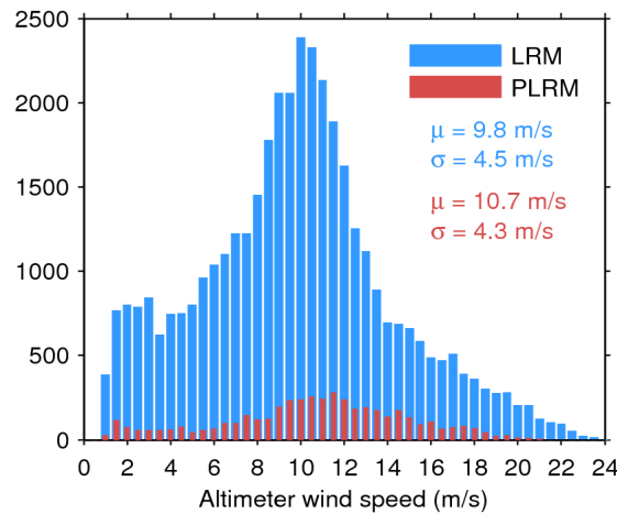
Figure 33. Histogram of flag-valid wind over oceans and lakes for LRM (blue) and PLRM (red) for 28/02/2017. The mean ( \mu ) and standard deviation ( \sigma ) are also shown. Note that values larger than 24 m/s are excluded from the histogram for the sake of readability but not from the computation of \mu and \sigma .
