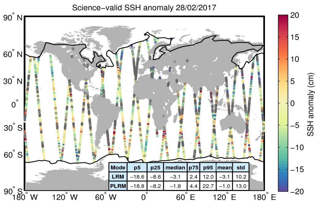
Figure 10. Geographical distribution of science-valid SSH anomaly data over oceans and lakes for 28/02/2017. The statistical values shown in the table refer to the SSH anomaly in cm and are calculated separately for LRM and PLRM regions. The black lines mark the outer limit of the Arctic and Antarctic polar polygons. Gray circles denote records that have been rejected based on the editing criteria described in Table 2.
