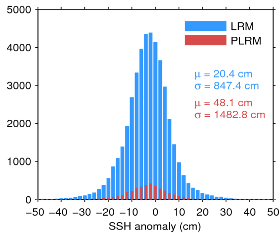
Figure 7. Histogram of flag-valid SSH anomaly over oceans and lakes for LRM (blue) and PLRM (red) for 27/02/2017. The mean ( \mu ) and standard deviation ( \sigma ) are also shown. Note that values outside [-50 50] cm are excluded from the histogram for the sake of readability but not from the computation of \mu and \sigma .
