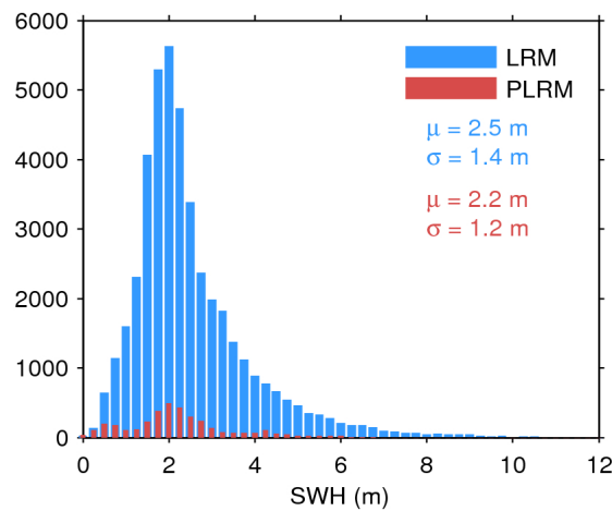
Figure 20. Histogram of science-valid SWH over oceans and lakes for LRM (blue) and PLRM (red) for 27/02/2017. The mean ( \mu ) and standard deviation ( \sigma ) are also shown. Note that values larger than 12 m are excluded from the histogram for the sake of readability but not from the computation of \mu and \sigma .
