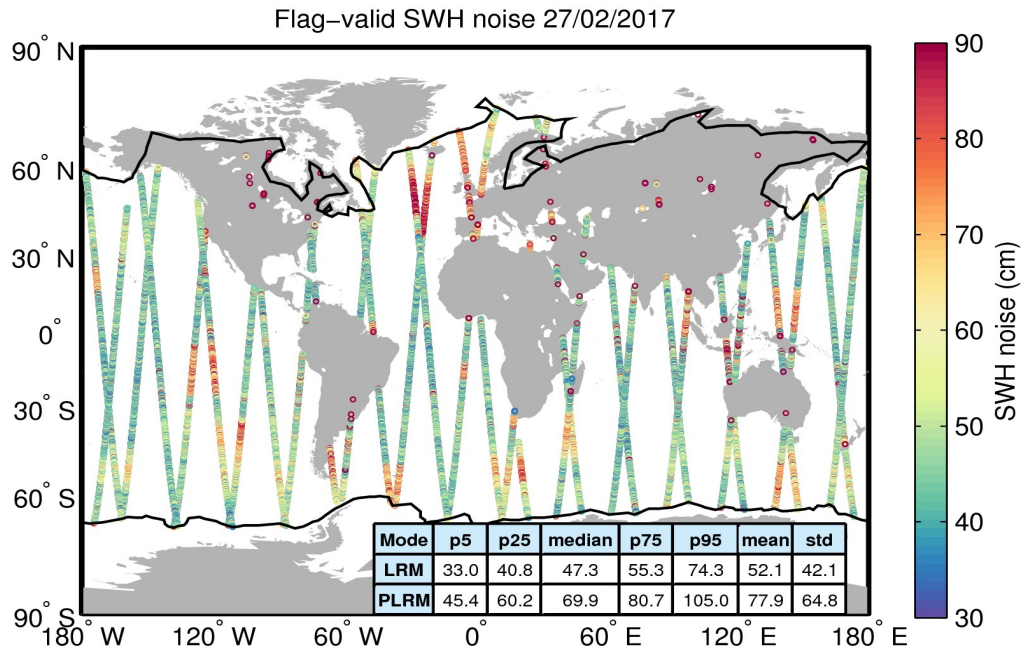
Figure 18. Geographical distribution of flag-valid 20-Hz SWH measurement noise over oceans and lakes for 27/02/2017. The statistical values shown in the table refer to the SWH noise and are calculated separately for LRM and PLRM regions. Measurements taken over polar polygons have been excluded from the computation of the statistical values. The black lines mark the outer limit of the Arctic and Antarctic polar polygons.
