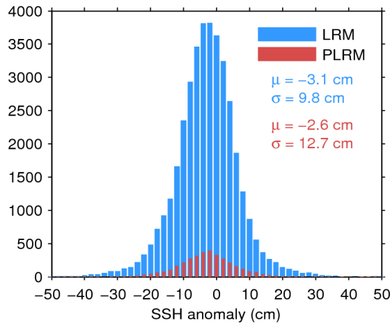
Figure 11. Histogram of science-valid SSH anomaly over oceans and lakes for LRM (blue) and PLRM (red) for 27/02/2017. The mean ( \mu ) and standard deviation ( \sigma ) are also shown. Note that values outside [-50 50] cm are excluded from the histogram for the sake of readability but not from the computation of \mu and \sigma .
