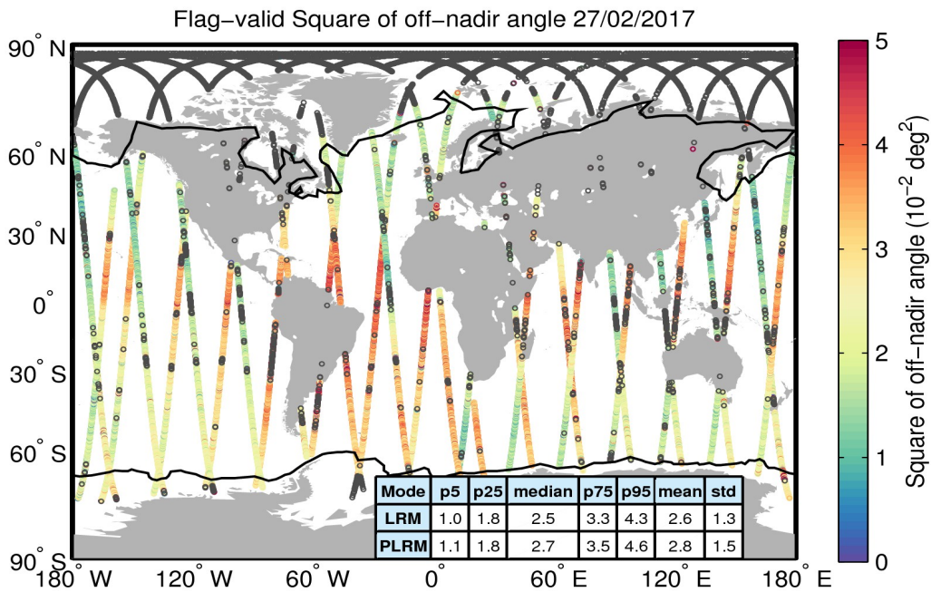
Figure 37. Geographical distribution of flag-valid mispointing data over oceans and lakes for 27/02/2017. The statistical values shown in the table refer to the mispointing in 10^{-2} deg 2 and are calculated separately for LRM and PLRM regions. Measurements taken over polar polygons have been excluded from the computation of the statistical values. The black lines mark the outer limit of the Arctic and Antarctic polar polygons. Gray circles denote negative values.
