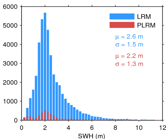
Figure 17. Histogram of flag-valid SWH over oceans and lakes for LRM (blue) and PLRM (red) for 27/02/2017. The mean ( \mu ) and standard deviation ( \sigma ) are also shown. Note that values larger than 12 m are excluded from the histogram for the sake of readability but not from the computation of \mu and \sigma .
