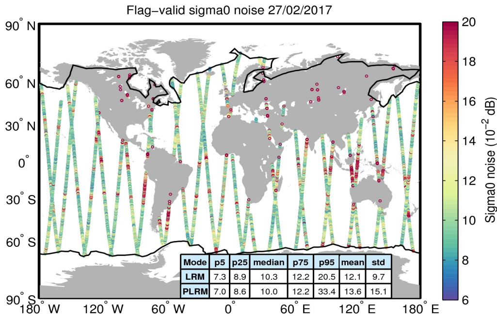
Figure 26. Geographical distribution of flag-valid 20-Hz sigma0 measurement noise over oceans and lakes for 27/02/2017. The statistical values shown in the table refer to the sigma0 noise and are calculated separately for LRM and PLRM regions. Measurements taken over polar polygons have been excluded from the computation of the statistical values. The black lines mark the outer limit of the Arctic and Antarctic polar polygons.
