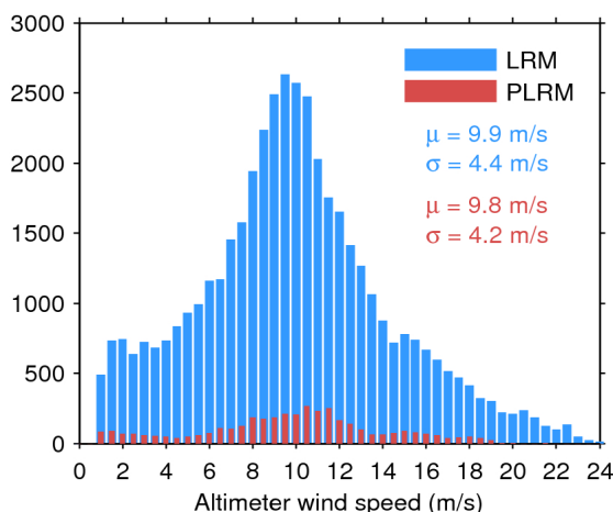
Figure 33. Histogram of flag-valid wind over oceans and lakes for LRM (blue) and PLRM (red) for 27/02/2017. The mean ( \mu ) and standard deviation ( \sigma ) are also shown. Note that values larger than 24 m/s are excluded from the histogram for the sake of readability but not from the computation of \mu and \sigma .
