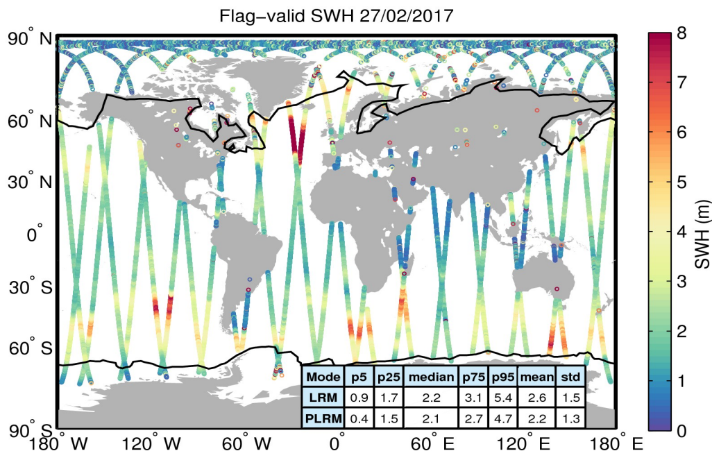
Figure 15. Geographical distribution of flag-valid SWH data over oceans and lakes for 27/02/2017. The statistical values shown in the table refer to the SWH in m and are calculated separately for LRM and PLRM regions. Measurements taken over polar polygons have been excluded from the computation of the statistical values. The black lines mark the outer limit of the Arctic and Antarctic polar polygons.
