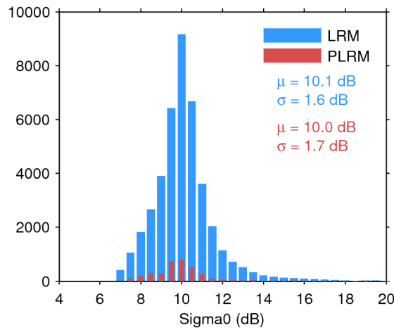
Figure 28. Histogram of science-valid sigma0 over oceans and lakes for LRM (blue) and PLRM (red) for 27/02/2017. The mean ( \mu ) and standard deviation ( \sigma ) are also shown. Note that values outside [4 20] dB are excluded from the histogram for the sake of readability but not from the computation of \mu and \sigma .
