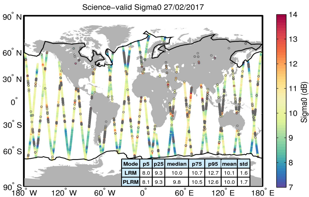
Figure 27. Geographical distribution of science-valid sigma0 data over oceans and lakes for 27/02/2017. The statistical values shown in the table refer to the sigma0 in dB and are calculated separately for LRM and PLRM regions. The black lines mark the outer limit of the Arctic and Antarctic polar polygons. Gray circles denote records that have been rejected based on the editing criteria described in Table 4.
