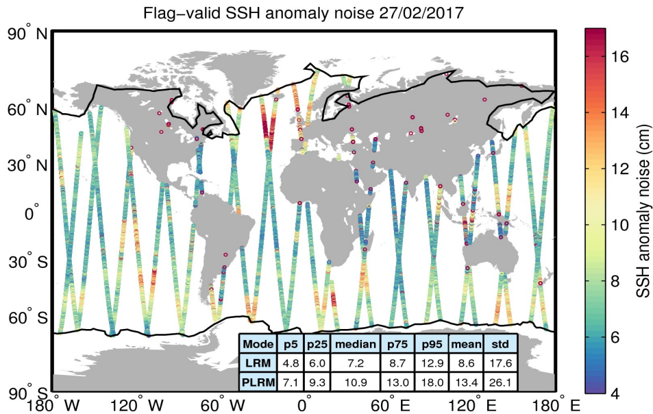
Figure 8. Geographical distribution of flag-valid 20-Hz SSH anomaly measurement noise over oceans and lakes for 27/02/2017. The statistical values shown in the table refer to the SSH anomaly noise and are calculated separately for LRM and PLRM regions. Measurements taken over polar polygons have been excluded from the computation of the statistical values. The black lines mark the outer limit of the Arctic and Antarctic polar polygons.
