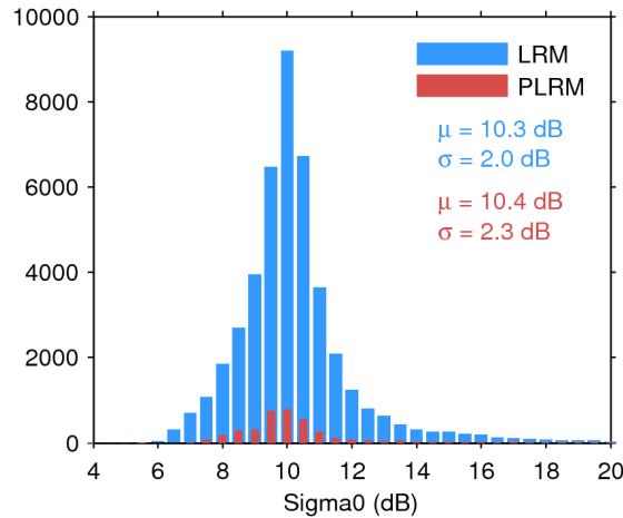
Figure 25. Histogram of flag-valid sigma0 over oceans and lakes for LRM (blue) and PLRM (red) for 27/02/2017. The mean ( \mu ) and standard deviation ( \sigma ) are also shown. Note that values outside [4 20] dB are excluded from the histogram for the sake of readability but not from the computation of \mu and \sigma .
