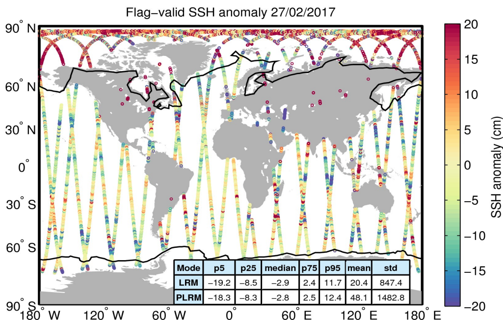
Figure 5. Geographical distribution of flag-valid 1-Hz SSH anomaly data over oceans and lakes for 27/02/2017. The statistical values shown in the table refer to the SSH anomaly in cm and are calculated separately for LRM and PLRM regions. Measurements taken over polar polygons have been excluded from the computation of the statistical values. The black lines mark the outer limit of the Arctic and Antarctic polar polygons.
