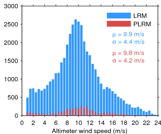
Figure 35. Histogram of science-valid wind over oceans and lakes for LRM (blue) and PLRM (red) for 27/02/2017. The mean ( \mu ) and standard deviation ( \sigma ) are also shown. Note that values larger than 24 m/s are excluded from the histogram for the sake of readability but not from the computation of \mu and \sigma .
