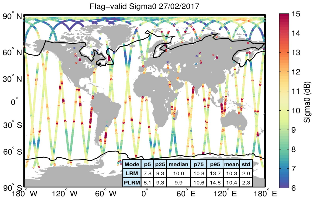
Figure 23. Geographical distribution of flag-valid sigma0 data over oceans and lakes for 27/02/2017. The statistical values shown in the table refer to the sigma0 in dB and are calculated separately for LRM and PLRM regions. Measurements taken over polar polygons have been excluded from the computation of the statistical values. The black lines mark the outer limit of the Arctic and Antarctic polar polygons.
