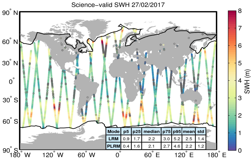
Figure 19. Geographical distribution of science-valid SWH data over oceans and lakes for 27/02/2017. The statistical values shown in the table refer to the SWH in m and are calculated separately for LRM and PLRM regions. The black lines mark the outer limit of the Arctic and Antarctic polar polygons. Gray circles denote records that have been rejected based on the editing criteria described in Table 3.
