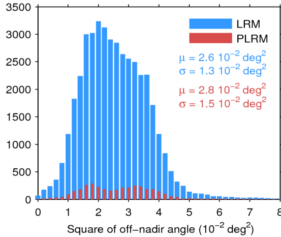
Figure 39. Histogram of flag-valid mispointing over oceans and lakes for LRM (blue) and PLRM (red) for 27/02/2017. Only positive values have been considered. The mean ( \mu ) and standard deviation ( \sigma ) are also shown. Note that values larger than 8 \cdot 10^{-2} \text{ deg}^2 are excluded from the histogram for the sake of readability but not from the computation of \mu and \sigma .
