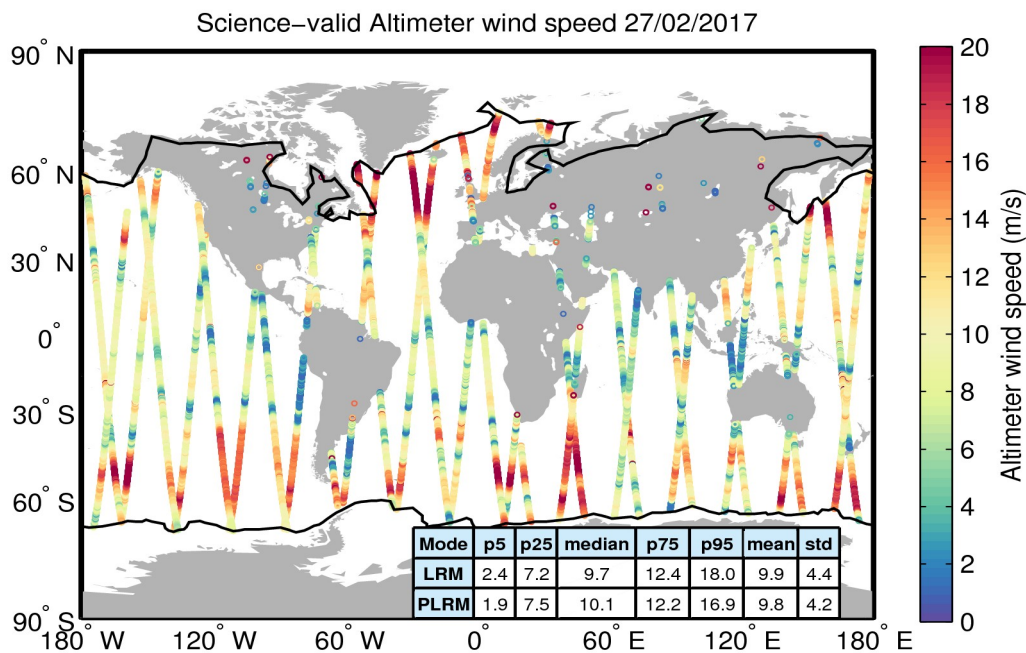
Figure 34. Geographical distribution of science-valid wind data over oceans and lakes for 27/02/2017. The statistical values shown in the table refer to the wind in m/s and are calculated separately for LRM and PLRM regions. The black lines mark the outer limit of the Arctic and Antarctic polar polygons. Gray circles denote records that have been rejected based on the editing criteria described in Table 5.
