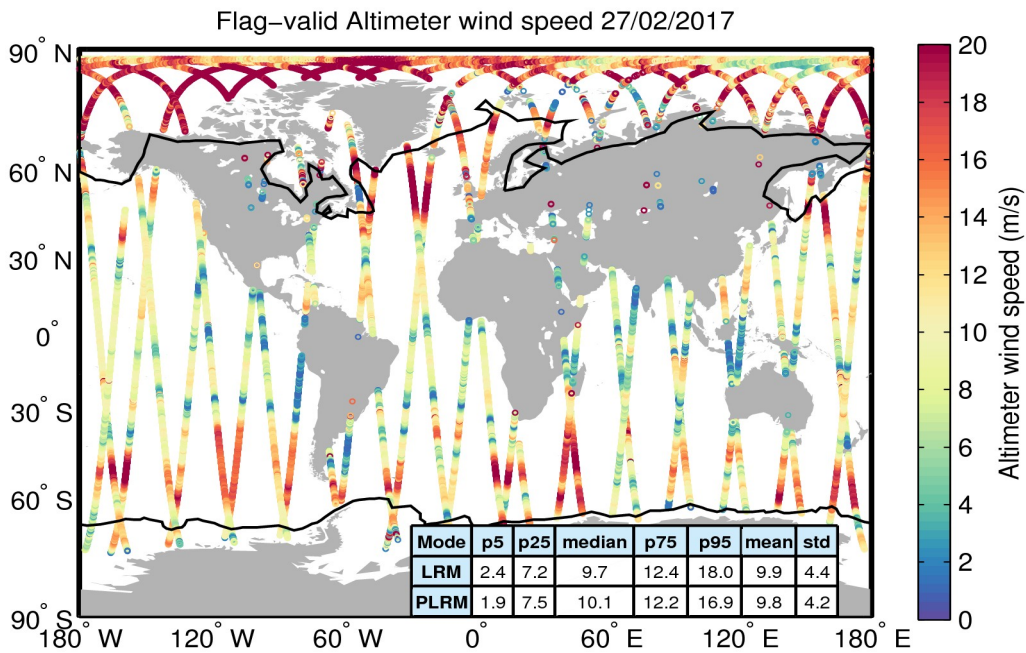
Figure 31. Geographical distribution of flag-valid wind data over oceans and lakes for 27/02/2017. The statistical values shown in the table refer to the wind in m/s and are calculated separately for LRM and PLRM regions. Measurements taken over polar polygons have been excluded from the computation of the statistical values. The black lines mark the outer limit of the Arctic and Antarctic polar polygons.
