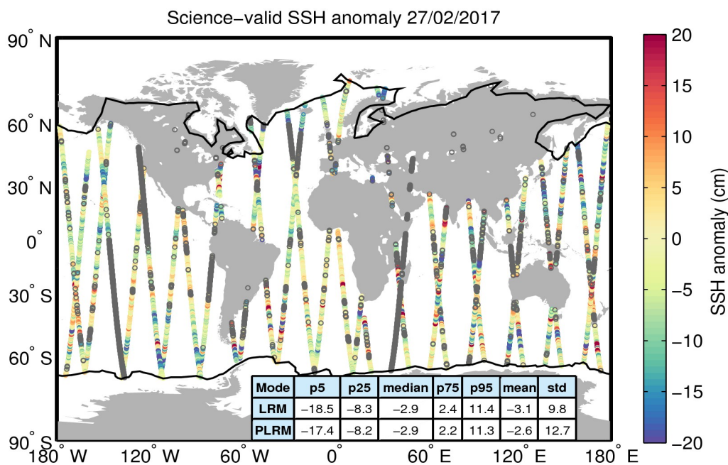
Figure 10. Geographical distribution of science-valid SSH anomaly data over oceans and lakes for 27/02/2017. The statistical values shown in the table refer to the SSH anomaly in cm and are calculated separately for LRM and PLRM regions. The black lines mark the outer limit of the Arctic and Antarctic polar polygons. Gray circles denote records that have been rejected based on the editing criteria described in Table 2.
