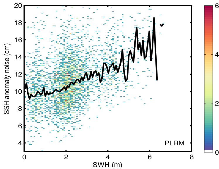
Figure 9. 2D histogram showing flag-valid SSH anomaly noise as a function of SWH for LRM (top) and PLRM (bottom) for 27/02/2017. The black line denotes the median SSH anomaly noise as a function of SWH.
