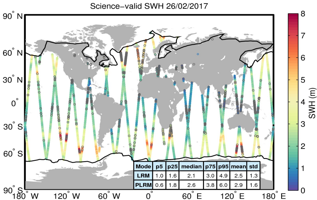
Figure 19. Geographical distribution of science-valid SWH data over oceans and lakes for 26/02/2017. The statistical values shown in the table refer to the SWH in m and are calculated separately for LRM and PLRM regions. The black lines mark the outer limit of the Arctic and Antarctic polar polygons. Gray circles denote records that have been rejected based on the editing criteria described in Table 3.
