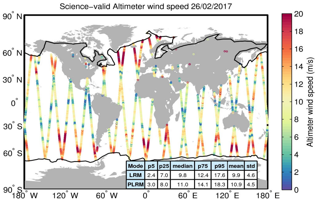
Figure 34. Geographical distribution of science-valid wind data over oceans and lakes for 26/02/2017. The statistical values shown in the table refer to the wind in m/s and are calculated separately for LRM and PLRM regions. The black lines mark the outer limit of the Arctic and Antarctic polar polygons. Gray circles denote records that have been rejected based on the editing criteria described in Table 5.
