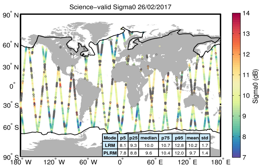
Figure 27. Geographical distribution of science-valid sigma0 data over oceans and lakes for 26/02/2017. The statistical values shown in the table refer to the sigma0 in dB and are calculated separately for LRM and PLRM regions. The black lines mark the outer limit of the Arctic and Antarctic polar polygons. Gray circles denote records that have been rejected based on the editing criteria described in Table 4.
