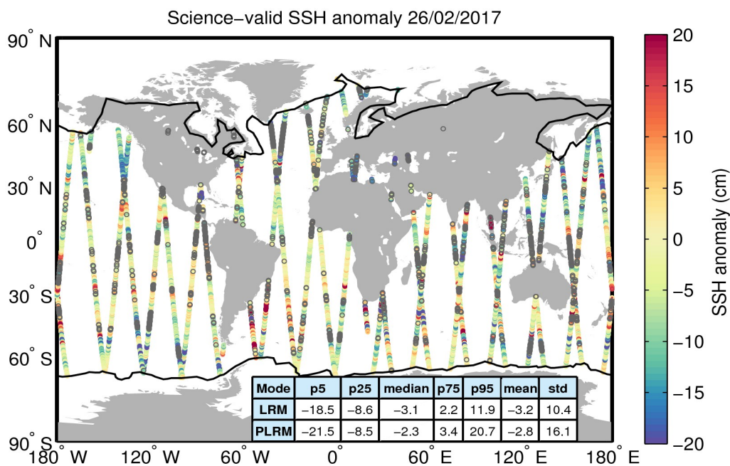
Figure 10. Geographical distribution of science-valid SSH anomaly data over oceans and lakes for 26/02/2017. The statistical values shown in the table refer to the SSH anomaly in cm and are calculated separately for LRM and PLRM regions. The black lines mark the outer limit of the Arctic and Antarctic polar polygons. Gray circles denote records that have been rejected based on the editing criteria described in Table 2.
