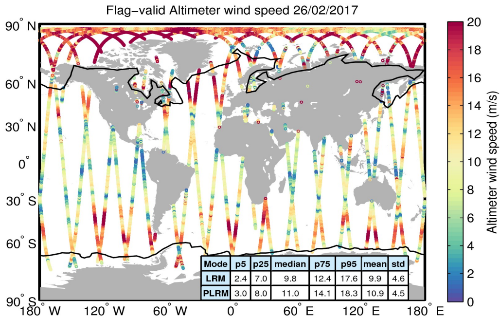
Figure 31. Geographical distribution of flag-valid wind data over oceans and lakes for 26/02/2017. The statistical values shown in the table refer to the wind in m/s and are calculated separately for LRM and PLRM regions. Measurements taken over polar polygons have been excluded from the computation of the statistical values. The black lines mark the outer limit of the Arctic and Antarctic polar polygons.
