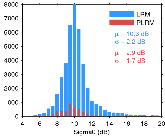
Figure 25. Histogram of flag-valid sigma0 over oceans and lakes for LRM (blue) and PLRM (red) for 26/02/2017. The mean ( \mu ) and standard deviation ( \sigma ) are also shown. Note that values outside [4 20] dB are excluded from the histogram for the sake of readability but not from the computation of \mu and \sigma .
