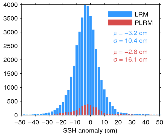
Figure 11. Histogram of science-valid SSH anomaly over oceans and lakes for LRM (blue) and PLRM (red) for 26/02/2017. The mean ( \mu ) and standard deviation ( \sigma ) are also shown. Note that values outside [-50 50] cm are excluded from the histogram for the sake of readability but not from the computation of \mu and \sigma .
