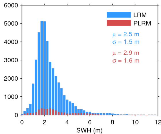
Figure 17. Histogram of flag-valid SWH over oceans and lakes for LRM (blue) and PLRM (red) for 26/02/2017. The mean ( \mu ) and standard deviation ( \sigma ) are also shown. Note that values larger than 12 m are excluded from the histogram for the sake of readability but not from the computation of \mu and \sigma .
