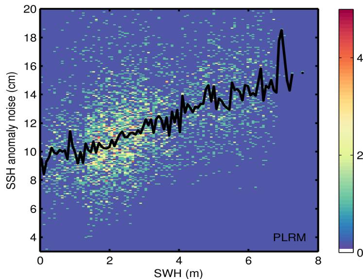
Figure 9. 2D histogram showing flag-valid SSH anomaly noise as a function of SWH for LRM (top) and PLRM (bottom) for 26/02/2017. The black line denotes the median SSH anomaly noise as a function of SWH.
