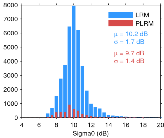
Figure 28. Histogram of science-valid sigma0 over oceans and lakes for LRM (blue) and PLRM (red) for 26/02/2017. The mean ( \mu ) and standard deviation ( \sigma ) are also shown. Note that values outside [4 20] dB are excluded from the histogram for the sake of readability but not from the computation of \mu and \sigma .
