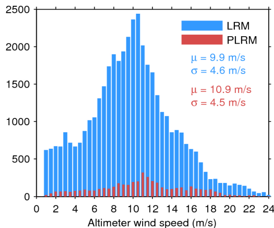
Figure 35. Histogram of science-valid wind over oceans and lakes for LRM (blue) and PLRM (red) for 26/02/2017. The mean ( \mu ) and standard deviation ( \sigma ) are also shown. Note that values larger than 24 m/s are excluded from the histogram for the sake of readability but not from the computation of \mu and \sigma .
