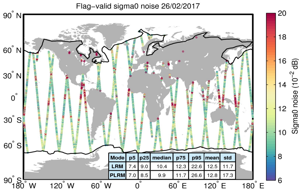
Figure 26. Geographical distribution of flag-valid 20-Hz sigma0 measurement noise over oceans and lakes for 26/02/2017. The statistical values shown in the table refer to the sigma0 noise and are calculated separately for LRM and PLRM regions. Measurements taken over polar polygons have been excluded from the computation of the statistical values. The black lines mark the outer limit of the Arctic and Antarctic polar polygons.
