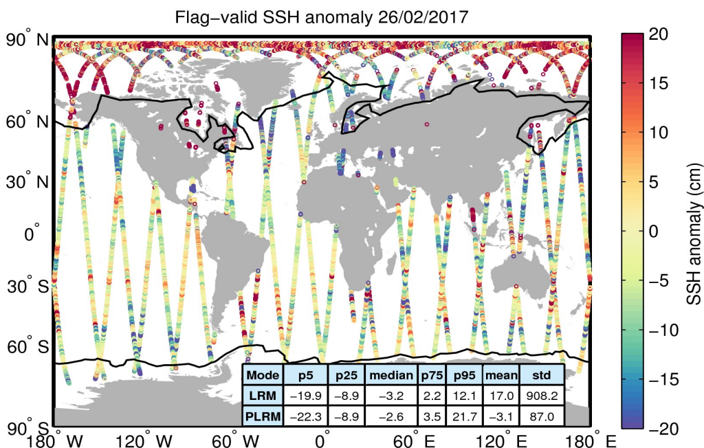
Figure 5. Geographical distribution of flag-valid 1-Hz SSH anomaly data over oceans and lakes for 26/02/2017. The statistical values shown in the table refer to the SSH anomaly in cm and are calculated separately for LRM and PLRM regions. Measurements taken over polar polygons have been excluded from the computation of the statistical values. The black lines mark the outer limit of the Arctic and Antarctic polar polygons.
