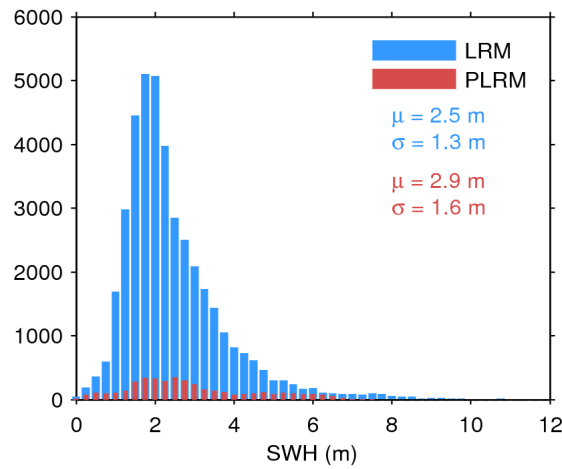
Figure 20. Histogram of science-valid SWH over oceans and lakes for LRM (blue) and PLRM (red) for 26/02/2017. The mean ( \mu ) and standard deviation ( \sigma ) are also shown. Note that values larger than 12 m are excluded from the histogram for the sake of readability but not from the computation of \mu and \sigma .
