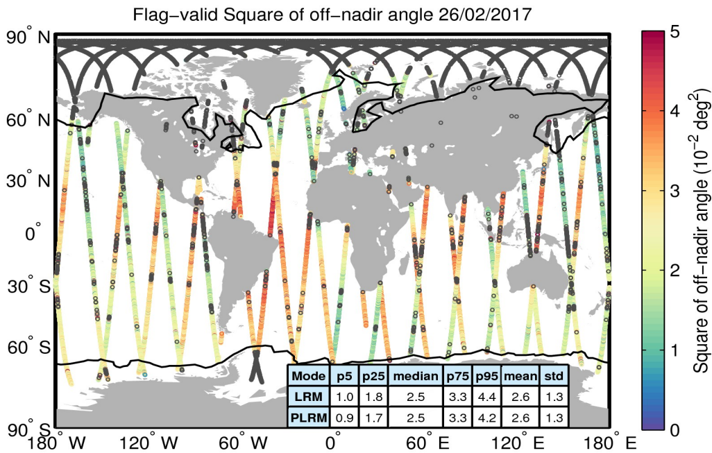
Figure 37. Geographical distribution of flag-valid mispointing data over oceans and lakes for 26/02/2017. The statistical values shown in the table refer to the mispointing in 10^{-2} deg 2 and are calculated separately for LRM and PLRM regions. Measurements taken over polar polygons have been excluded from the computation of the statistical values. The black lines mark the outer limit of the Arctic and Antarctic polar polygons. Gray circles denote negative values.
