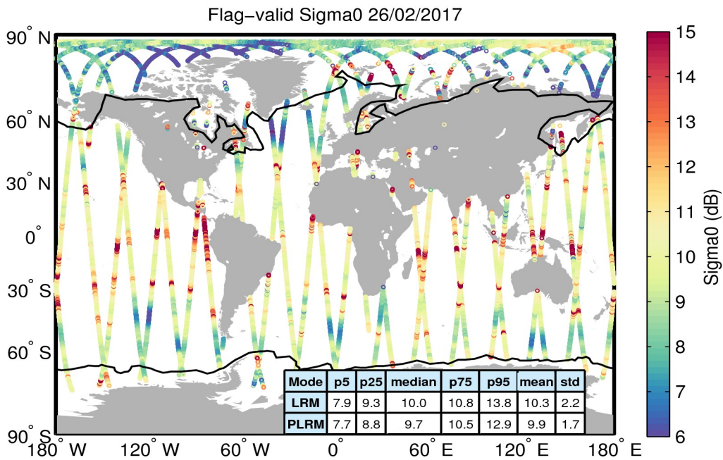
Figure 23. Geographical distribution of flag-valid sigma0 data over oceans and lakes for 26/02/2017. The statistical values shown in the table refer to the sigma0 in dB and are calculated separately for LRM and PLRM regions. Measurements taken over polar polygons have been excluded from the computation of the statistical values. The black lines mark the outer limit of the Arctic and Antarctic polar polygons.
