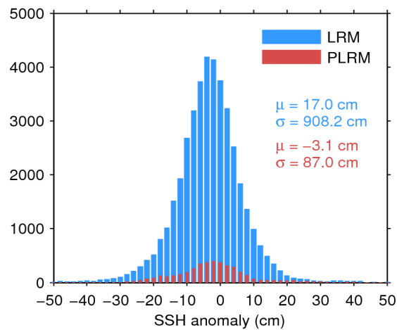
Figure 7. Histogram of flag-valid SSH anomaly over oceans and lakes for LRM (blue) and PLRM (red) for 26/02/2017. The mean ( \mu ) and standard deviation ( \sigma ) are also shown. Note that values outside [-50 50] cm are excluded from the histogram for the sake of readability but not from the computation of \mu and \sigma .
