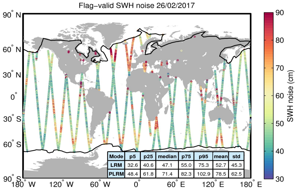
Figure 18. Geographical distribution of flag-valid 20-Hz SWH measurement noise over oceans and lakes for 26/02/2017. The statistical values shown in the table refer to the SWH noise and are calculated separately for LRM and PLRM regions. Measurements taken over polar polygons have been excluded from the computation of the statistical values. The black lines mark the outer limit of the Arctic and Antarctic polar polygons.
