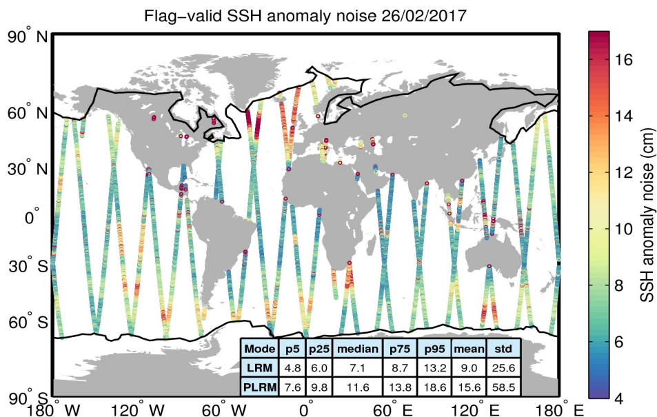
Figure 8. Geographical distribution of flag-valid 20-Hz SSH anomaly measurement noise over oceans and lakes for 26/02/2017. The statistical values shown in the table refer to the SSH anomaly noise and are calculated separately for LRM and PLRM regions. Measurements taken over polar polygons have been excluded from the computation of the statistical values. The black lines mark the outer limit of the Arctic and Antarctic polar polygons.
