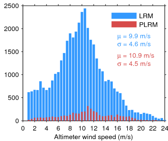
Figure 33. Histogram of flag-valid wind over oceans and lakes for LRM (blue) and PLRM (red) for 26/02/2017. The mean ( \mu ) and standard deviation ( \sigma ) are also shown. Note that values larger than 24 m/s are excluded from the histogram for the sake of readability but not from the computation of \mu and \sigma .
