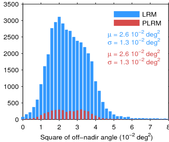
Figure 39. Histogram of flag-valid mispointing over oceans and lakes for LRM (blue) and PLRM (red) for 26/02/2017. Only positive values have been considered. The mean ( \mu ) and standard deviation ( \sigma ) are also shown. Note that values larger than 8 \cdot 10^{-2} \text{ deg}^2 are excluded from the histogram for the sake of readability but not from the computation of \mu and \sigma .
