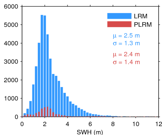
Figure 17. Histogram of flag-valid SWH over oceans and lakes for LRM (blue) and PLRM (red) for 25/02/2017. The mean ( \mu ) and standard deviation ( \sigma ) are also shown. Note that values larger than 12 m are excluded from the histogram for the sake of readability but not from the computation of \mu and \sigma .
