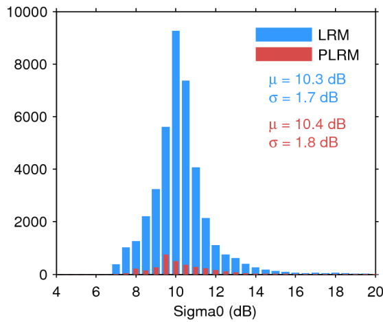
Figure 28. Histogram of science-valid sigma0 over oceans and lakes for LRM (blue) and PLRM (red) for 25/02/2017. The mean ( \mu ) and standard deviation ( \sigma ) are also shown. Note that values outside [4 20] dB are excluded from the histogram for the sake of readability but not from the computation of \mu and \sigma .
