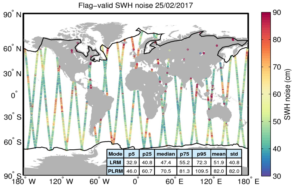
Figure 18. Geographical distribution of flag-valid 20-Hz SWH measurement noise over oceans and lakes for 25/02/2017. The statistical values shown in the table refer to the SWH noise and are calculated separately for LRM and PLRM regions. Measurements taken over polar polygons have been excluded from the computation of the statistical values. The black lines mark the outer limit of the Arctic and Antarctic polar polygons.
