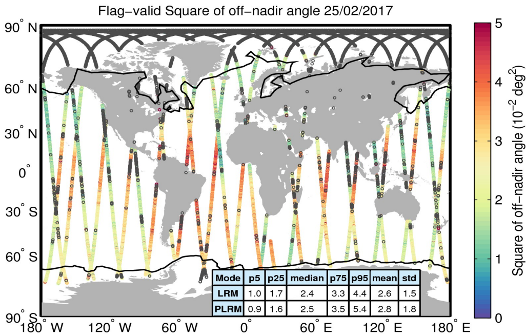
Figure 37. Geographical distribution of flag-valid mispointing data over oceans and lakes for 25/02/2017. The statistical values shown in the table refer to the mispointing in 10^{-2} deg 2 and are calculated separately for LRM and PLRM regions. Measurements taken over polar polygons have been excluded from the computation of the statistical values. The black lines mark the outer limit of the Arctic and Antarctic polar polygons. Gray circles denote negative values.
