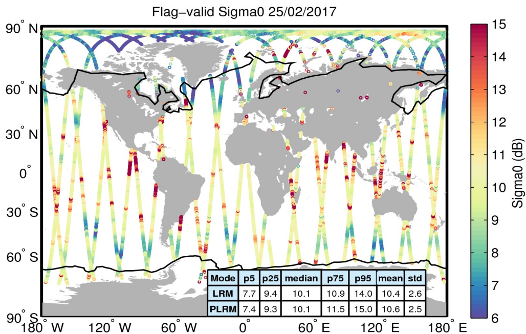
Figure 23. Geographical distribution of flag-valid sigma0 data over oceans and lakes for 25/02/2017. The statistical values shown in the table refer to the sigma0 in dB and are calculated separately for LRM and PLRM regions. Measurements taken over polar polygons have been excluded from the computation of the statistical values. The black lines mark the outer limit of the Arctic and Antarctic polar polygons.
