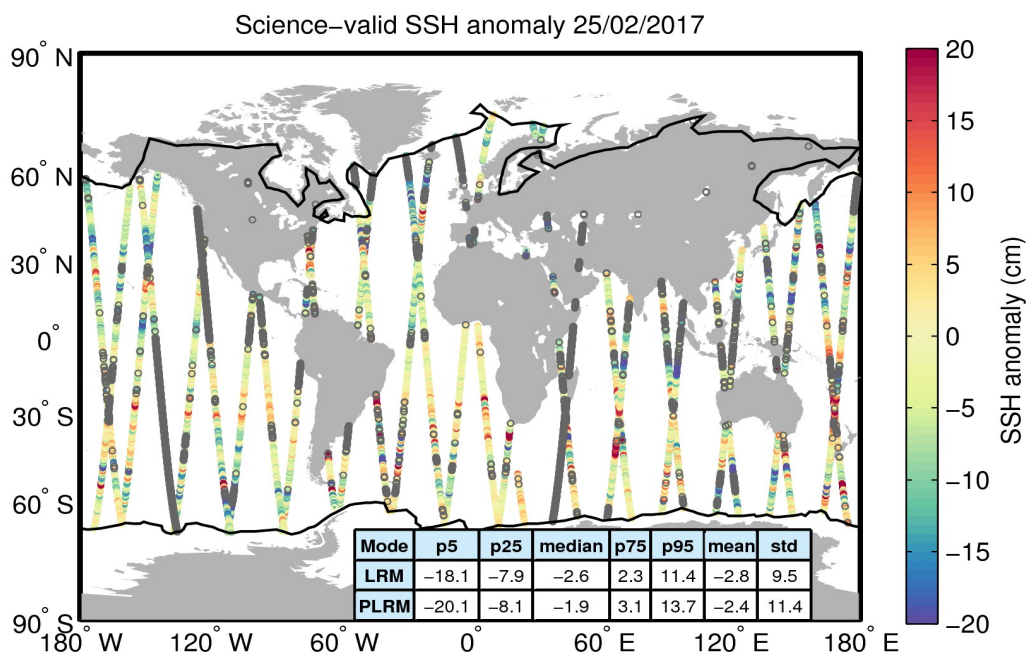
Figure 10. Geographical distribution of science-valid SSH anomaly data over oceans and lakes for 25/02/2017. The statistical values shown in the table refer to the SSH anomaly in cm and are calculated separately for LRM and PLRM regions. The black lines mark the outer limit of the Arctic and Antarctic polar polygons. Gray circles denote records that have been rejected based on the editing criteria described in Table 2.
