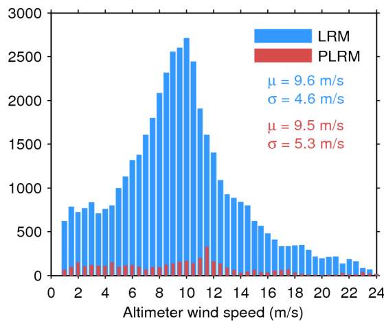
Figure 35. Histogram of science-valid wind over oceans and lakes for LRM (blue) and PLRM (red) for 25/02/2017. The mean ( \mu ) and standard deviation ( \sigma ) are also shown. Note that values larger than 24 m/s are excluded from the histogram for the sake of readability but not from the computation of \mu and \sigma .
