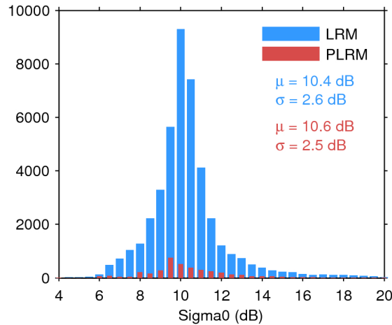
Figure 25. Histogram of flag-valid sigma0 over oceans and lakes for LRM (blue) and PLRM (red) for 25/02/2017. The mean ( \mu ) and standard deviation ( \sigma ) are also shown. Note that values outside [4 20] dB are excluded from the histogram for the sake of readability but not from the computation of \mu and \sigma .
