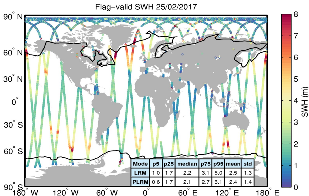
Figure 15. Geographical distribution of flag-valid SWH data over oceans and lakes for 25/02/2017. The statistical values shown in the table refer to the SWH in m and are calculated separately for LRM and PLRM regions. Measurements taken over polar polygons have been excluded from the computation of the statistical values. The black lines mark the outer limit of the Arctic and Antarctic polar polygons.
