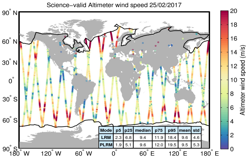
Figure 34. Geographical distribution of science-valid wind data over oceans and lakes for 25/02/2017. The statistical values shown in the table refer to the wind in m/s and are calculated separately for LRM and PLRM regions. The black lines mark the outer limit of the Arctic and Antarctic polar polygons. Gray circles denote records that have been rejected based on the editing criteria described in Table 5.
