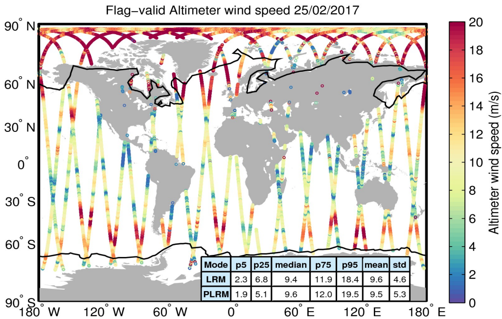
Figure 31. Geographical distribution of flag-valid wind data over oceans and lakes for 25/02/2017. The statistical values shown in the table refer to the wind in m/s and are calculated separately for LRM and PLRM regions. Measurements taken over polar polygons have been excluded from the computation of the statistical values. The black lines mark the outer limit of the Arctic and Antarctic polar polygons.
