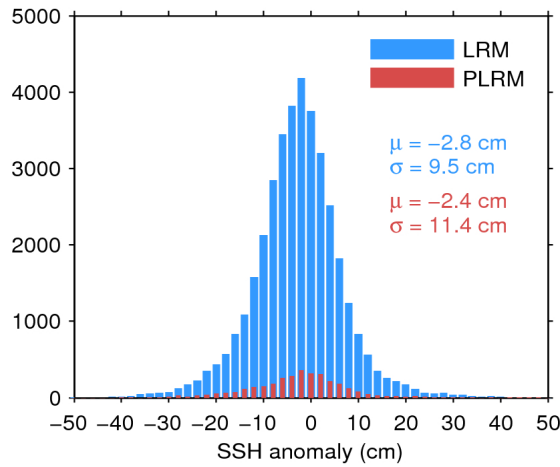
Figure 11. Histogram of science-valid SSH anomaly over oceans and lakes for LRM (blue) and PLRM (red) for 25/02/2017. The mean ( \mu ) and standard deviation ( \sigma ) are also shown. Note that values outside [-50 50] cm are excluded from the histogram for the sake of readability but not from the computation of \mu and \sigma .
