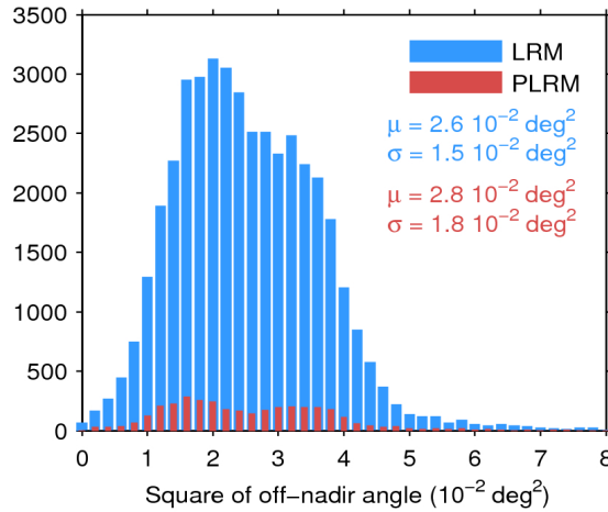
Figure 39. Histogram of flag-valid mispointing over oceans and lakes for LRM (blue) and PLRM (red) for 25/02/2017. Only positive values have been considered. The mean ( \mu ) and standard deviation ( \sigma ) are also shown. Note that values larger than 8 \cdot 10^{-2} \text{ deg}^2 are excluded from the histogram for the sake of readability but not from the computation of \mu and \sigma .
