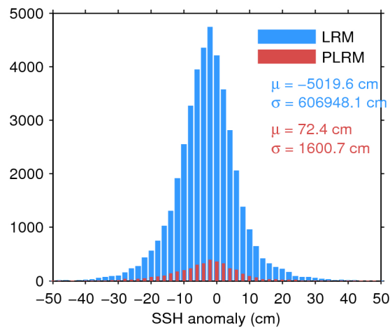
Figure 7. Histogram of flag-valid SSH anomaly over oceans and lakes for LRM (blue) and PLRM (red) for 25/02/2017. The mean ( \mu ) and standard deviation ( \sigma ) are also shown. Note that values outside [-50 \ 50] cm are excluded from the histogram for the sake of readability but not from the computation of \mu and \sigma .
