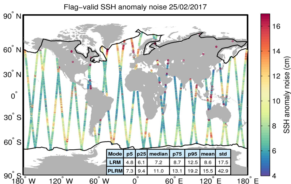
Figure 8. Geographical distribution of flag-valid 20-Hz SSH anomaly measurement noise over oceans and lakes for 25/02/2017. The statistical values shown in the table refer to the SSH anomaly noise and are calculated separately for LRM and PLRM regions. Measurements taken over polar polygons have been excluded from the computation of the statistical values. The black lines mark the outer limit of the Arctic and Antarctic polar polygons.
