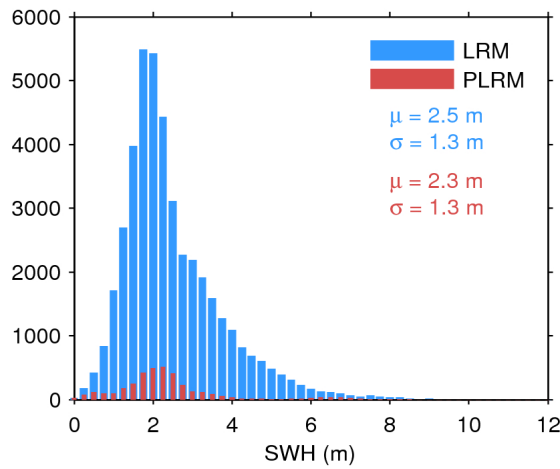
Figure 20. Histogram of science-valid SWH over oceans and lakes for LRM (blue) and PLRM (red) for 25/02/2017. The mean ( \mu ) and standard deviation ( \sigma ) are also shown. Note that values larger than 12 m are excluded from the histogram for the sake of readability but not from the computation of \mu and \sigma .
