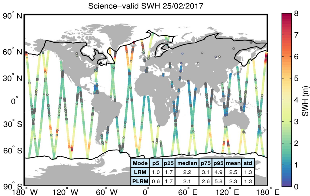
Figure 19. Geographical distribution of science-valid SWH data over oceans and lakes for 25/02/2017. The statistical values shown in the table refer to the SWH in m and are calculated separately for LRM and PLRM regions. The black lines mark the outer limit of the Arctic and Antarctic polar polygons. Gray circles denote records that have been rejected based on the editing criteria described in Table 3.
