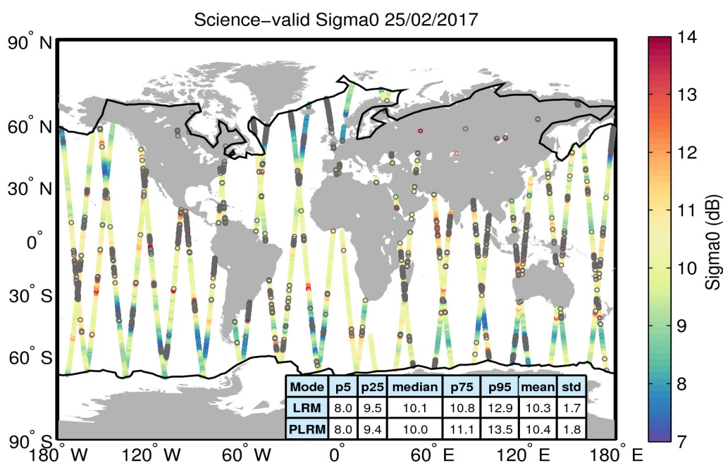
Figure 27. Geographical distribution of science-valid sigma0 data over oceans and lakes for 25/02/2017. The statistical values shown in the table refer to the sigma0 in dB and are calculated separately for LRM and PLRM regions. The black lines mark the outer limit of the Arctic and Antarctic polar polygons. Gray circles denote records that have been rejected based on the editing criteria described in Table 4.
