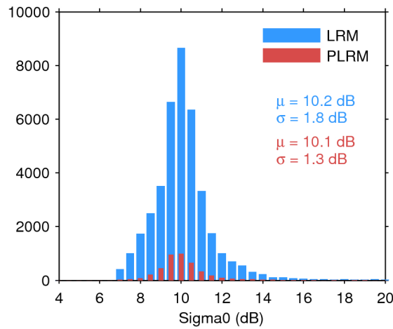
Figure 28. Histogram of science-valid sigma0 over oceans and lakes for LRM (blue) and PLRM (red) for 24/02/2017. The mean ( \mu ) and standard deviation ( \sigma ) are also shown. Note that values outside [4 20] dB are excluded from the histogram for the sake of readability but not from the computation of \mu and \sigma .
