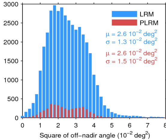
Figure 39. Histogram of flag-valid mispointing over oceans and lakes for LRM (blue) and PLRM (red) for 24/02/2017. Only positive values have been considered. The mean ( \mu ) and standard deviation ( \sigma ) are also shown. Note that values larger than 8 \cdot 10^{-2} \text{ deg}^2 are excluded from the histogram for the sake of readability but not from the computation of \mu and \sigma .
