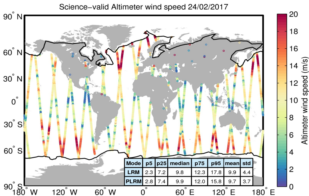
Figure 34. Geographical distribution of science-valid wind data over oceans and lakes for 24/02/2017. The statistical values shown in the table refer to the wind in m/s and are calculated separately for LRM and PLRM regions. The black lines mark the outer limit of the Arctic and Antarctic polar polygons. Gray circles denote records that have been rejected based on the editing criteria described in Table 5.
