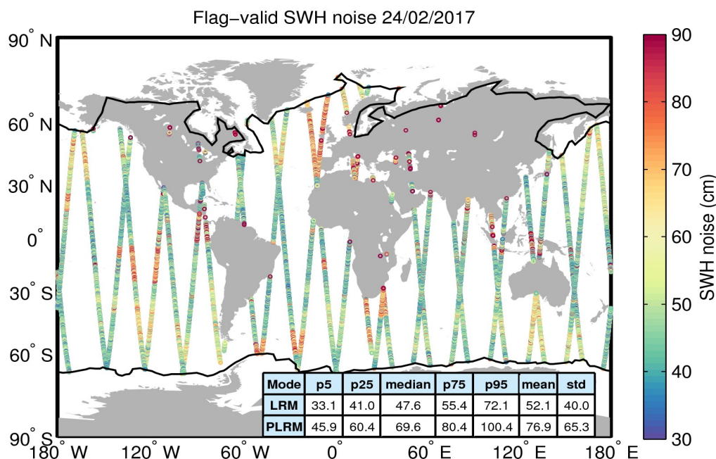
Figure 18. Geographical distribution of flag-valid 20-Hz SWH measurement noise over oceans and lakes for 24/02/2017. The statistical values shown in the table refer to the SWH noise and are calculated separately for LRM and PLRM regions. Measurements taken over polar polygons have been excluded from the computation of the statistical values. The black lines mark the outer limit of the Arctic and Antarctic polar polygons.
