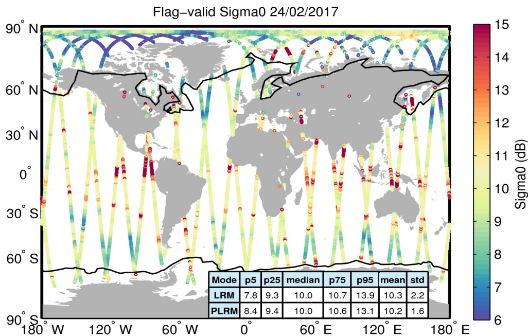
Figure 23. Geographical distribution of flag-valid sigma0 data over oceans and lakes for 24/02/2017. The statistical values shown in the table refer to the sigma0 in dB and are calculated separately for LRM and PLRM regions. Measurements taken over polar polygons have been excluded from the computation of the statistical values. The black lines mark the outer limit of the Arctic and Antarctic polar polygons.
