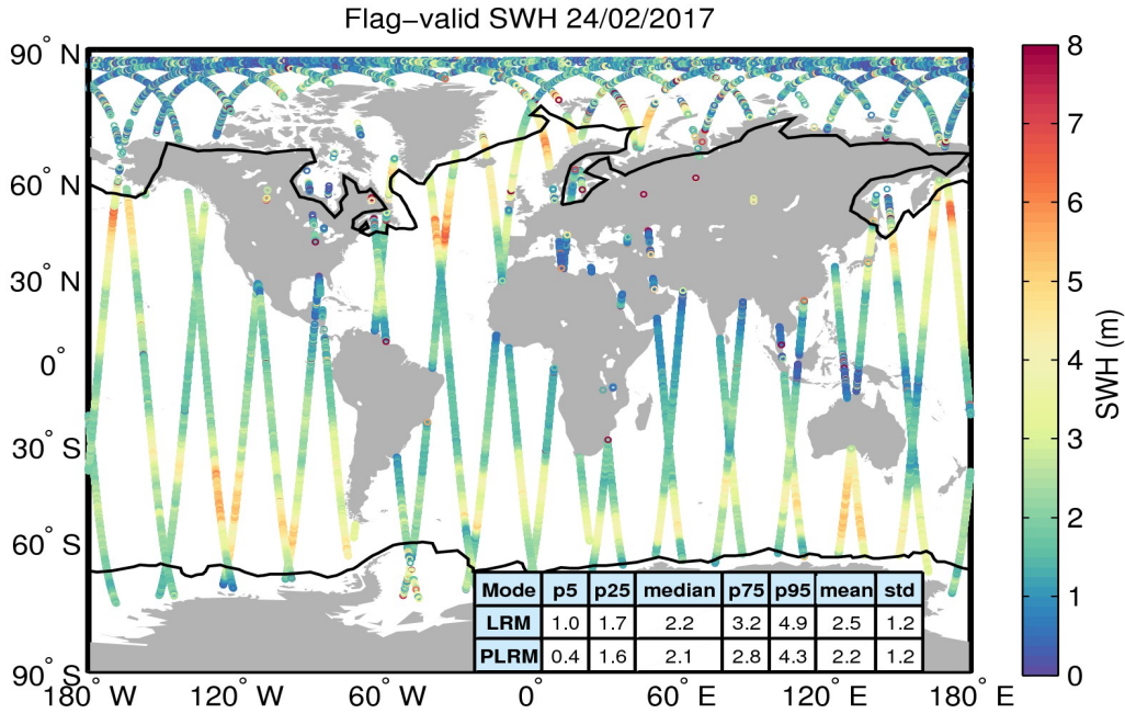
Figure 15. Geographical distribution of flag-valid SWH data over oceans and lakes for 24/02/2017. The statistical values shown in the table refer to the SWH in m and are calculated separately for LRM and PLRM regions. Measurements taken over polar polygons have been excluded from the computation of the statistical values. The black lines mark the outer limit of the Arctic and Antarctic polar polygons.
