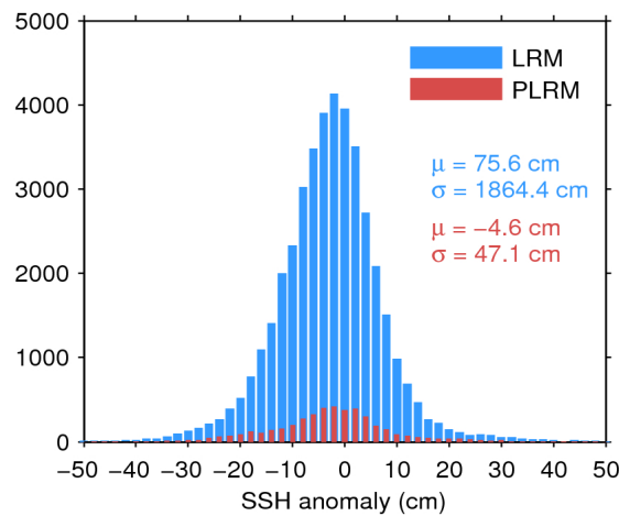
Figure 7. Histogram of flag-valid SSH anomaly over oceans and lakes for LRM (blue) and PLRM (red) for 24/02/2017. The mean ( \mu ) and standard deviation ( \sigma ) are also shown. Note that values outside [-50 \ 50] cm are excluded from the histogram for the sake of readability but not from the computation of \mu and \sigma .
