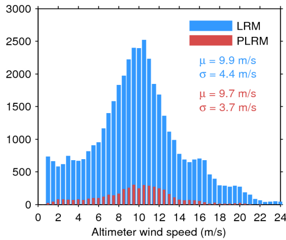
Figure 33. Histogram of flag-valid wind over oceans and lakes for LRM (blue) and PLRM (red) for 24/02/2017. The mean ( \mu ) and standard deviation ( \sigma ) are also shown. Note that values larger than 24 m/s are excluded from the histogram for the sake of readability but not from the computation of \mu and \sigma .
