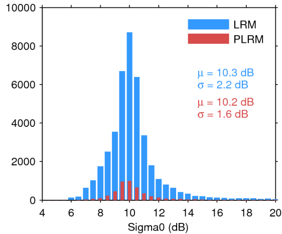
Figure 25. Histogram of flag-valid sigma0 over oceans and lakes for LRM (blue) and PLRM (red) for 24/02/2017. The mean ( \mu ) and standard deviation ( \sigma ) are also shown. Note that values outside [4 20] dB are excluded from the histogram for the sake of readability but not from the computation of \mu and \sigma .
