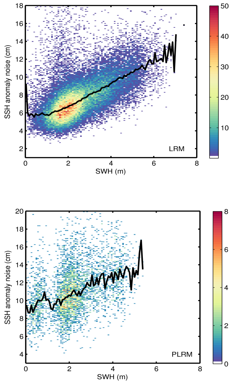
Figure 9. 2D histogram showing flag-valid SSH anomaly noise as a function of SWH for LRM (top) and PLRM (bottom) for 24/02/2017. The black line denotes the median SSH anomaly noise as a function of SWH.
