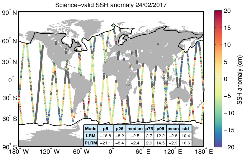
Figure 10. Geographical distribution of science-valid SSH anomaly data over oceans and lakes for 24/02/2017. The statistical values shown in the table refer to the SSH anomaly in cm and are calculated separately for LRM and PLRM regions. The black lines mark the outer limit of the Arctic and Antarctic polar polygons. Gray circles denote records that have been rejected based on the editing criteria described in Table 2.
