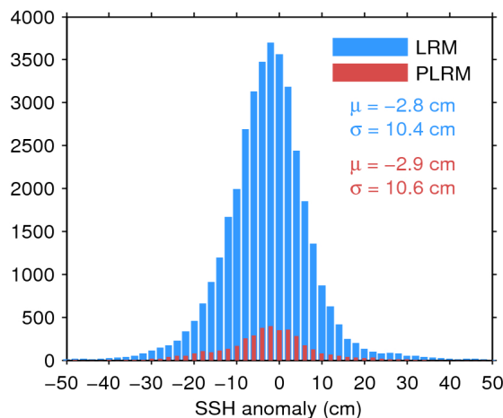
Figure 11. Histogram of science-valid SSH anomaly over oceans and lakes for LRM (blue) and PLRM (red) for 24/02/2017. The mean ( \mu ) and standard deviation ( \sigma ) are also shown. Note that values outside [-50 50] cm are excluded from the histogram for the sake of readability but not from the computation of \mu and \sigma .
