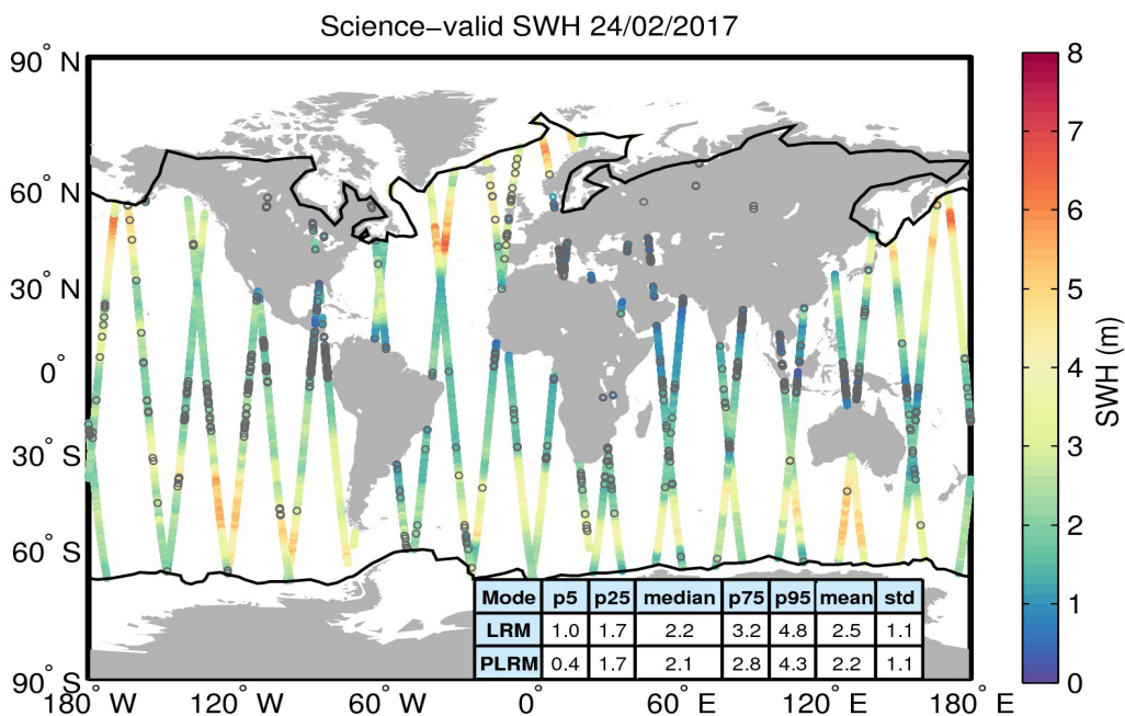
Figure 19. Geographical distribution of science-valid SWH data over oceans and lakes for 24/02/2017. The statistical values shown in the table refer to the SWH in m and are calculated separately for LRM and PLRM regions. The black lines mark the outer limit of the Arctic and Antarctic polar polygons. Gray circles denote records that have been rejected based on the editing criteria described in Table 3.
