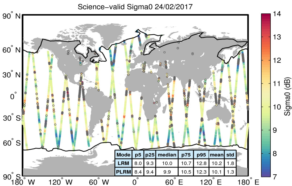
Figure 27. Geographical distribution of science-valid sigma0 data over oceans and lakes for 24/02/2017. The statistical values shown in the table refer to the sigma0 in dB and are calculated separately for LRM and PLRM regions. The black lines mark the outer limit of the Arctic and Antarctic polar polygons. Gray circles denote records that have been rejected based on the editing criteria described in Table 4.
