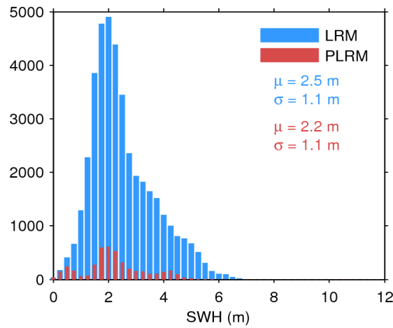
Figure 20. Histogram of science-valid SWH over oceans and lakes for LRM (blue) and PLRM (red) for 24/02/2017. The mean ( \mu ) and standard deviation ( \sigma ) are also shown. Note that values larger than 12 m are excluded from the histogram for the sake of readability but not from the computation of \mu and \sigma .
