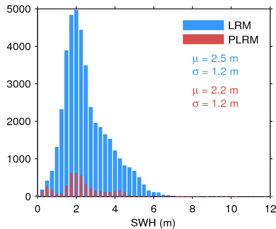
Figure 17. Histogram of flag-valid SWH over oceans and lakes for LRM (blue) and PLRM (red) for 24/02/2017. The mean ( \mu ) and standard deviation ( \sigma ) are also shown. Note that values larger than 12 m are excluded from the histogram for the sake of readability but not from the computation of \mu and \sigma .
