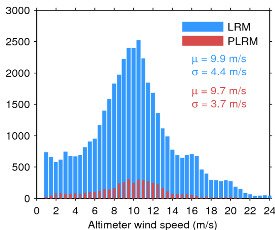
Figure 35. Histogram of science-valid wind over oceans and lakes for LRM (blue) and PLRM (red) for 24/02/2017. The mean ( \mu ) and standard deviation ( \sigma ) are also shown. Note that values larger than 24 m/s are excluded from the histogram for the sake of readability but not from the computation of \mu and \sigma .
