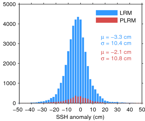
Figure 11. Histogram of science-valid SSH anomaly over oceans and lakes for LRM (blue) and PLRM (red) for 23/02/2017. The mean ( \mu ) and standard deviation ( \sigma ) are also shown. Note that values outside [-50 50] cm are excluded from the histogram for the sake of readability but not from the computation of \mu and \sigma .
