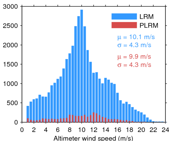
Figure 33. Histogram of flag-valid wind over oceans and lakes for LRM (blue) and PLRM (red) for 23/02/2017. The mean ( \mu ) and standard deviation ( \sigma ) are also shown. Note that values larger than 24 m/s are excluded from the histogram for the sake of readability but not from the computation of \mu and \sigma .
