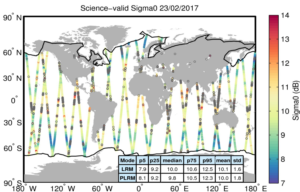
Figure 27. Geographical distribution of science-valid sigma0 data over oceans and lakes for 23/02/2017. The statistical values shown in the table refer to the sigma0 in dB and are calculated separately for LRM and PLRM regions. The black lines mark the outer limit of the Arctic and Antarctic polar polygons. Gray circles denote records that have been rejected based on the editing criteria described in Table 4.
