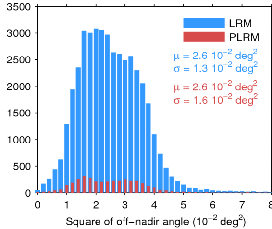
Figure 39. Histogram of flag-valid mispointing over oceans and lakes for LRM (blue) and PLRM (red) for 23/02/2017. Only positive values have been considered. The mean ( \mu ) and standard deviation ( \sigma ) are also shown. Note that values larger than 8 \cdot 10^{-2} \text{ deg}^2 are excluded from the histogram for the sake of readability but not from the computation of \mu and \sigma .
