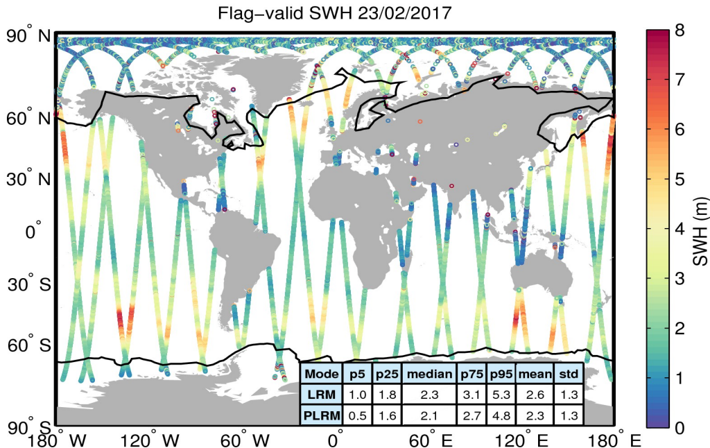
Figure 15. Geographical distribution of flag-valid SWH data over oceans and lakes for 23/02/2017. The statistical values shown in the table refer to the SWH in m and are calculated separately for LRM and PLRM regions. Measurements taken over polar polygons have been excluded from the computation of the statistical values. The black lines mark the outer limit of the Arctic and Antarctic polar polygons.
