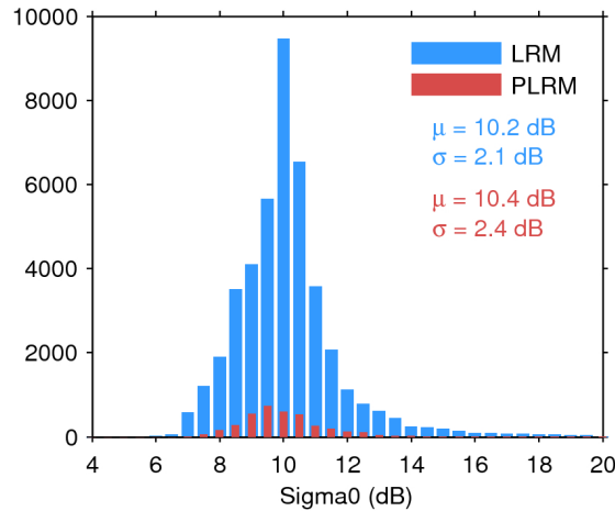
Figure 25. Histogram of flag-valid sigma0 over oceans and lakes for LRM (blue) and PLRM (red) for 23/02/2017. The mean ( \mu ) and standard deviation ( \sigma ) are also shown. Note that values outside [4 20] dB are excluded from the histogram for the sake of readability but not from the computation of \mu and \sigma .
