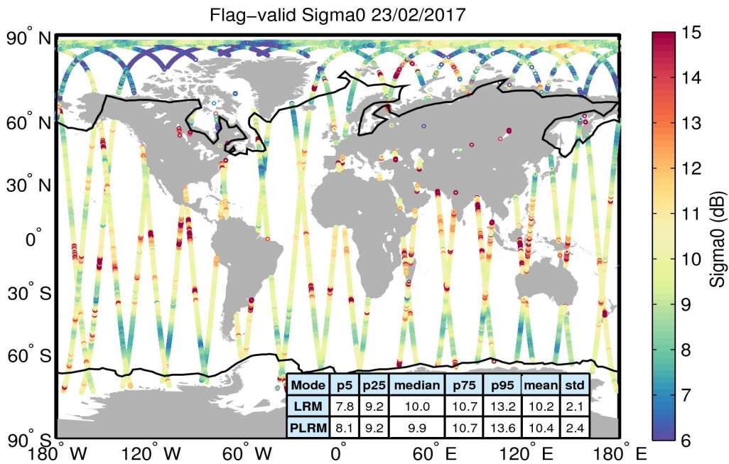
Figure 23. Geographical distribution of flag-valid sigma0 data over oceans and lakes for 23/02/2017. The statistical values shown in the table refer to the sigma0 in dB and are calculated separately for LRM and PLRM regions. Measurements taken over polar polygons have been excluded from the computation of the statistical values. The black lines mark the outer limit of the Arctic and Antarctic polar polygons.
