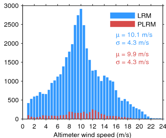
Figure 35. Histogram of science-valid wind over oceans and lakes for LRM (blue) and PLRM (red) for 23/02/2017. The mean ( \mu ) and standard deviation ( \sigma ) are also shown. Note that values larger than 24 m/s are excluded from the histogram for the sake of readability but not from the computation of \mu and \sigma .
