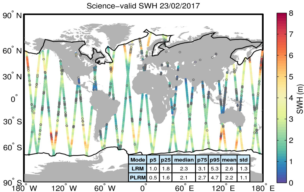
Figure 19. Geographical distribution of science-valid SWH data over oceans and lakes for 23/02/2017. The statistical values shown in the table refer to the SWH in m and are calculated separately for LRM and PLRM regions. The black lines mark the outer limit of the Arctic and Antarctic polar polygons. Gray circles denote records that have been rejected based on the editing criteria described in Table 3.
