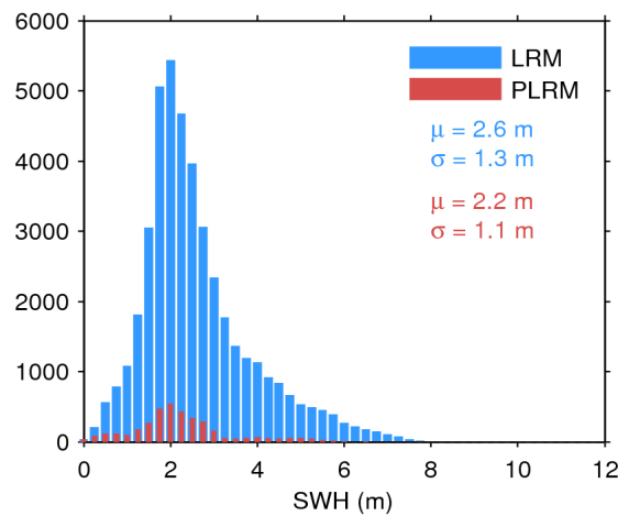
Figure 20. Histogram of science-valid SWH over oceans and lakes for LRM (blue) and PLRM (red) for 23/02/2017. The mean ( \mu ) and standard deviation ( \sigma ) are also shown. Note that values larger than 12 m are excluded from the histogram for the sake of readability but not from the computation of \mu and \sigma .
