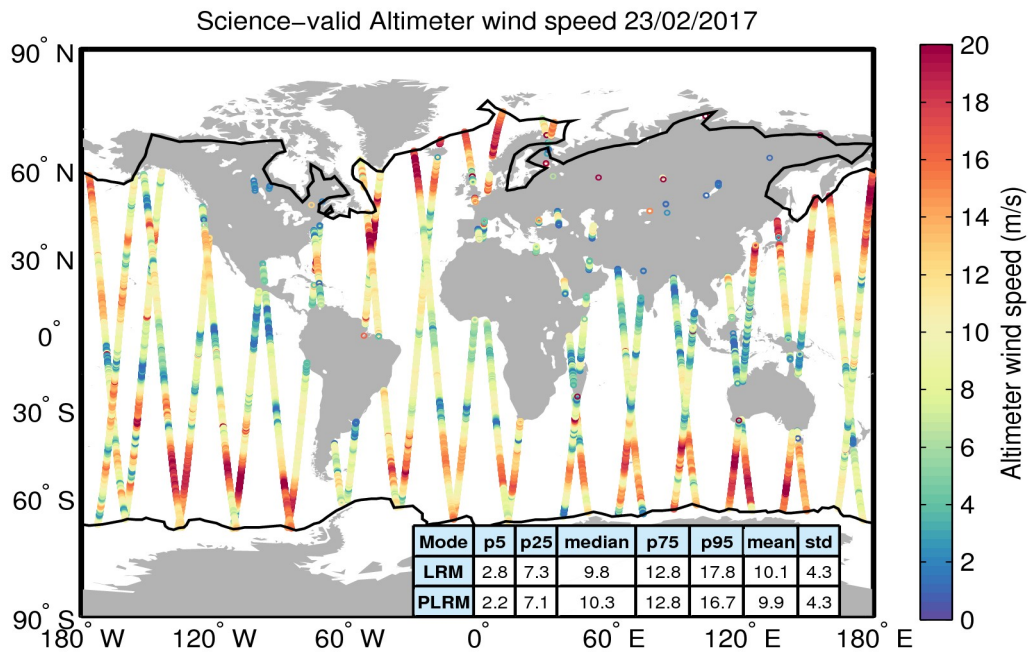
Figure 34. Geographical distribution of science-valid wind data over oceans and lakes for 23/02/2017. The statistical values shown in the table refer to the wind in m/s and are calculated separately for LRM and PLRM regions. The black lines mark the outer limit of the Arctic and Antarctic polar polygons. Gray circles denote records that have been rejected based on the editing criteria described in Table 5.
