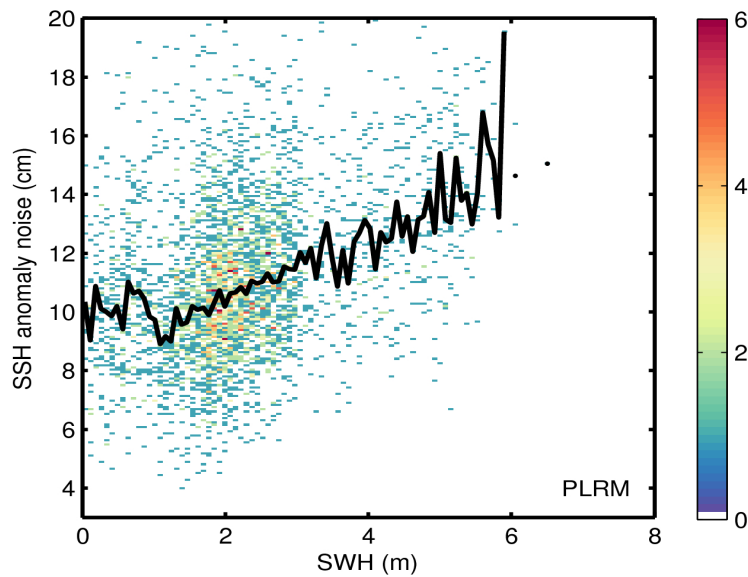
Figure 9. 2D histogram showing flag-valid SSH anomaly noise as a function of SWH for LRM (top) and PLRM (bottom) for 23/02/2017. The black line denotes the median SSH anomaly noise as a function of SWH.
