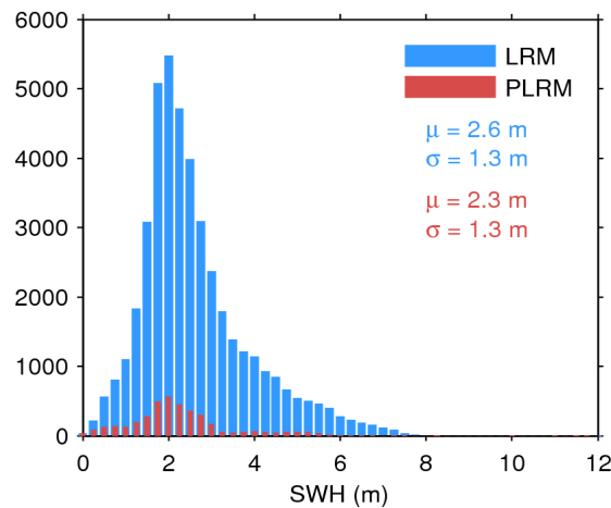
Figure 17. Histogram of flag-valid SWH over oceans and lakes for LRM (blue) and PLRM (red) for 23/02/2017. The mean ( \mu ) and standard deviation ( \sigma ) are also shown. Note that values larger than 12 m are excluded from the histogram for the sake of readability but not from the computation of \mu and \sigma .
