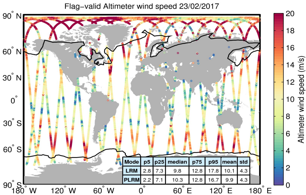
Figure 31. Geographical distribution of flag-valid wind data over oceans and lakes for 23/02/2017. The statistical values shown in the table refer to the wind in m/s and are calculated separately for LRM and PLRM regions. Measurements taken over polar polygons have been excluded from the computation of the statistical values. The black lines mark the outer limit of the Arctic and Antarctic polar polygons.
