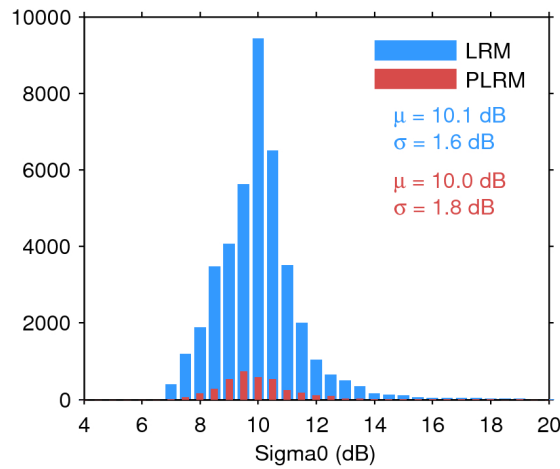
Figure 28. Histogram of science-valid sigma0 over oceans and lakes for LRM (blue) and PLRM (red) for 23/02/2017. The mean ( \mu ) and standard deviation ( \sigma ) are also shown. Note that values outside [4 20] dB are excluded from the histogram for the sake of readability but not from the computation of \mu and \sigma .
