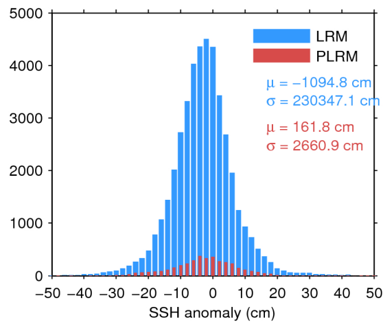
Figure 7. Histogram of flag-valid SSH anomaly over oceans and lakes for LRM (blue) and PLRM (red) for 23/02/2017. The mean ( \mu ) and standard deviation ( \sigma ) are also shown. Note that values outside [-50 50] cm are excluded from the histogram for the sake of readability but not from the computation of \mu and \sigma .
