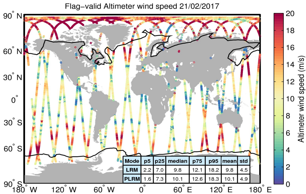
Figure 31. Geographical distribution of flag-valid wind data over oceans and lakes for 21/02/2017. The statistical values shown in the table refer to the wind in m/s and are calculated separately for LRM and PLRM regions. Measurements taken over polar polygons have been excluded from the computation of the statistical values. The black lines mark the outer limit of the Arctic and Antarctic polar polygons.
