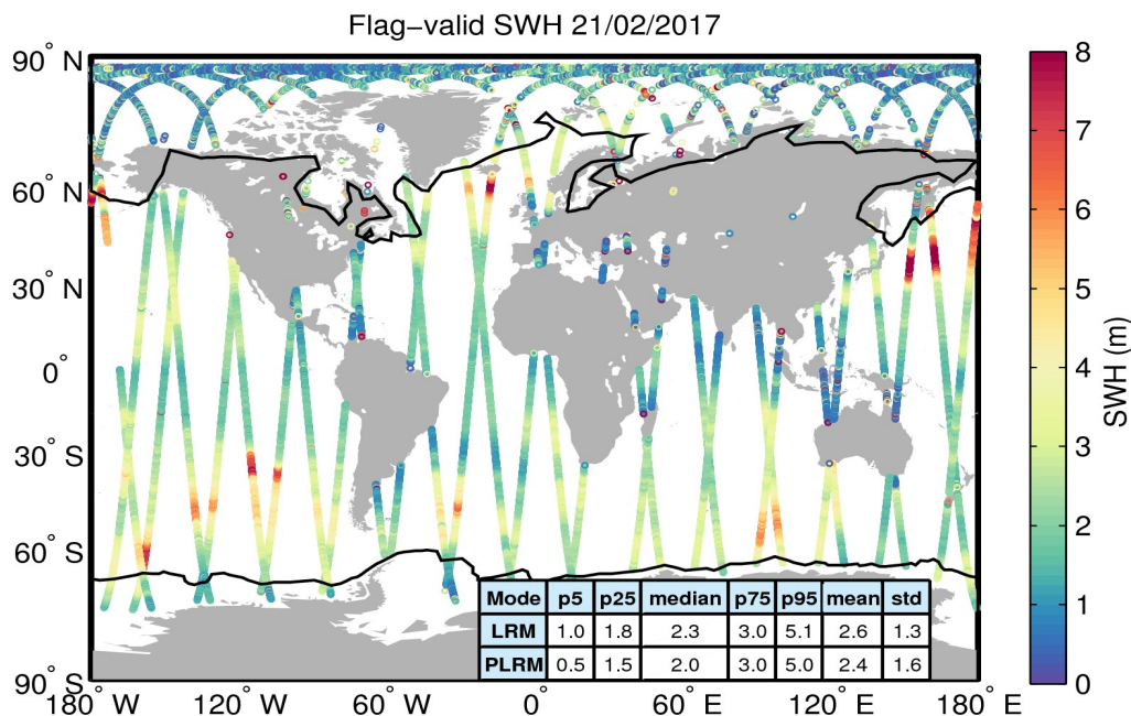
Figure 15. Geographical distribution of flag-valid SWH data over oceans and lakes for 21/02/2017. The statistical values shown in the table refer to the SWH in m and are calculated separately for LRM and PLRM regions. Measurements taken over polar polygons have been excluded from the computation of the statistical values. The black lines mark the outer limit of the Arctic and Antarctic polar polygons.
