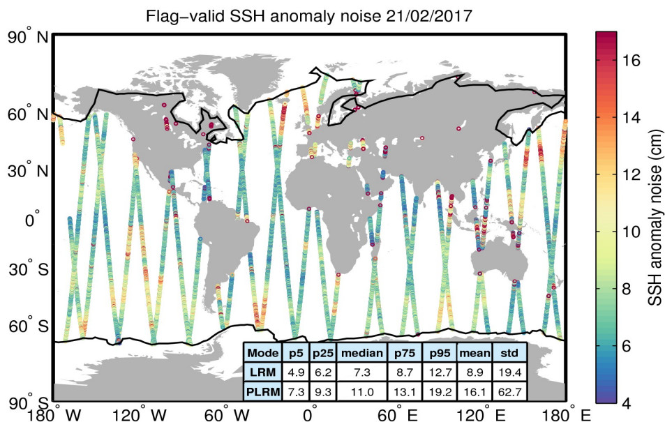
Figure 8. Geographical distribution of flag-valid 20-Hz SSH anomaly measurement noise over oceans and lakes for 21/02/2017. The statistical values shown in the table refer to the SSH anomaly noise and are calculated separately for LRM and PLRM regions. Measurements taken over polar polygons have been excluded from the computation of the statistical values. The black lines mark the outer limit of the Arctic and Antarctic polar polygons.
