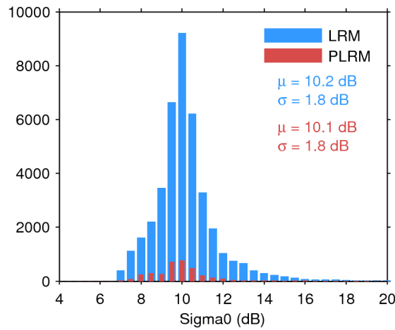
Figure 28. Histogram of science-valid sigma0 over oceans and lakes for LRM (blue) and PLRM (red) for 21/02/2017. The mean ( \mu ) and standard deviation ( \sigma ) are also shown. Note that values outside [4 20] dB are excluded from the histogram for the sake of readability but not from the computation of \mu and \sigma .
