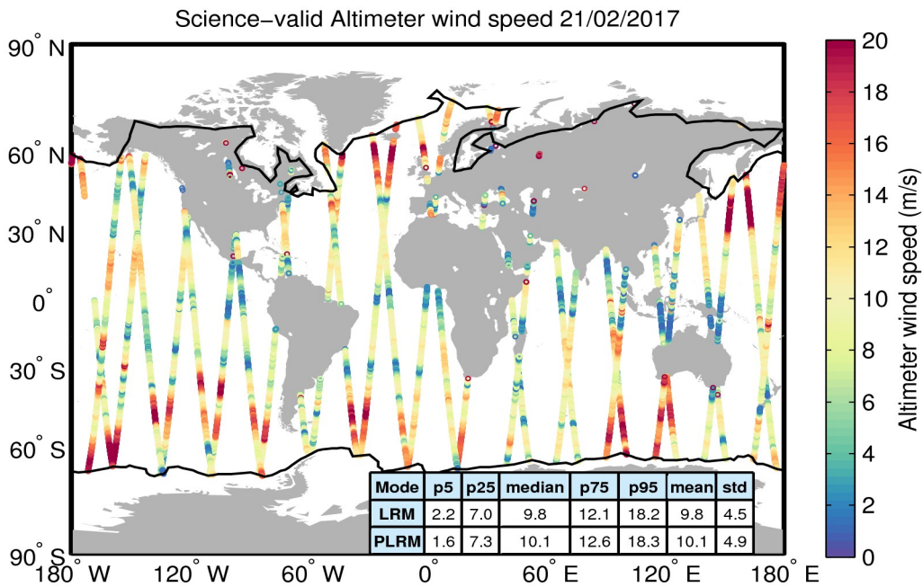
Figure 34. Geographical distribution of science-valid wind data over oceans and lakes for 21/02/2017. The statistical values shown in the table refer to the wind in m/s and are calculated separately for LRM and PLRM regions. The black lines mark the outer limit of the Arctic and Antarctic polar polygons. Gray circles denote records that have been rejected based on the editing criteria described in Table 5.
