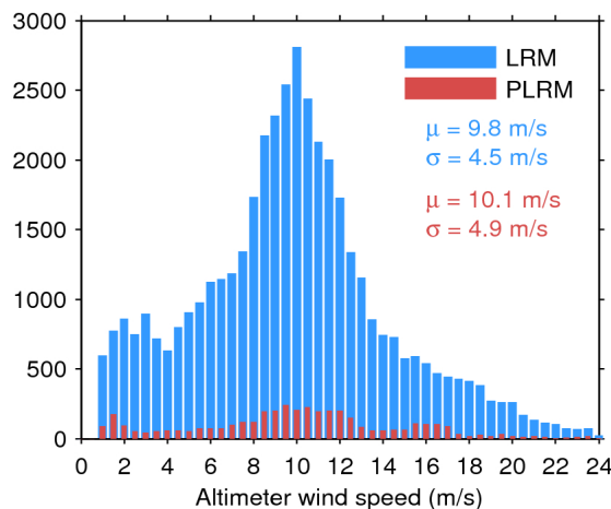
Figure 35. Histogram of science-valid wind over oceans and lakes for LRM (blue) and PLRM (red) for 21/02/2017. The mean ( \mu ) and standard deviation ( \sigma ) are also shown. Note that values larger than 24 m/s are excluded from the histogram for the sake of readability but not from the computation of \mu and \sigma .
