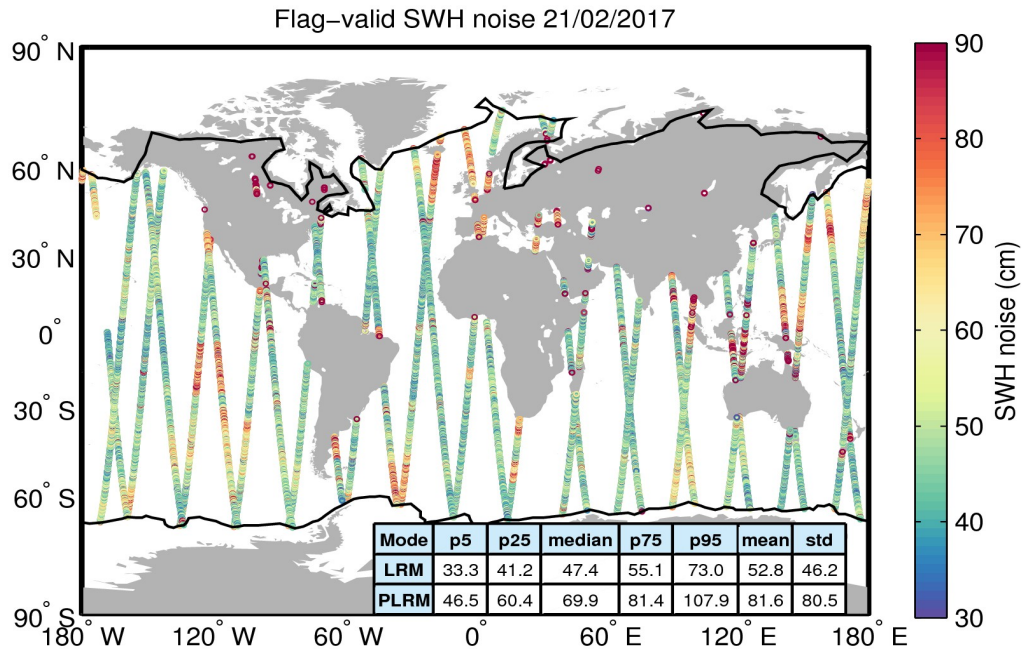
Figure 18. Geographical distribution of flag-valid 20-Hz SWH measurement noise over oceans and lakes for 21/02/2017. The statistical values shown in the table refer to the SWH noise and are calculated separately for LRM and PLRM regions. Measurements taken over polar polygons have been excluded from the computation of the statistical values. The black lines mark the outer limit of the Arctic and Antarctic polar polygons.
