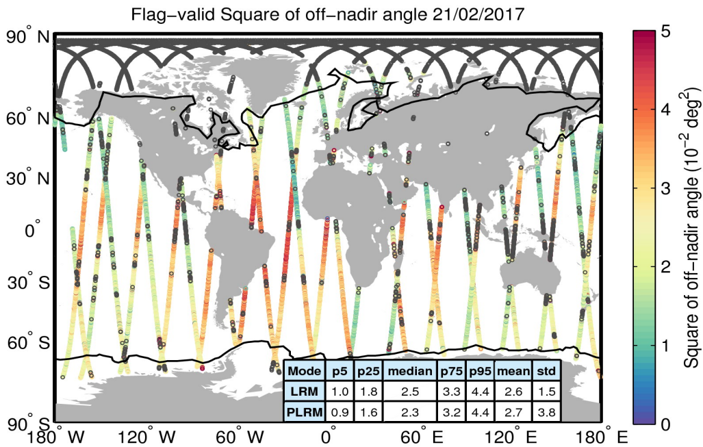
Figure 37. Geographical distribution of flag-valid mispointing data over oceans and lakes for 21/02/2017. The statistical values shown in the table refer to the mispointing in 10^{-2} deg 2 and are calculated separately for LRM and PLRM regions. Measurements taken over polar polygons have been excluded from the computation of the statistical values. The black lines mark the outer limit of the Arctic and Antarctic polar polygons. Gray circles denote negative values.
