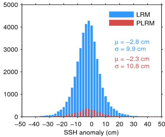
Figure 11. Histogram of science-valid SSH anomaly over oceans and lakes for LRM (blue) and PLRM (red) for 21/02/2017. The mean ( \mu ) and standard deviation ( \sigma ) are also shown. Note that values outside [-50\ 50] cm are excluded from the histogram for the sake of readability but not from the computation of \mu and \sigma .
