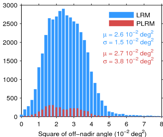
Figure 39. Histogram of flag-valid mispointing over oceans and lakes for LRM (blue) and PLRM (red) for 21/02/2017. Only positive values have been considered. The mean ( \mu ) and standard deviation ( \sigma ) are also shown. Note that values larger than 8 \cdot 10^{-2} \text{ deg}^2 are excluded from the histogram for the sake of readability but not from the computation of \mu and \sigma .
