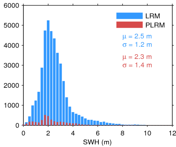
Figure 20. Histogram of science-valid SWH over oceans and lakes for LRM (blue) and PLRM (red) for 21/02/2017. The mean ( \mu ) and standard deviation ( \sigma ) are also shown. Note that values larger than 12 m are excluded from the histogram for the sake of readability but not from the computation of \mu and \sigma .
