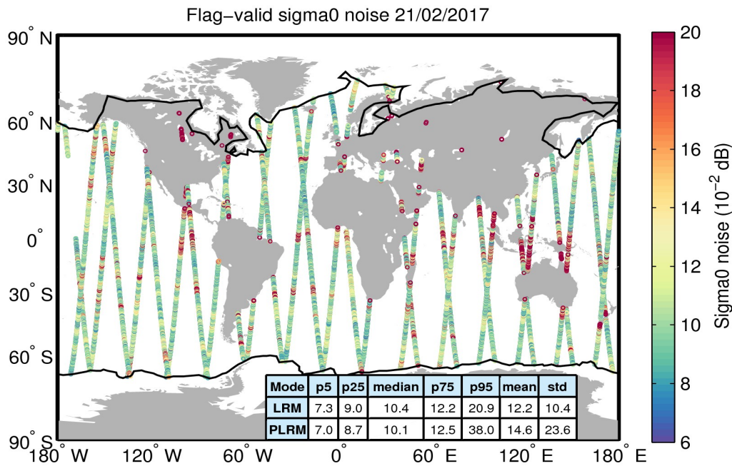
Figure 26. Geographical distribution of flag-valid 20-Hz sigma0 measurement noise over oceans and lakes for 21/02/2017. The statistical values shown in the table refer to the sigma0 noise and are calculated separately for LRM and PLRM regions. Measurements taken over polar polygons have been excluded from the computation of the statistical values. The black lines mark the outer limit of the Arctic and Antarctic polar polygons.
