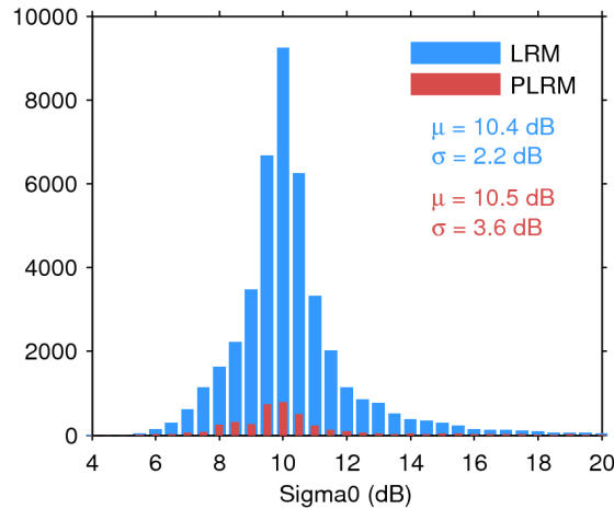
Figure 25. Histogram of flag-valid sigma0 over oceans and lakes for LRM (blue) and PLRM (red) for 21/02/2017. The mean ( \mu ) and standard deviation ( \sigma ) are also shown. Note that values outside [4 20] dB are excluded from the histogram for the sake of readability but not from the computation of \mu and \sigma .
