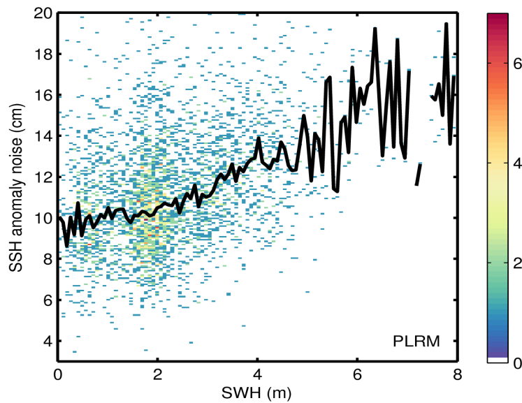
Figure 9. 2D histogram showing flag-valid SSH anomaly noise as a function of SWH for LRM (top) and PLRM (bottom) for 21/02/2017. The black line denotes the median SSH anomaly noise as a function of SWH.
