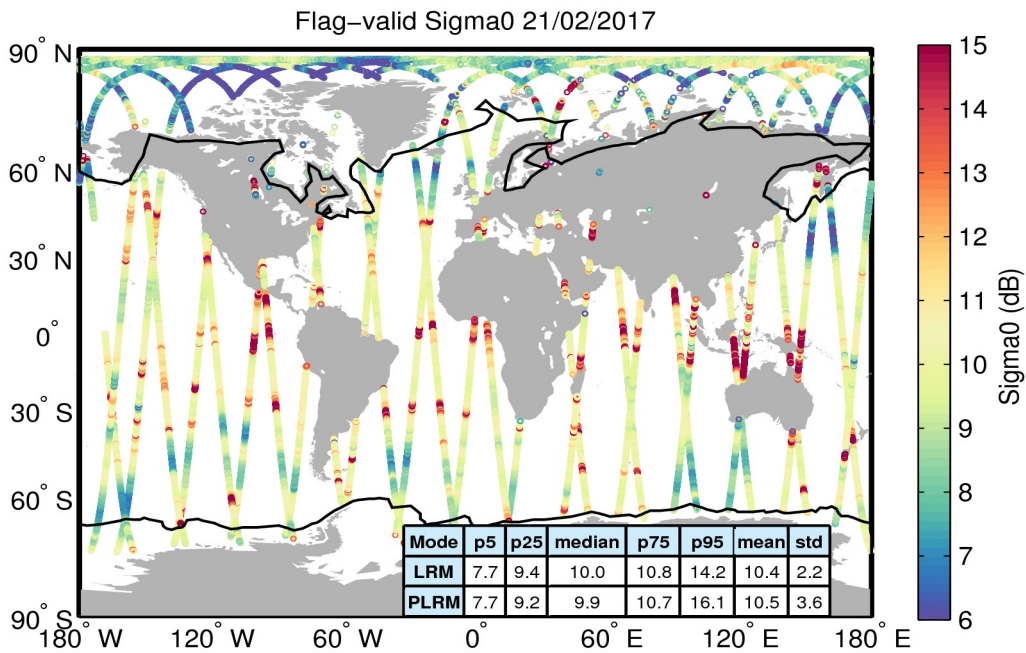
Figure 23. Geographical distribution of flag-valid sigma0 data over oceans and lakes for 21/02/2017. The statistical values shown in the table refer to the sigma0 in dB and are calculated separately for LRM and PLRM regions. Measurements taken over polar polygons have been excluded from the computation of the statistical values. The black lines mark the outer limit of the Arctic and Antarctic polar polygons.
