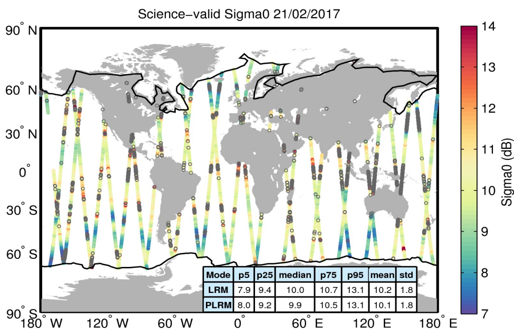
Figure 27. Geographical distribution of science-valid sigma0 data over oceans and lakes for 21/02/2017. The statistical values shown in the table refer to the sigma0 in dB and are calculated separately for LRM and PLRM regions. The black lines mark the outer limit of the Arctic and Antarctic polar polygons. Gray circles denote records that have been rejected based on the editing criteria described in Table 4.
