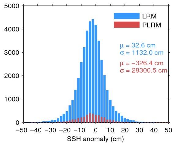
Figure 7. Histogram of flag-valid SSH anomaly over oceans and lakes for LRM (blue) and PLRM (red) for 21/02/2017. The mean ( \mu ) and standard deviation ( \sigma ) are also shown. Note that values outside [-50\ 50] cm are excluded from the histogram for the sake of readability but not from the computation of \mu and \sigma .
