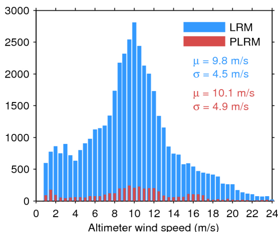
Figure 33. Histogram of flag-valid wind over oceans and lakes for LRM (blue) and PLRM (red) for 21/02/2017. The mean ( \mu ) and standard deviation ( \sigma ) are also shown. Note that values larger than 24 m/s are excluded from the histogram for the sake of readability but not from the computation of \mu and \sigma .
