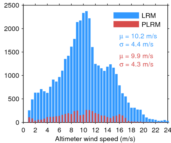
Figure 33. Histogram of flag-valid wind over oceans and lakes for LRM (blue) and PLRM (red) for 20/02/2017. The mean ( \mu ) and standard deviation ( \sigma ) are also shown. Note that values larger than 24 m/s are excluded from the histogram for the sake of readability but not from the computation of \mu and \sigma .
