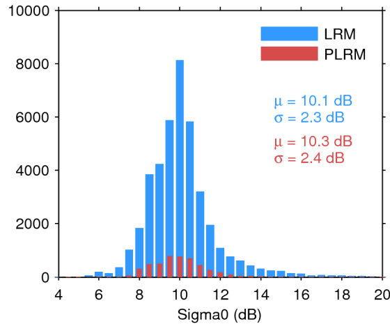
Figure 25. Histogram of flag-valid sigma0 over oceans and lakes for LRM (blue) and PLRM (red) for 20/02/2017. The mean ( \mu ) and standard deviation ( \sigma ) are also shown. Note that values outside [4 20] dB are excluded from the histogram for the sake of readability but not from the computation of \mu and \sigma .
