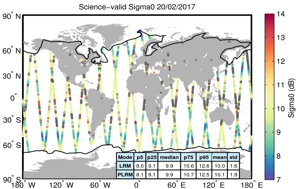
Figure 27. Geographical distribution of science-valid sigma0 data over oceans and lakes for 20/02/2017. The statistical values shown in the table refer to the sigma0 in dB and are calculated separately for LRM and PLRM regions. The black lines mark the outer limit of the Arctic and Antarctic polar polygons. Gray circles denote records that have been rejected based on the editing criteria described in Table 4.
