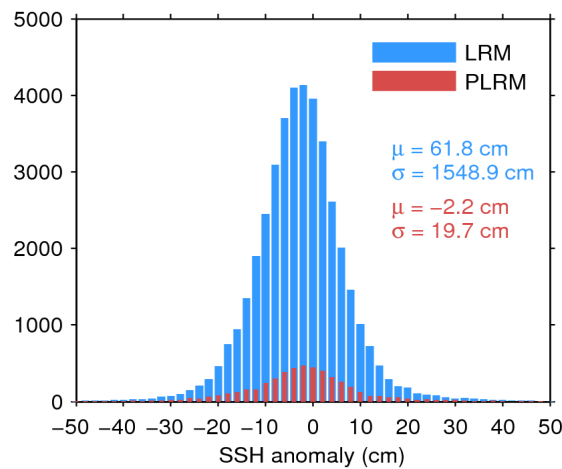
Figure 7. Histogram of flag-valid SSH anomaly over oceans and lakes for LRM (blue) and PLRM (red) for 20/02/2017. The mean ( \mu ) and standard deviation ( \sigma ) are also shown. Note that values outside [-50 50] cm are excluded from the histogram for the sake of readability but not from the computation of \mu and \sigma .
