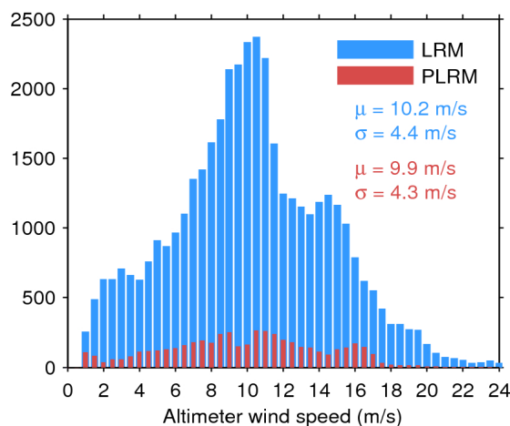
Figure 35. Histogram of science-valid wind over oceans and lakes for LRM (blue) and PLRM (red) for 20/02/2017. The mean ( \mu ) and standard deviation ( \sigma ) are also shown. Note that values larger than 24 m/s are excluded from the histogram for the sake of readability but not from the computation of \mu and \sigma .
