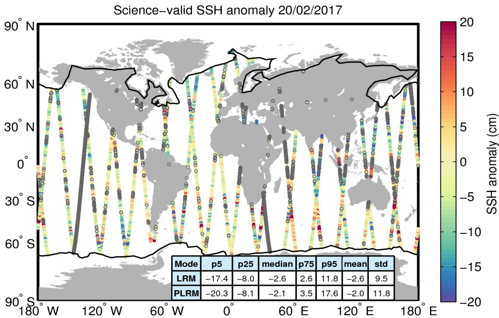
Figure 10. Geographical distribution of science-valid SSH anomaly data over oceans and lakes for 20/02/2017. The statistical values shown in the table refer to the SSH anomaly in cm and are calculated separately for LRM and PLRM regions. The black lines mark the outer limit of the Arctic and Antarctic polar polygons. Gray circles denote records that have been rejected based on the editing criteria described in Table 2.
