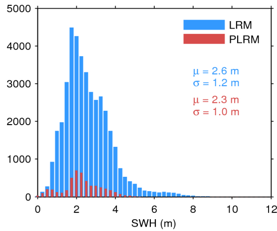
Figure 20. Histogram of science-valid SWH over oceans and lakes for LRM (blue) and PLRM (red) for 20/02/2017. The mean ( \mu ) and standard deviation ( \sigma ) are also shown. Note that values larger than 12 m are excluded from the histogram for the sake of readability but not from the computation of \mu and \sigma .
