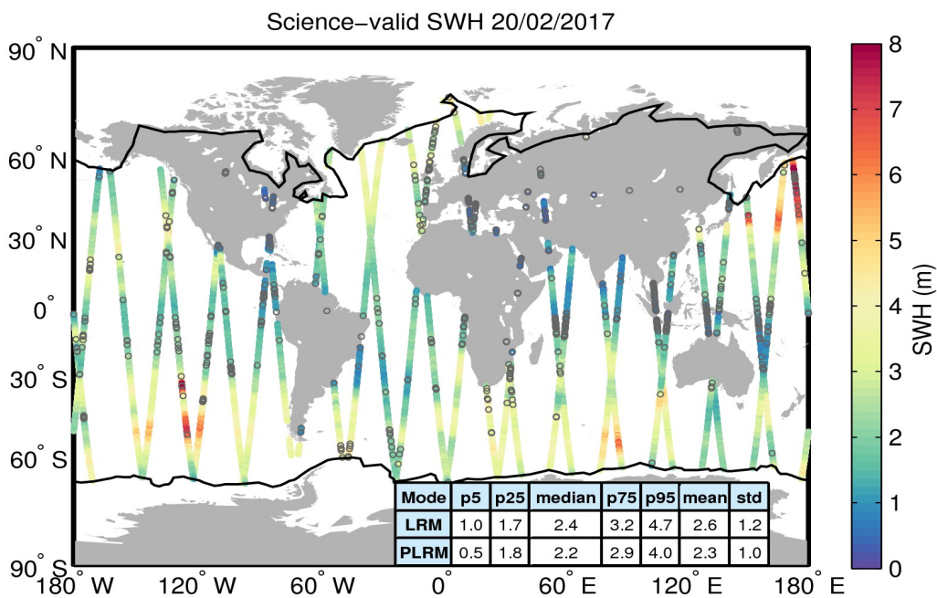
Figure 19. Geographical distribution of science-valid SWH data over oceans and lakes for 20/02/2017. The statistical values shown in the table refer to the SWH in m and are calculated separately for LRM and PLRM regions. The black lines mark the outer limit of the Arctic and Antarctic polar polygons. Gray circles denote records that have been rejected based on the editing criteria described in Table 3.
