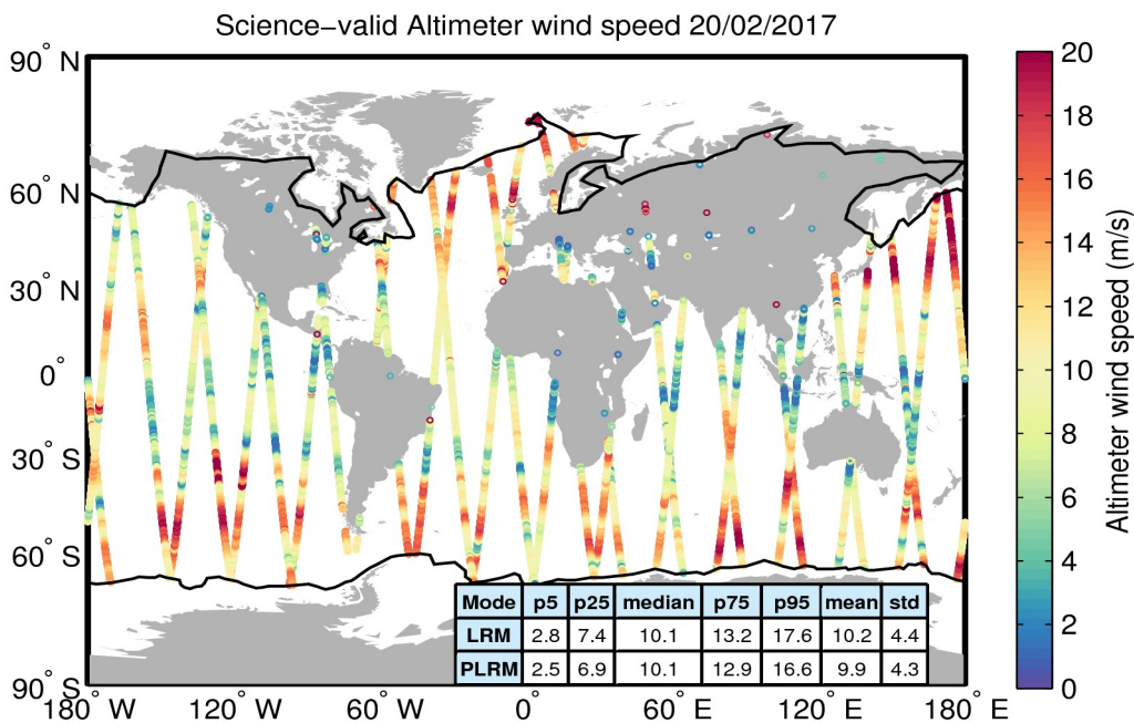
Figure 34. Geographical distribution of science-valid wind data over oceans and lakes for 20/02/2017. The statistical values shown in the table refer to the wind in m/s and are calculated separately for LRM and PLRM regions. The black lines mark the outer limit of the Arctic and Antarctic polar polygons. Gray circles denote records that have been rejected based on the editing criteria described in Table 5.
