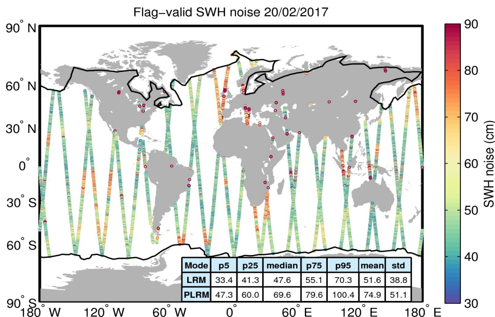
Figure 18. Geographical distribution of flag-valid 20-Hz SWH measurement noise over oceans and lakes for 20/02/2017. The statistical values shown in the table refer to the SWH noise and are calculated separately for LRM and PLRM regions. Measurements taken over polar polygons have been excluded from the computation of the statistical values. The black lines mark the outer limit of the Arctic and Antarctic polar polygons.
