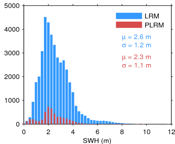
Figure 17. Histogram of flag-valid SWH over oceans and lakes for LRM (blue) and PLRM (red) for 20/02/2017. The mean ( \mu ) and standard deviation ( \sigma ) are also shown. Note that values larger than 12 m are excluded from the histogram for the sake of readability but not from the computation of \mu and \sigma .
