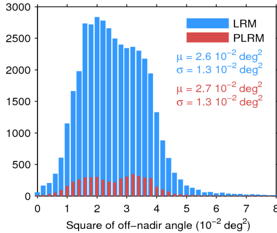
Figure 39. Histogram of flag-valid mispointing over oceans and lakes for LRM (blue) and PLRM (red) for 20/02/2017. Only positive values have been considered. The mean ( \mu ) and standard deviation ( \sigma ) are also shown. Note that values larger than 8 \cdot 10^{-2} \text{ deg}^2 are excluded from the histogram for the sake of readability but not from the computation of \mu and \sigma .
