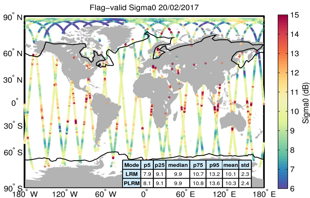
Figure 23. Geographical distribution of flag-valid sigma0 data over oceans and lakes for 20/02/2017. The statistical values shown in the table refer to the sigma0 in dB and are calculated separately for LRM and PLRM regions. Measurements taken over polar polygons have been excluded from the computation of the statistical values. The black lines mark the outer limit of the Arctic and Antarctic polar polygons.
