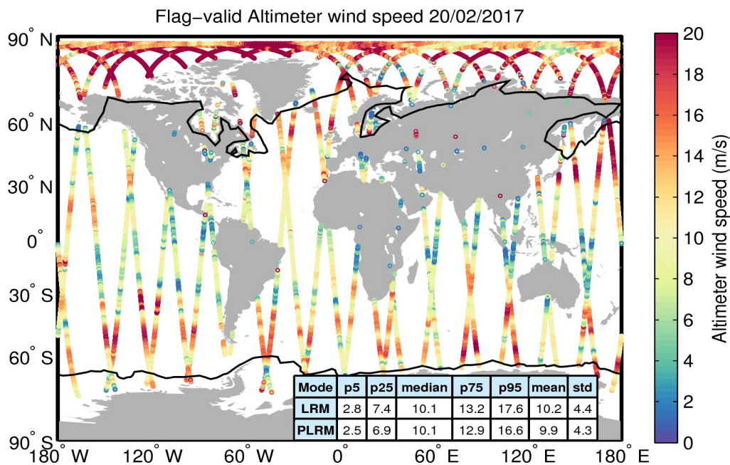
Figure 31. Geographical distribution of flag-valid wind data over oceans and lakes for 20/02/2017. The statistical values shown in the table refer to the wind in m/s and are calculated separately for LRM and PLRM regions. Measurements taken over polar polygons have been excluded from the computation of the statistical values. The black lines mark the outer limit of the Arctic and Antarctic polar polygons.
