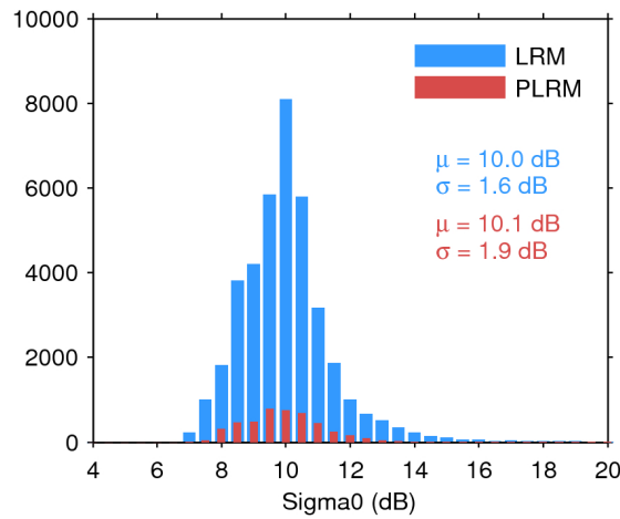
Figure 28. Histogram of science-valid sigma0 over oceans and lakes for LRM (blue) and PLRM (red) for 20/02/2017. The mean ( \mu ) and standard deviation ( \sigma ) are also shown. Note that values outside [4 20] dB are excluded from the histogram for the sake of readability but not from the computation of \mu and \sigma .
