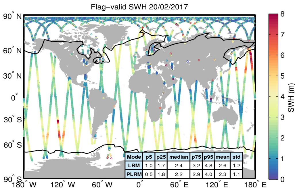
Figure 15. Geographical distribution of flag-valid SWH data over oceans and lakes for 20/02/2017. The statistical values shown in the table refer to the SWH in m and are calculated separately for LRM and PLRM regions. Measurements taken over polar polygons have been excluded from the computation of the statistical values. The black lines mark the outer limit of the Arctic and Antarctic polar polygons.
