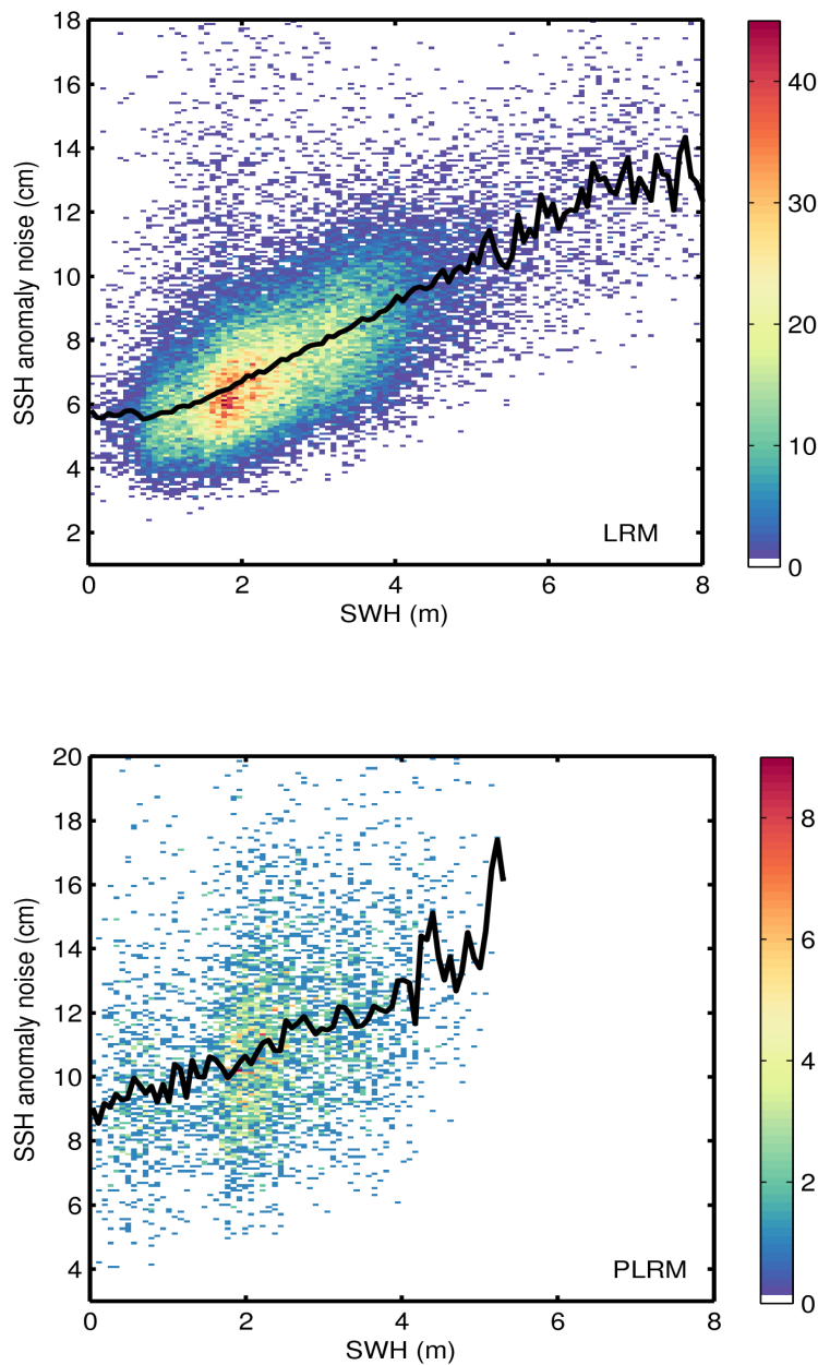
Figure 9. 2D histogram showing flag-valid SSH anomaly noise as a function of SWH for LRM (top) and PLRM (bottom) for 20/02/2017. The black line denotes the median SSH anomaly noise as a function of SWH.
