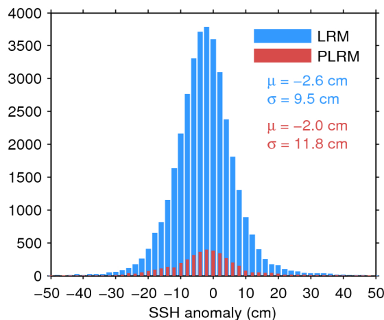
Figure 11. Histogram of science-valid SSH anomaly over oceans and lakes for LRM (blue) and PLRM (red) for 20/02/2017. The mean ( \mu ) and standard deviation ( \sigma ) are also shown. Note that values outside [-50 50] cm are excluded from the histogram for the sake of readability but not from the computation of \mu and \sigma .
