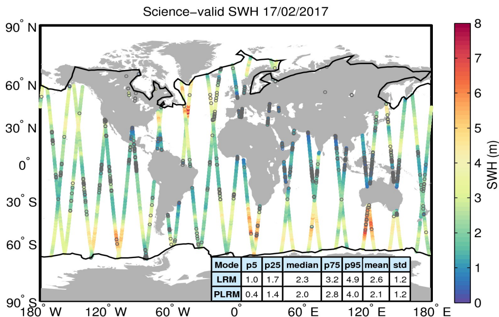
Figure 19. Geographical distribution of science-valid SWH data over oceans and lakes for 17/02/2017. The statistical values shown in the table refer to the SWH in m and are calculated separately for LRM and PLRM regions. The black lines mark the outer limit of the Arctic and Antarctic polar polygons. Gray circles denote records that have been rejected based on the editing criteria described in Table 3.
