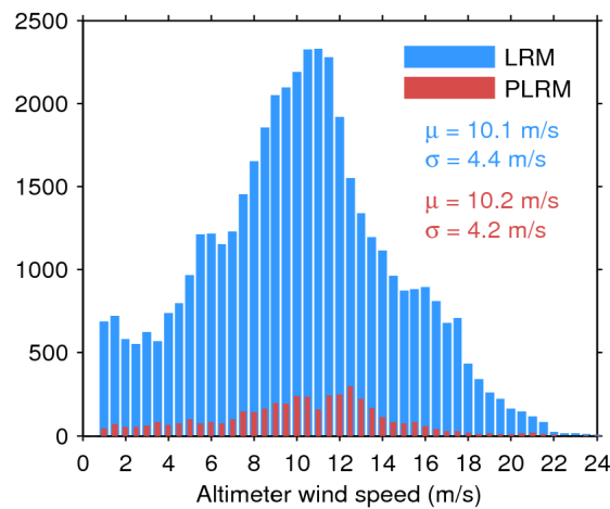
Figure 33. Histogram of flag-valid wind over oceans and lakes for LRM (blue) and PLRM (red) for 17/02/2017. The mean ( \mu ) and standard deviation ( \sigma ) are also shown. Note that values larger than 24 m/s are excluded from the histogram for the sake of readability but not from the computation of \mu and \sigma .
