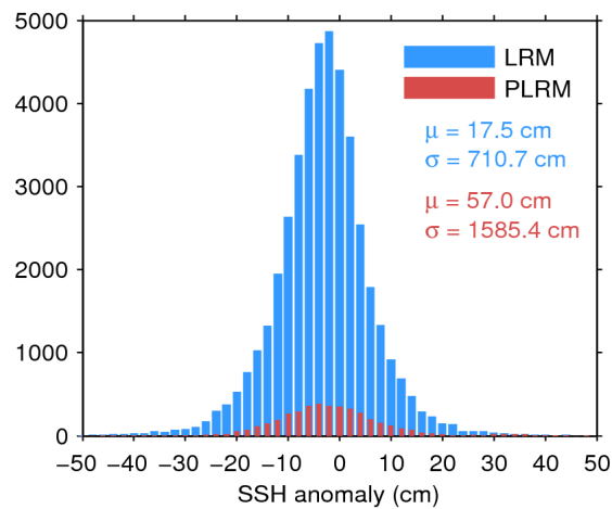
Figure 7. Histogram of flag-valid SSH anomaly over oceans and lakes for LRM (blue) and PLRM (red) for 17/02/2017. The mean ( \mu ) and standard deviation ( \sigma ) are also shown. Note that values outside [-50\ 50] cm are excluded from the histogram for the sake of readability but not from the computation of \mu and \sigma .
