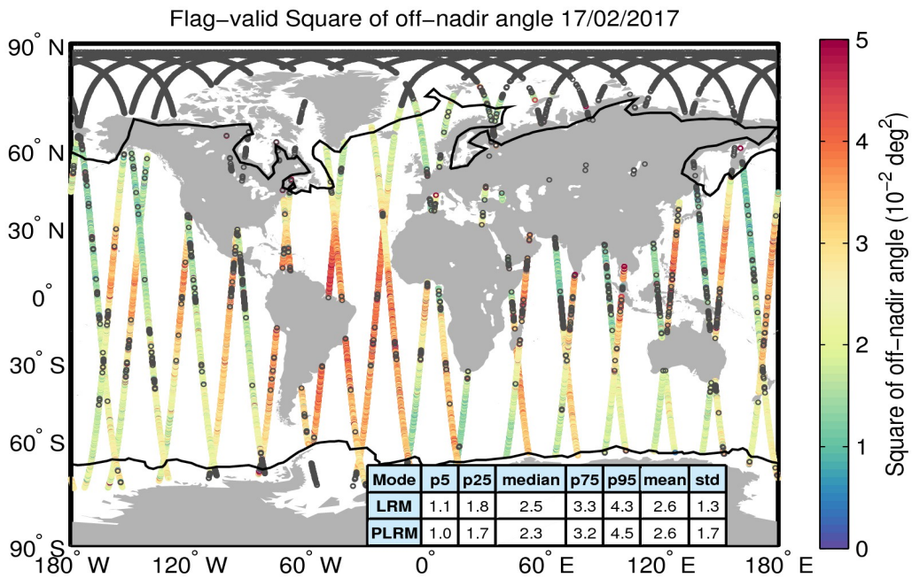
Figure 37. Geographical distribution of flag-valid mispointing data over oceans and lakes for 17/02/2017. The statistical values shown in the table refer to the mispointing in 10^{-2} \text{ deg}^2 and are calculated separately for LRM and PLRM regions. Measurements taken over polar polygons have been excluded from the computation of the statistical values. The black lines mark the outer limit of the Arctic and Antarctic polar polygons. Gray circles denote negative values.
