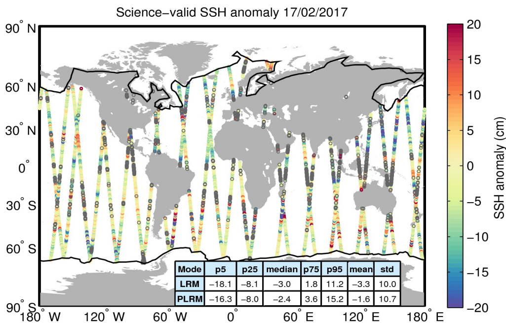
Figure 10. Geographical distribution of science-valid SSH anomaly data over oceans and lakes for 17/02/2017. The statistical values shown in the table refer to the SSH anomaly in cm and are calculated separately for LRM and PLRM regions. The black lines mark the outer limit of the Arctic and Antarctic polar polygons. Gray circles denote records that have been rejected based on the editing criteria described in Table 2.
