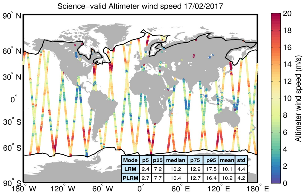
Figure 34. Geographical distribution of science-valid wind data over oceans and lakes for 17/02/2017. The statistical values shown in the table refer to the wind in m/s and are calculated separately for LRM and PLRM regions. The black lines mark the outer limit of the Arctic and Antarctic polar polygons. Gray circles denote records that have been rejected based on the editing criteria described in Table 5.
