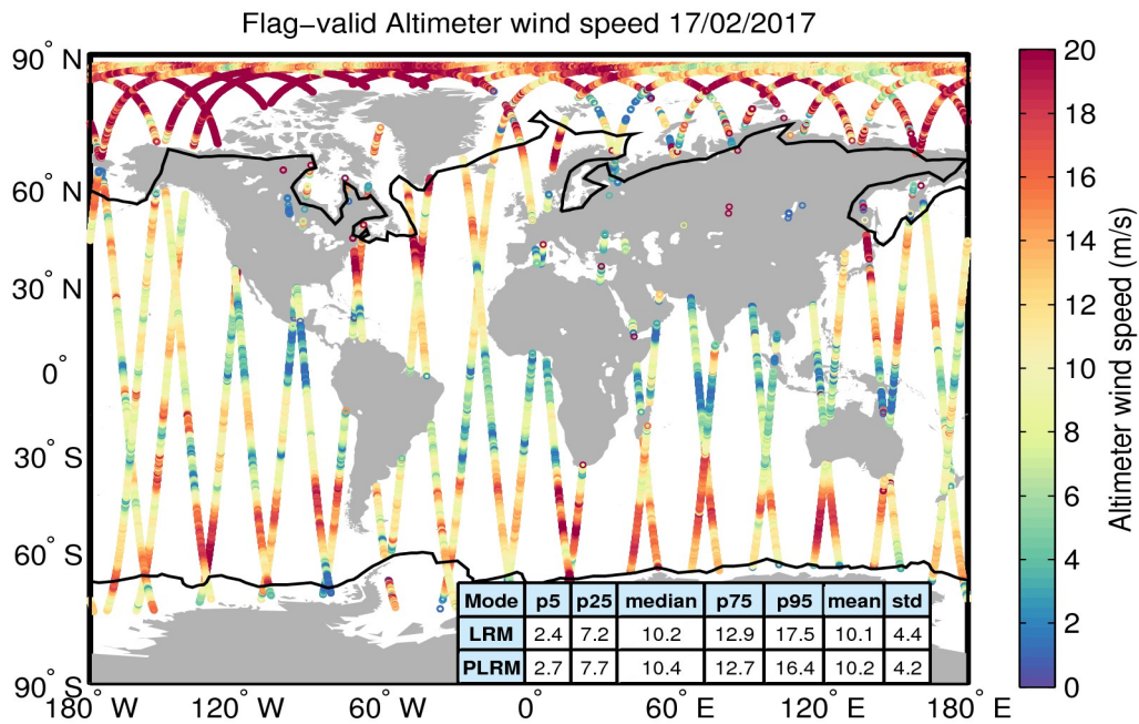
Figure 31. Geographical distribution of flag-valid wind data over oceans and lakes for 17/02/2017. The statistical values shown in the table refer to the wind in m/s and are calculated separately for LRM and PLRM regions. Measurements taken over polar polygons have been excluded from the computation of the statistical values. The black lines mark the outer limit of the Arctic and Antarctic polar polygons.
