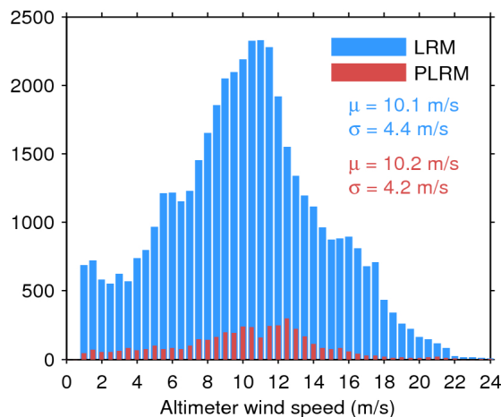
Figure 35. Histogram of science-valid wind over oceans and lakes for LRM (blue) and PLRM (red) for 17/02/2017. The mean ( \mu ) and standard deviation ( \sigma ) are also shown. Note that values larger than 24 m/s are excluded from the histogram for the sake of readability but not from the computation of \mu and \sigma .
