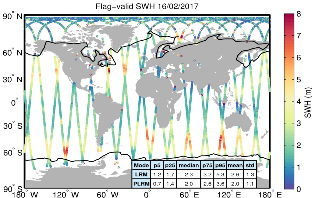
Figure 15. Geographical distribution of flag-valid SWH data over oceans and lakes for 16/02/2017. The statistical values shown in the table refer to the SWH in m and are calculated separately for LRM and PLRM regions. Measurements taken over polar polygons have been excluded from the computation of the statistical values. The black lines mark the outer limit of the Arctic and Antarctic polar polygons.
