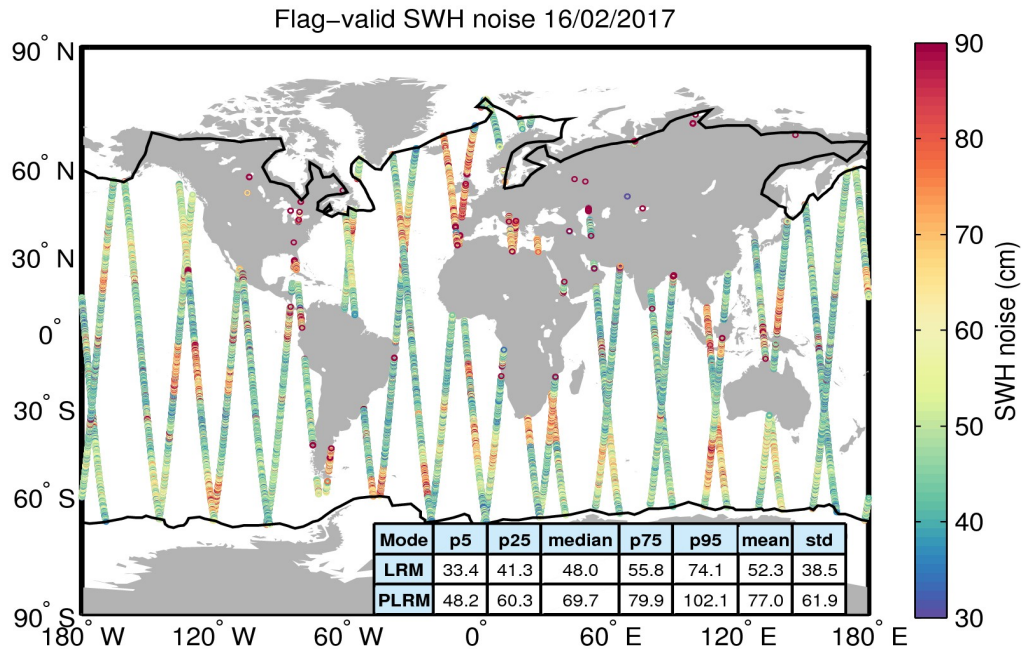
Figure 18. Geographical distribution of flag-valid 20-Hz SWH measurement noise over oceans and lakes for 16/02/2017. The statistical values shown in the table refer to the SWH noise and are calculated separately for LRM and PLRM regions. Measurements taken over polar polygons have been excluded from the computation of the statistical values. The black lines mark the outer limit of the Arctic and Antarctic polar polygons.
