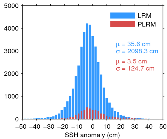
Figure 7. Histogram of flag-valid SSH anomaly over oceans and lakes for LRM (blue) and PLRM (red) for 16/02/2017. The mean ( \mu ) and standard deviation ( \sigma ) are also shown. Note that values outside [-50\ 50] cm are excluded from the histogram for the sake of readability but not from the computation of \mu and \sigma .
