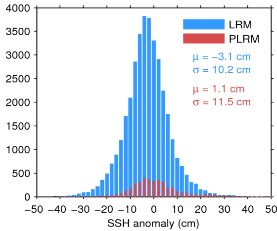
Figure 11. Histogram of science-valid SSH anomaly over oceans and lakes for LRM (blue) and PLRM (red) for 16/02/2017. The mean ( \mu ) and standard deviation ( \sigma ) are also shown. Note that values outside [-50 50] cm are excluded from the histogram for the sake of readability but not from the computation of \mu and \sigma .
