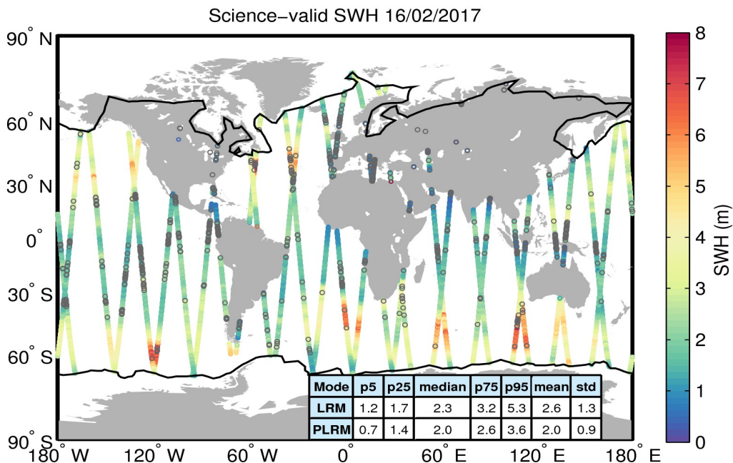
Figure 19. Geographical distribution of science-valid SWH data over oceans and lakes for 16/02/2017. The statistical values shown in the table refer to the SWH in m and are calculated separately for LRM and PLRM regions. The black lines mark the outer limit of the Arctic and Antarctic polar polygons. Gray circles denote records that have been rejected based on the editing criteria described in Table 3.
