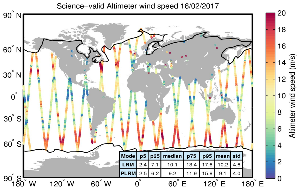
Figure 34. Geographical distribution of science-valid wind data over oceans and lakes for 16/02/2017. The statistical values shown in the table refer to the wind in m/s and are calculated separately for LRM and PLRM regions. The black lines mark the outer limit of the Arctic and Antarctic polar polygons. Gray circles denote records that have been rejected based on the editing criteria described in Table 5.
