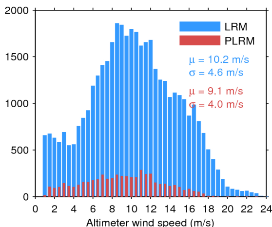
Figure 33. Histogram of flag-valid wind over oceans and lakes for LRM (blue) and PLRM (red) for 16/02/2017. The mean ( \mu ) and standard deviation ( \sigma ) are also shown. Note that values larger than 24 m/s are excluded from the histogram for the sake of readability but not from the computation of \mu and \sigma .
