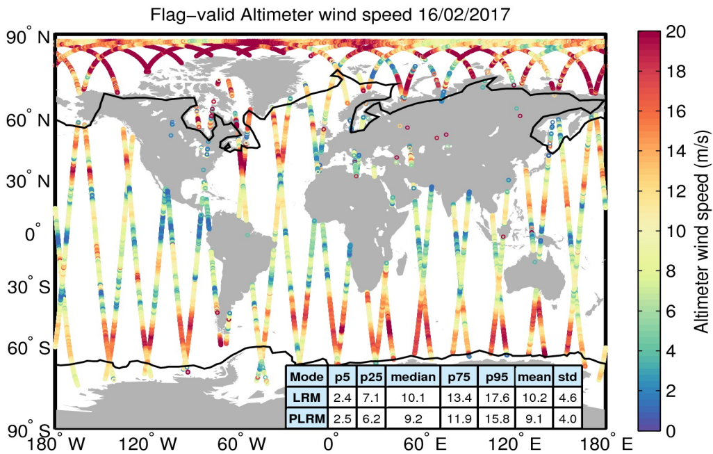
Figure 31. Geographical distribution of flag-valid wind data over oceans and lakes for 16/02/2017. The statistical values shown in the table refer to the wind in m/s and are calculated separately for LRM and PLRM regions. Measurements taken over polar polygons have been excluded from the computation of the statistical values. The black lines mark the outer limit of the Arctic and Antarctic polar polygons.
