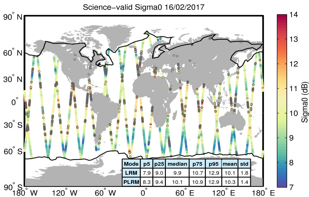
Figure 27. Geographical distribution of science-valid sigma0 data over oceans and lakes for 16/02/2017. The statistical values shown in the table refer to the sigma0 in dB and are calculated separately for LRM and PLRM regions. The black lines mark the outer limit of the Arctic and Antarctic polar polygons. Gray circles denote records that have been rejected based on the editing criteria described in Table 4.
