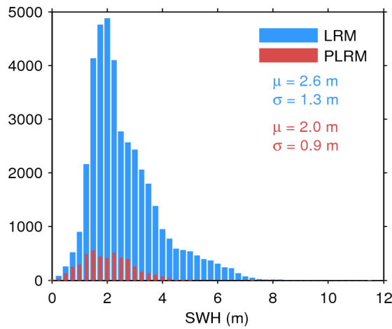
Figure 20. Histogram of science-valid SWH over oceans and lakes for LRM (blue) and PLRM (red) for 16/02/2017. The mean ( \mu ) and standard deviation ( \sigma ) are also shown. Note that values larger than 12 m are excluded from the histogram for the sake of readability but not from the computation of \mu and \sigma .
