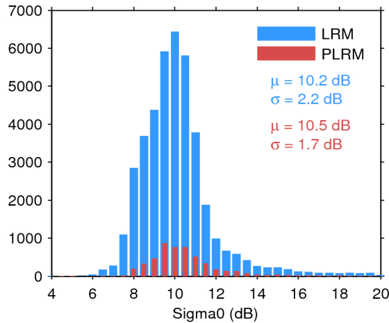
Figure 25. Histogram of flag-valid sigma0 over oceans and lakes for LRM (blue) and PLRM (red) for 16/02/2017. The mean ( \mu ) and standard deviation ( \sigma ) are also shown. Note that values outside [4 20] dB are excluded from the histogram for the sake of readability but not from the computation of \mu and \sigma .
