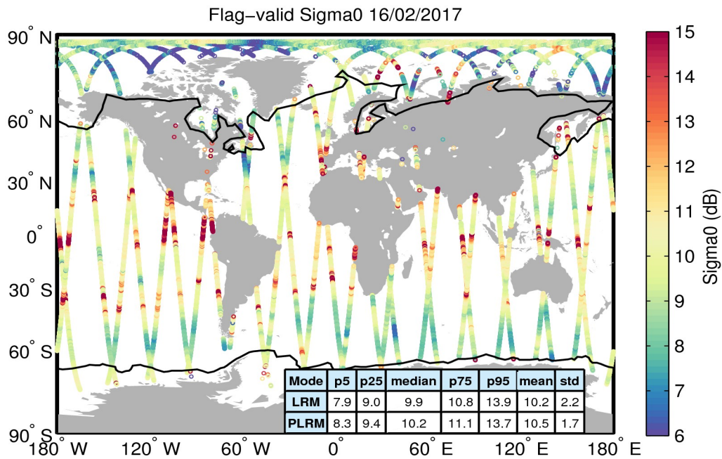
Figure 23. Geographical distribution of flag-valid sigma0 data over oceans and lakes for 16/02/2017. The statistical values shown in the table refer to the sigma0 in dB and are calculated separately for LRM and PLRM regions. Measurements taken over polar polygons have been excluded from the computation of the statistical values. The black lines mark the outer limit of the Arctic and Antarctic polar polygons.
