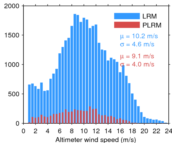
Figure 35. Histogram of science-valid wind over oceans and lakes for LRM (blue) and PLRM (red) for 16/02/2017. The mean ( \mu ) and standard deviation ( \sigma ) are also shown. Note that values larger than 24 m/s are excluded from the histogram for the sake of readability but not from the computation of \mu and \sigma .
