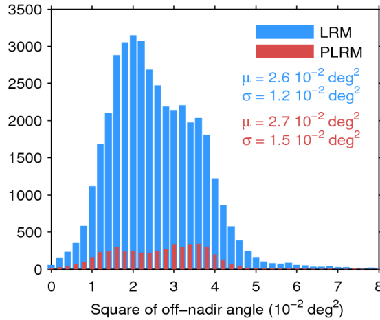
Figure 39. Histogram of flag-valid mispointing over oceans and lakes for LRM (blue) and PLRM (red) for 16/02/2017. Only positive values have been considered. The mean ( \mu ) and standard deviation ( \sigma ) are also shown. Note that values larger than 8 \cdot 10^{-2} \text{ deg}^2 are excluded from the histogram for the sake of readability but not from the computation of \mu and \sigma .
