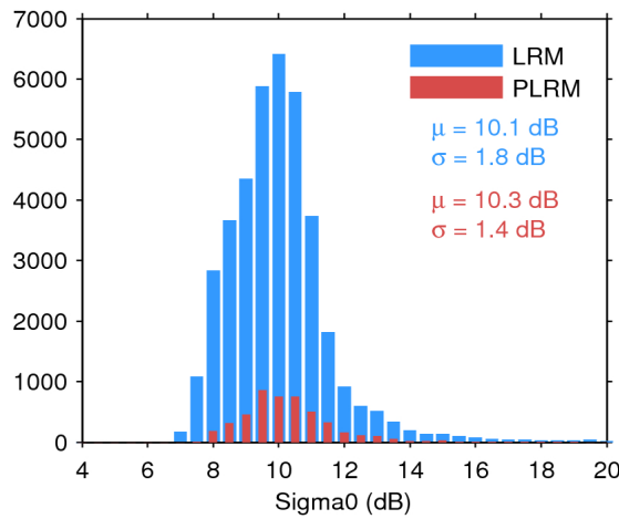
Figure 28. Histogram of science-valid sigma0 over oceans and lakes for LRM (blue) and PLRM (red) for 16/02/2017. The mean ( \mu ) and standard deviation ( \sigma ) are also shown. Note that values outside [4 20] dB are excluded from the histogram for the sake of readability but not from the computation of \mu and \sigma .
