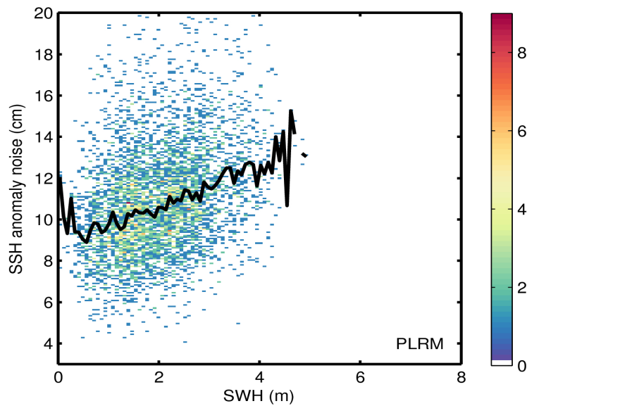
Figure 9. 2D histogram showing flag-valid SSH anomaly noise as a function of SWH for LRM (top) and PLRM (bottom) for 16/02/2017. The black line denotes the median SSH anomaly noise as a function of SWH.
