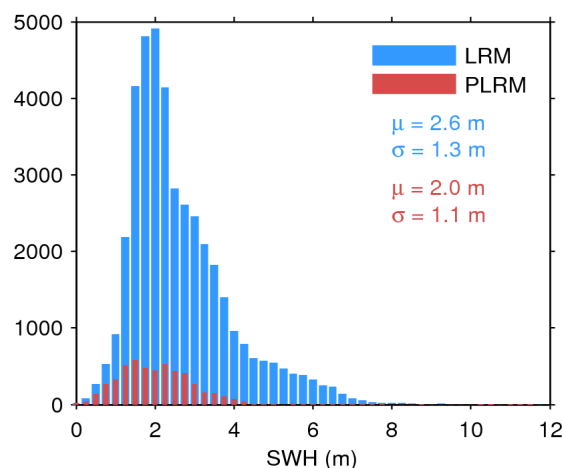
Figure 17. Histogram of flag-valid SWH over oceans and lakes for LRM (blue) and PLRM (red) for 16/02/2017. The mean ( \mu ) and standard deviation ( \sigma ) are also shown. Note that values larger than 12 m are excluded from the histogram for the sake of readability but not from the computation of \mu and \sigma .
