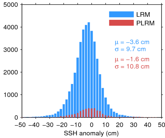
Figure 11. Histogram of science-valid SSH anomaly over oceans and lakes for LRM (blue) and PLRM (red) for 15/02/2017. The mean ( \mu ) and standard deviation ( \sigma ) are also shown. Note that values outside [-50 50] cm are excluded from the histogram for the sake of readability but not from the computation of \mu and \sigma .
