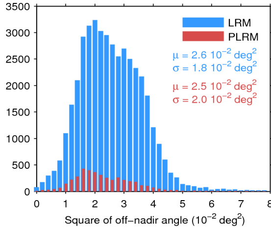
Figure 39. Histogram of flag-valid mispointing over oceans and lakes for LRM (blue) and PLRM (red) for 15/02/2017. Only positive values have been considered. The mean ( \mu ) and standard deviation ( \sigma ) are also shown. Note that values larger than 8 \cdot 10^{-2} \text{ deg}^2 are excluded from the histogram for the sake of readability but not from the computation of \mu and \sigma .
