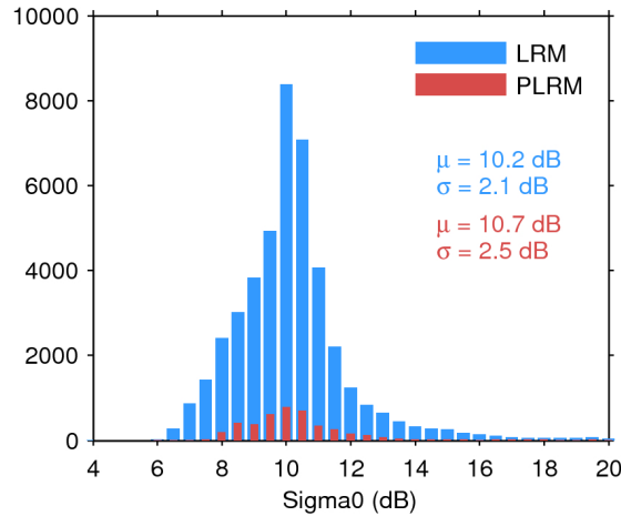
Figure 25. Histogram of flag-valid sigma0 over oceans and lakes for LRM (blue) and PLRM (red) for 15/02/2017. The mean ( \mu ) and standard deviation ( \sigma ) are also shown. Note that values outside [4 20] dB are excluded from the histogram for the sake of readability but not from the computation of \mu and \sigma .
