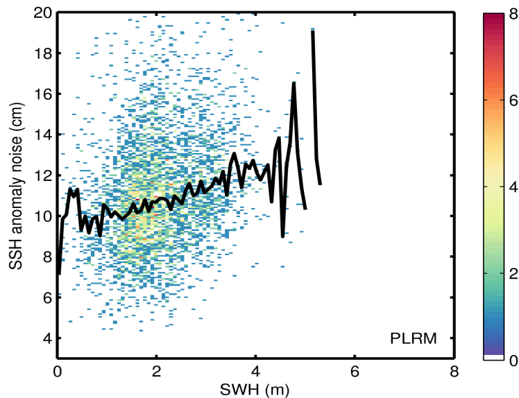
Figure 9. 2D histogram showing flag-valid SSH anomaly noise as a function of SWH for LRM (top) and PLRM (bottom) for 15/02/2017. The black line denotes the median SSH anomaly noise as a function of SWH.
