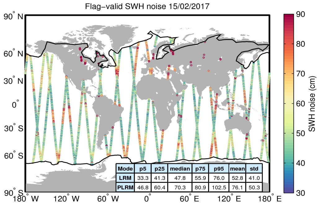
Figure 18. Geographical distribution of flag-valid 20-Hz SWH measurement noise over oceans and lakes for 15/02/2017. The statistical values shown in the table refer to the SWH noise and are calculated separately for LRM and PLRM regions. Measurements taken over polar polygons have been excluded from the computation of the statistical values. The black lines mark the outer limit of the Arctic and Antarctic polar polygons.
