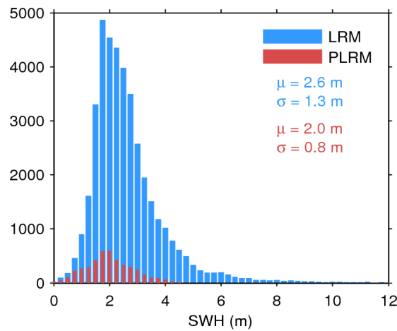
Figure 20. Histogram of science-valid SWH over oceans and lakes for LRM (blue) and PLRM (red) for 14/02/2017. The mean ( \mu ) and standard deviation ( \sigma ) are also shown. Note that values larger than 12 m are excluded from the histogram for the sake of readability but not from the computation of \mu and \sigma .
