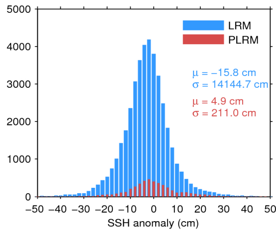
Figure 7. Histogram of flag-valid SSH anomaly over oceans and lakes for LRM (blue) and PLRM (red) for 14/02/2017. The mean ( \mu ) and standard deviation ( \sigma ) are also shown. Note that values outside [-50 50] cm are excluded from the histogram for the sake of readability but not from the computation of \mu and \sigma .
