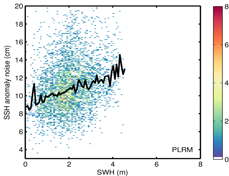
Figure 9. 2D histogram showing flag-valid SSH anomaly noise as a function of SWH for LRM (top) and PLRM (bottom) for 14/02/2017. The black line denotes the median SSH anomaly noise as a function of SWH.
