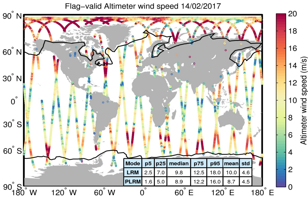
Figure 31. Geographical distribution of flag-valid wind data over oceans and lakes for 14/02/2017. The statistical values shown in the table refer to the wind in m/s and are calculated separately for LRM and PLRM regions. Measurements taken over polar polygons have been excluded from the computation of the statistical values. The black lines mark the outer limit of the Arctic and Antarctic polar polygons.
