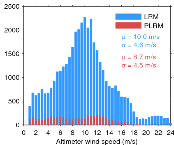
Figure 35. Histogram of science-valid wind over oceans and lakes for LRM (blue) and PLRM (red) for 14/02/2017. The mean ( \mu ) and standard deviation ( \sigma ) are also shown. Note that values larger than 24 m/s are excluded from the histogram for the sake of readability but not from the computation of \mu and \sigma .
