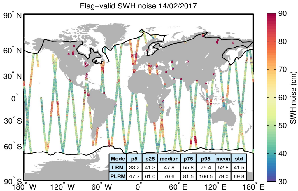
Figure 18. Geographical distribution of flag-valid 20-Hz SWH measurement noise over oceans and lakes for 14/02/2017. The statistical values shown in the table refer to the SWH noise and are calculated separately for LRM and PLRM regions. Measurements taken over polar polygons have been excluded from the computation of the statistical values. The black lines mark the outer limit of the Arctic and Antarctic polar polygons.
