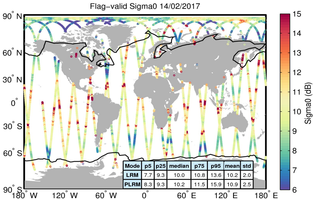
Figure 23. Geographical distribution of flag-valid sigma0 data over oceans and lakes for 14/02/2017. The statistical values shown in the table refer to the sigma0 in dB and are calculated separately for LRM and PLRM regions. Measurements taken over polar polygons have been excluded from the computation of the statistical values. The black lines mark the outer limit of the Arctic and Antarctic polar polygons.
