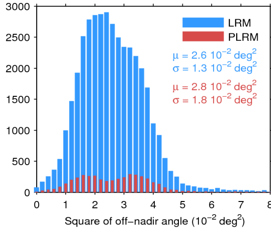
Figure 39. Histogram of flag-valid mispointing over oceans and lakes for LRM (blue) and PLRM (red) for 14/02/2017. Only positive values have been considered. The mean ( \mu ) and standard deviation ( \sigma ) are also shown. Note that values larger than 8 \cdot 10^{-2} \text{ deg}^2 are excluded from the histogram for the sake of readability but not from the computation of \mu and \sigma .
