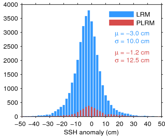
Figure 11. Histogram of science-valid SSH anomaly over oceans and lakes for LRM (blue) and PLRM (red) for 14/02/2017. The mean ( \mu ) and standard deviation ( \sigma ) are also shown. Note that values outside [-50\ 50] cm are excluded from the histogram for the sake of readability but not from the computation of \mu and \sigma .
