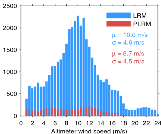
Figure 33. Histogram of flag-valid wind over oceans and lakes for LRM (blue) and PLRM (red) for 14/02/2017. The mean ( \mu ) and standard deviation ( \sigma ) are also shown. Note that values larger than 24 m/s are excluded from the histogram for the sake of readability but not from the computation of \mu and \sigma .
