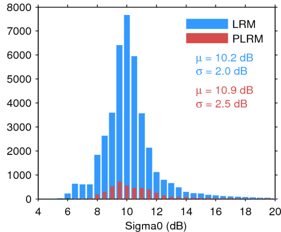
Figure 25. Histogram of flag-valid sigma0 over oceans and lakes for LRM (blue) and PLRM (red) for 14/02/2017. The mean ( \mu ) and standard deviation ( \sigma ) are also shown. Note that values outside [4 20] dB are excluded from the histogram for the sake of readability but not from the computation of \mu and \sigma .
