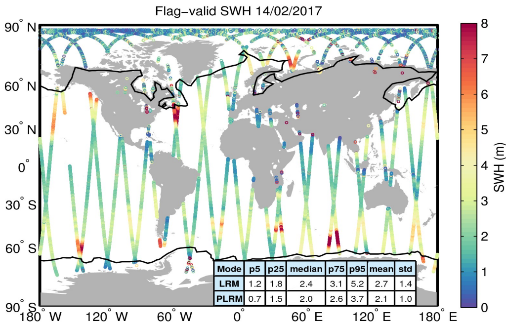
Figure 15. Geographical distribution of flag-valid SWH data over oceans and lakes for 14/02/2017. The statistical values shown in the table refer to the SWH in m and are calculated separately for LRM and PLRM regions. Measurements taken over polar polygons have been excluded from the computation of the statistical values. The black lines mark the outer limit of the Arctic and Antarctic polar polygons.
