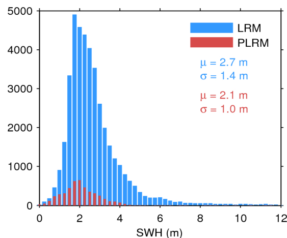
Figure 17. Histogram of flag-valid SWH over oceans and lakes for LRM (blue) and PLRM (red) for 14/02/2017. The mean ( \mu ) and standard deviation ( \sigma ) are also shown. Note that values larger than 12 m are excluded from the histogram for the sake of readability but not from the computation of \mu and \sigma .
