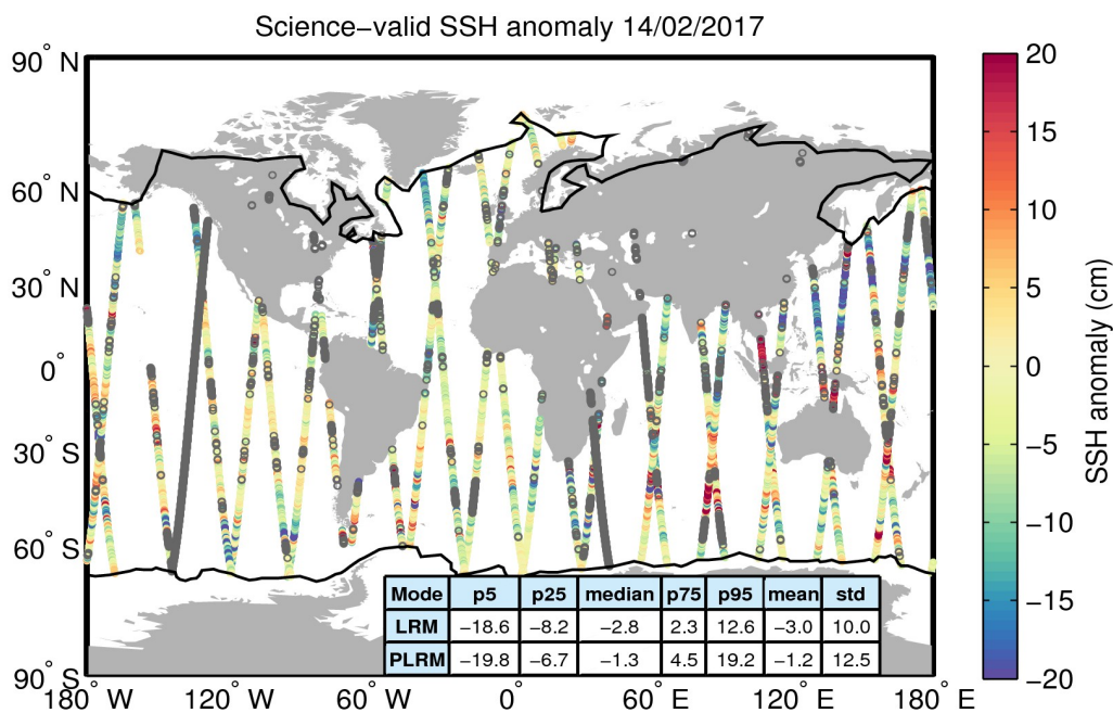
Figure 10. Geographical distribution of science-valid SSH anomaly data over oceans and lakes for 14/02/2017. The statistical values shown in the table refer to the SSH anomaly in cm and are calculated separately for LRM and PLRM regions. The black lines mark the outer limit of the Arctic and Antarctic polar polygons. Gray circles denote records that have been rejected based on the editing criteria described in Table 2.
