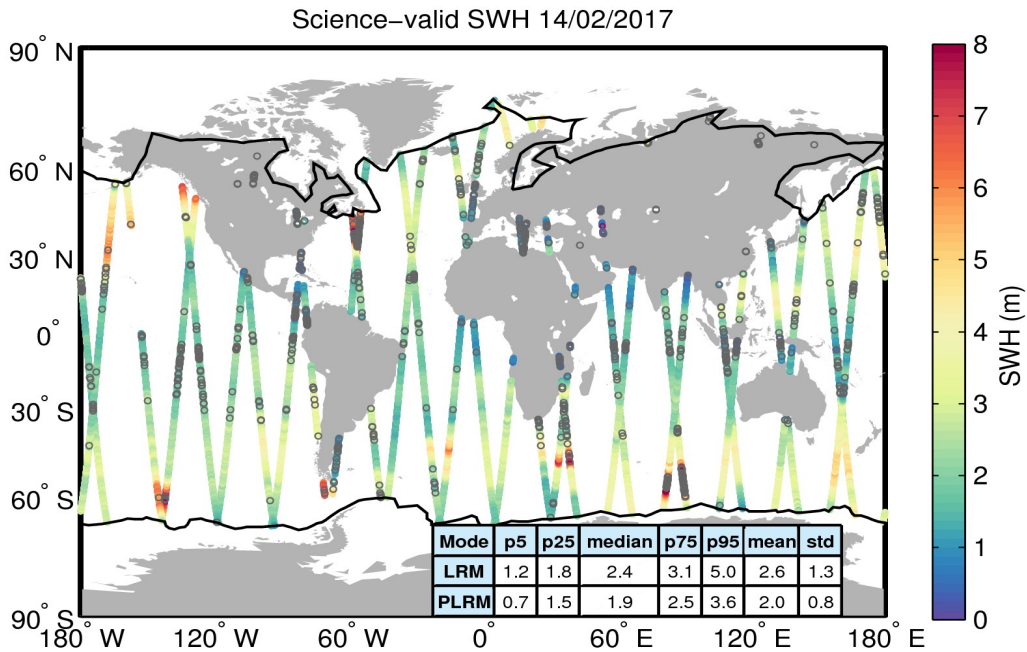
Figure 19. Geographical distribution of science-valid SWH data over oceans and lakes for 14/02/2017. The statistical values shown in the table refer to the SWH in m and are calculated separately for LRM and PLRM regions. The black lines mark the outer limit of the Arctic and Antarctic polar polygons. Gray circles denote records that have been rejected based on the editing criteria described in Table 3.
