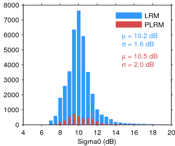
Figure 28. Histogram of science-valid sigma0 over oceans and lakes for LRM (blue) and PLRM (red) for 14/02/2017. The mean ( \mu ) and standard deviation ( \sigma ) are also shown. Note that values outside [4 20] dB are excluded from the histogram for the sake of readability but not from the computation of \mu and \sigma .
