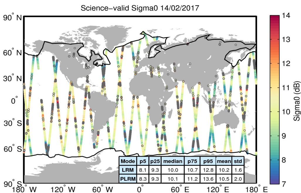
Figure 27. Geographical distribution of science-valid sigma0 data over oceans and lakes for 14/02/2017. The statistical values shown in the table refer to the sigma0 in dB and are calculated separately for LRM and PLRM regions. The black lines mark the outer limit of the Arctic and Antarctic polar polygons. Gray circles denote records that have been rejected based on the editing criteria described in Table 4.
