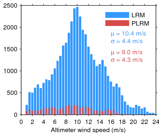
Figure 35. Histogram of science-valid wind over oceans and lakes for LRM (blue) and PLRM (red) for 13/02/2017. The mean ( \mu ) and standard deviation ( \sigma ) are also shown. Note that values larger than 24 m/s are excluded from the histogram for the sake of readability but not from the computation of \mu and \sigma .
