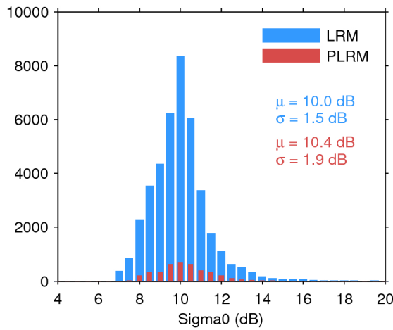
Figure 28. Histogram of science-valid sigma0 over oceans and lakes for LRM (blue) and PLRM (red) for 13/02/2017. The mean ( \mu ) and standard deviation ( \sigma ) are also shown. Note that values outside [4 20] dB are excluded from the histogram for the sake of readability but not from the computation of \mu and \sigma .
