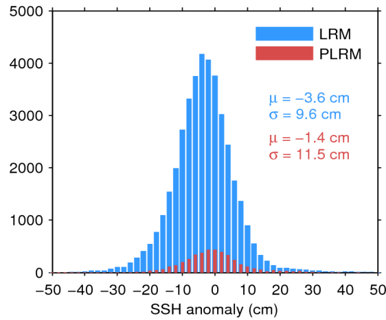
Figure 11. Histogram of science-valid SSH anomaly over oceans and lakes for LRM (blue) and PLRM (red) for 13/02/2017. The mean ( \mu ) and standard deviation ( \sigma ) are also shown. Note that values outside [-50 50] cm are excluded from the histogram for the sake of readability but not from the computation of \mu and \sigma .
