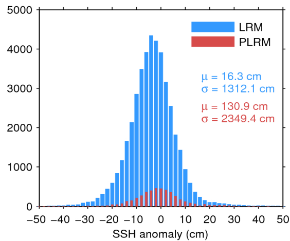
Figure 7. Histogram of flag-valid SSH anomaly over oceans and lakes for LRM (blue) and PLRM (red) for 13/02/2017. The mean ( \mu ) and standard deviation ( \sigma ) are also shown. Note that values outside [-50\ 50] cm are excluded from the histogram for the sake of readability but not from the computation of \mu and \sigma .
