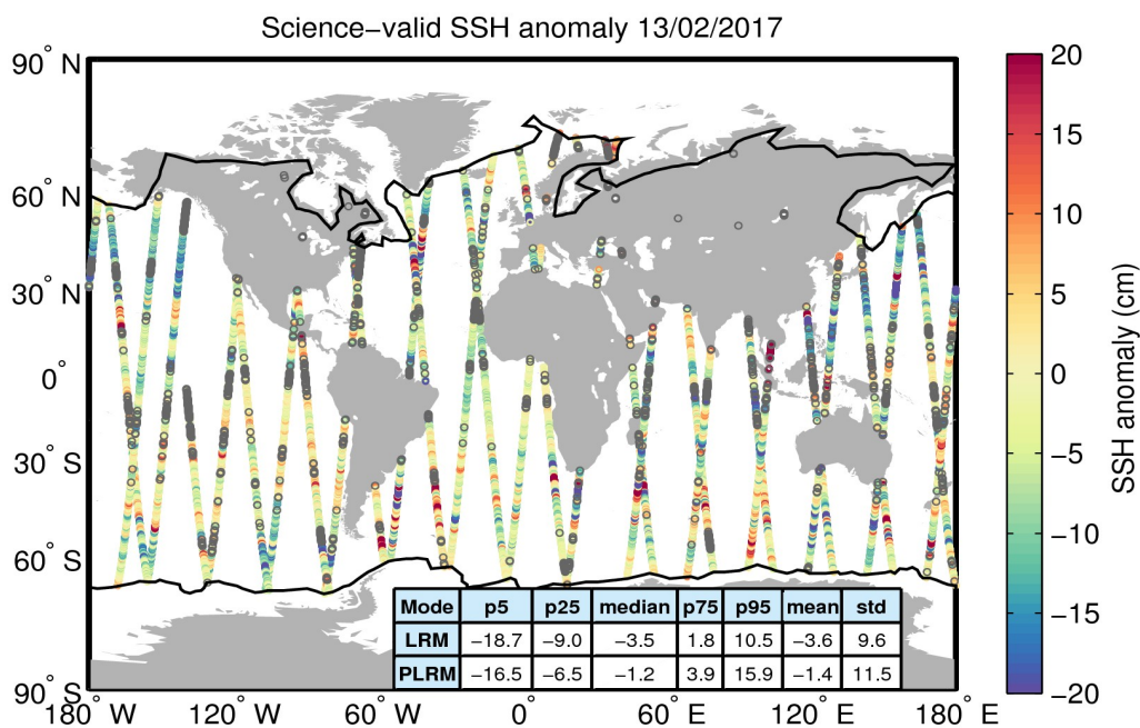
Figure 10. Geographical distribution of science-valid SSH anomaly data over oceans and lakes for 13/02/2017. The statistical values shown in the table refer to the SSH anomaly in cm and are calculated separately for LRM and PLRM regions. The black lines mark the outer limit of the Arctic and Antarctic polar polygons. Gray circles denote records that have been rejected based on the editing criteria described in Table 2.
