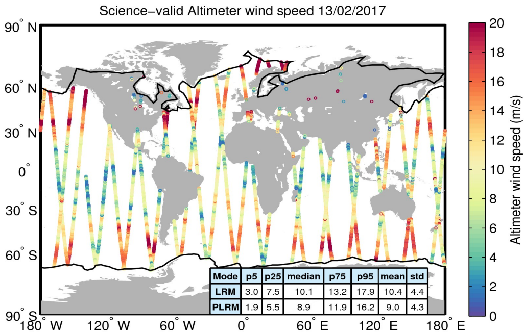
Figure 34. Geographical distribution of science-valid wind data over oceans and lakes for 13/02/2017. The statistical values shown in the table refer to the wind in m/s and are calculated separately for LRM and PLRM regions. The black lines mark the outer limit of the Arctic and Antarctic polar polygons. Gray circles denote records that have been rejected based on the editing criteria described in Table 5.
