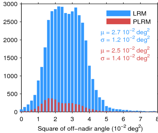
Figure 39. Histogram of flag-valid mispointing over oceans and lakes for LRM (blue) and PLRM (red) for 13/02/2017. Only positive values have been considered. The mean ( \mu ) and standard deviation ( \sigma ) are also shown. Note that values larger than 8 \cdot 10^{-2} \text{ deg}^2 are excluded from the histogram for the sake of readability but not from the computation of \mu and \sigma .
