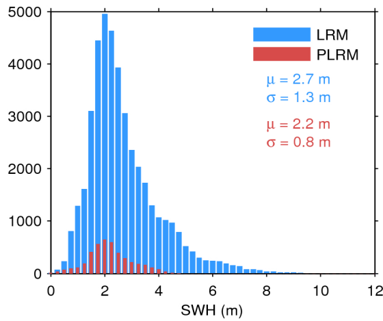
Figure 20. Histogram of science-valid SWH over oceans and lakes for LRM (blue) and PLRM (red) for 13/02/2017. The mean ( \mu ) and standard deviation ( \sigma ) are also shown. Note that values larger than 12 m are excluded from the histogram for the sake of readability but not from the computation of \mu and \sigma .
