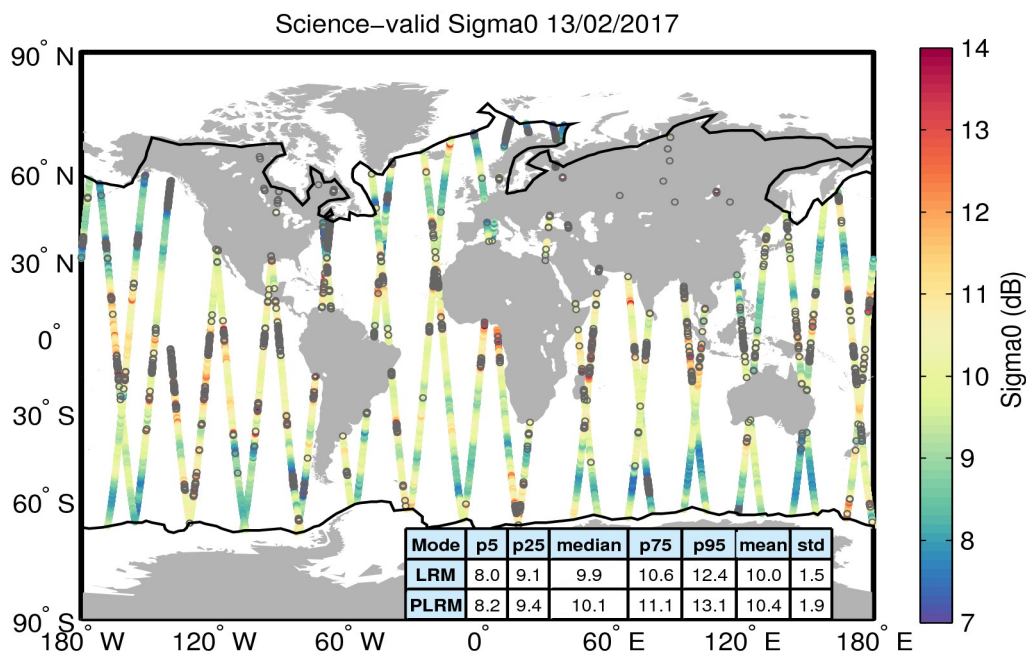
Figure 27. Geographical distribution of science-valid sigma0 data over oceans and lakes for 13/02/2017. The statistical values shown in the table refer to the sigma0 in dB and are calculated separately for LRM and PLRM regions. The black lines mark the outer limit of the Arctic and Antarctic polar polygons. Gray circles denote records that have been rejected based on the editing criteria described in Table 4.
