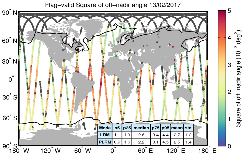
Figure 37. Geographical distribution of flag-valid mispointing data over oceans and lakes for 13/02/2017. The statistical values shown in the table refer to the mispointing in 10^{-2} \text{ deg}^2 and are calculated separately for LRM and PLRM regions. Measurements taken over polar polygons have been excluded from the computation of the statistical values. The black lines mark the outer limit of the Arctic and Antarctic polar polygons. Gray circles denote negative values.
