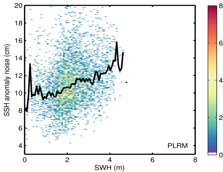
Figure 9. 2D histogram showing flag-valid SSH anomaly noise as a function of SWH for LRM (top) and PLRM (bottom) for 13/02/2017. The black line denotes the median SSH anomaly noise as a function of SWH.
