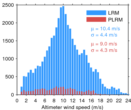
Figure 33. Histogram of flag-valid wind over oceans and lakes for LRM (blue) and PLRM (red) for 13/02/2017. The mean ( \mu ) and standard deviation ( \sigma ) are also shown. Note that values larger than 24 m/s are excluded from the histogram for the sake of readability but not from the computation of \mu and \sigma .
