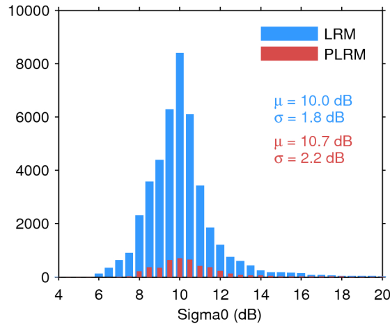
Figure 25. Histogram of flag-valid sigma0 over oceans and lakes for LRM (blue) and PLRM (red) for 13/02/2017. The mean ( \mu ) and standard deviation ( \sigma ) are also shown. Note that values outside [4 20] dB are excluded from the histogram for the sake of readability but not from the computation of \mu and \sigma .
