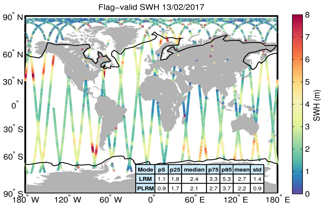
Figure 15. Geographical distribution of flag-valid SWH data over oceans and lakes for 13/02/2017. The statistical values shown in the table refer to the SWH in m and are calculated separately for LRM and PLRM regions. Measurements taken over polar polygons have been excluded from the computation of the statistical values. The black lines mark the outer limit of the Arctic and Antarctic polar polygons.
