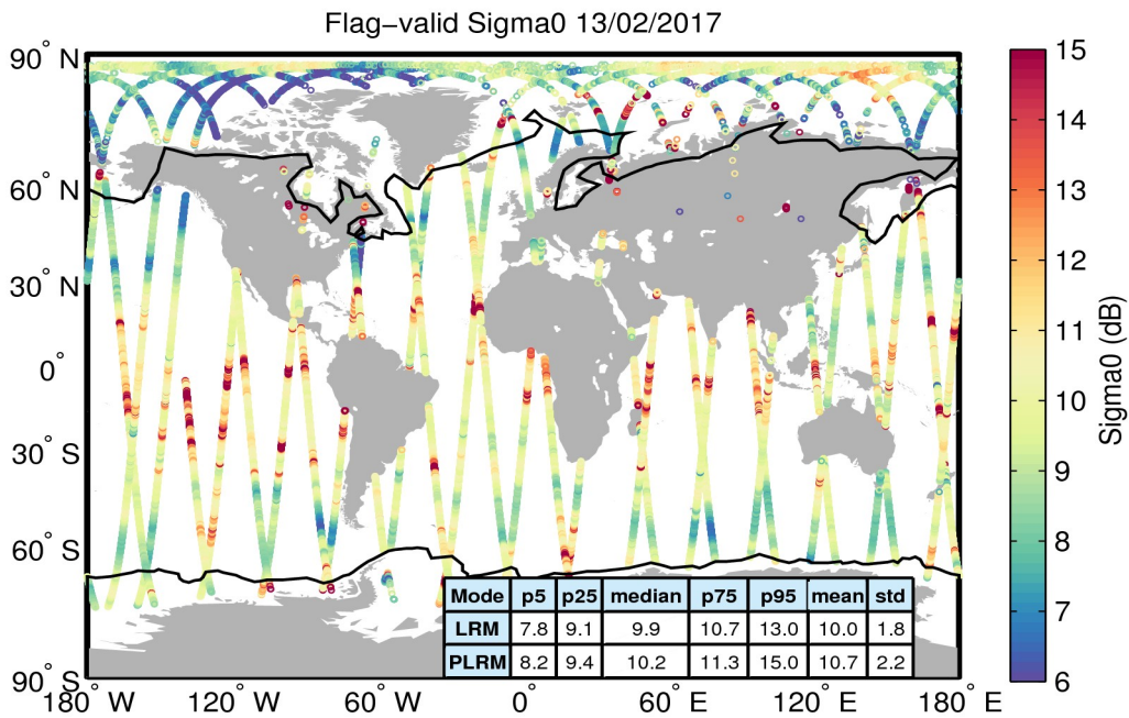
Figure 23. Geographical distribution of flag-valid sigma0 data over oceans and lakes for 13/02/2017. The statistical values shown in the table refer to the sigma0 in dB and are calculated separately for LRM and PLRM regions. Measurements taken over polar polygons have been excluded from the computation of the statistical values. The black lines mark the outer limit of the Arctic and Antarctic polar polygons.
