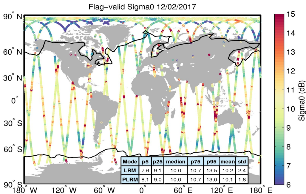
Figure 23. Geographical distribution of flag-valid sigma0 data over oceans and lakes for 12/02/2017. The statistical values shown in the table refer to the sigma0 in dB and are calculated separately for LRM and PLRM regions. Measurements taken over polar polygons have been excluded from the computation of the statistical values. The black lines mark the outer limit of the Arctic and Antarctic polar polygons.
