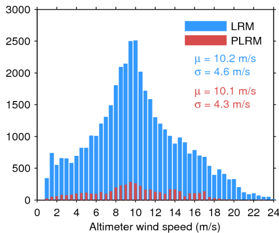
Figure 35. Histogram of science-valid wind over oceans and lakes for LRM (blue) and PLRM (red) for 12/02/2017. The mean ( \mu ) and standard deviation ( \sigma ) are also shown. Note that values larger than 24 m/s are excluded from the histogram for the sake of readability but not from the computation of \mu and \sigma .
