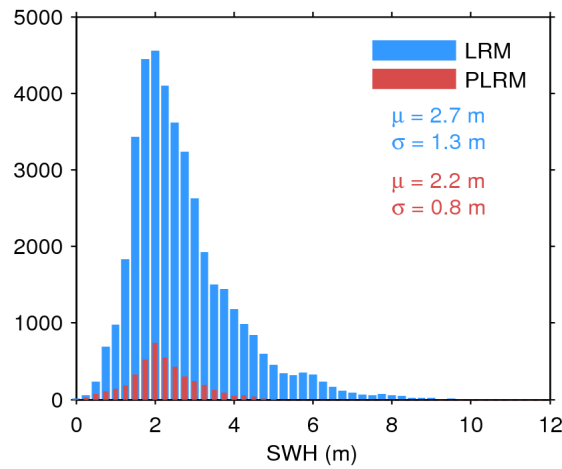
Figure 20. Histogram of science-valid SWH over oceans and lakes for LRM (blue) and PLRM (red) for 12/02/2017. The mean ( \mu ) and standard deviation ( \sigma ) are also shown. Note that values larger than 12 m are excluded from the histogram for the sake of readability but not from the computation of \mu and \sigma .
