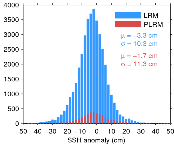
Figure 11. Histogram of science-valid SSH anomaly over oceans and lakes for LRM (blue) and PLRM (red) for 12/02/2017. The mean ( \mu ) and standard deviation ( \sigma ) are also shown. Note that values outside [-50\ 50] cm are excluded from the histogram for the sake of readability but not from the computation of \mu and \sigma .
