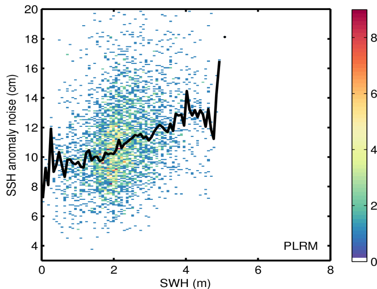
Figure 9. 2D histogram showing flag-valid SSH anomaly noise as a function of SWH for LRM (top) and PLRM (bottom) for 12/02/2017. The black line denotes the median SSH anomaly noise as a function of SWH.
