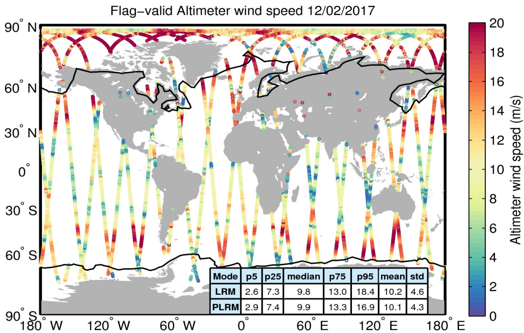
Figure 31. Geographical distribution of flag-valid wind data over oceans and lakes for 12/02/2017. The statistical values shown in the table refer to the wind in m/s and are calculated separately for LRM and PLRM regions. Measurements taken over polar polygons have been excluded from the computation of the statistical values. The black lines mark the outer limit of the Arctic and Antarctic polar polygons.
