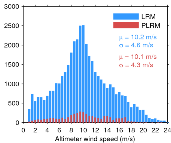
Figure 33. Histogram of flag-valid wind over oceans and lakes for LRM (blue) and PLRM (red) for 12/02/2017. The mean ( \mu ) and standard deviation ( \sigma ) are also shown. Note that values larger than 24 m/s are excluded from the histogram for the sake of readability but not from the computation of \mu and \sigma .
