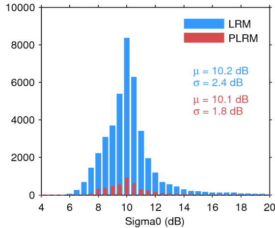
Figure 25. Histogram of flag-valid sigma0 over oceans and lakes for LRM (blue) and PLRM (red) for 12/02/2017. The mean ( \mu ) and standard deviation ( \sigma ) are also shown. Note that values outside [4 20] dB are excluded from the histogram for the sake of readability but not from the computation of \mu and \sigma .
