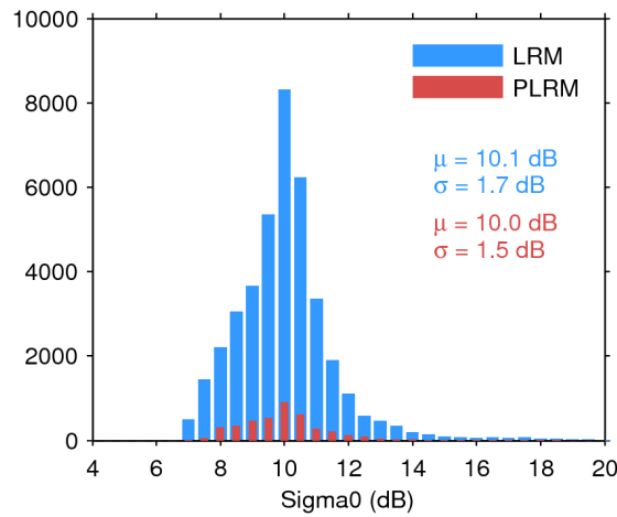
Figure 28. Histogram of science-valid sigma0 over oceans and lakes for LRM (blue) and PLRM (red) for 12/02/2017. The mean ( \mu ) and standard deviation ( \sigma ) are also shown. Note that values outside [4 20] dB are excluded from the histogram for the sake of readability but not from the computation of \mu and \sigma .
