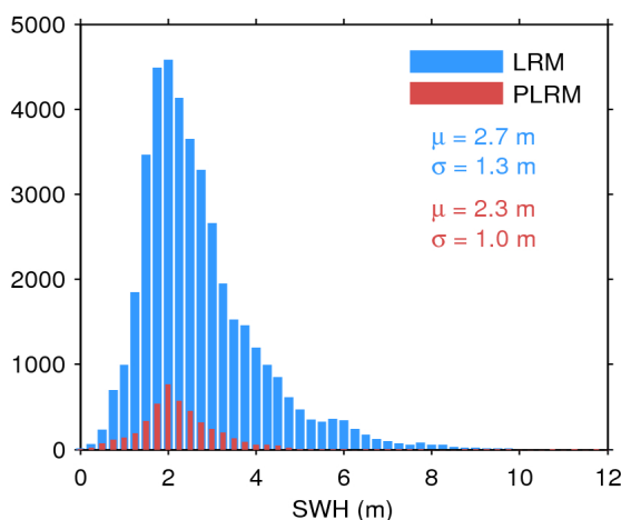
Figure 17. Histogram of flag-valid SWH over oceans and lakes for LRM (blue) and PLRM (red) for 12/02/2017. The mean ( \mu ) and standard deviation ( \sigma ) are also shown. Note that values larger than 12 m are excluded from the histogram for the sake of readability but not from the computation of \mu and \sigma .
