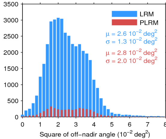
Figure 39. Histogram of flag-valid mispointing over oceans and lakes for LRM (blue) and PLRM (red) for 12/02/2017. Only positive values have been considered. The mean ( \mu ) and standard deviation ( \sigma ) are also shown. Note that values larger than 8 \cdot 10^{-2} \text{ deg}^2 are excluded from the histogram for the sake of readability but not from the computation of \mu and \sigma .
