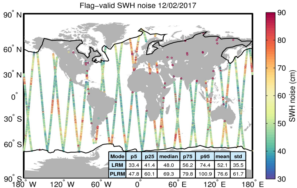
Figure 18. Geographical distribution of flag-valid 20-Hz SWH measurement noise over oceans and lakes for 12/02/2017. The statistical values shown in the table refer to the SWH noise and are calculated separately for LRM and PLRM regions. Measurements taken over polar polygons have been excluded from the computation of the statistical values. The black lines mark the outer limit of the Arctic and Antarctic polar polygons.
