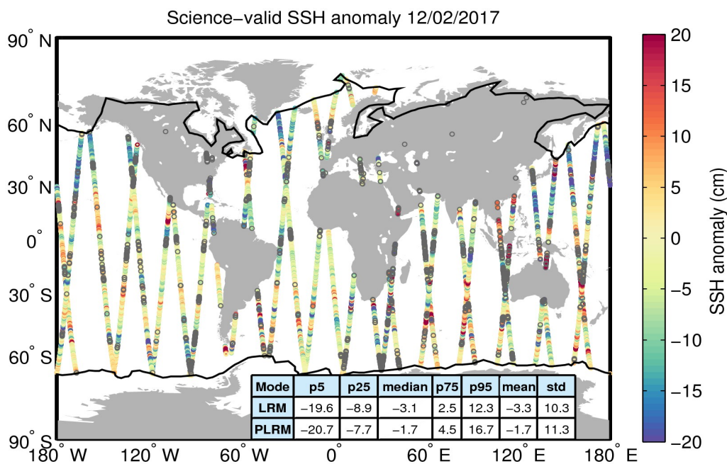
Figure 10. Geographical distribution of science-valid SSH anomaly data over oceans and lakes for 12/02/2017. The statistical values shown in the table refer to the SSH anomaly in cm and are calculated separately for LRM and PLRM regions. The black lines mark the outer limit of the Arctic and Antarctic polar polygons. Gray circles denote records that have been rejected based on the editing criteria described in Table 2.
