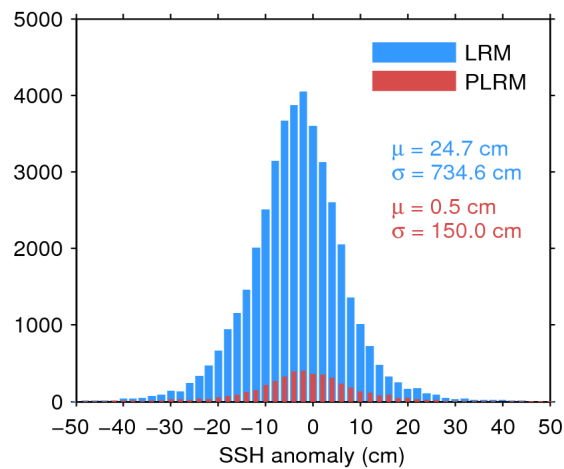
Figure 7. Histogram of flag-valid SSH anomaly over oceans and lakes for LRM (blue) and PLRM (red) for 12/02/2017. The mean ( \mu ) and standard deviation ( \sigma ) are also shown. Note that values outside [-50 \ 50] cm are excluded from the histogram for the sake of readability but not from the computation of \mu and \sigma .
