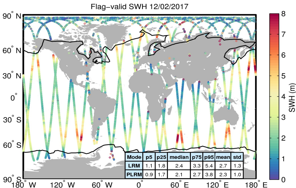
Figure 15. Geographical distribution of flag-valid SWH data over oceans and lakes for 12/02/2017. The statistical values shown in the table refer to the SWH in m and are calculated separately for LRM and PLRM regions. Measurements taken over polar polygons have been excluded from the computation of the statistical values. The black lines mark the outer limit of the Arctic and Antarctic polar polygons.
